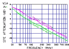
Figure 3-4. Normalized Site Attenuation Curves (H&V)
