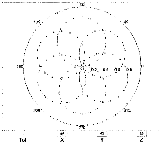
f=600 MHz,TEM
