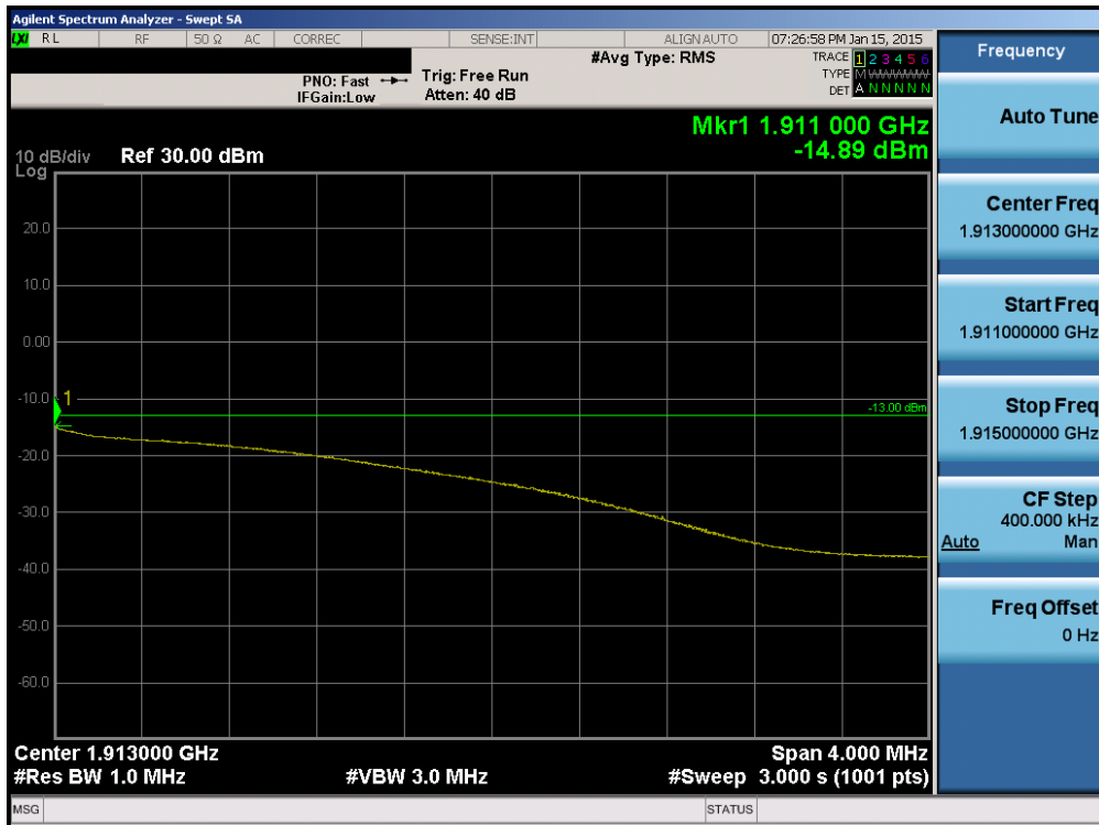
Plot 6-47. 4MHz Span Plot (PCS WCDMA Mode – Ch. 9538)
