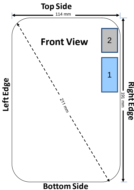
Figure 1 – DUT Antenna Locations
