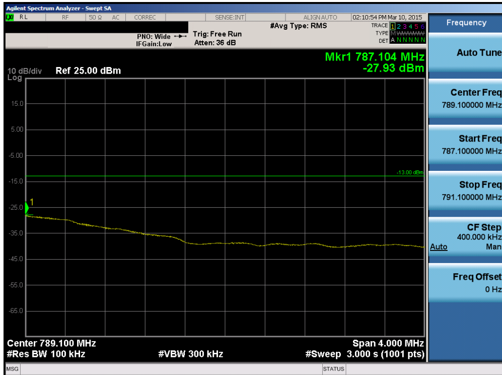
Plot 6-42. Upper Extended Band Edge Plot (Band 13 – 10.0MHz QPSK – RB Size 50)
