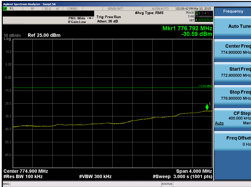
Plot 6-40. Lower Extended Band Edge Plot (Band 13 – 10.0MHz QPSK – RB Size 50)
