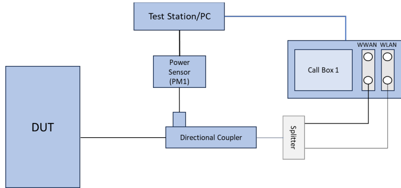
(g) Appendix A - Test Setup 11 Figure 5-1 Conducted power measurement setup
