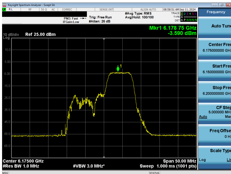
Plot 7-57. Power Spectral Density Plot MIMO ANT1 (20MHz 802.11be (52+26 Tones) (UNII Band 5) – Ch. 45) - LPI
