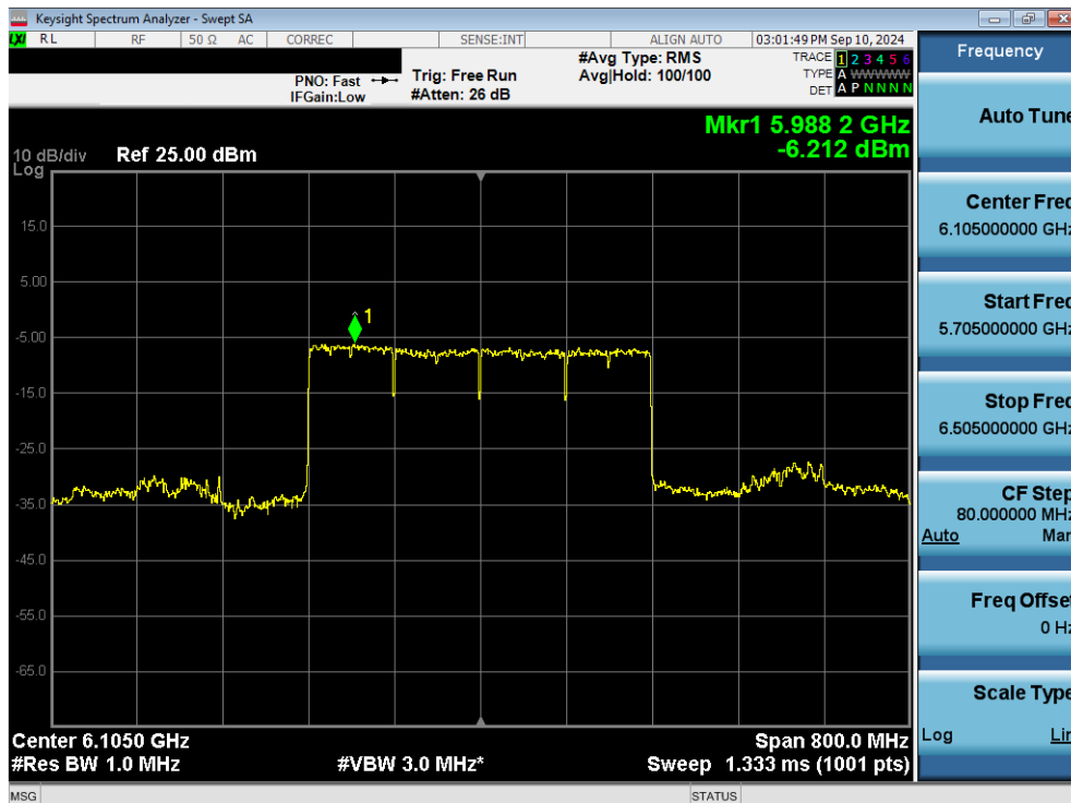
Plot 7-72. Power Spectral Density Plot MIMO ANT1 (320MHz 802.11ax/be (Full Tones) (UNII Band 5) – Ch. 31) - LPI/SP
