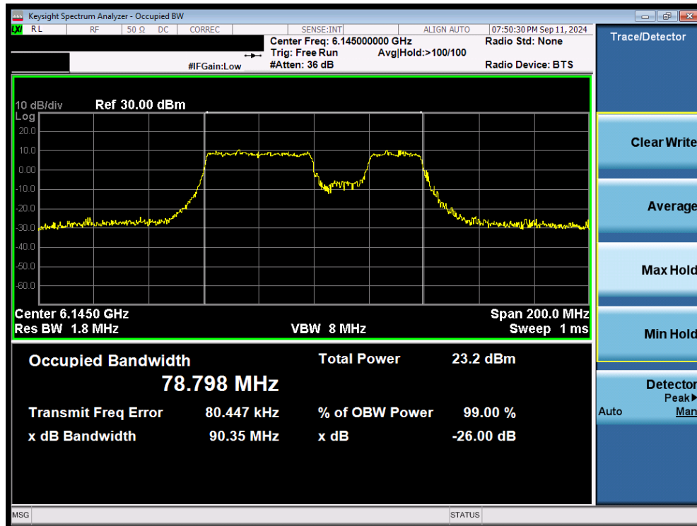
Plot 7-36. 26dB Bandwidth Plot MIMO ANT2 (80MHz 802.11be (484+242 Tones) (UNII Band 5) – Ch. 39) LPI/SP
