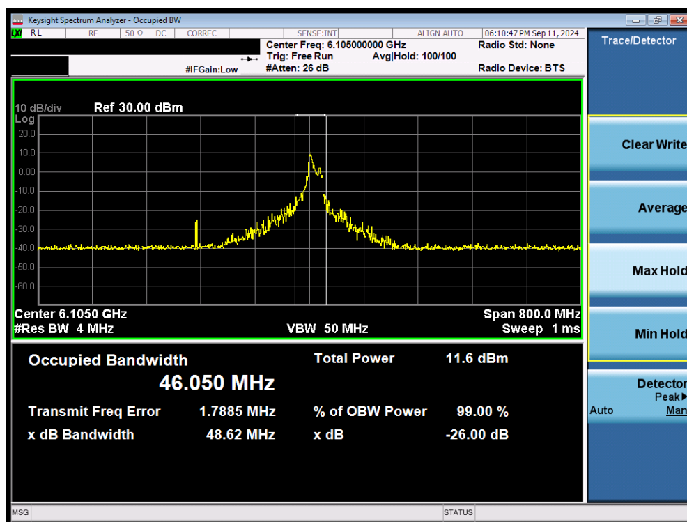
Plot 7-34. 26dB Bandwidth Plot MIMO ANT2 (320MHz 802.11ax/be (26 Tones) (UNII Band 5) – Ch. 31) - LPI
