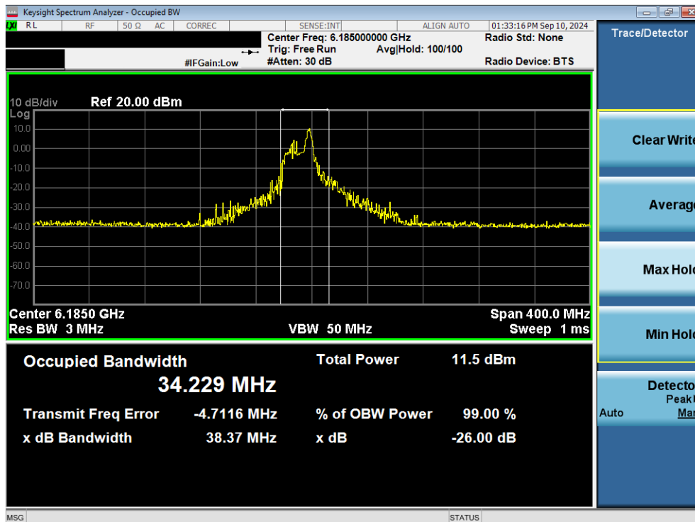
Plot 7-11. 26dB Bandwidth Plot MIMO ANT1 (160MHz 802.11ax/be (26 Tones) (UNII Band 5) – Ch. 47) - LPI
