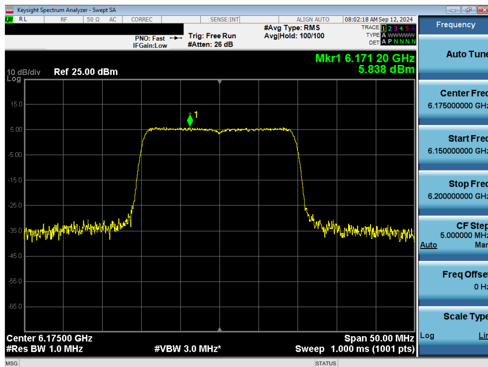
Plot 7-73. Power Spectral Density Plot MIMO ANT1 (20MHz 802.11ax/be (Full Tones) (UNII Band 5) – Ch. 45) - SP
