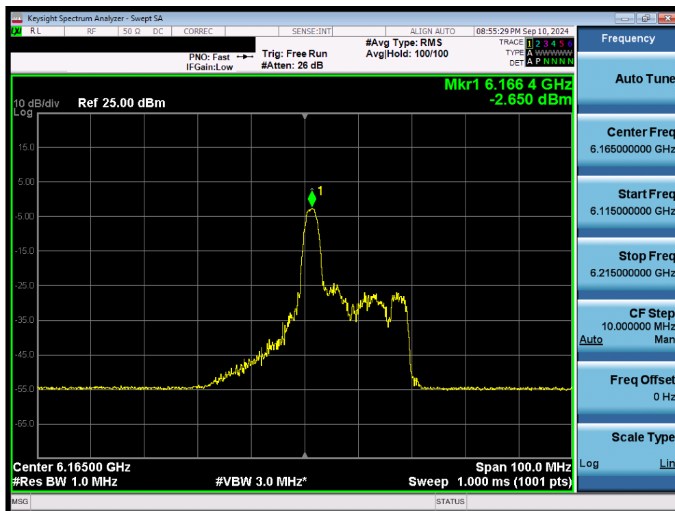
Plot 7-77. Power Spectral Density Plot MIMO ANT2 (40MHz 802.11ax/be (26 Tones) (UNII Band 5) – Ch. 43) - LPI
