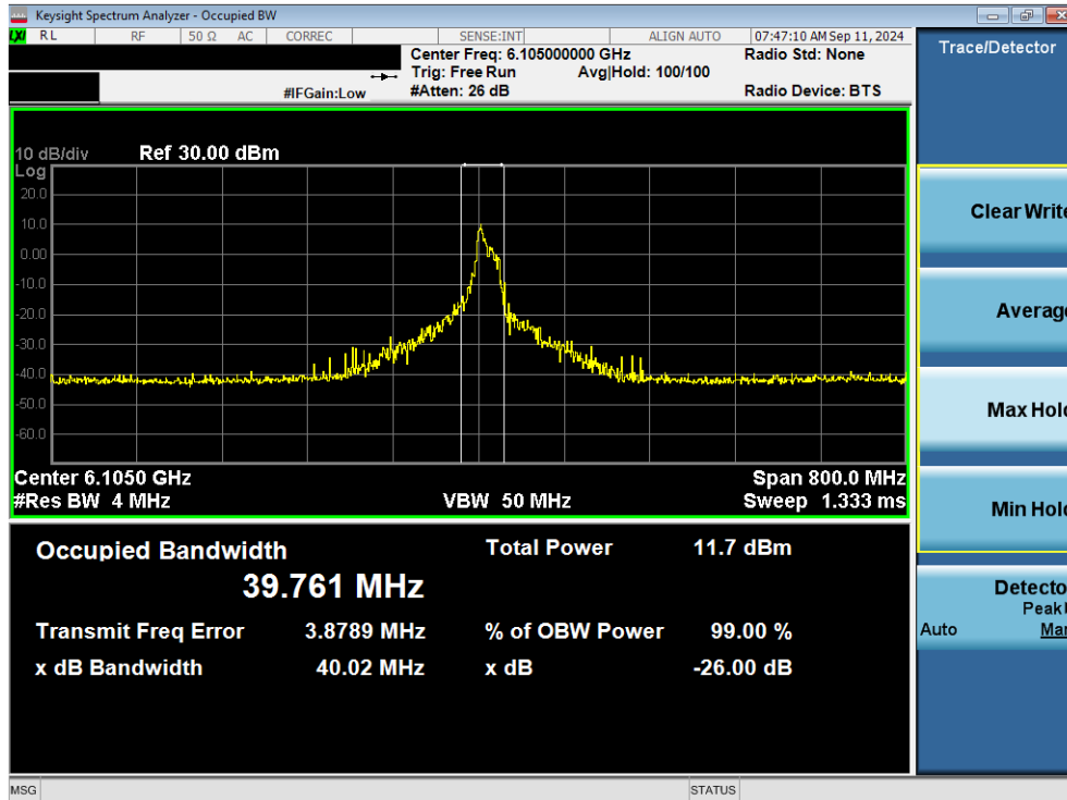
Plot 7-12. 26dB Bandwidth Plot MIMO ANT1 (320MHz 802.11ax/be (26 Tones) (UNII Band 5) – Ch. 31) - LPI
