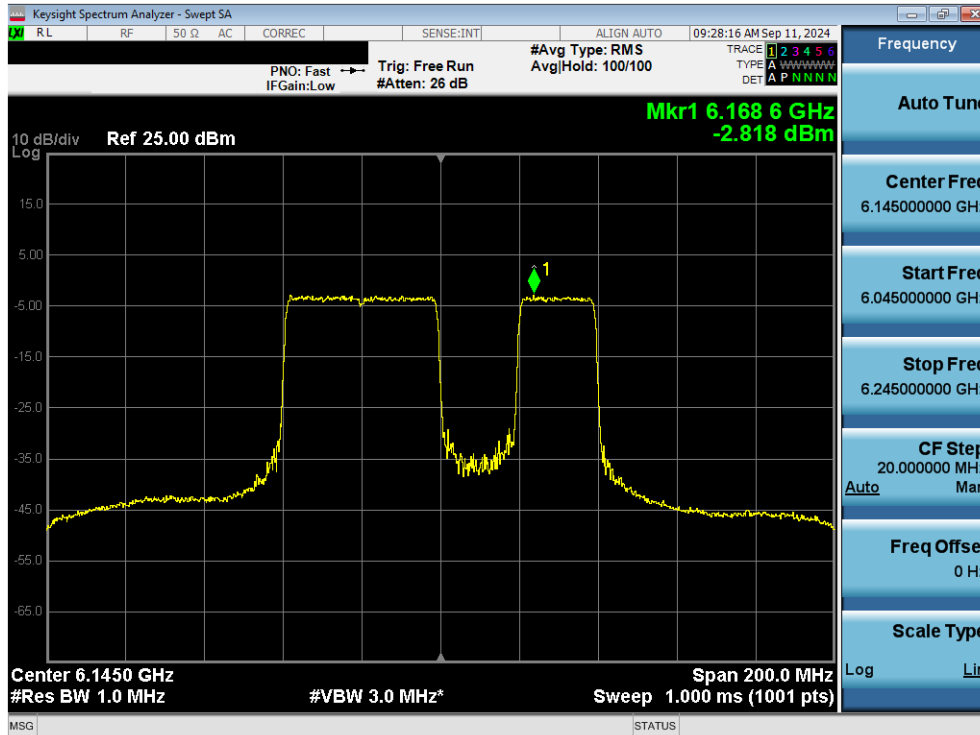
Plot 7-58. Power Spectral Density Plot MIMO ANT1 (80MHz 802.11be (484+242 Tones) (UNII Band 5) – Ch. 39) LPI
