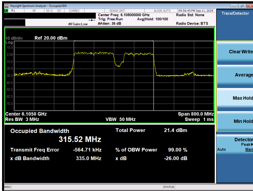
Plot 7-38. 26dB Bandwidth Plot MIMO ANT2 (320MHz 802.11be (3*996+484 Tones) (UNII Band 5) – Ch. 31) LPI/SP
