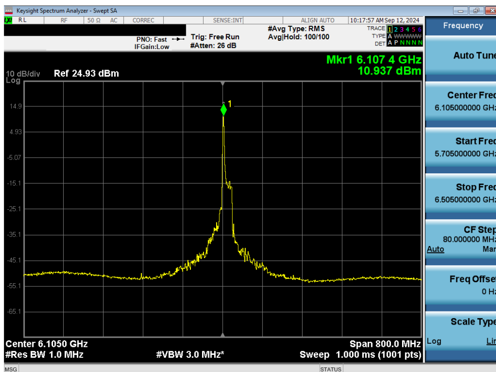
Plot 7-65. Power Spectral Density Plot MIMO ANT1 (320MHz 802.11ax/be (26 Tones) (UNII Band 5) – Ch. 31) - SP
