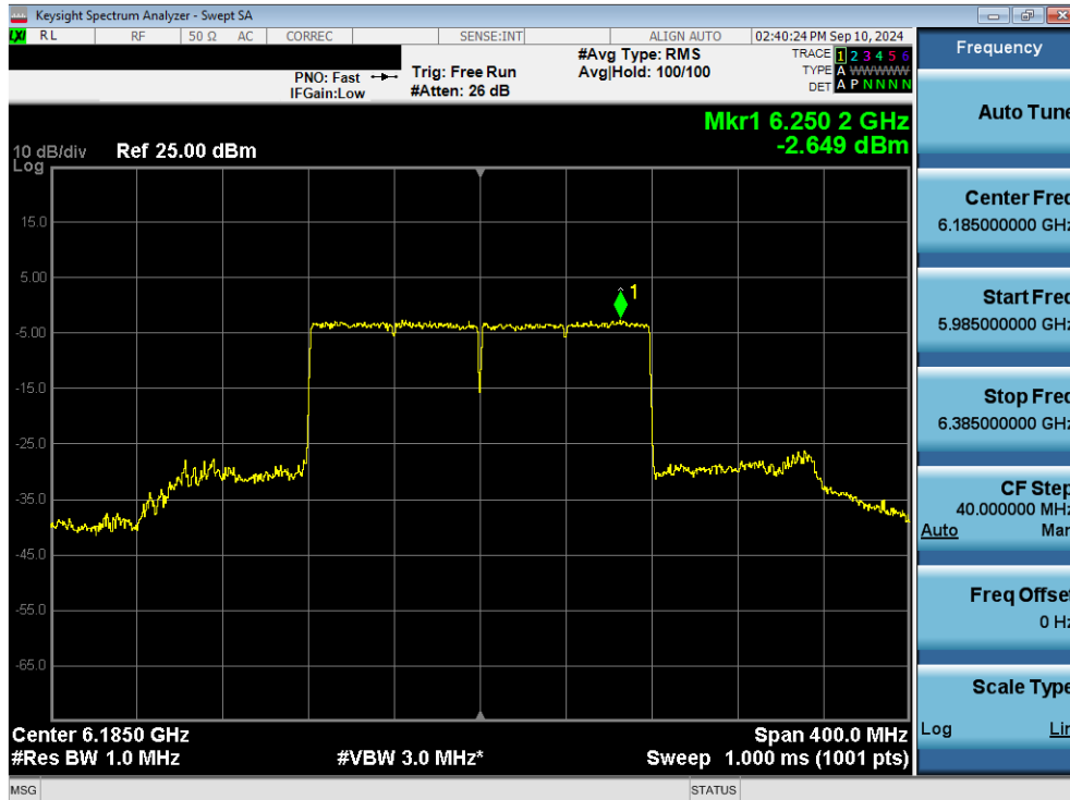
Plot 7-71. Power Spectral Density Plot MIMO ANT1 (160MHz 802.11ax/be (Full Tones) (UNII Band 5) – Ch. 47) - LPI/SP
