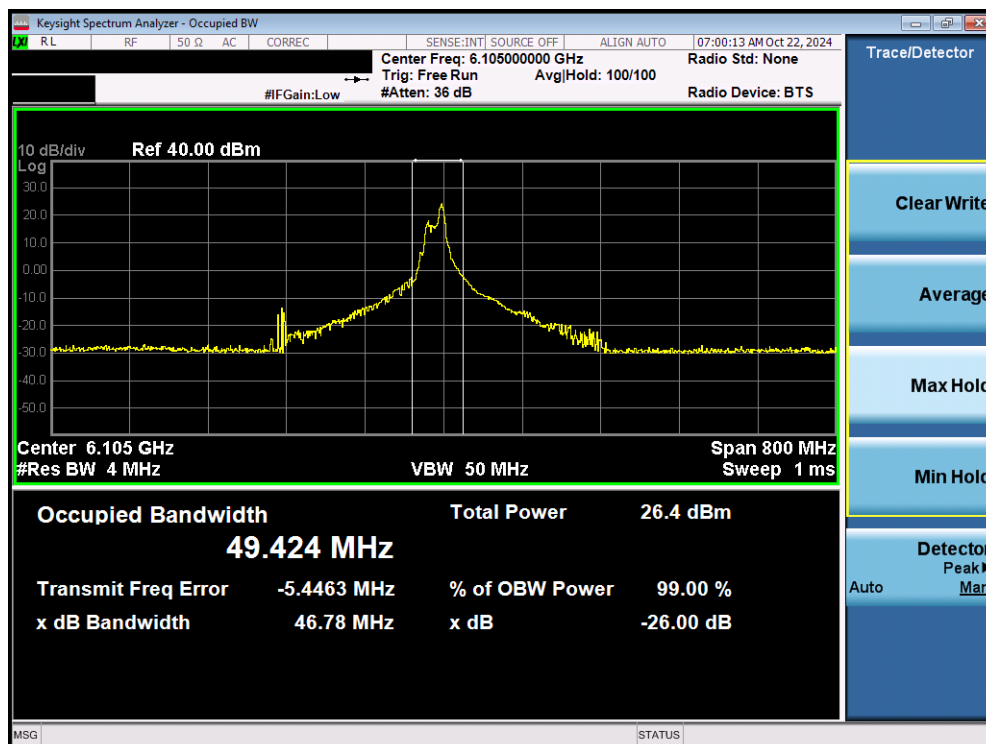
Plot 7-21. 26dB Bandwidth Plot MIMO ANT1 (320MHz 802.11ax/be (26 Tones) (UNII Band 5) – Ch. 31) - SP
