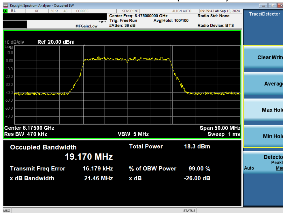
Plot 7-23. 26dB Bandwidth Plot MIMO ANT1 (20MHz 802.11ax/be (Full Tones) (UNII Band 5) – Ch. 45) – LPI
