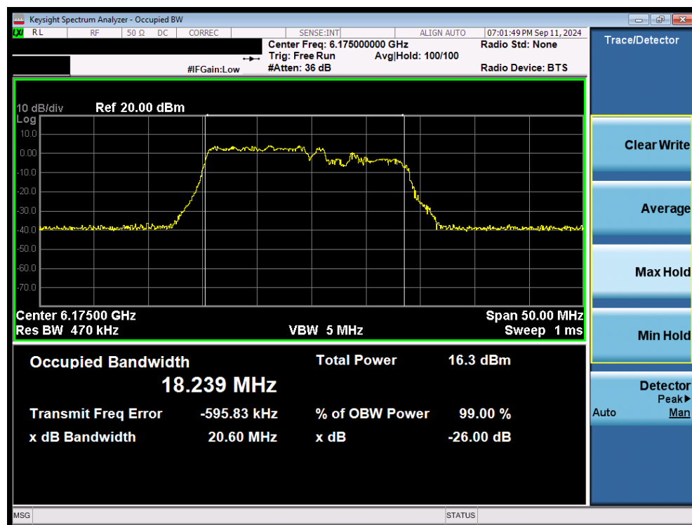
Plot 7-35. 26dB Bandwidth Plot MIMO ANT2 (20MHz 802.11be (106+26 Tones) (UNII Band 5) – Ch. 45) - LPI
