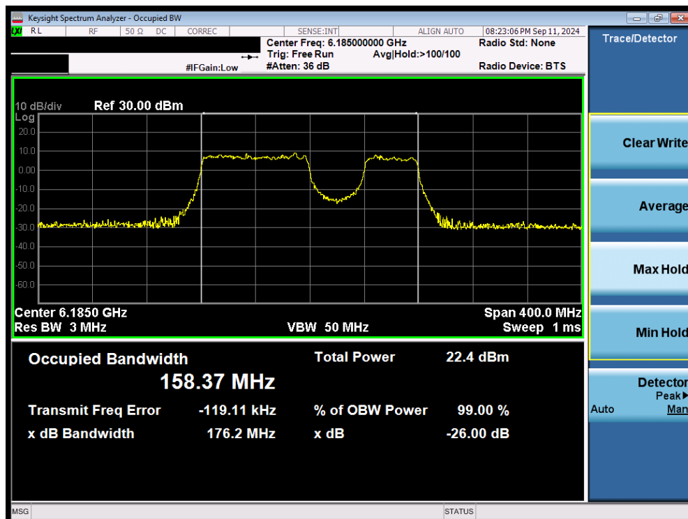
Plot 7-37. 26dB Bandwidth Plot MIMO ANT2 (160MHz 802.11be (996+484 Tones) (UNII Band 5) – Ch. 47) LPI/SP
