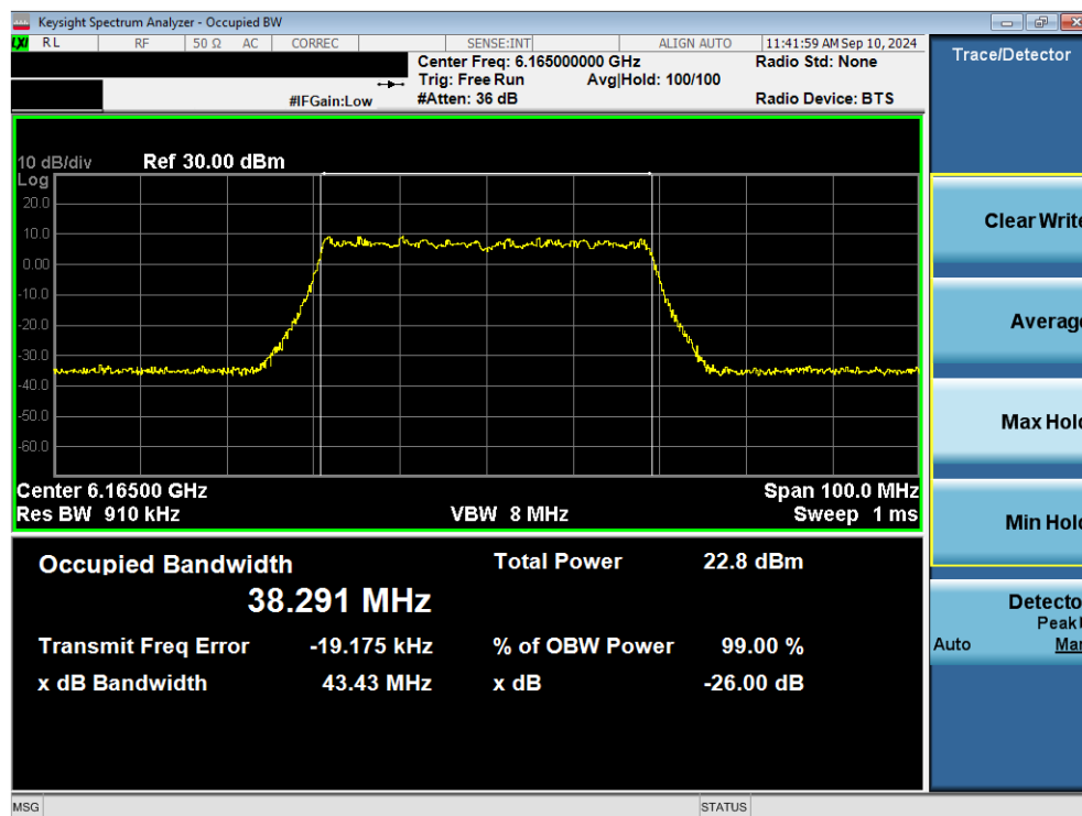
Plot 7-24. 26dB Bandwidth Plot MIMO ANT1 (40MHz 802.11ax/be (Full Tones) (UNII Band 5) – Ch. 43) - LPI
