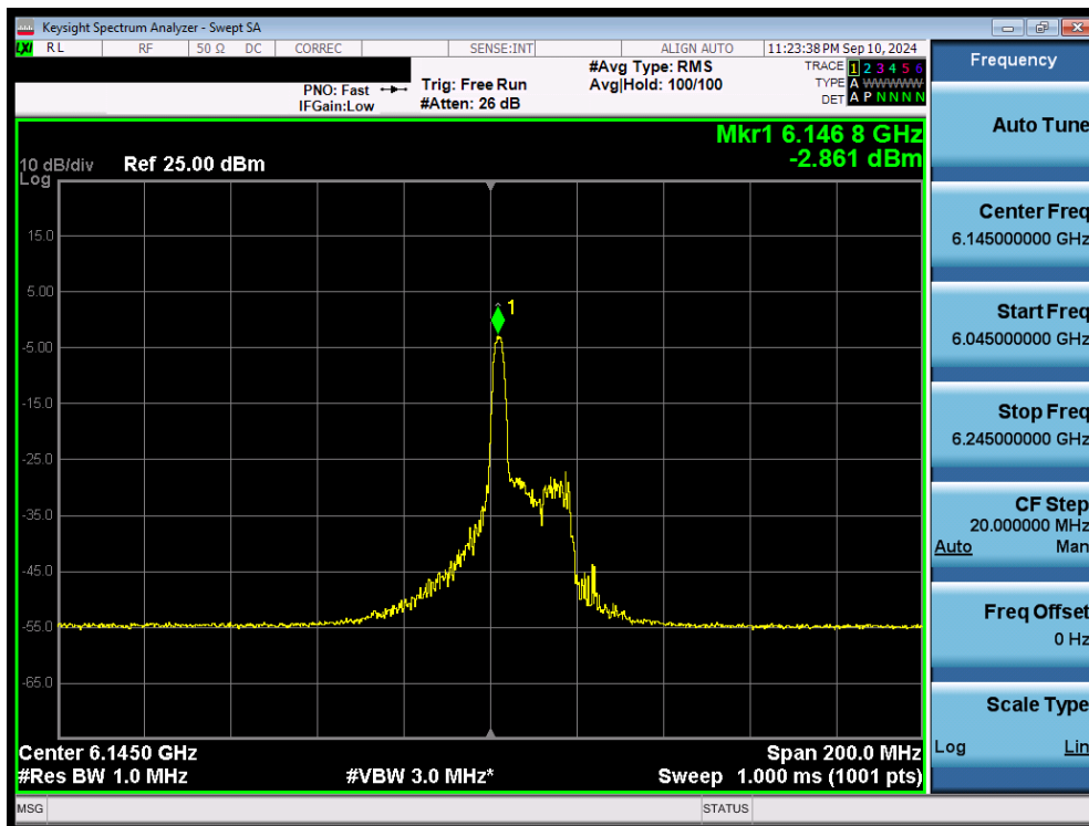
Plot 7-78. Power Spectral Density Plot MIMO ANT2 (80MHz 802.11ax/be (26 Tones) (UNII Band 5) – Ch. 39) - LPI
