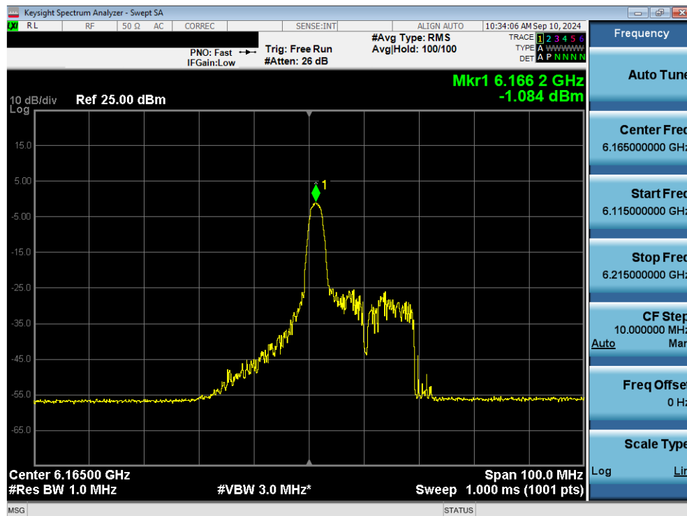
Plot 7-53. Power Spectral Density Plot MIMO ANT1 (40MHz 802.11ax/be (26 Tones) (UNII Band 5) – Ch. 43) - LPI
