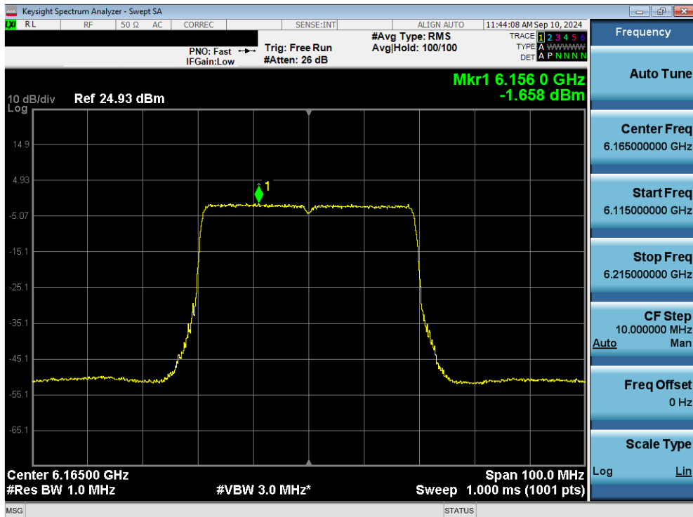
Plot 7-69. Power Spectral Density Plot MIMO ANT1 (40MHz 802.11ax/be (Full Tones) (UNII Band 5) – Ch. 43) - LPI
