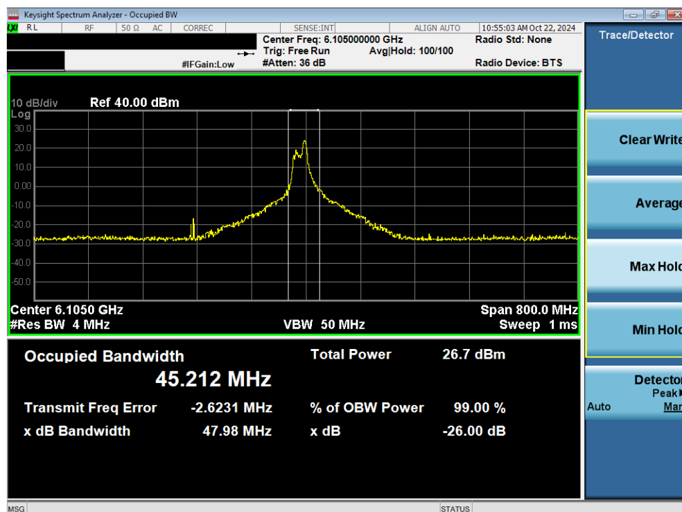
Plot 7-43. 26dB Bandwidth Plot MIMO ANT2 (320MHz 802.11ax/be (26 Tones) (UNII Band 5) – Ch. 31) - SP
