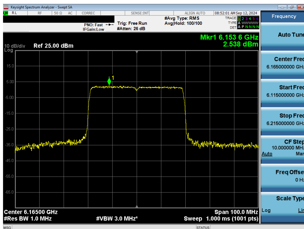
Plot 7-74. Power Spectral Density Plot MIMO ANT1 (40MHz 802.11ax/be (Full Tones) (UNII Band 5) – Ch. 43) - SP
