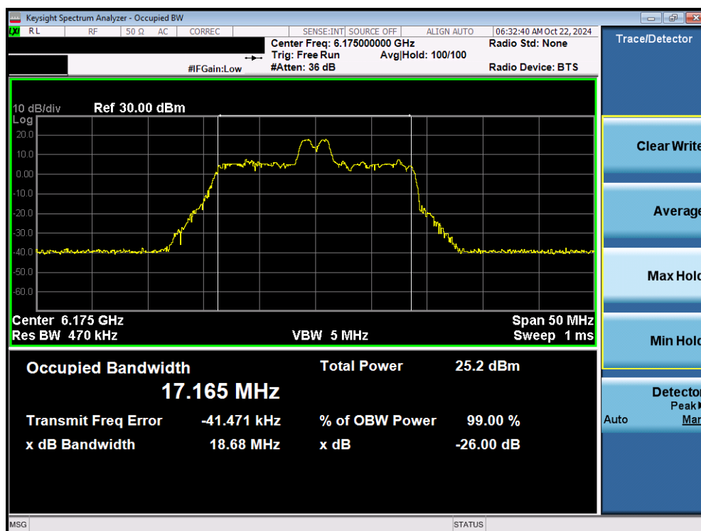
Plot 7-17. 26dB Bandwidth Plot MIMO ANT1 (20MHz 802.11ax/be (26 Tones) (UNII Band 5) – Ch. 45) – SP
