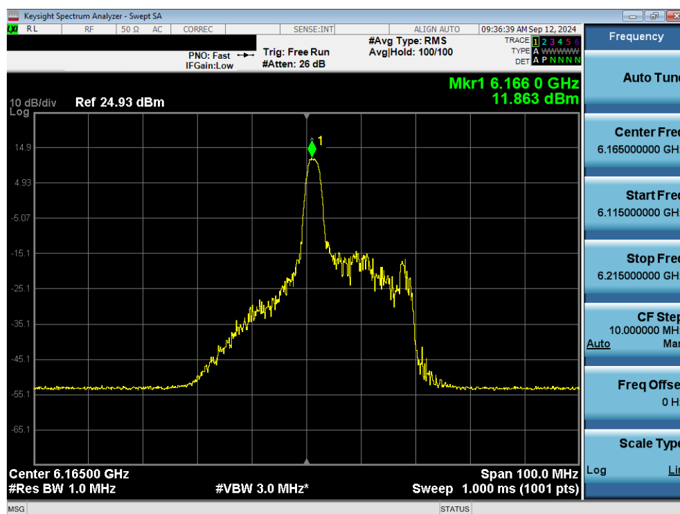
Plot 7-62. Power Spectral Density Plot MIMO ANT1 (40MHz 802.11ax/be (26 Tones) (UNII Band 5) – Ch. 43) - SP
