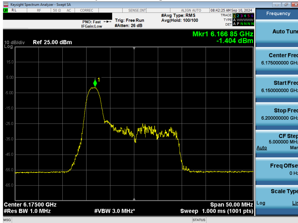
Plot 7-52. Power Spectral Density Plot MIMO ANT1 (20MHz 802.11ax/be (26 Tones) (UNII Band 5) – Ch. 45) - LPI
