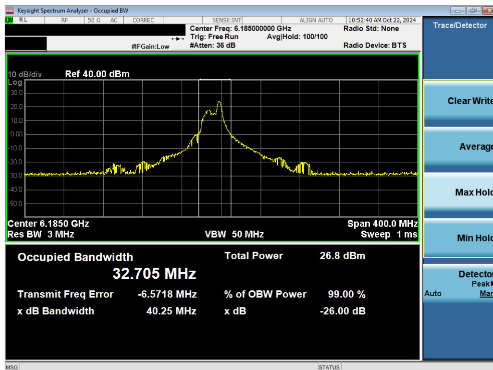
Plot 7-42. 26dB Bandwidth Plot MIMO ANT2 (160MHz 802.11ax/be (26 Tones) (UNII Band 5) – Ch. 47) - SP
