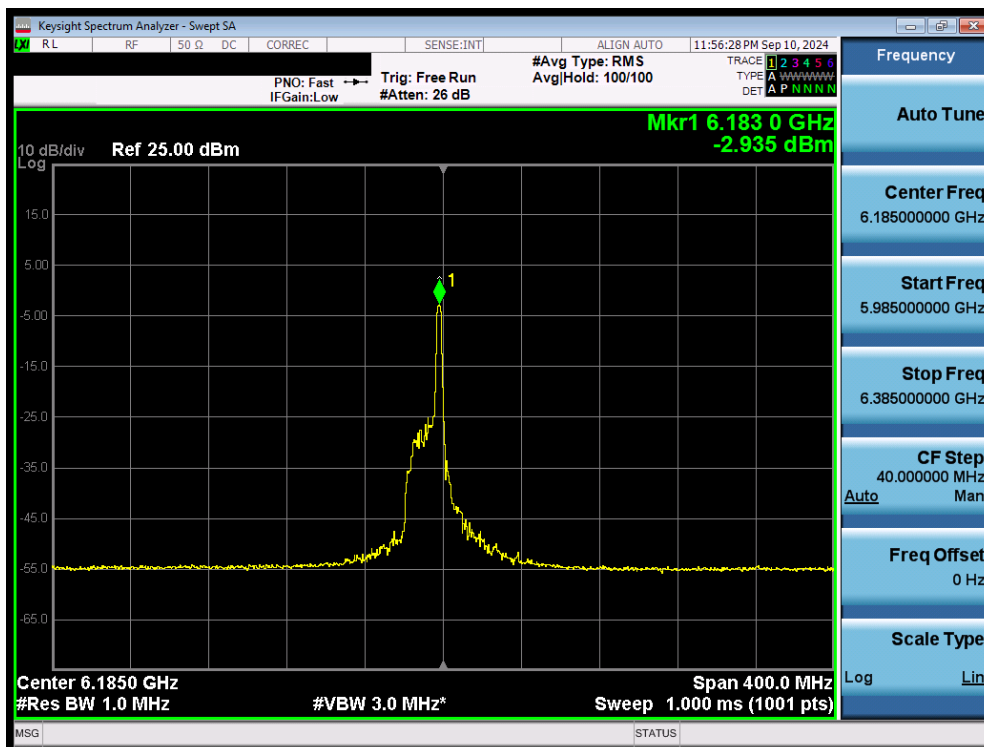
Plot 7-79. Power Spectral Density Plot MIMO ANT2 (160MHz 802.11ax/be (26 Tones) (UNII Band 5) – Ch. 47) - LPI
