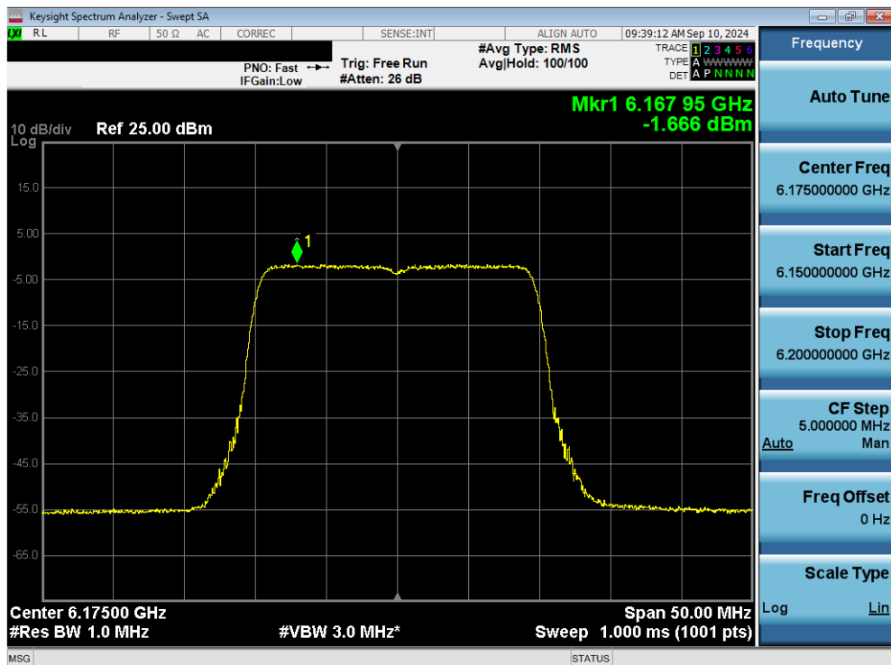
Plot 7-68. Power Spectral Density Plot MIMO ANT1 (20MHz 802.11ax/be (Full Tones) (UNII Band 5) – Ch. 45) - LPI
