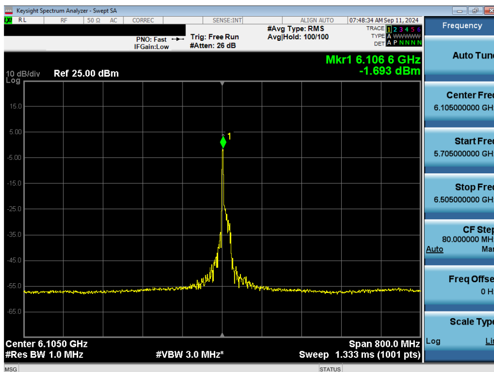
Plot 7-56. Power Spectral Density Plot MIMO ANT1 (320MHz 802.11ax/be (26 Tones) (UNII Band 5) – Ch. 31) - LPI
