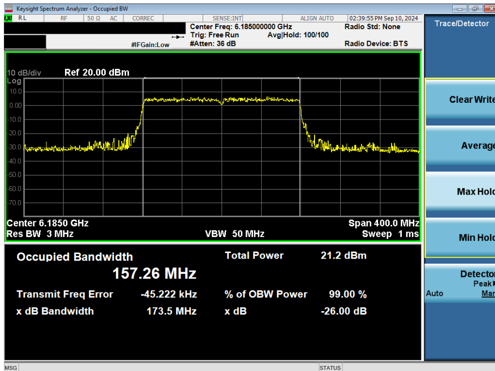
Plot 7-26. 26dB Bandwidth Plot MIMO ANT1 (160MHz 802.11ax/be (Full Tones) (UNII Band 5) – Ch. 47) - LPI/SP
