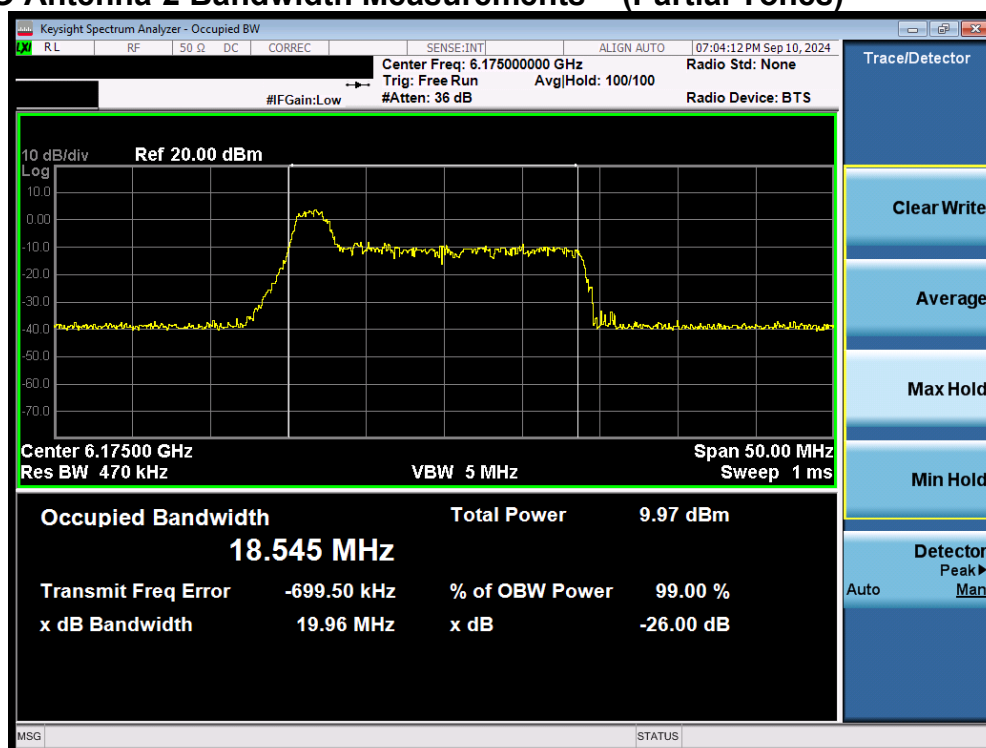
Plot 7-30. 26dB Bandwidth Plot MIMO ANT2 (20MHz 802.11ax/be (26 Tones) (UNII Band 5) – Ch. 45) - LPI
