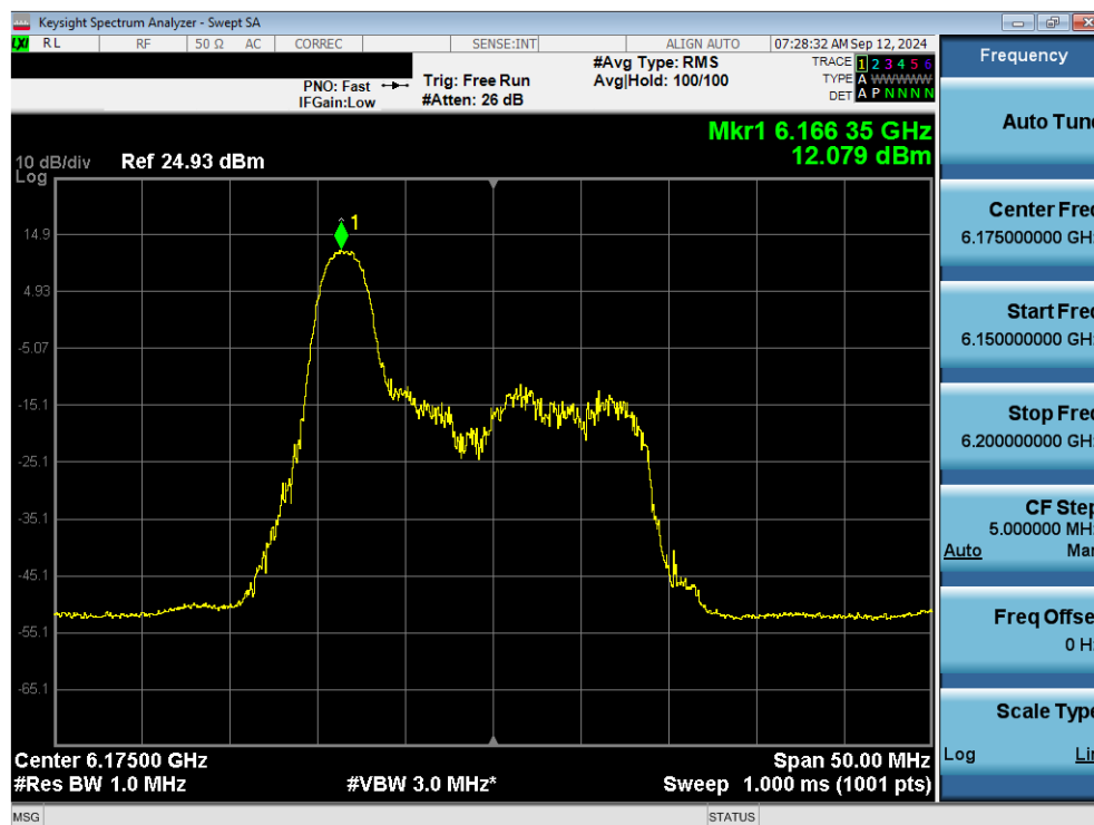
Plot 7-61. Power Spectral Density Plot MIMO ANT1 (20MHz 802.11ax/be (26 Tones) (UNII Band 5) – Ch. 45) - SP
