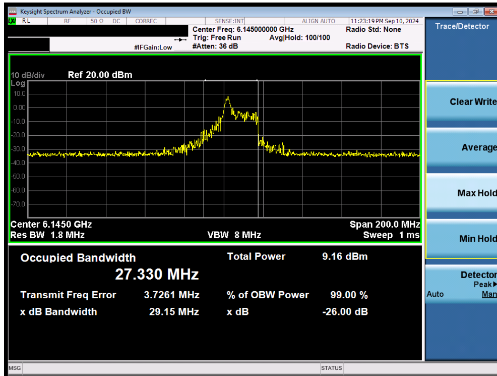
Plot 7-32. 26dB Bandwidth Plot MIMO ANT2 (80MHz 802.11ax/be (26 Tones) (UNII Band 5) – Ch. 39) - LPI
