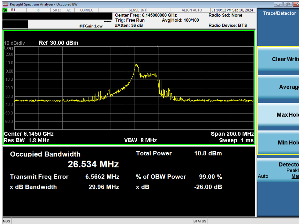
Plot 7-10. 26dB Bandwidth Plot MIMO ANT1 (80MHz 802.11ax/be (26 Tones) (UNII Band 5) – Ch. 39) - LPI
