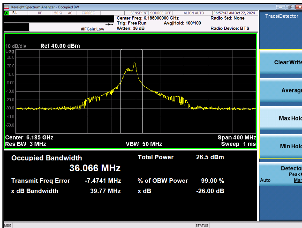
Plot 7-20. 26dB Bandwidth Plot MIMO ANT1 (160MHz 802.11ax/be (26 Tones) (UNII Band 5) – Ch. 47) - SP
