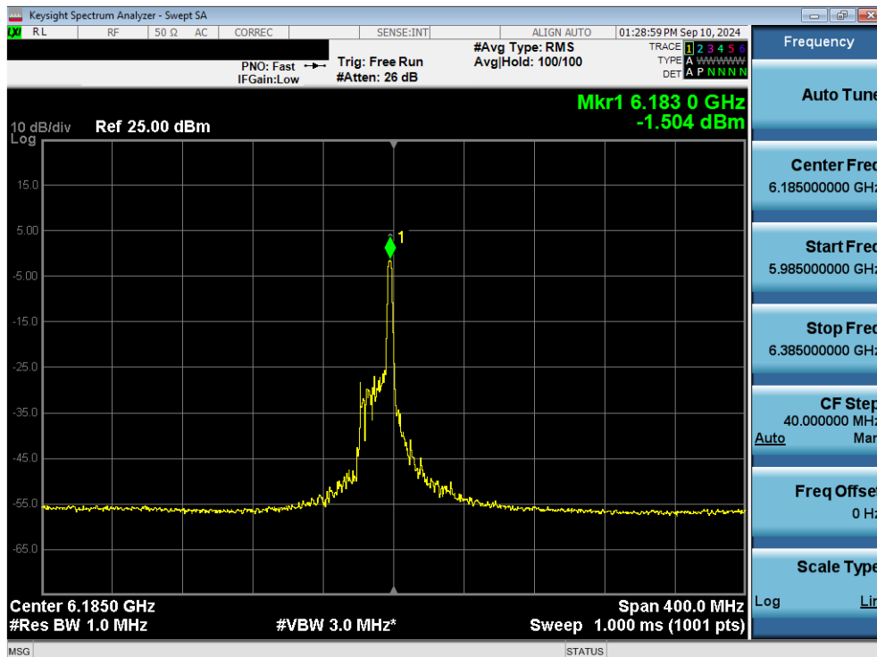
Plot 7-55. Power Spectral Density Plot MIMO ANT1 (160MHz 802.11ax/be (26 Tones) (UNII Band 5) – Ch. 47) - LPI
