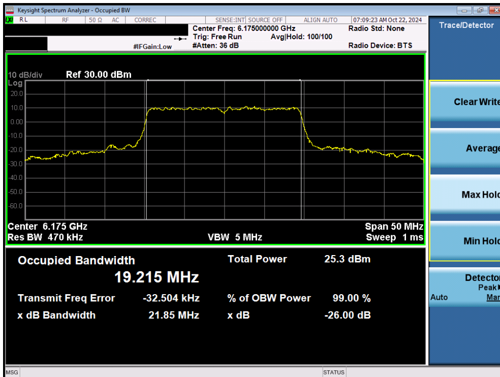
Plot 7-28. 26dB Bandwidth Plot MIMO ANT1 (20MHz 802.11ax/be (Full Tones) (UNII Band 5) – Ch. 45) - SP
