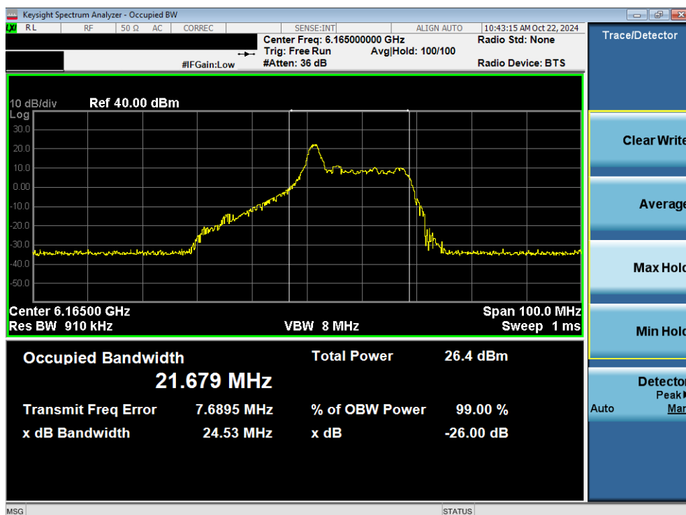
Plot 7-40. 26dB Bandwidth Plot MIMO ANT2 (40MHz 802.11ax/be (26 Tones) (UNII Band 5) – Ch. 43) - SP
