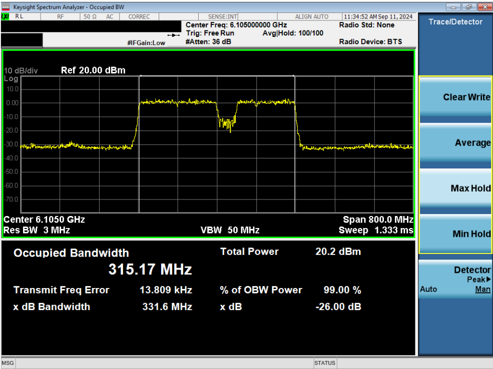
Plot 7-16. 26dB Bandwidth Plot MIMO ANT1 (320MHz 802.11be (3*996+484 Tones) (UNII Band 5) – Ch. 31) LPI/SP
