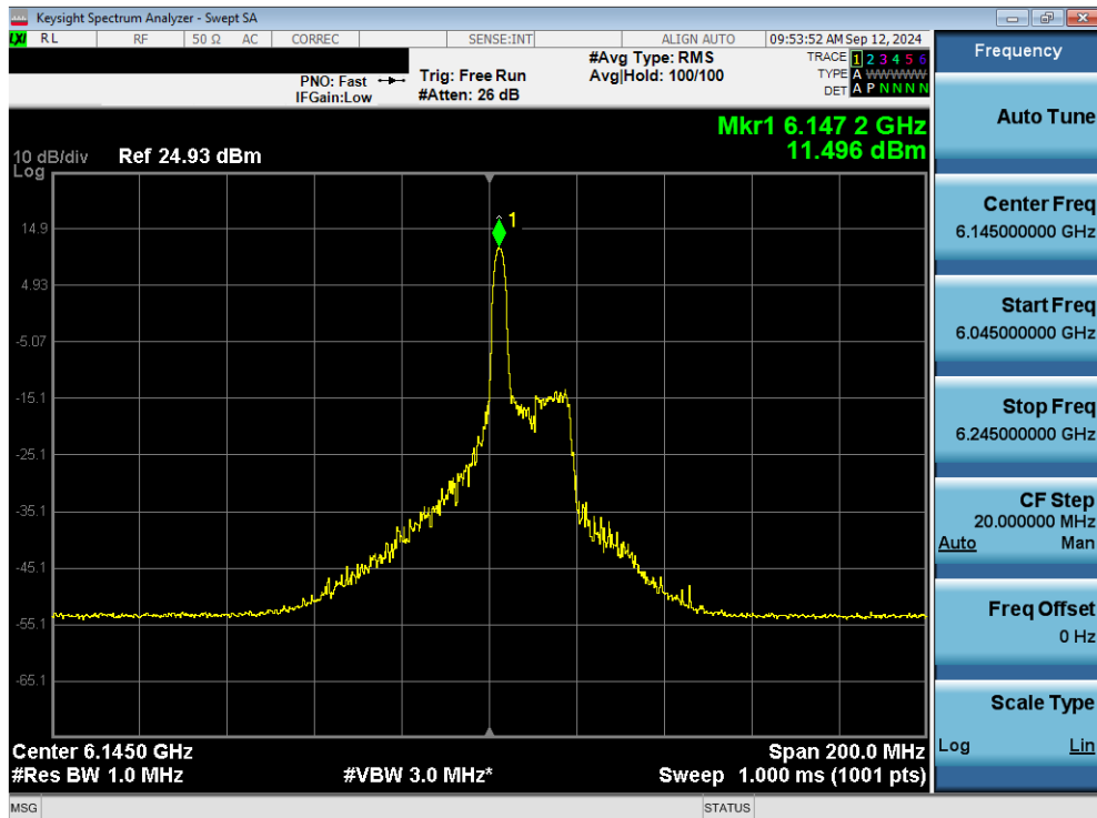
Plot 7-63. Power Spectral Density Plot MIMO ANT1 (80MHz 802.11ax/be (26 Tones) (UNII Band 5) – Ch. 39) - SP
