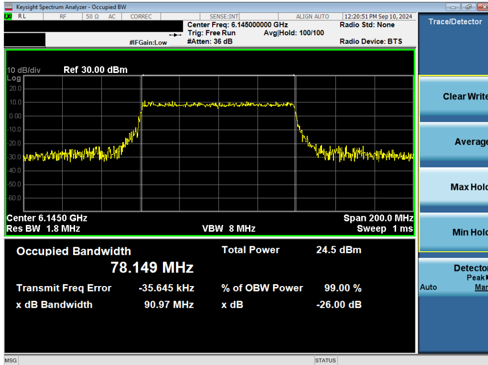
Plot 7-25. 26dB Bandwidth Plot MIMO ANT1 (80MHz 802.11ax/be (Full Tones) (UNII Band 5) – Ch. 39) - LPI/SP
