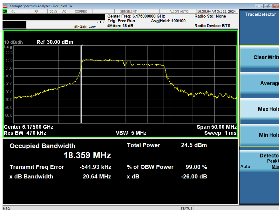
Plot 7-44. 26dB Bandwidth Plot MIMO ANT2 (20MHz 802.11be (106+26 Tones) (UNII Band 5) – Ch. 45) - SP
