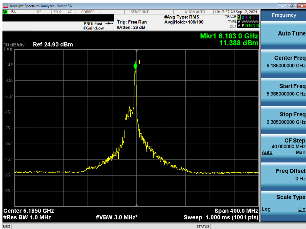
Plot 7-64. Power Spectral Density Plot MIMO ANT1 (160MHz 802.11ax/be (26 Tones) (UNII Band 5) – Ch. 47) - SP
