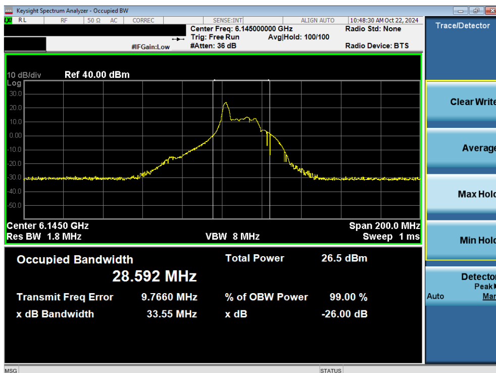
Plot 7-41. 26dB Bandwidth Plot MIMO ANT2 (80MHz 802.11ax/be (26 Tones) (UNII Band 5) – Ch. 39) - SP
