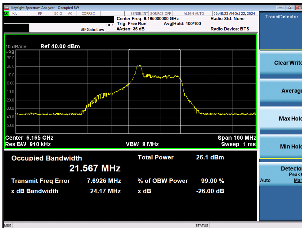
Plot 7-18. 26dB Bandwidth Plot MIMO ANT1 (40MHz 802.11ax/be (26 Tones) (UNII Band 5) – Ch. 43) - SP
