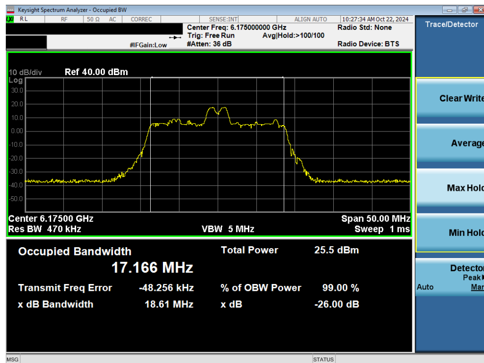
Plot 7-39. 26dB Bandwidth Plot MIMO ANT2 (20MHz 802.11ax/be (26 Tones) (UNII Band 5) – Ch. 45) - SP
