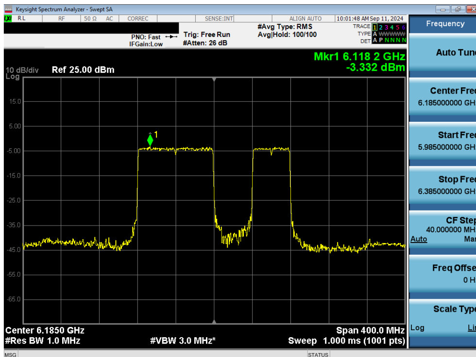
Plot 7-59. Power Spectral Density Plot MIMO ANT1 (160MHz 802.11be (996+484 Tones) (UNII Band 5) – Ch. 47) LPI/SP
