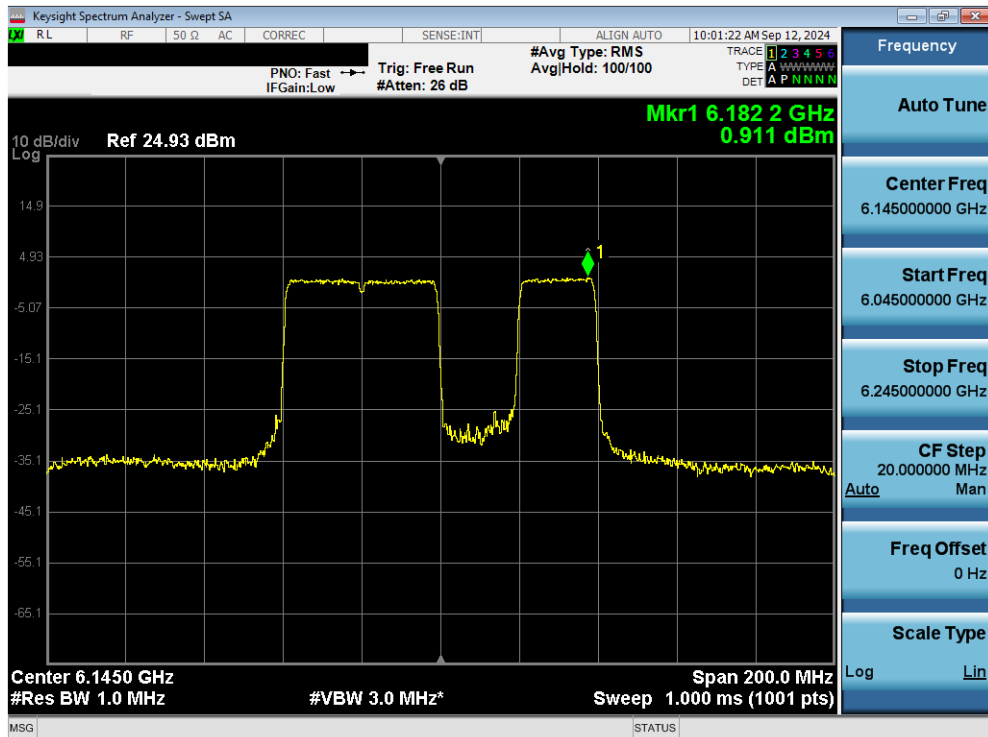
Plot 7-67. Power Spectral Density Plot MIMO ANT1 (80MHz 802.11be (484+242 Tones) (UNII Band 5) – Ch. 39) SP
