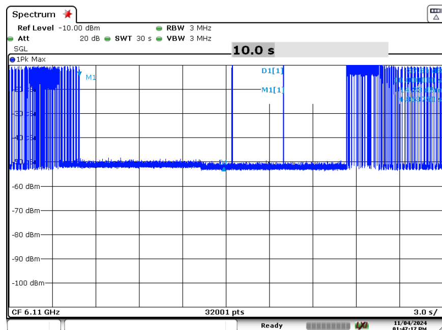
Plot 7-1. Contention Based Protocol Timing Plot (320MHz (UNII Band 5) – Ch. 31 Low)
