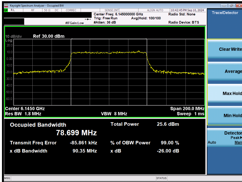
Plot 7-47. 26dB Bandwidth Plot MIMO ANT2 (80MHz 802.11ax/be (Full Tones) (UNII Band 5) – Ch. 39) - LPI/SP
