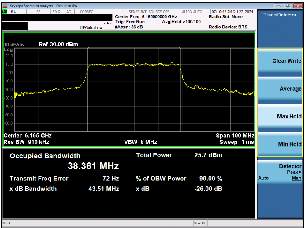
Plot 7-29. 26dB Bandwidth Plot MIMO ANT1 (40MHz 802.11ax/be (Full Tones) (UNII Band 5) – Ch. 43) - SP
