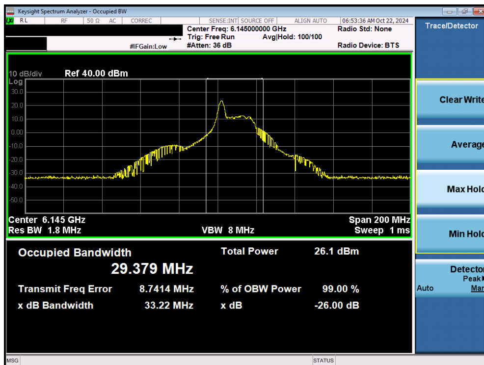
Plot 7-19. 26dB Bandwidth Plot MIMO ANT1 (80MHz 802.11ax/be (26 Tones) (UNII Band 5) – Ch. 39) - SP
