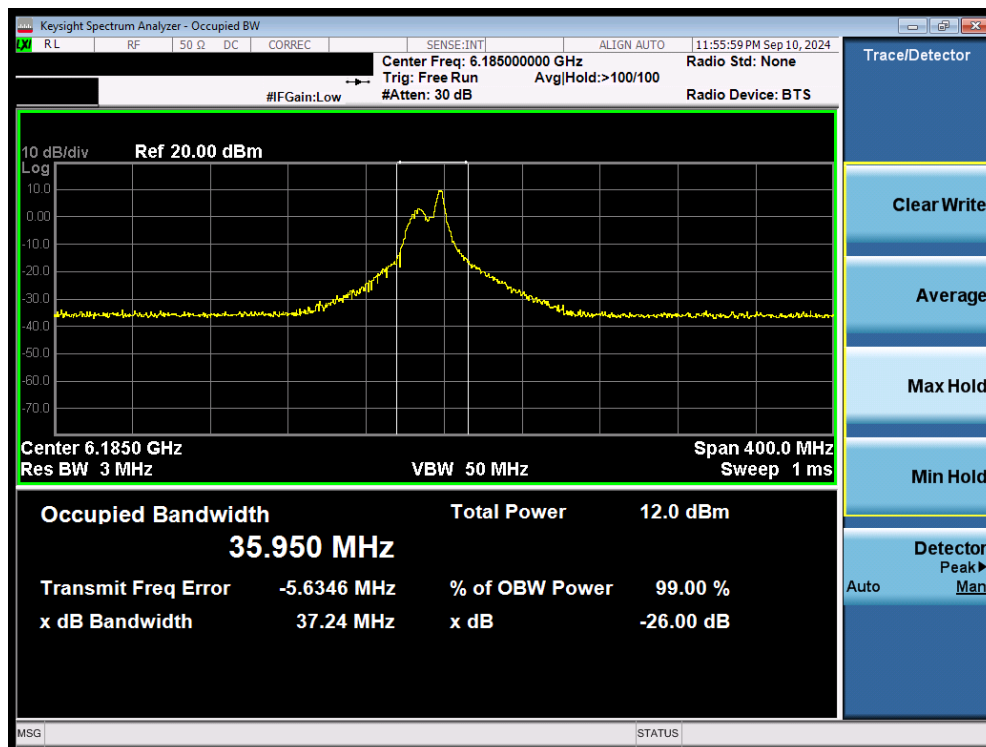
Plot 7-33. 26dB Bandwidth Plot MIMO ANT2 (160MHz 802.11ax/be (26 Tones) (UNII Band 5) – Ch. 47) - LPI
