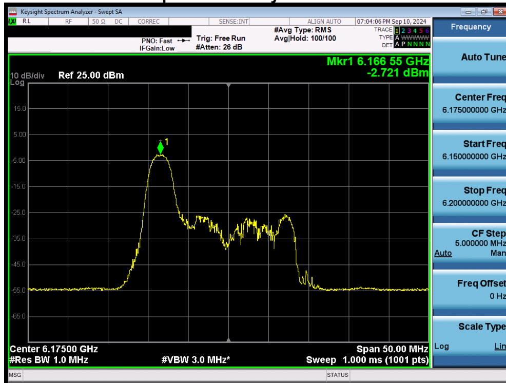
Plot 7-76. Power Spectral Density Plot MIMO ANT2 (20MHz 802.11ax/be (26 Tones) (UNII Band 5) – Ch. 45) - LPI
