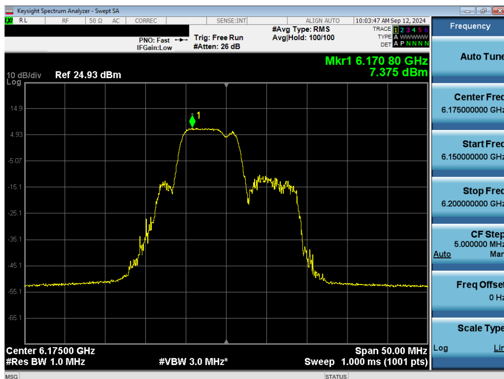
Plot 7-66. Power Spectral Density Plot MIMO ANT1 (20MHz 802.11be (52+26 Tones) (UNII Band 5) – Ch. 45) - SP
