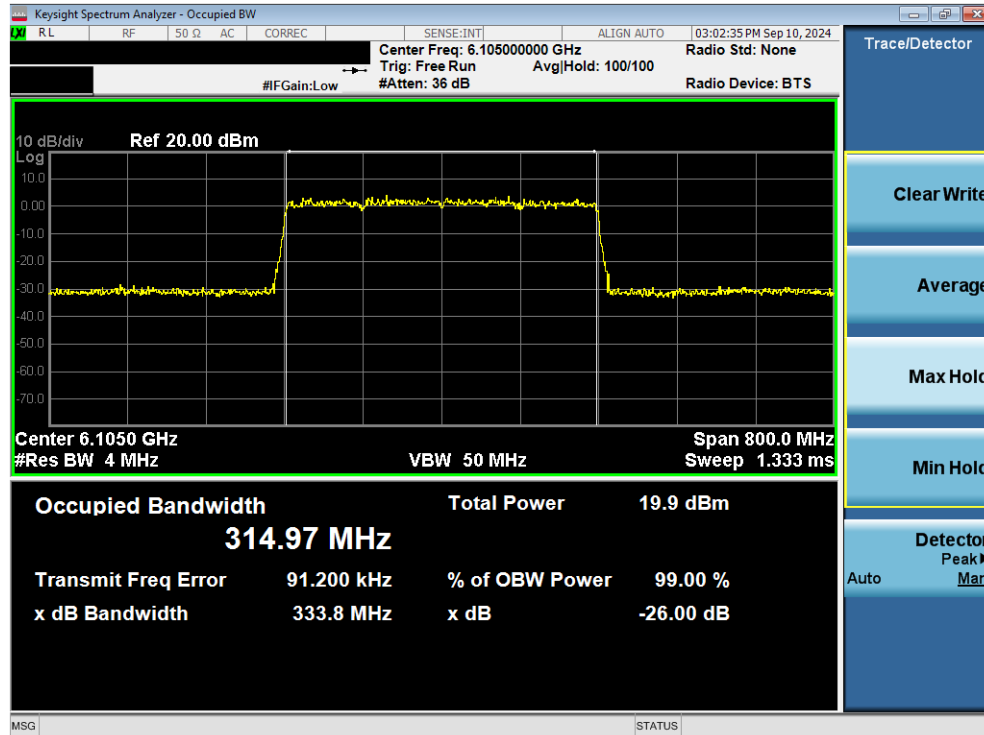
Plot 7-27. 26dB Bandwidth Plot MIMO ANT1 (320MHz 802.11ax/be (Full Tones) (UNII Band 5) – Ch. 31) - LPI/SP
