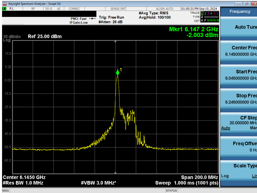
Plot 7-54. Power Spectral Density Plot MIMO ANT1 (80MHz 802.11ax/be (26 Tones) (UNII Band 5) – Ch. 39) - LPI
