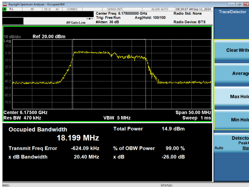
Plot 7-13. 26dB Bandwidth Plot MIMO ANT1 (20MHz 802.11be (106+26 Tones) (UNII Band 5) – Ch. 45) - LPI
