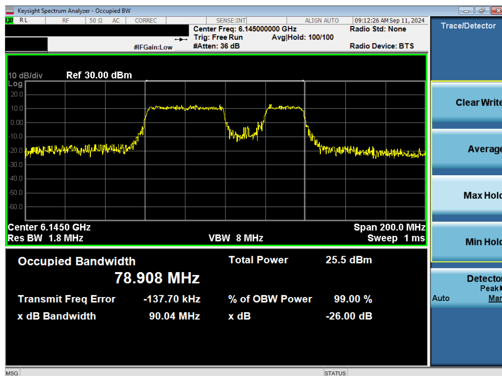
Plot 7-14. 26dB Bandwidth Plot MIMO ANT1 (80MHz 802.11be (484+242 Tones) (UNII Band 5) – Ch. 39) - LPI
