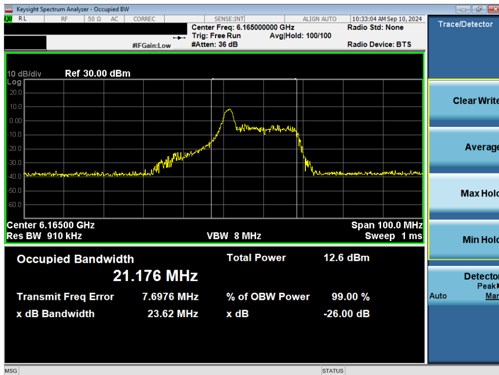
Plot 7-9. 26dB Bandwidth Plot MIMO ANT1 (40MHz 802.11ax/be (26 Tones) (UNII Band 5) – Ch. 43) - LPI
