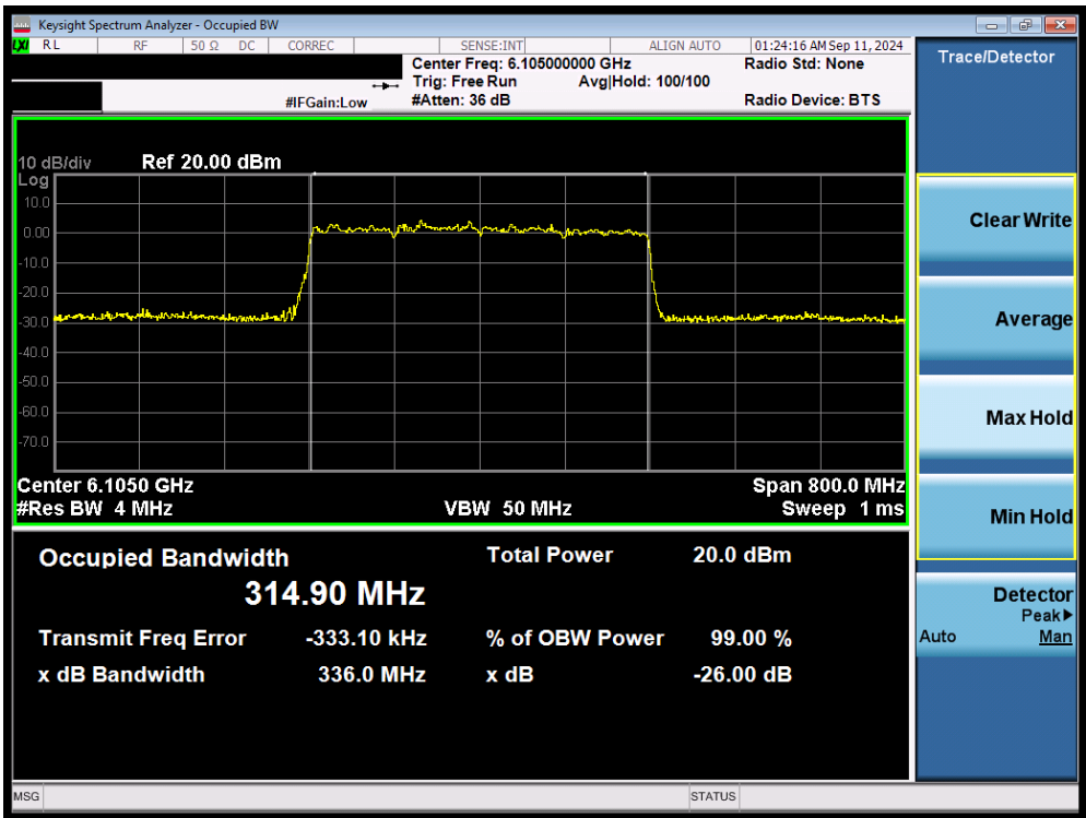
Plot 7-49. 26dB Bandwidth Plot MIMO ANT2 (320MHz 802.11ax/be (Full Tones) (UNII Band 5) – Ch. 31) - LPI/SP
