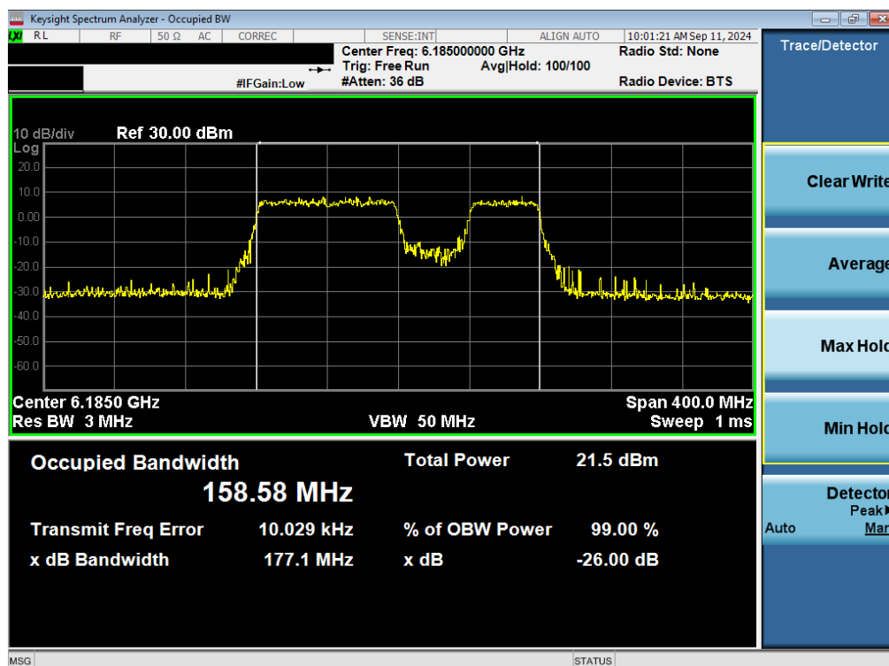
Plot 7-15. 26dB Bandwidth Plot MIMO ANT1 (160MHz 802.11be (996+484 Tones) (UNII Band 5) – Ch. 47) LPI/SP
