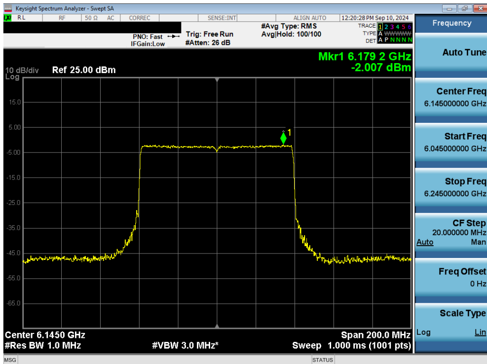
Plot 7-70. Power Spectral Density Plot MIMO ANT1 (80MHz 802.11ax/be (Full Tones) (UNII Band 5) – Ch. 39) - LPI
