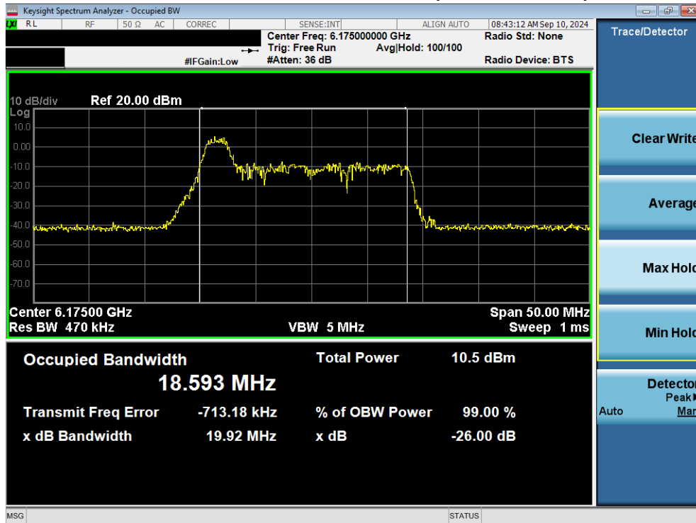
Plot 7-8. 26dB Bandwidth Plot MIMO ANT1 (20MHz 802.11ax/be (26 Tones) (UNII Band 5) – Ch. 45) - LPI
