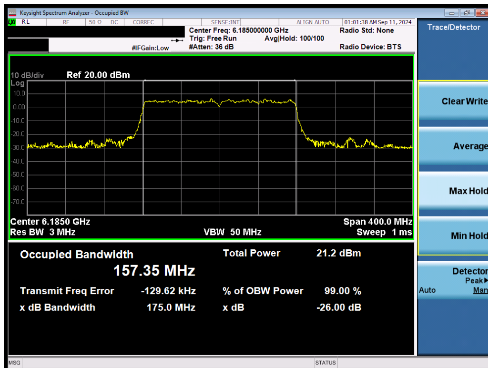
Plot 7-48. 26dB Bandwidth Plot MIMO ANT2 (160MHz 802.11ax/be (Full Tones) (UNII Band 5) – Ch. 47) - LPI/SP
