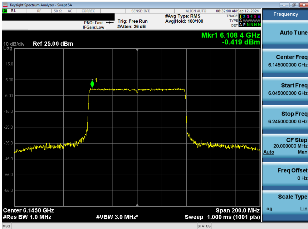
Plot 7-75. Power Spectral Density Plot MIMO ANT1 (80MHz 802.11ax/be (Full Tones) (UNII Band 5) – Ch. 39) - SP
