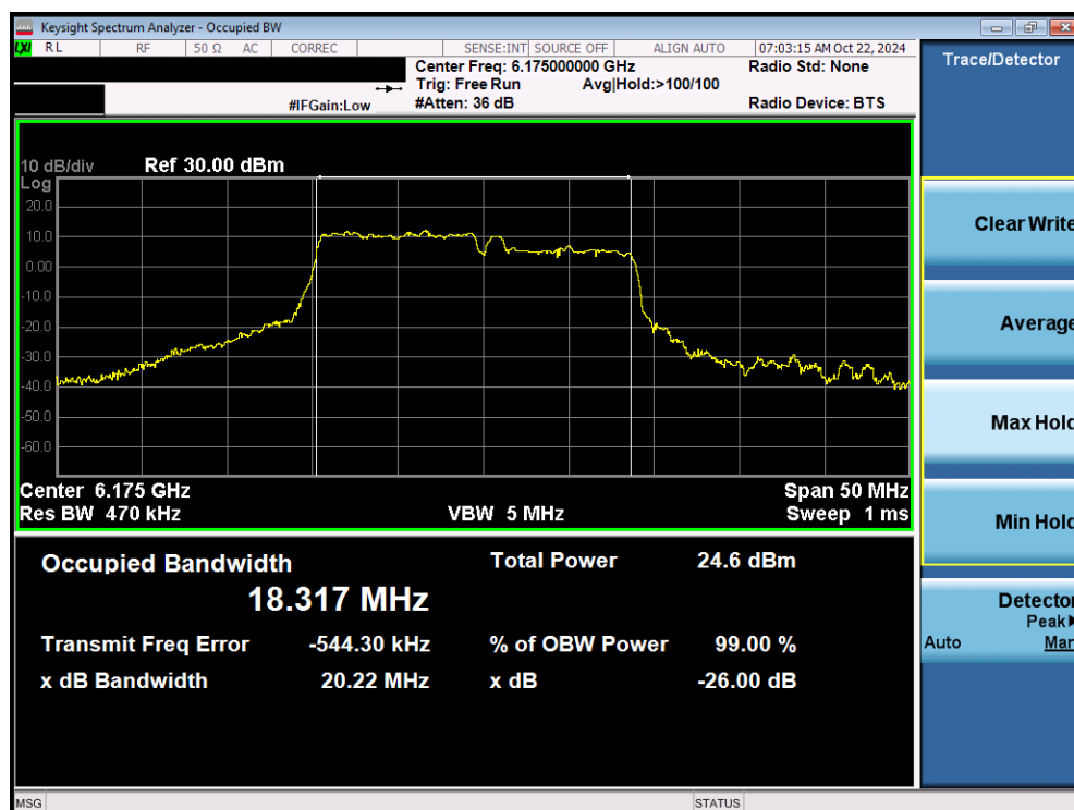
Plot 7-22. 26dB Bandwidth Plot MIMO ANT1 (20MHz 802.11be (106+26 Tones) (UNII Band 5) – Ch. 45) - SP
