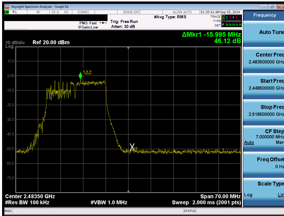
Plot 7-34. Band Edge Plot MIMO ANT1 (802.11be OFDMA – 106+26 Tones – Ch. 12)
