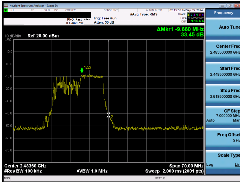
Plot 7-46. Band Edge Plot MIMO ANT2 (802.11ax/be OFDMA – 106 Tones – Ch. 13)
