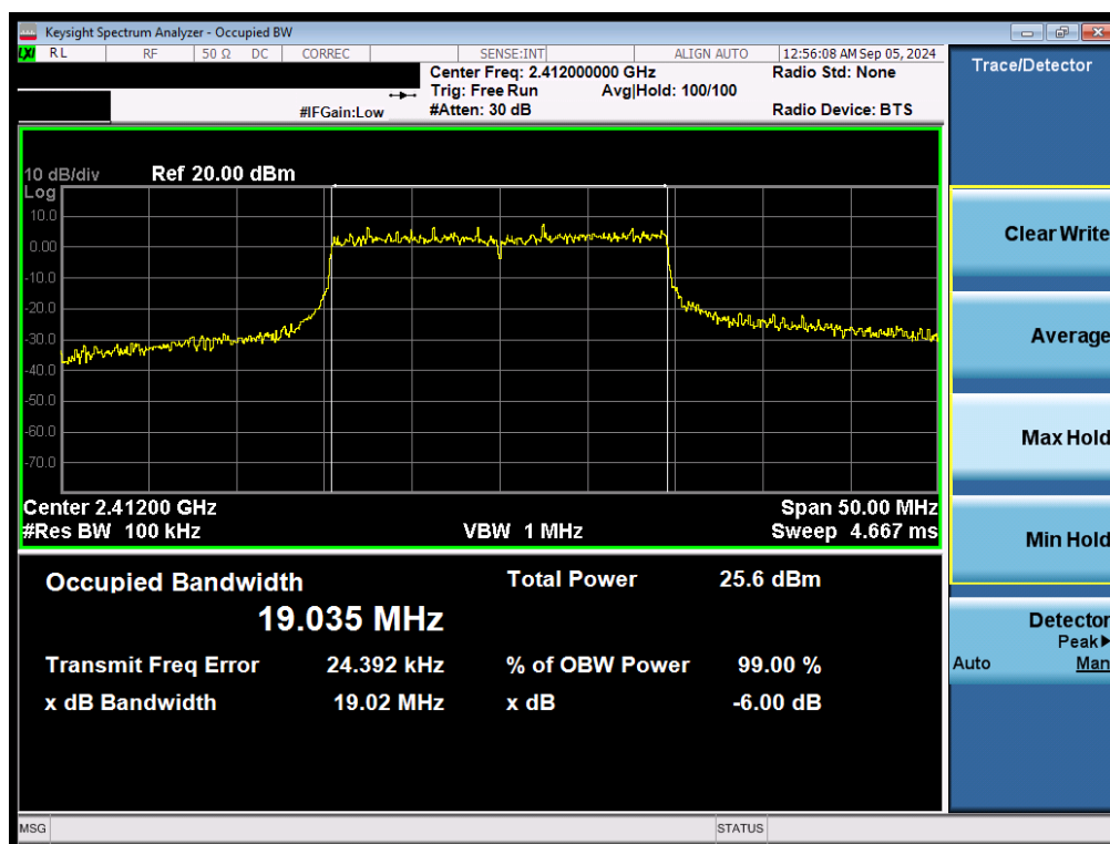
Plot 7-7. 6dB Bandwidth Plot MIMO ANT1 (802.11ax/be OFDMA – 242 Tones – Ch. 1)
