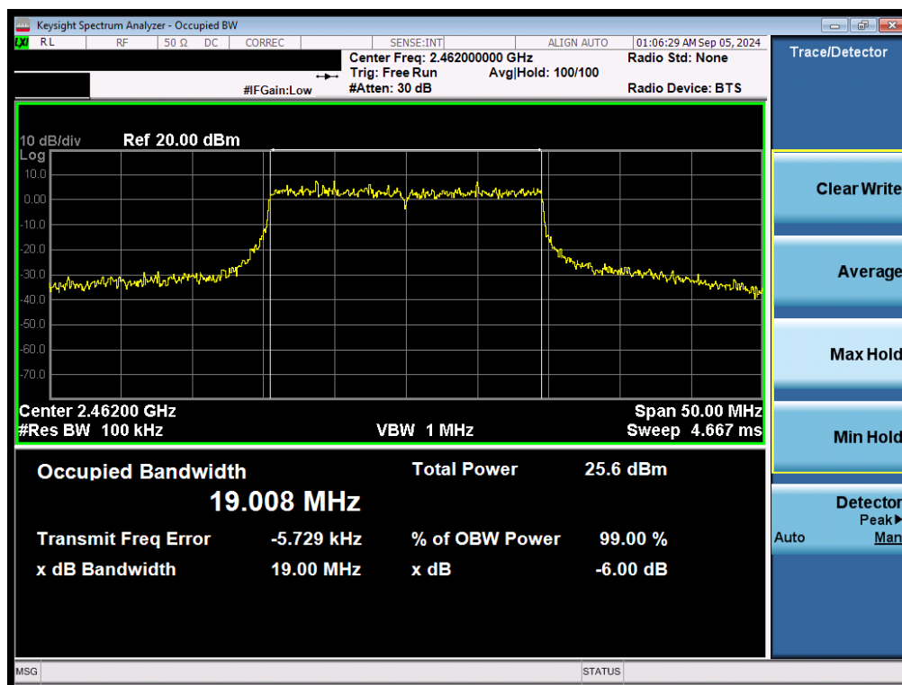
Plot 7-9. 6dB Bandwidth Plot MIMO ANT1 (802.11ax/be OFDMA – 242 Tones – Ch. 11)
