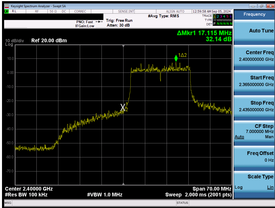
Plot 7-36. Band Edge Plot MIMO ANT1 (802.11ax/be OFDMA – 242 Tones – Ch. 1)
