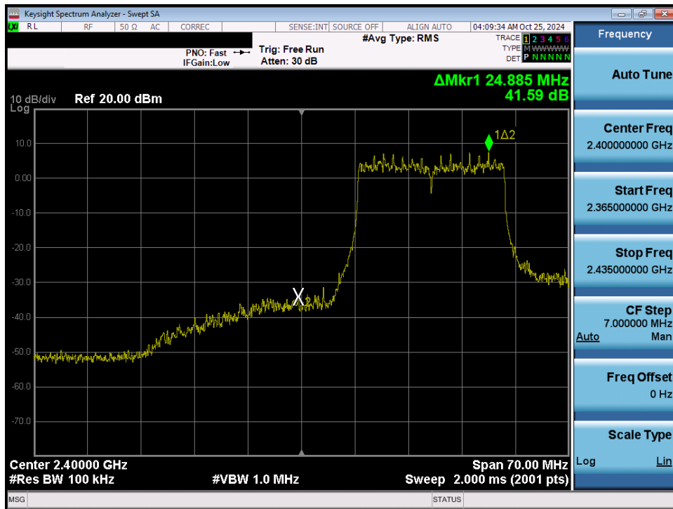
Plot 7-37. Band Edge Plot MIMO ANT1 (802.11ax/be OFDMA – 242 Tones – Ch. 2)
