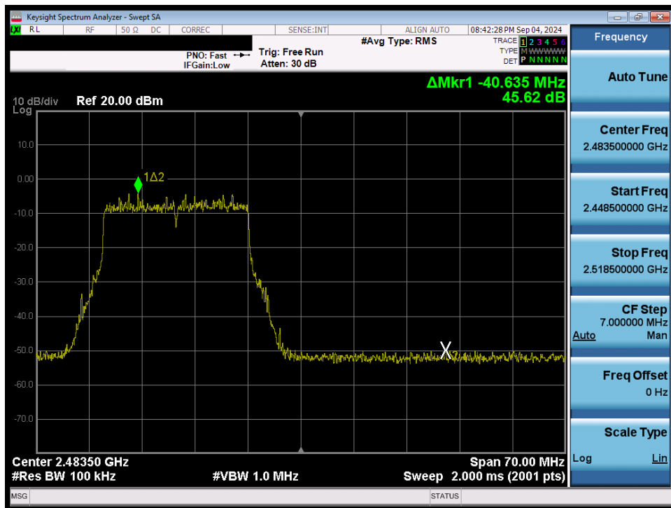
Plot 7-86. Band Edge Plot (802.11ax/be (2.4GHz) – Ch. 12) MIMO ANT2
