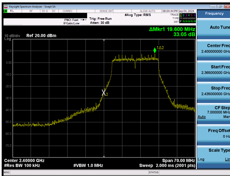
Plot 7-60. Band Edge Plot (802.11n/ac (2.4GHz) – Ch. 1) MIMO ANT1
