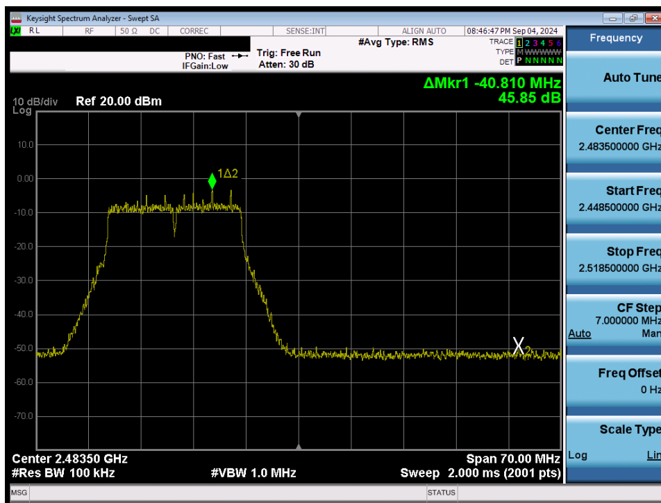
Plot 7-80. Band Edge Plot (802.11n/ac (2.4GHz) – Ch. 12) MIMO ANT2
