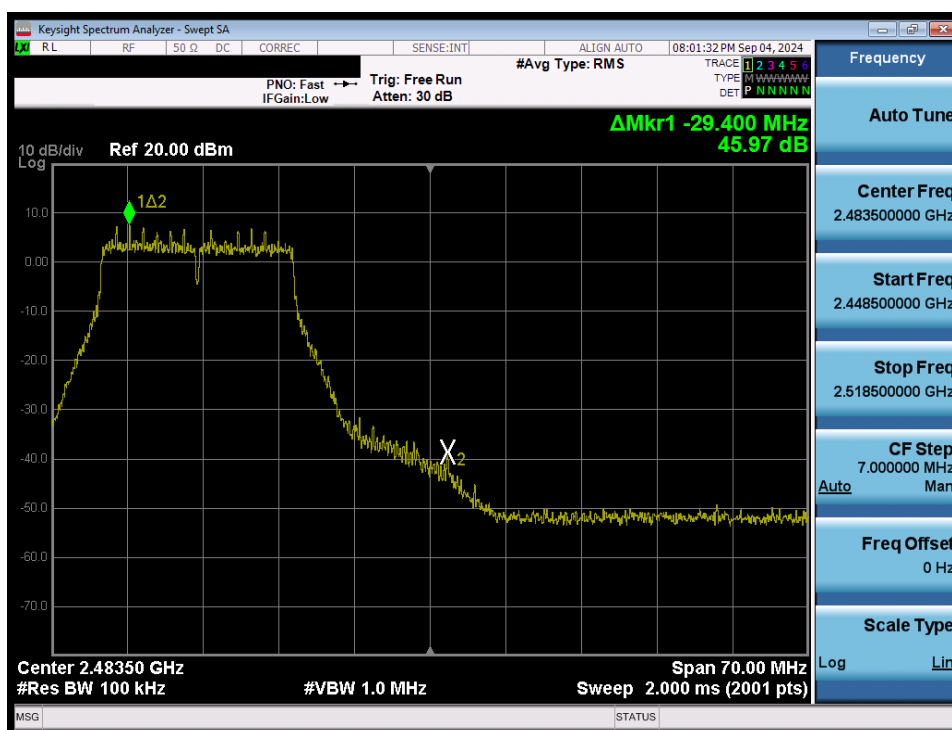
Plot 7-61. Band Edge Plot (802.11n/ac (2.4GHz) – Ch. 11) MIMO ANT1
