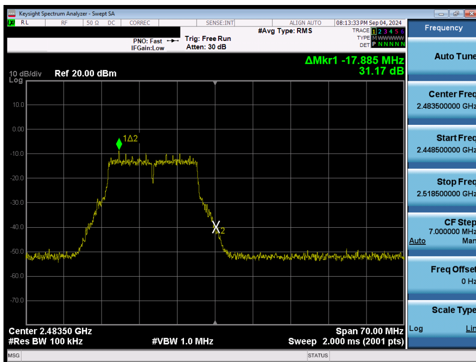
Plot 7-59. Band Edge Plot (802.11g – Ch. 13) MIMO ANT1
