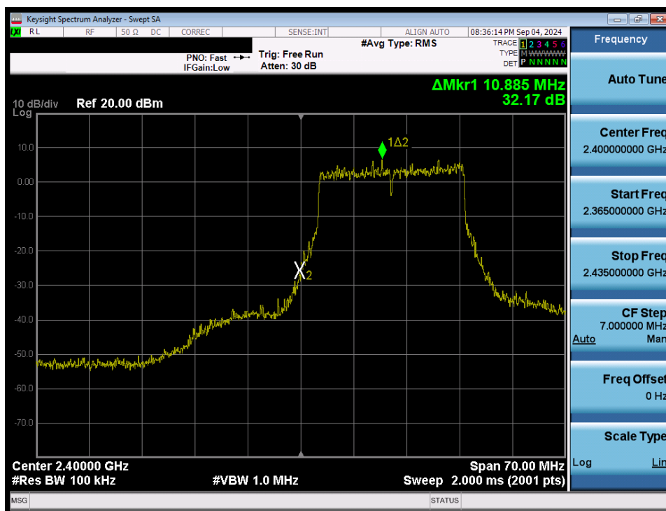
Plot 7-82. Band Edge Plot (802.11ax/be (2.4GHz) – Ch. 1) MIMO ANT2
