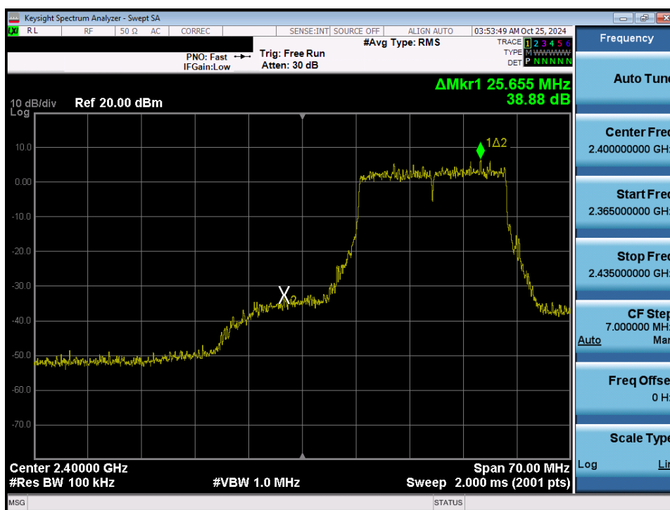
Plot 7-83. Band Edge Plot (802.11ax/be (2.4GHz) – Ch. 2) MIMO ANT2
