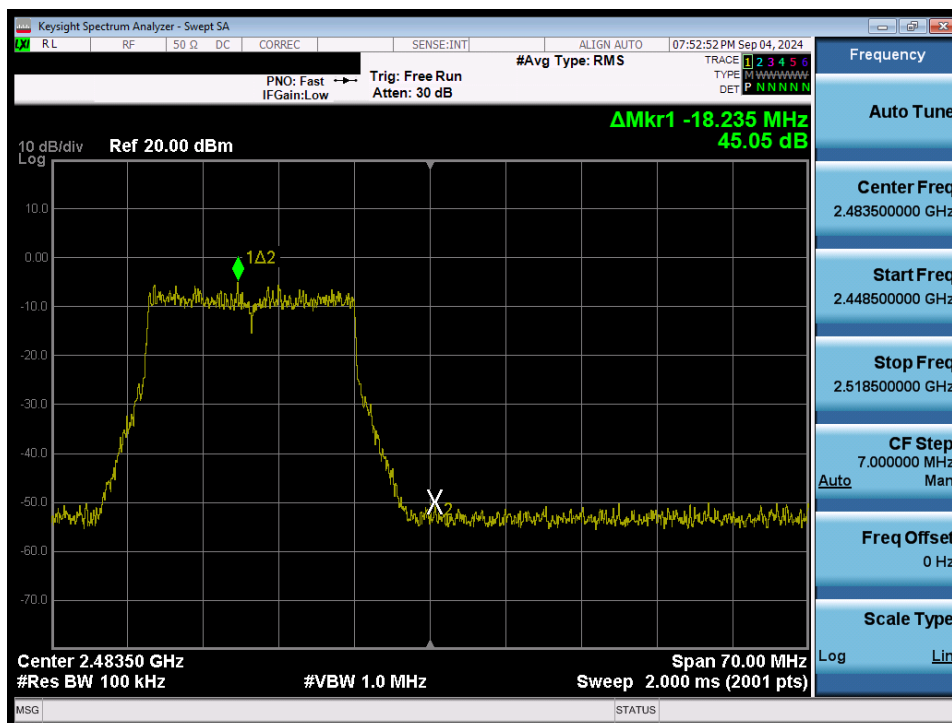
Plot 7-68. Band Edge Plot (802.11ax/be (2.4GHz) – Ch. 12) MIMO ANT1
