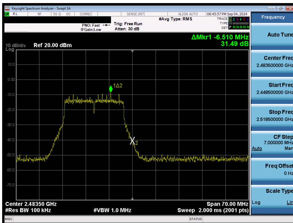
Plot 7-81. Band Edge Plot (802.11n/ac (2.4GHz) – Ch. 13) MIMO ANT2
