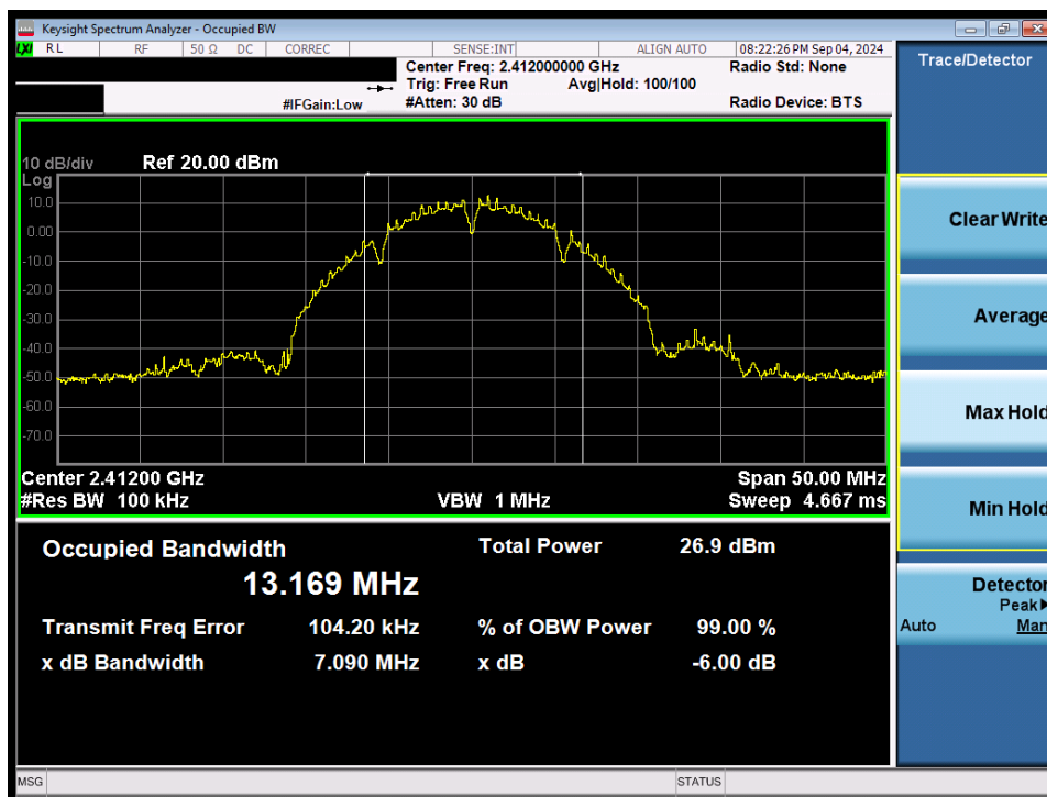
Plot 7-4. 6dB Bandwidth Plot (802.11b – Ch. 1) SISO ANT1
