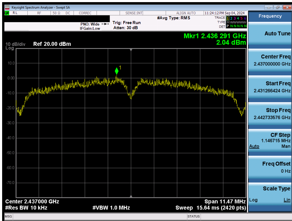
Plot 7-41. Power Spectral Density Plot (802.11b – Ch. 6) SISO ANT2
