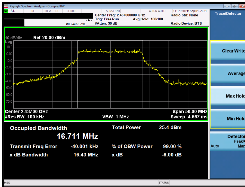
Plot 7-20. 6dB Bandwidth Plot (802.11g – Ch. 6) MIMO ANT2
