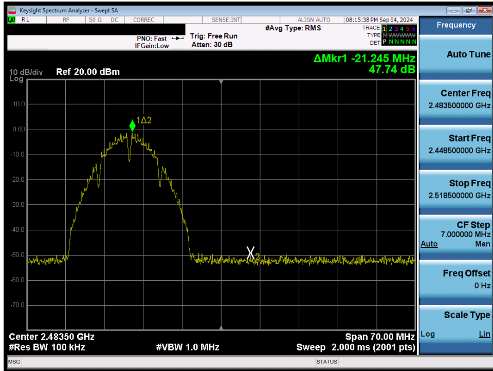
Plot 7-54. Band Edge Plot (802.11b – Ch. 12) SISO ANT1
