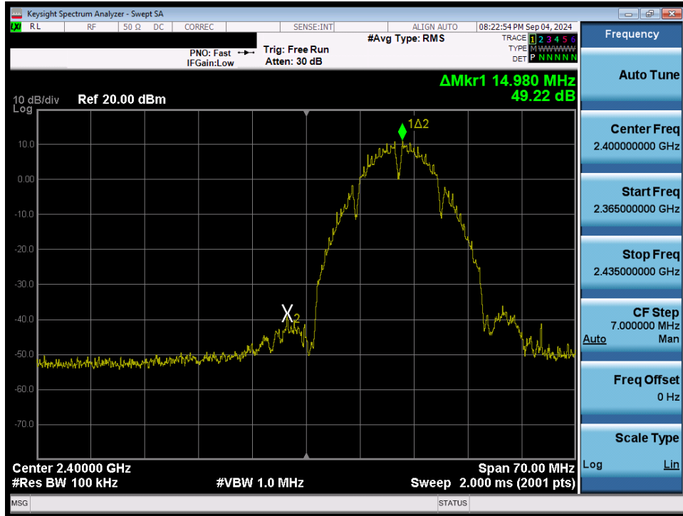
Plot 7-52. Band Edge Plot (802.11b – Ch. 1) SISO ANT1
