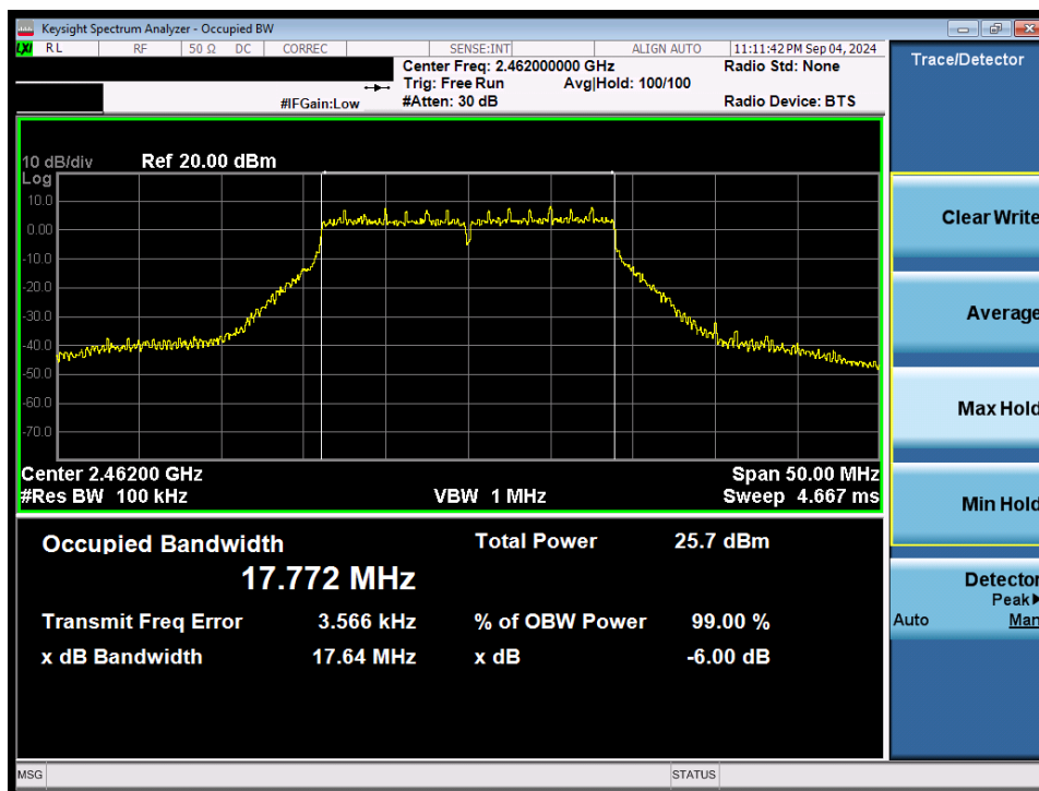
Plot 7-24. 6dB Bandwidth Plot (802.11n/ac (2.4GHz) – Ch. 11) MIMO ANT2
