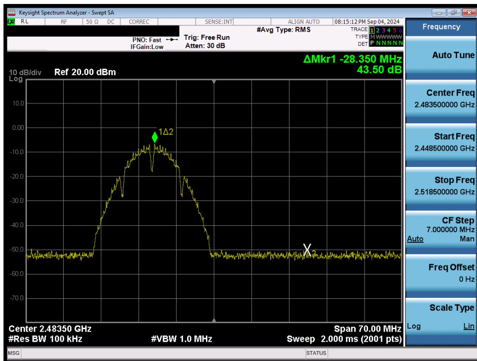
Plot 7-55. Band Edge Plot (802.11b – Ch. 13) SISO ANT1
