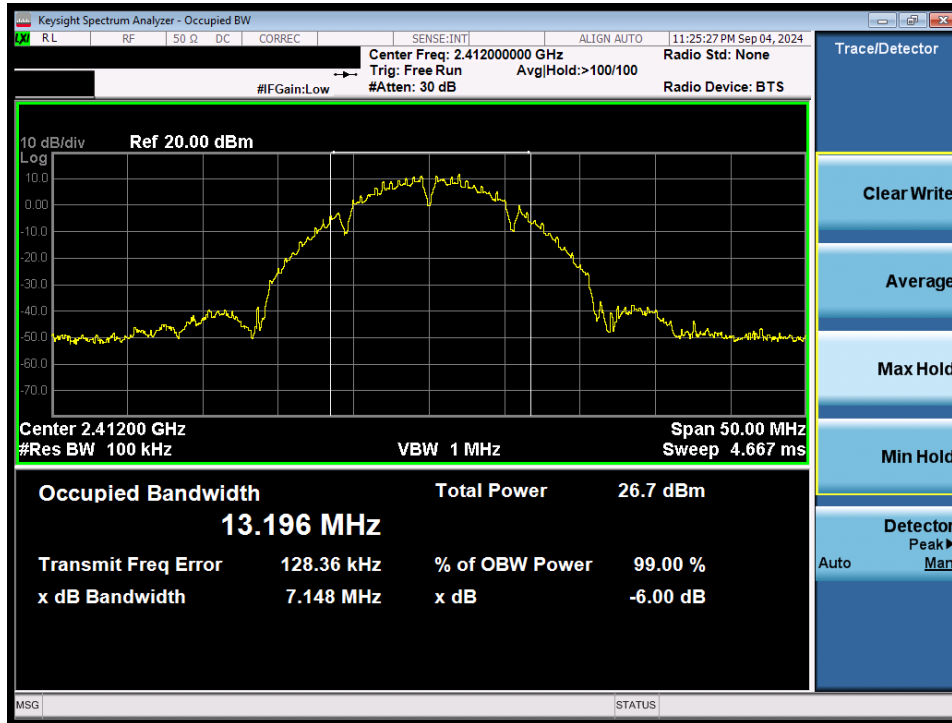
Plot 7-16. 6dB Bandwidth Plot (802.11b – Ch. 1) SISO ANT2
