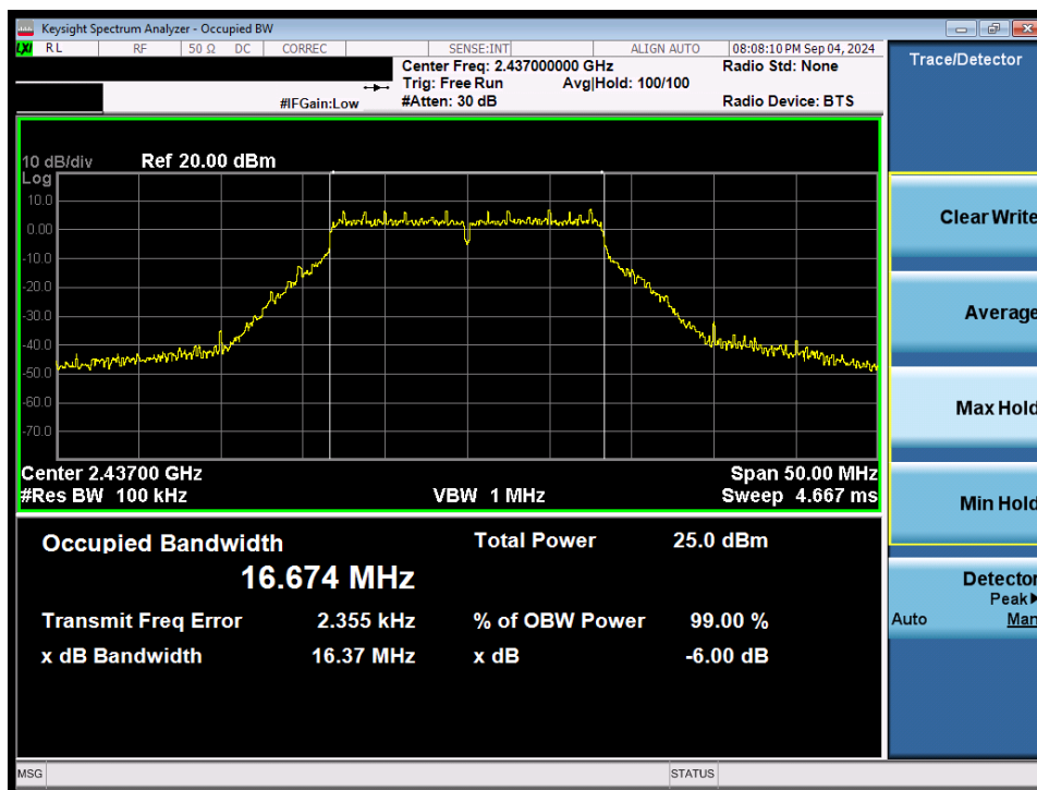
Plot 7-8. 6dB Bandwidth Plot (802.11g – Ch. 6) MIMO ANT1
