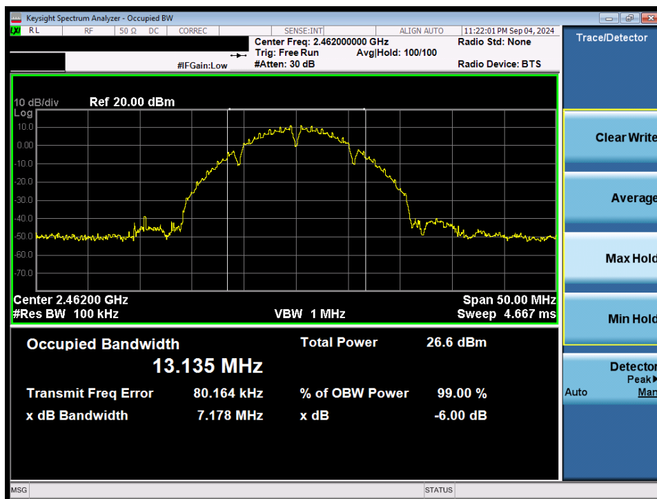
Plot 7-18. 6dB Bandwidth Plot (802.11b – Ch. 11) SISO ANT2
