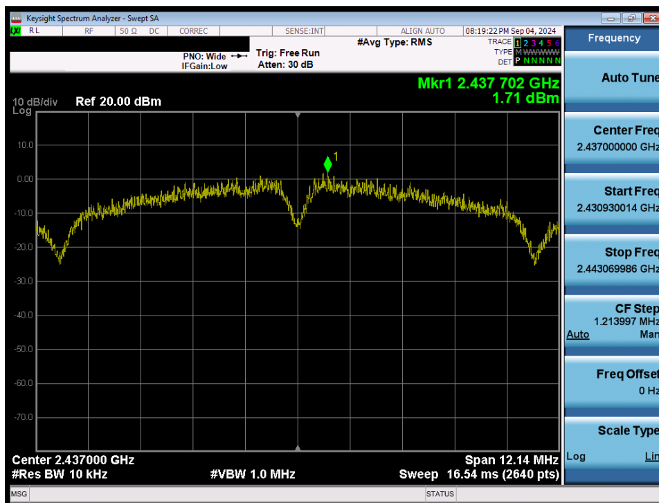
Plot 7-29. Power Spectral Density Plot (802.11b – Ch. 6) SISO ANT1
