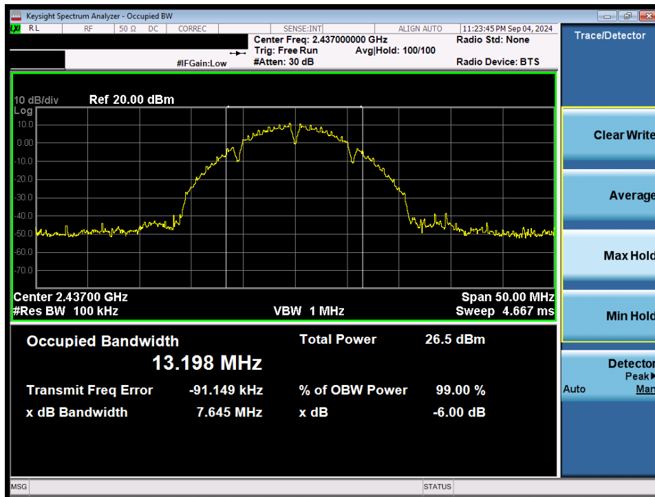
Plot 7-17. 6dB Bandwidth Plot (802.11b – Ch. 6) SISO ANT2
