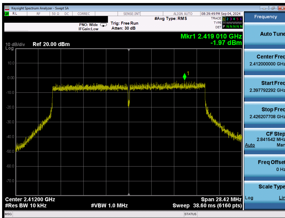
Plot 7-49. Power Spectral Density Plot (802.11ax/be (2.4GHz) – Ch. 1) MIMO ANT2
