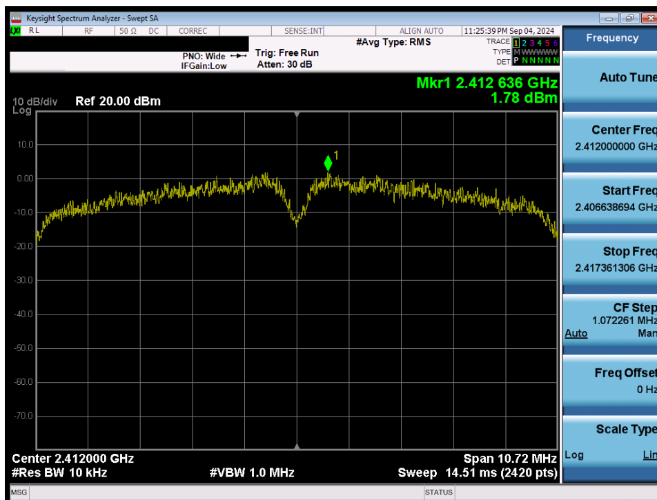
Plot 7-40. Power Spectral Density Plot (802.11b – Ch. 1) SISO ANT2
