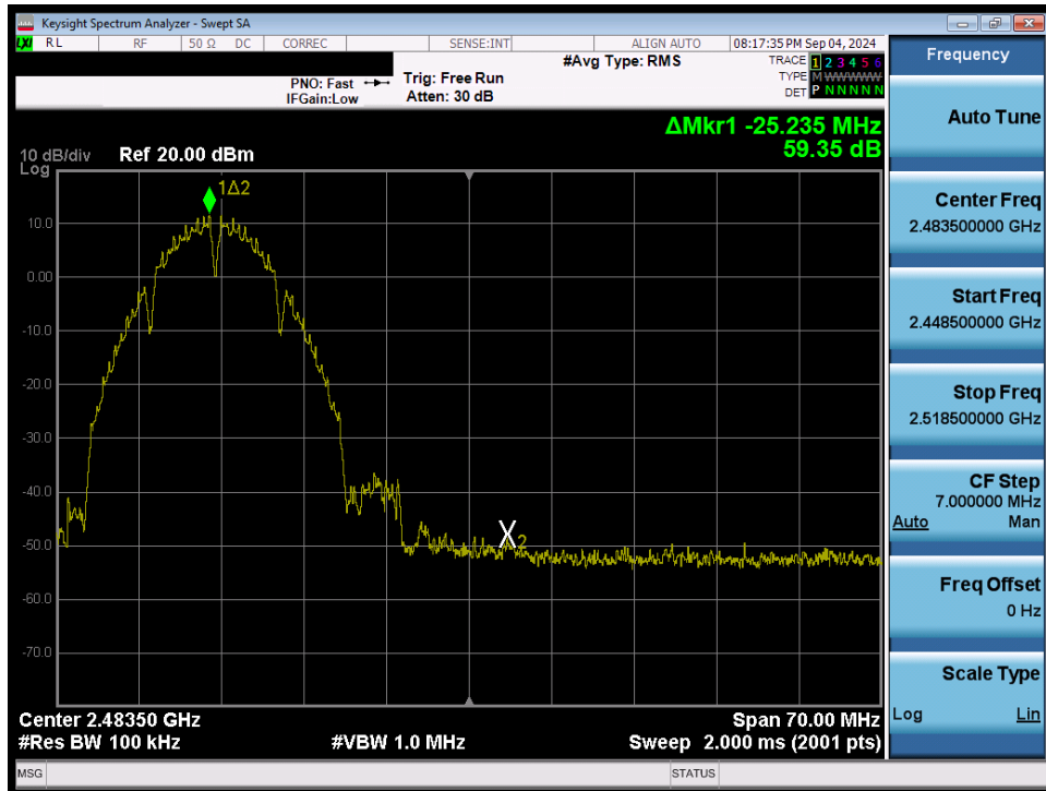
Plot 7-53. Band Edge Plot (802.11b – Ch. 11) SISO ANT1
