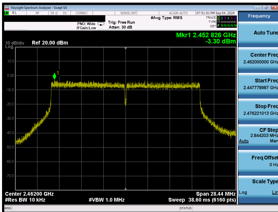
Plot 7-39. Power Spectral Density Plot (802.11ax/be (2.4GHz) – Ch. 11) MIMO ANT1
