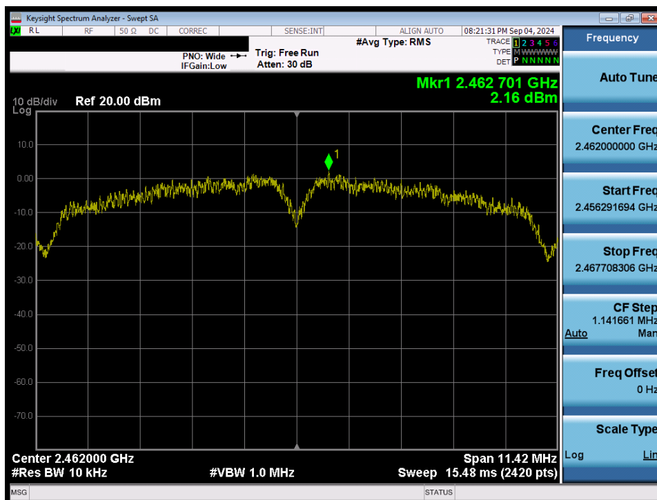
Plot 7-30. Power Spectral Density Plot (802.11b – Ch. 11) SISO ANT1
