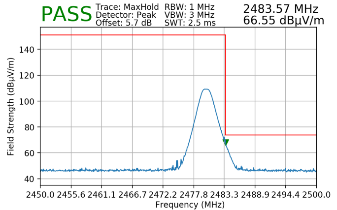
Plot 7-171. Radiated Restricted Upper Band Edge Measurement (Peak) – Ant 2
