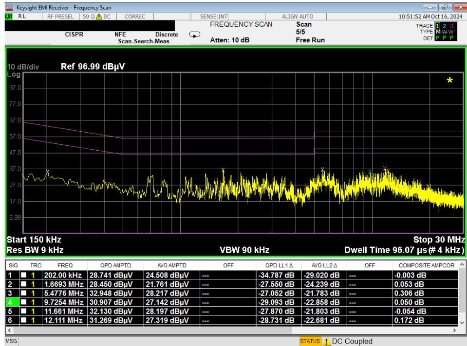
Plot 7-177. Line Conducted Plot with Bluetooth LE (L1)
