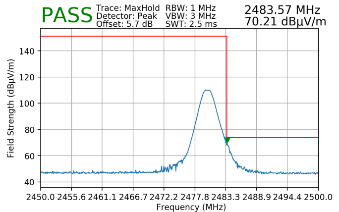
Plot 7-173. Radiated Restricted Upper Band Edge Measurement (Peak) – Dual Ant
