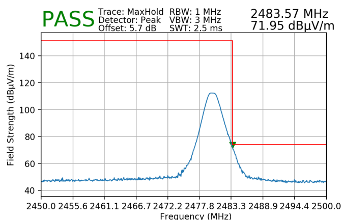
Plot 7-169. Radiated Restricted Upper Band Edge Measurement (Peak) – Ant 1
