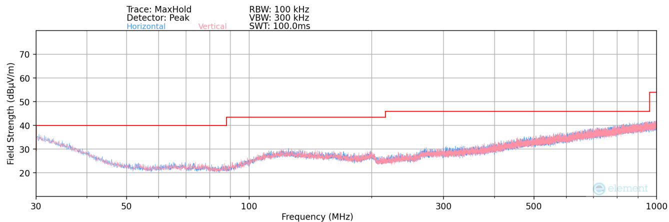
Plot 7-176. Radiated Spurious Plot below 1GHz –Dual Ant
