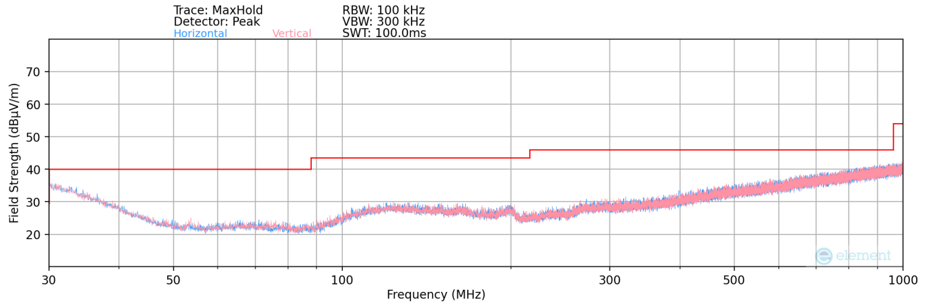
Plot 7-174. Radiated Spurious Plot below 1GHz – Ant 1
