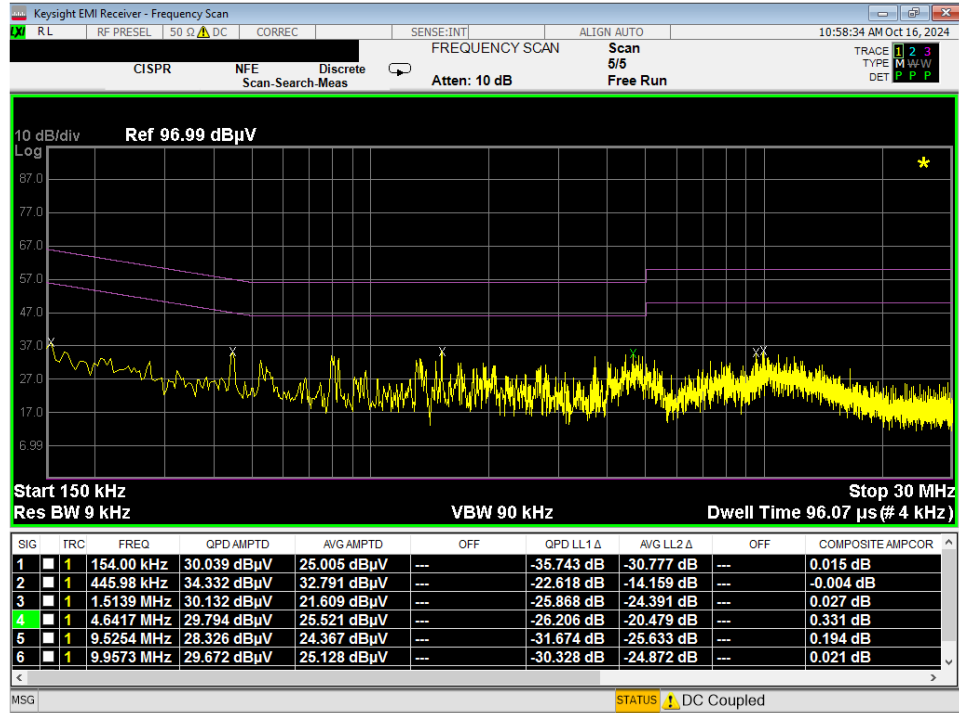
Plot 7-179. Line Conducted Plot with Bluetooth LE (L1) - WCP
