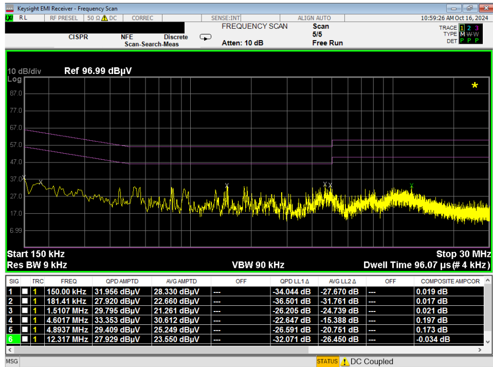
Plot 7-180. Line Conducted Plot with Bluetooth LE (N) - WCP
