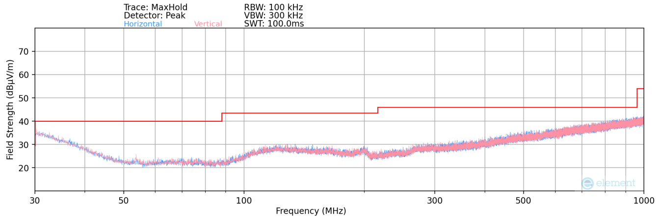
Plot 7-175. Radiated Spurious Plot below 1GHz – Ant 2
