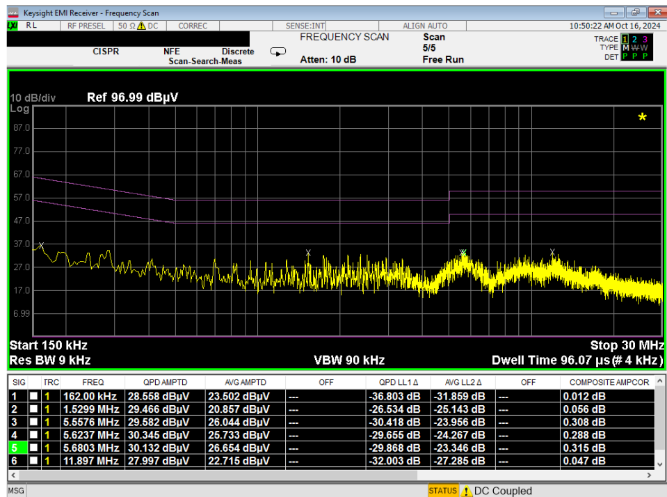
Plot 7-178. Line Conducted Plot with Bluetooth LE (N)
