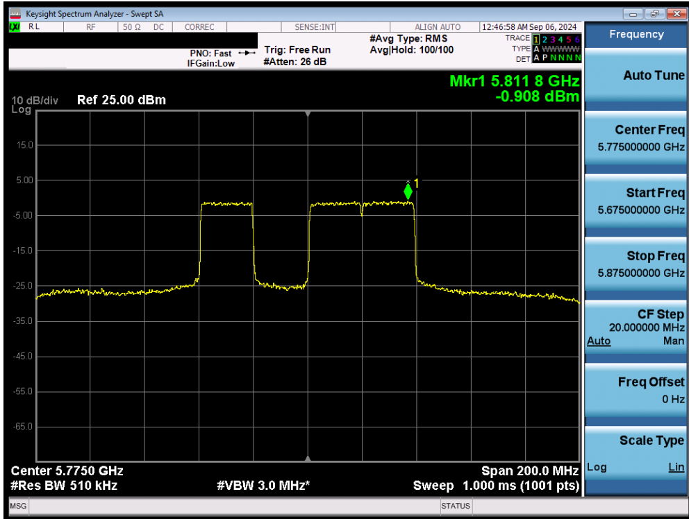
Plot 7-110. Power Spectral Density Plot MIMO ANT2 (80MHz 802.11be (20MHz Puncture) (UNII Band 3) – Ch. 155)
