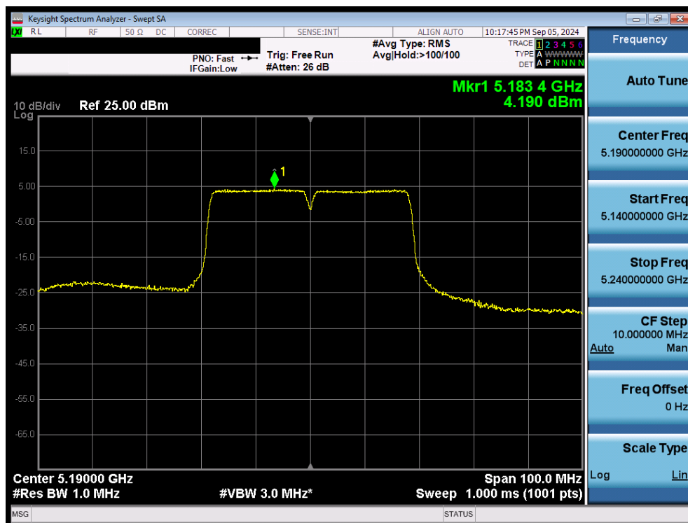
Plot 7-95. Power Spectral Density Plot MIMO ANT2 (40MHz 802.11n (UNII Band 1) – Ch. 38)
