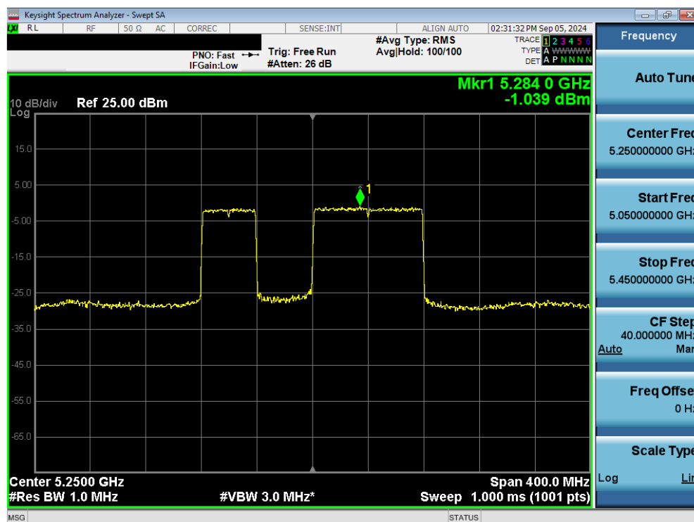
Plot 7-102. Power Spectral Density Plot MIMO ANT2 (160MHz 802.11be (40MHz Puncture) (UNII Band 1/2A) – Ch. 50)
