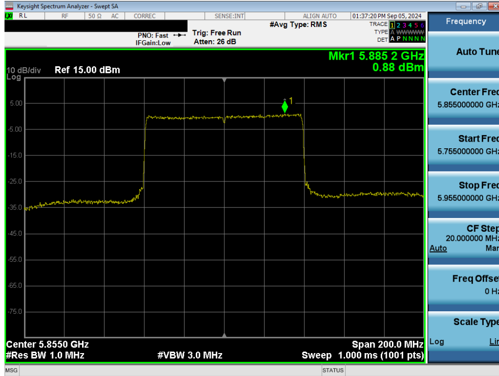
Plot 7-87. Power Spectral Density Plot MIMO ANT1 (80MHz 802.11ax/be (UNII Band 3/4) – Ch. 171)
