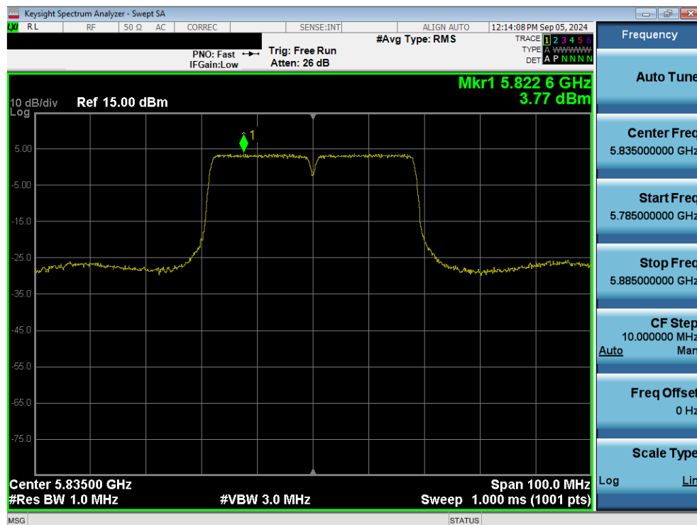
Plot 7-84. Power Spectral Density Plot MIMO ANT1 (40MHz 802.11n (UNII Band 3/4) – Ch. 167)
