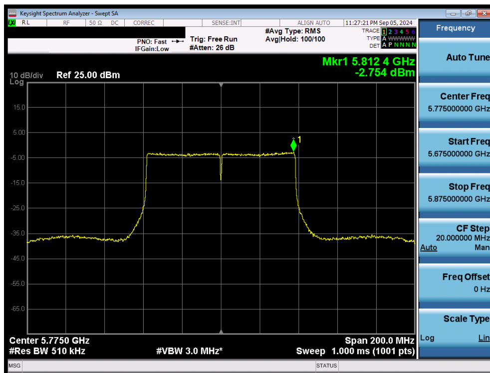
Plot 7-108. Power Spectral Density Plot MIMO ANT2 (80MHz 802.11ac (UNII Band 3) – Ch. 155)
