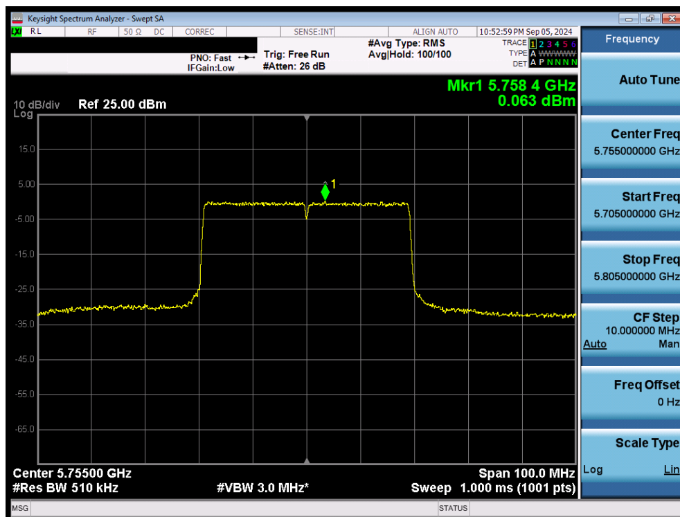
Plot 7-107. Power Spectral Density Plot MIMO ANT2 (40MHz 802.11ax/be (UNII Band 3) – Ch. 151)
