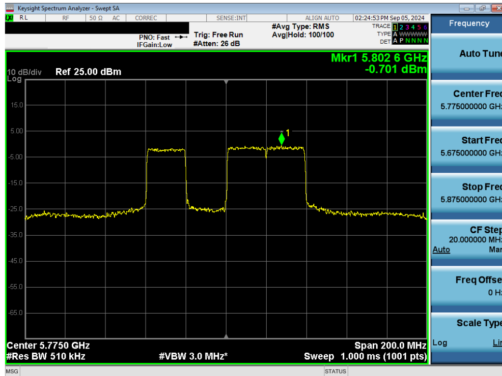
Plot 7-80. Power Spectral Density Plot MIMO ANT1 (80MHz 802.11be (20MHz Puncture) (UNII Band 3) – Ch. 155)
