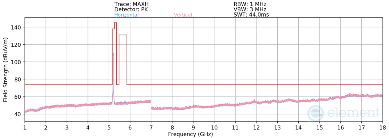
Plot 7-123. Radiated Spurious Plot above 1GHz MIMO (802.11ax – UNII Band 1 Ch. 40)
