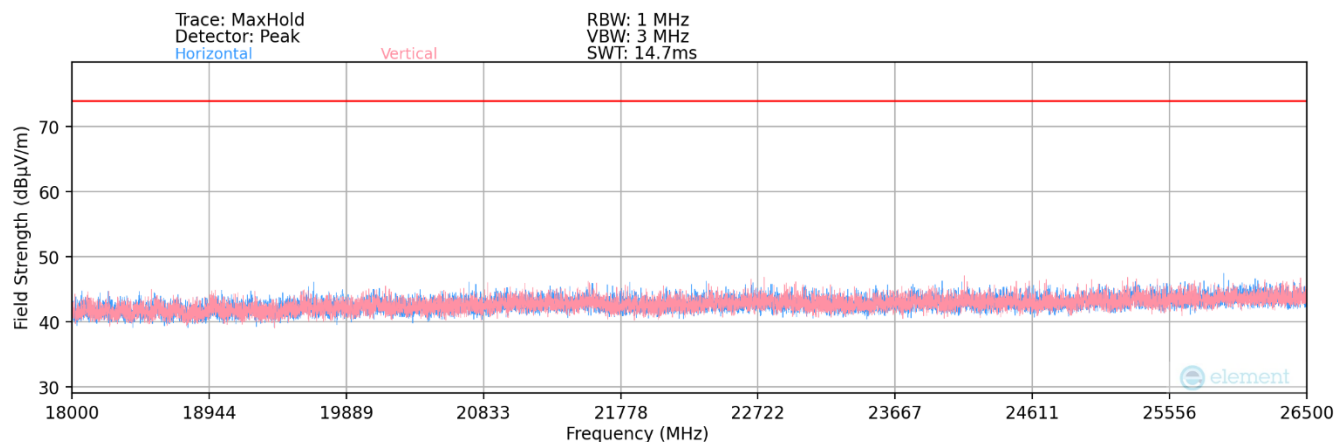
Plot 7-128. Radiated Spurious Plot 18GHz – 26.5GHz MIMO (802.11ax)
