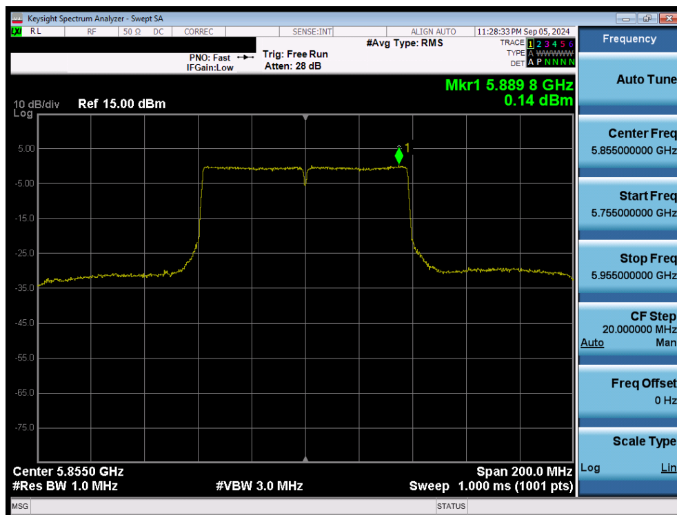
Plot 7-116. Power Spectral Density Plot MIMO ANT2 (80MHz 802.11ac (UNII Band 3/4) – Ch. 171)
