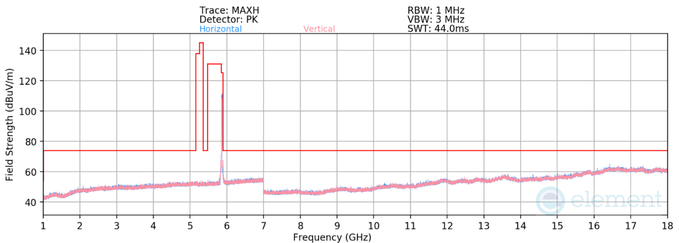
Plot 7-127. Radiated Spurious Plot above 1GHz MIMO (802.11ax – UNII Band 4 Ch. 173)
