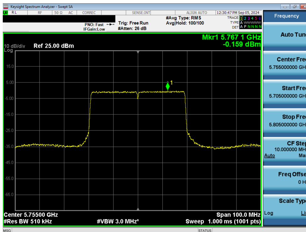
Plot 7-77. Power Spectral Density Plot MIMO ANT1 (40MHz 802.11ax/be (UNII Band 3) – Ch. 151)
