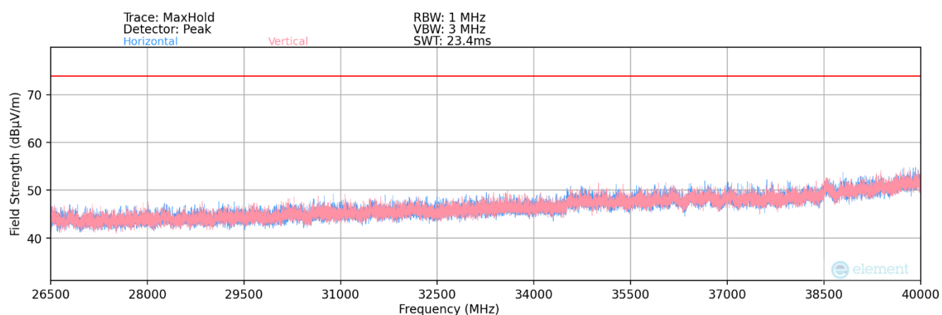
Plot 7-129. Radiated Spurious Plot 26.5GHz – 40GHz MIMO (802.11ax)
