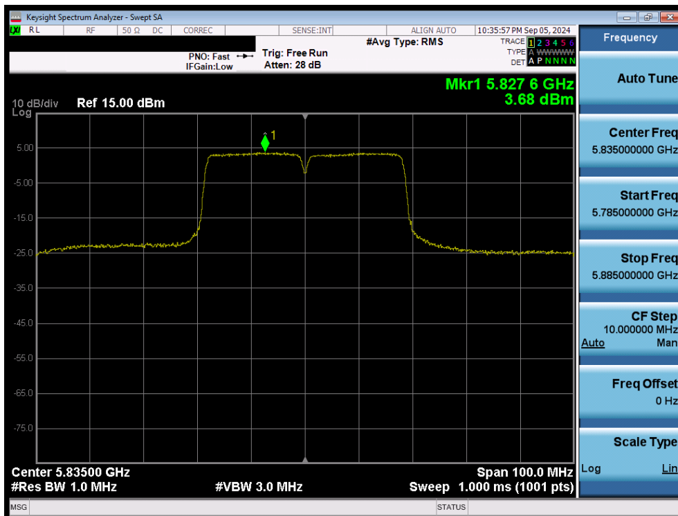
Plot 7-114. Power Spectral Density Plot MIMO ANT2 (40MHz 802.11n (UNII Band 3/4) – Ch. 167)
