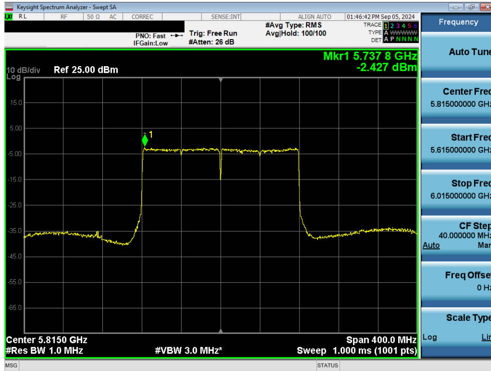
Plot 7-89. Power Spectral Density Plot MIMO ANT1 (160MHz 802.11ax/be (UNII Band 3/4) – Ch. 163)
