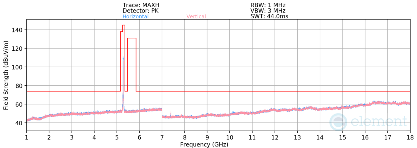
Plot 7-124. Radiated Spurious Plot above 1GHz MIMO (802.11ax – UNII Band 2A Ch. 56)
