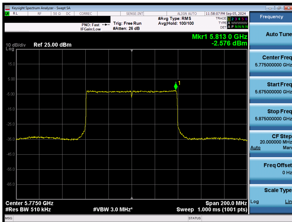
Plot 7-109. Power Spectral Density Plot MIMO ANT2 (80MHz 802.11ax/be (UNII Band 3) – Ch. 155)
