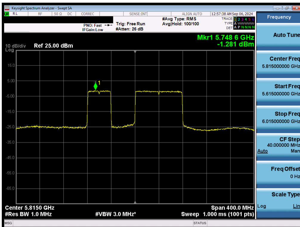
Plot 7-121. Power Spectral Density Plot MIMO ANT2 (160MHz 802.11be (40MHz Puncture) (UNII Band 3/4) – Ch. 163)
