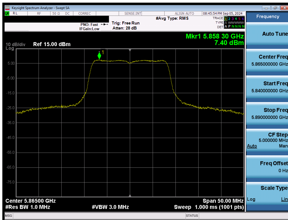
Plot 7-111. Power Spectral Density Plot MIMO ANT2 (20MHz 802.11a (UNII Band 4) – Ch.173)
