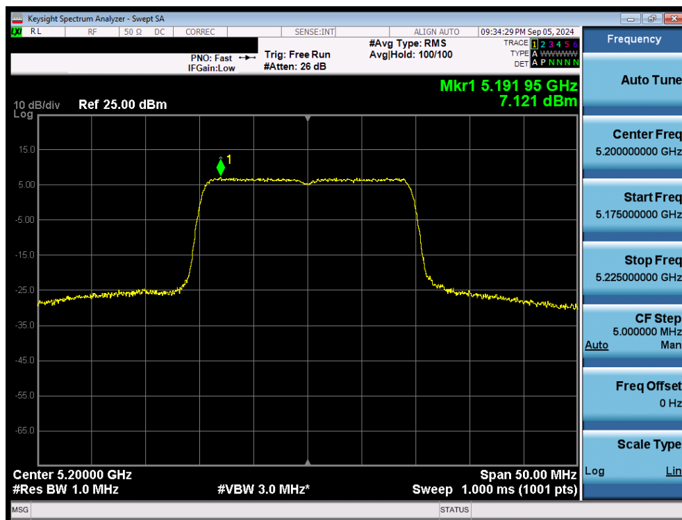
Plot 7-94. Power Spectral Density Plot MIMO ANT2 (20MHz 802.11ax/be (UNII Band 1) – Ch. 40)
