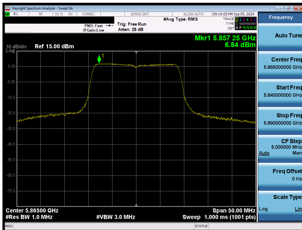
Plot 7-112. Power Spectral Density Plot MIMO ANT2 (20MHz 802.11n (UNII Band 4) – Ch.173)
