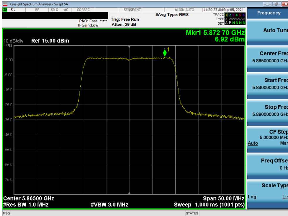
Plot 7-83. Power Spectral Density Plot MIMO ANT1 (20MHz 802.11ax/be (UNII Band 4) – Ch.173)
