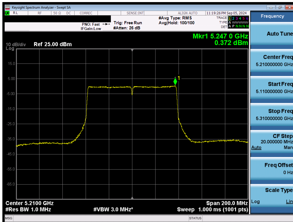
Plot 7-97. Power Spectral Density Plot MIMO ANT2 (80MHz 802.11ac (UNII Band 1) – Ch. 42)
