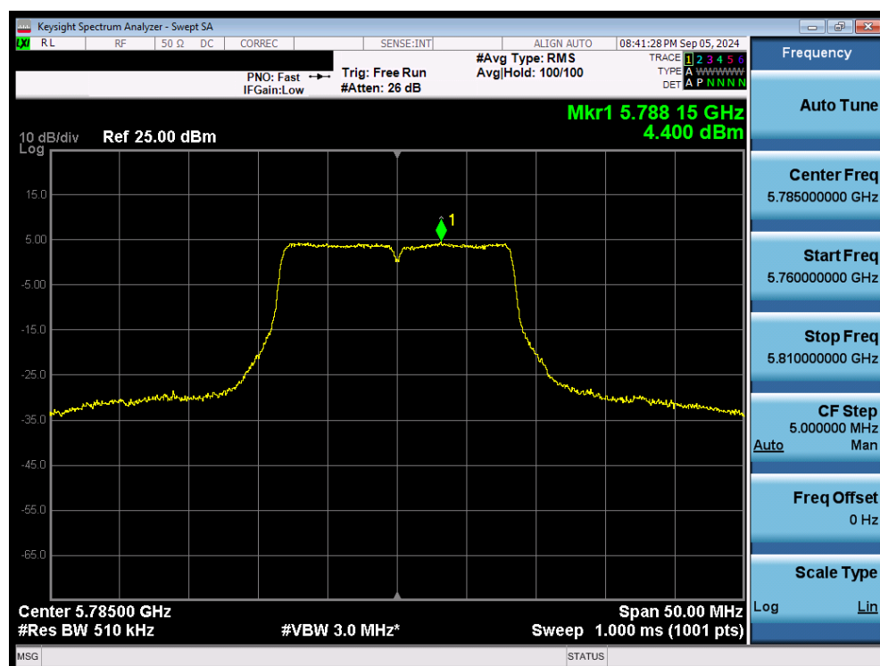
Plot 7-103. Power Spectral Density Plot MIMO ANT2 (20MHz 802.11a (UNII Band 3) – Ch.157)
