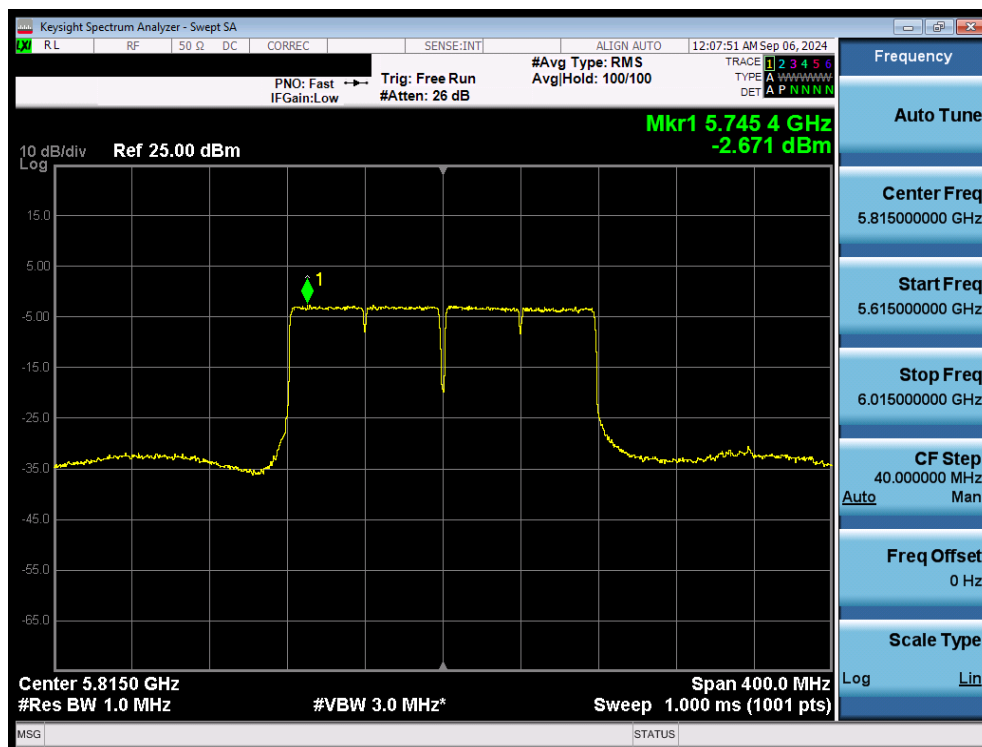
Plot 7-118. Power Spectral Density Plot MIMO ANT2 (160MHz 802.11ac (UNII Band 3/4) – Ch. 163)
