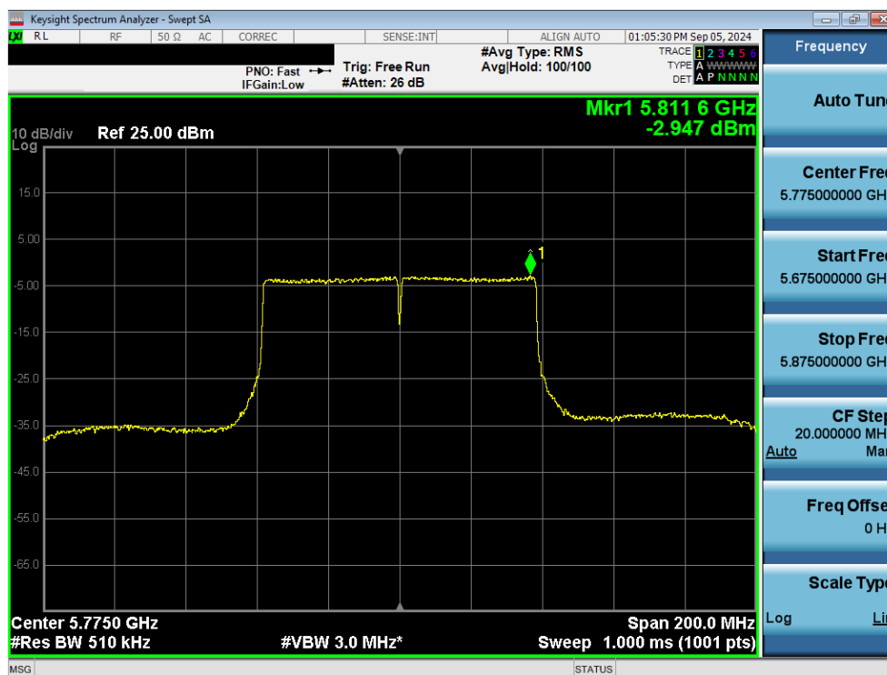
Plot 7-78. Power Spectral Density Plot MIMO ANT1 (80MHz 802.11ac (UNII Band 3) – Ch. 155)
