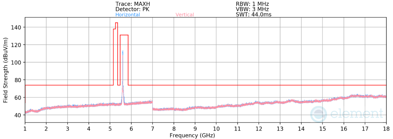
Plot 7-125. Radiated Spurious Plot above 1GHz MIMO (802.11ax – UNII Band 2C Ch. 120)
