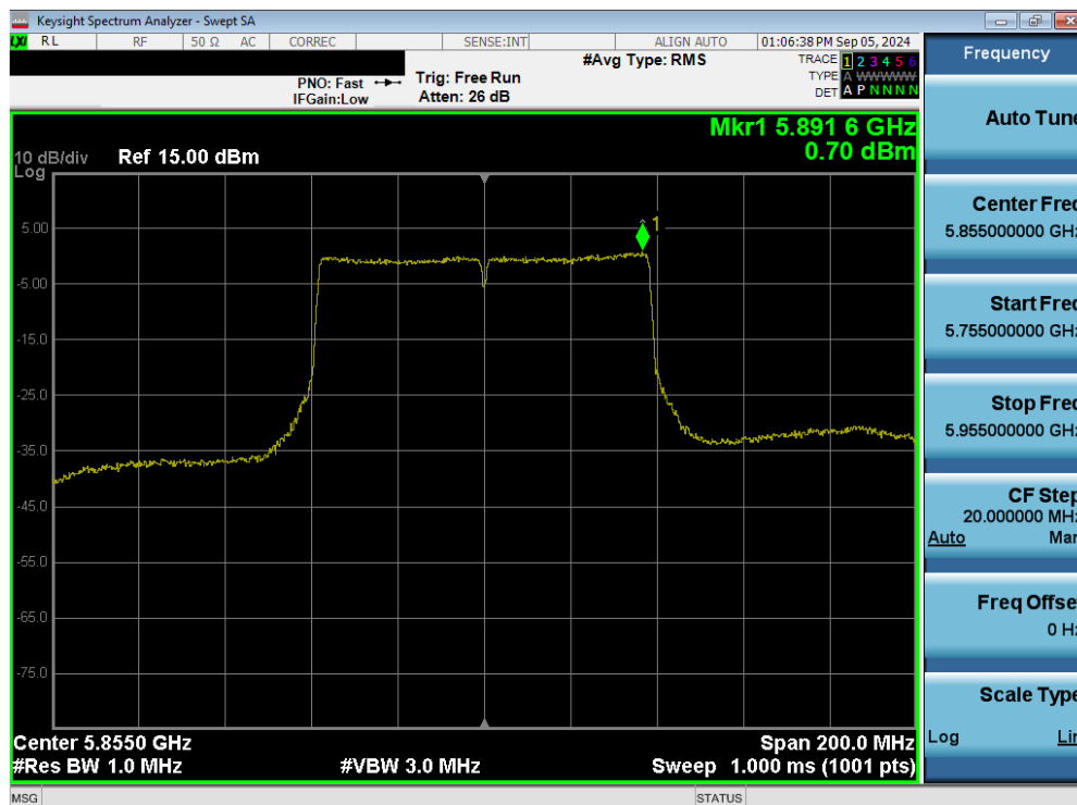
Plot 7-86. Power Spectral Density Plot MIMO ANT1 (80MHz 802.11ac (UNII Band 3/4) – Ch. 171)
