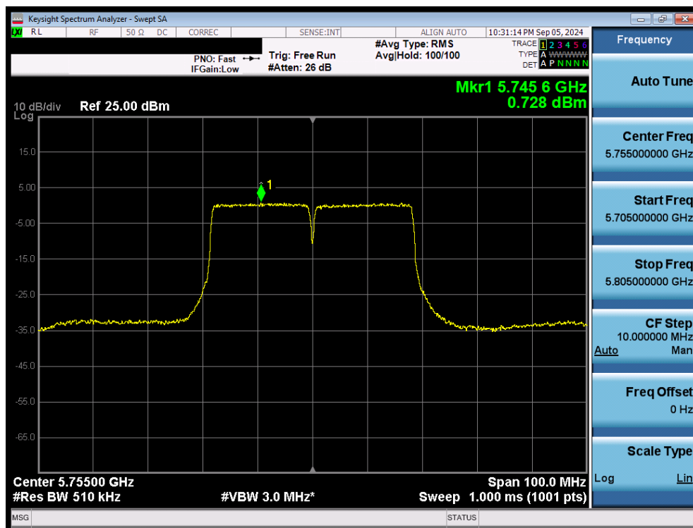
Plot 7-106. Power Spectral Density Plot MIMO ANT2 (40MHz 802.11n (UNII Band 3) – Ch. 151)
