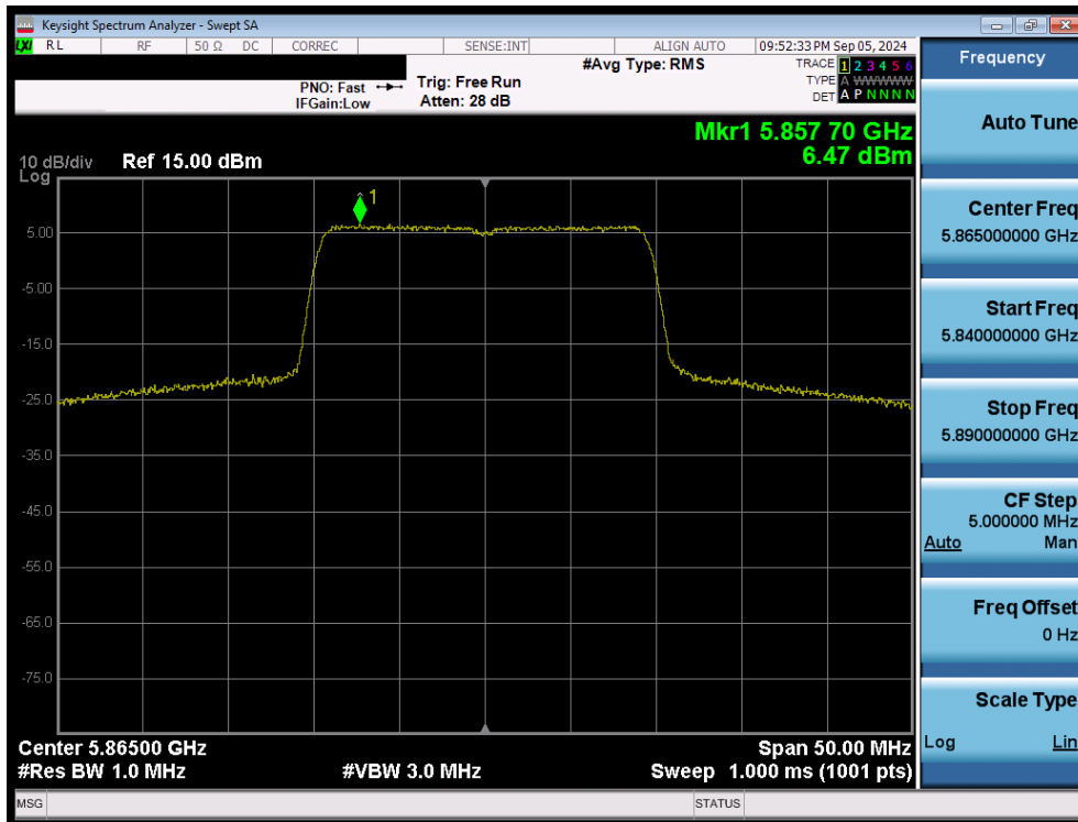
Plot 7-113. Power Spectral Density Plot MIMO ANT2 (20MHz 802.11ax/be (UNII Band 4) – Ch.173)
