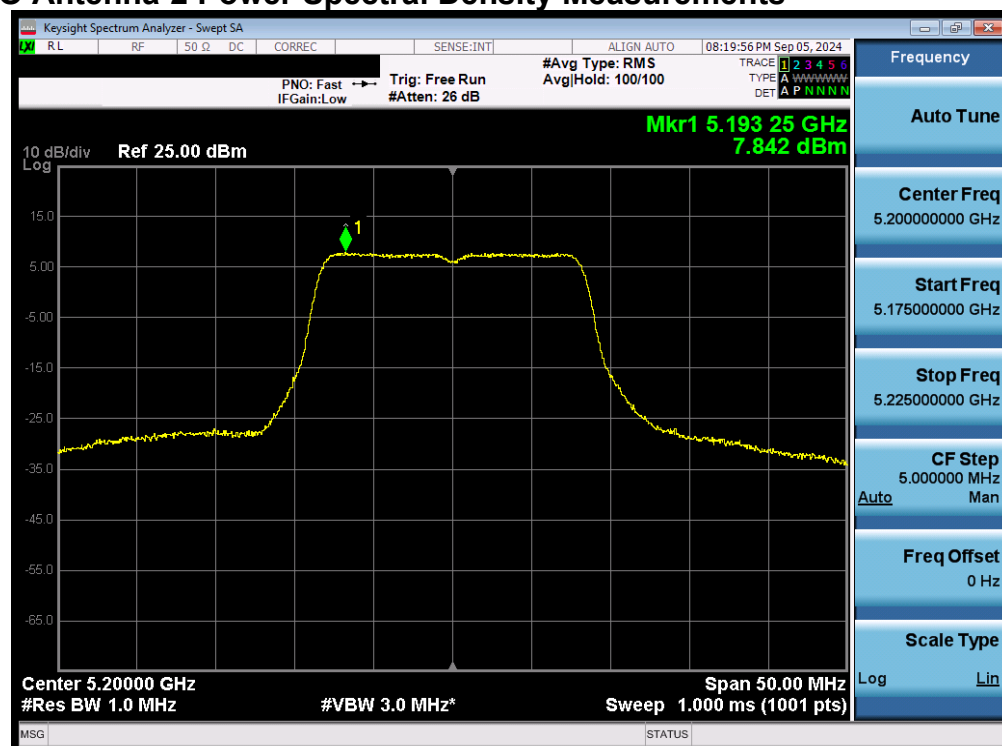
Plot 7-92. Power Spectral Density Plot MIMO ANT2 (20MHz 802.11a (UNII Band 1) – Ch. 40)
