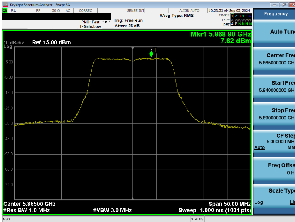
Plot 7-81. Power Spectral Density Plot MIMO ANT1 (20MHz 802.11a (UNII Band 4) – Ch.173)
