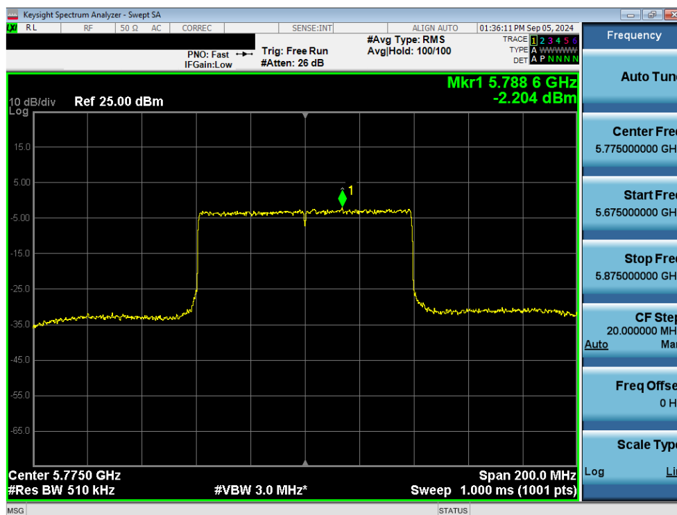
Plot 7-79. Power Spectral Density Plot MIMO ANT1 (80MHz 802.11ax/be (UNII Band 3) – Ch. 155)
