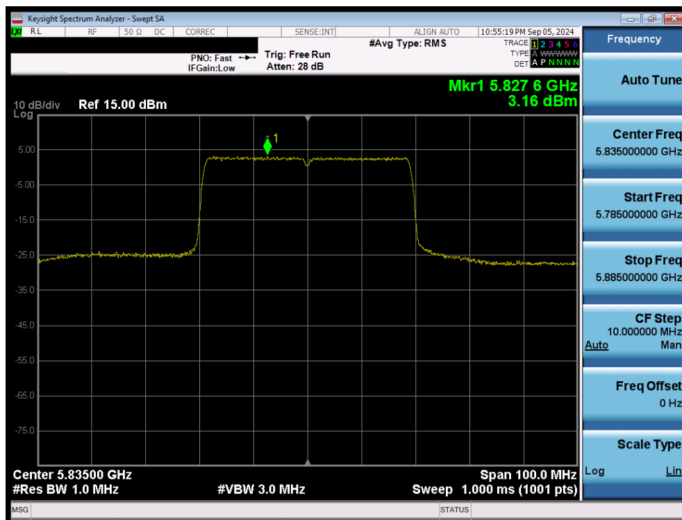
Plot 7-115. Power Spectral Density Plot MIMO ANT2 (40MHz 802.11ax/be (UNII Band 3/4) – Ch. 167)
