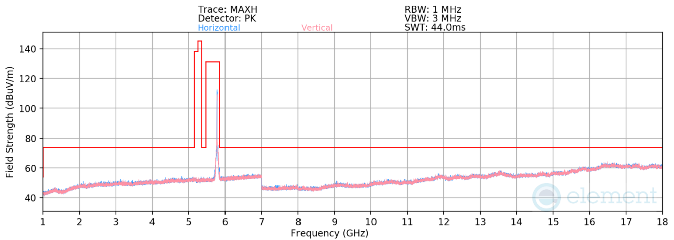
Plot 7-126. Radiated Spurious Plot above 1GHz MIMO (802.11ax – UNII Band 3 Ch. 157)
