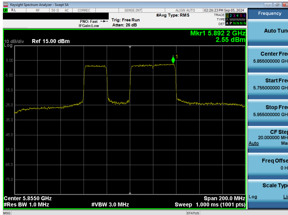
Plot 7-90. Power Spectral Density Plot MIMO ANT1 (80MHz 802.11be (20MHz Puncture) (UNII Band 3/4) – Ch. 171)
