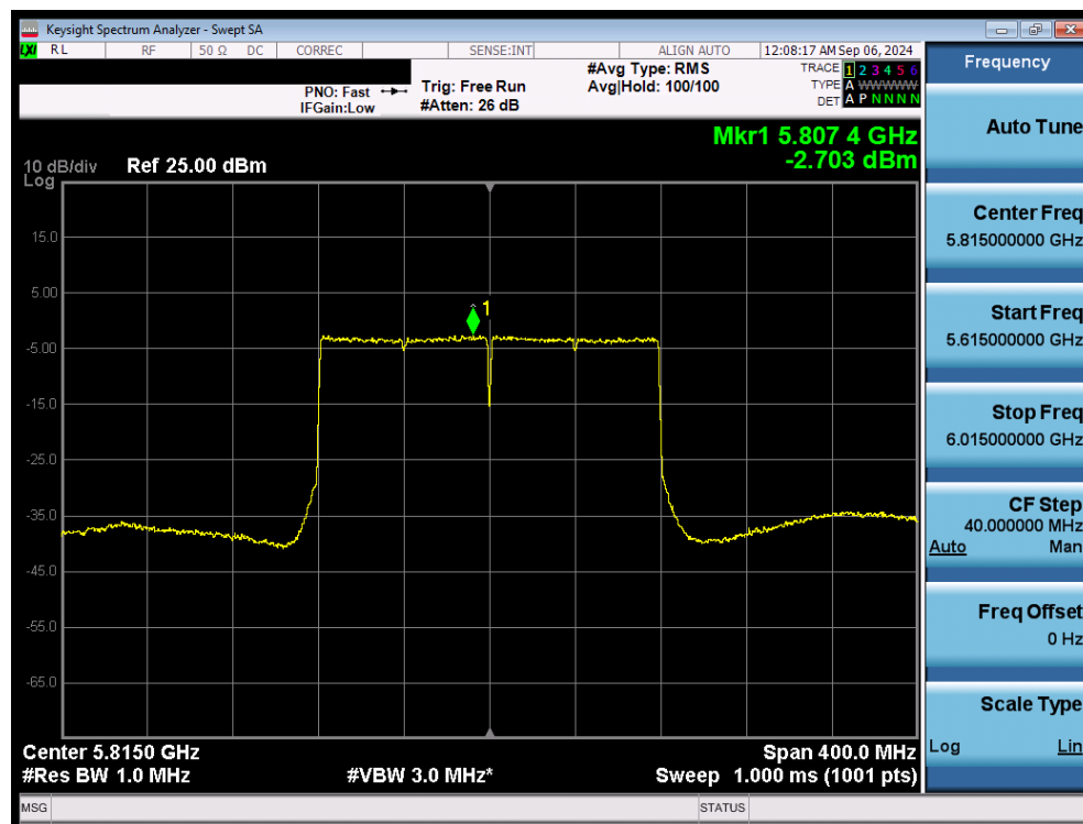
Plot 7-119. Power Spectral Density Plot MIMO ANT2 (160MHz 802.11ax/be (UNII Band 3/4) – Ch. 163)
