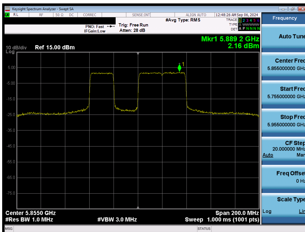
Plot 7-120. Power Spectral Density Plot MIMO ANT2 (80MHz 802.11be (20MHz Puncture) (UNII Band 3/4) – Ch. 171)
