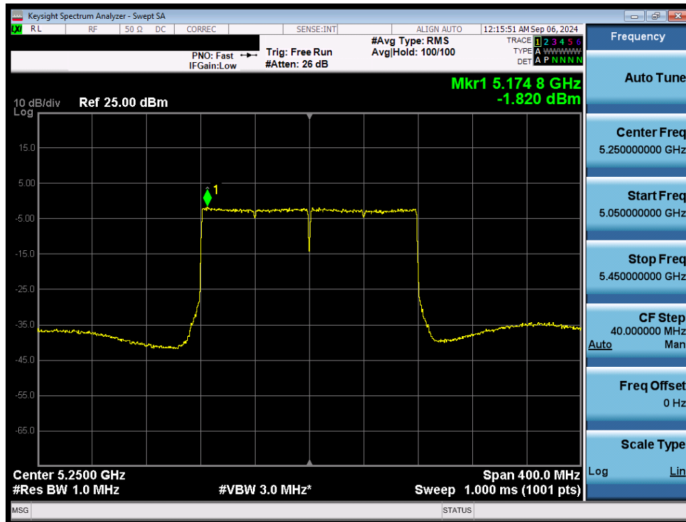
Plot 7-100. Power Spectral Density Plot MIMO ANT2 (160MHz 802.11ax/be (UNII Band 1/2A) – Ch. 50)
