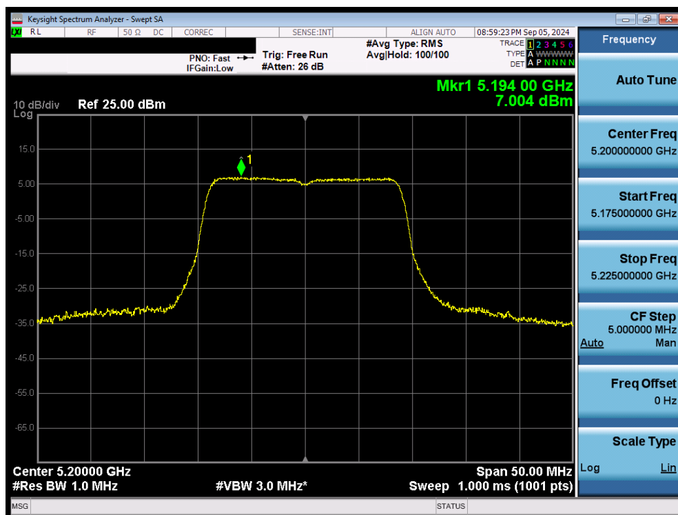
Plot 7-93. Power Spectral Density Plot MIMO ANT2 (20MHz 802.11n (UNII Band 1) – Ch. 40)
