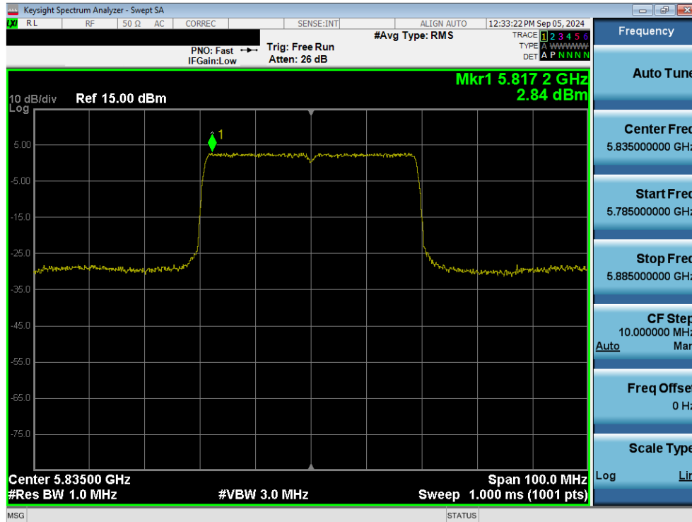
Plot 7-85. Power Spectral Density Plot MIMO ANT1 (40MHz 802.11ax/be (UNII Band 3/4) – Ch. 167)
