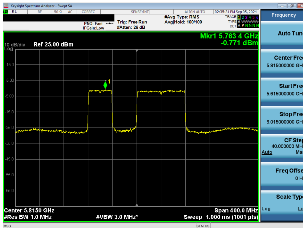
Plot 7-91. Power Spectral Density Plot MIMO ANT1 (160MHz 802.11be (40MHz Puncture) (UNII Band 3/4) – Ch. 163)
