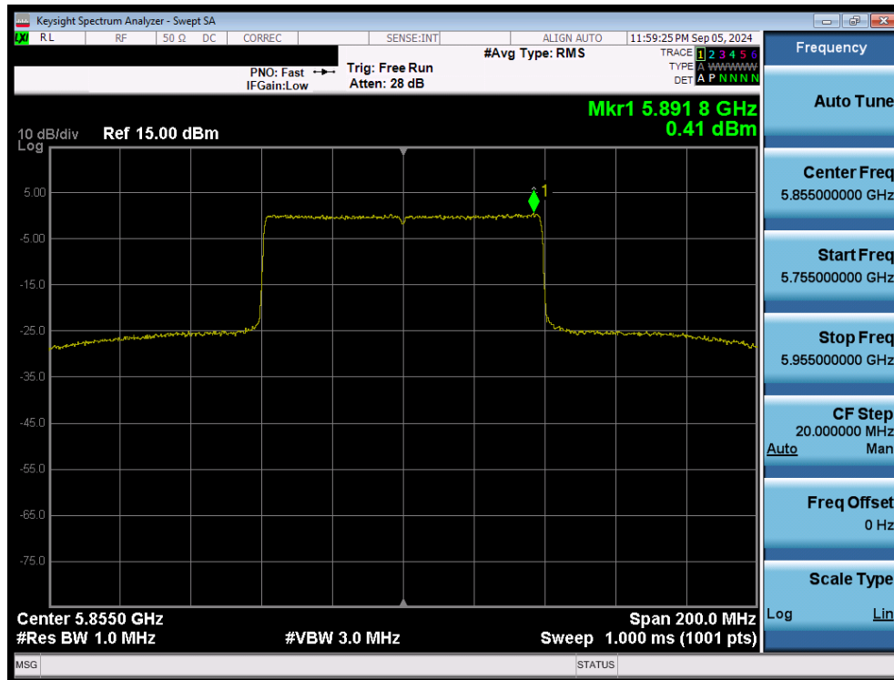
Plot 7-117. Power Spectral Density Plot MIMO ANT2 (80MHz 802.11ax/be (UNII Band 3/4) – Ch. 171)
