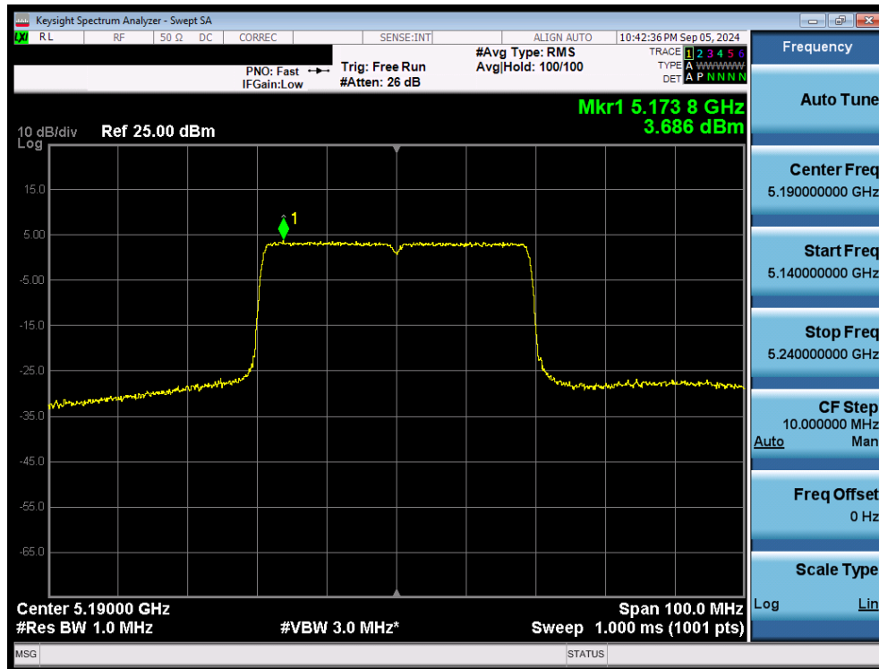
Plot 7-96. Power Spectral Density Plot MIMO ANT2 (40MHz 802.11ax/be (UNII Band 1) – Ch. 38)
