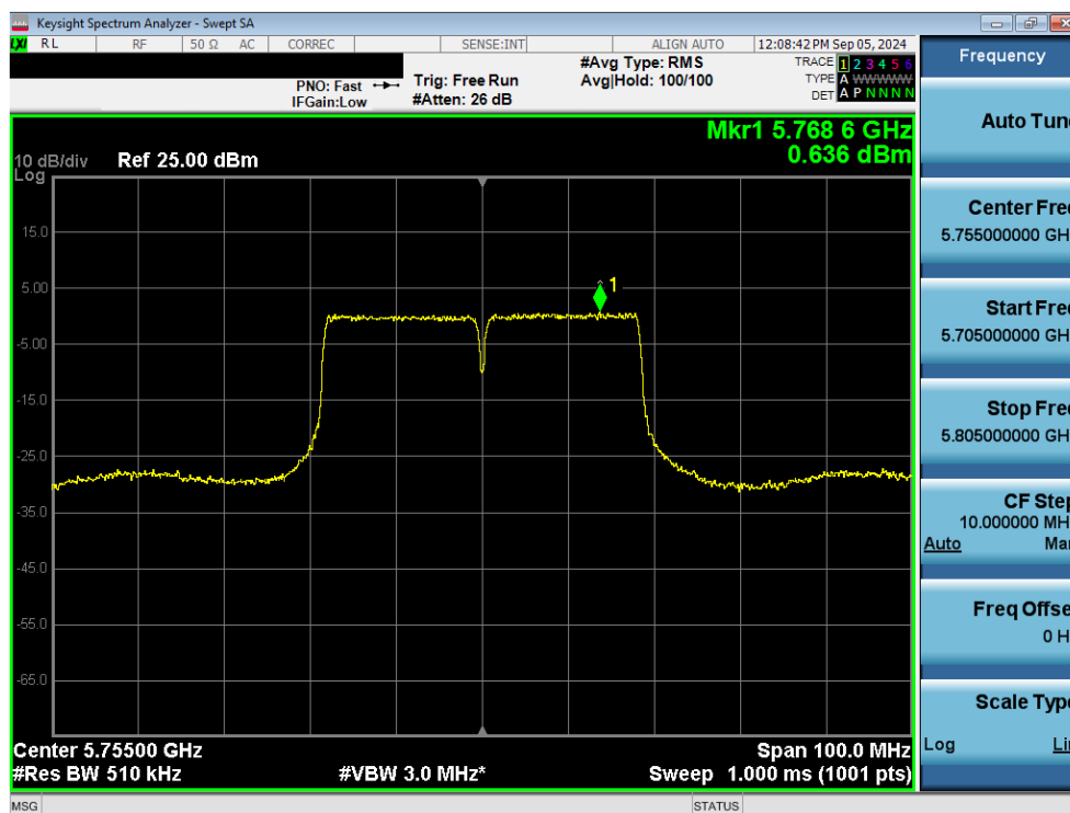
Plot 7-76. Power Spectral Density Plot MIMO ANT1 (40MHz 802.11n (UNII Band 3) – Ch. 151)
