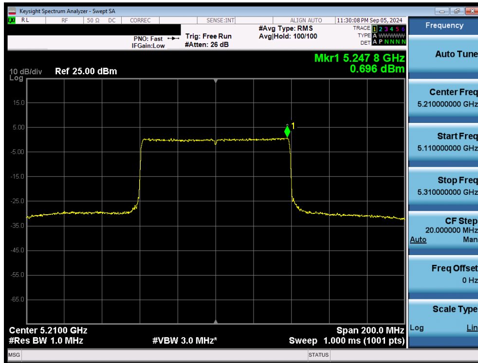
Plot 7-98. Power Spectral Density Plot MIMO ANT2 (80MHz 802.11ax/be (UNII Band 1) – Ch. 42)
