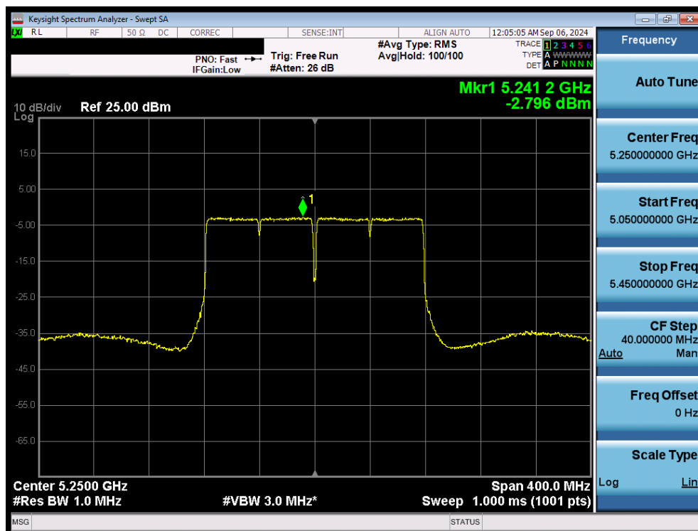
Plot 7-99. Power Spectral Density Plot MIMO ANT2 (160MHz 802.11ac (UNII Band 1/2A) – Ch. 50)
