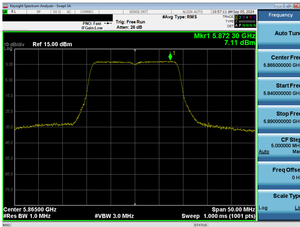
Plot 7-82. Power Spectral Density Plot MIMO ANT1 (20MHz 802.11n (UNII Band 4) – Ch.173)
