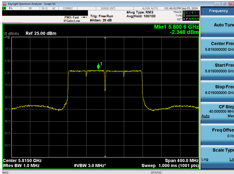
Plot 7-88. Power Spectral Density Plot MIMO ANT1 (160MHz 802.11ac (UNII Band 3/4) – Ch. 163)
