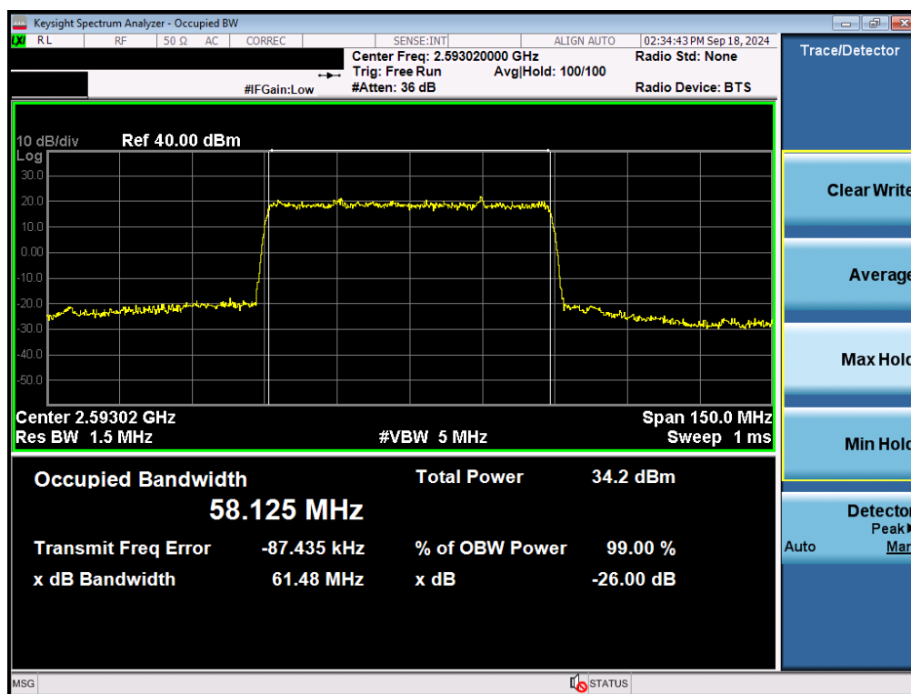
Plot 7-99. Occupied Bandwidth Plot (NR Band n41 - 60MHz \pi/2 BPSK - Full RB - Ant B)
