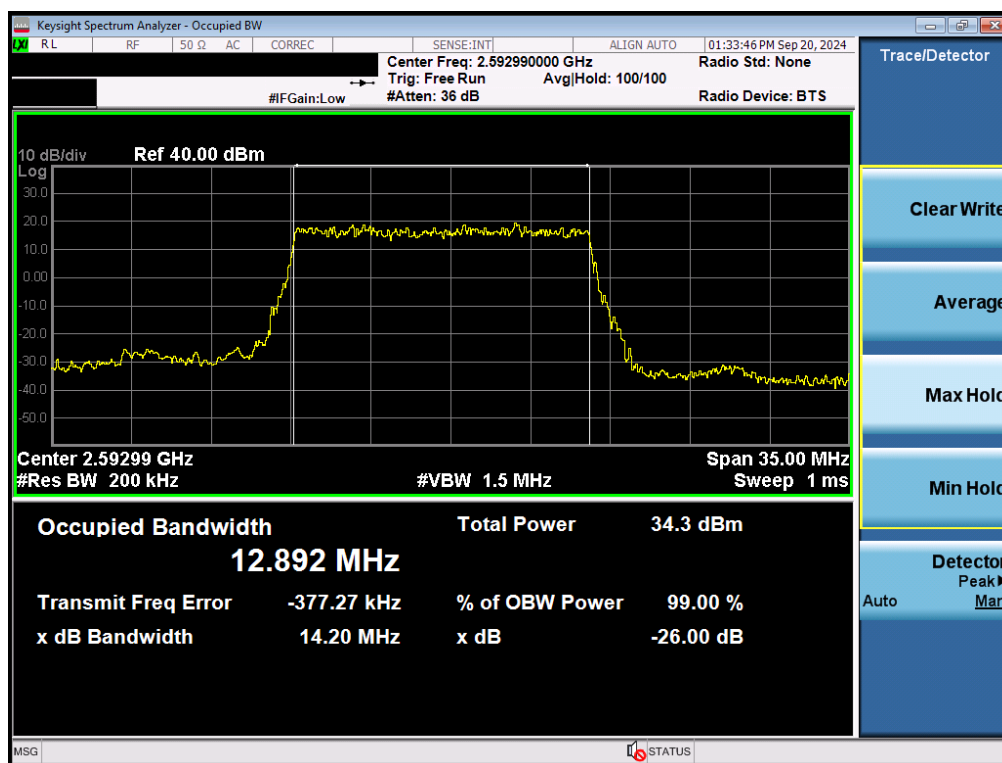
Plot 7-123. Occupied Bandwidth Plot (NR Band n41 - 15MHz \pi/2 BPSK - Full RB - Ant B)
