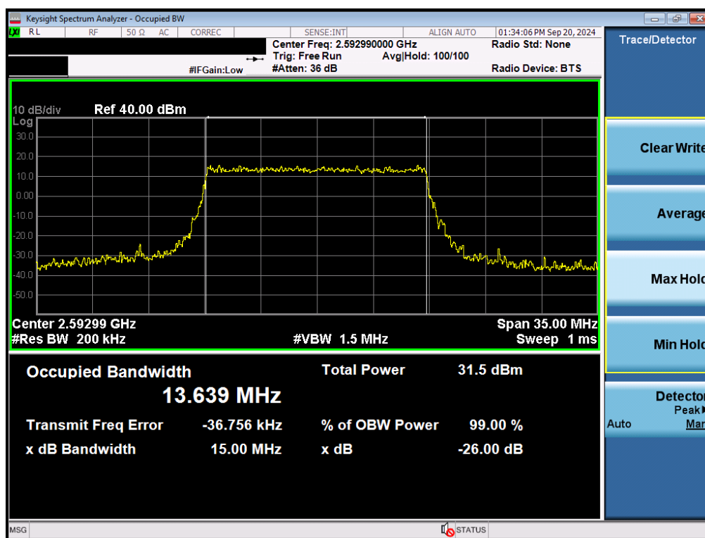
Plot 7-124. Occupied Bandwidth Plot (NR Band n41 - 15MHz QPSK - Full RB - Ant B)
