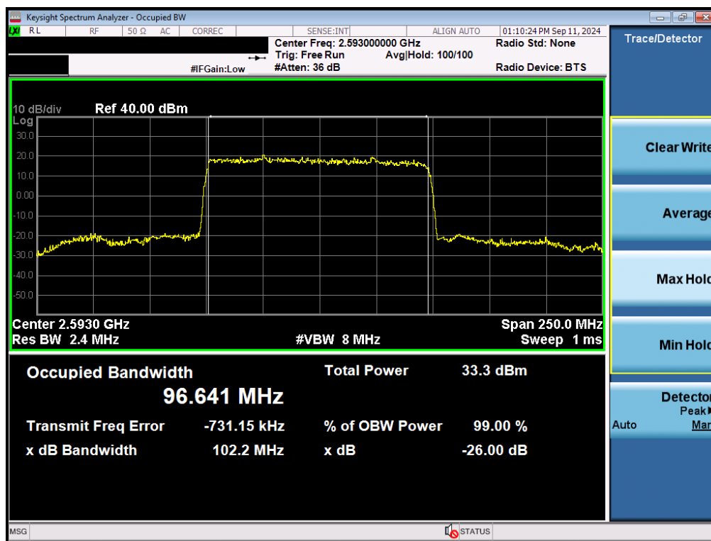
Plot 7-138. Occupied Bandwidth Plot (NR Band n41 - 100MHz \pi/2 BPSK - Full RB - Ant D)
