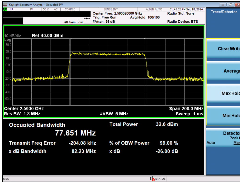
Plot 7-95. Occupied Bandwidth Plot (NR Band n41 - 80MHz 16-QAM - Full RB - Ant B)
