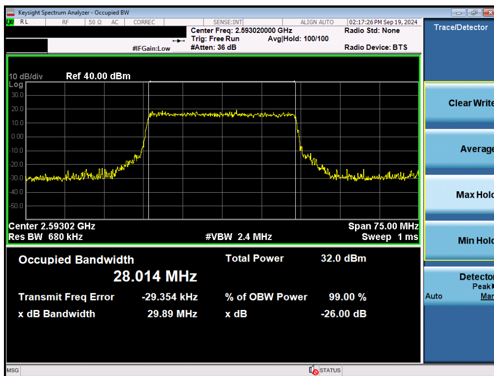
Plot 7-115. Occupied Bandwidth Plot (NR Band n41 - 30MHz QPSK - Full RB - Ant B)
