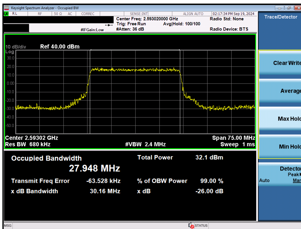
Plot 7-116. Occupied Bandwidth Plot (NR Band n41 - 30MHz 16-QAM - Full RB - Ant B)
