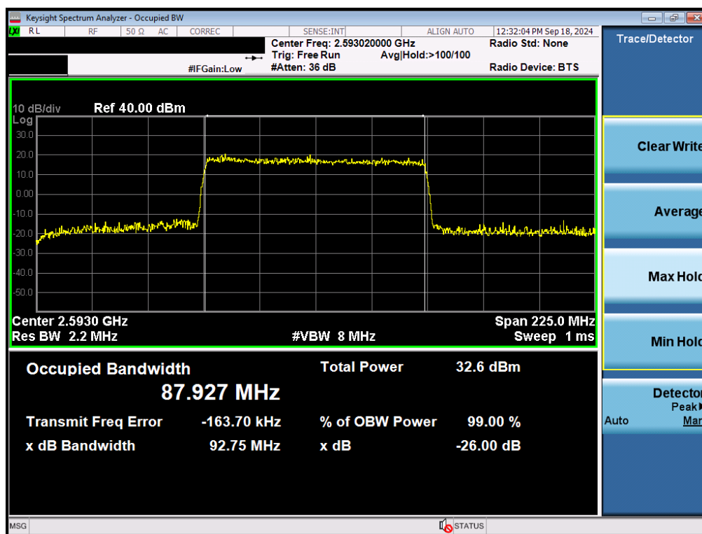
Plot 7-91. Occupied Bandwidth Plot (NR Band n41 - 90MHz QPSK - Full RB - Ant B)
