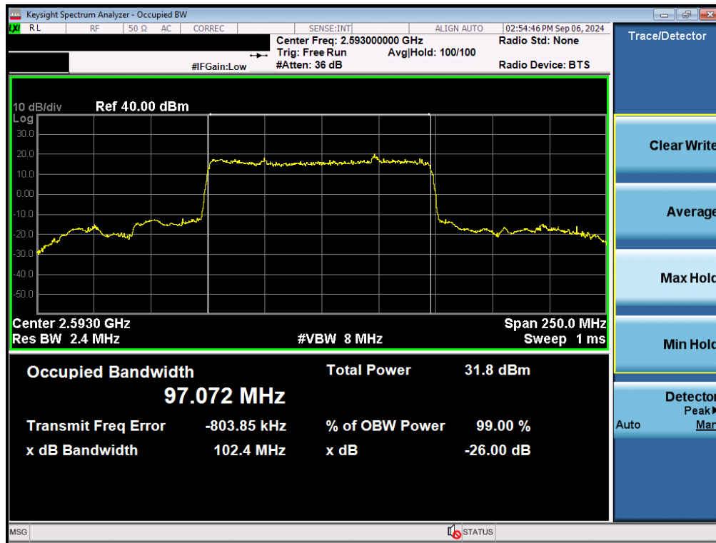
Plot 7-129. Occupied Bandwidth Plot (NR Band n41 - 100MHz \pi/2 BPSK - Full RB - Ant B)
