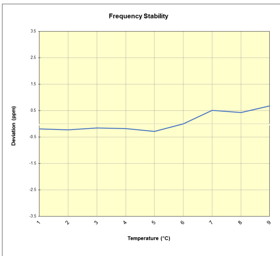
Plot 7-199. LTE Band 66/4 Frequency Stability Chart
