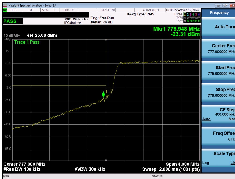
Plot 7-137. Lower Band Edge Plot (LTE Band 13 - 5MHz QPSK – Full RB - ANT1)
