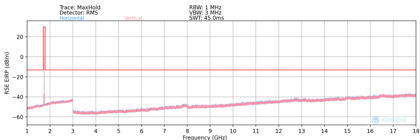
Plot 7-185. Radiated Spurious Plot (LTE Band 66/4) – Ant1
