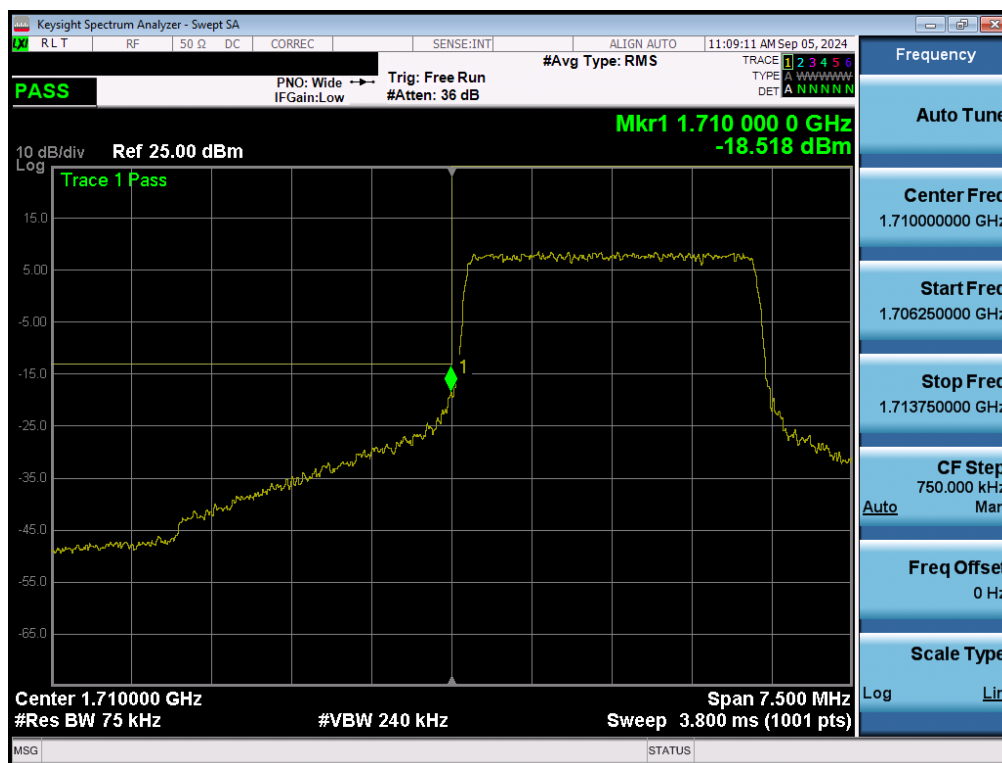
Plot 7-141. Lower Band Edge Plot (LTE Band 66/4 - 3MHz QPSK – Full RB - ANT1)
