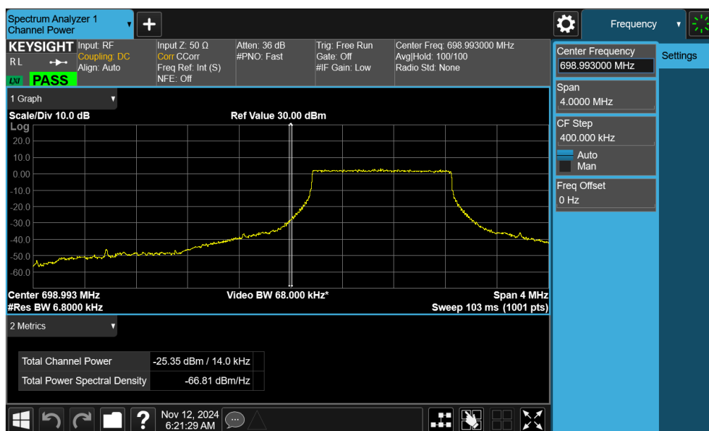
Plot 7-135. Lower Band Edge Plot (LTE Band 12/17 – 1.4MHz QPSK – Full RB - ANT1)
