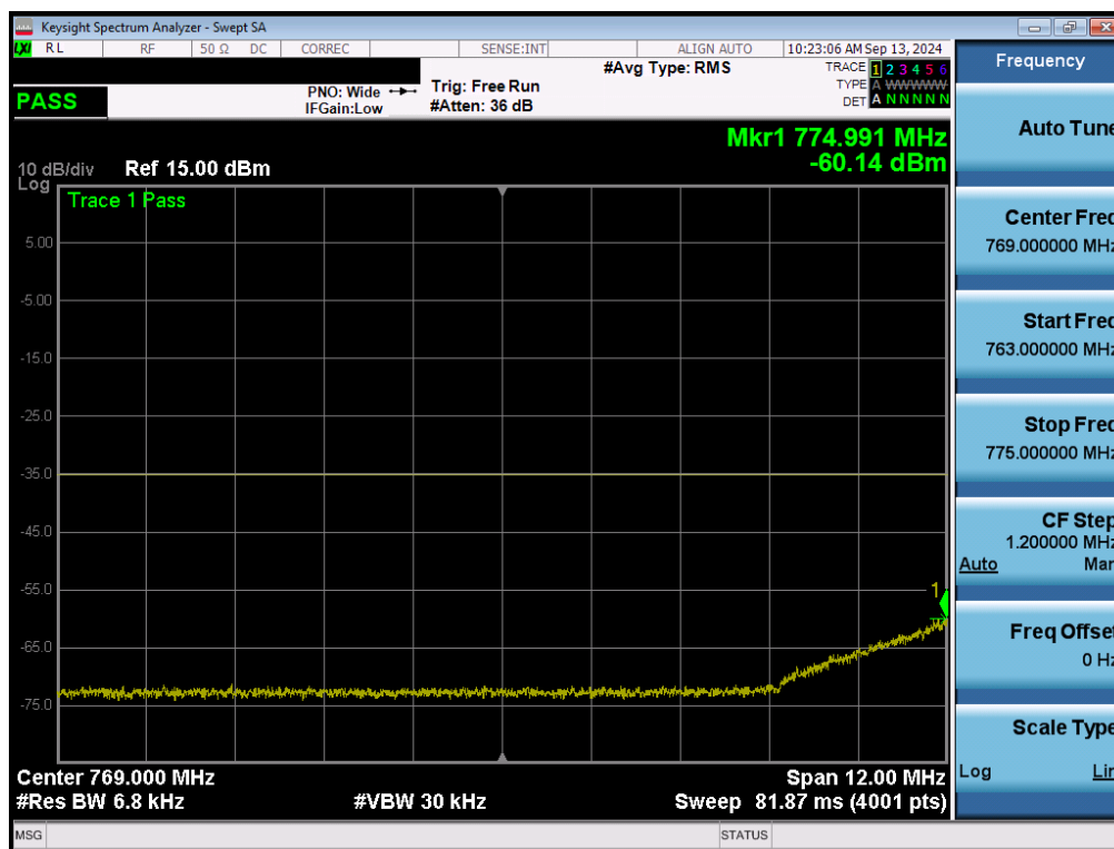
Plot 7-154. Lower Emission Mask Plot (LTE Band 13 - 5MHz QPSK – Full RB - ANT2)
