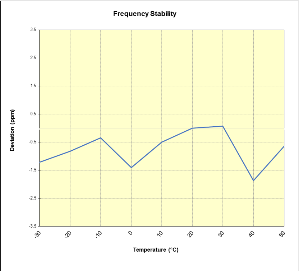
Plot 7-201. NR Band n66 Frequency Stability Chart
