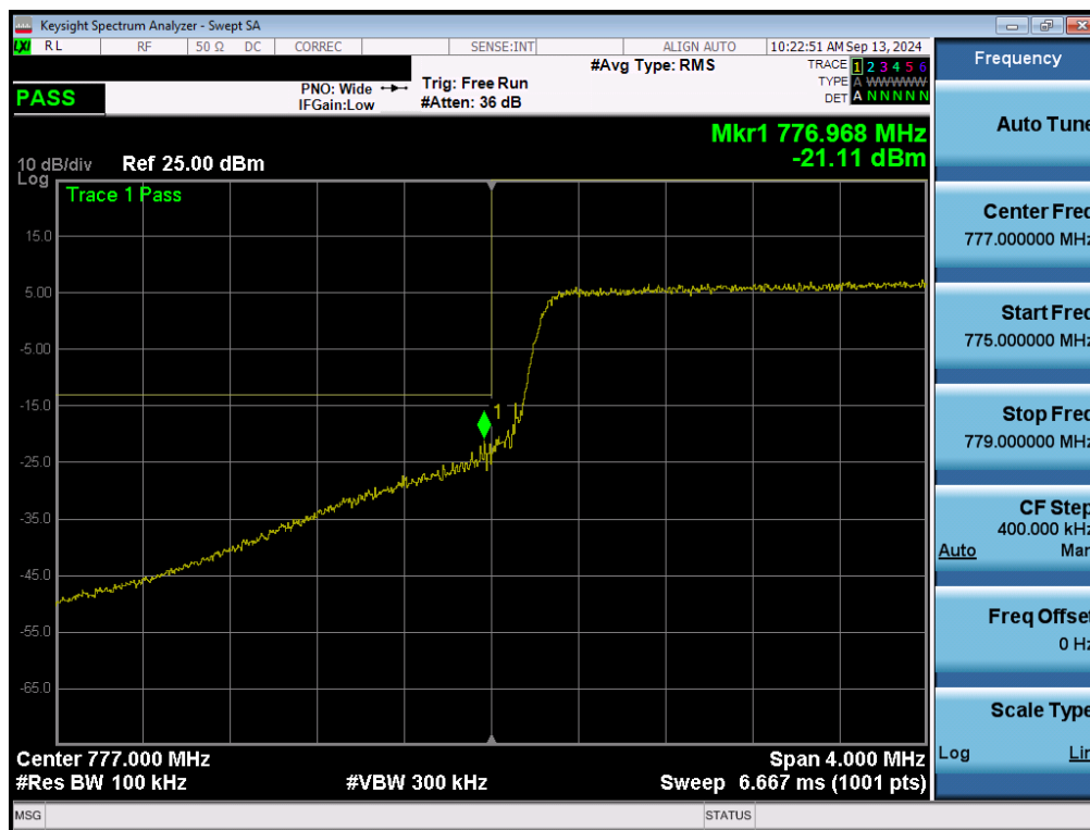
Plot 7-153. Lower Band Edge Plot (LTE Band 13 - 5MHz QPSK – Full RB - ANT2)
