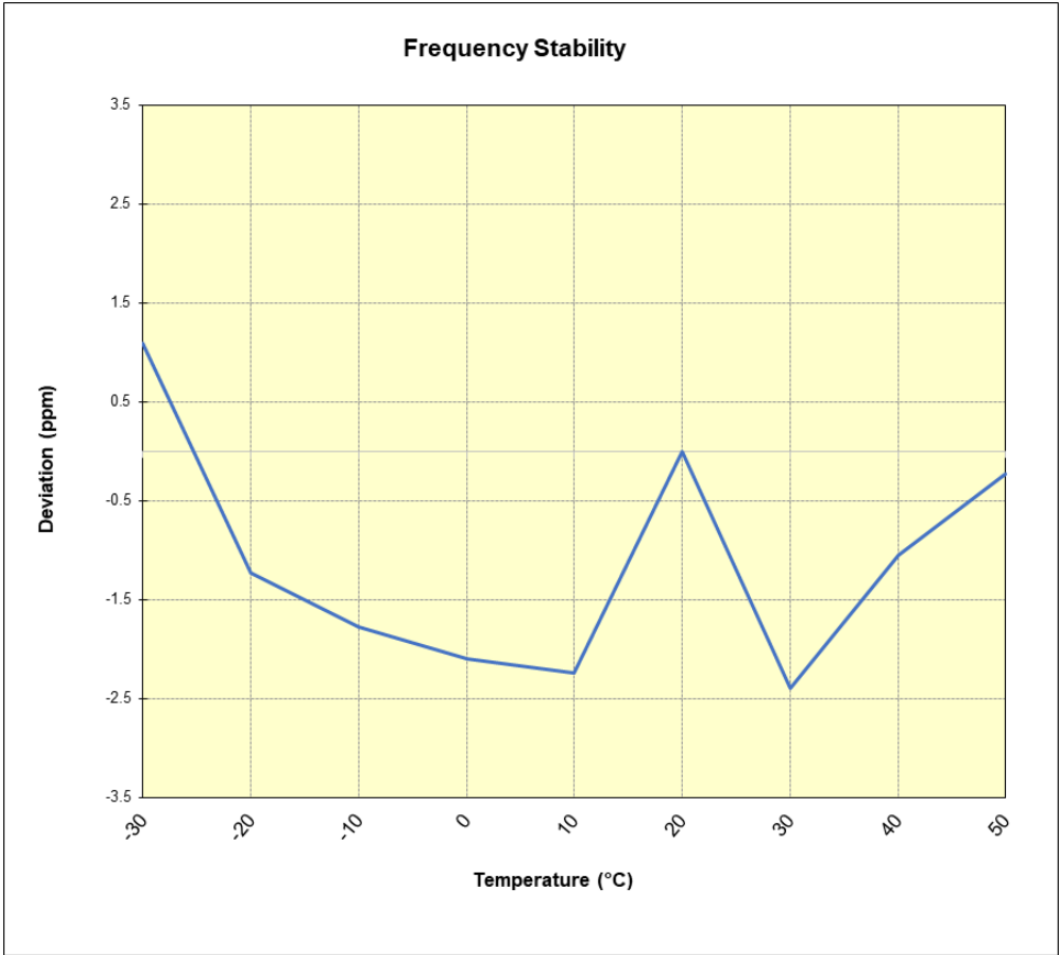
Plot 7-197. LTE Band 12 Frequency Stability Chart
