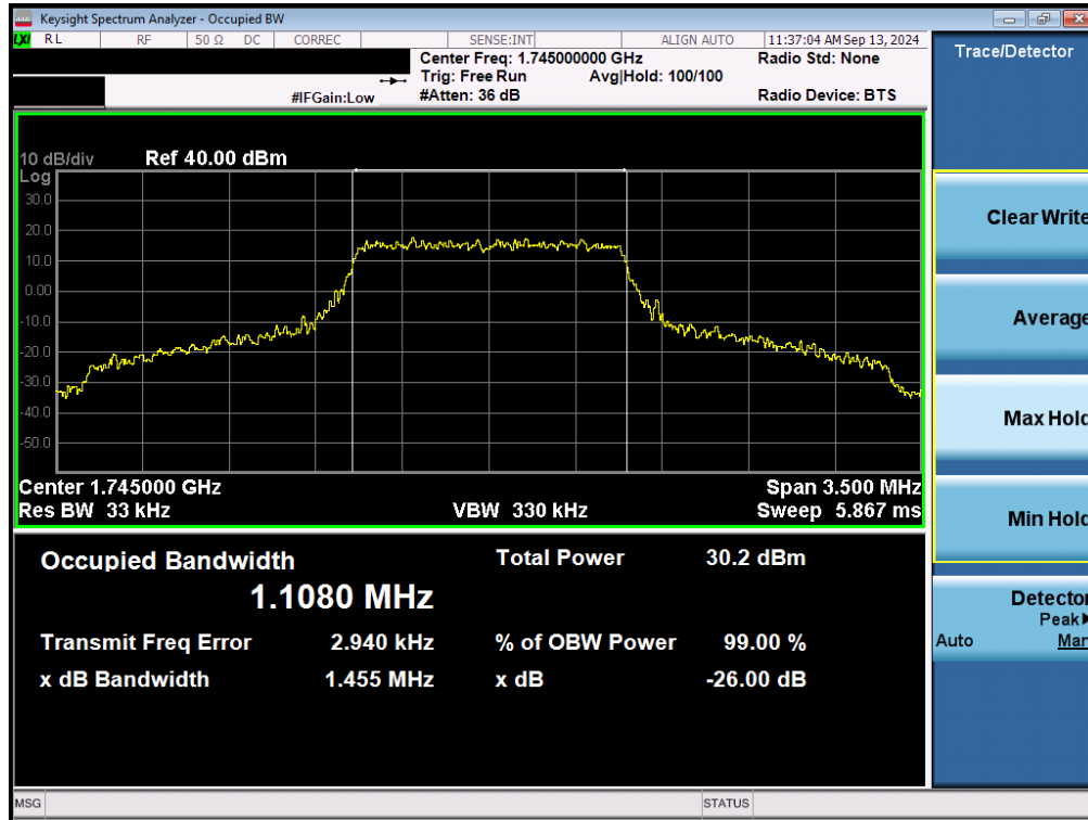
Plot 7-77. Occupied Bandwidth Plot (LTE Band 66/4 - 1.4MHz QPSK - Full RB - ANT2)
