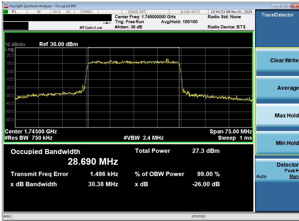
Plot 7-90. Occupied Bandwidth Plot (NR Band n66 - 30.0MHz CP-OFDM 16QAM - Full RB – ANT2)
