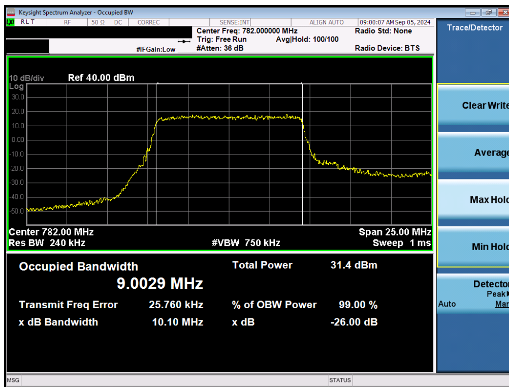
Plot 7-12. Occupied Bandwidth Plot (LTE Band 13 - 10MHz QPSK - Full RB – ANT1)
