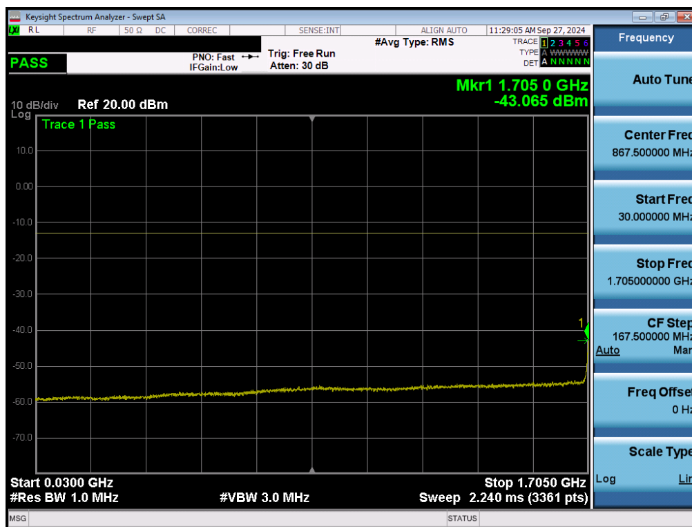
Plot 7-106. Conducted Spurious Plot (WCDMA-AWS - 5MHz QPSK - 1 RB – Low Channel)
