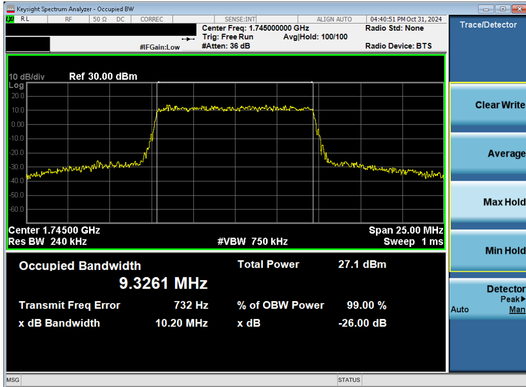
Plot 7-50. Occupied Bandwidth Plot (NR Band n66 - 10.0MHz CP-OFDM QPSK - Full RB - ANT1)
