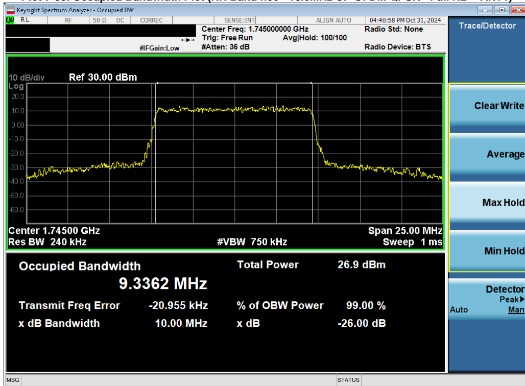
Plot 7-51. Occupied Bandwidth Plot (NR Band n66 - 10.0MHz CP-OFDM 16QAM - Full RB - ANT1)
