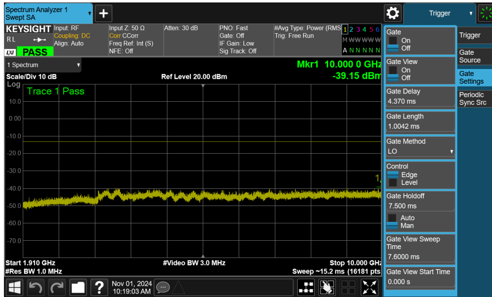
Plot 7-80. Conducted Spurious Plot (GPRS Ch. 661 - Ant1)
