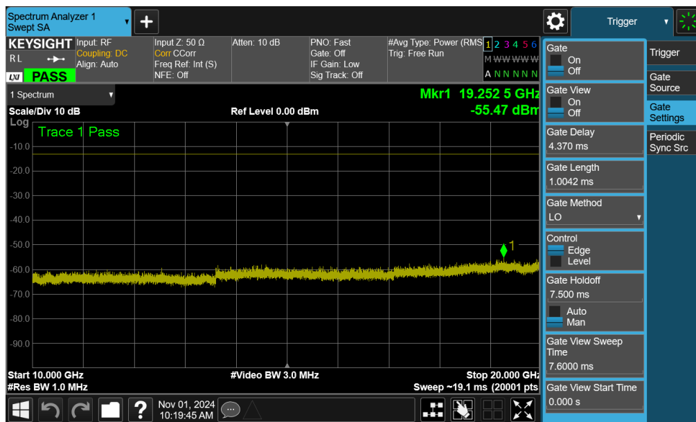
Plot 7-81. Conducted Spurious Plot (GPRS Ch. 661 - Ant1)
