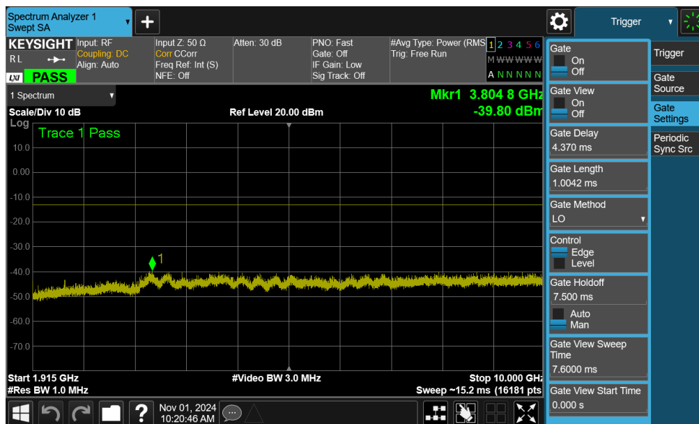
Plot 7-83. Conducted Spurious Plot (GPRS Ch. 810 - Ant1)
