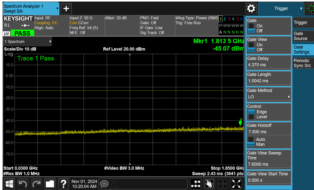
Plot 7-82. Conducted Spurious Plot (GPRS Ch. 810 - Ant1)
