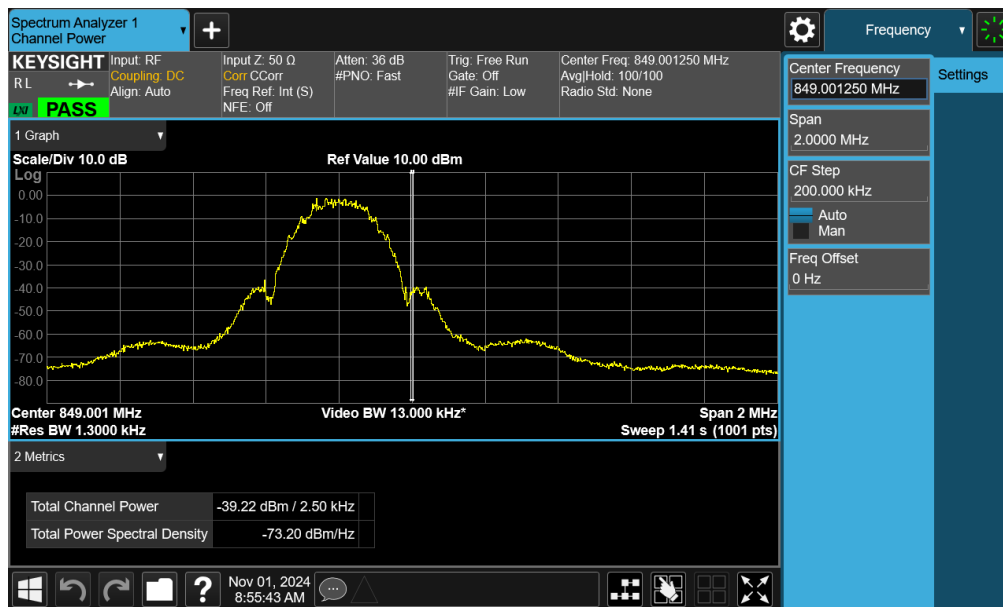
Plot 7-85. Upper Band Edge Plot (GPRS Cell – Ch. 251 – Ant2)
