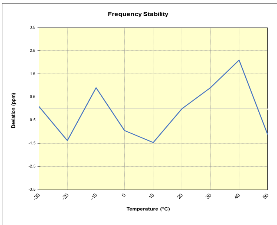
Plot 7-111. NR Band n26/5 Frequency Stability Chart
