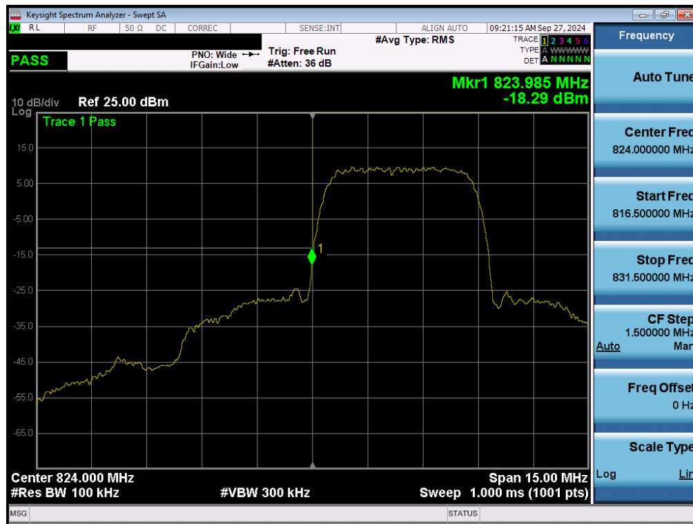
Plot 7-86. Lower Band Edge Plot (WCDMA Cell – Ch. 4132 – Ant2)
