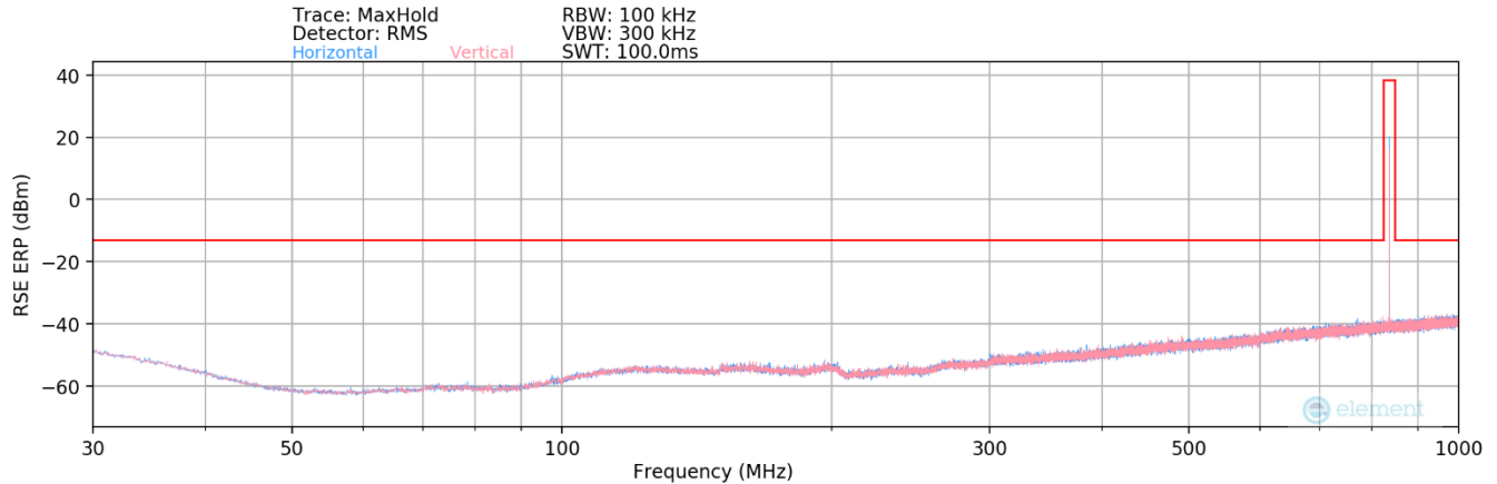
Plot 7-92. Radiated Spurious Plot Below 1GHz (GPRS Cell) – Ant1
