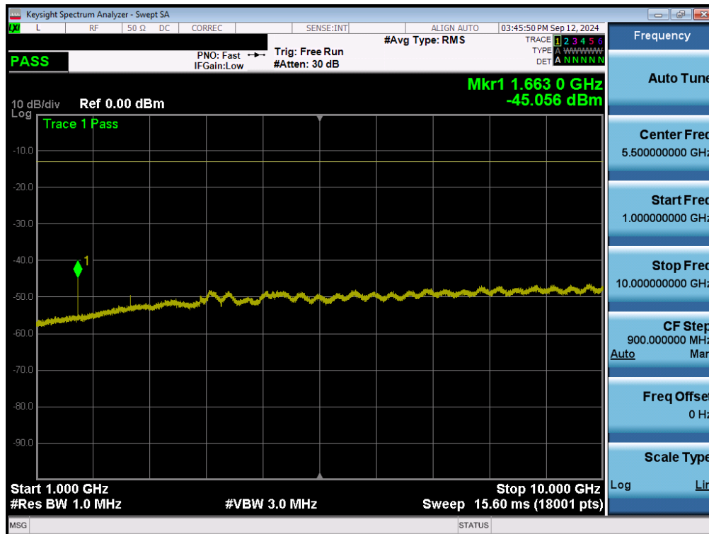
Plot 7-72. Conducted Spurious Plot (LTE Band 26/5 - 10MHz QPSK - 1 RB - Low Channel – Ant2)
