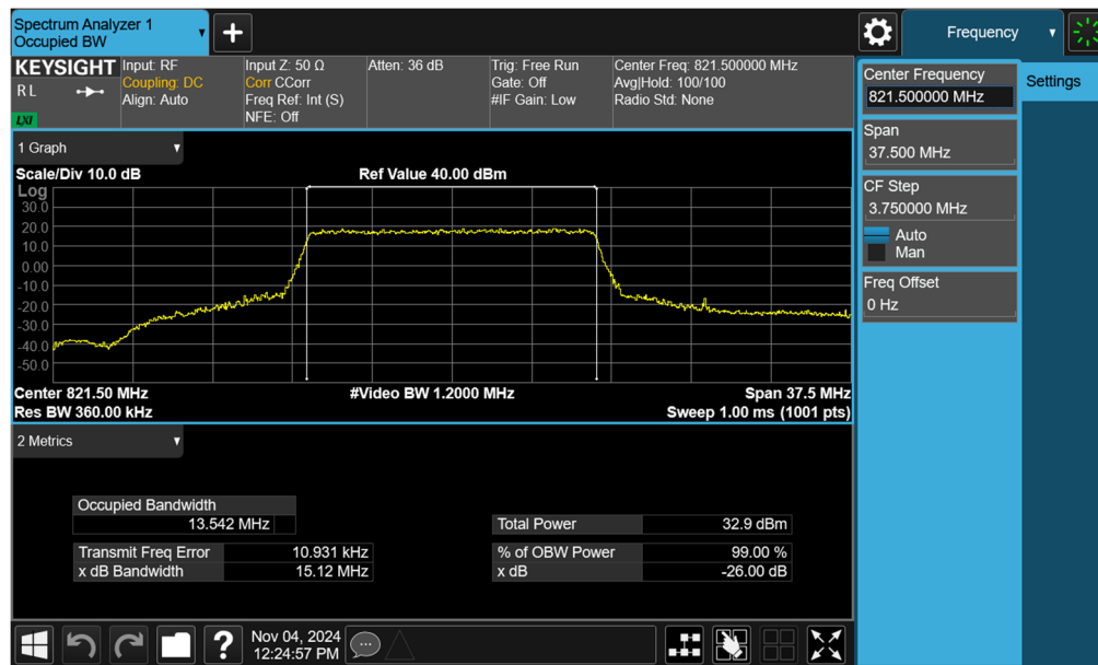
Plot 7-1. Occupied Bandwidth (Spot-check)
