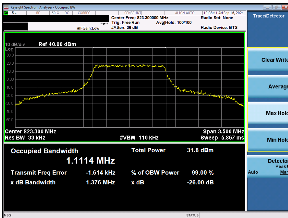
Plot 7-16. Occupied Bandwidth Plot (LTE Band 26 – 1.4MHz QPSK High Channel - Full RB)
