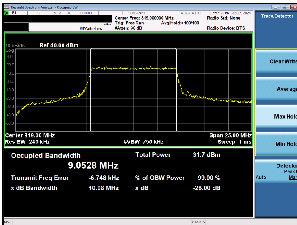
Plot 7-21. Occupied Bandwidth Plot (LTE Band 26 - 10MHz QPSK - Full RB)
