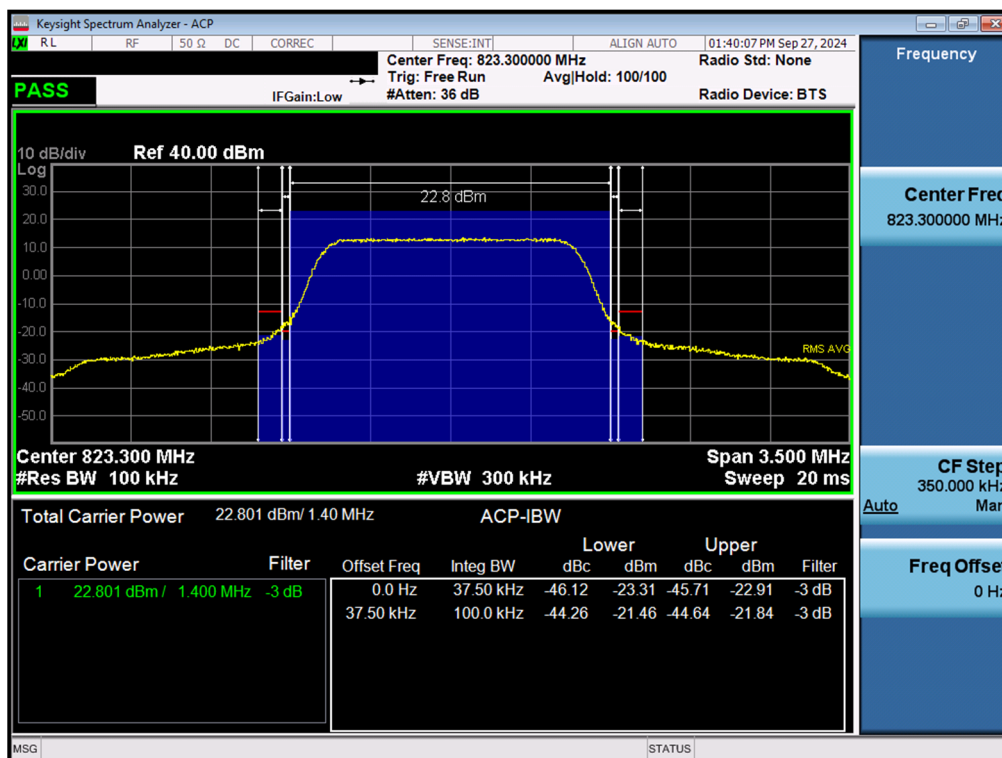
Plot 7-46. Channel - Edge Plot (LTE Band 26 - 1.4MHz QPSK - High Channel)
