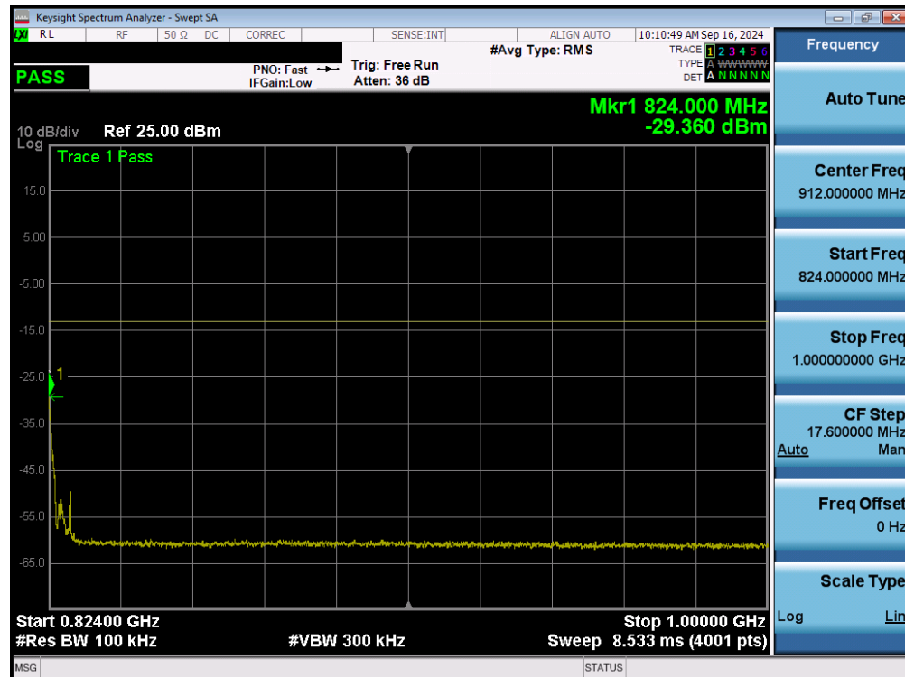
Plot 7-38. Conducted Spurious Plot (LTE Band 26 - 15MHz QPSK - RB Size 1, RB Offset 37)
