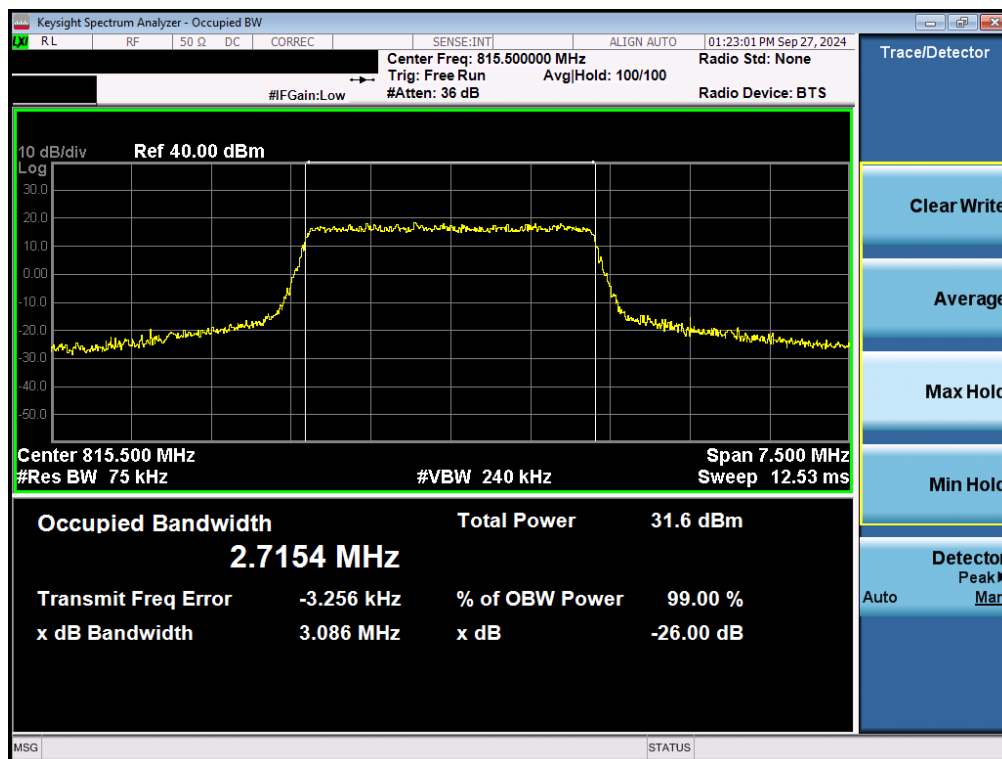
Plot 7-27. Occupied Bandwidth Plot (LTE Band 26 - 3MHz QPSK Low Channel- Full RB)
