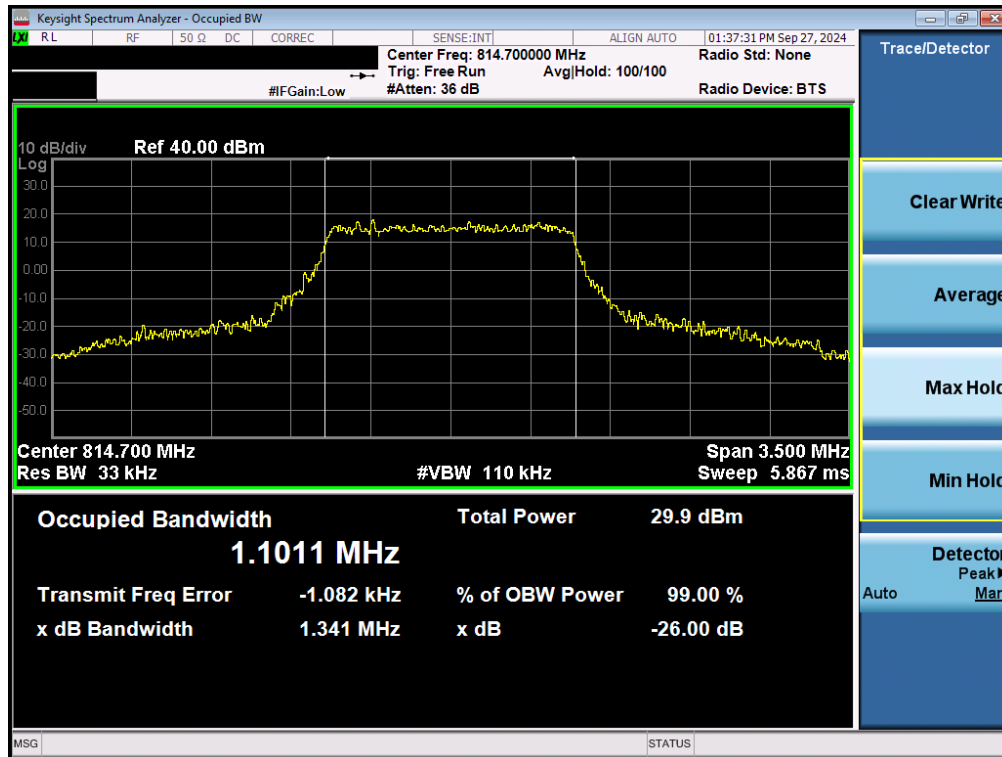
Plot 7-35. Occupied Bandwidth Plot (LTE Band 26 – 1.4MHz 16-QAM Low Channel - Full RB)
