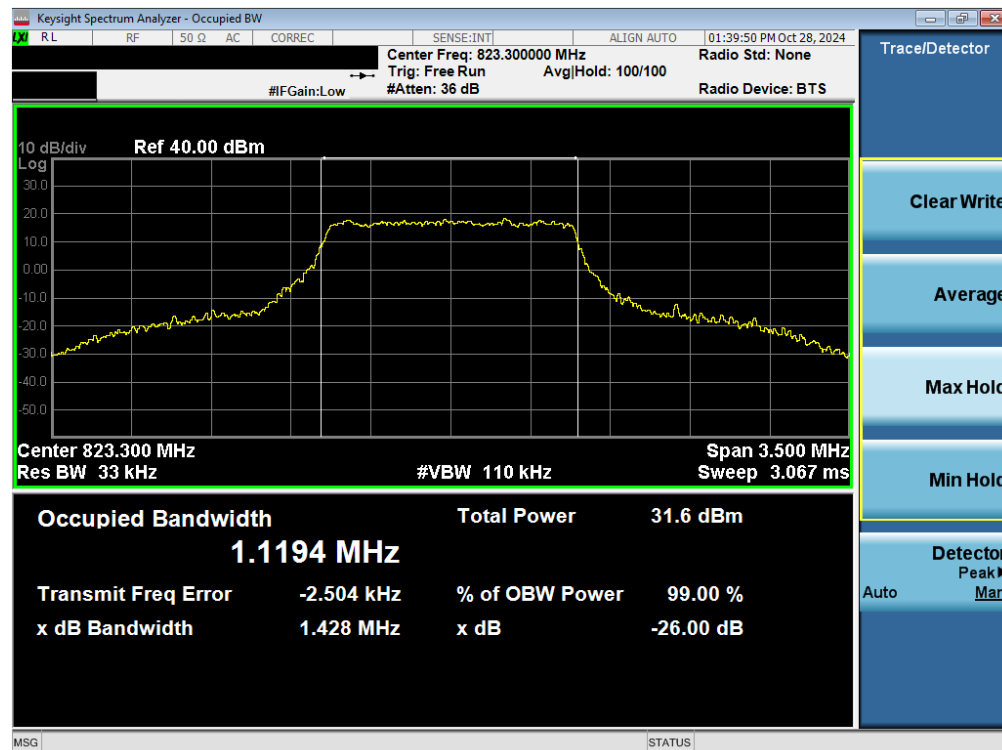
Plot 7-36. Occupied Bandwidth Plot (LTE Band 26 – 1.4MHz 16-QAM High Channel - Full RB)
