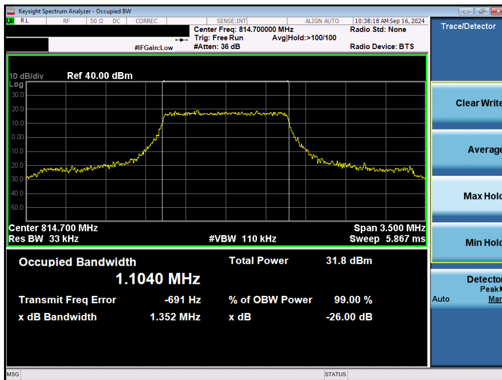
Plot 7-15. Occupied Bandwidth Plot (LTE Band 26 – 1.4MHz QPSK Low Channel- Full RB)
