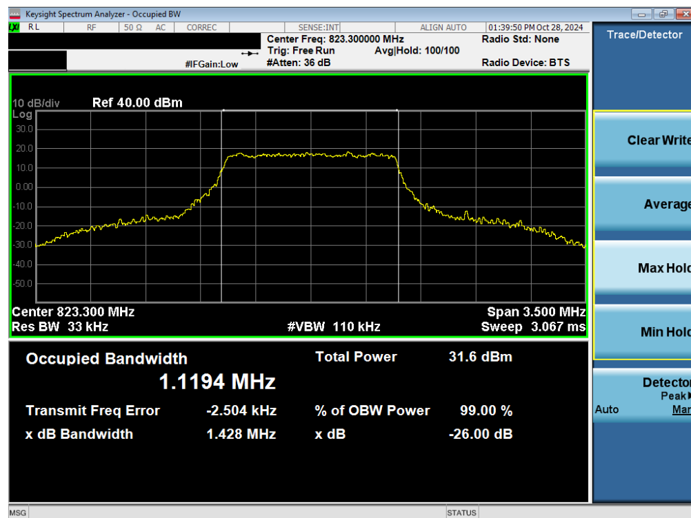
Plot 7-32. Occupied Bandwidth Plot (LTE Band 26 – 1.4MHz 16-QAM High Channel - Full RB)
