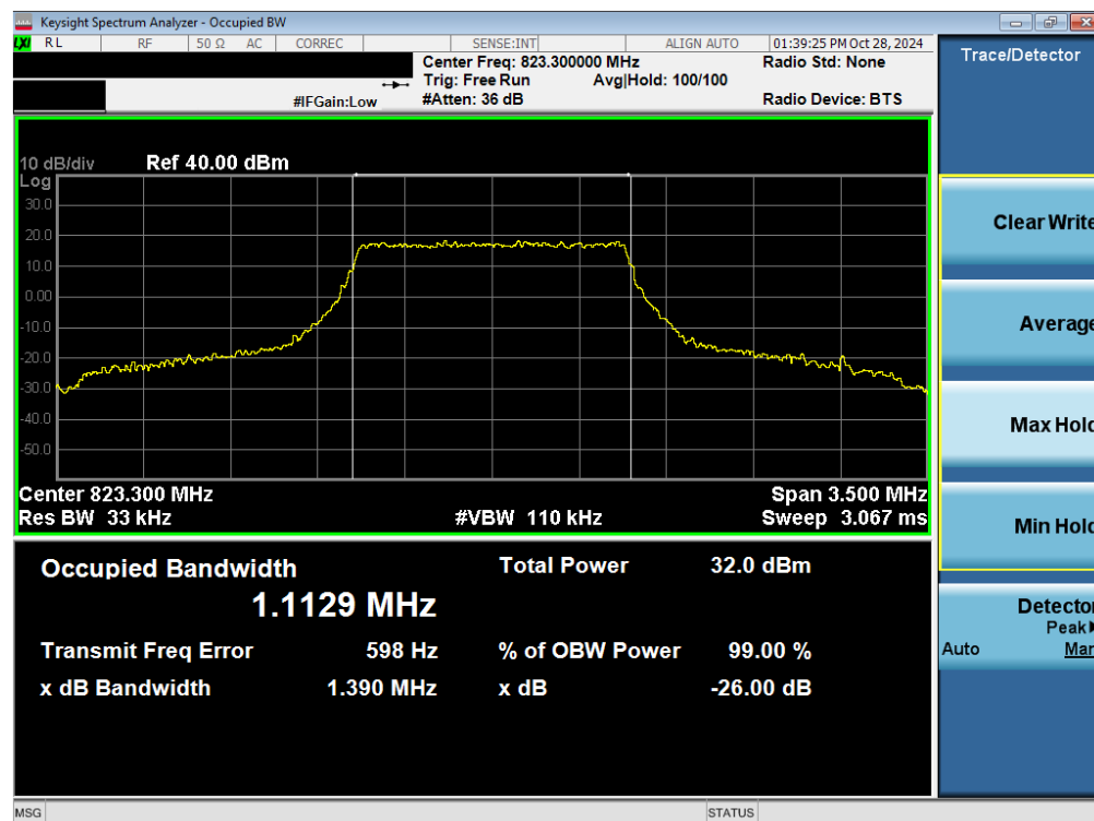
Plot 7-34. Occupied Bandwidth Plot (LTE Band 26 – 1.4MHz QPSK High Channel - Full RB)
