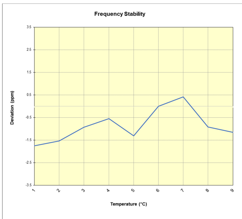
Plot 7-51. LTE Band 26 Frequency Stability Chart
