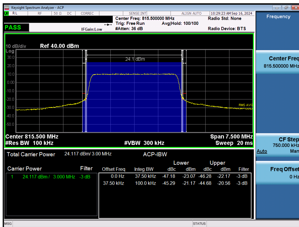
Plot 7-43. Channel - Edge Plot (LTE Band 26 - 3MHz QPSK - Low Channel)
