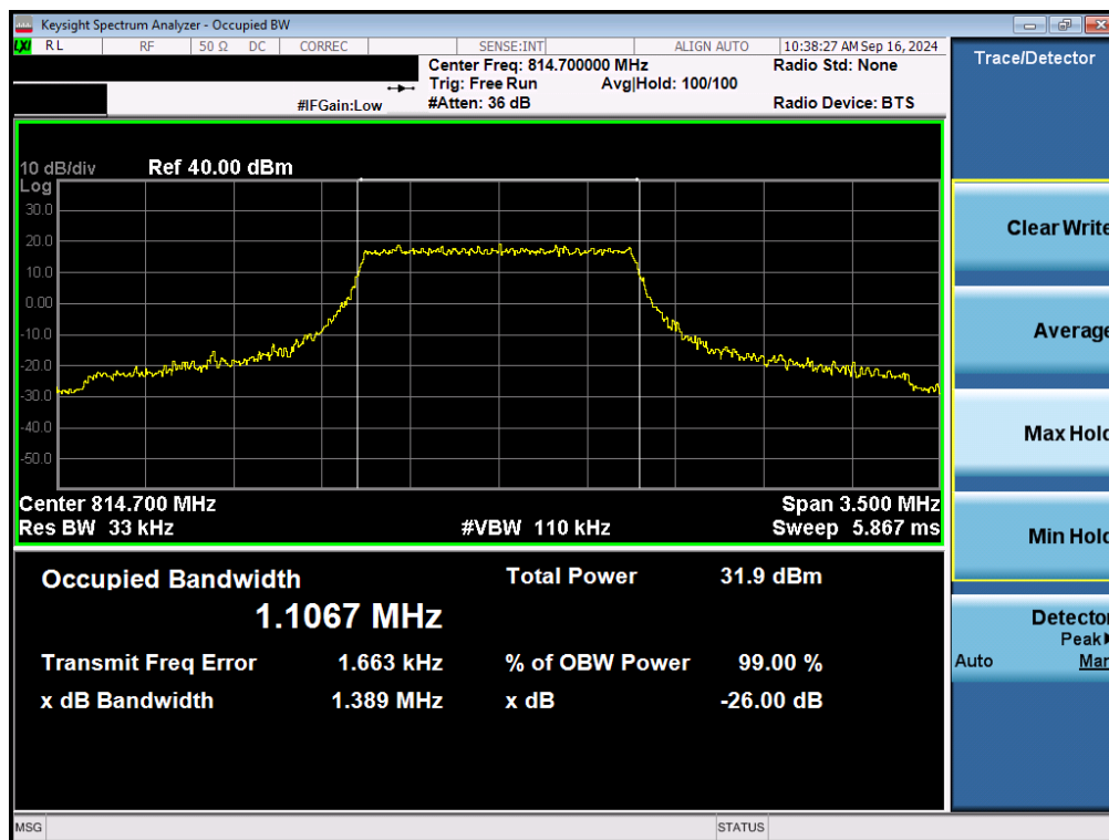
Plot 7-13. Occupied Bandwidth Plot (LTE Band 26 – 1.4MHz 16-QAM Low Channel - Full RB)
