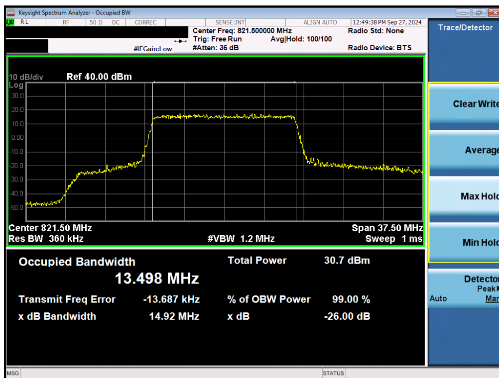
Plot 7-20. Occupied Bandwidth Plot (LTE Band 26 - 15MHz 16-QAM - Full RB)
