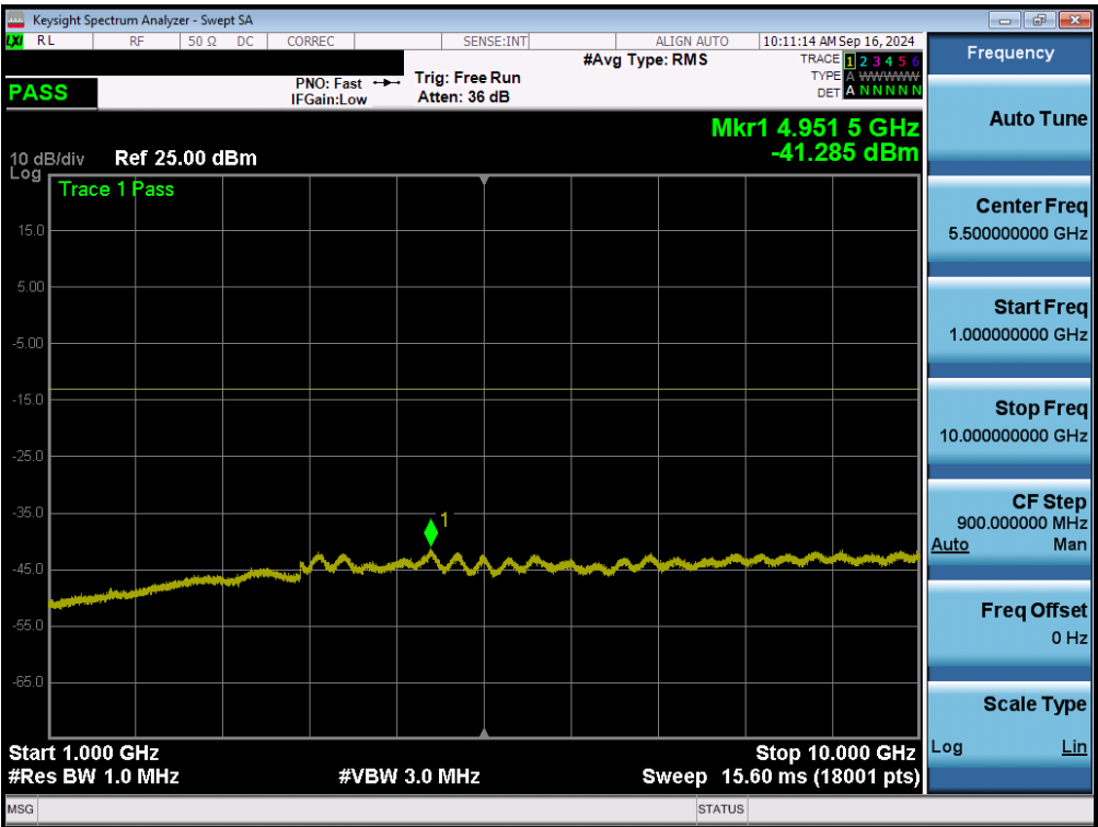
Plot 7-39. Conducted Spurious Plot (LTE Band 26 - 15MHz QPSK - RB Size 1, RB Offset 37)
