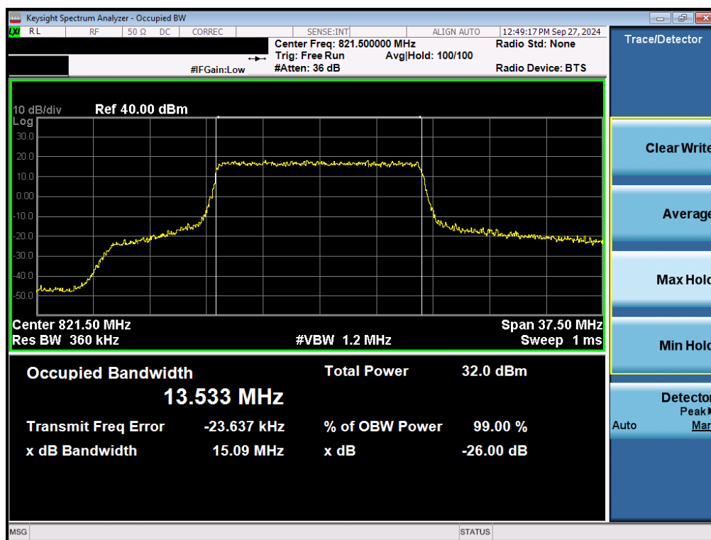
Plot 7-19. Occupied Bandwidth Plot (LTE Band 26 - 15MHz QPSK - Full RB)
