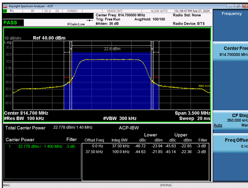
Plot 7-45. Channel - Edge Plot (LTE Band 26 - 1.4MHz QPSK - Low Channel)
