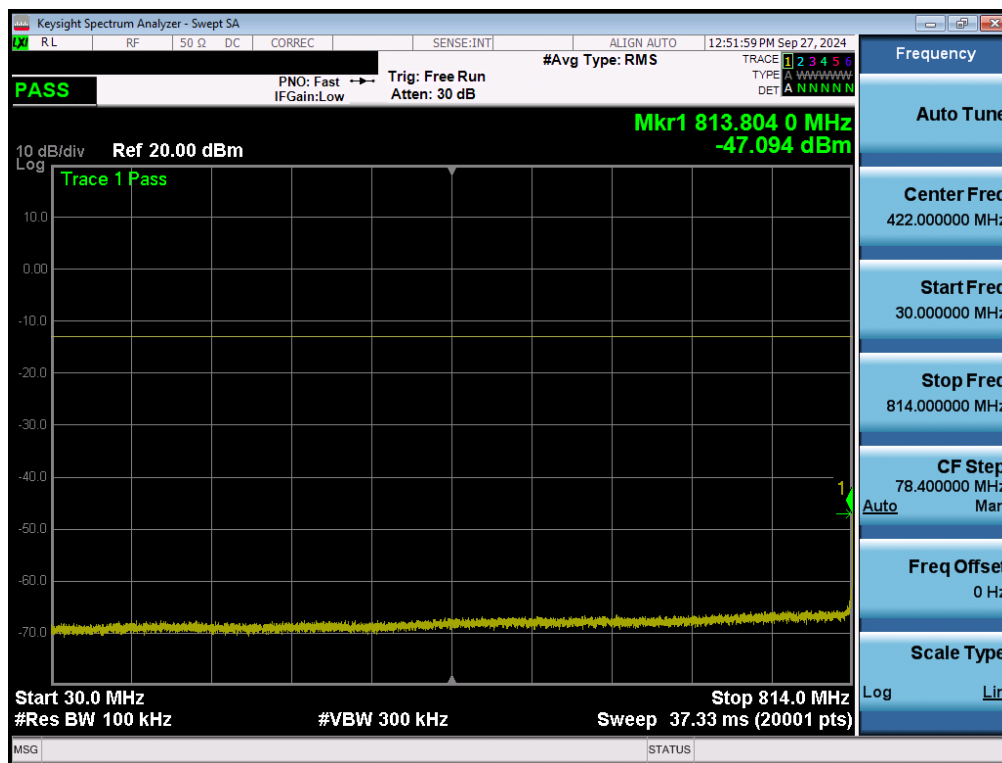
Plot 7-40. Conducted Spurious Plot (LTE Band 26 - 15MHz QPSK - RB Size 1, RB Offset 37)
