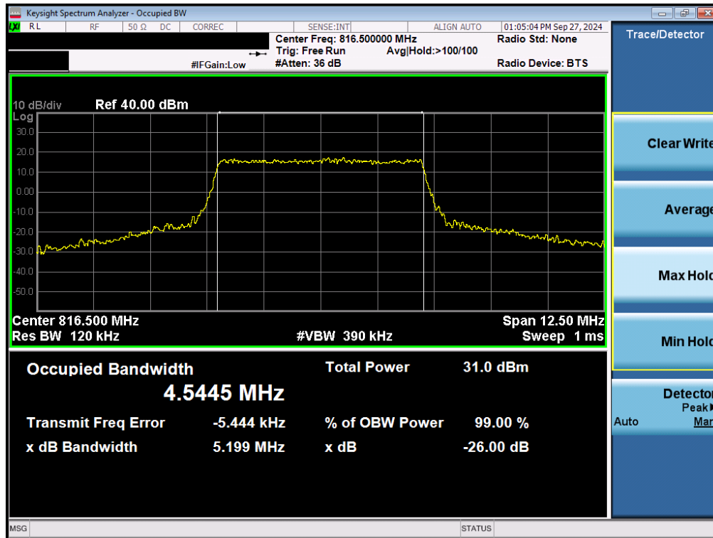
Plot 7-25. Occupied Bandwidth Plot (LTE Band 26 - 5MHz 16-QAM Low Channel - Full RB)
