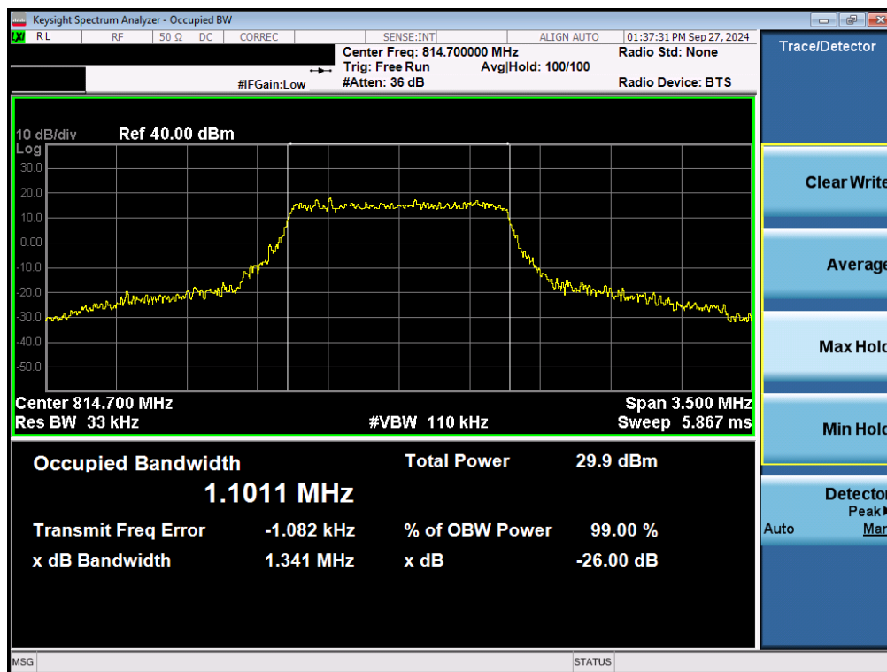
Plot 7-31. Occupied Bandwidth Plot (LTE Band 26 – 1.4MHz 16-QAM Low Channel - Full RB)
