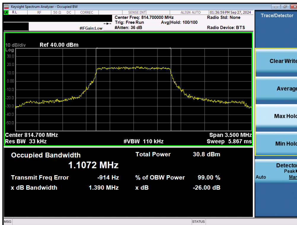
Plot 7-33. Occupied Bandwidth Plot (LTE Band 26 – 1.4MHz QPSK Low Channel- Full RB)
