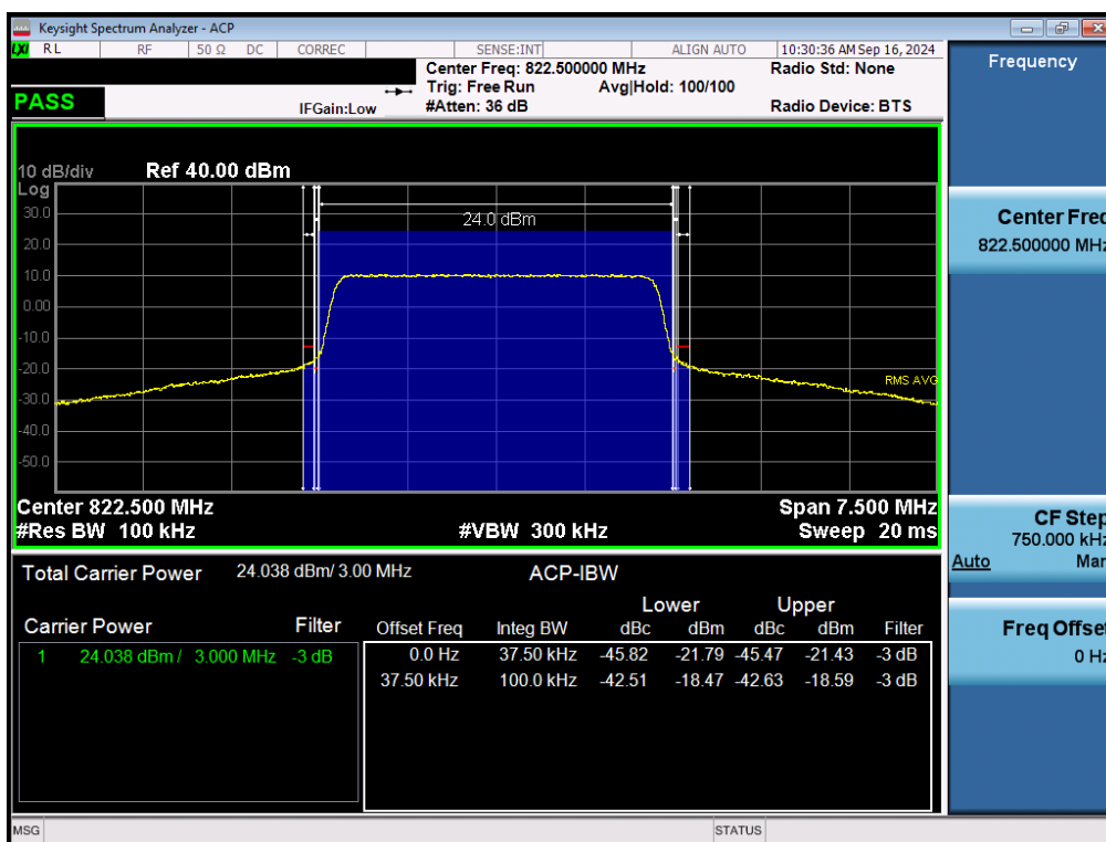
Plot 7-44. Channel - Edge Plot (LTE Band 26 - 3MHz QPSK - High Channel)
