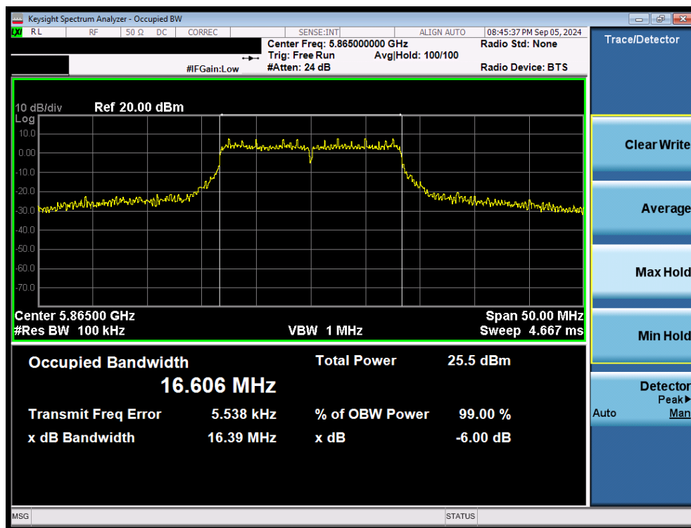
Plot 7-51. 6dB Bandwidth Plot MIMO ANT2 (20MHz 802.11a (UNII Band 4) – Ch.173)
