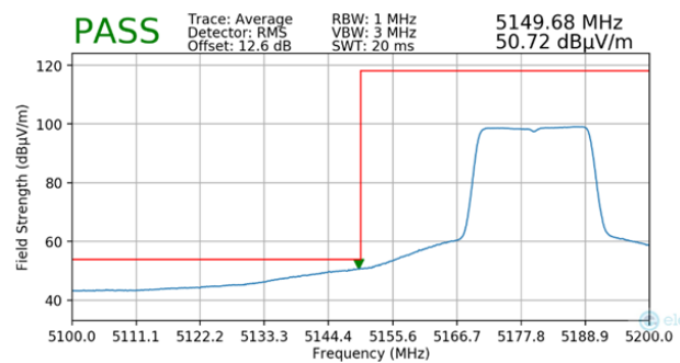
Plot 7-1. Radiated Lower Band Edge Plot MIMO (Average – UNII Band 1)
