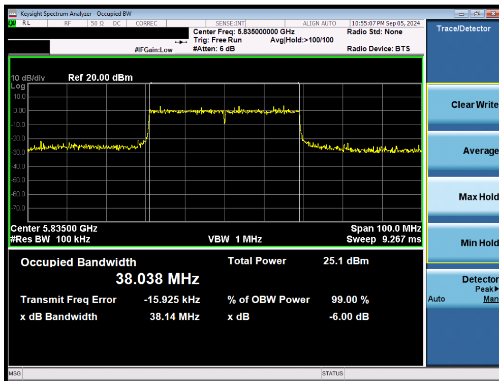
Plot 7-55. 6dB Bandwidth Plot MIMO ANT2 (40MHz 802.11ax/be (UNII Band 3/4) – Ch. 167)
