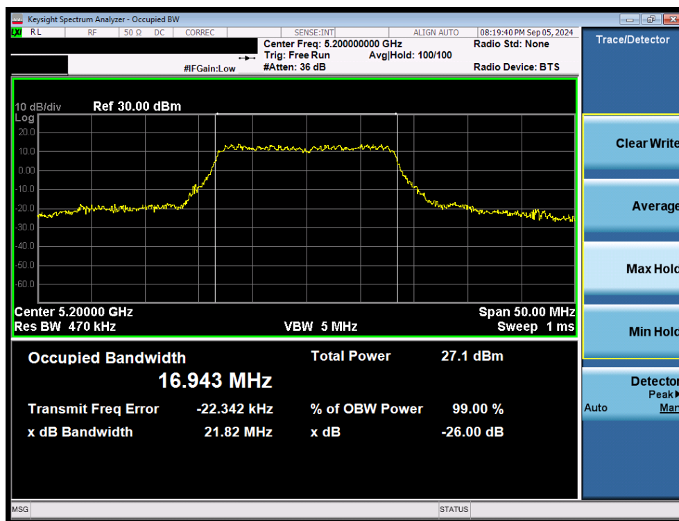
Plot 7-13. 26dB Bandwidth Plot MIMO ANT2 (20MHz 802.11a (UNII Band 1) – Ch. 40)
