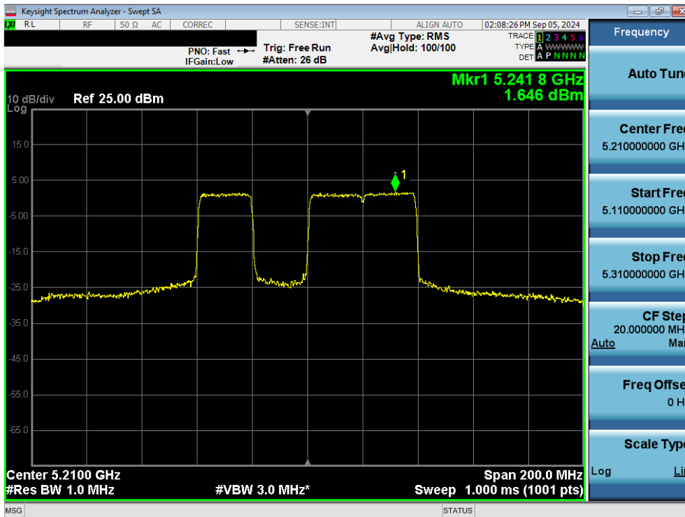
Plot 7-71. Power Spectral Density Plot MIMO ANT1 (80MHz 802.11be (20MHz Puncture) (UNII Band 1) – Ch. 42)
