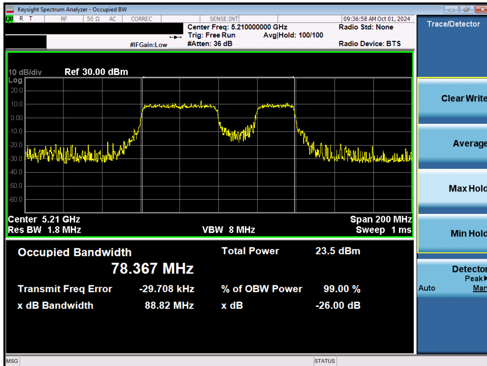
Plot 7-11. 26dB Bandwidth Plot MIMO ANT1 (80MHz 802.11be (20MHz Puncture Tones) (UNII Band 1) – Ch. 42)
