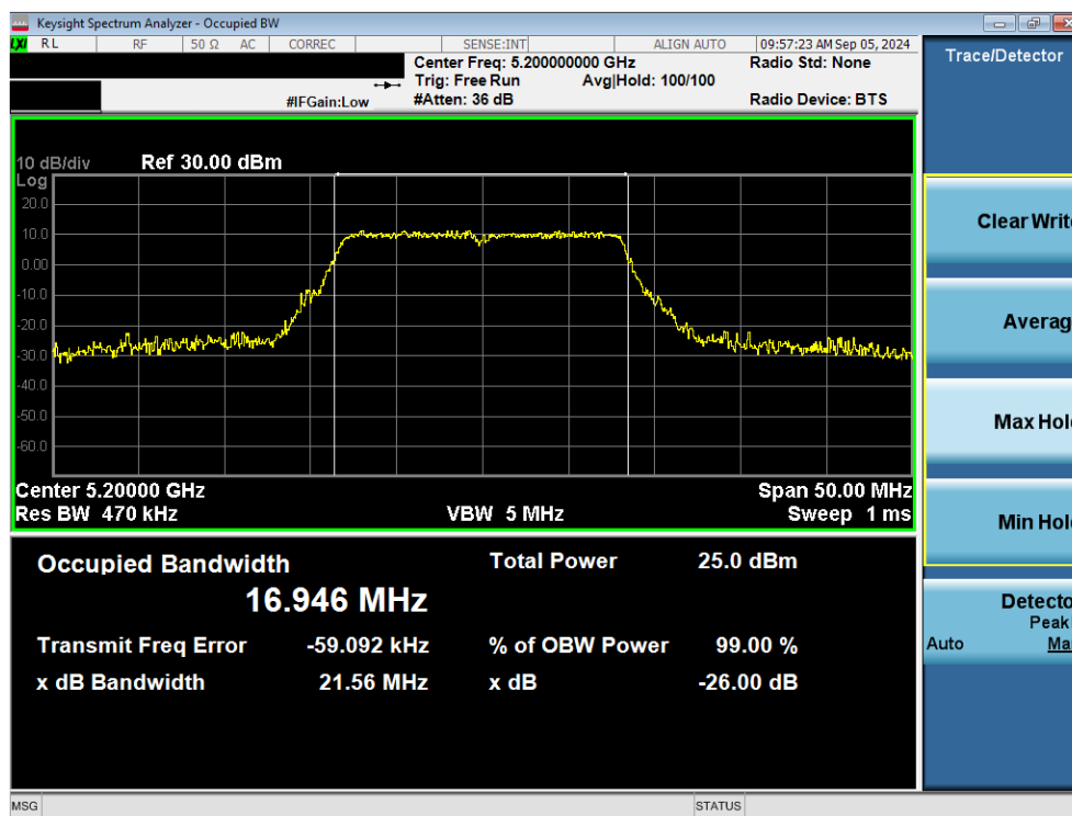
Plot 7-2. 26dB Bandwidth Plot MIMO ANT1 (20MHz 802.11a (UNII Band 1) – Ch. 40)
