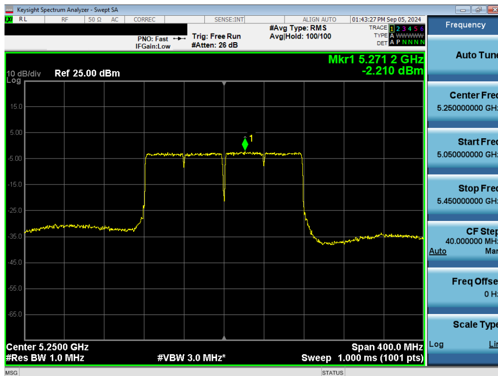
Plot 7-69. Power Spectral Density Plot MIMO ANT1 (160MHz 802.11ac (UNII Band 1/2A) – Ch. 50)
