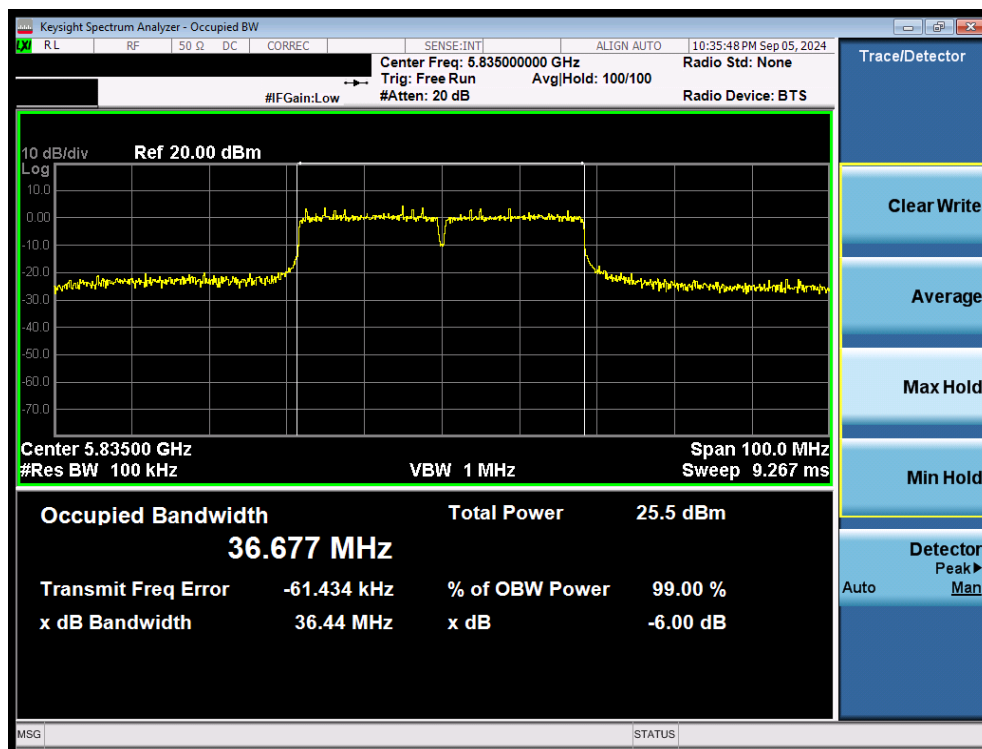
Plot 7-54. 6dB Bandwidth Plot MIMO ANT2 (40MHz 802.11n (UNII Band 3/4) – Ch. 167)
