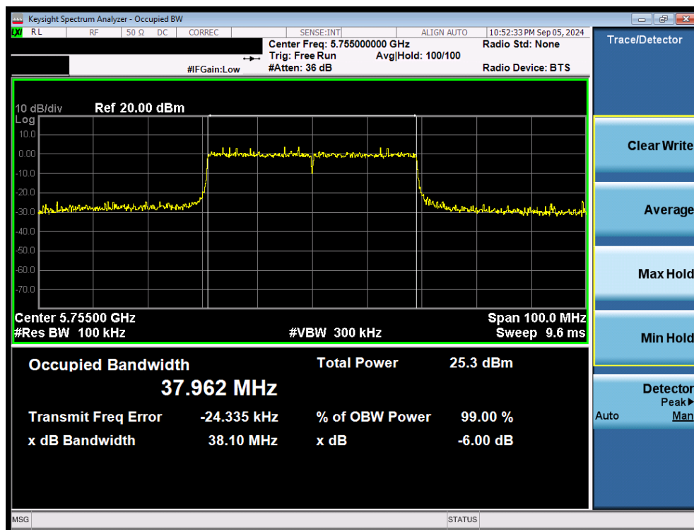
Plot 7-47. 6dB Bandwidth Plot MIMO ANT2 (40MHz 802.11ax/be (UNII Band 3) – Ch. 151)
