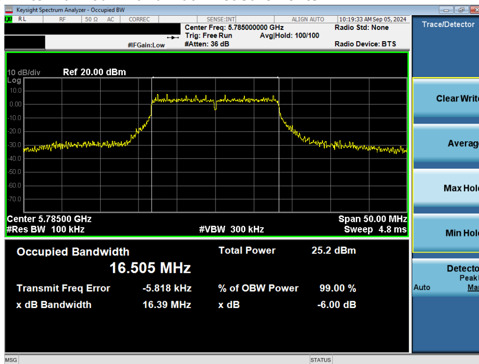
Plot 7-24. 6dB Bandwidth Plot MIMO ANT1 (20MHz 802.11a (UNII Band 3) – Ch.157)
