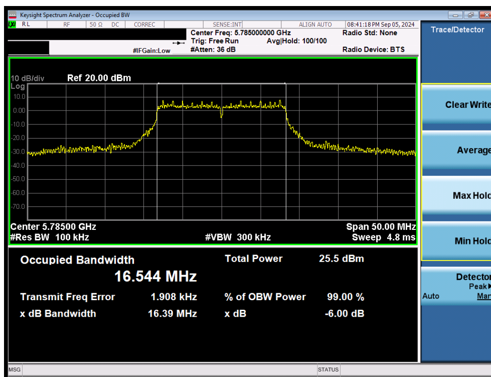
Plot 7-43. 6dB Bandwidth Plot MIMO ANT2 (20MHz 802.11a (UNII Band 3) – Ch.157)
