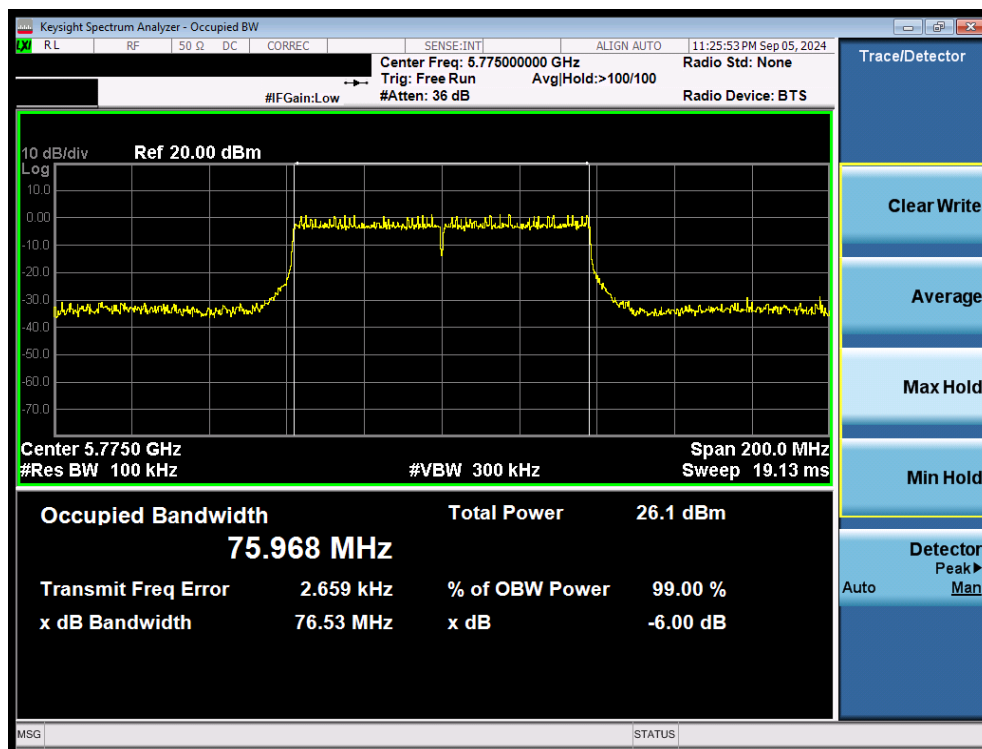
Plot 7-48. 6dB Bandwidth Plot MIMO ANT2 (80MHz 802.11ac (UNII Band 3) – Ch. 155)
