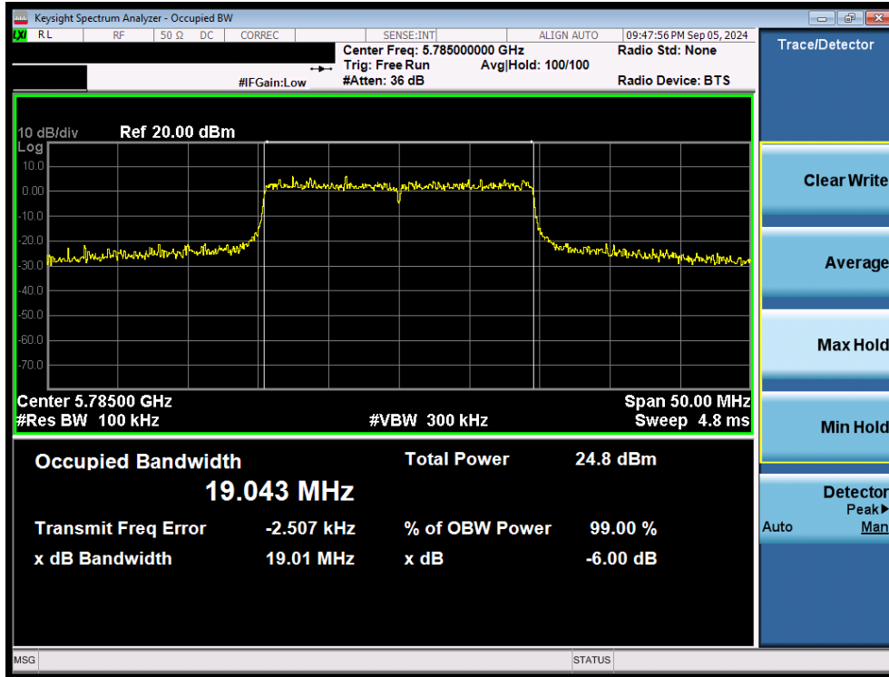
Plot 7-45. 6dB Bandwidth Plot MIMO ANT2 (20MHz 802.11ax/be (UNII Band 3) – Ch.157)
