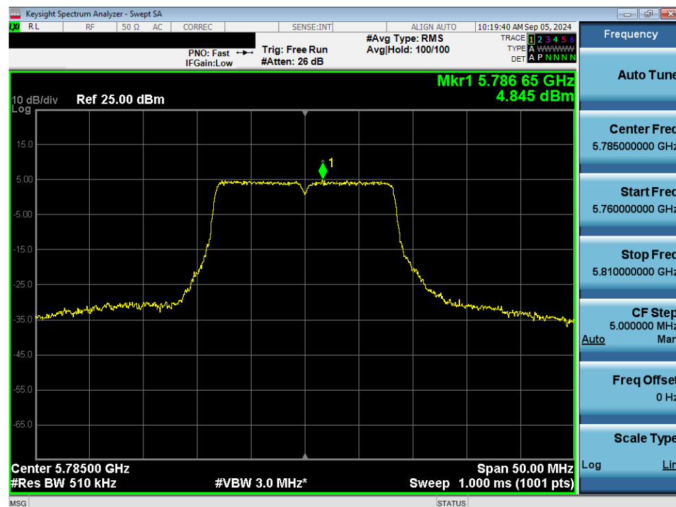
Plot 7-73. Power Spectral Density Plot MIMO ANT1 (20MHz 802.11a (UNII Band 3) – Ch.157)
