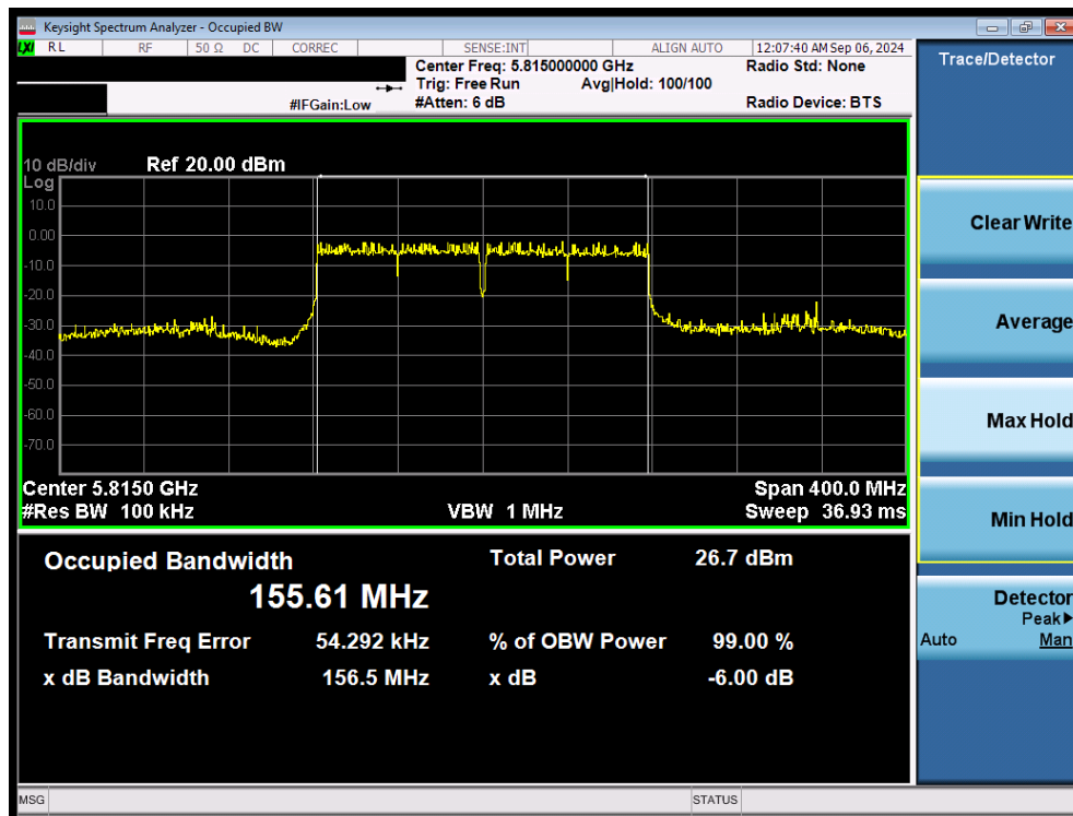
Plot 7-58. 6dB Bandwidth Plot MIMO ANT2 (160MHz 802.11ac (UNII Band 3/4) – Ch. 163)
