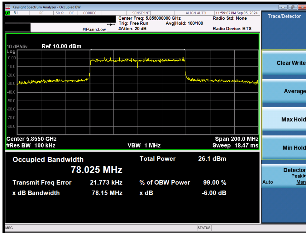
Plot 7-57. 6dB Bandwidth Plot MIMO ANT2 (80MHz 802.11ax/be (UNII Band 3/4) – Ch. 171)
