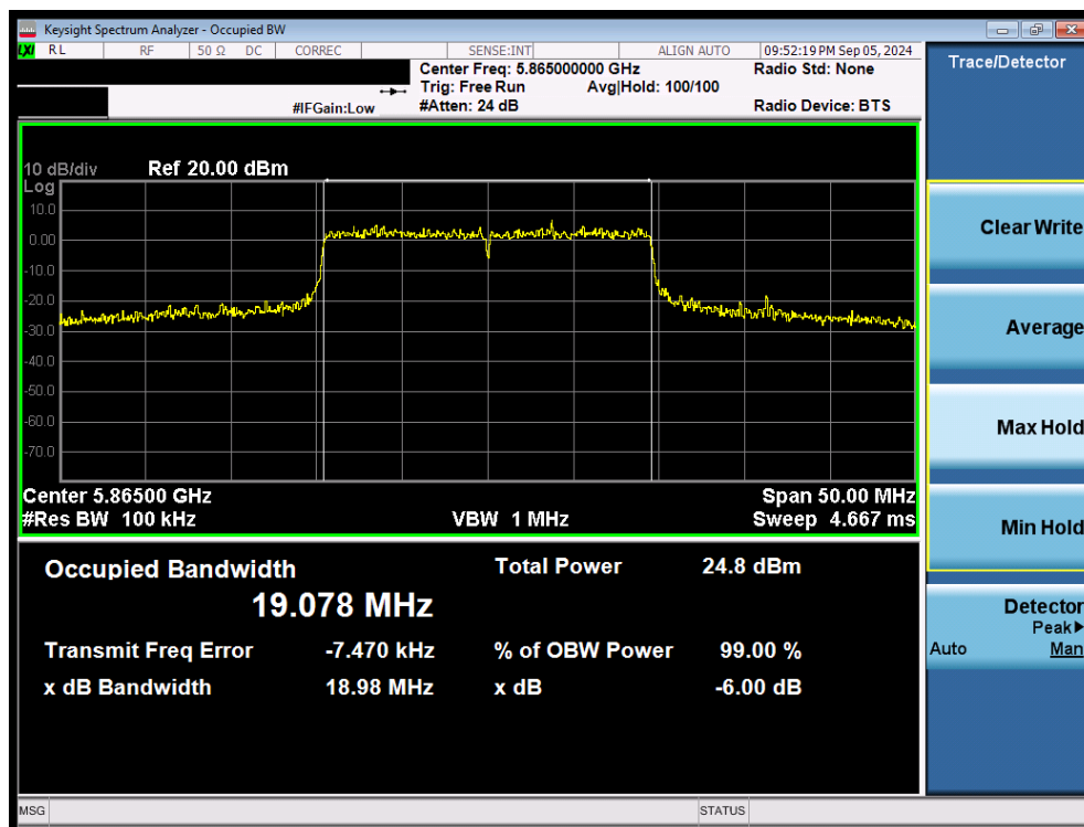
Plot 7-53. 6dB Bandwidth Plot MIMO ANT2 (20MHz 802.11ax/be (UNII Band 4) – Ch.173)
