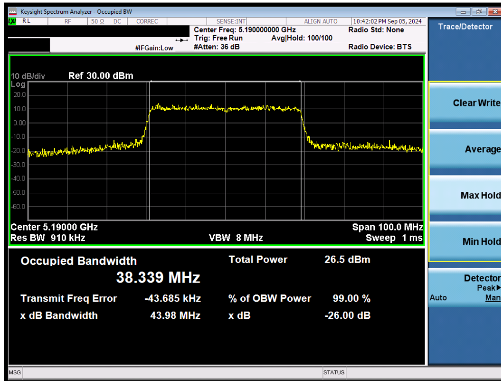
Plot 7-17. 26dB Bandwidth Plot MIMO ANT2 (40MHz 802.11ax/be (UNII Band 1) – Ch. 38)
