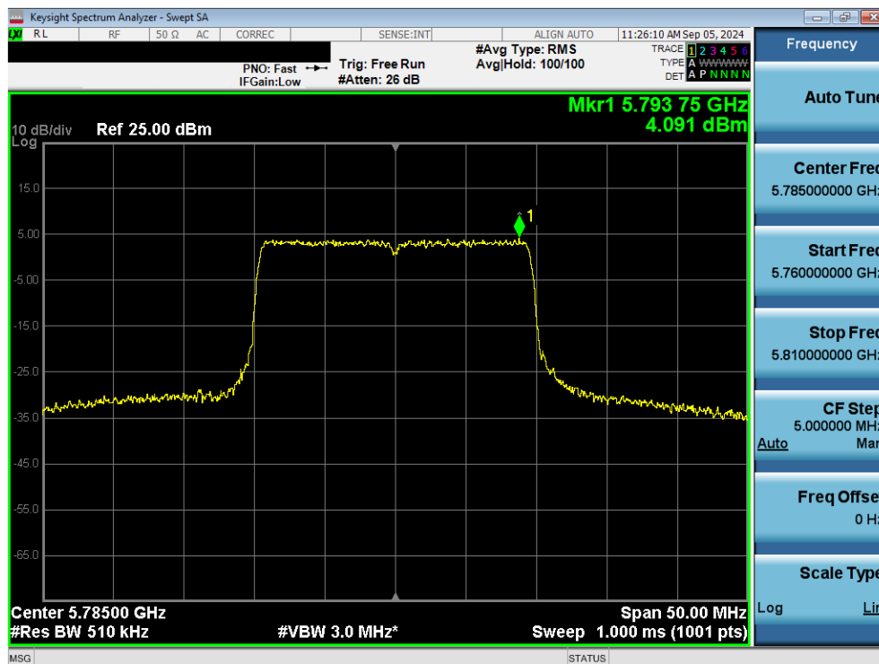
Plot 7-75. Power Spectral Density Plot MIMO ANT1 (20MHz 802.11ax/be (UNII Band 3) – Ch.157)
