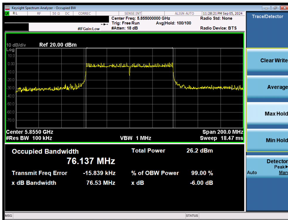
Plot 7-56. 6dB Bandwidth Plot MIMO ANT2 (80MHz 802.11ac (UNII Band 3/4) – Ch. 171)
