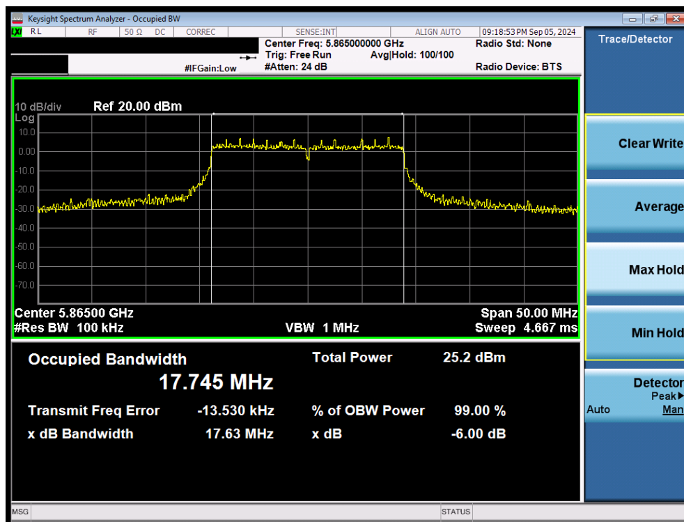
Plot 7-52. 6dB Bandwidth Plot MIMO ANT2 (20MHz 802.11n (UNII Band 4) – Ch.173)
