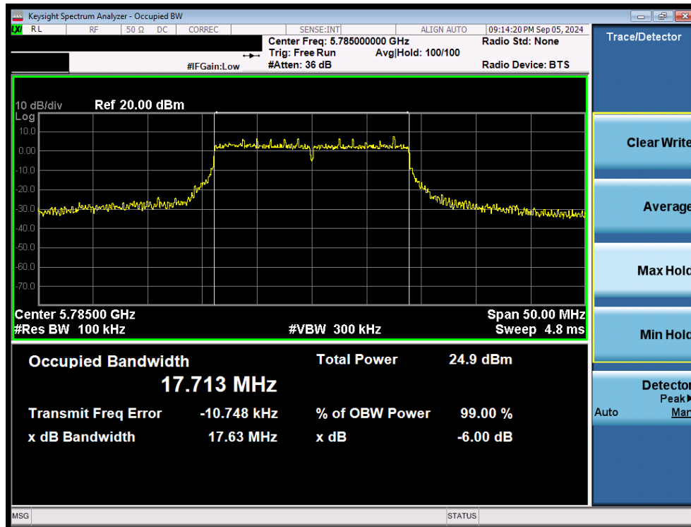
Plot 7-44. 6dB Bandwidth Plot MIMO ANT2 (20MHz 802.11n (UNII Band 3) – Ch.157)
