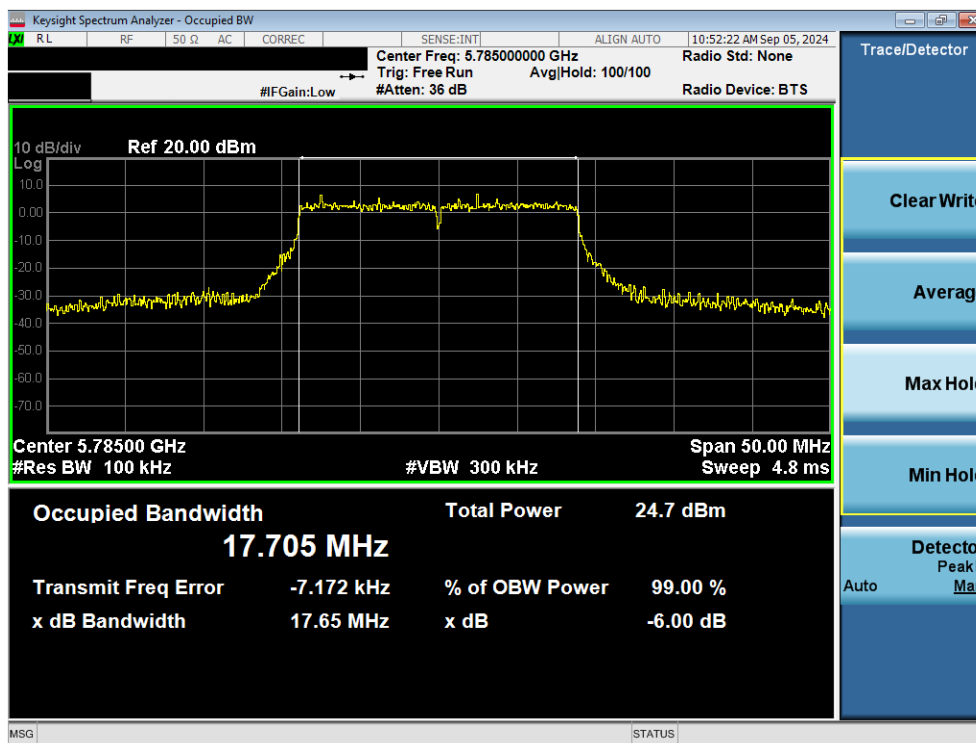
Plot 7-25. 6dB Bandwidth Plot MIMO ANT1 (20MHz 802.11n (UNII Band 3) – Ch.157)
