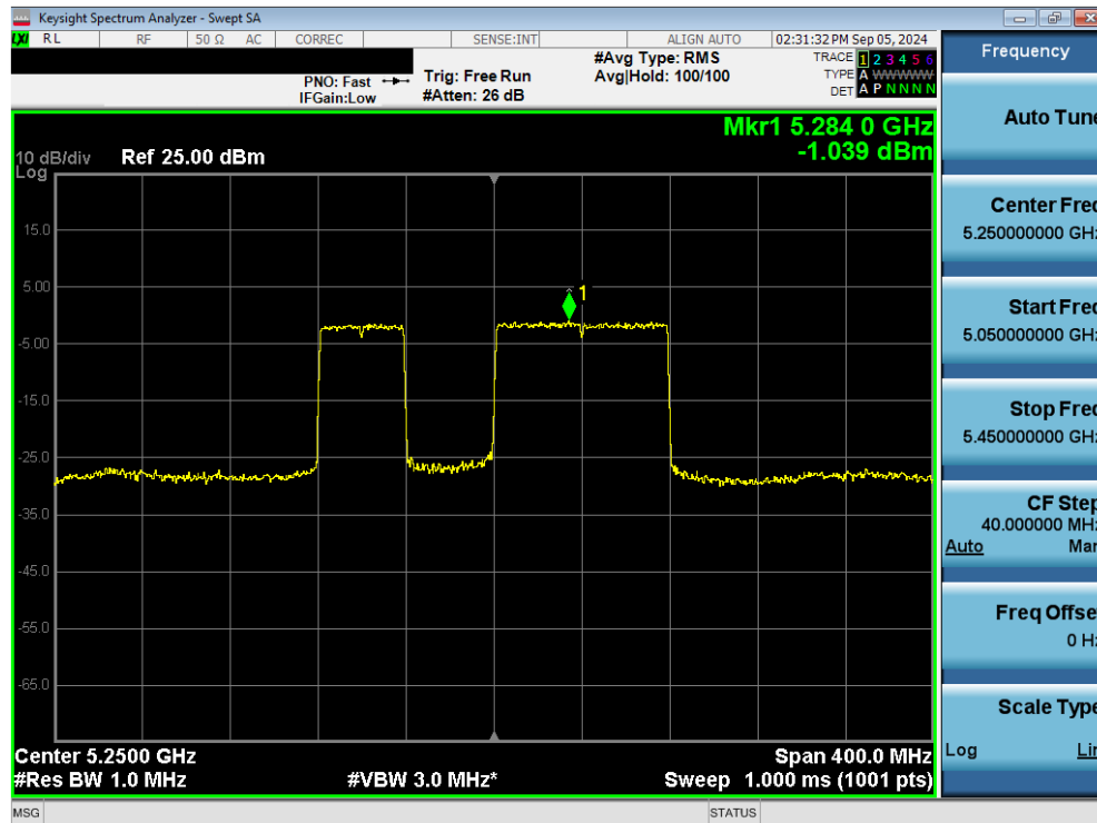
Plot 7-72. Power Spectral Density Plot MIMO ANT1 (160MHz 802.11be (40MHz Puncture) (UNII Band 1/2A) – Ch. 50)
