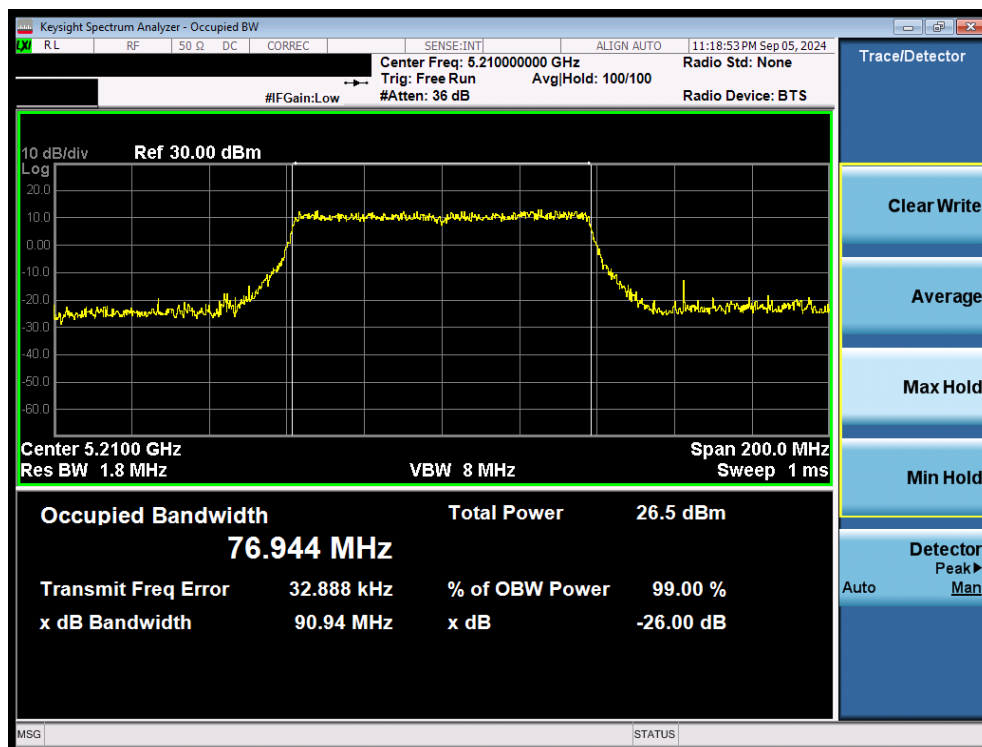
Plot 7-18. 26dB Bandwidth Plot MIMO ANT2 (80MHz 802.11ac (UNII Band 1) – Ch. 42)
