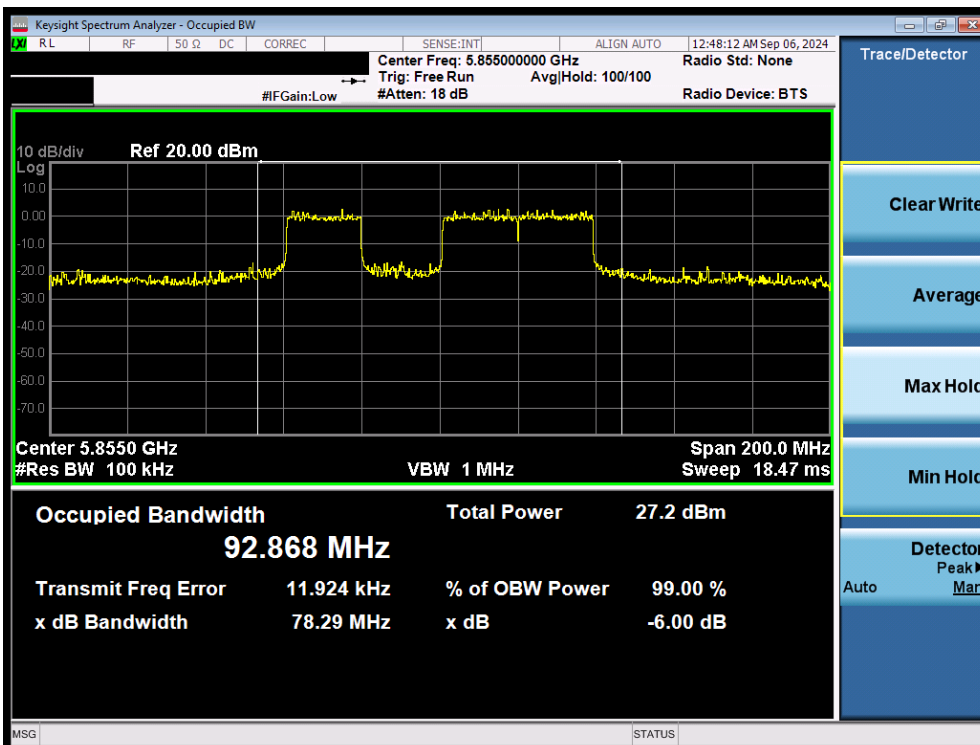
Plot 7-60. 6dB Bandwidth Plot MIMO ANT2 (80MHz 802.11be (20MHz Puncture) (UNII Band 3/4) – Ch. 171)
