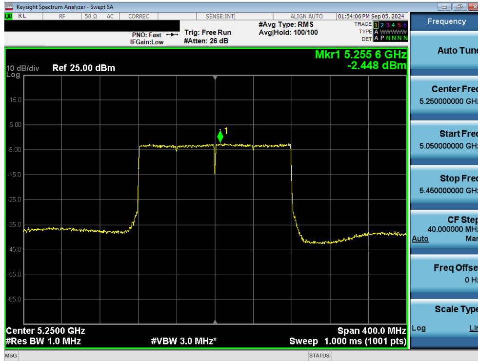
Plot 7-70. Power Spectral Density Plot MIMO ANT1 (160MHz 802.11ax/be (UNII Band 1/2A) – Ch. 50)
