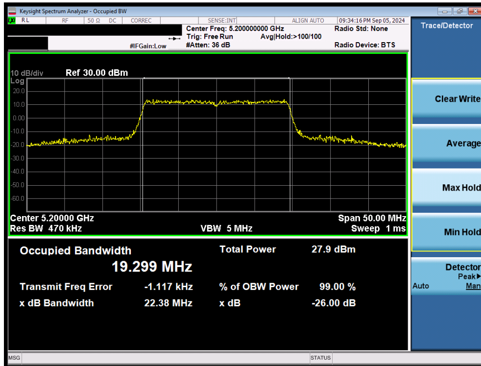
Plot 7-15. 26dB Bandwidth Plot MIMO ANT2 (20MHz 802.11ax/be (UNII Band 1) – Ch. 40)
