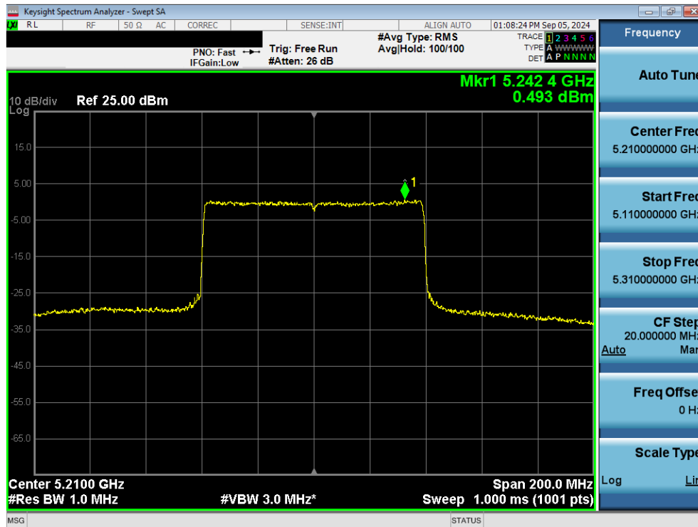
Plot 7-68. Power Spectral Density Plot MIMO ANT1 (80MHz 802.11ax/be (UNII Band 1) – Ch. 42)
