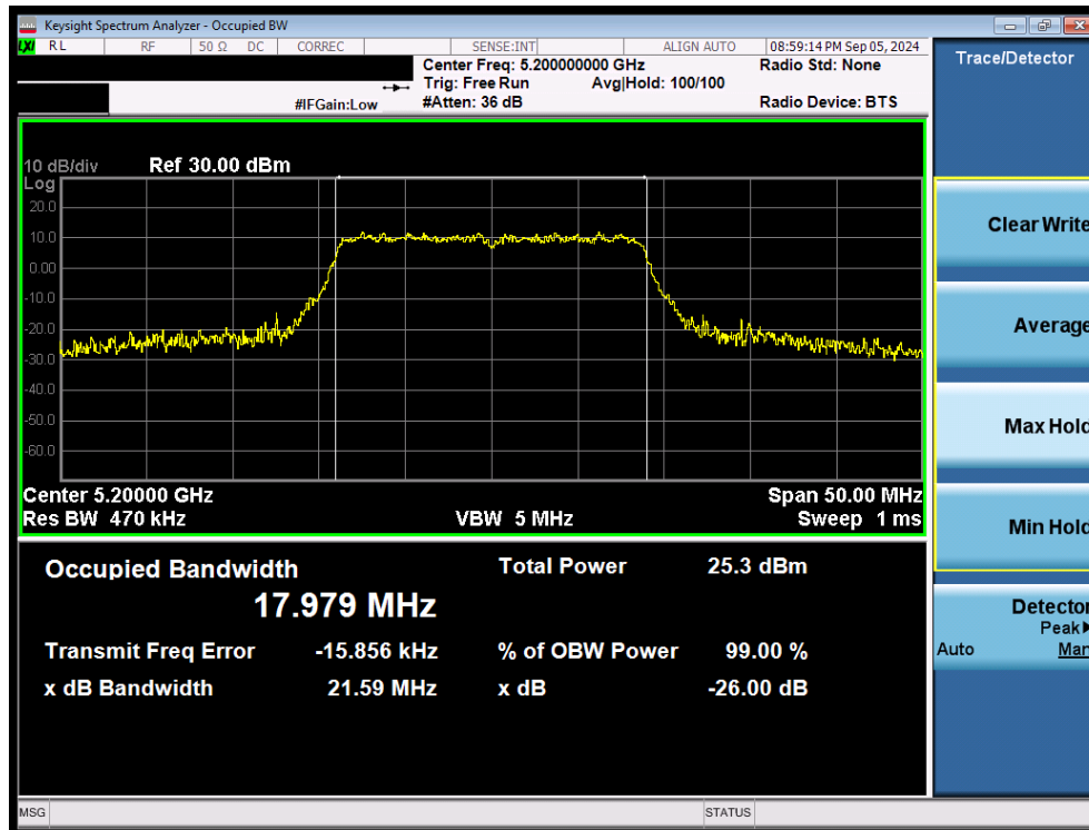
Plot 7-14. 26dB Bandwidth Plot MIMO ANT2 (20MHz 802.11n (UNII Band 1) – Ch. 40)
