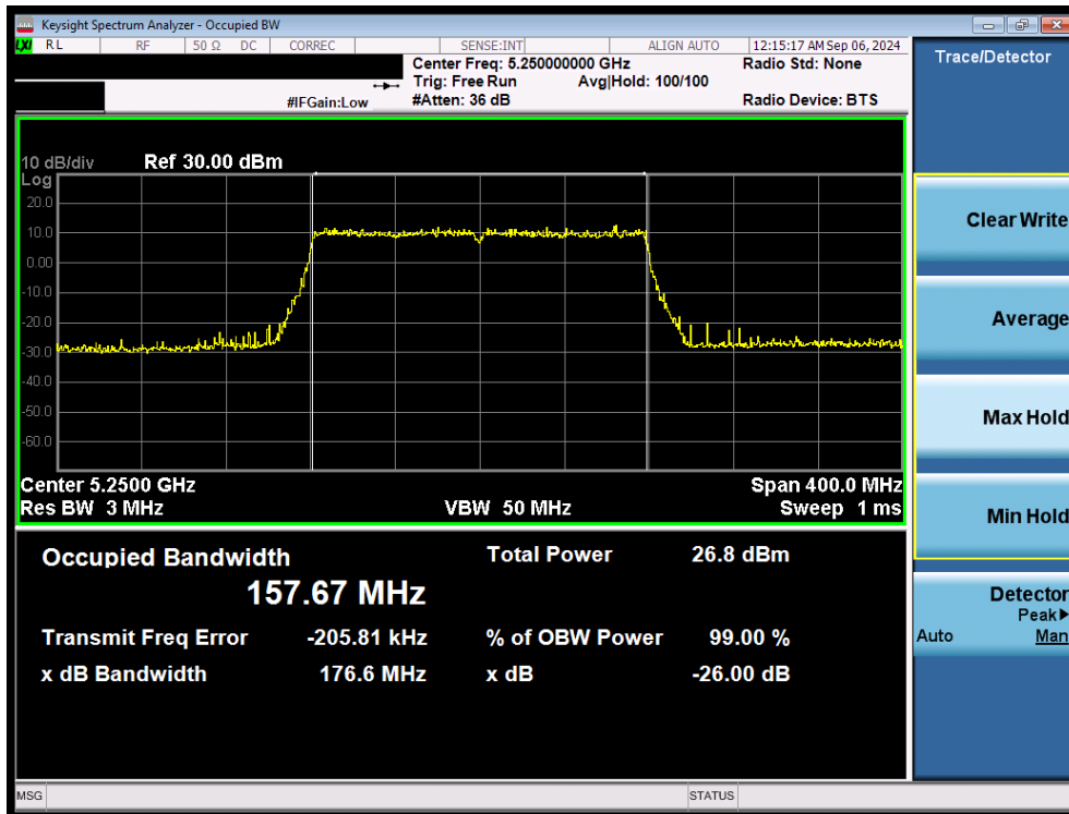
Plot 7-21. 26dB Bandwidth Plot MIMO ANT2 (160MHz 802.11ax/be (UNII Band 1/2A) – Ch. 50)
