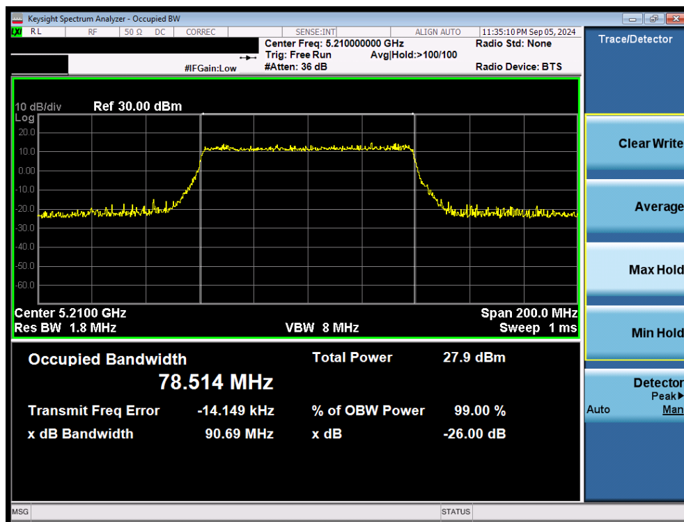
Plot 7-19. 26dB Bandwidth Plot MIMO ANT2 (80MHz 802.11ax/be (UNII Band 1) – Ch. 42)
