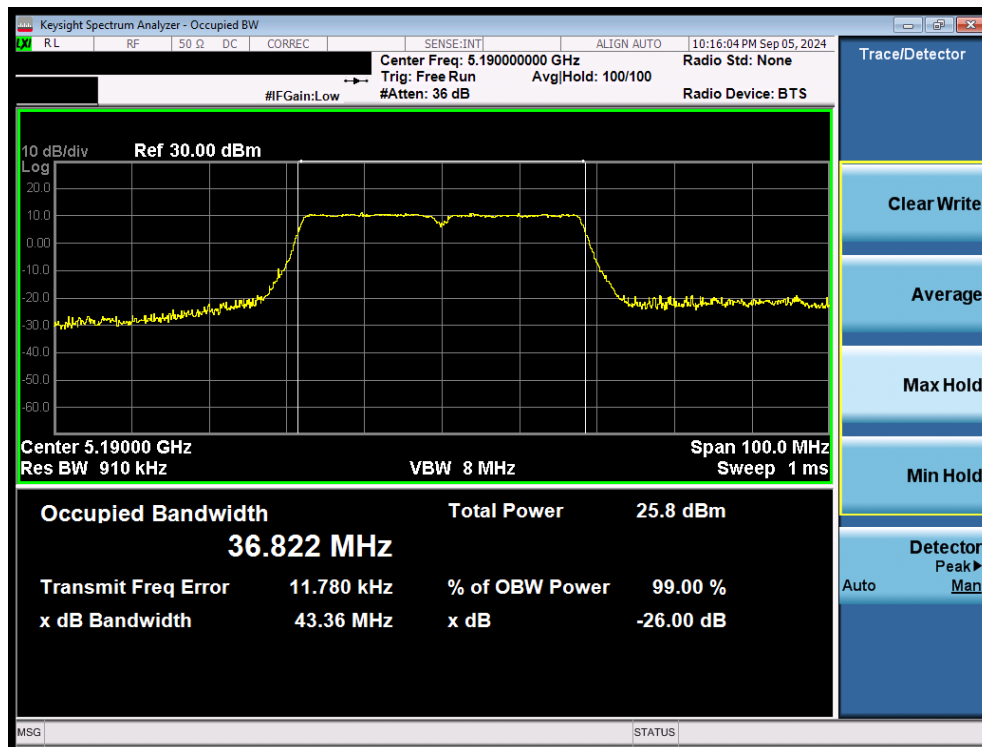
Plot 7-16. 26dB Bandwidth Plot MIMO ANT2 (40MHz 802.11n (UNII Band 1) – Ch. 38)
