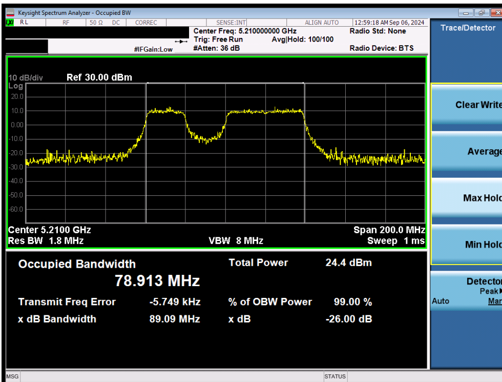
Plot 7-22. 26dB Bandwidth Plot MIMO ANT2 (80MHz 802.11be (20MHz Puncture) (UNII Band 1) – Ch. 42)
