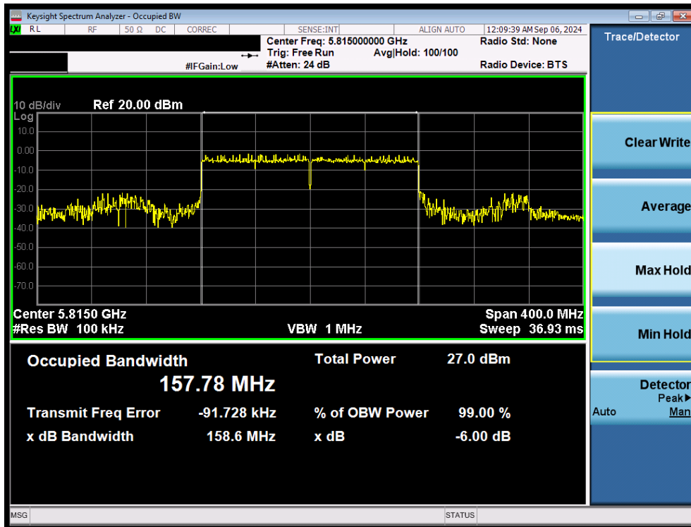
Plot 7-59. 6dB Bandwidth Plot MIMO ANT2 (160MHz 802.11ax/be (UNII Band 3/4) – Ch. 163)
