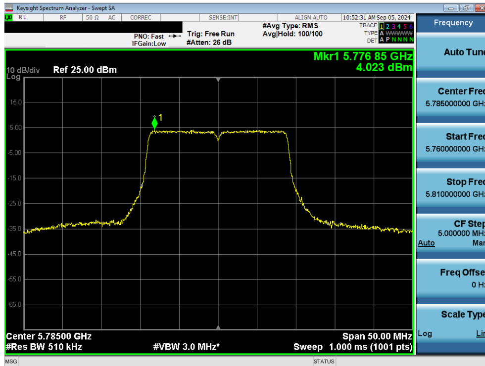
Plot 7-74. Power Spectral Density Plot MIMO ANT1 (20MHz 802.11n (UNII Band 3) – Ch.157)
