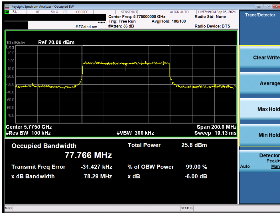
Plot 7-49. 6dB Bandwidth Plot MIMO ANT2 (80MHz 802.11ax/be (UNII Band 3) – Ch. 155)
