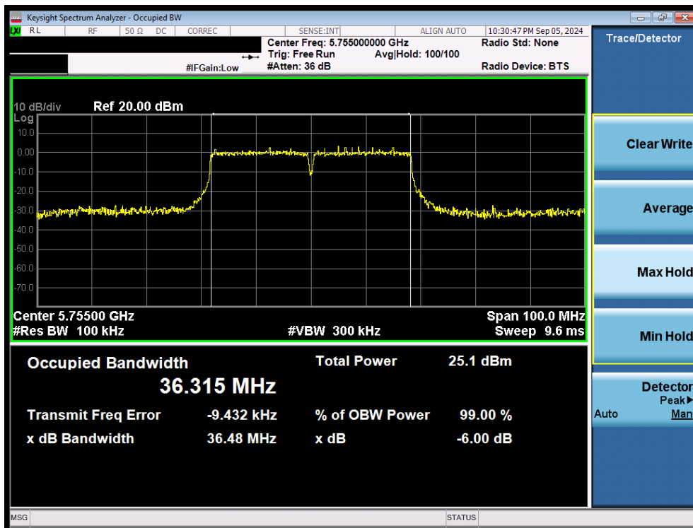
Plot 7-46. 6dB Bandwidth Plot MIMO ANT2 (40MHz 802.11n (UNII Band 3) – Ch. 151)
