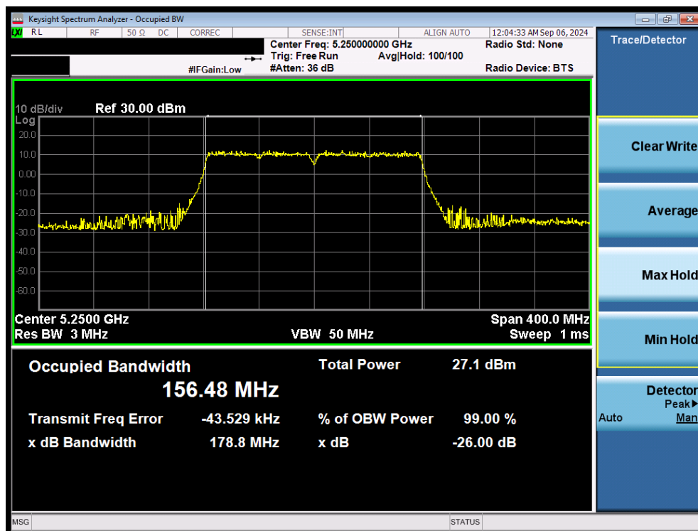
Plot 7-20. 26dB Bandwidth Plot MIMO ANT2 (160MHz 802.11ac (UNII Band 1/2A) – Ch. 50)
