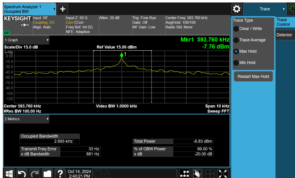
Plot 7-6. Occupied Bandwidth Measurement – Eraser
