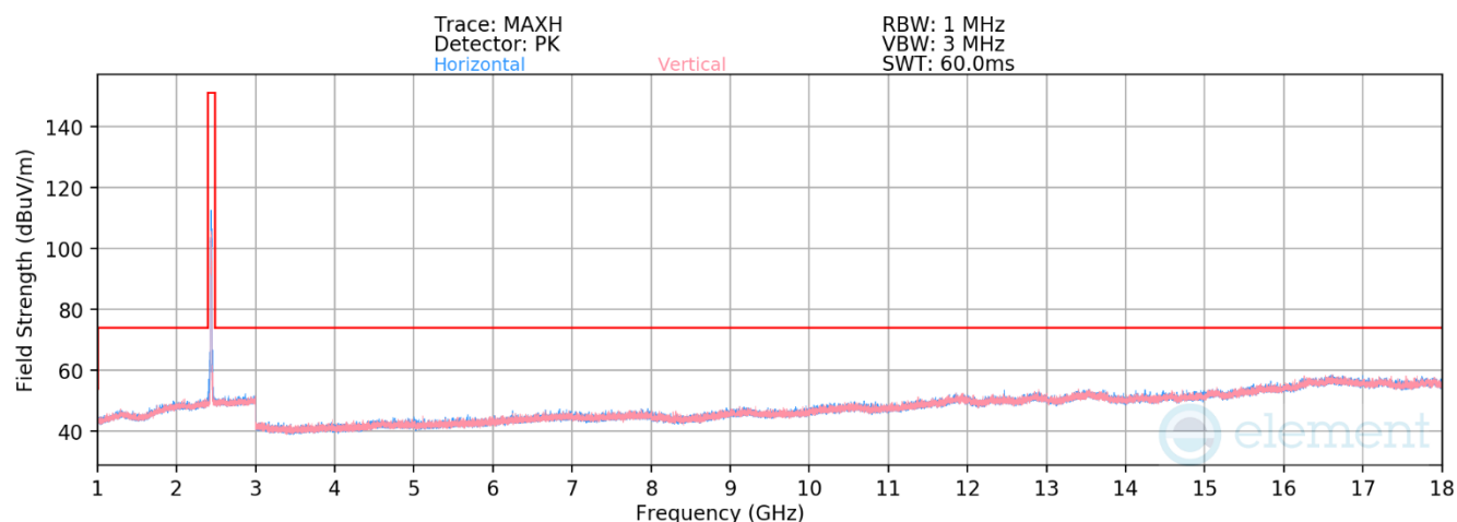
Plot 7-67. Radiated Spurious Plot above 1GHz MIMO (802.11ax/be OFDMA – 26 Tones – Ch. 6)
