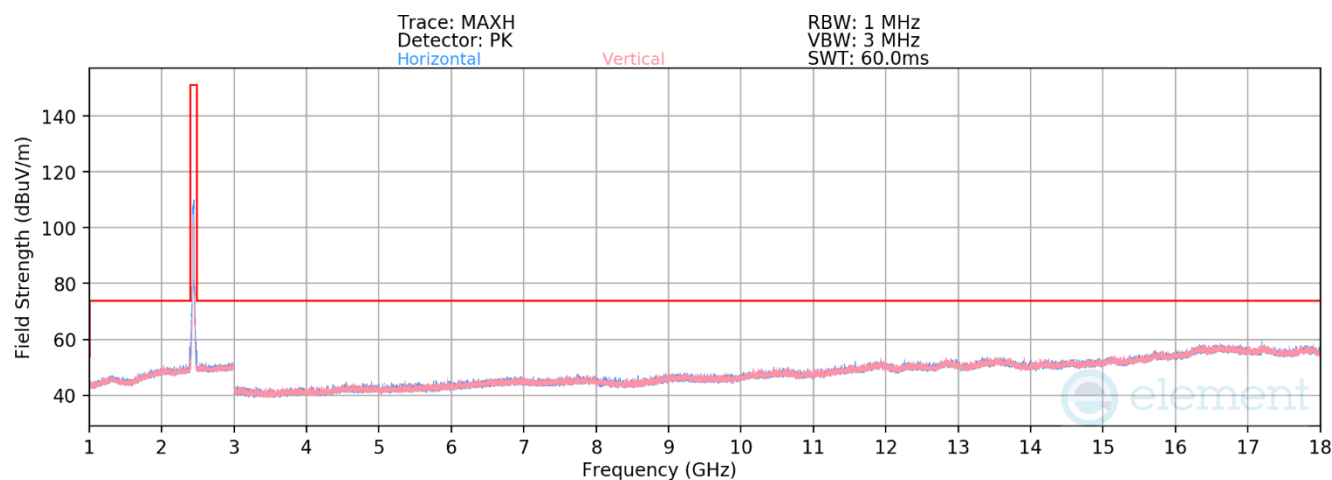
Plot 7-71. Radiated Spurious Plot above 1GHz MIMO (802.11ax/be OFDMA – 242 Tones – Ch. 6)
