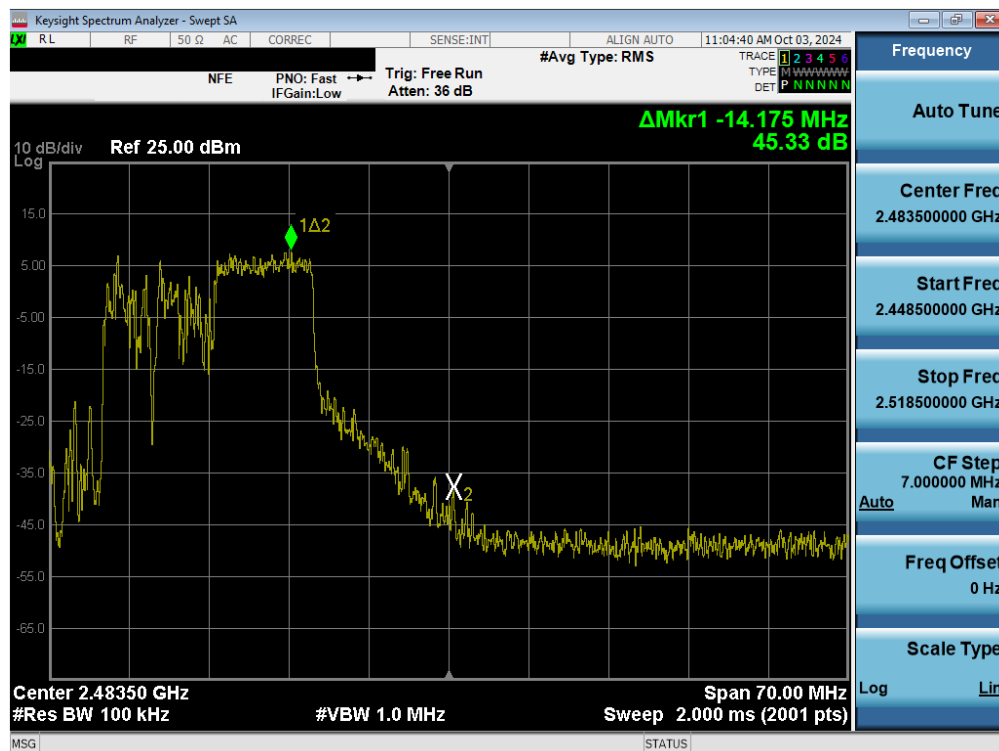
Plot 7-27. Band Edge Plot MIMO ANT1 (802.11ax/be OFDMA – 106 Tones – Ch. 11)
