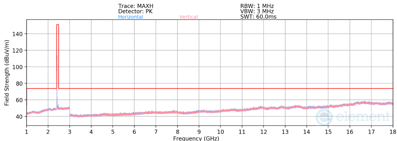
Plot 7-66. Radiated Spurious Plot above 1GHz MIMO (802.11ax/be OFDMA – 26 Tones – Ch. 1)
