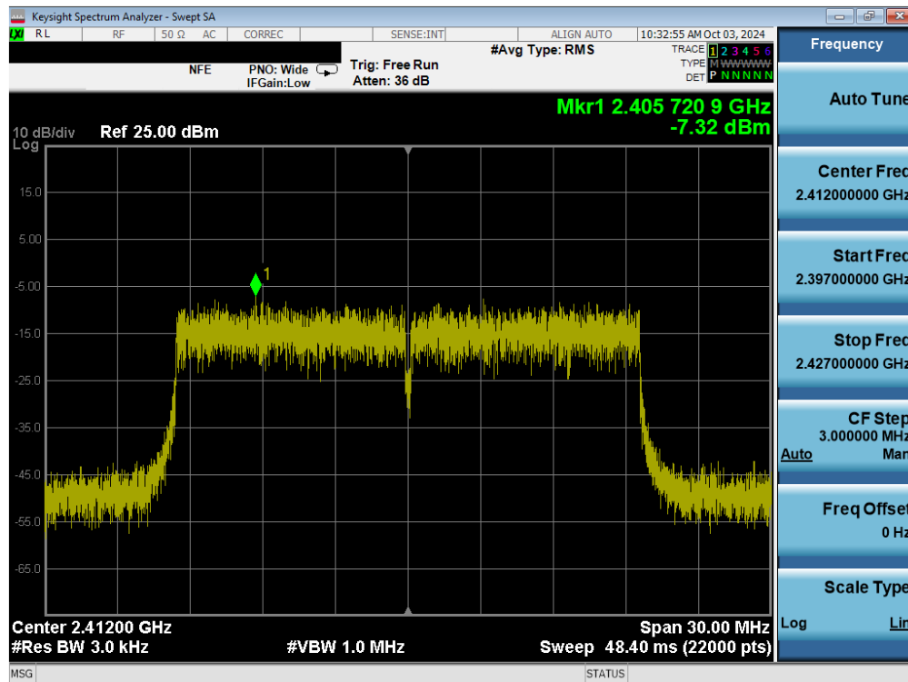
Plot 7-23. Power Spectral Density Plot MIMO ANT2 (802.11ax/be OFDMA – 242 Tones – Ch. 1)
