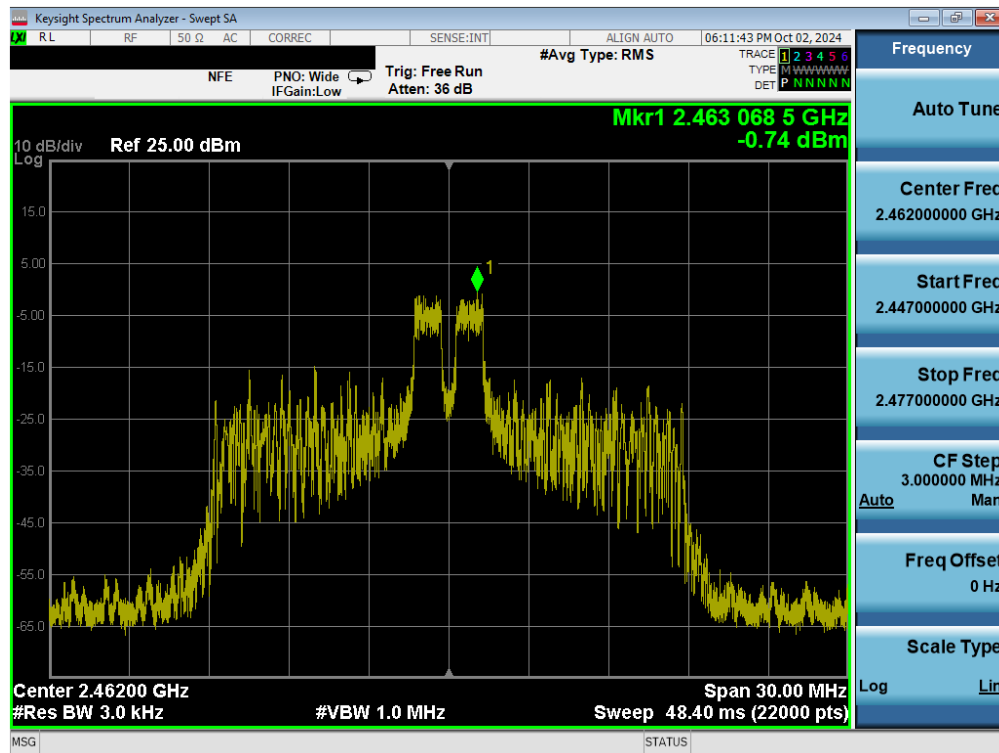
Plot 7-22. Power Spectral Density Plot MIMO ANT2 (802.11ax/be OFDMA – 26 Tones – Ch. 11)
