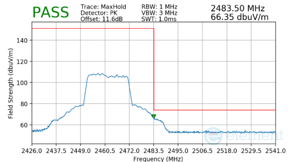
Plot 7-85. Radiated Restricted Upper Band Edge Measurement MIMO (Peak – 242 Tones)
