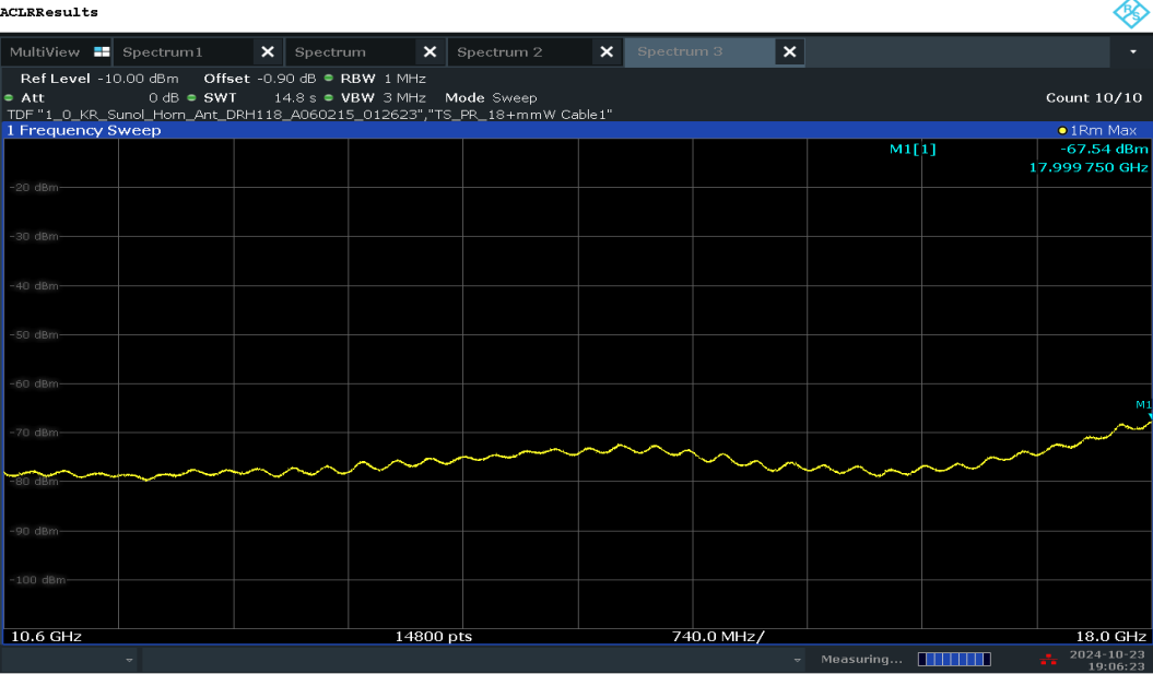
Plot 7-41. Radiated Spurious Pre-Scan 10600 - 18000 MHz - CH.5
