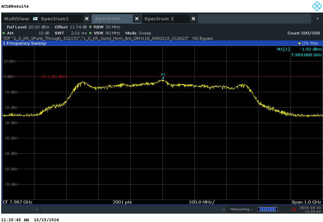
Plot 7-33. UWB Peak Power Measurement - CH.9 – BPRF
