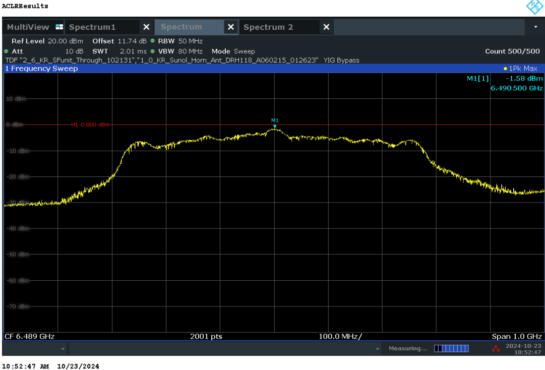
Plot 7-32. UWB Peak Power Measurement - CH.5 – BPRF
