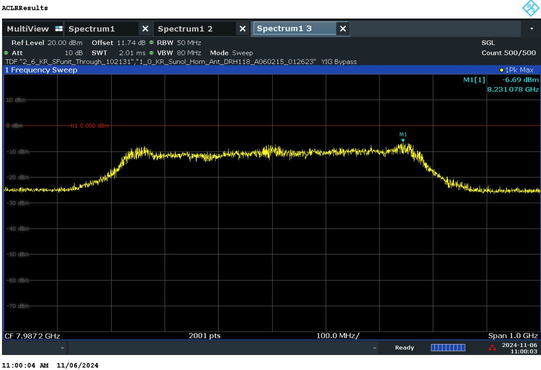
Plot 7-37. UWB Peak Power Measurement - CH.9 – HPRF
