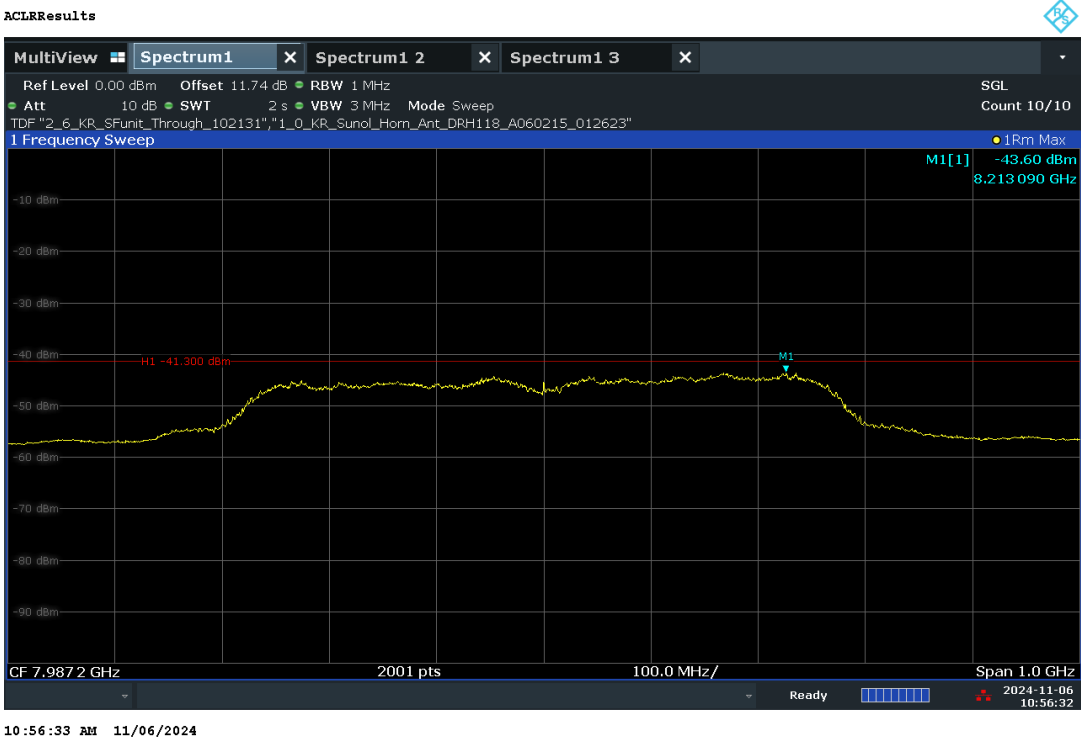
Plot 7-39. UWB Average Power Measurement - CH.9 – HPRF
