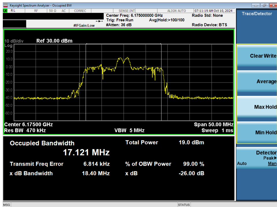
Plot 7-45. 26dB Bandwidth Plot MIMO ANT2 (20MHz 802.11ax/be (26 Tones) (UNII Band 5) – Ch. 45) - SP
