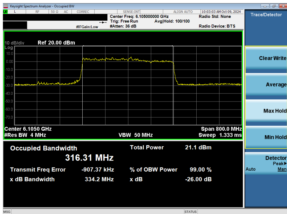
Plot 7-58. 26dB Bandwidth Plot MIMO ANT2 (320MHz 802.11ax/be (Full Tones) (UNII Band 5) – Ch. 31) - LPI
