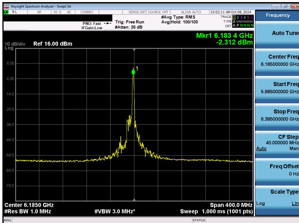
Plot 7-67. Power Spectral Density Plot MIMO ANT1 (160MHz 802.11ax/be (26 Tones) (UNII Band 5) – Ch. 47) - LPI
