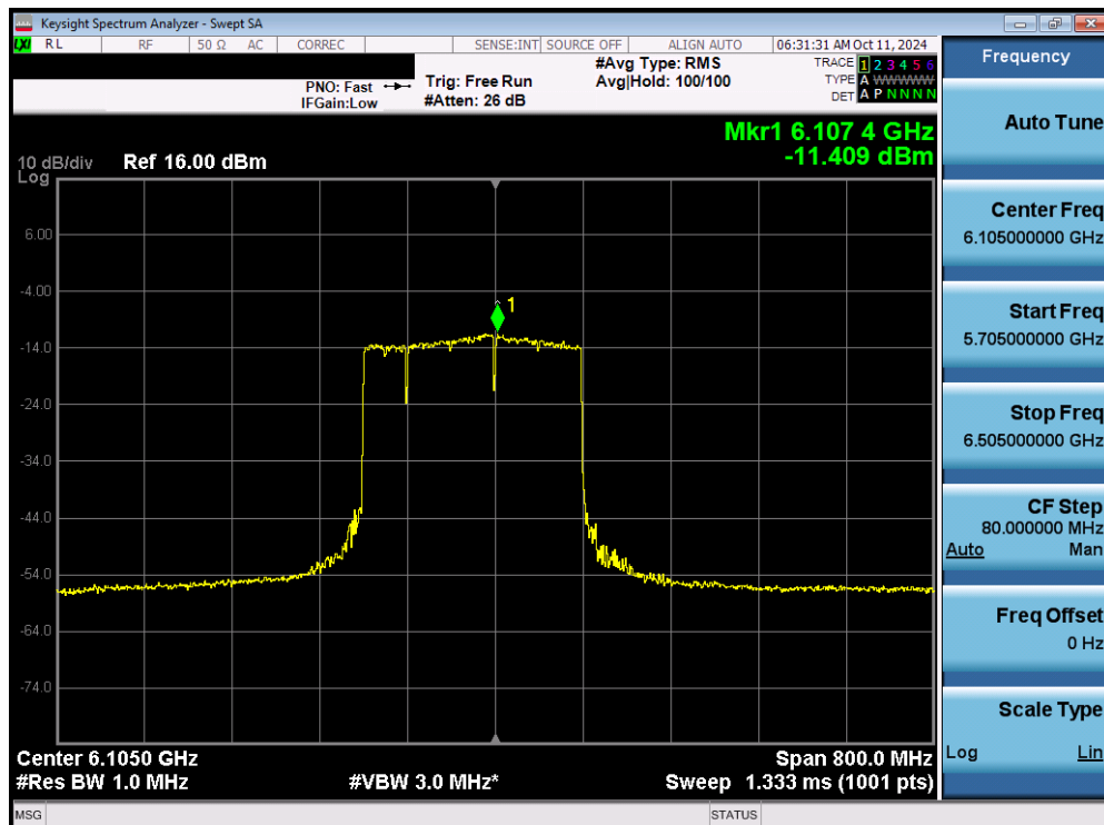
Plot 7-71. Power Spectral Density Plot MIMO ANT1 (320MHz 802.11be (UNII Band 5) – Ch. 31) LPI
