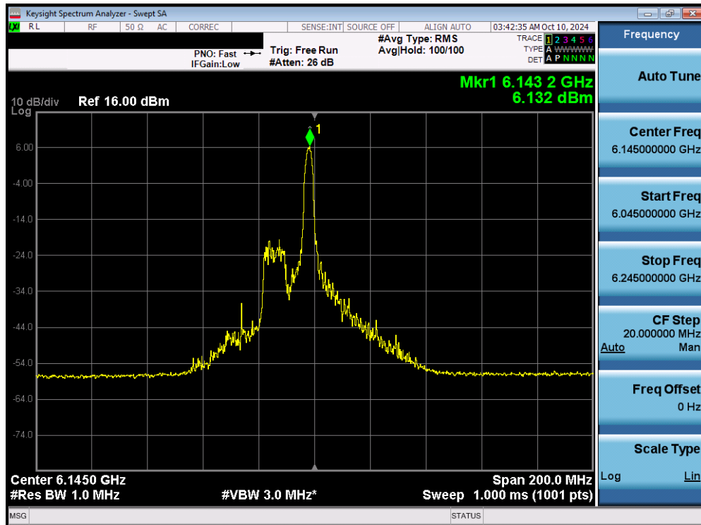
Plot 7-74. Power Spectral Density Plot MIMO ANT1 (80MHz 802.11ax/be (26 Tones) (UNII Band 5) – Ch. 39) - SP
