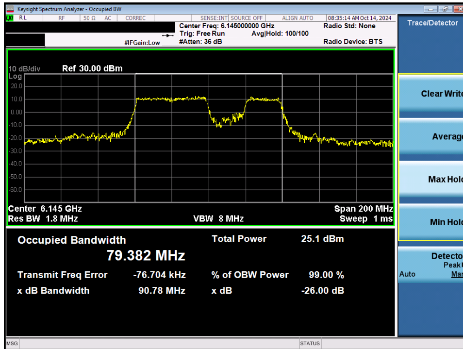
Plot 7-23. 26dB Bandwidth Plot MIMO ANT1 (80MHz 802.11be (484+242 Tones) (UNII Band 5) – Ch. 39) SP
