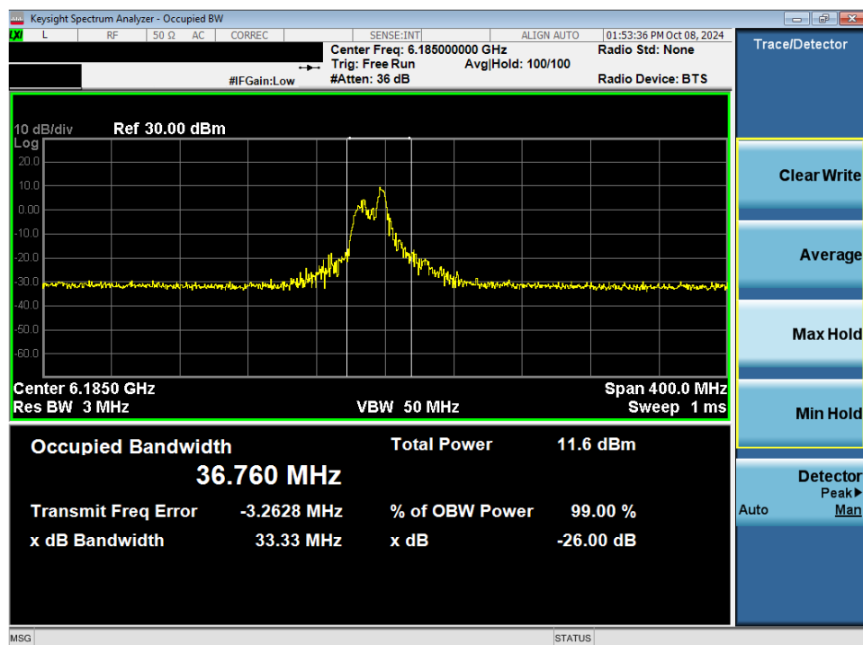
Plot 7-39. 26dB Bandwidth Plot MIMO ANT2 (160MHz 802.11ax/be (26 Tones) (UNII Band 5) – Ch. 47) - LPI
