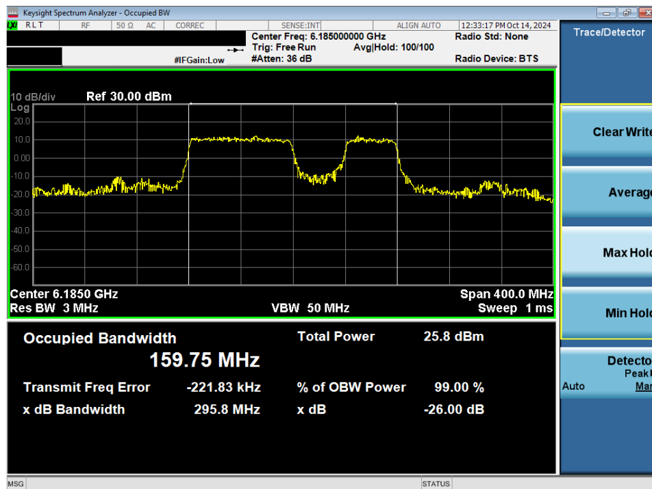
Plot 7-52. 26dB Bandwidth Plot MIMO ANT2 (160MHz 802.11be (996+484 Tones) (UNII Band 5) – Ch. 47) SP
