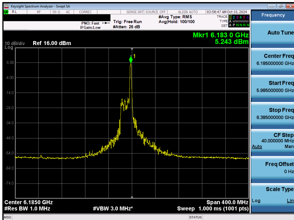
Plot 7-75. Power Spectral Density Plot MIMO ANT1 (160MHz 802.11ax/be (26 Tones) (UNII Band 5) – Ch. 47) - SP
