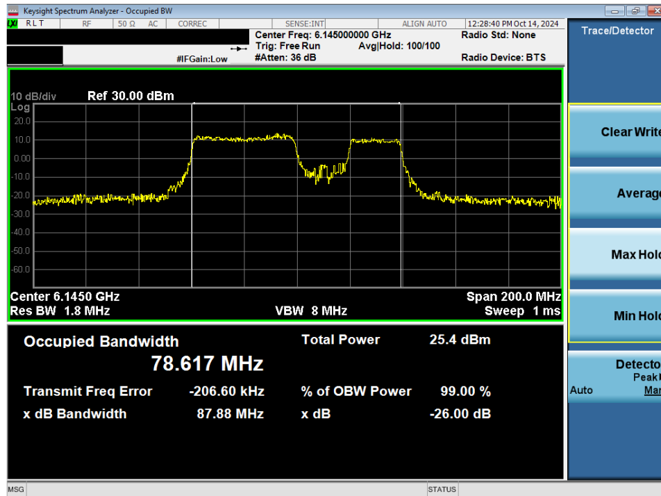
Plot 7-51. 26dB Bandwidth Plot MIMO ANT2 (80MHz 802.11be (484+242 Tones) (UNII Band 5) – Ch. 39) SP
