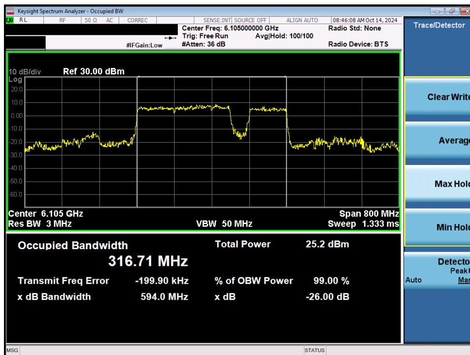
Plot 7-25. 26dB Bandwidth Plot MIMO ANT1 (320MHz 802.11be (3*996+484 Tones) (UNII Band 5) – Ch. 31) SP
