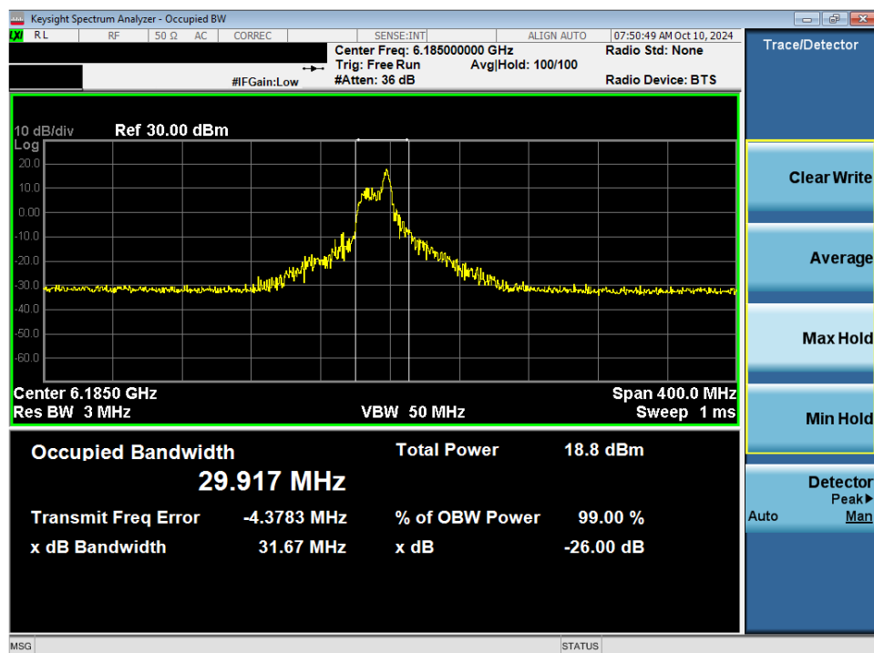
Plot 7-48. 26dB Bandwidth Plot MIMO ANT2 (160MHz 802.11ax/be (26 Tones) (UNII Band 5) – Ch. 47) - SP
