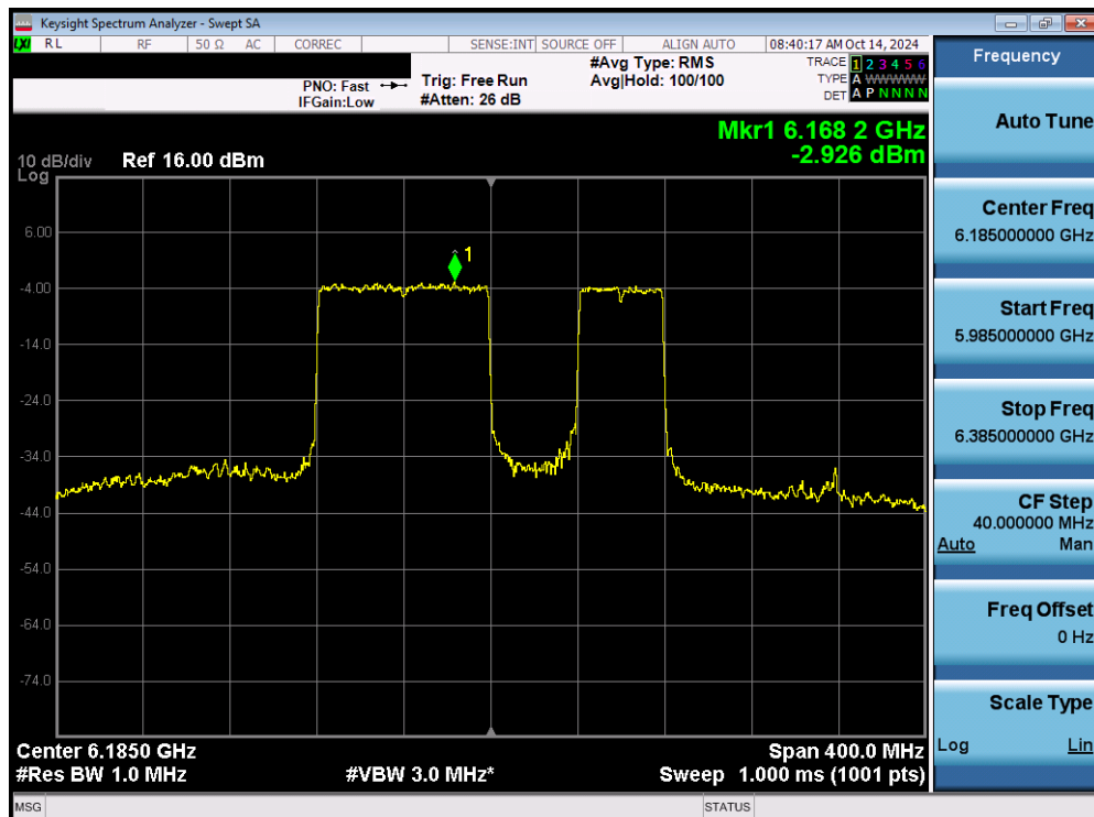
Plot 7-79. Power Spectral Density Plot MIMO ANT1 (160MHz 802.11be (996+484 Tones) (UNII Band 5) – Ch. 47) SP
