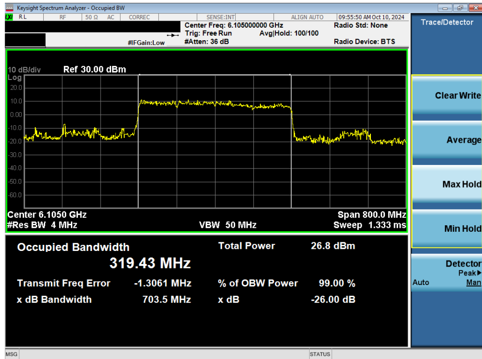
Plot 7-63. 26dB Bandwidth Plot MIMO ANT2 (320MHz 802.11ax/be (Full Tones) (UNII Band 5) – Ch. 31) - SP
