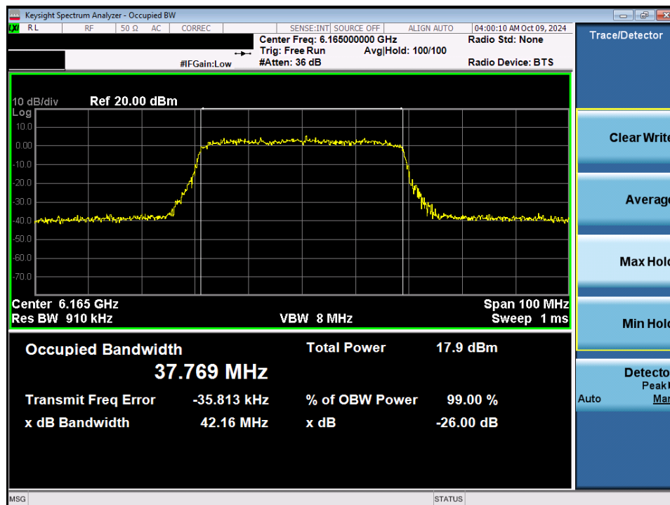
Plot 7-27. 26dB Bandwidth Plot MIMO ANT1 (40MHz 802.11ax/be (Full Tones) (UNII Band 5) – Ch. 43) - LPI
