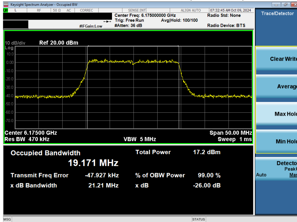
Plot 7-54. 26dB Bandwidth Plot MIMO ANT2 (20MHz 802.11ax/be (Full Tones) (UNII Band 5) – Ch. 45) - LPI
