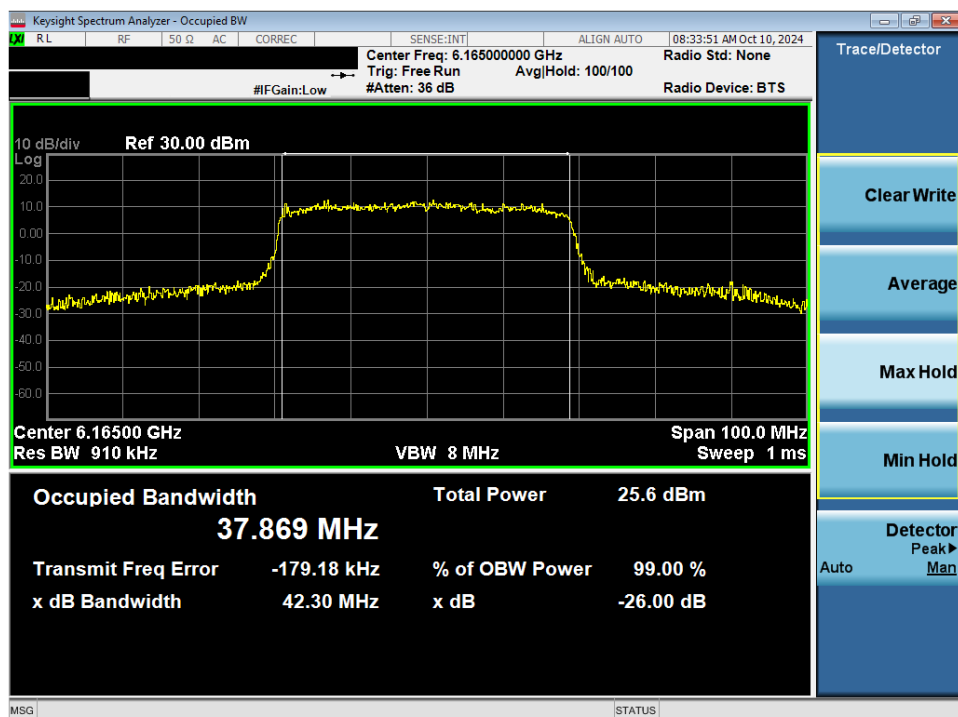
Plot 7-60. 26dB Bandwidth Plot MIMO ANT2 (40MHz 802.11ax/be (Full Tones) (UNII Band 5) – Ch. 43) - SP
