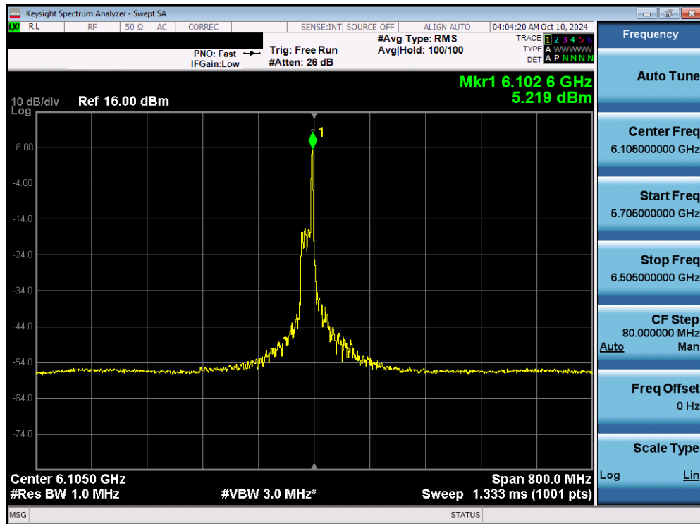
Plot 7-76. Power Spectral Density Plot MIMO ANT1 (320MHz 802.11ax/be (26 Tones) (UNII Band 5) – Ch. 31) - SP
