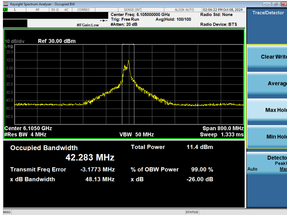
Plot 7-40. 26dB Bandwidth Plot MIMO ANT2 (320MHz 802.11ax/be (26 Tones) (UNII Band 5) – Ch. 31) - LPI
