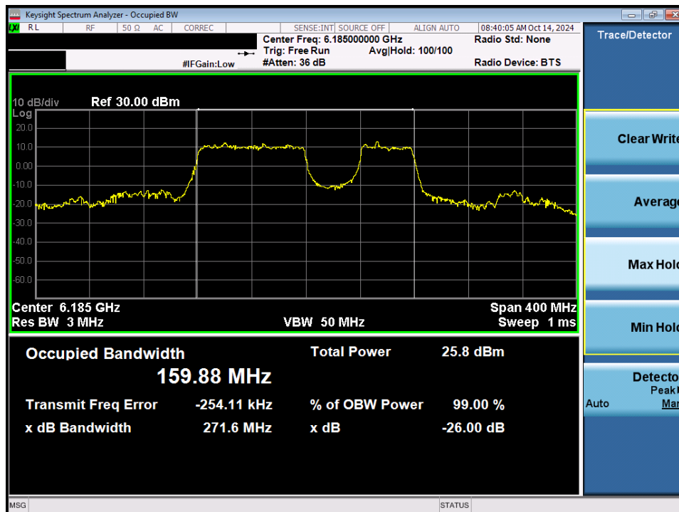
Plot 7-24. 26dB Bandwidth Plot MIMO ANT1 (160MHz 802.11be (996+484 Tones) (UNII Band 5) – Ch. 47) SP
