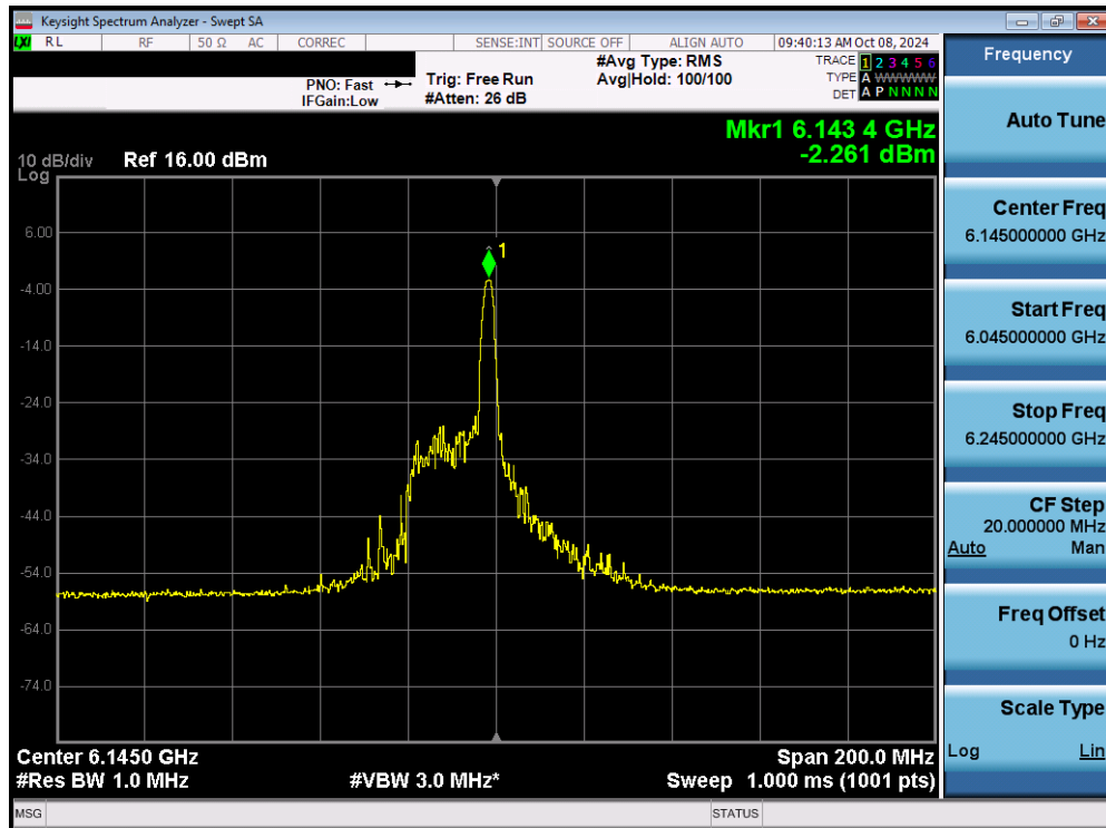
Plot 7-66. Power Spectral Density Plot MIMO ANT1 (80MHz 802.11ax/be (26 Tones) (UNII Band 5) – Ch. 39) - LPI
