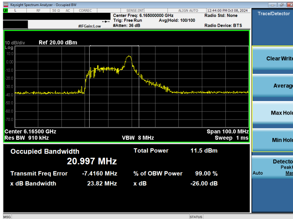
Plot 7-37. 26dB Bandwidth Plot MIMO ANT2 (40MHz 802.11ax/be (26 Tones) (UNII Band 5) – Ch. 43) - LPI
