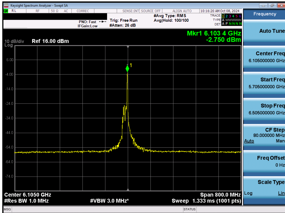
Plot 7-68. Power Spectral Density Plot MIMO ANT1 (320MHz 802.11ax/be (26 Tones) (UNII Band 5) – Ch. 31) - LPI
