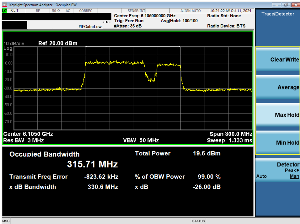
Plot 7-44. 26dB Bandwidth Plot MIMO ANT2 (320MHz 802.11be (3*996+484 Tones) (UNII Band 5) – Ch. 31) LPI
