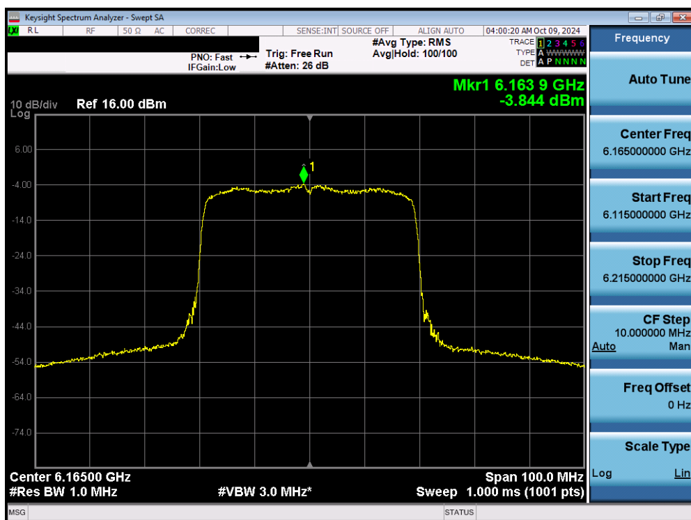
Plot 7-82. Power Spectral Density Plot MIMO ANT1 (40MHz 802.11ax/be (Full Tones) (UNII Band 5) – Ch. 43) - LPI
