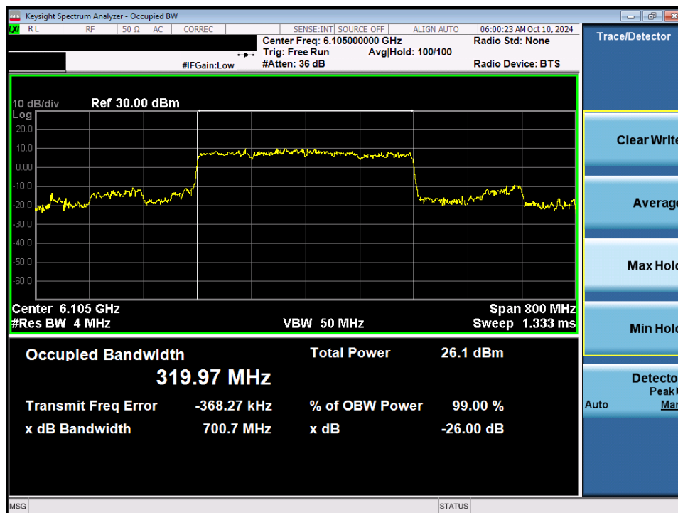
Plot 7-35. 26dB Bandwidth Plot MIMO ANT1 (320MHz 802.11ax/be (Full Tones) (UNII Band 5) – Ch. 31) - SP
