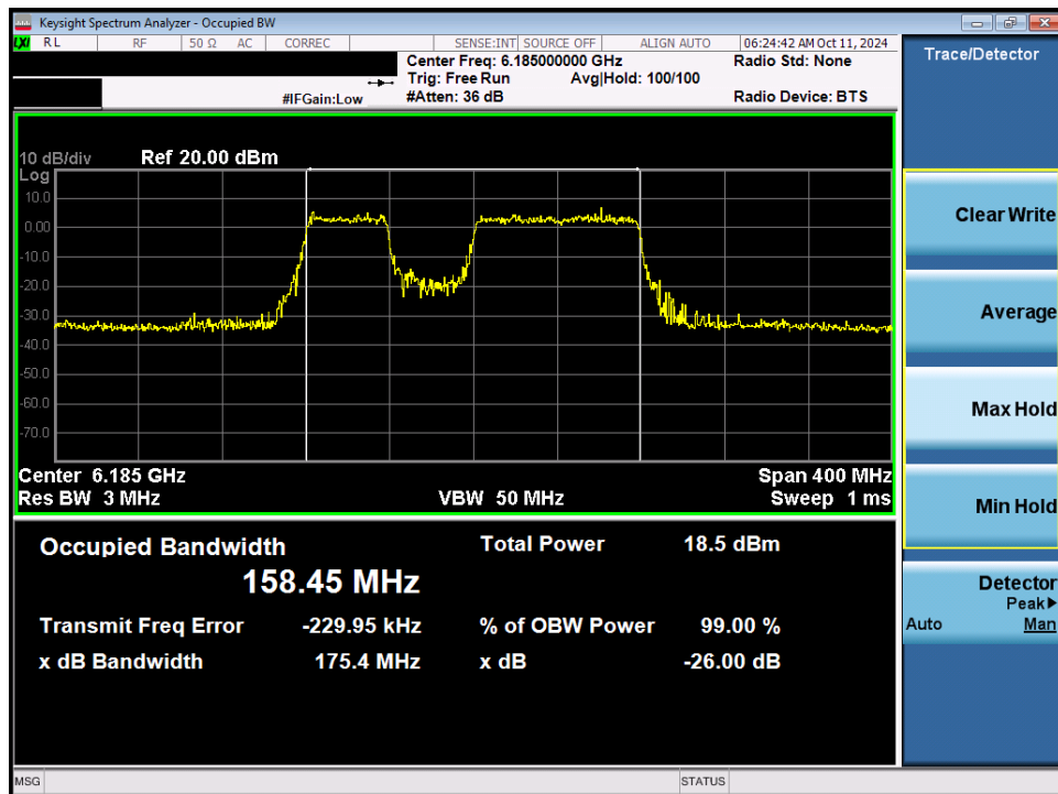
Plot 7-15. 26dB Bandwidth Plot MIMO ANT1 (160MHz 802.11be (996+484 Tones) (UNII Band 5) – Ch. 47) LPI
