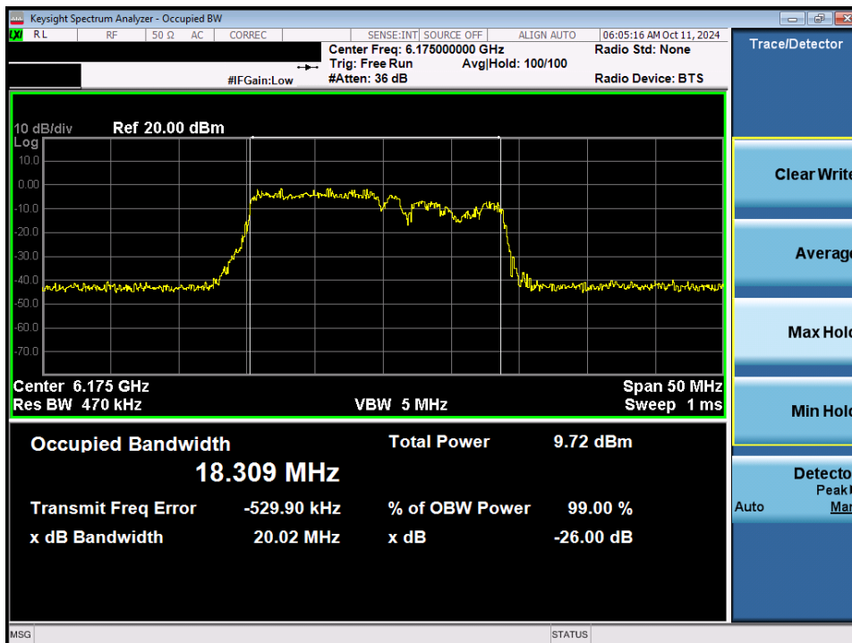
Plot 7-41. 26dB Bandwidth Plot MIMO ANT2 (20MHz 802.11be (106+26 Tones) (UNII Band 5) – Ch. 45) - LPI
