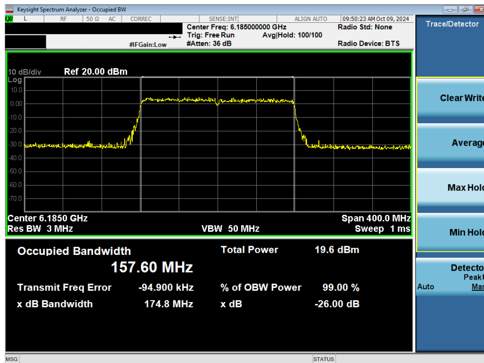
Plot 7-57. 26dB Bandwidth Plot MIMO ANT2 (160MHz 802.11ax/be (Full Tones) (UNII Band 5) – Ch. 47) - LPI
