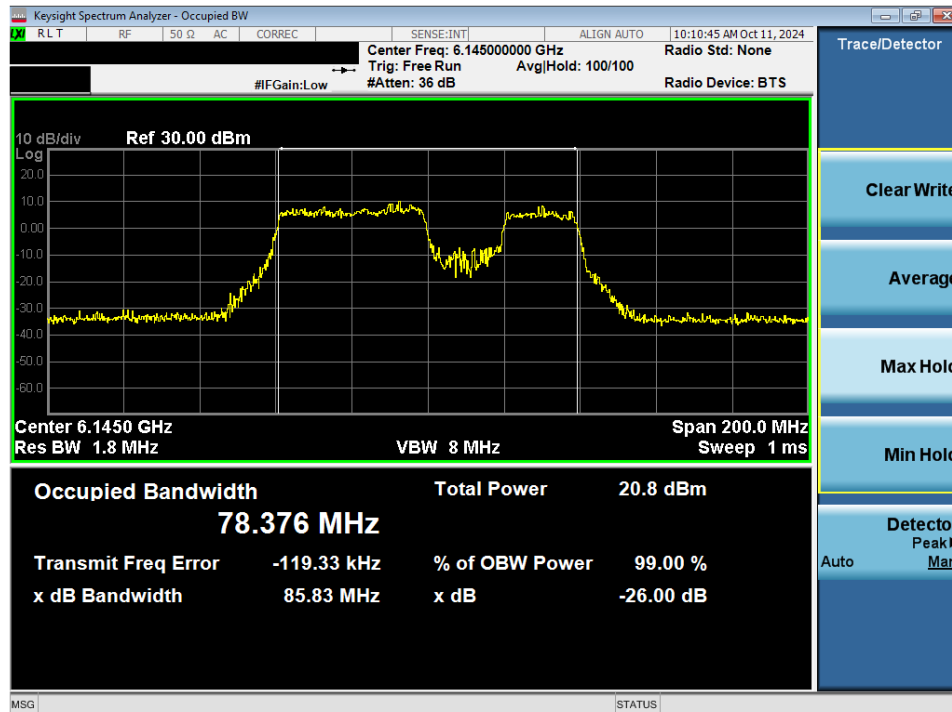
Plot 7-42. 26dB Bandwidth Plot MIMO ANT2 (80MHz 802.11be (484+242 Tones) (UNII Band 5) – Ch. 39) LPI
