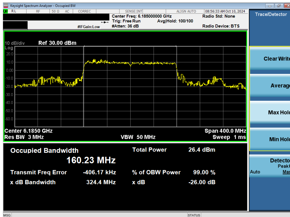
Plot 7-62. 26dB Bandwidth Plot MIMO ANT2 (160MHz 802.11ax/be (Full Tones) (UNII Band 5) – Ch. 47) - SP
