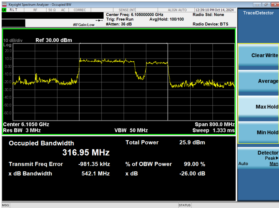
Plot 7-53. 26dB Bandwidth Plot MIMO ANT2 (320MHz 802.11be (3*996+484 Tones) (UNII Band 5) – Ch. 31) SP
