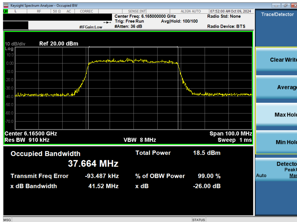
Plot 7-55. 26dB Bandwidth Plot MIMO ANT2 (40MHz 802.11ax/be (Full Tones) (UNII Band 5) – Ch. 43) - LPI
