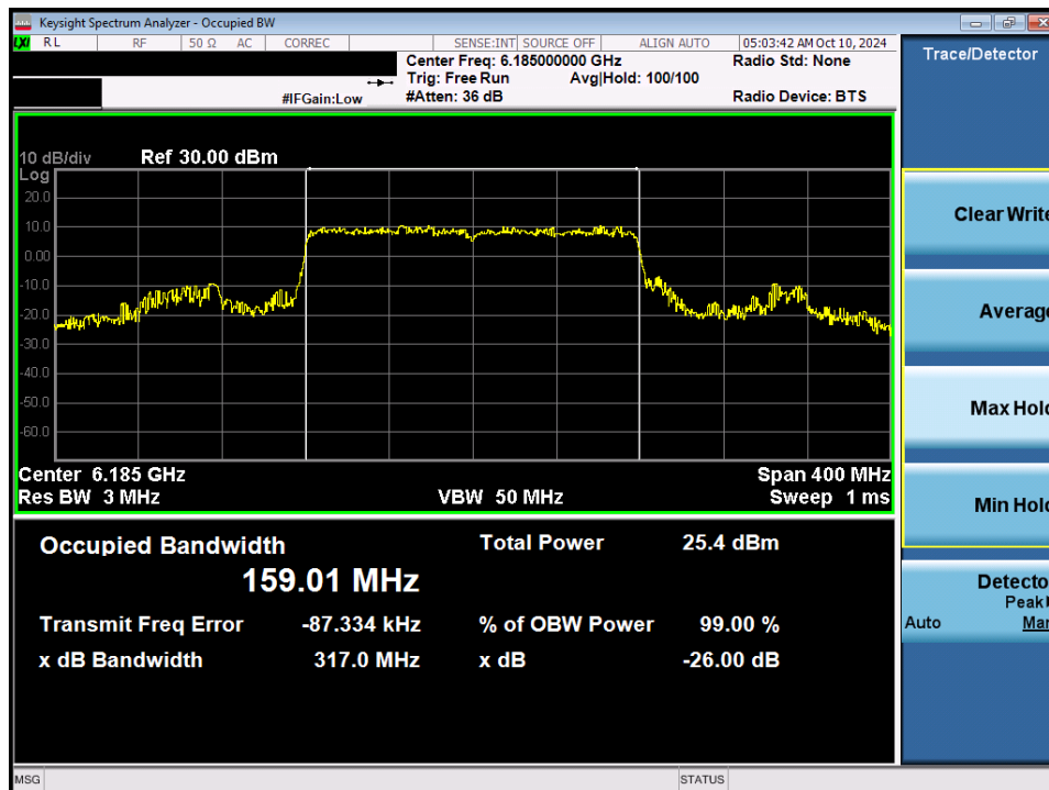
Plot 7-34. 26dB Bandwidth Plot MIMO ANT1 (160MHz 802.11ax/be (Full Tones) (UNII Band 5) – Ch. 47) - SP
