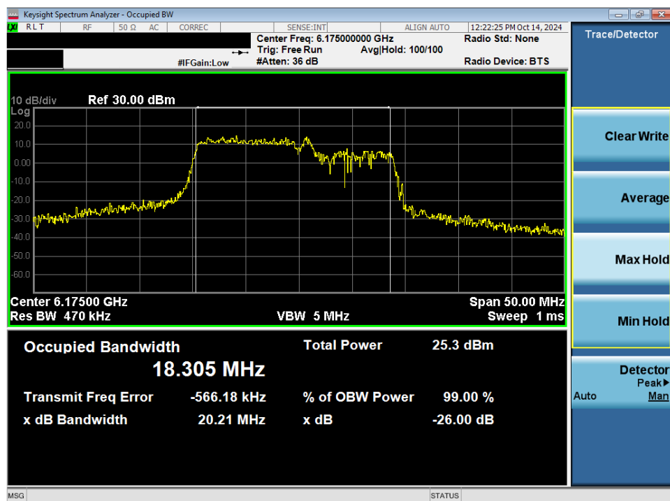
Plot 7-50. 26dB Bandwidth Plot MIMO ANT2 (20MHz 802.11be (106+26 Tones) (UNII Band 5) – Ch. 45) - SP
