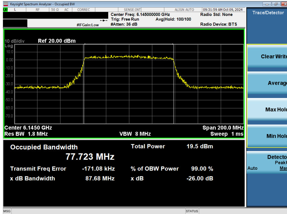
Plot 7-56. 26dB Bandwidth Plot MIMO ANT2 (80MHz 802.11ax/be (Full Tones) (UNII Band 5) – Ch. 39) - LPI
