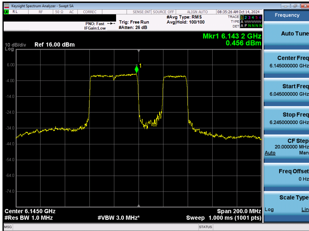
Plot 7-78. Power Spectral Density Plot MIMO ANT1 (80MHz 802.11be (484+242 Tones) (UNII Band 5) – Ch. 39) SP
