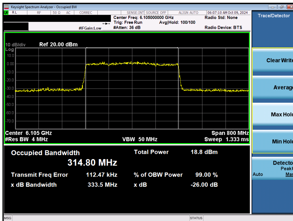
Plot 7-30. 26dB Bandwidth Plot MIMO ANT1 (320MHz 802.11ax/be (Full Tones) (UNII Band 5) – Ch. 31) - LPI
