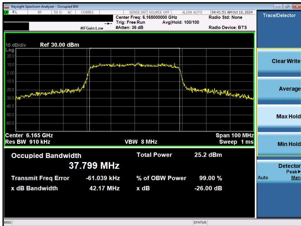
Plot 7-32. 26dB Bandwidth Plot MIMO ANT1 (40MHz 802.11ax/be (Full Tones) (UNII Band 5) – Ch. 43) - SP
