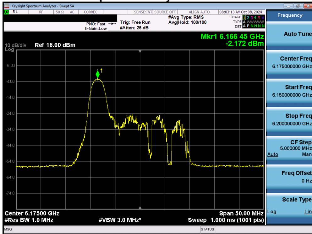
Plot 7-64. Power Spectral Density Plot MIMO ANT1 (20MHz 802.11ax/be (26 Tones) (UNII Band 5) – Ch. 45) - LPI
