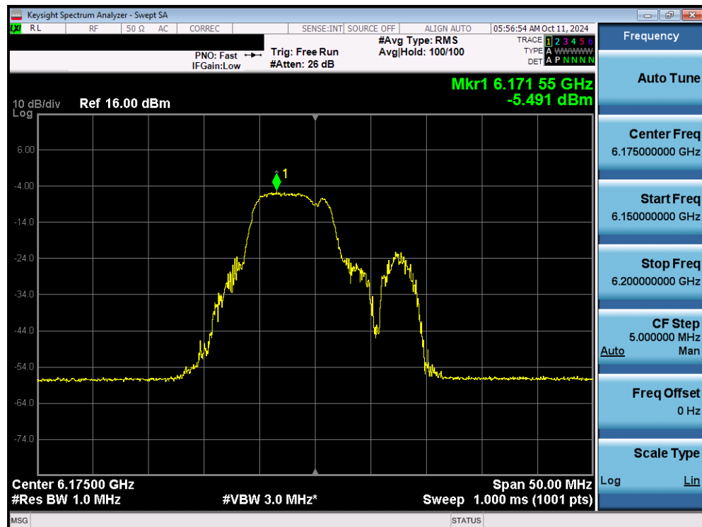
Plot 7-69. Power Spectral Density Plot MIMO ANT1 (20MHz 802.11be (52+26 Tones) (UNII Band 5) – Ch. 45) - LPI
