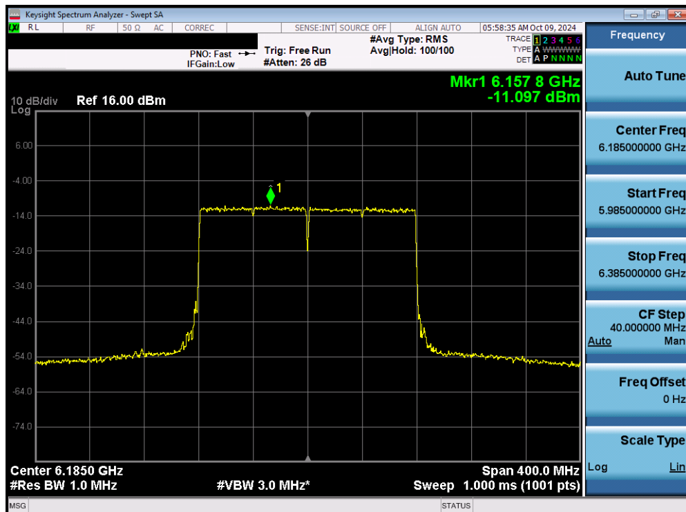
Plot 7-84. Power Spectral Density Plot MIMO ANT1 (160MHz 802.11ax/be (Full Tones) (UNII Band 5) – Ch. 47) - LPI
