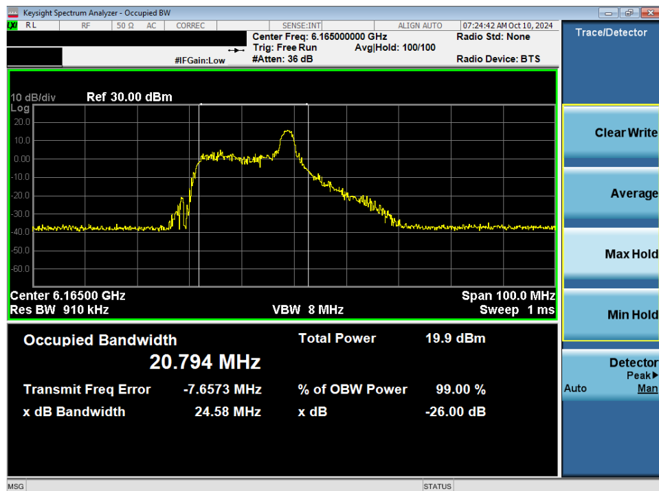
Plot 7-46. 26dB Bandwidth Plot MIMO ANT2 (40MHz 802.11ax/be (26 Tones) (UNII Band 5) – Ch. 43) - SP
