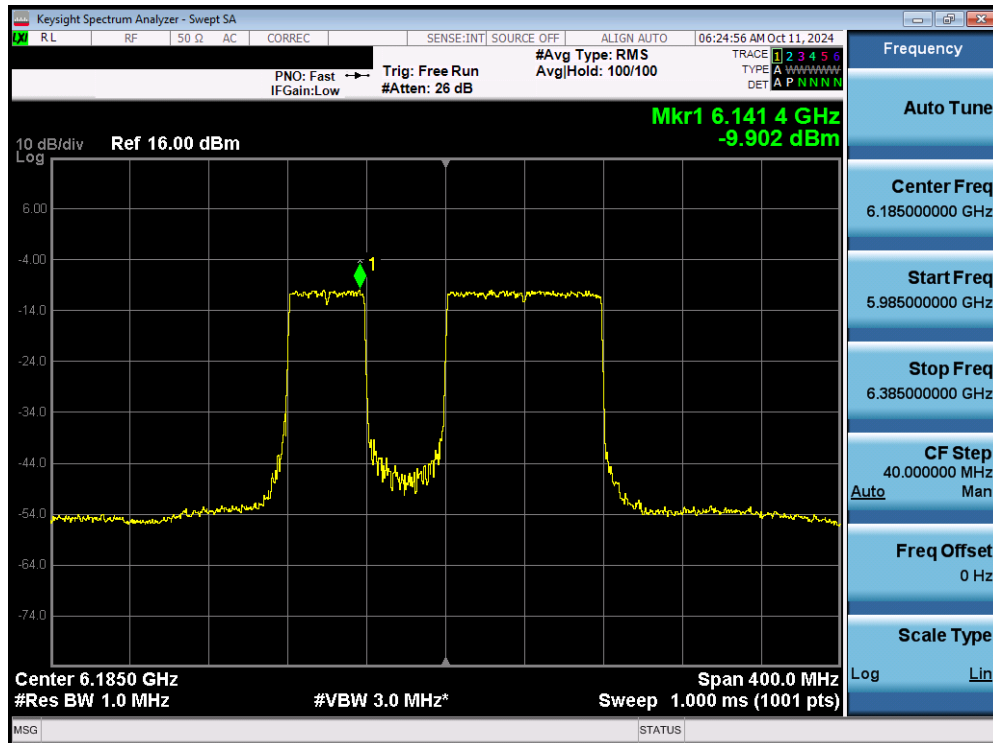
Plot 7-70. Power Spectral Density Plot MIMO ANT1 (160MHz 802.11be (996+484 Tones) (UNII Band 5) – Ch. 47) LPI
