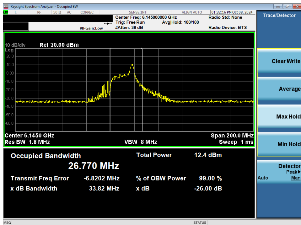
Plot 7-38. 26dB Bandwidth Plot MIMO ANT2 (80MHz 802.11ax/be (26 Tones) (UNII Band 5) – Ch. 39) - LPI
