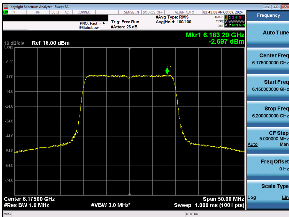
Plot 7-81. Power Spectral Density Plot MIMO ANT1 (20MHz 802.11ax/be (Full Tones) (UNII Band 5) – Ch. 45) - LPI
