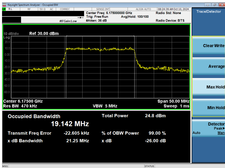
Plot 7-59. 26dB Bandwidth Plot MIMO ANT2 (20MHz 802.11ax/be (Full Tones) (UNII Band 5) – Ch. 45) - SP
