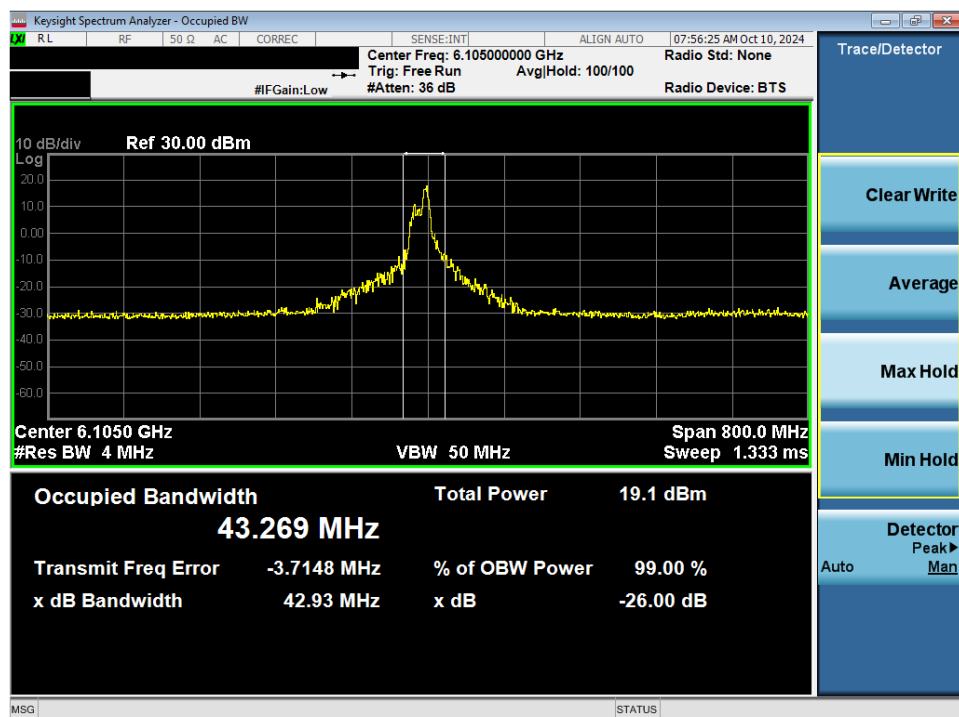
Plot 7-49. 26dB Bandwidth Plot MIMO ANT2 (320MHz 802.11ax/be (26 Tones) (UNII Band 5) – Ch. 31) - SP
