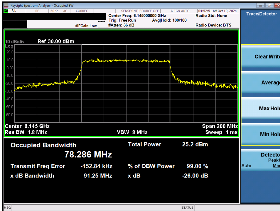
Plot 7-33. 26dB Bandwidth Plot MIMO ANT1 (80MHz 802.11ax/be (Full Tones) (UNII Band 5) – Ch. 39) - SP
