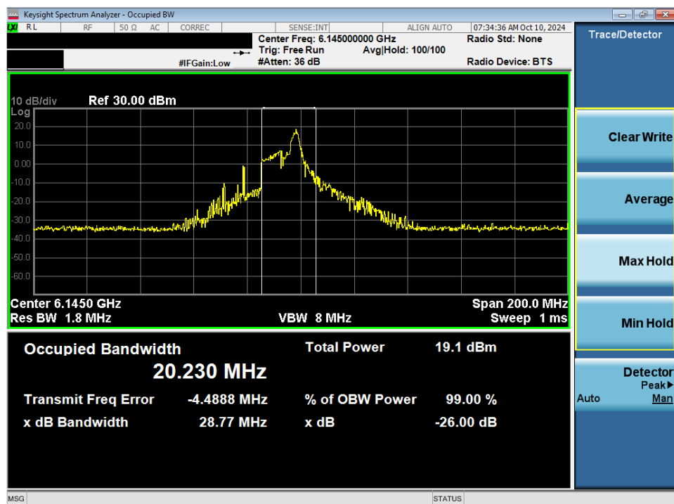
Plot 7-47. 26dB Bandwidth Plot MIMO ANT2 (80MHz 802.11ax/be (26 Tones) (UNII Band 5) – Ch. 39) - SP
