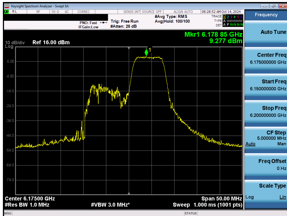
Plot 7-77. Power Spectral Density Plot MIMO ANT1 (20MHz 802.11be (52+26 Tones) (UNII Band 5) – Ch. 45) - SP
