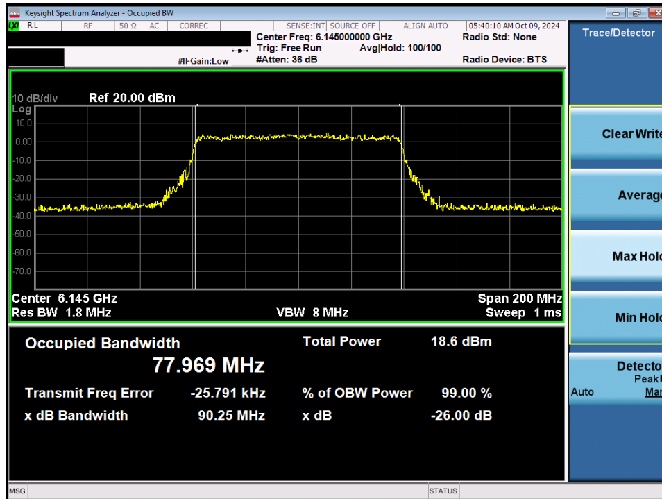
Plot 7-28. 26dB Bandwidth Plot MIMO ANT1 (80MHz 802.11ax/be (Full Tones) (UNII Band 5) – Ch. 39) - LPI
