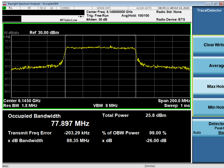
Plot 7-61. 26dB Bandwidth Plot MIMO ANT2 (80MHz 802.11ax/be (Full Tones) (UNII Band 5) – Ch. 39) - SP
