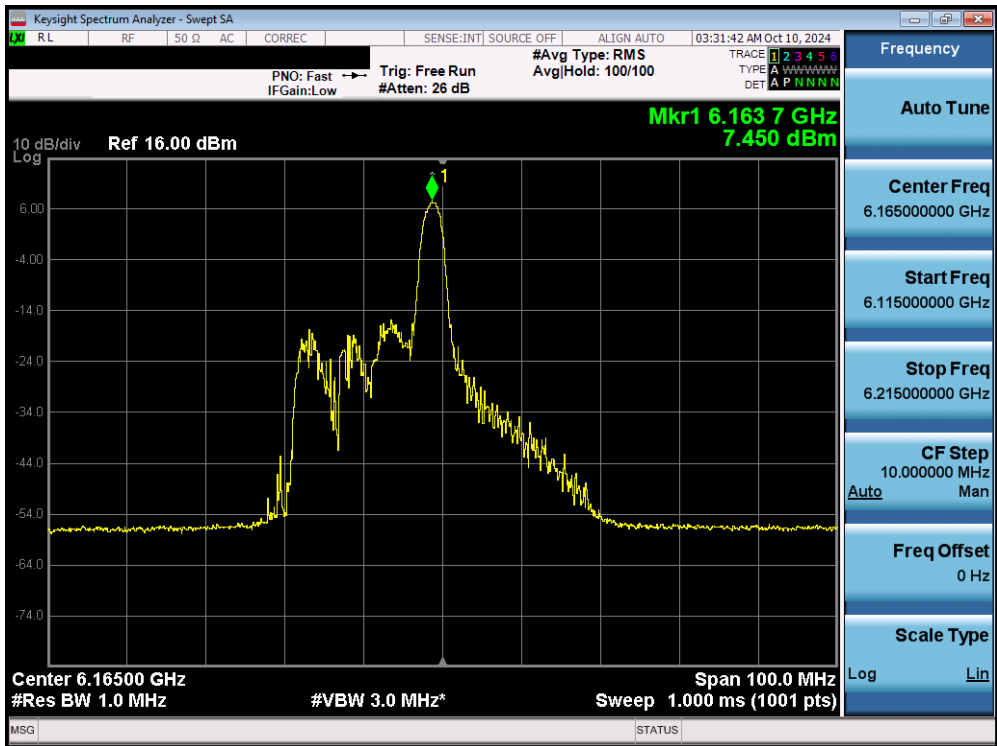
Plot 7-73. Power Spectral Density Plot MIMO ANT1 (40MHz 802.11ax/be (26 Tones) (UNII Band 5) – Ch. 43) - SP
