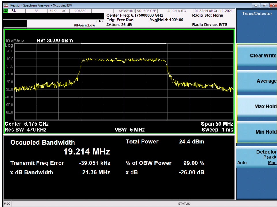
Plot 7-31. 26dB Bandwidth Plot MIMO ANT1 (20MHz 802.11ax/be (Full Tones) (UNII Band 5) – Ch. 45) - SP
