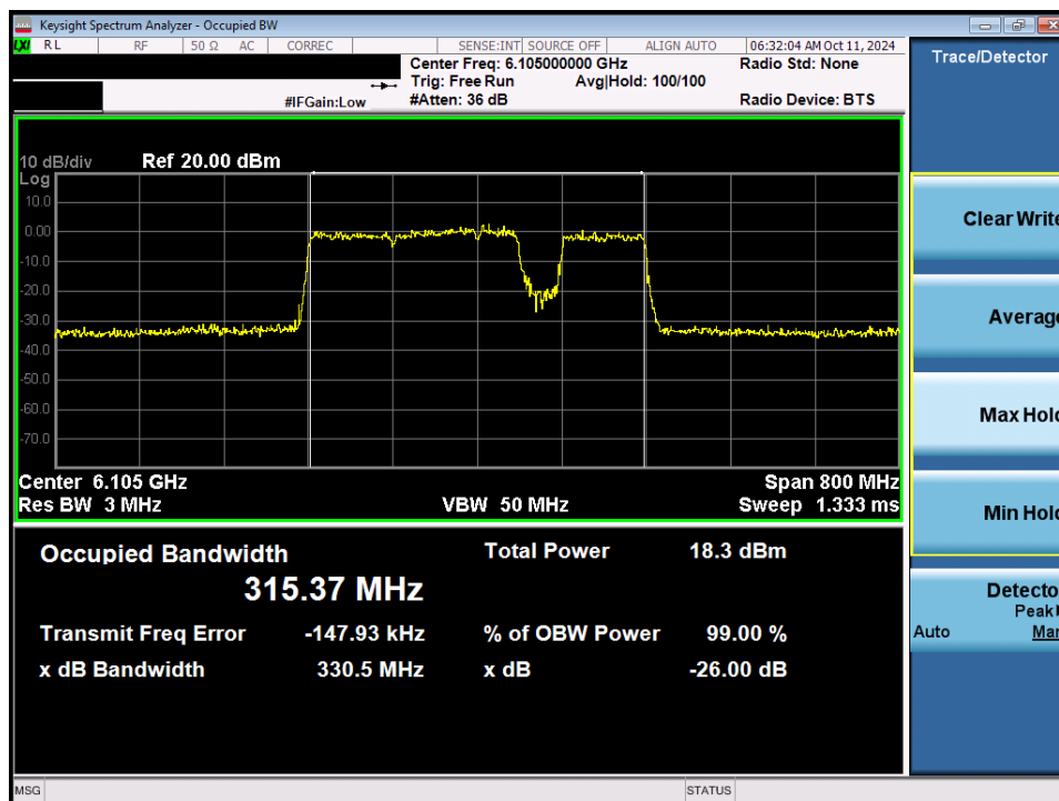
Plot 7-16. 26dB Bandwidth Plot MIMO ANT1 (320MHz 802.11be (3*996+484 Tones) (UNII Band 5) – Ch. 31) LPI
