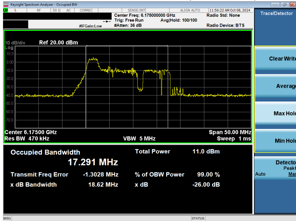
Plot 7-36. 26dB Bandwidth Plot MIMO ANT2 (20MHz 802.11ax/be (26 Tones) (UNII Band 5) – Ch. 45) - LPI
