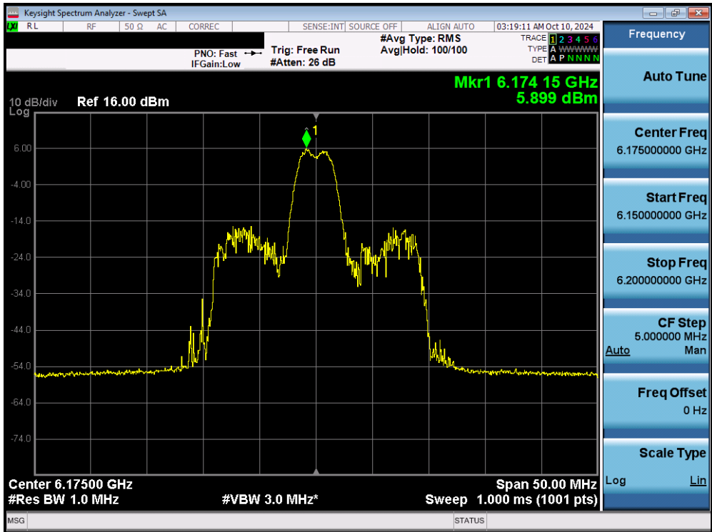
Plot 7-72. Power Spectral Density Plot MIMO ANT1 (20MHz 802.11ax/be (26 Tones) (UNII Band 5) – Ch. 45) - SP
