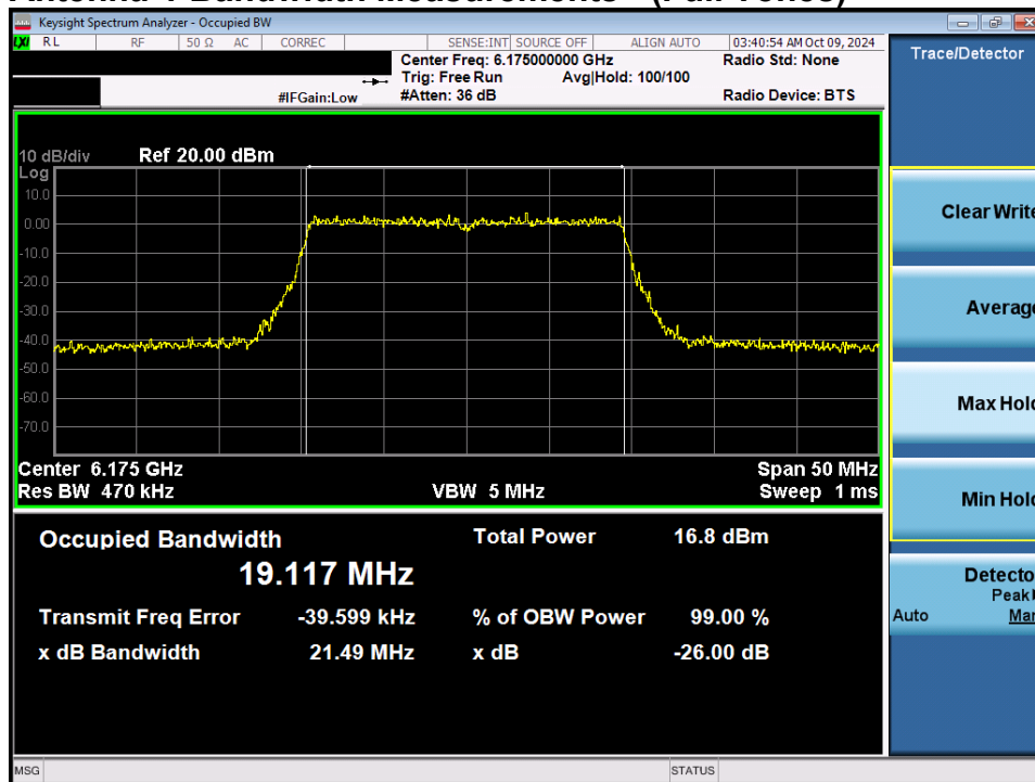
Plot 7-26. 26dB Bandwidth Plot MIMO ANT1 (20MHz 802.11ax/be (Full Tones) (UNII Band 5) – Ch. 45) - LPI
