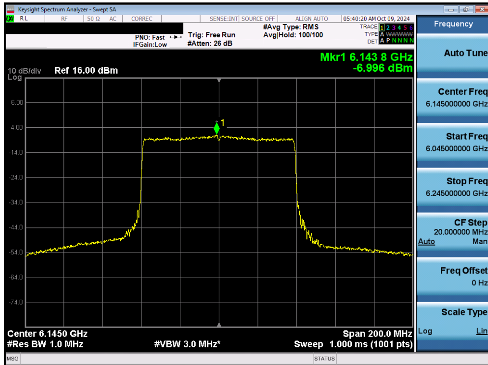
Plot 7-83. Power Spectral Density Plot MIMO ANT1 (80MHz 802.11ax/be (Full Tones) (UNII Band 5) – Ch. 39) - LPI
