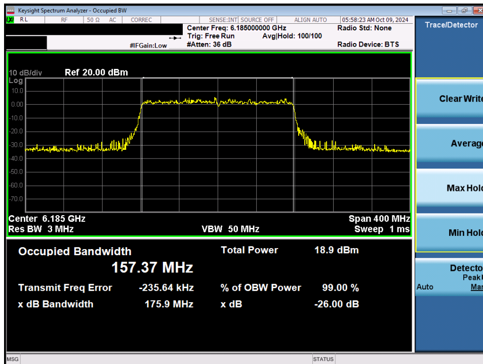
Plot 7-29. 26dB Bandwidth Plot MIMO ANT1 (160MHz 802.11ax/be (Full Tones) (UNII Band 5) – Ch. 47) - LPI
