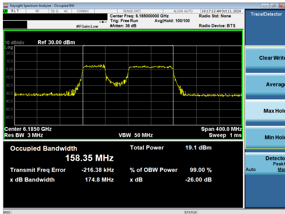
Plot 7-43. 26dB Bandwidth Plot MIMO ANT2 (160MHz 802.11be (996+484 Tones) (UNII Band 5) – Ch. 47) LPI
