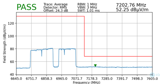
Plot 7-172. Radiated Upper Band Edge Plot MIMO (Average – UNII Band 8)
