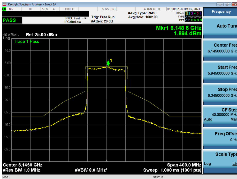
Plot 7-110. In Band Emissions Plot MIMO ANT2 (80MHz 802.11ax/be (UNII Band 5) – Ch. 39) - SP
