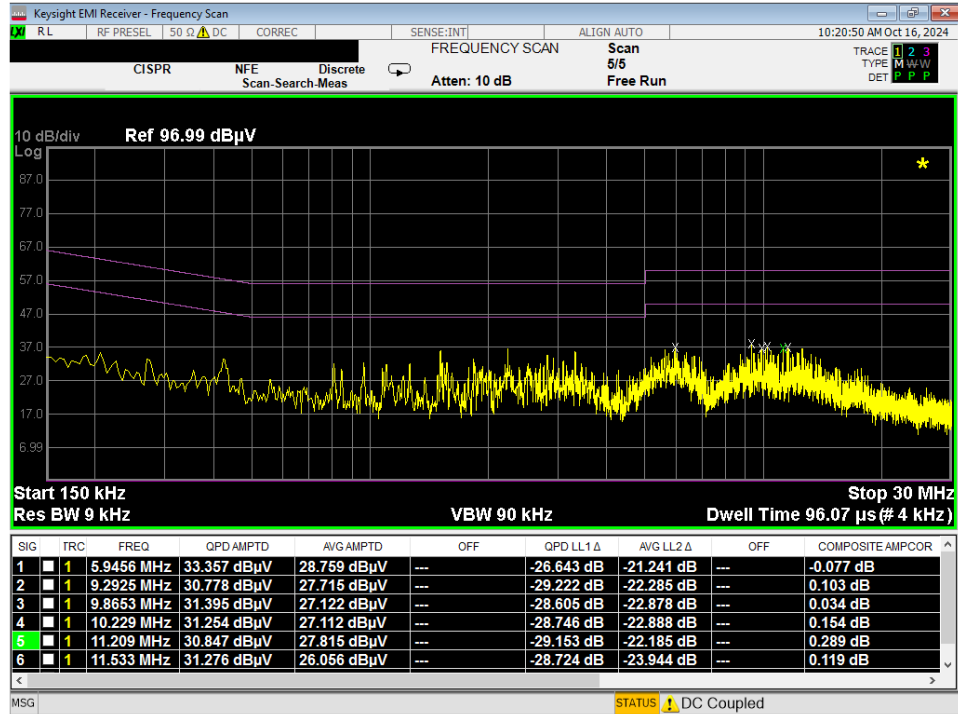
Plot 7-176. Line Conducted Plot with 802.11a UNII Band 6 (L1)
