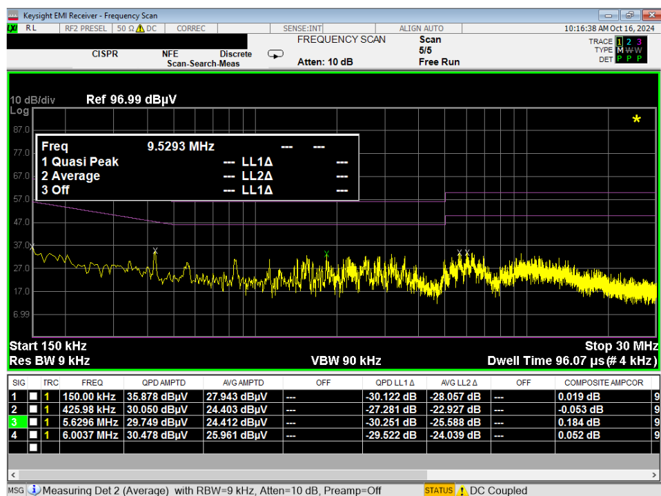
Plot 7-175. Line Conducted Plot with 802.11a UNII Band 5 (N)
