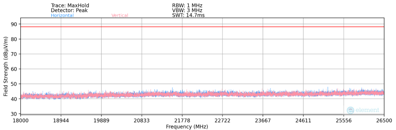
Plot 7-140. Radiated Spurious Plot 18GHz - 26.5GHz (802.11a)
