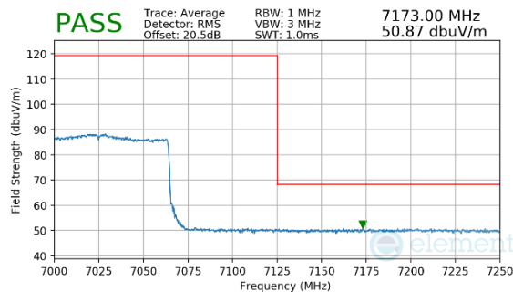
Plot 7-152. Radiated Upper Band Edge Plot MIMO (Average – UNII Band 8)
