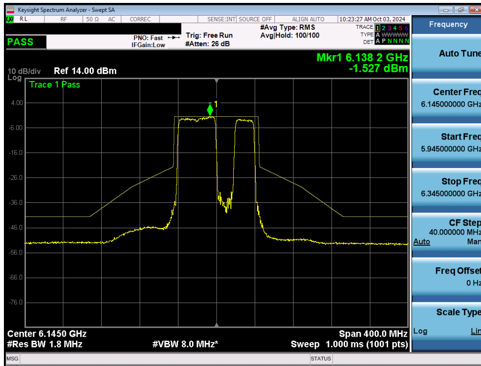
Plot 7-104. In Band Emissions Plot MIMO ANT2 (80MHz 802.11ax/be (UNII Band 5) – Ch. 39) – 20MHz Punctured - LPI
