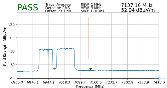
Plot 7-164. Radiated Upper Band Edge Plot MIMO (Average – UNII Band 8)
