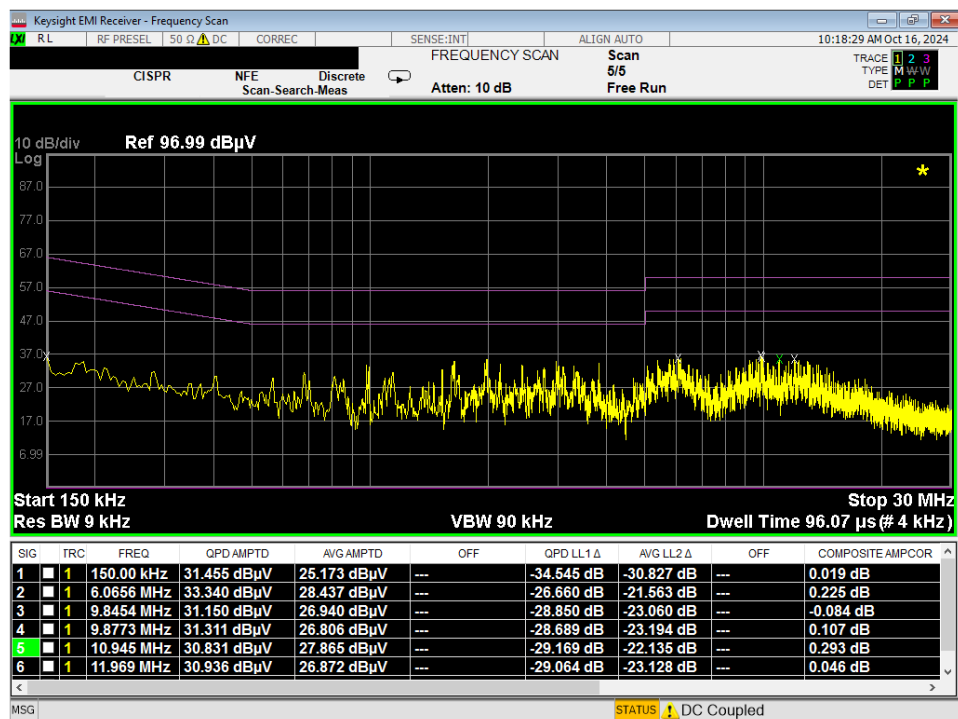
Plot 7-174. Line Conducted Plot with 802.11a UNII Band 5 (L1)
