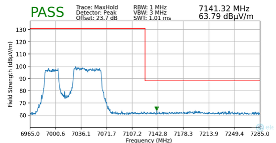
Plot 7-157. Radiated Upper Band Edge Plot MIMO (Peak – UNII Band 8)
