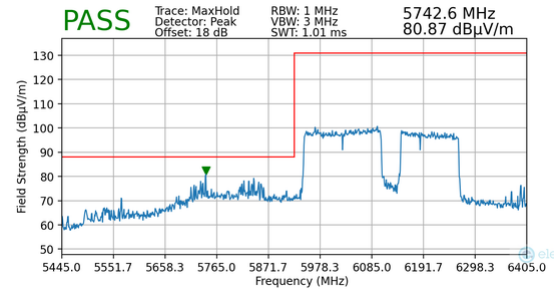
Plot 7-171. Radiated Lower Band Edge Plot MIMO (Peak – UNII Band 5)
