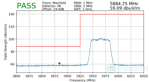
Plot 7-147. Radiated Lower Band Edge Plot MIMO (Peak – UNII Band 5)
