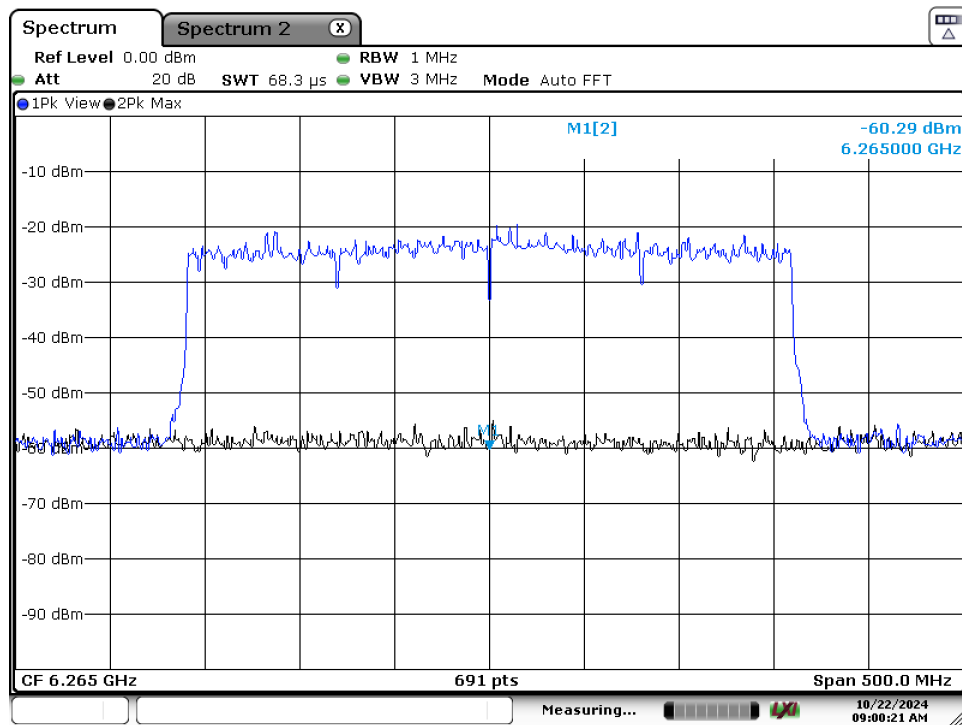
Plot 7-134. CBP 320MHz Channel - Injection Center – [6265 MHz]
