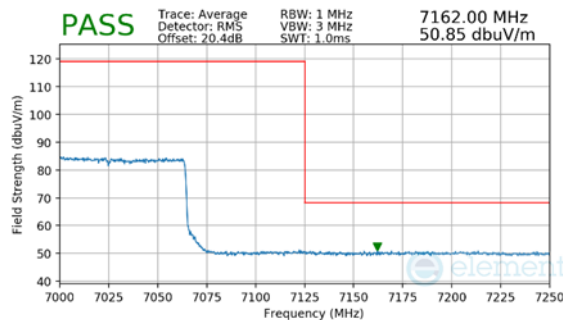
Plot 7-160. Radiated Upper Band Edge Plot MIMO (Average – UNII Band 8)
