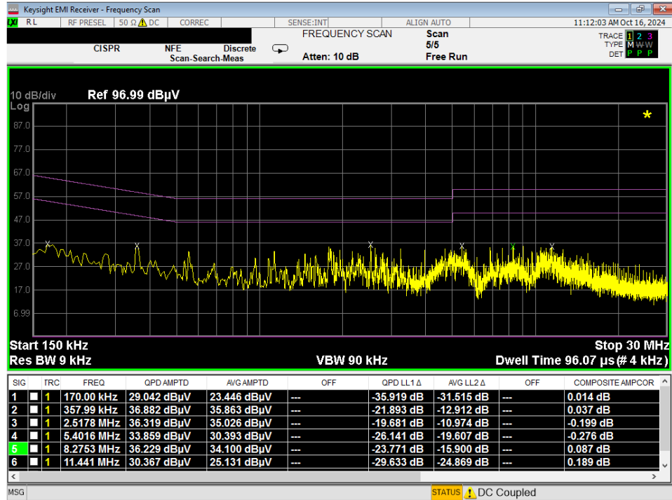
Plot 7-182. Line Conducted Plot with 802.11a UNII Band 5 (L1) with WCP
