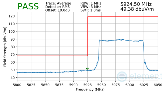
Plot 7-150. Radiated Lower Band Edge Plot MIMO (Average – UNII Band 5)
