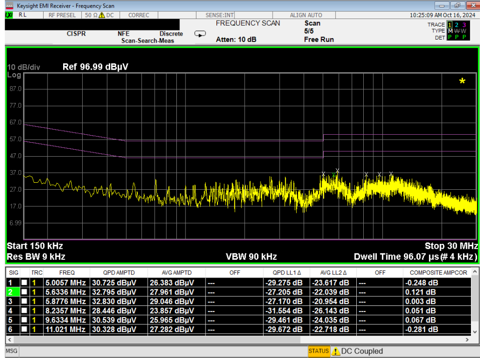
Plot 7-178. Line Conducted Plot with 802.11a UNII Band 7 (L1)
