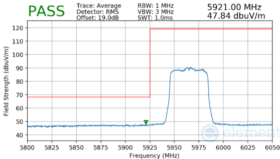
Plot 7-146. Radiated Lower Band Edge Plot MIMO (Average – UNII Band 5)
