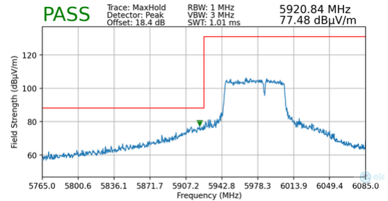
Plot 7-155. Radiated Lower Band Edge Plot MIMO (Peak – UNII Band 5)
