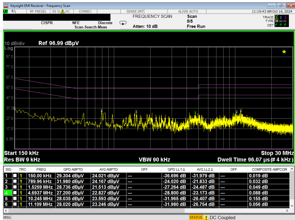
Plot 7-189. Line Conducted Plot with 802.11a UNII Band 8 (N) with WCP
