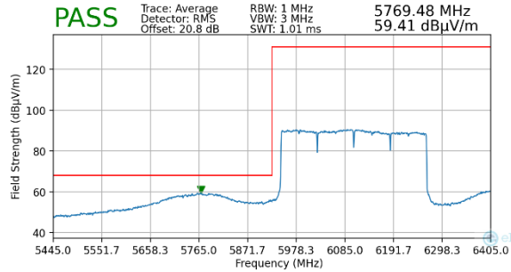
Plot 7-166. Radiated Lower Band Edge Plot MIMO (Average – UNII Band 5)
