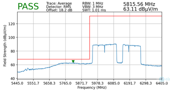
Plot 7-170. Radiated Lower Band Edge Plot MIMO (Average – UNII Band 5)
