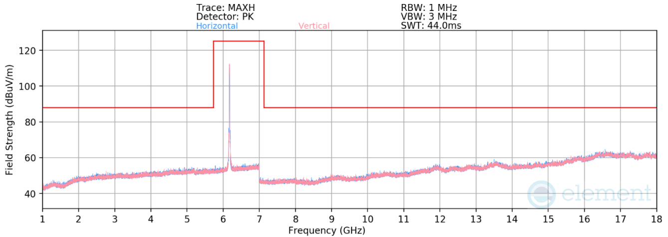
Plot 7-136. Radiated Spurious Plot 1GHz – 18GHz MIMO (802.11a – UNII Band 5 Ch. 45)
