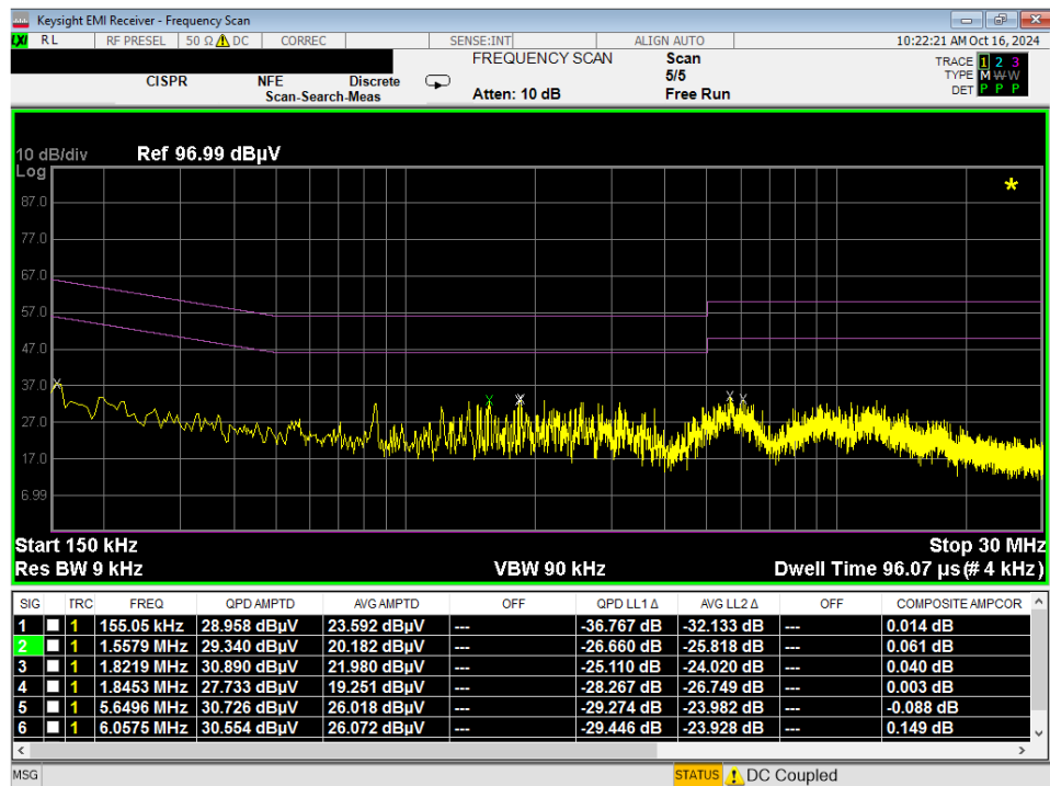
Plot 7-177. Line Conducted Plot with 802.11a UNII Band 6 (N)
