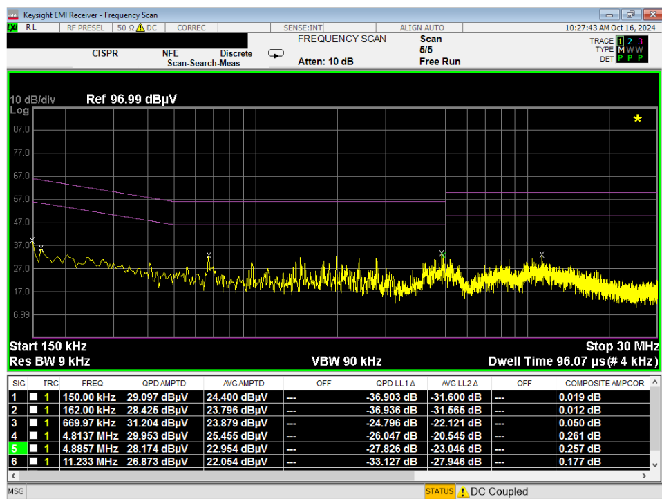
Plot 7-181. Line Conducted Plot with 802.11a UNII Band 8 (N)
