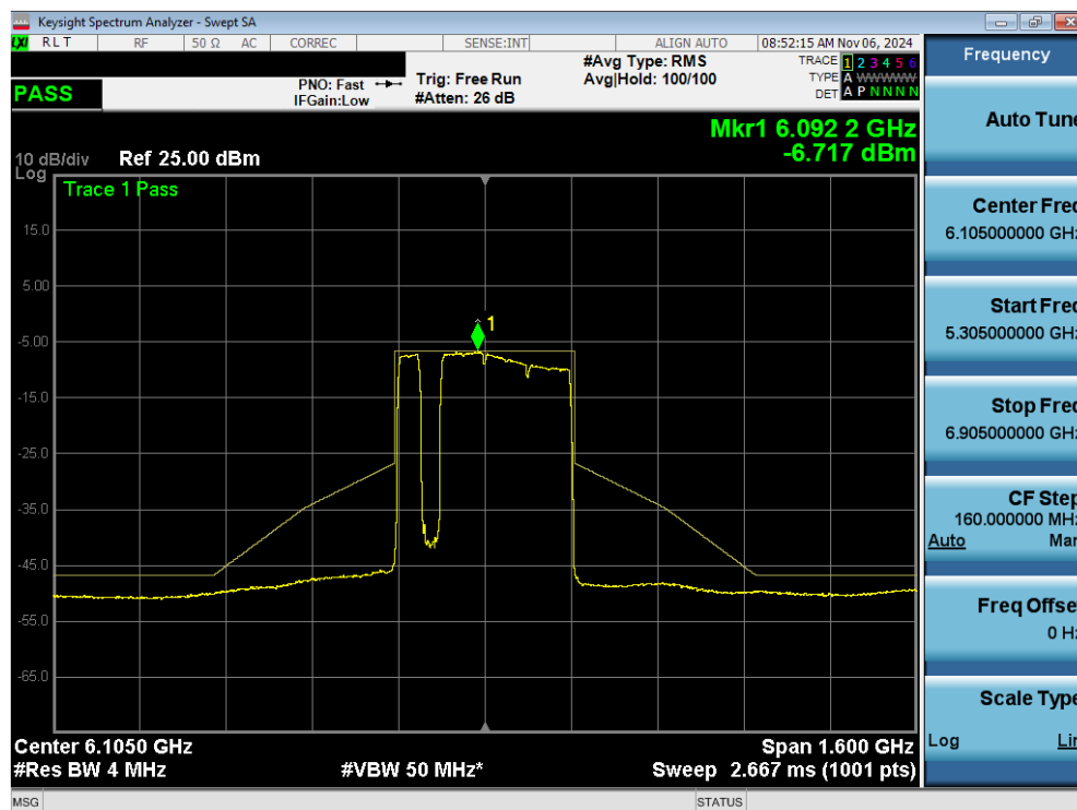
Plot 7-106. In Band Emissions Plot MIMO ANT2 (320MHz 802.11ax/be (UNII Band 5) – Ch. 31) – 40MHz Punctured – LPI
