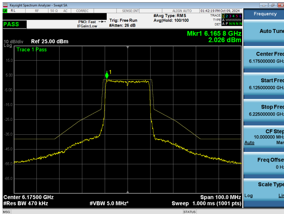
Plot 7-108. In Band Emissions Plot MIMO ANT2 (20MHz 802.11ax/be (UNII Band 5) – Ch. 45) - SP
