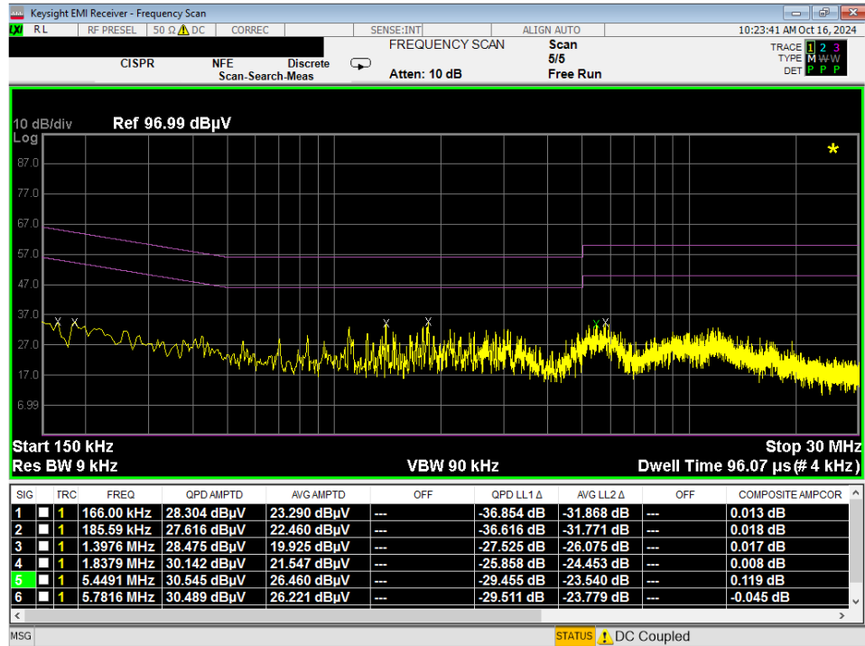
Plot 7-179. Line Conducted Plot with 802.11a UNII Band 7 (N)
