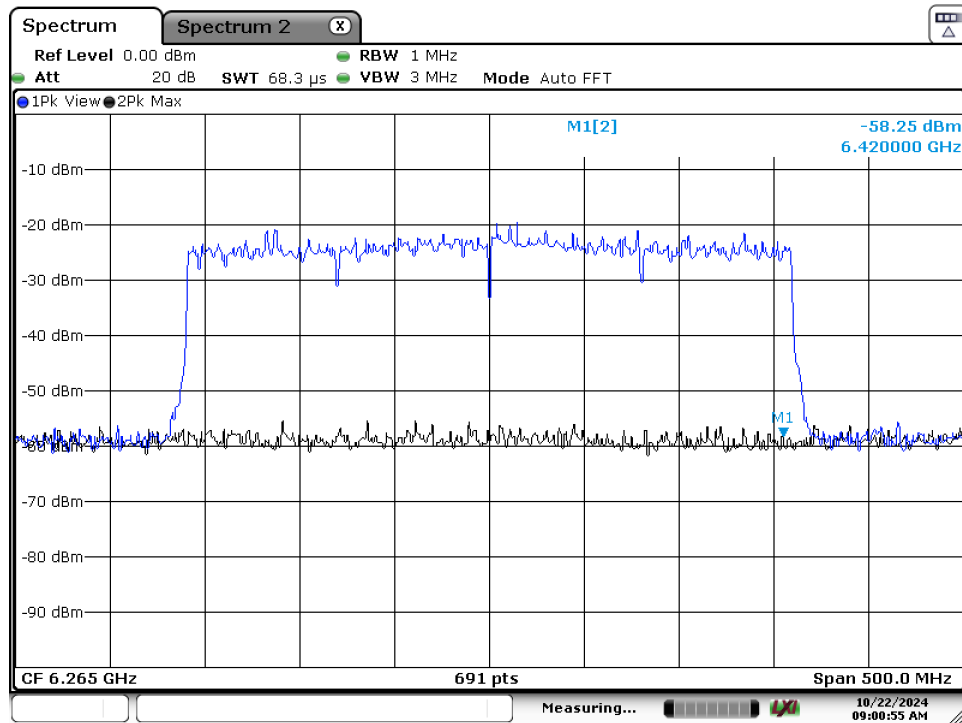
Plot 7-135. CBP 320MHz Channel - Injection Upper Edge – [6420 MHz]
