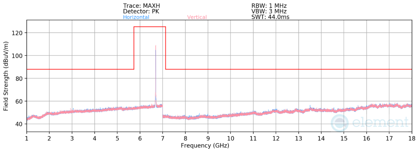
Plot 7-138. Radiated Spurious Plot 1GHz – 18GHz MIMO (802.11a – UNII Band 7 Ch. 149)
