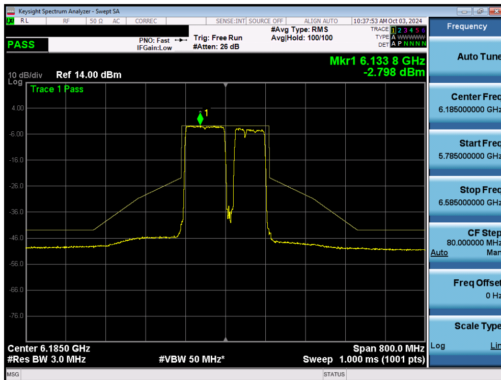
Plot 7-105. In Band Emissions Plot MIMO ANT2 (160MHz 802.11ax/be (UNII Band 5) – Ch. 47) – 20MHz Punctured - LPI
