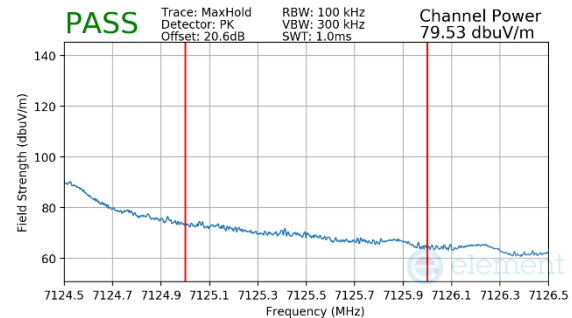
Plot 7-145. Radiated Upper Band Edge Plot MIMO (Peak – UNII Band 8)
