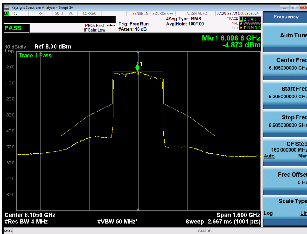
Plot 7-103. In Band Emissions Plot MIMO ANT2 (320MHz 802.11ax/be (UNII Band 5) – Ch. 31) - LPI
