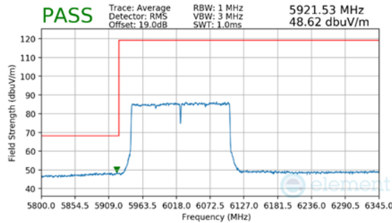
Plot 7-158. Radiated Lower Band Edge Plot MIMO (Average – UNII Band 5)
