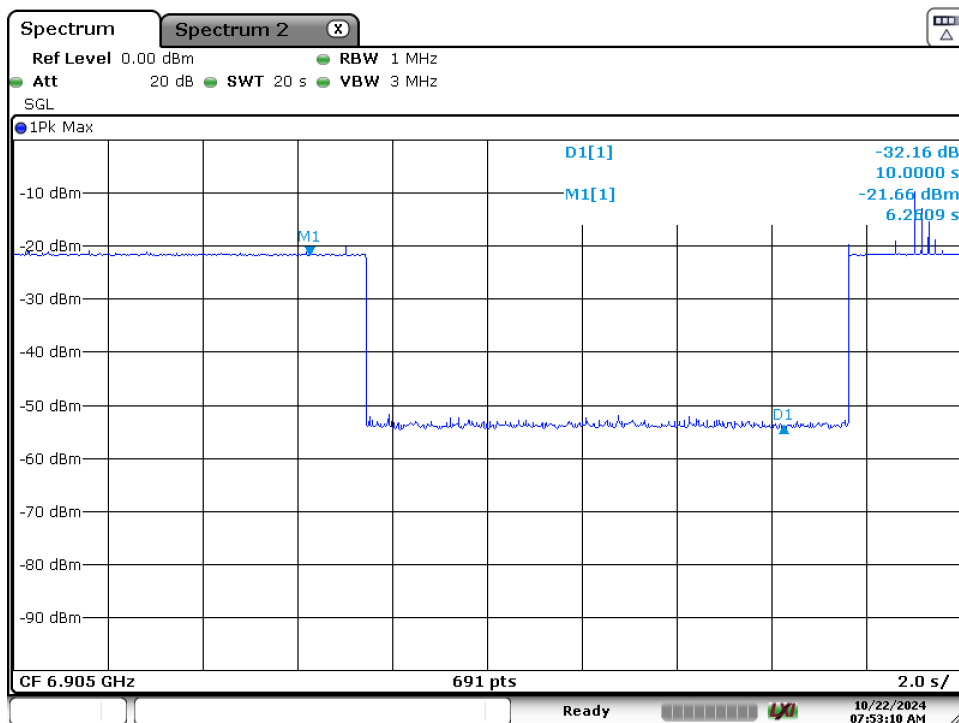
Plot 7-131. Contention Based Protocol Timing Plot (320MHz (UNII Band 8) – Ch. 191 Mid)
