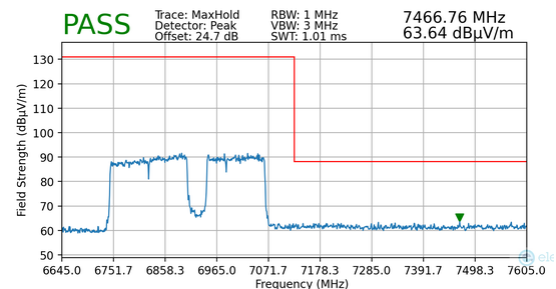
Plot 7-173. Radiated Upper Band Edge Plot MIMO (Peak – UNII Band 8)
