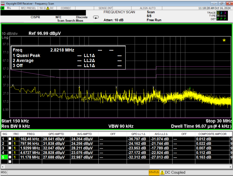
Plot 7-187. Line Conducted Plot with 802.11a UNII Band 7 (N) with WCP
