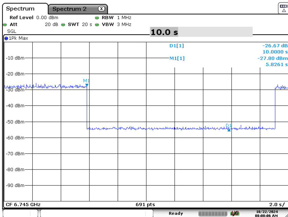
Plot 7-127. Contention Based Protocol Timing Plot (320MHz (UNII Band 7) – Ch. 159 Mid)
