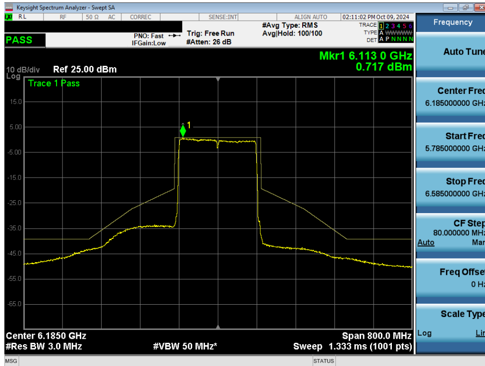
Plot 7-111. In Band Emissions Plot MIMO ANT2 (160MHz 802.11ax/be (UNII Band 5) – Ch. 47) - SP
