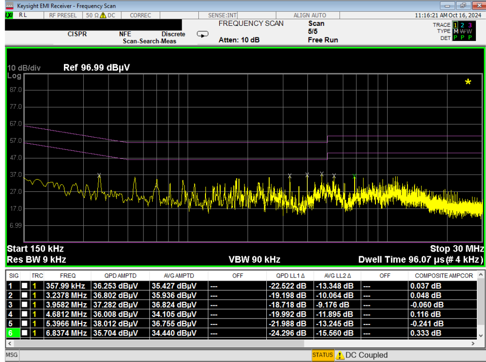
Plot 7-184. Line Conducted Plot with 802.11a UNII Band 6 (L1) with WCP
