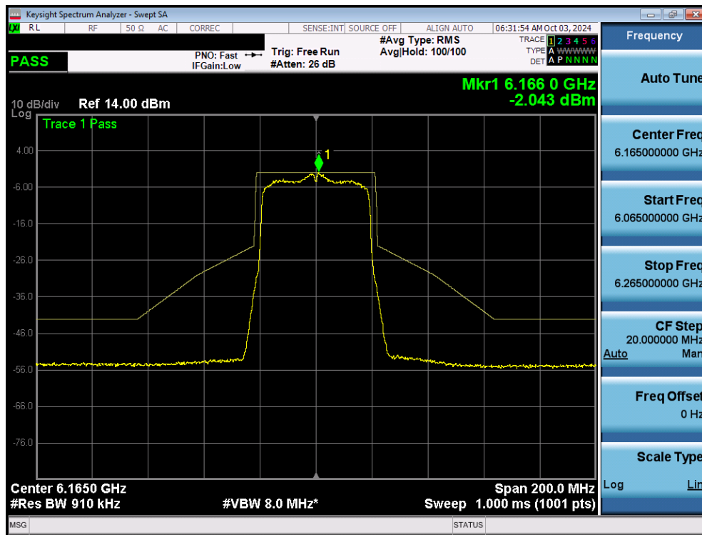
Plot 7-100. In Band Emissions Plot MIMO ANT2 (40MHz 802.11ax/be (UNII Band 5) – Ch. 43) - LPI
