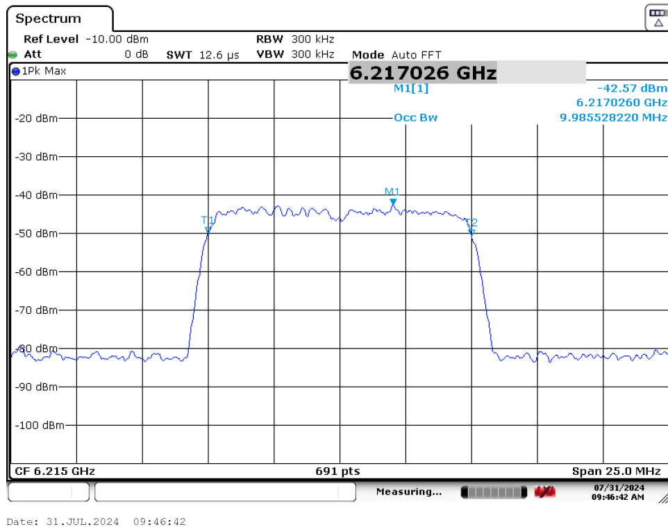
Plot 7-116. AWGN Signal (Demonstration)
