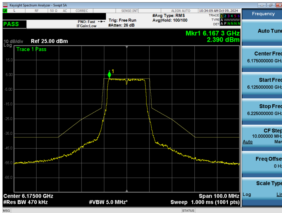
Plot 7-107. In Band Emissions Plot MIMO ANT2 (20MHz 802.11a (UNII Band 5) – Ch. 45) - SP
