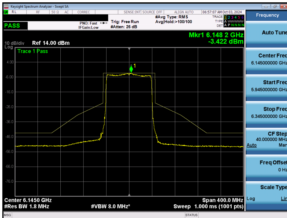
Plot 7-101. In Band Emissions Plot MIMO ANT2 (80MHz 802.11ax/be (UNII Band 5) – Ch. 39) - LPI
