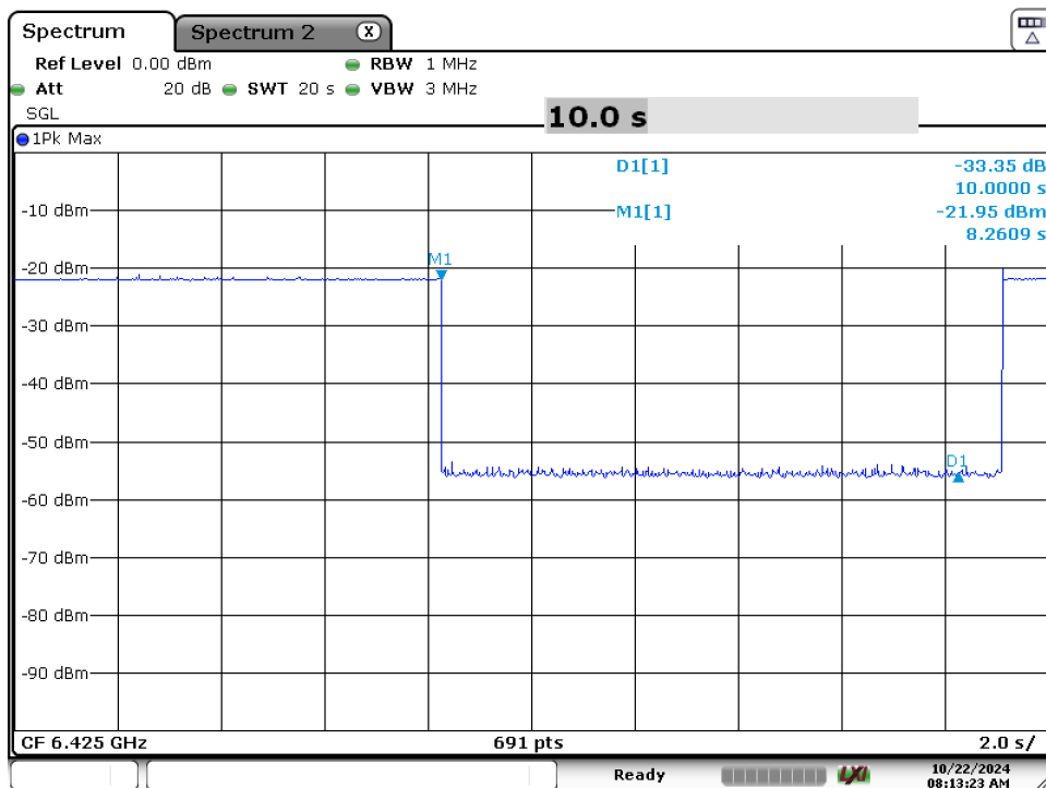
Plot 7-123. Contention Based Protocol Timing Plot (320MHz (UNII Band 6) – Ch. 95 Mid)
