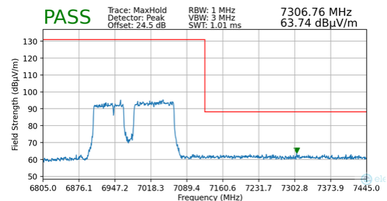
Plot 7-165. Radiated Upper Band Edge Plot MIMO (Peak – UNII Band 8)
