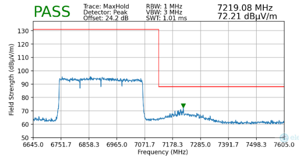
Plot 7-169. Radiated Upper Band Edge Plot MIMO (Peak – UNII Band 8)
