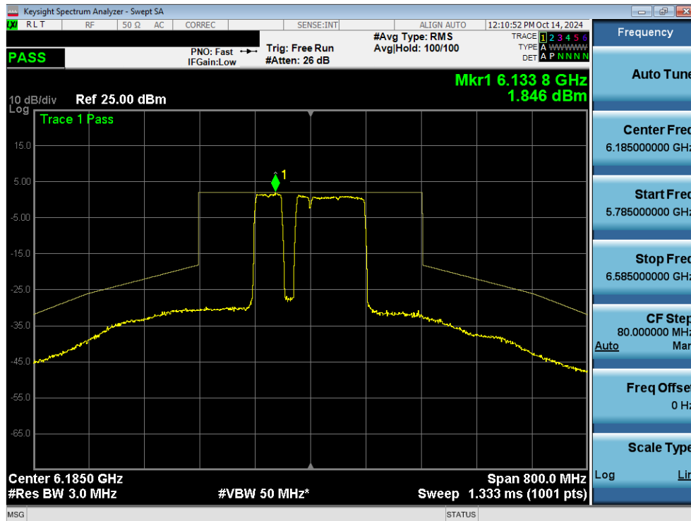
Plot 7-114. In Band Emissions Plot MIMO ANT2 (160MHz 802.11ax/be (UNII Band 5) – Ch. 47) – 20MHz Punctured - SP
