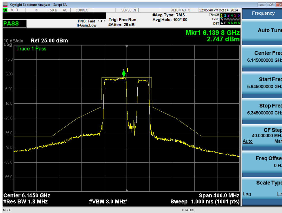
Plot 7-113. In Band Emissions Plot MIMO ANT2 (80MHz 802.11ax/be (UNII Band 5) – Ch. 39) – 20MHz Punctured - SP
