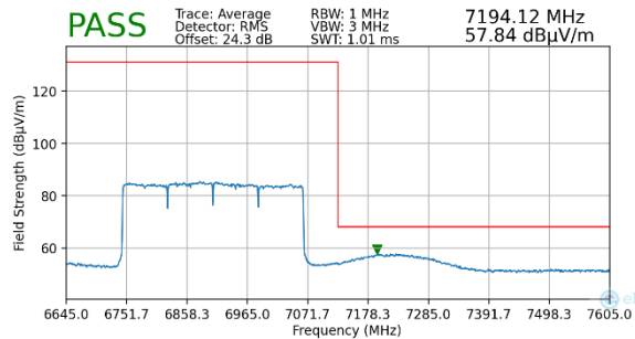
Plot 7-168. Radiated Upper Band Edge Plot MIMO (Average – UNII Band 8)
