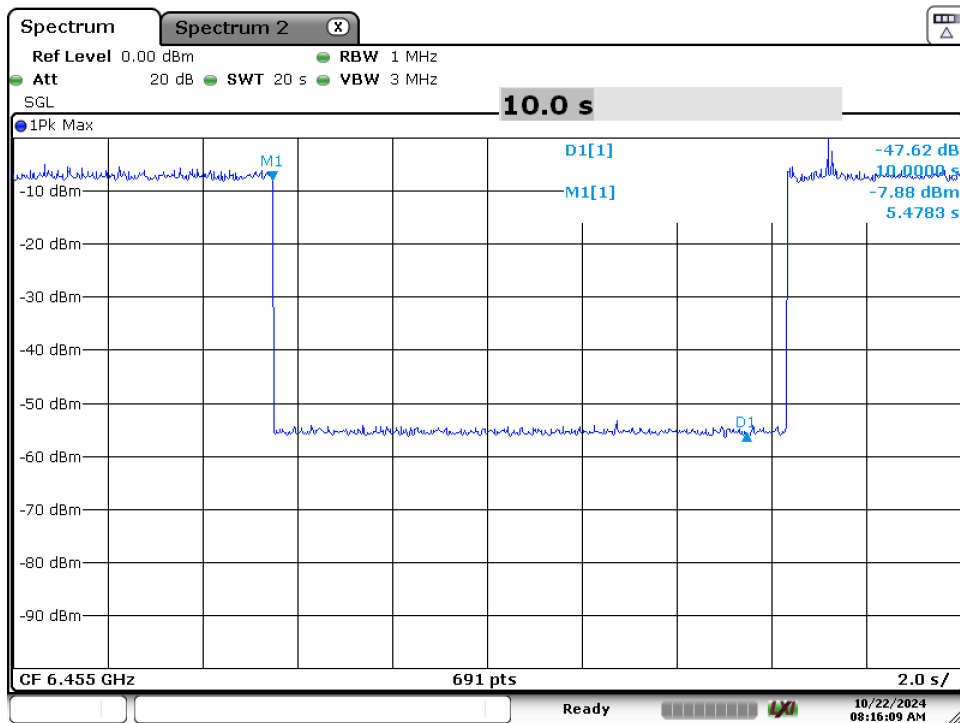
Plot 7-121. Contention Based Protocol Timing Plot (20MHz (UNII Band 6) – Ch. 101)
