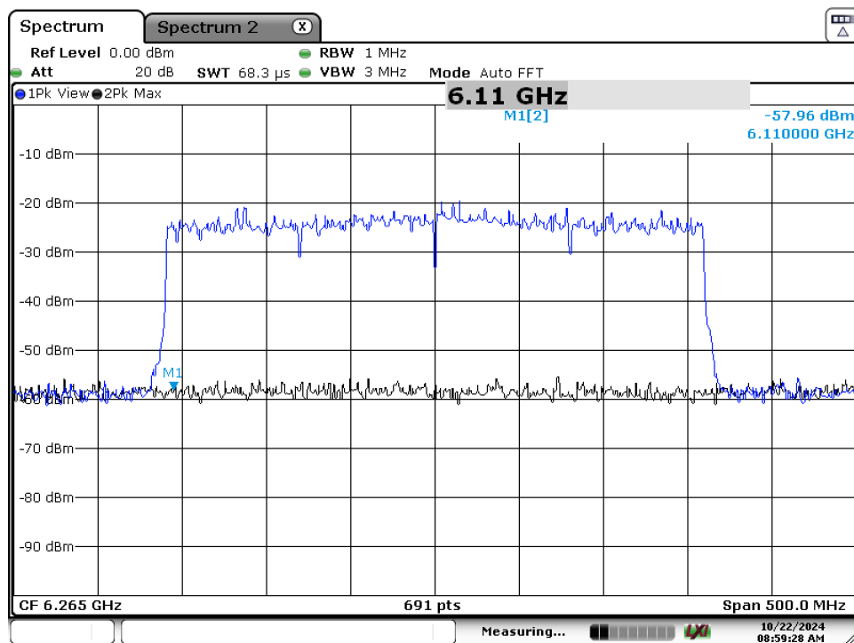
Plot 7-133. CBP 320MHz Channel - Injection Lower Edge – [6110 MHz]
