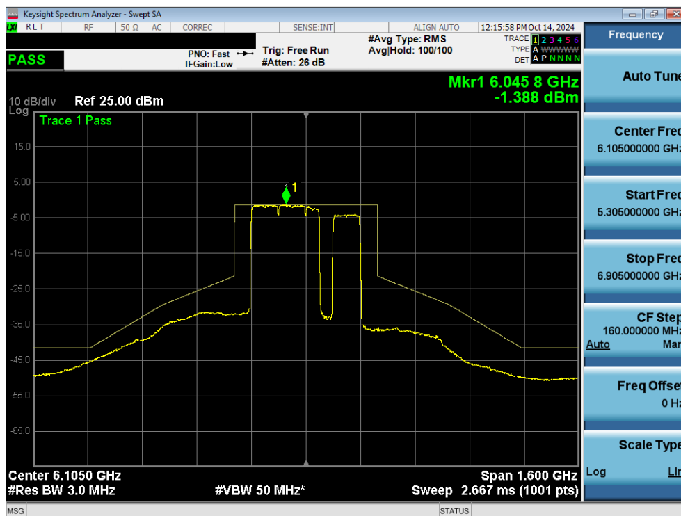
Plot 7-115. In Band Emissions Plot MIMO ANT2 (320MHz 802.11ax/be (UNII Band 5) – Ch. 31) – 40MHz Punctured - SP
