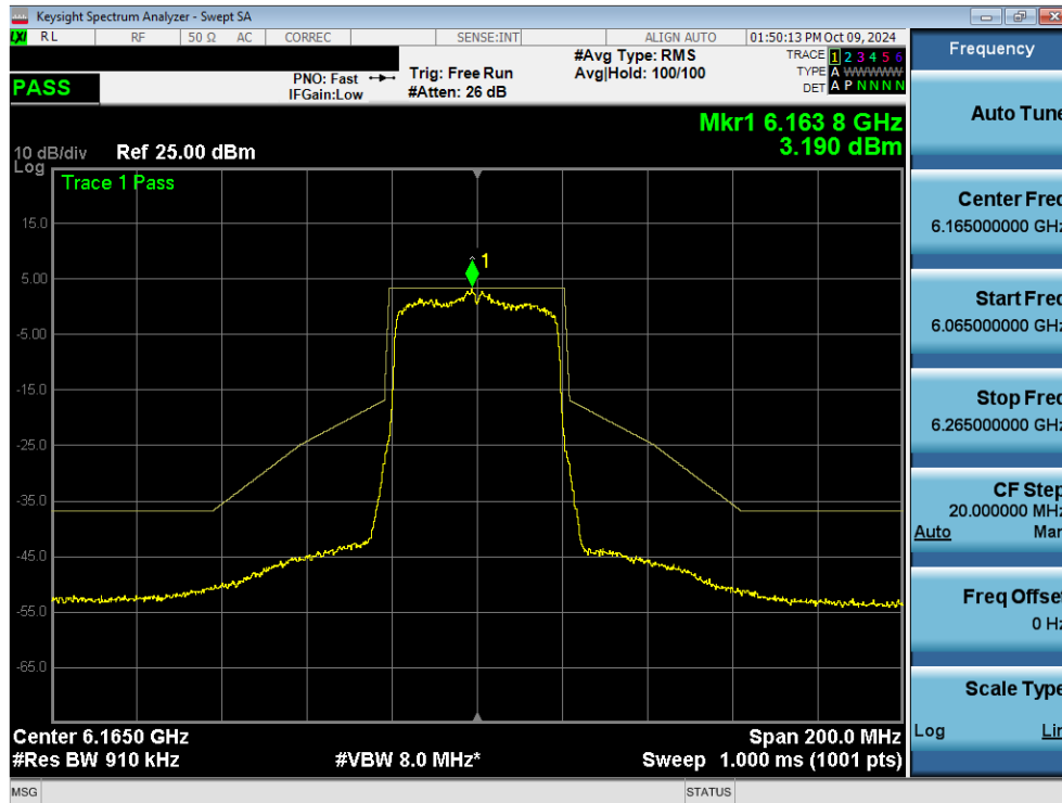
Plot 7-109. In Band Emissions Plot MIMO ANT2 (40MHz 802.11ax/be (UNII Band 5) – Ch. 43) - SP
