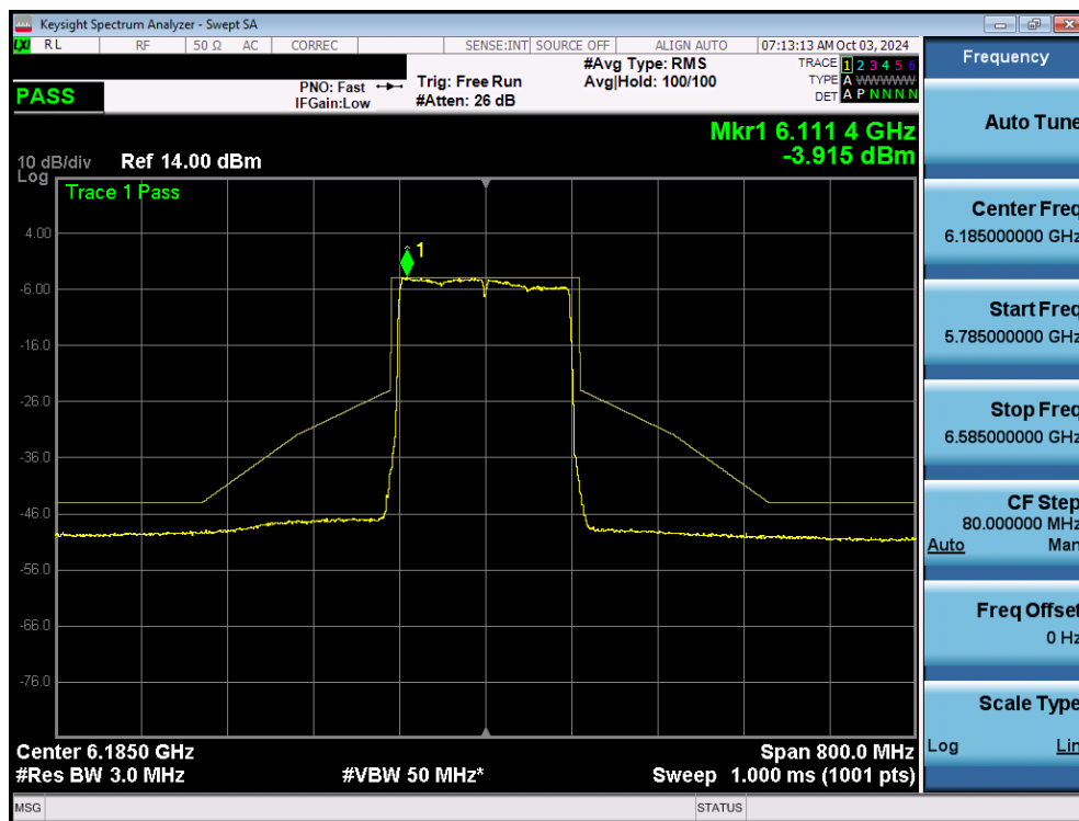
Plot 7-102. In Band Emissions Plot MIMO ANT2 (160MHz 802.11ax/be (UNII Band 5) – Ch. 47) - LPI
