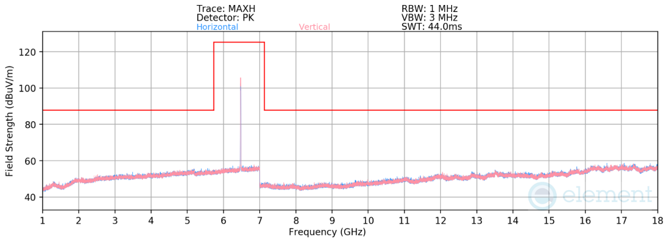
Plot 7-137. Radiated Spurious Plot 1GHz – 18GHz MIMO (802.11a – UNII Band 6 Ch. 105)
