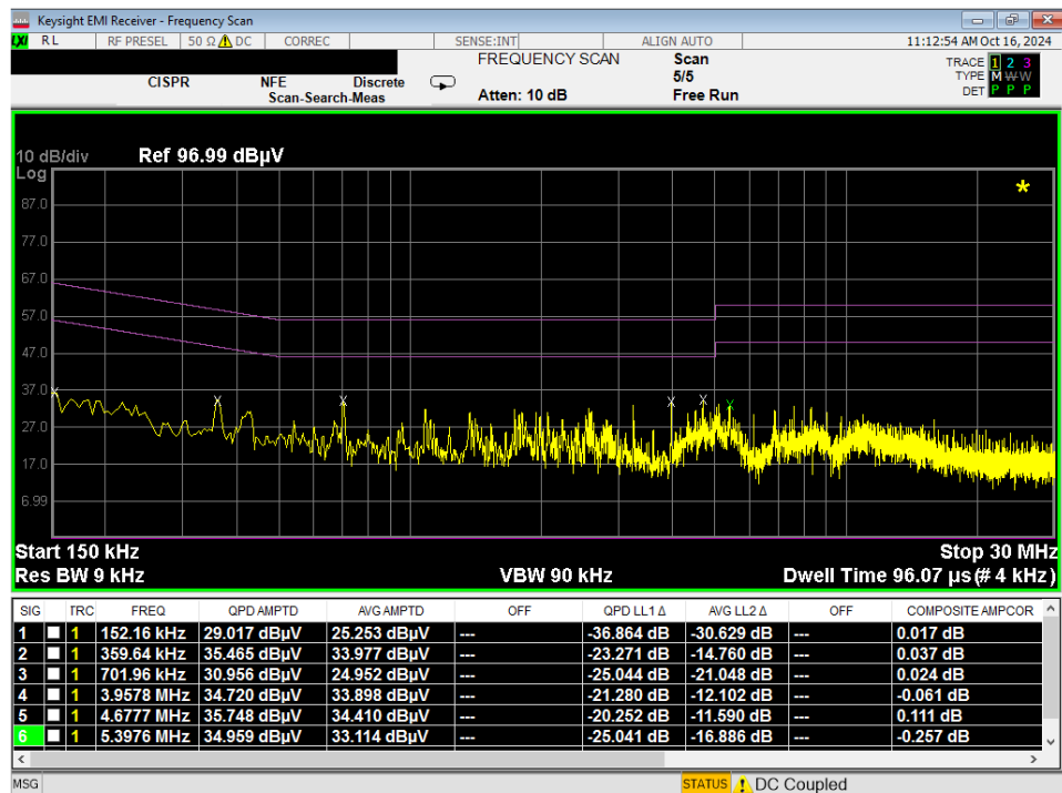
Plot 7-183. Line Conducted Plot with 802.11a UNII Band 5 (N) with WCP
