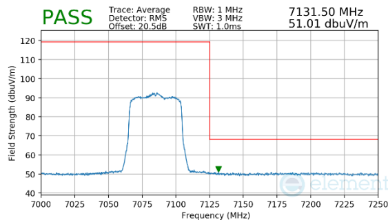
Plot 7-148. Radiated Upper Band Edge Plot MIMO (Average – UNII Band 8)
