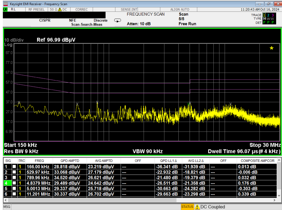
Plot 7-188. Line Conducted Plot with 802.11a UNII Band 8 (L1) with WCP
