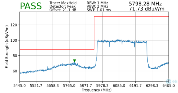
Plot 7-167. Radiated Lower Band Edge Plot MIMO (Peak – UNII Band 5)
