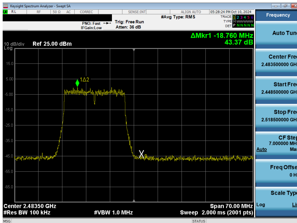
Plot 7-75. Band Edge Plot (802.11n (2.4GHz) – Ch. 13) MIMO ANT1
