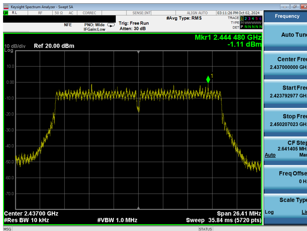
Plot 7-59. Power Spectral Density Plot (802.11ac (2.4GHz) – Ch. 6) MIMO ANT2
