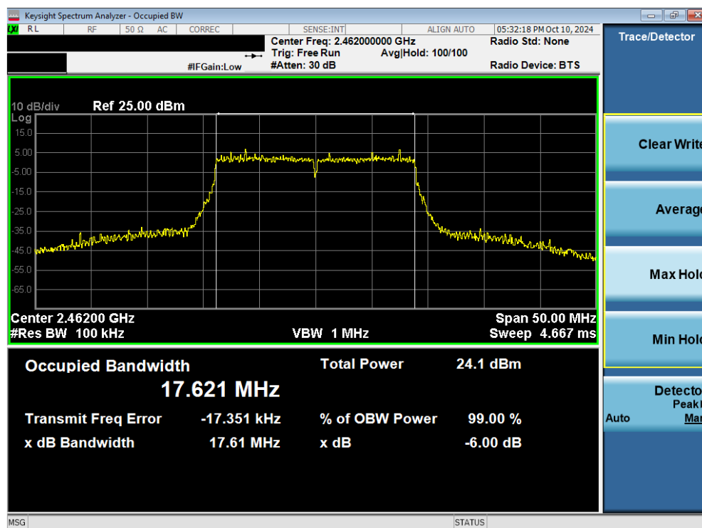
Plot 7-12. 6dB Bandwidth Plot (802.11n (2.4GHz) – Ch. 11) MIMO ANT1
