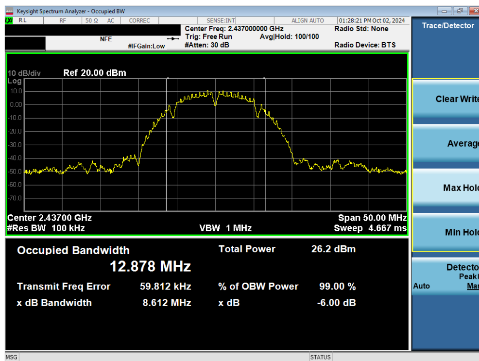
Plot 7-5. 6dB Bandwidth Plot (802.11b – Ch. 6) MIMO ANT1
