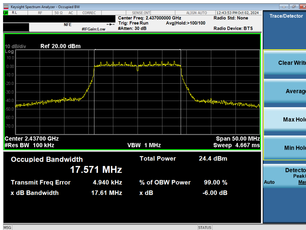
Plot 7-14. 6dB Bandwidth Plot (802.11ac (2.4GHz) – Ch. 6) MIMO ANT1
