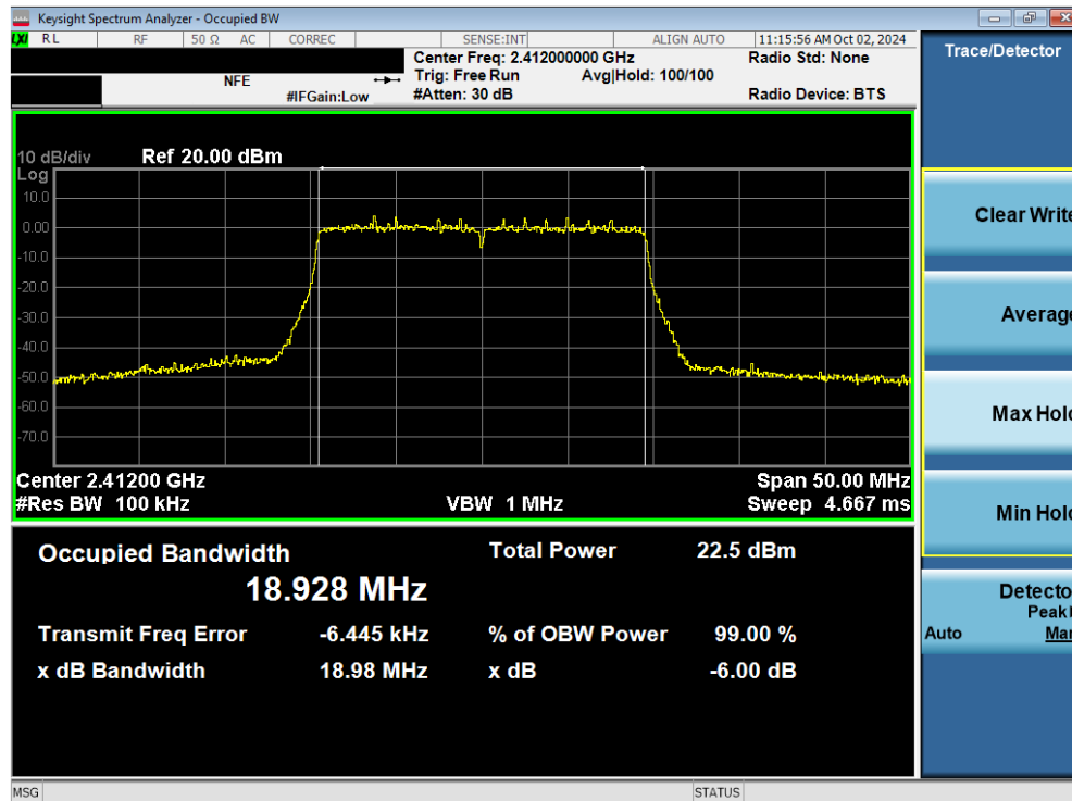
Plot 7-16. 6dB Bandwidth Plot (802.11ax/be (2.4GHz) – Ch. 1) MIMO ANT1
