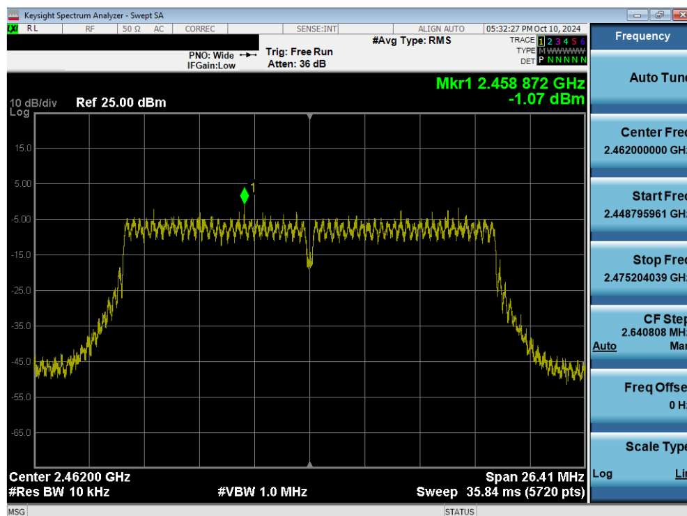
Plot 7-42. Power Spectral Density Plot (802.11n (2.4GHz) – Ch. 11) MIMO ANT1
