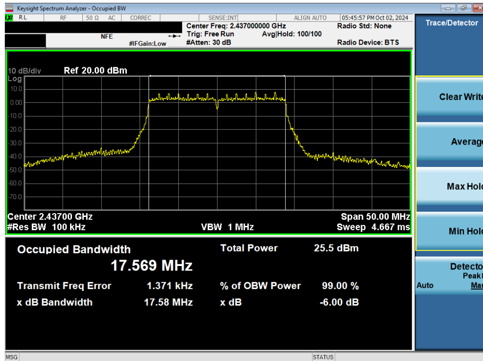
Plot 7-26. 6dB Bandwidth Plot (802.11n (2.4GHz) – Ch. 6) MIMO ANT2
