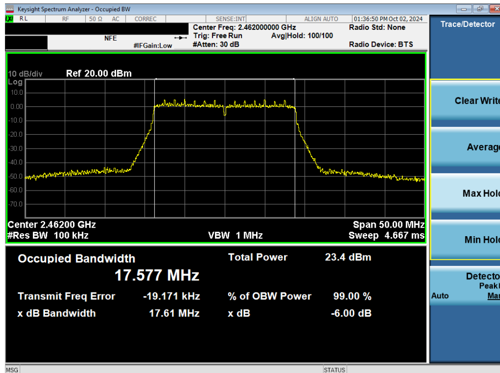
Plot 7-33. 6dB Bandwidth Plot (802.11ax/be (2.4GHz) – Ch. 11) MIMO ANT2
