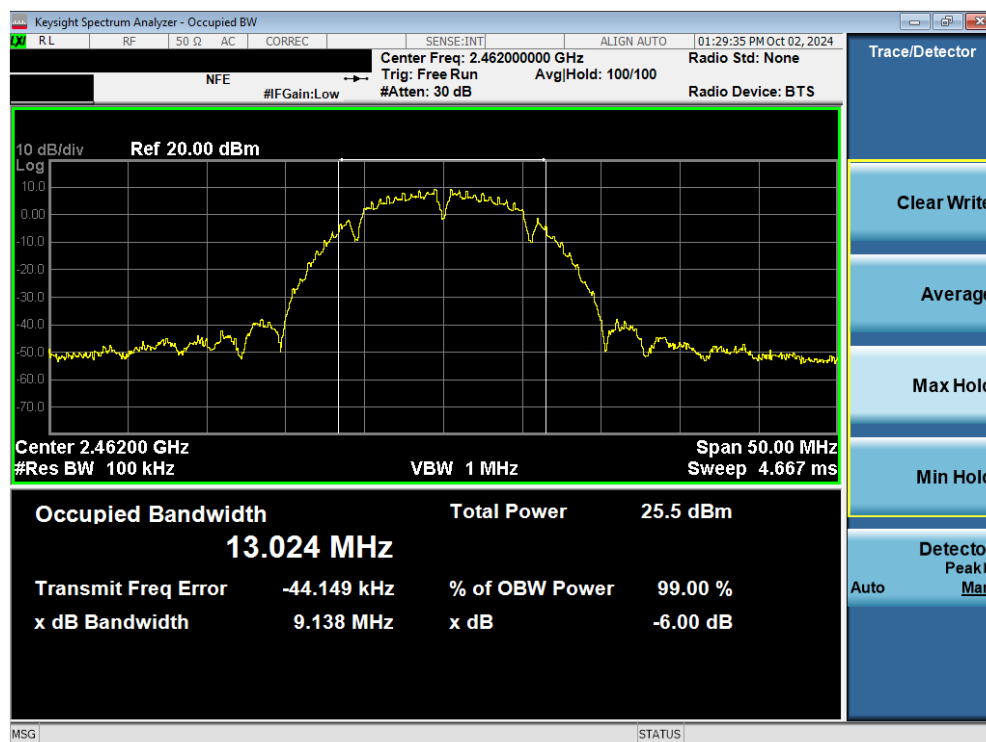
Plot 7-6. 6dB Bandwidth Plot (802.11b – Ch. 11) MIMO ANT1
