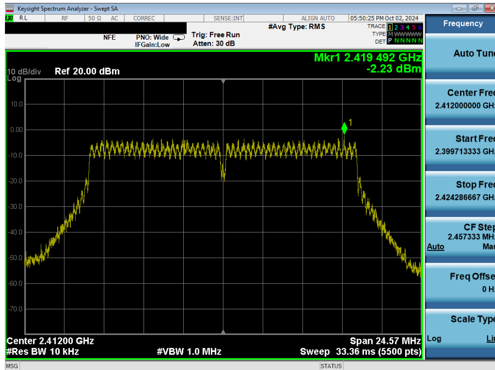
Plot 7-52. Power Spectral Density Plot (802.11g – Ch. 1) MIMO ANT2
