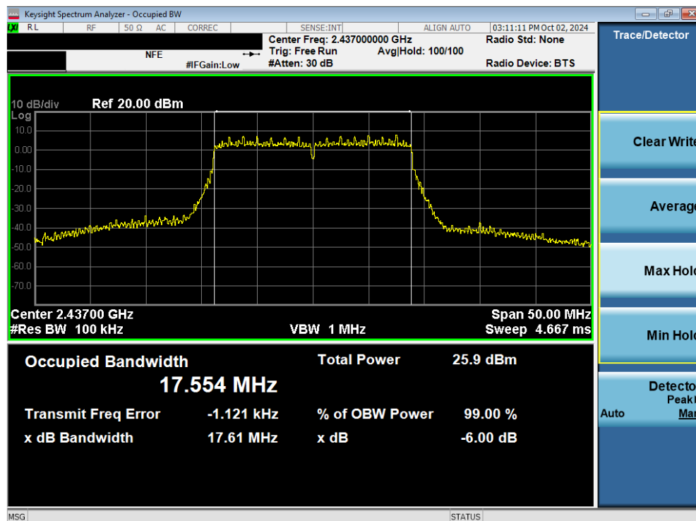
Plot 7-29. 6dB Bandwidth Plot (802.11ac (2.4GHz) – Ch. 6) MIMO ANT2
