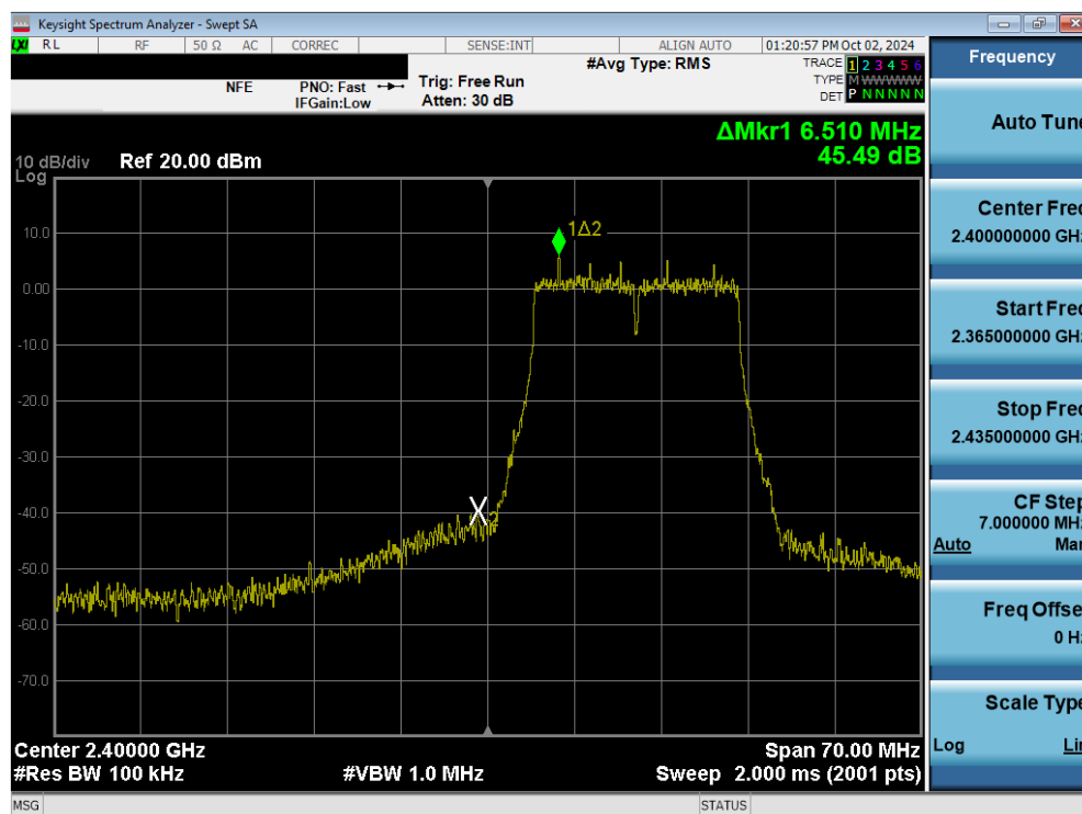
Plot 7-68. Band Edge Plot (802.11g– Ch. 1) MIMO ANT1
