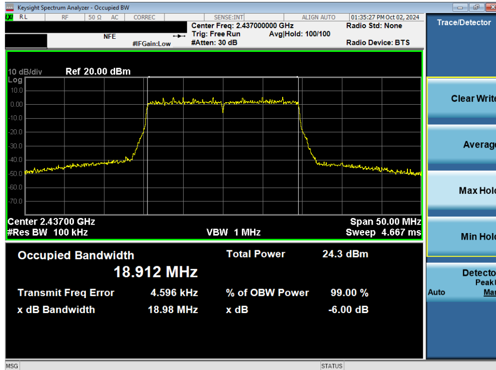
Plot 7-32. 6dB Bandwidth Plot (802.11ax/be (2.4GHz) – Ch. 6) MIMO ANT2
