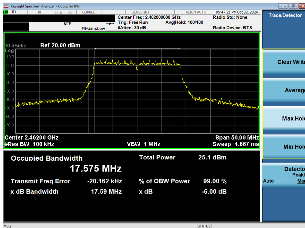
Plot 7-27. 6dB Bandwidth Plot (802.11n (2.4GHz) – Ch. 11) MIMO ANT2
