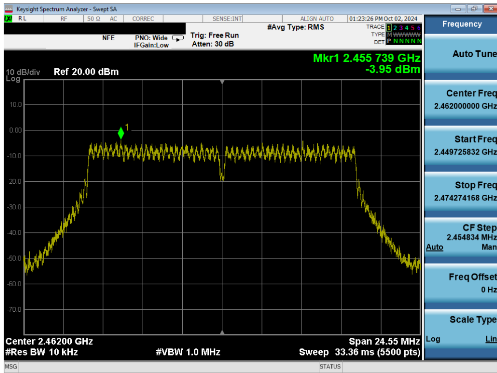
Plot 7-39. Power Spectral Density Plot (802.11g – Ch. 11) MIMO ANT1
