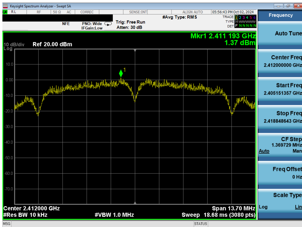
Plot 7-49. Power Spectral Density Plot (802.11b – Ch. 1) MIMO ANT2
