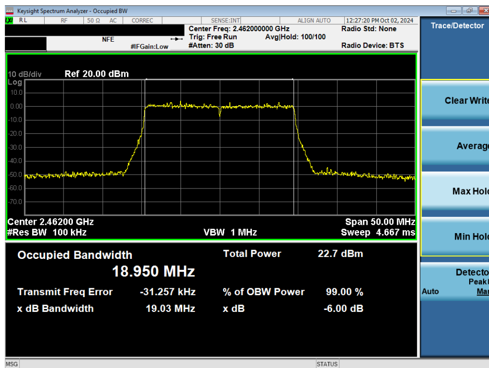
Plot 7-18. 6dB Bandwidth Plot (802.11ax/be (2.4GHz) – Ch. 11) MIMO ANT1
