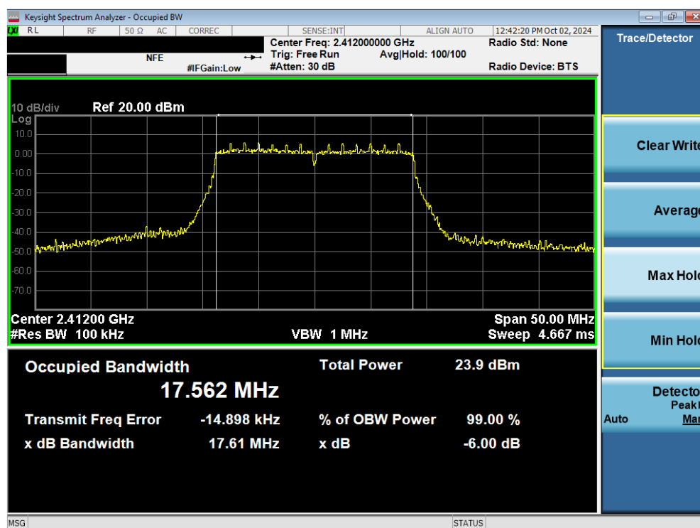
Plot 7-13. 6dB Bandwidth Plot (802.11ac (2.4GHz) – Ch. 1) MIMO ANT1
