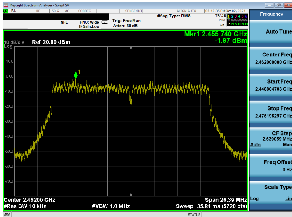
Plot 7-57. Power Spectral Density Plot (802.11n (2.4GHz) – Ch. 11) MIMO ANT2
