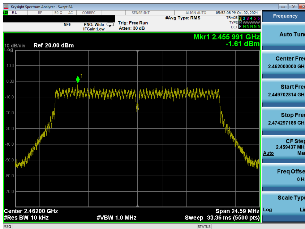
Plot 7-54. Power Spectral Density Plot (802.11g – Ch. 11) MIMO ANT2
