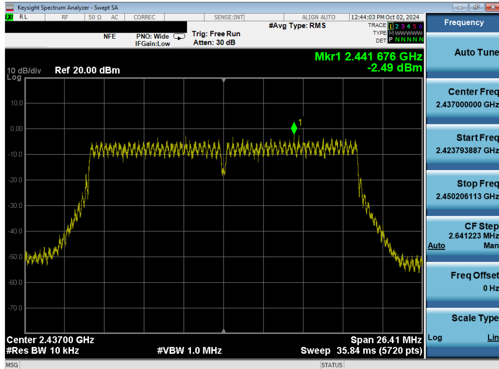
Plot 7-44. Power Spectral Density Plot (802.11ac (2.4GHz) – Ch. 6) MIMO ANT1
