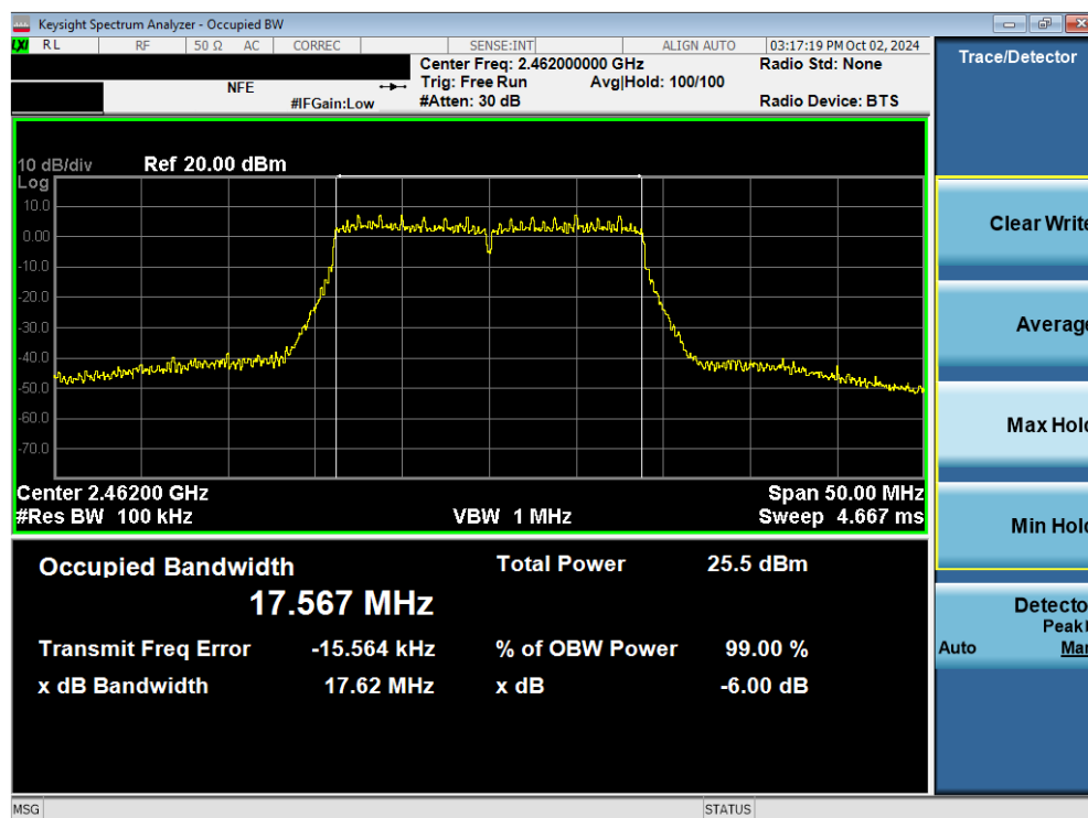
Plot 7-30. 6dB Bandwidth Plot (802.11ac (2.4GHz) – Ch. 11) MIMO ANT2
