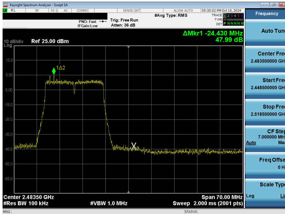
Plot 7-74. Band Edge Plot (802.11n (2.4GHz) – Ch. 12) MIMO ANT1
