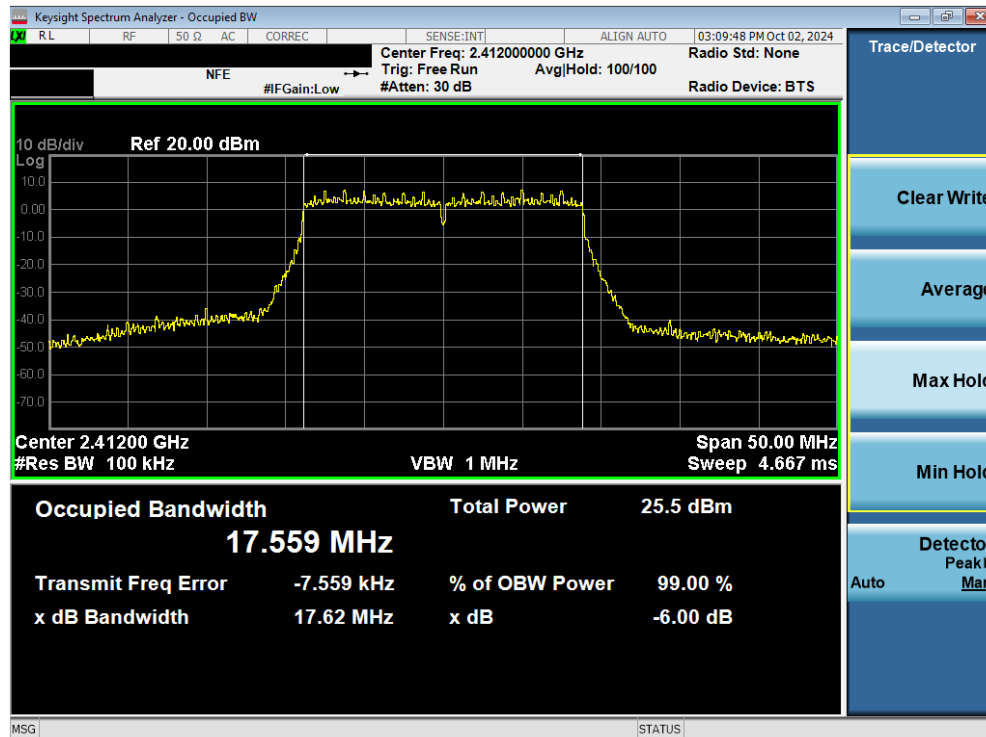
Plot 7-28. 6dB Bandwidth Plot (802.11ac (2.4GHz) – Ch. 1) MIMO ANT2
