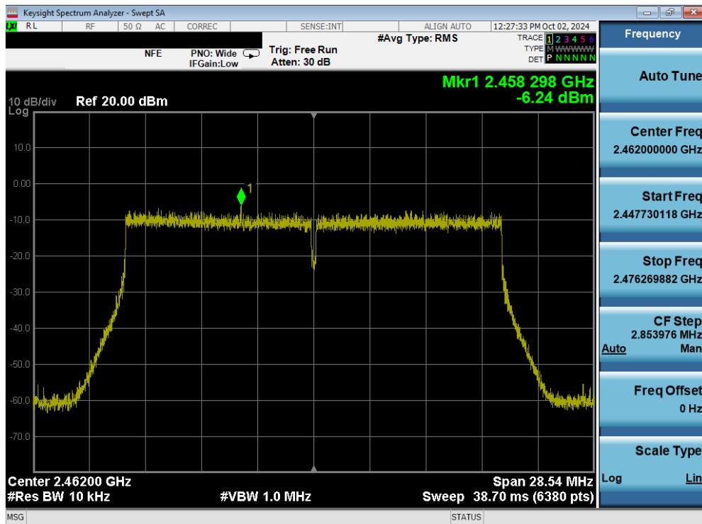
Plot 7-48. Power Spectral Density Plot (802.11ax/be (2.4GHz) – Ch. 11) MIMO ANT1
