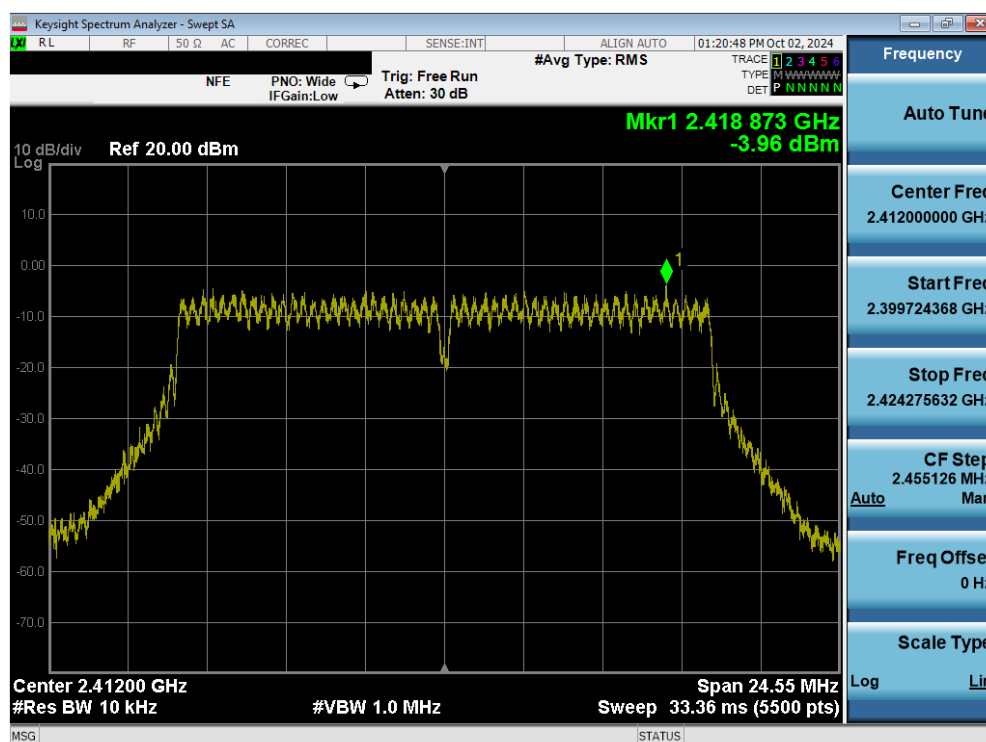
Plot 7-37. Power Spectral Density Plot (802.11g – Ch. 1) MIMO ANT1
