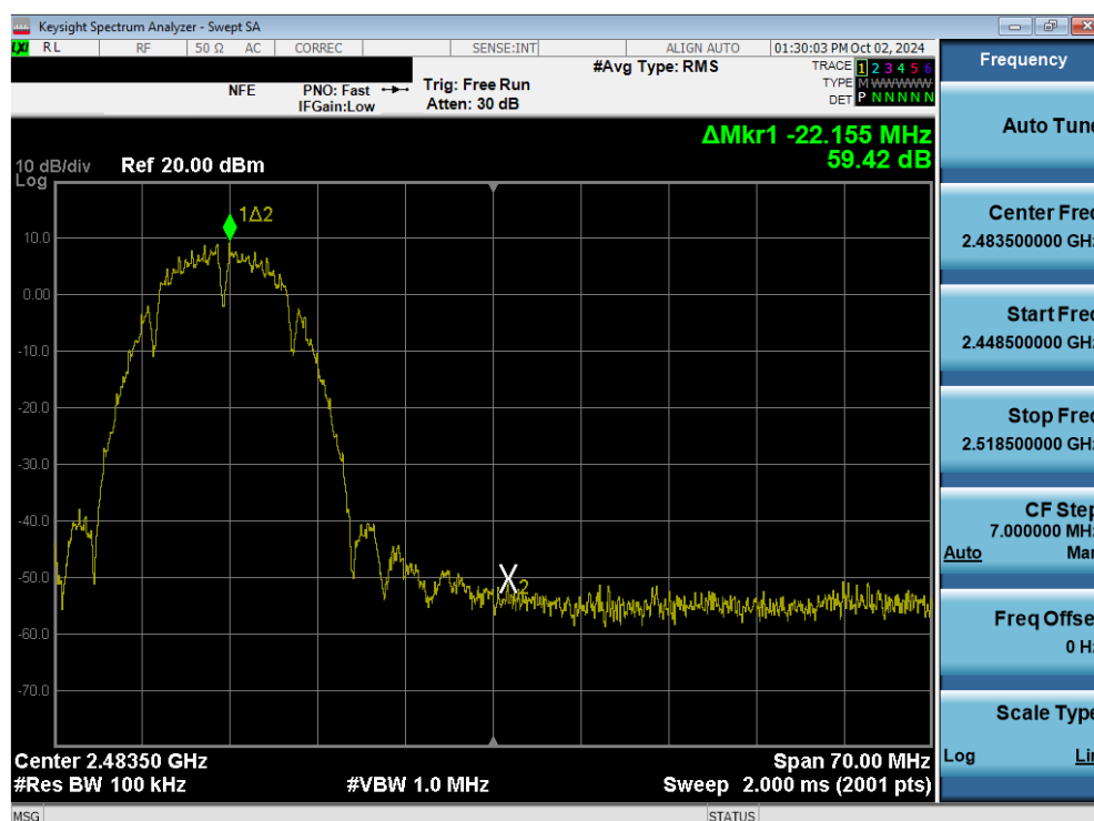
Plot 7-65. Band Edge Plot (802.11b - Ch. 11) MIMO ANT1
