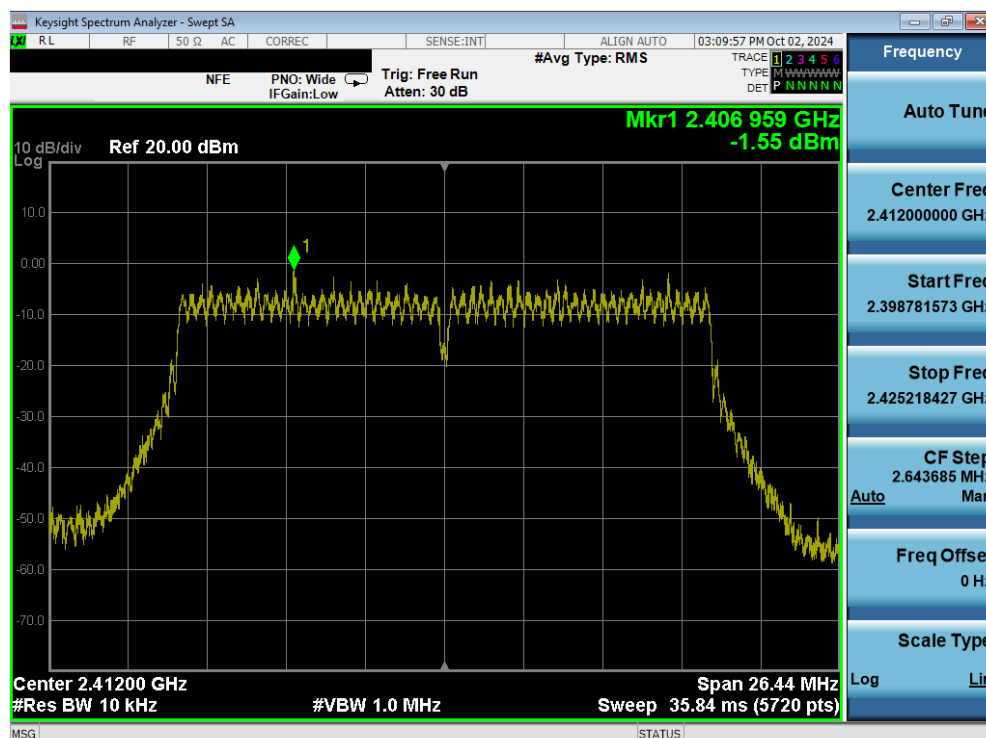
Plot 7-58. Power Spectral Density Plot (802.11ac (2.4GHz) – Ch. 1) MIMO ANT2
