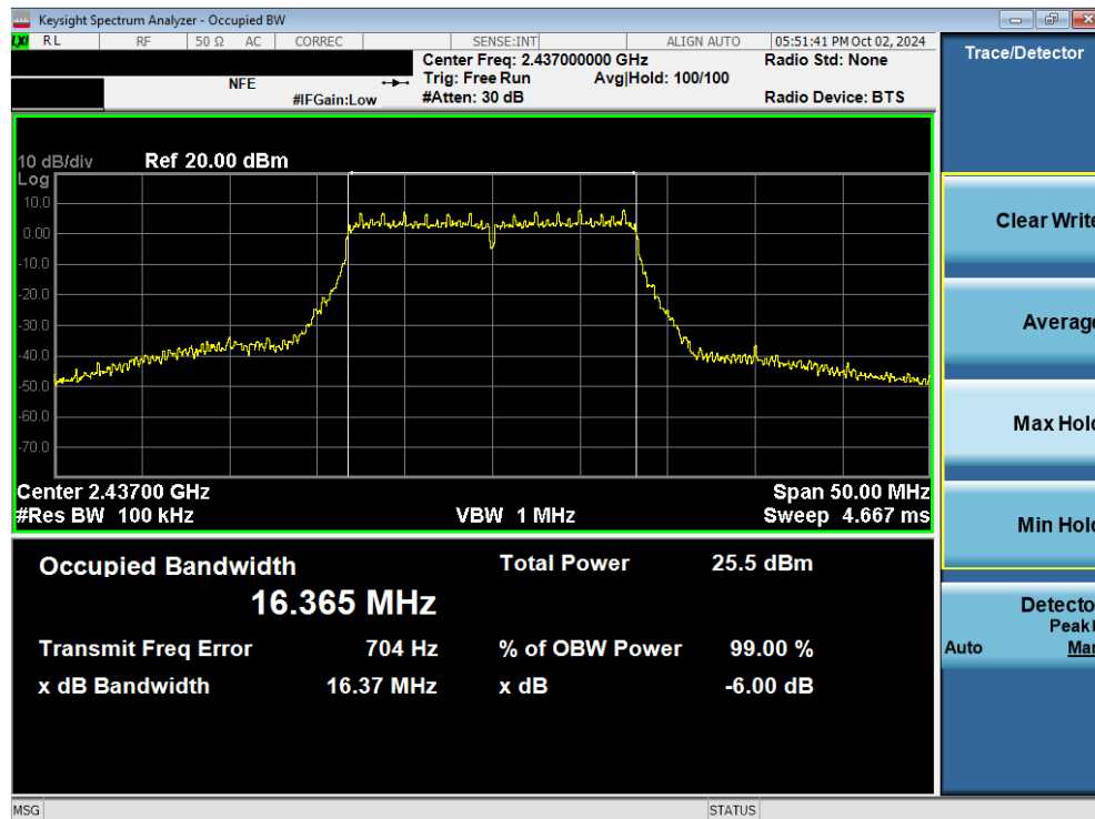
Plot 7-23. 6dB Bandwidth Plot (802.11g – Ch. 6) MIMO ANT2
