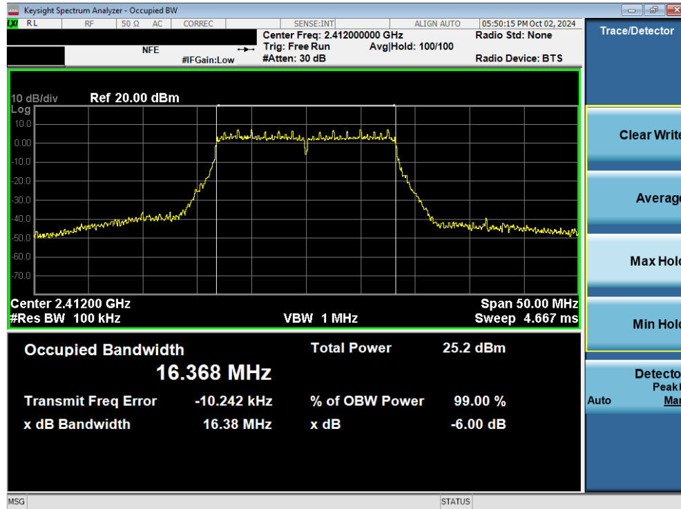
Plot 7-22. 6dB Bandwidth Plot (802.11g – Ch. 1) MIMO ANT2
