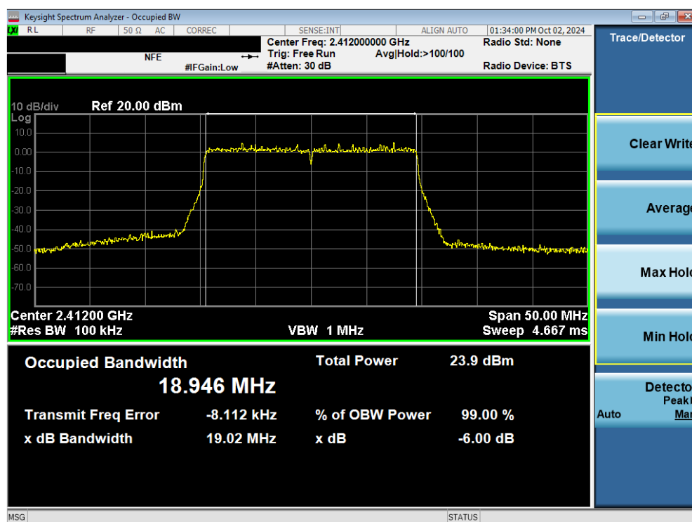
Plot 7-31. 6dB Bandwidth Plot (802.11ax/be (2.4GHz) – Ch. 1) MIMO ANT2
