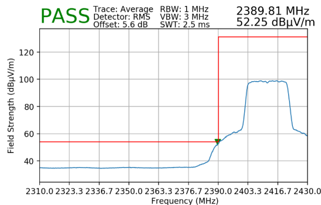
Plot 7-3. Radiated Restricted Lower Band Edge Measurement (Average)
