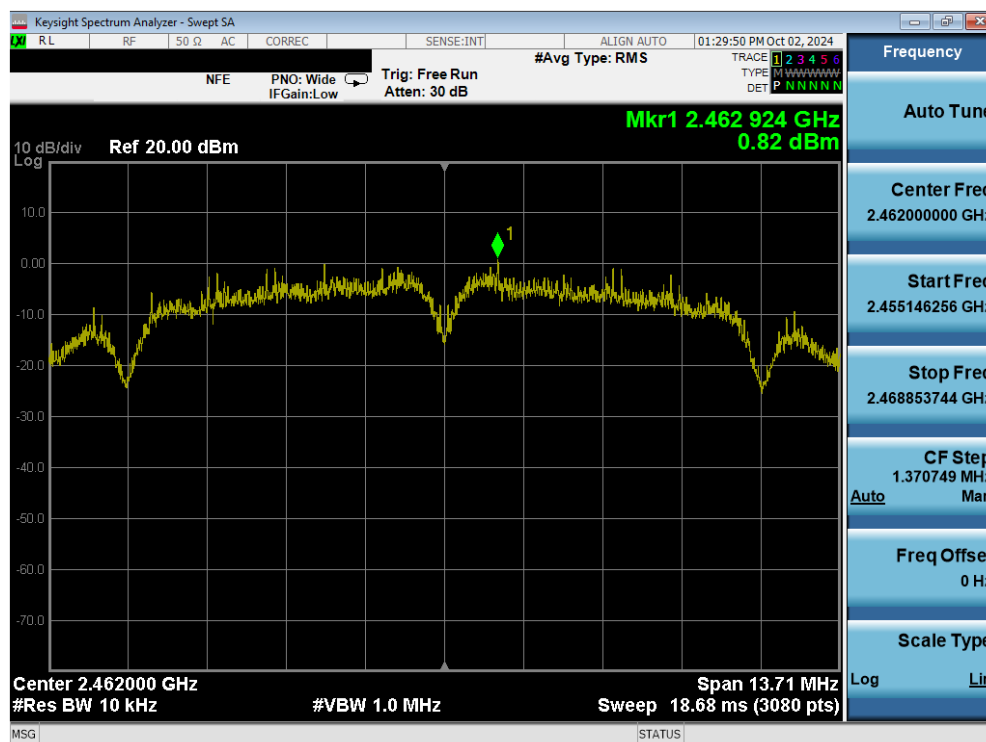
Plot 7-36. Power Spectral Density Plot (802.11b – Ch. 11) MIMO ANT1
