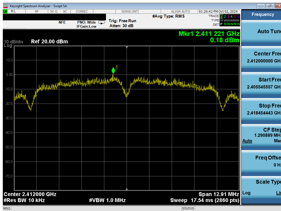
Plot 7-34. Power Spectral Density Plot (802.11b – Ch. 1) MIMO ANT1
