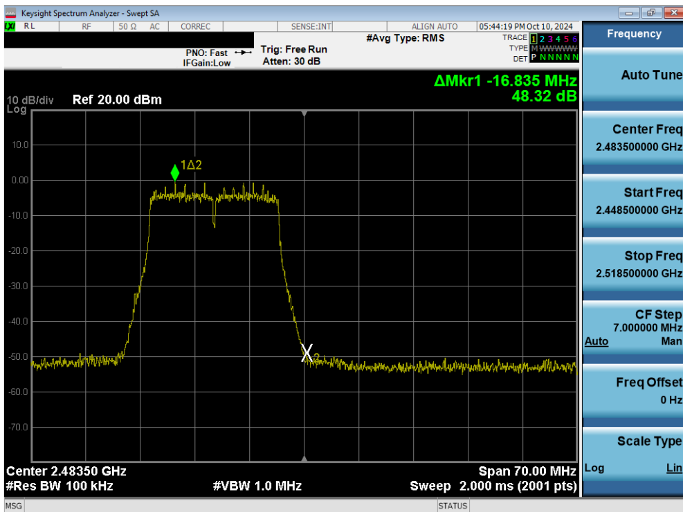
Plot 7-71. Band Edge Plot (802.11g – Ch. 13) MIMO ANT1
