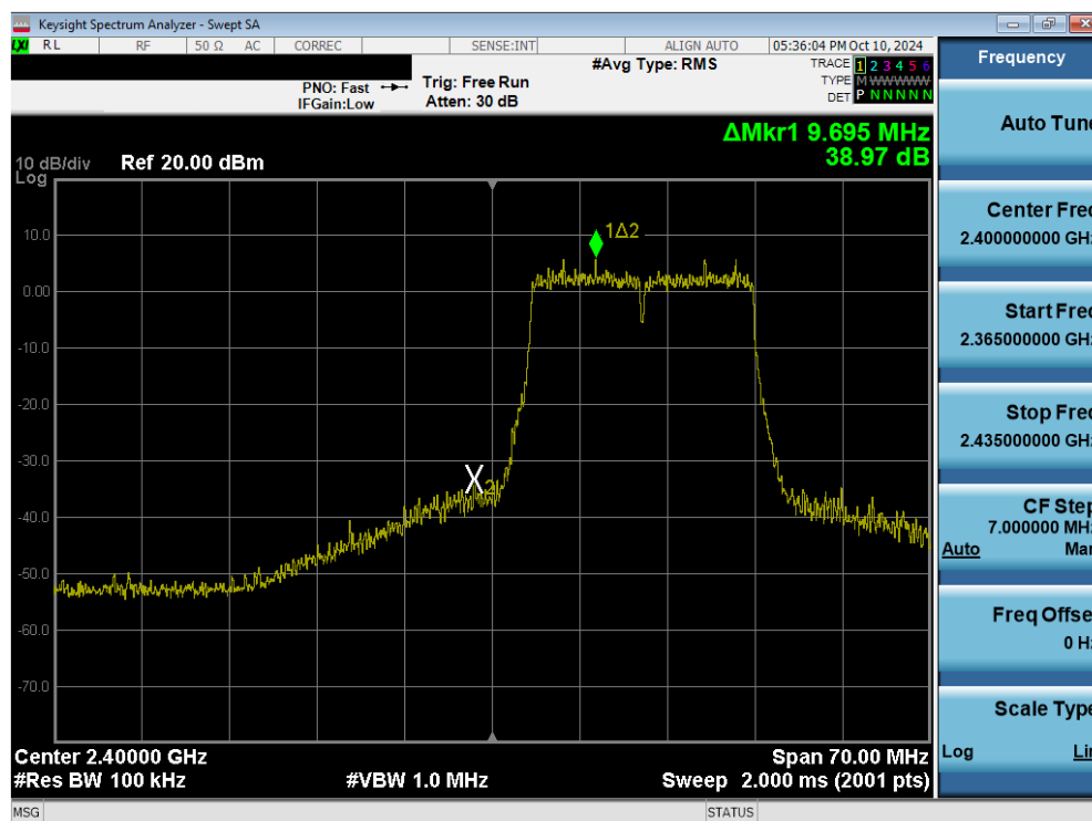
Plot 7-72. Band Edge Plot (802.11n (2.4GHz) – Ch. 1) MIMO ANT1
