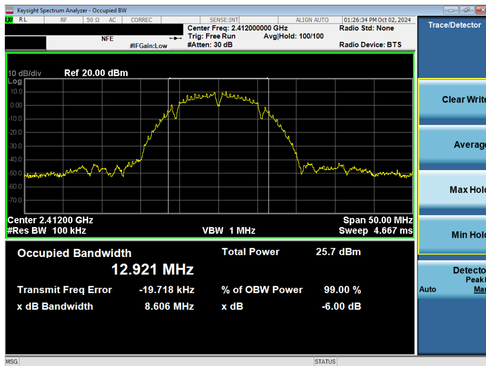
Plot 7-4. 6dB Bandwidth Plot (802.11b – Ch. 1) MIMO ANT1
