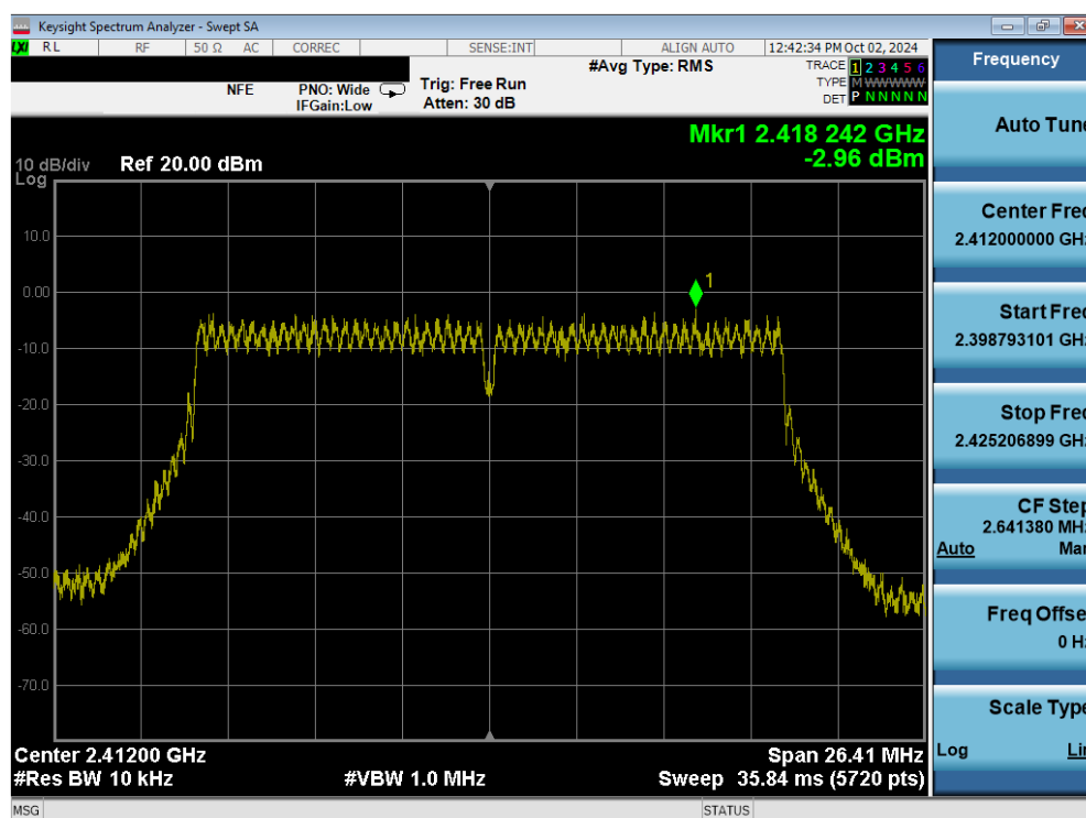
Plot 7-43. Power Spectral Density Plot (802.11ac (2.4GHz) – Ch. 1) MIMO ANT1
