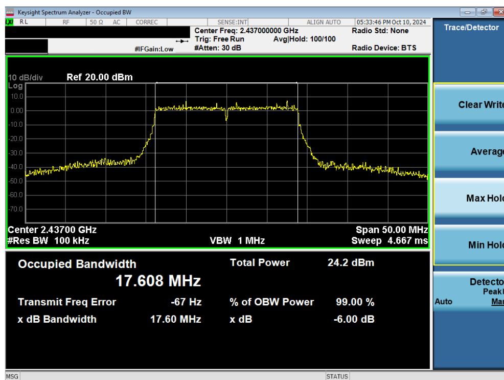
Plot 7-11. 6dB Bandwidth Plot (802.11n (2.4GHz) – Ch. 6) MIMO ANT1
