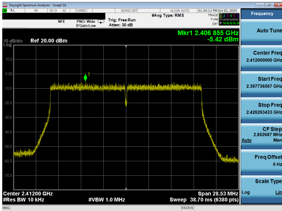
Plot 7-61. Power Spectral Density Plot (802.11ax (2.4GHz) – Ch. 1) MIMO ANT2
