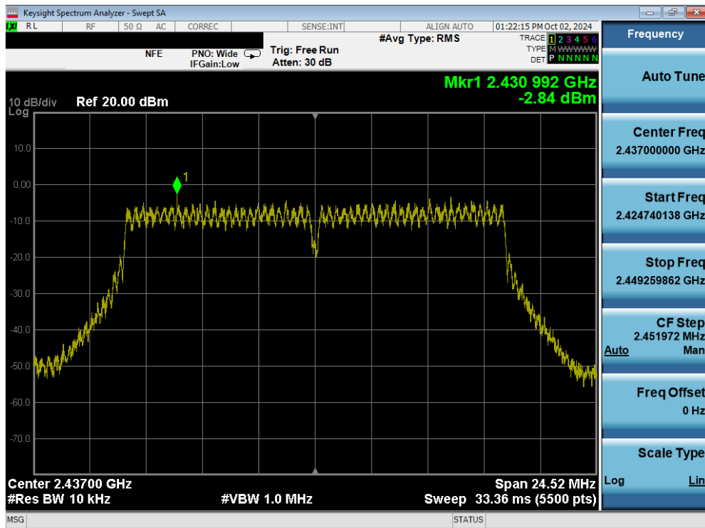
Plot 7-38. Power Spectral Density Plot (802.11g – Ch. 6) MIMO ANT1
