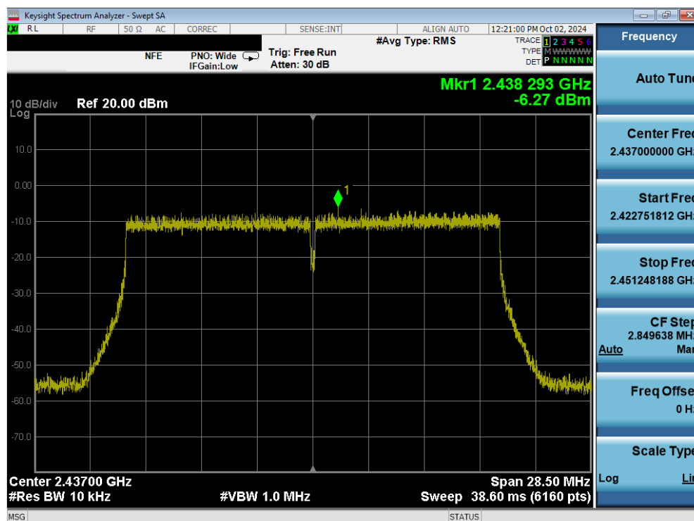
Plot 7-47. Power Spectral Density Plot (802.11ax/be (2.4GHz) – Ch. 6) MIMO ANT1
