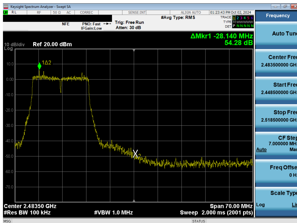
Plot 7-69. Band Edge Plot (802.11g – Ch. 11) MIMO ANT1
