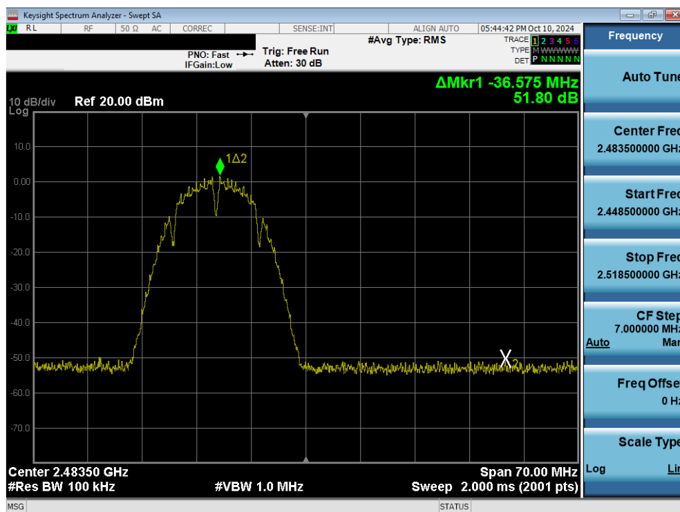
Plot 7-67. Band Edge Plot (802.11b – Ch. 13) MIMO ANT1
