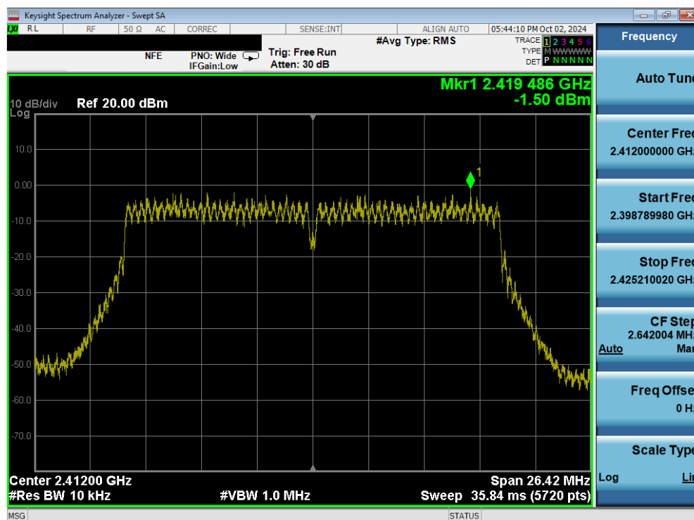
Plot 7-55. Power Spectral Density Plot (802.11n (2.4GHz) – Ch. 1) MIMO ANT2
