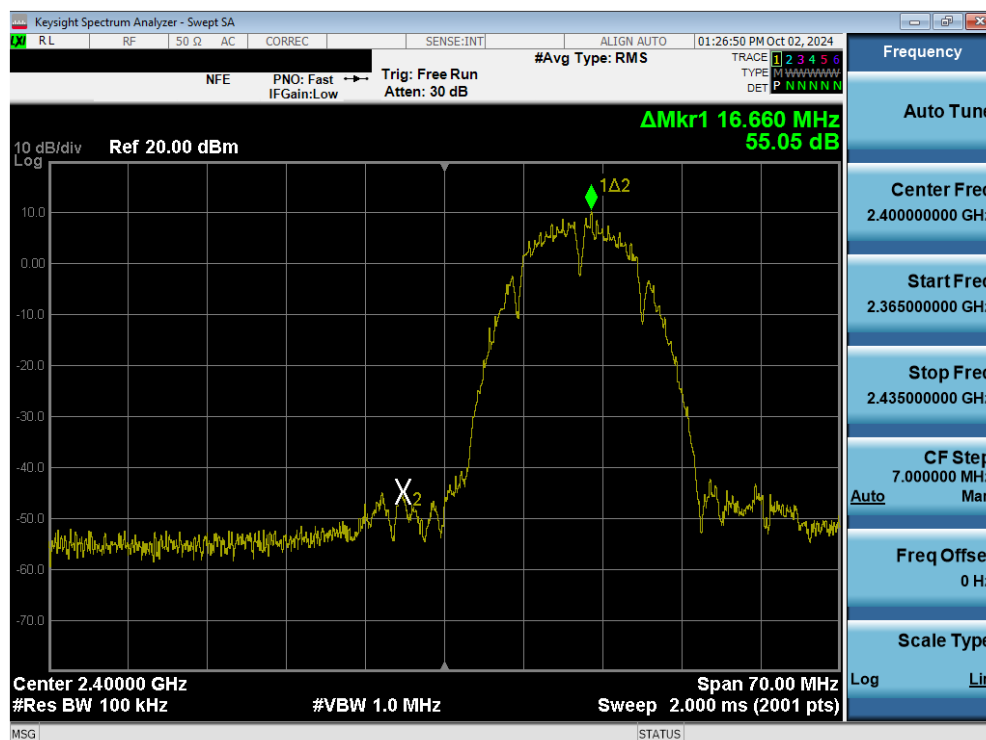
Plot 7-64. Band Edge Plot (802.11b - Ch. 1) - MIMO ANT1
