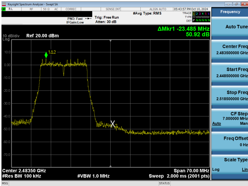
Plot 7-70. Band Edge Plot (802.11g – Ch. 12) MIMO ANT1
