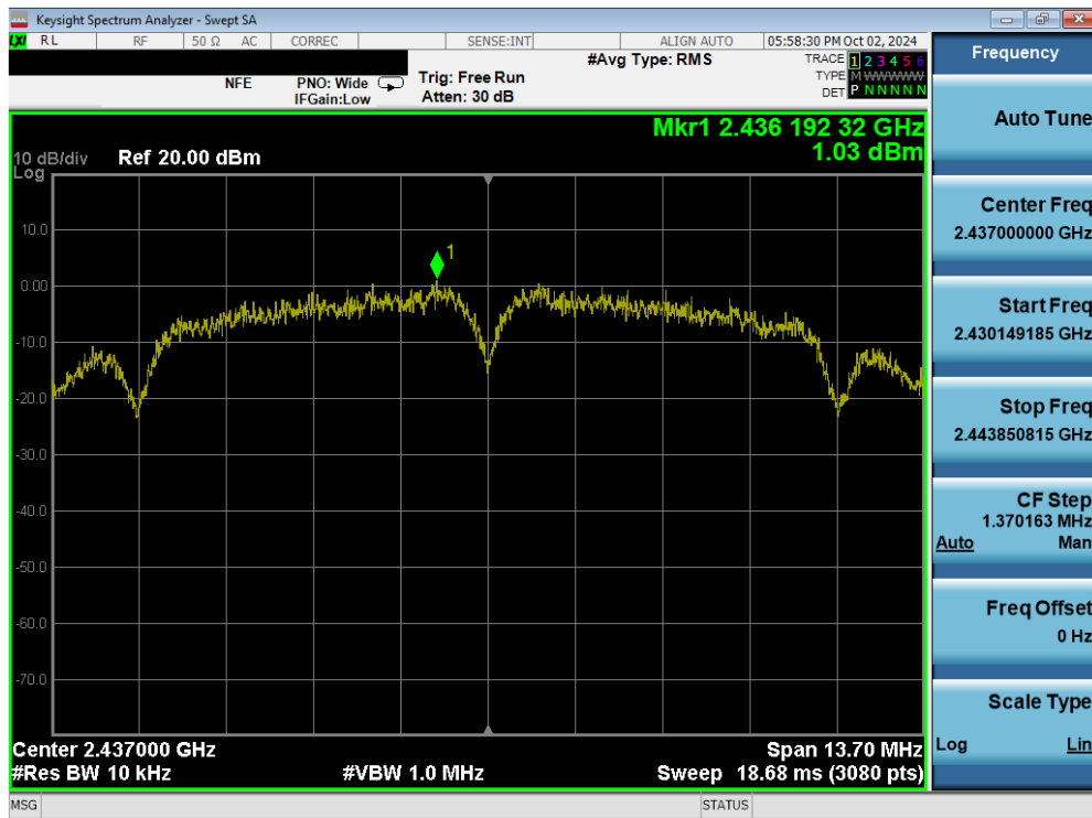
Plot 7-50. Power Spectral Density Plot (802.11b – Ch. 6) MIMO ANT2
