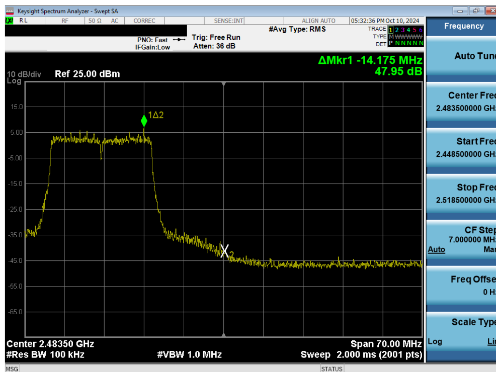
Plot 7-73. Band Edge Plot (802.11n (2.4GHz) – Ch. 11) MIMO ANT1
