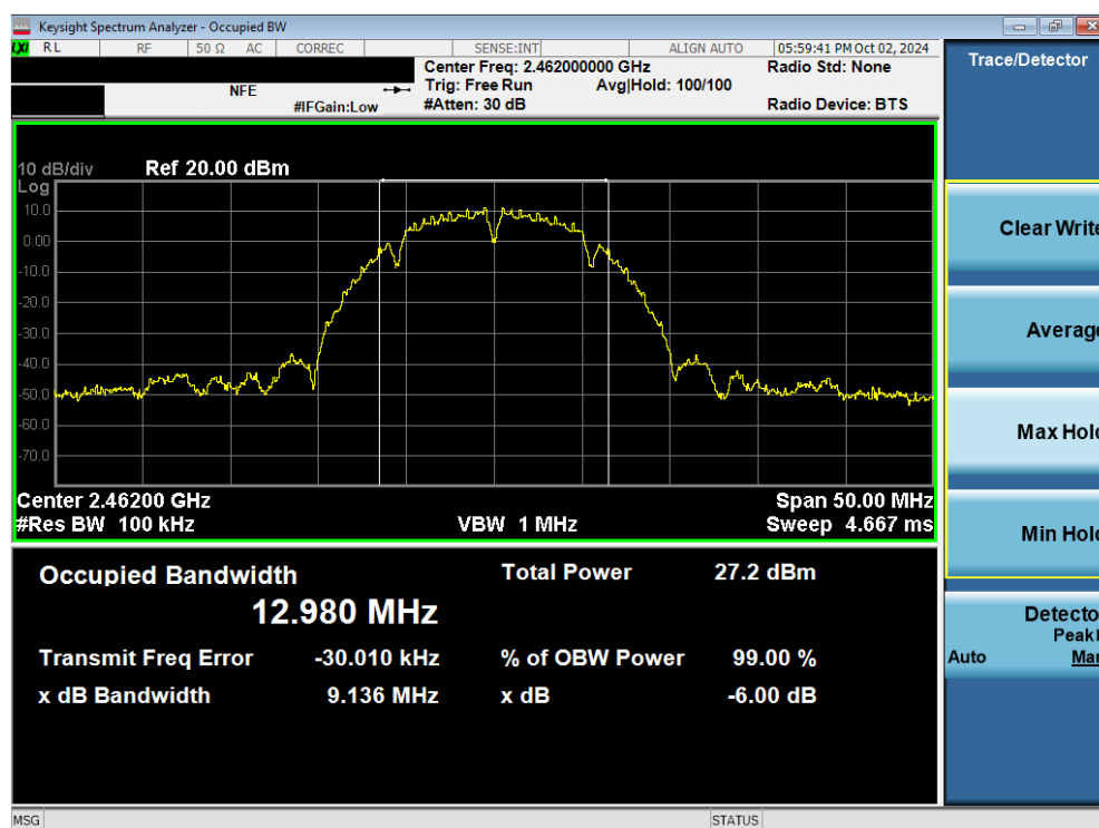
Plot 7-21. 6dB Bandwidth Plot (802.11b – Ch. 11) MIMO ANT2
