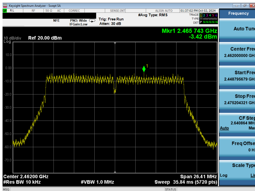
Plot 7-63. Power Spectral Density Plot (802.11ax (2.4GHz) – Ch. 11) MIMO ANT2
