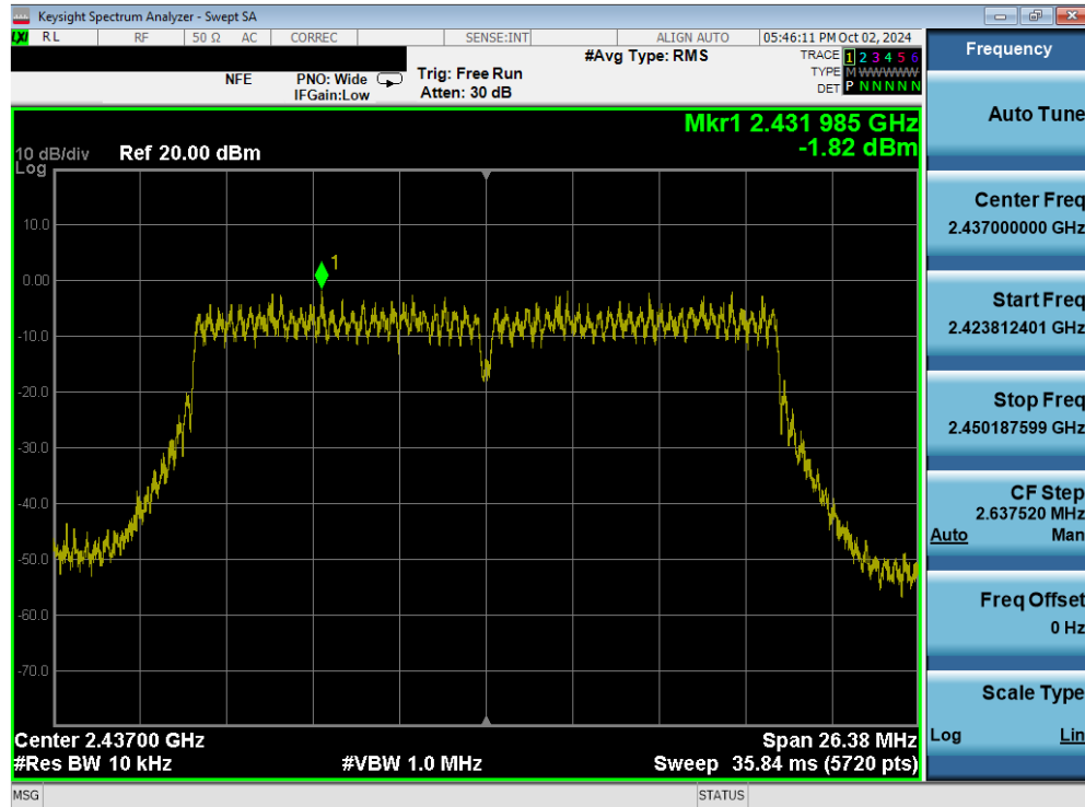
Plot 7-56. Power Spectral Density Plot (802.11n (2.4GHz) – Ch. 6) MIMO ANT2
