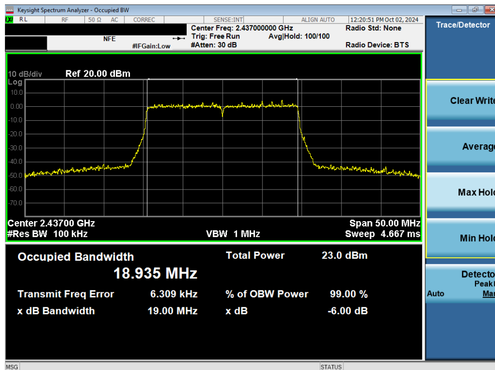
Plot 7-17. 6dB Bandwidth Plot (802.11ax/be (2.4GHz) – Ch. 6) MIMO ANT1
