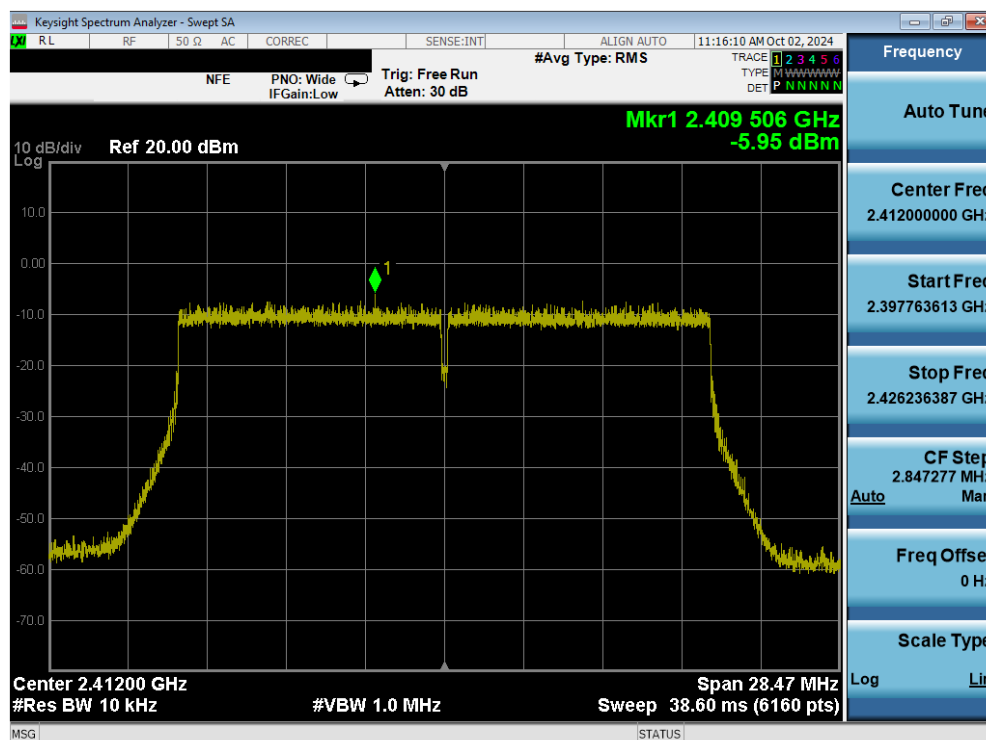
Plot 7-46. Power Spectral Density Plot (802.11ax/be (2.4GHz) – Ch. 1) MIMO ANT1
