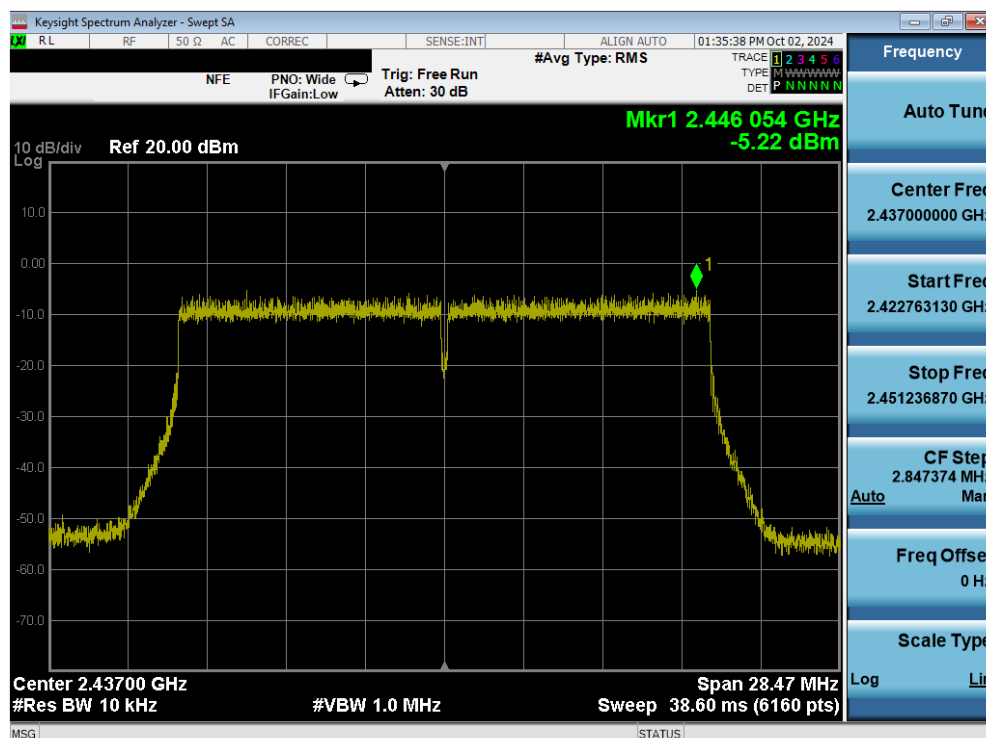
Plot 7-62. Power Spectral Density Plot (802.11ax (2.4GHz) – Ch. 6) MIMO ANT2
