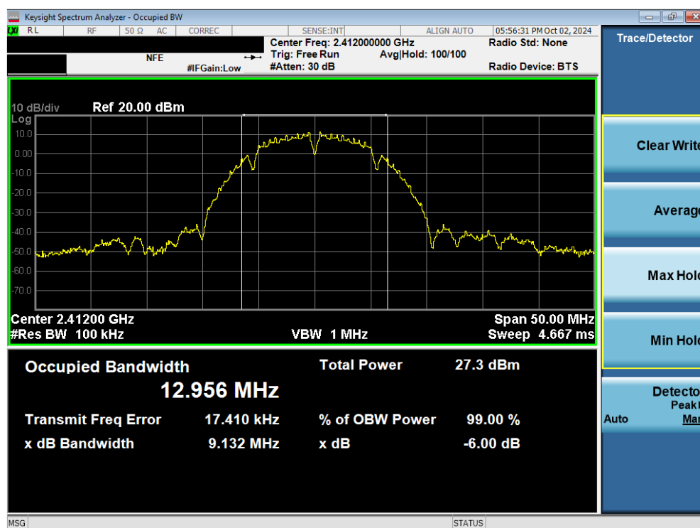
Plot 7-19. 6dB Bandwidth Plot (802.11b – Ch. 1) MIMO ANT2
