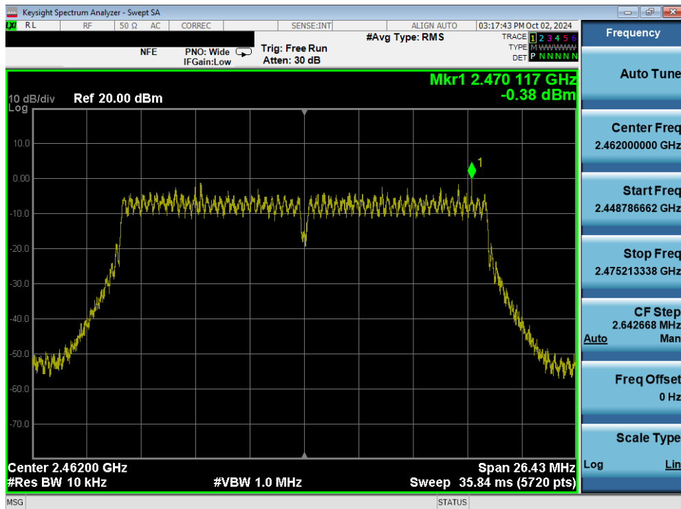
Plot 7-60. Power Spectral Density Plot (802.11ac (2.4GHz) – Ch. 11) MIMO ANT2
