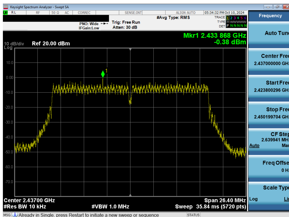
Plot 7-41. Power Spectral Density Plot (802.11n (2.4GHz) – Ch. 6) MIMO ANT1
