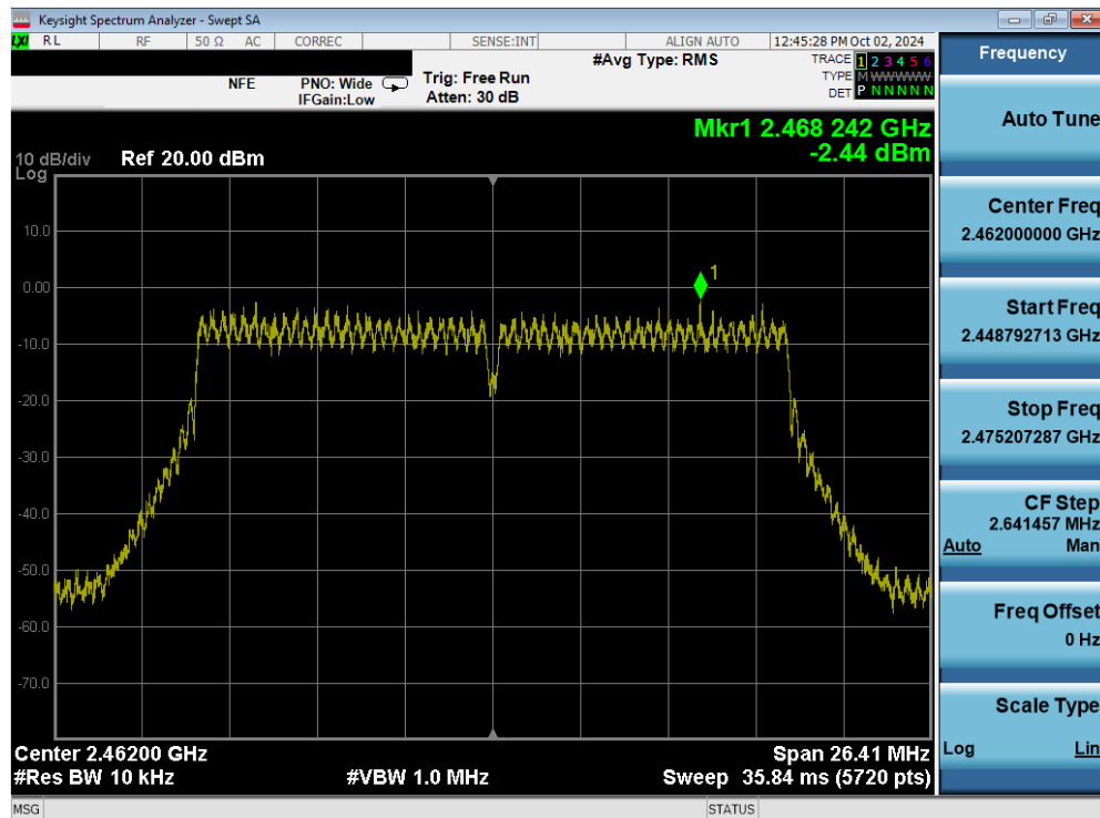
Plot 7-45. Power Spectral Density Plot (802.11ac (2.4GHz) – Ch. 11) MIMO ANT1
