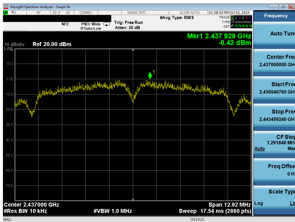
Plot 7-35. Power Spectral Density Plot (802.11b – Ch. 6) MIMO ANT1
