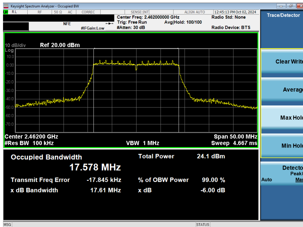
Plot 7-15. 6dB Bandwidth Plot (802.11ac (2.4GHz) – Ch. 11) MIMO ANT1
