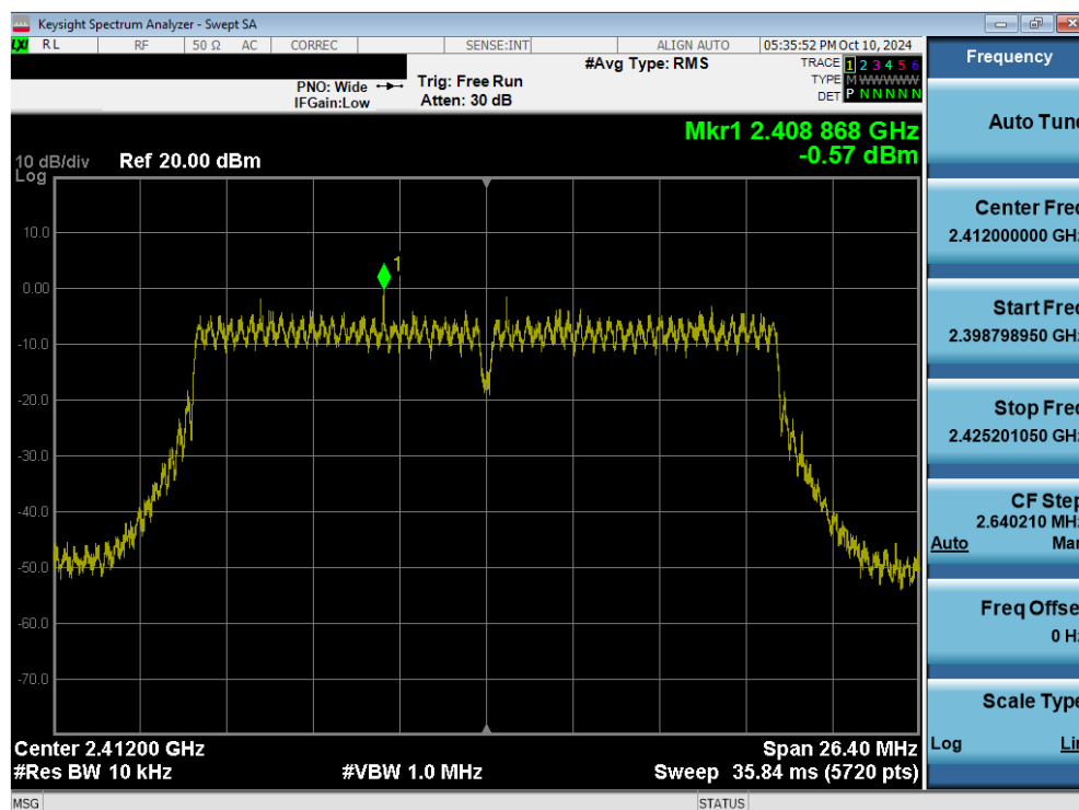
Plot 7-40. Power Spectral Density Plot (802.11n (2.4GHz) – Ch. 1) MIMO ANT1
