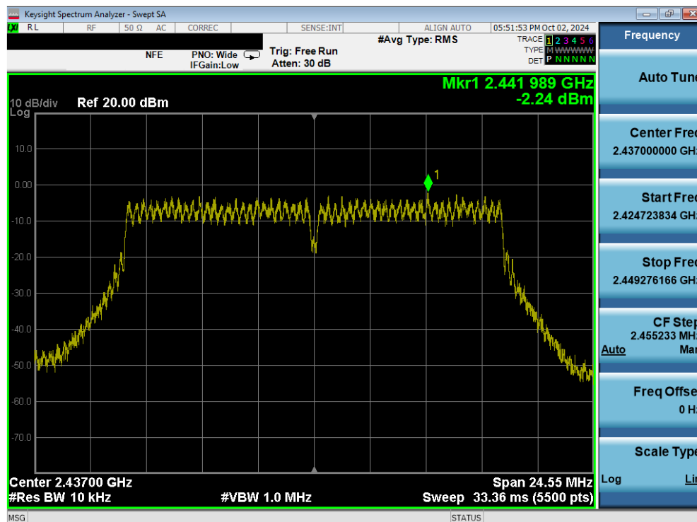
Plot 7-53. Power Spectral Density Plot (802.11g – Ch. 6) MIMO ANT2
