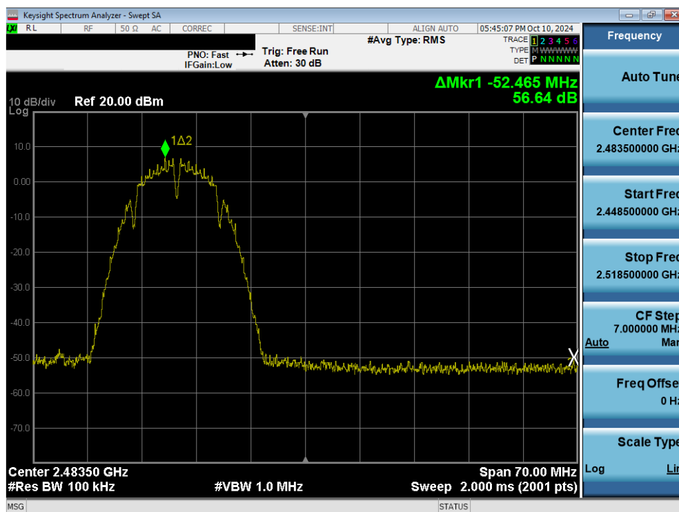
Plot 7-66. Band Edge Plot (802.11b – Ch. 12) MIMO ANT1
