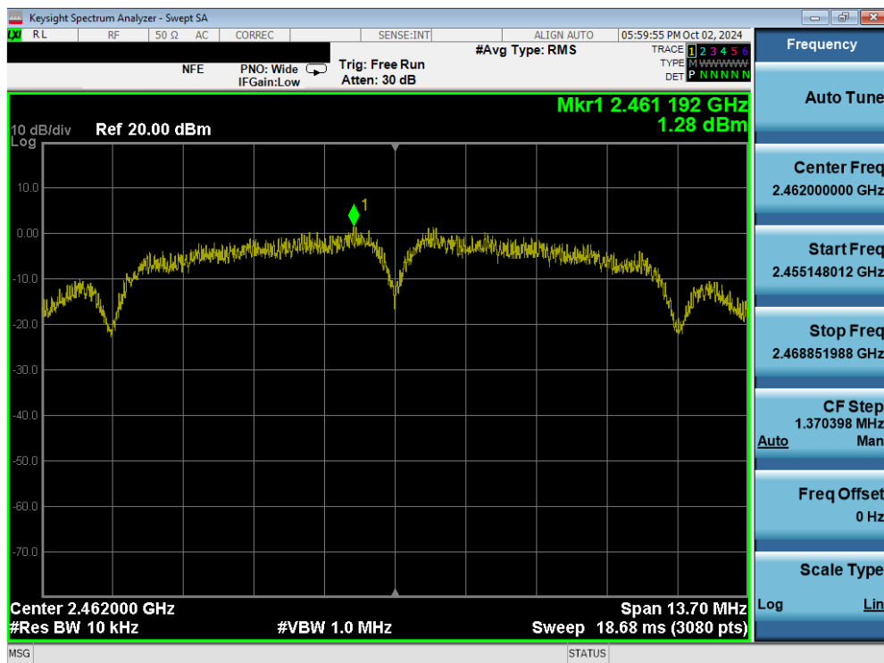
Plot 7-51. Power Spectral Density Plot (802.11b – Ch. 11) MIMO ANT2
