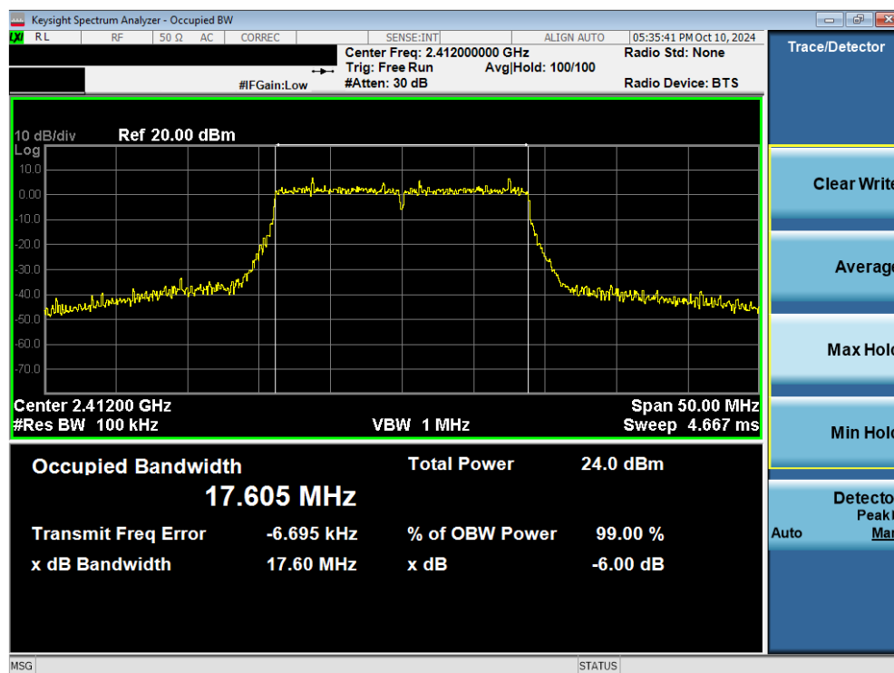
Plot 7-10. 6dB Bandwidth Plot (802.11n (2.4GHz) – Ch. 1) MIMO ANT1
