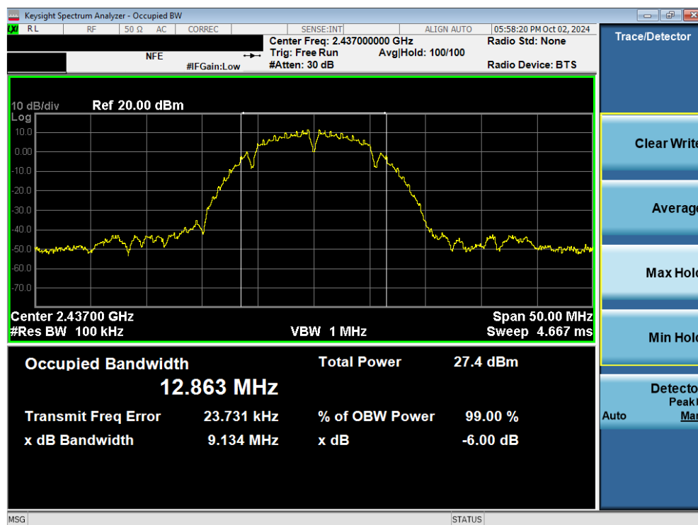
Plot 7-20. 6dB Bandwidth Plot (802.11b – Ch. 6) MIMO ANT2
