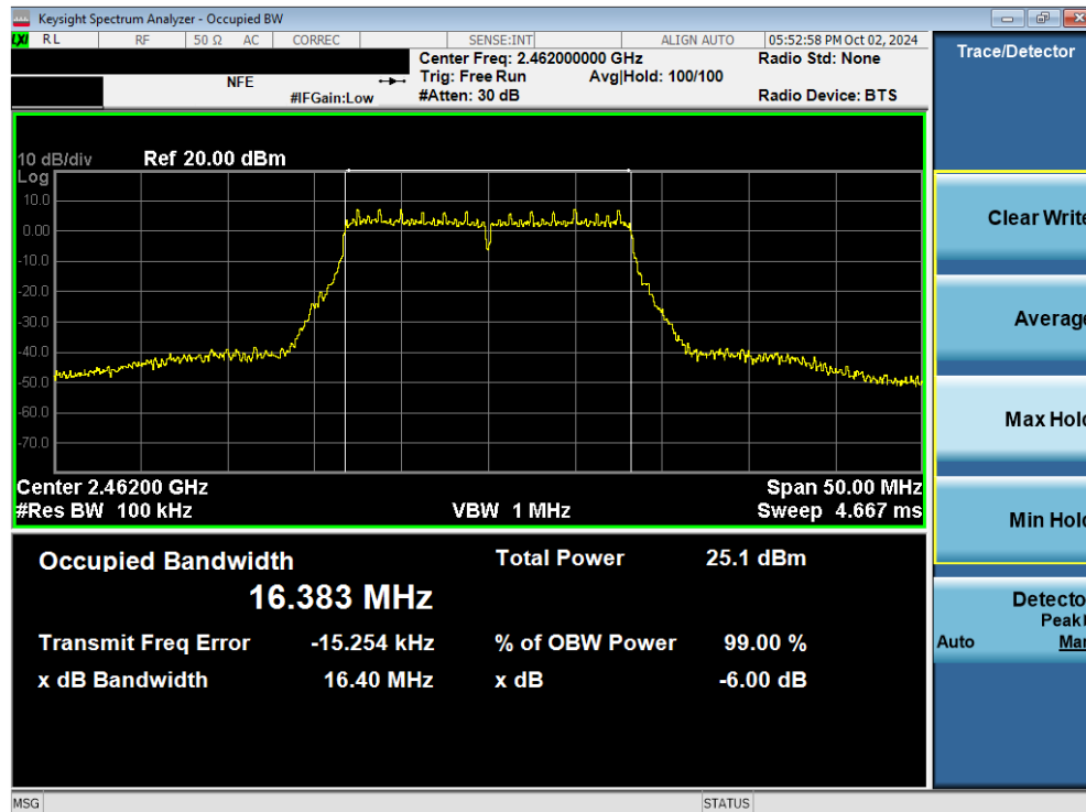
Plot 7-24. 6dB Bandwidth Plot (802.11g – Ch. 11) MIMO ANT2
