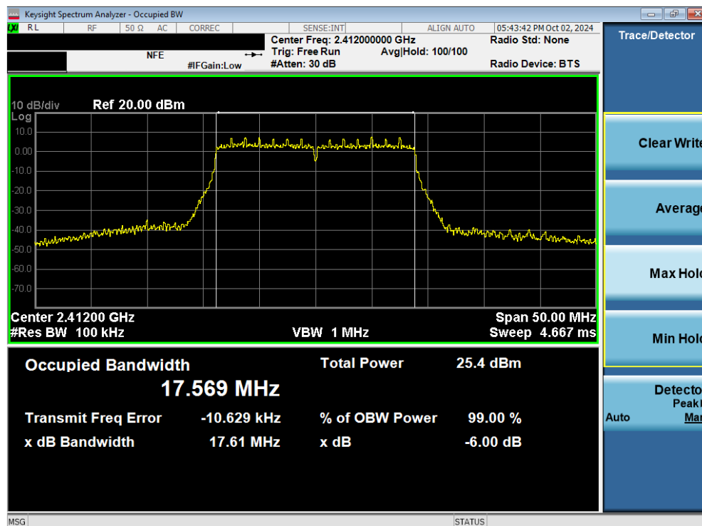
Plot 7-25. 6dB Bandwidth Plot (802.11n (2.4GHz) – Ch. 1) MIMO ANT2
