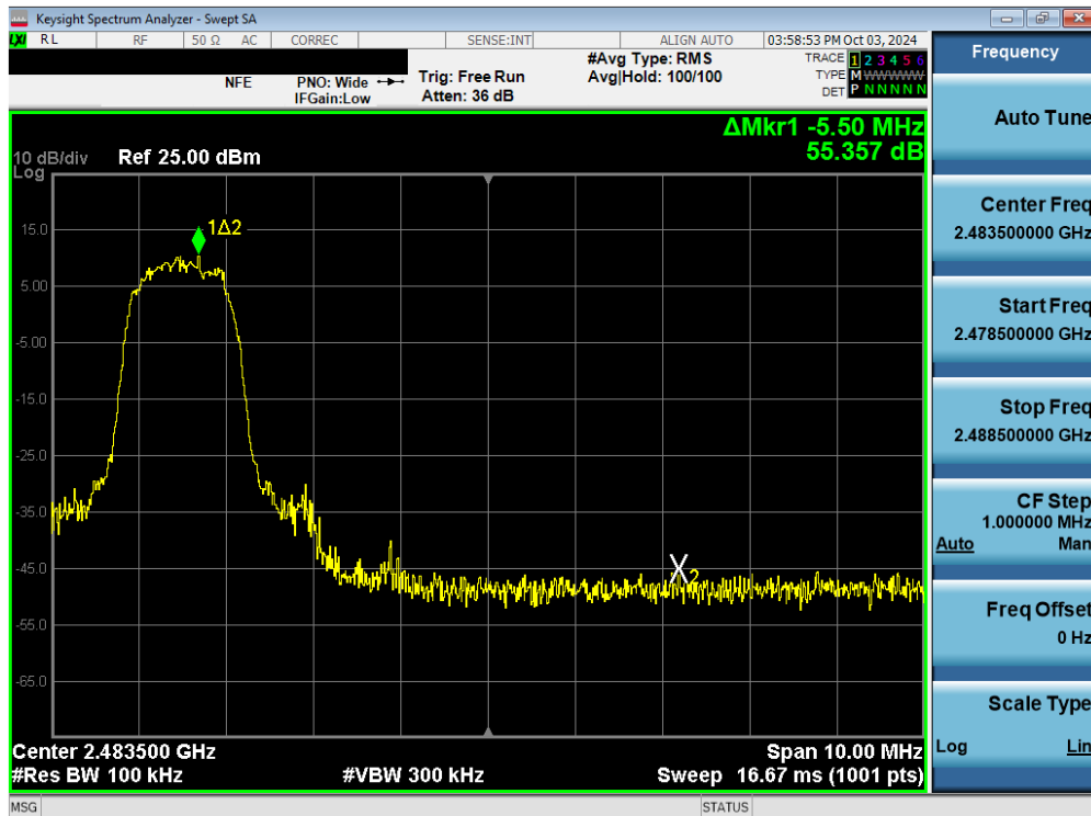
Plot 7-124. Band Edge Plot (Bluetooth with Hopping Disabled, 3 Mbps – Ch. 78) – Dual Ant 2
