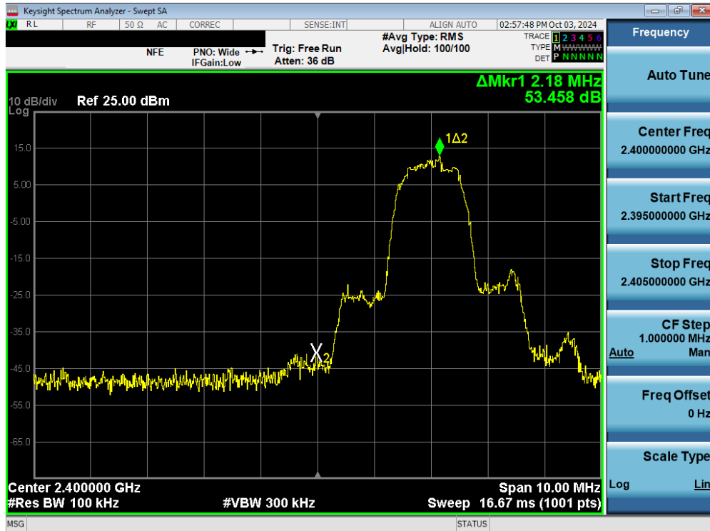
Plot 7-119. Band Edge Plot (Bluetooth with Hopping Disabled, 3 Mbps – Ch. 0) – Dual Ant 1
