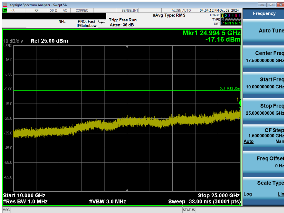
Plot 7-166. Conducted Spurious Plot (Bluetooth, 1Mbps – Ch. 78) – Dual Ant 2
