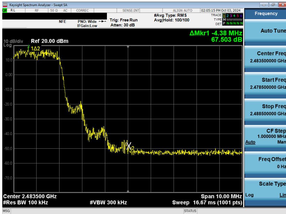
Plot 7-118. Band Edge Plot (Bluetooth with Hopping Enabled, 3 Mbps) – Ant 2
