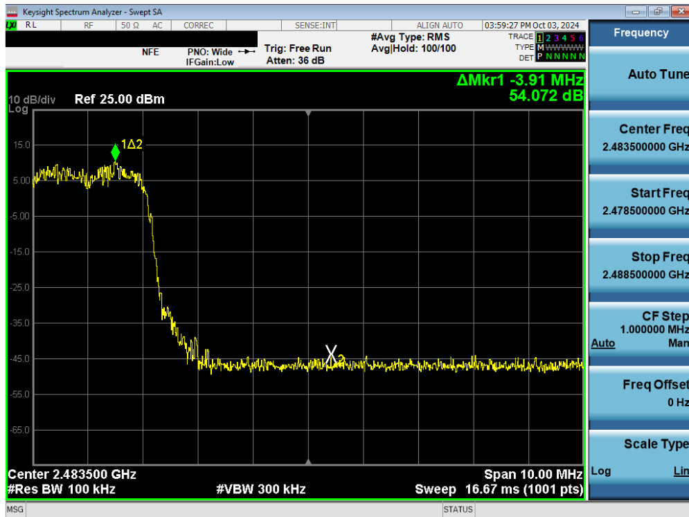
Plot 7-126. Band Edge Plot (Bluetooth with Hopping Enabled, 3 Mbps) – Dual Ant 2
