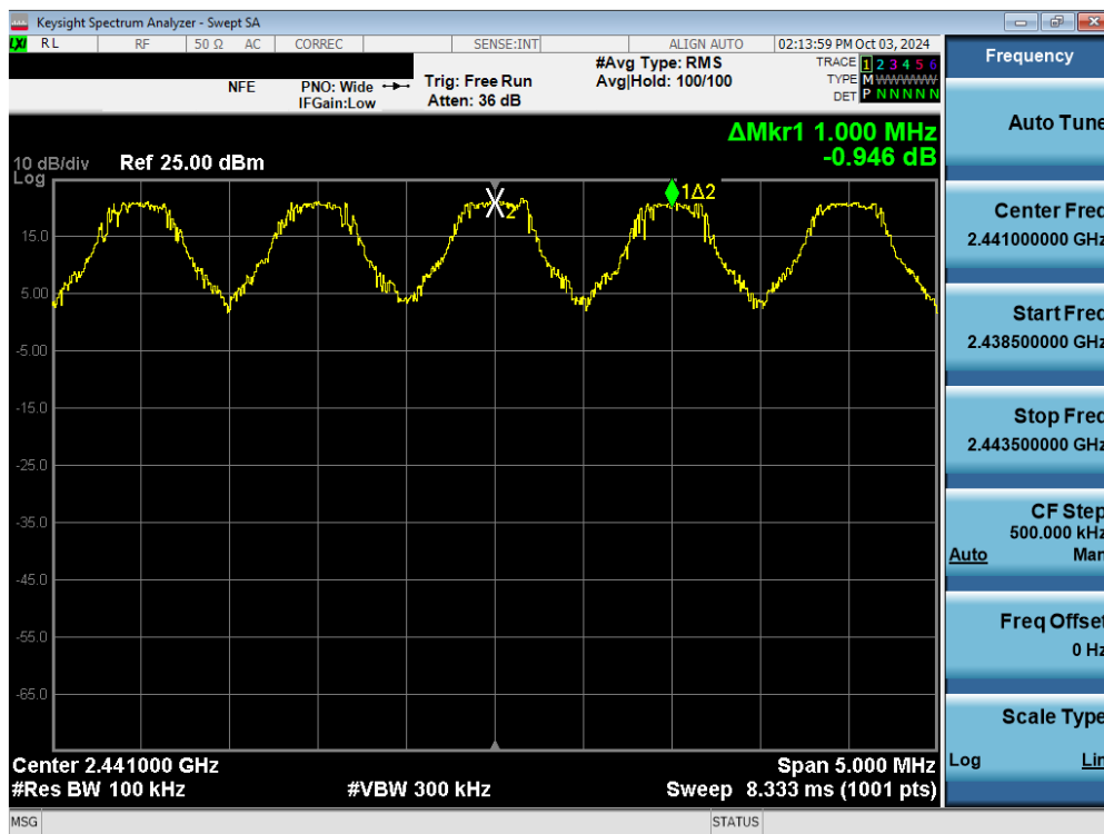
Plot 7-128. Channel Spacing Plot (Bluetooth) – Ant 2
