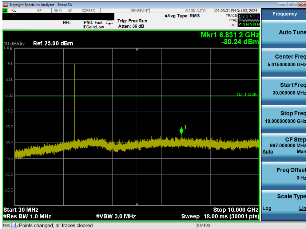
Plot 7-165. Conducted Spurious Plot (Bluetooth, 1Mbps – Ch. 78) – Dual Ant 2
