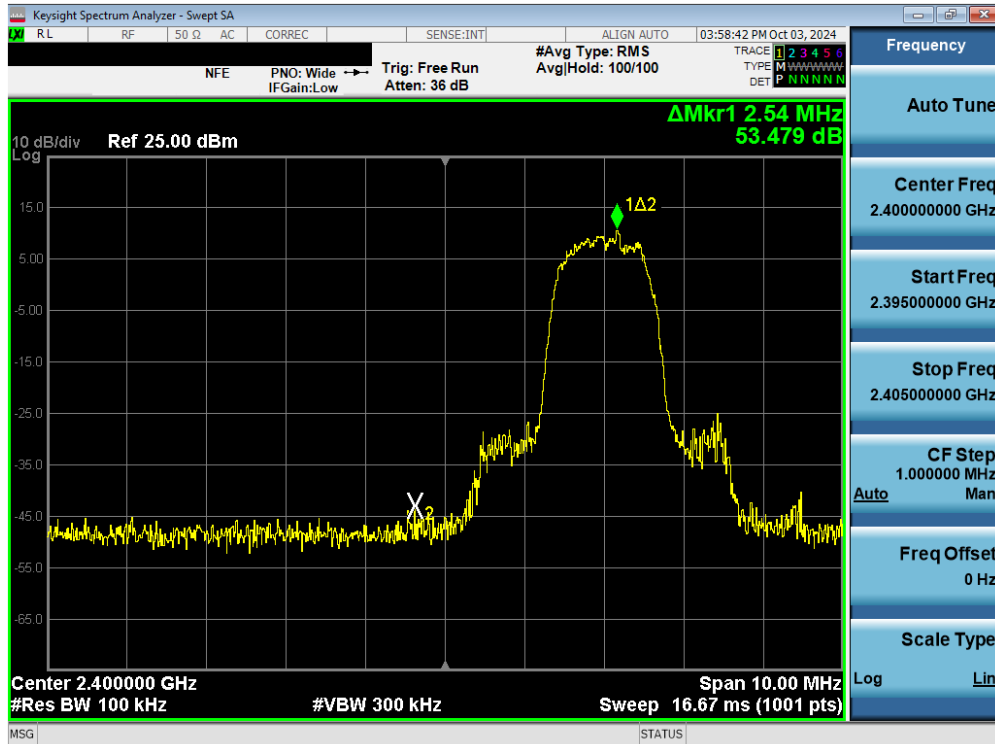
Plot 7-123. Band Edge Plot (Bluetooth with Hopping Disabled, 3 Mbps – Ch. 0) – Dual Ant 2
