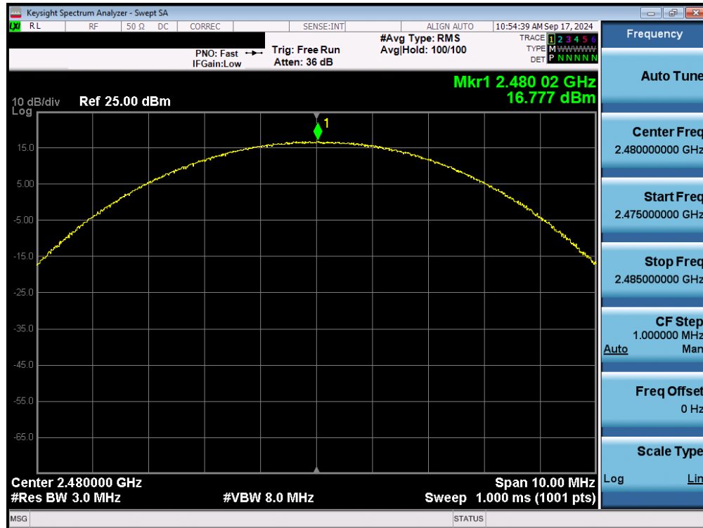
Plot 7-44. Peak Conducted Power (2Mbps – Ch. 78) – Ant 1
