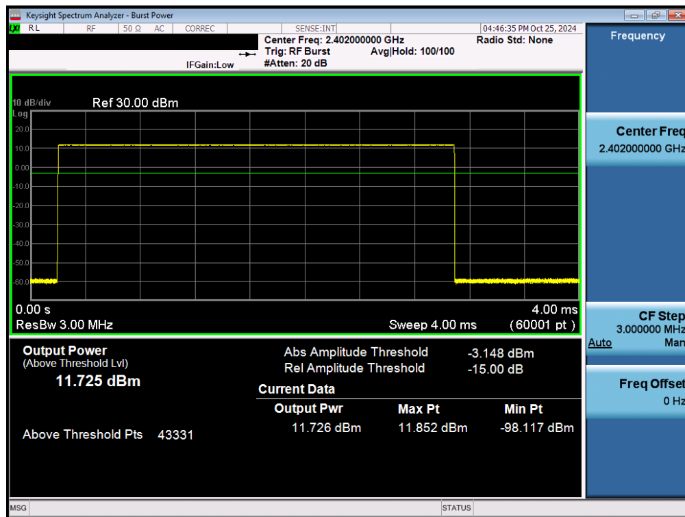
Plot 7-84. Average Conducted Power (1Mbps – Ch. 0) – Dual Ant 1
