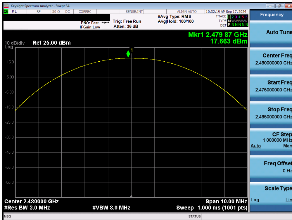
Plot 7-41. Peak Conducted Power (1Mbps – Ch. 78) – Ant 1
