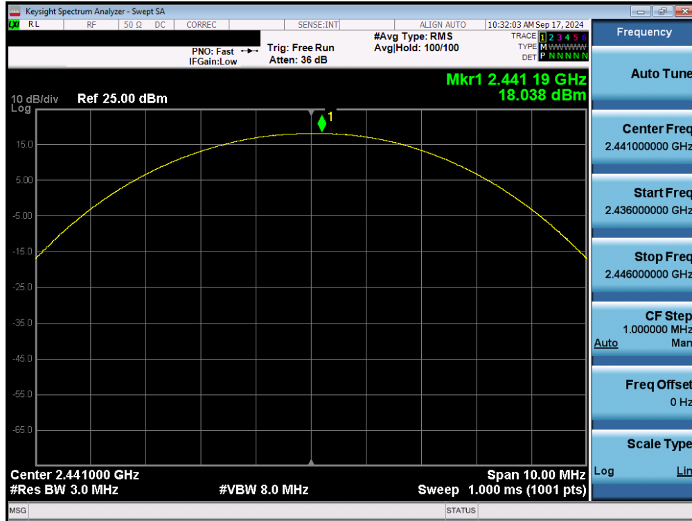
Plot 7-40. Peak Conducted Power (1Mbps – Ch. 39) – Ant 1
