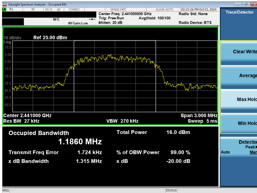
Plot 7-10. 20dB Bandwidth Plot (Bluetooth, 3Mbps – Ch. 39) – Ant 1
