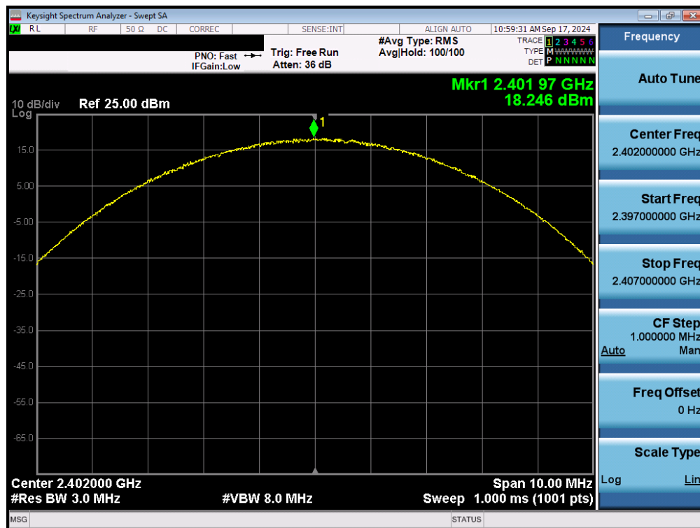
Plot 7-45. Peak Conducted Power (3Mbps – Ch. 0) – Ant 1
