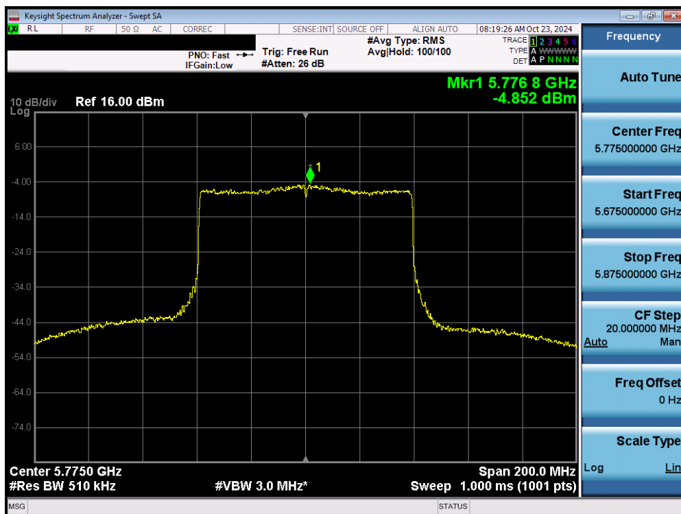
Plot 7-79. Power Spectral Density Plot MIMO ANT1 (80MHz 802.11ax/be (UNII Band 3) – Ch. 155)
