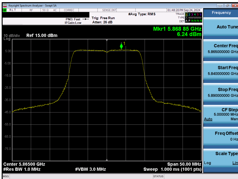
Plot 7-112. Power Spectral Density Plot MIMO ANT2 (20MHz 802.11n (UNII Band 4) – Ch.173)
