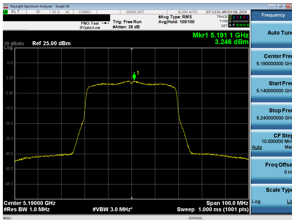
Plot 7-96. Power Spectral Density Plot MIMO ANT2 (40MHz 802.11ax/be (UNII Band 1) – Ch. 38)
