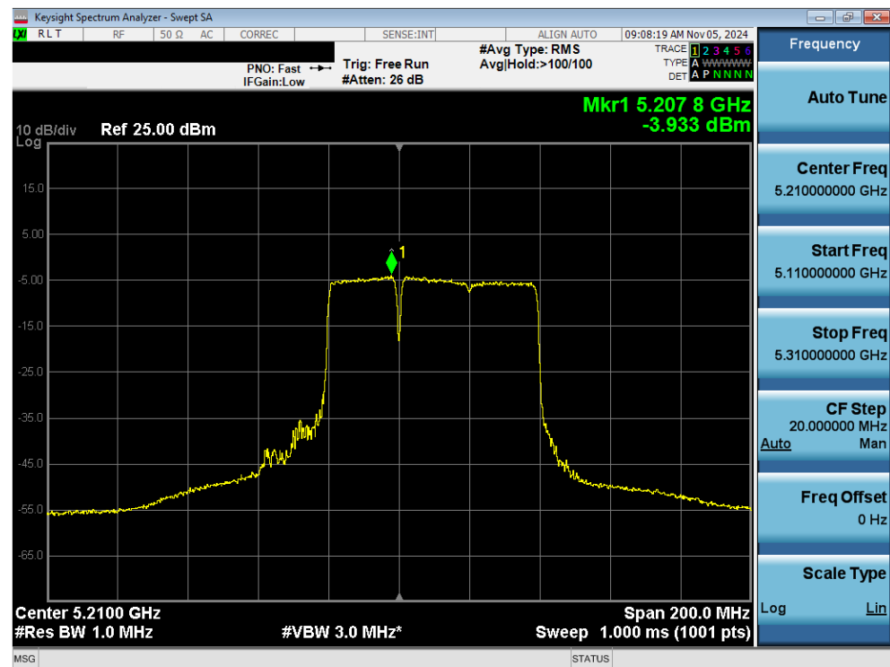
Plot 7-101. Power Spectral Density Plot MIMO ANT2 (80MHz 802.11be (20MHz Puncture) (UNII Band 1) – Ch. 42)
