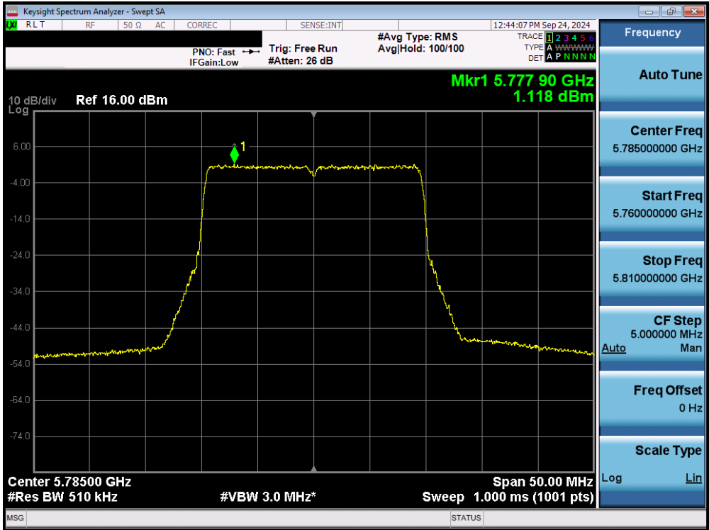
Plot 7-105. Power Spectral Density Plot MIMO ANT2 (20MHz 802.11ax/be (UNII Band 3) – Ch.157)
