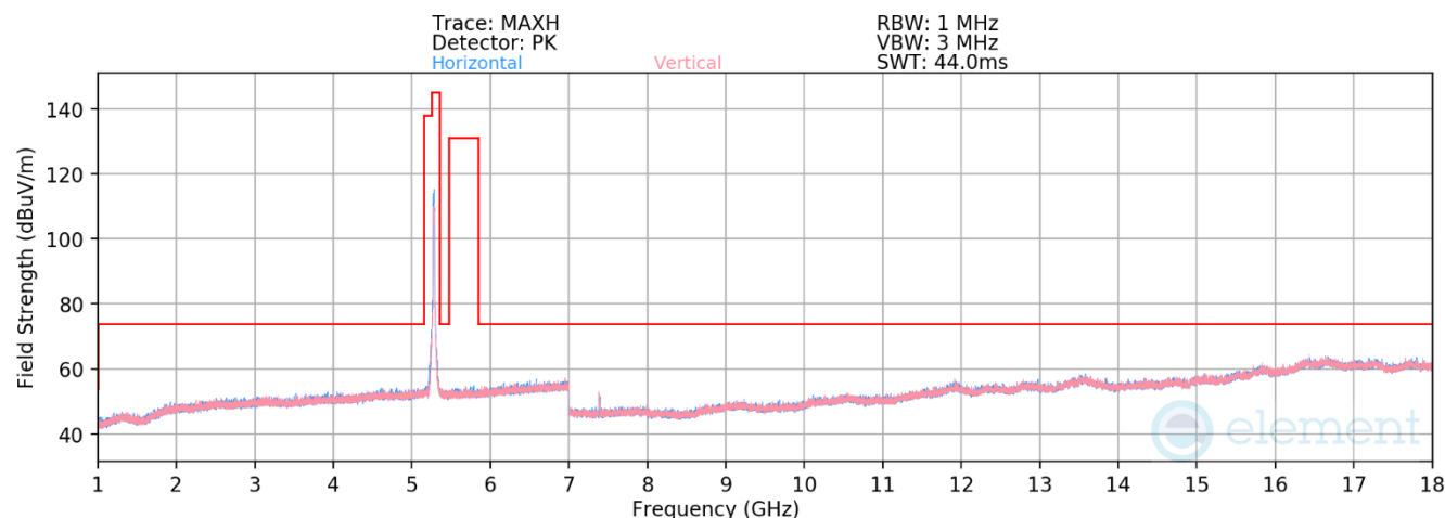
Plot 7-124. Radiated Spurious Plot above 1GHz MIMO (802.11ax – UNII Band 2A Ch. 56)
