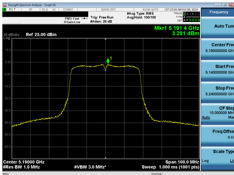
Plot 7-95. Power Spectral Density Plot MIMO ANT2 (40MHz 802.11n (UNII Band 1) – Ch. 38)
