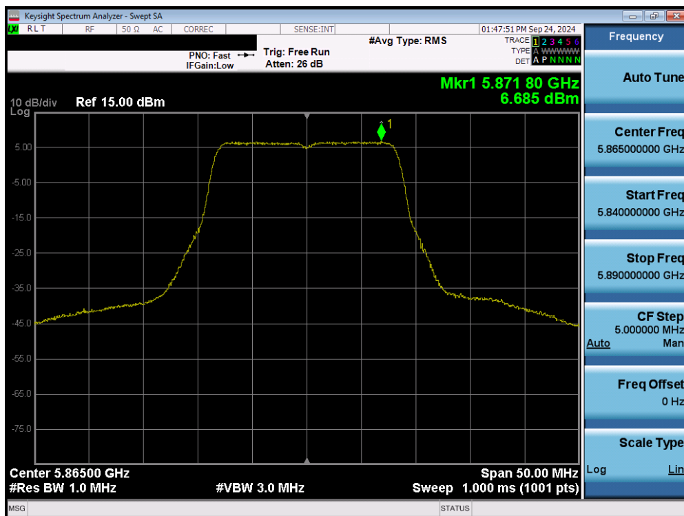
Plot 7-111. Power Spectral Density Plot MIMO ANT2 (20MHz 802.11a (UNII Band 4) – Ch.173)
