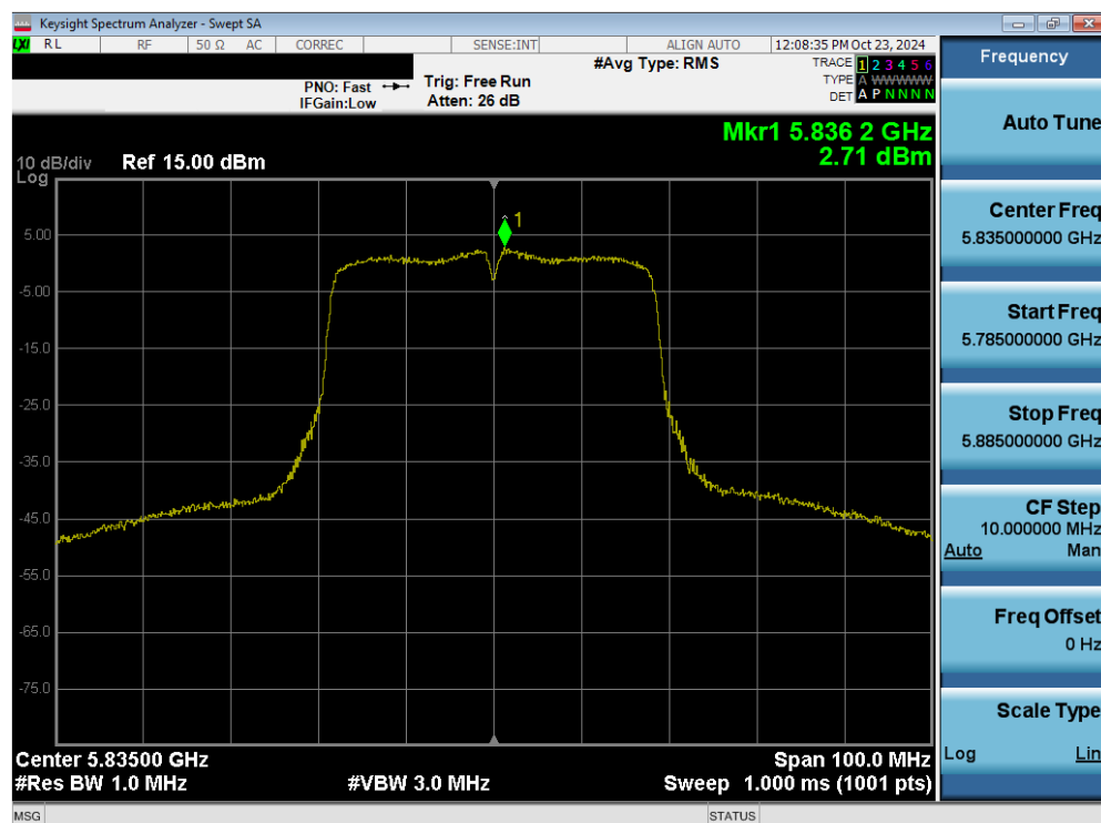
Plot 7-114. Power Spectral Density Plot MIMO ANT2 (40MHz 802.11n (UNII Band 3/4) – Ch. 167)
