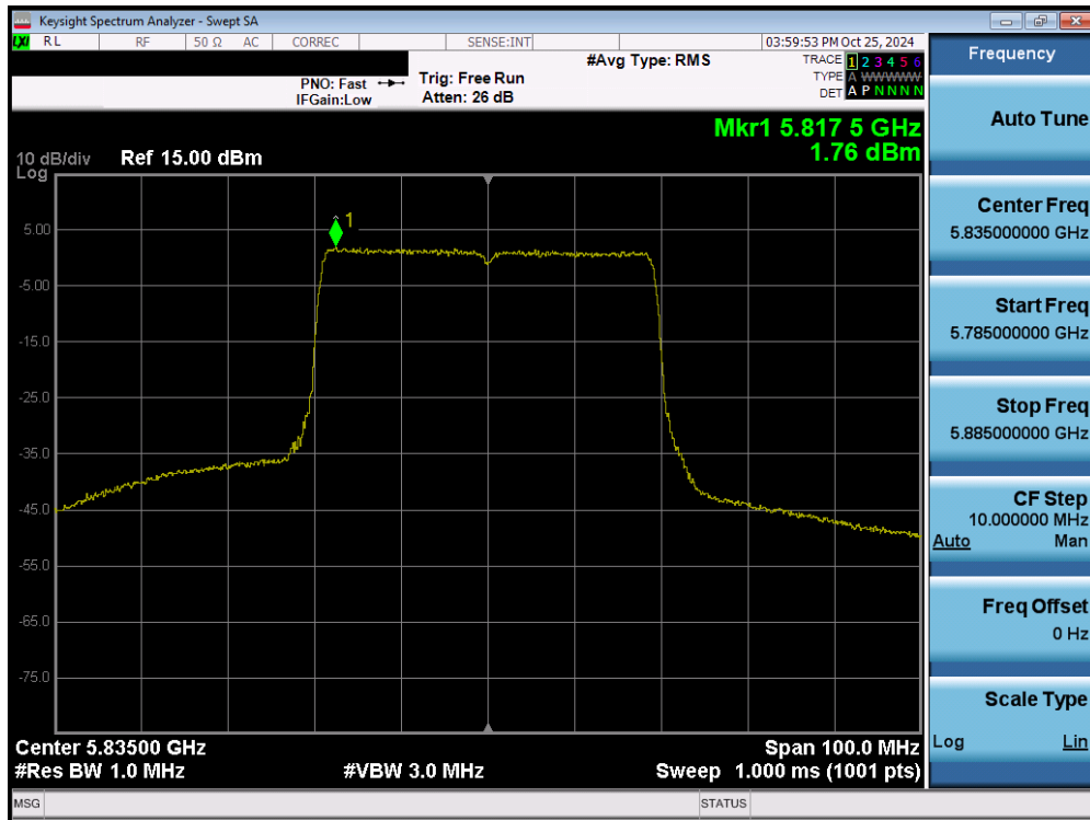
Plot 7-115. Power Spectral Density Plot MIMO ANT2 (40MHz 802.11ax/be (UNII Band 3/4) – Ch. 167)
