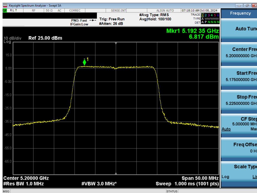
Plot 7-94. Power Spectral Density Plot MIMO ANT2 (20MHz 802.11ax/be (UNII Band 1) – Ch. 40)
