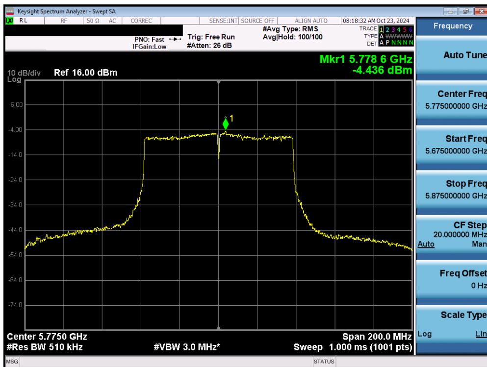
Plot 7-78. Power Spectral Density Plot MIMO ANT1 (80MHz 802.11ac (UNII Band 3) – Ch. 155)
