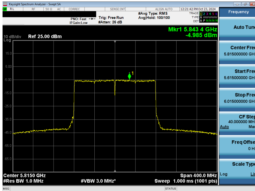
Plot 7-119. Power Spectral Density Plot MIMO ANT2 (160MHz 802.11ax/be (UNII Band 3/4) – Ch. 163)
