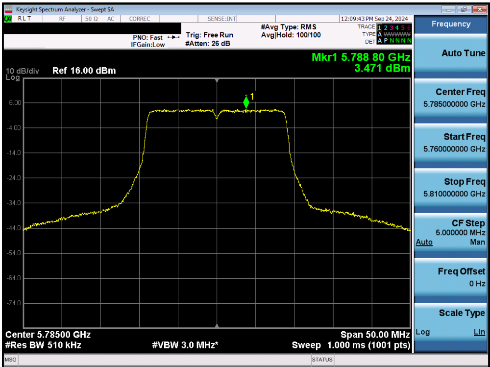
Plot 7-104. Power Spectral Density Plot MIMO ANT2 (20MHz 802.11n (UNII Band 3) – Ch.157)
