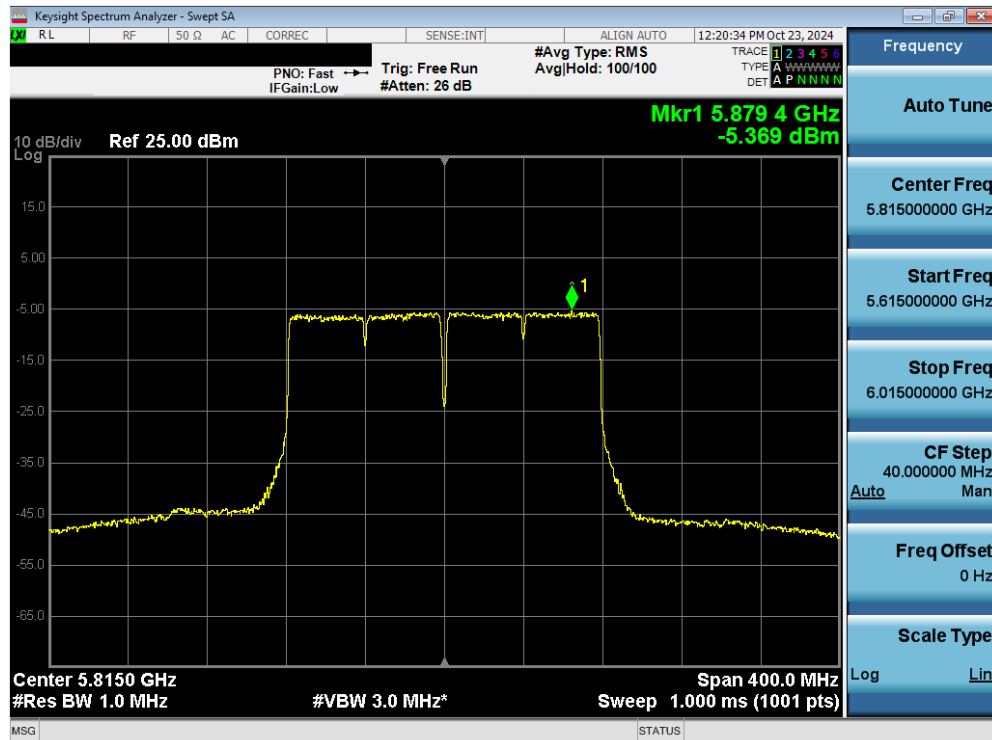
Plot 7-118. Power Spectral Density Plot MIMO ANT2 (160MHz 802.11ac (UNII Band 3/4) – Ch. 163)
