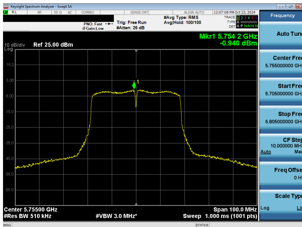
Plot 7-106. Power Spectral Density Plot MIMO ANT2 (40MHz 802.11n (UNII Band 3) – Ch. 151)
