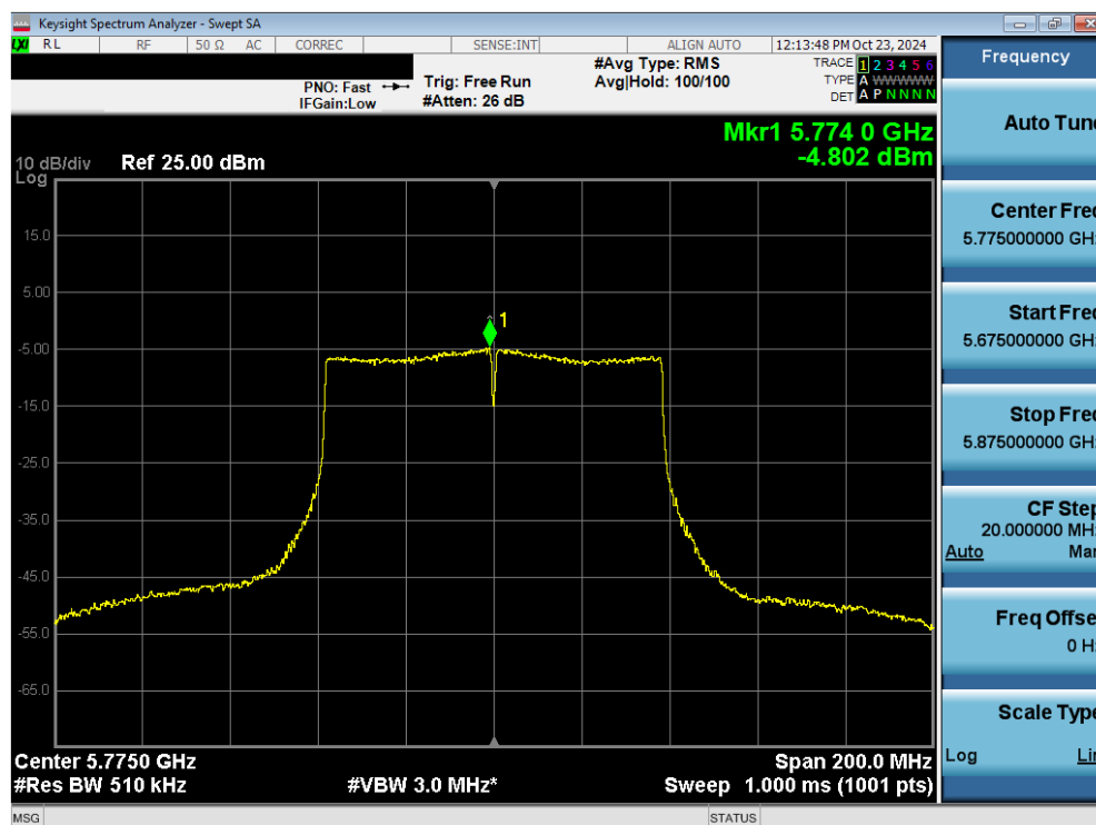
Plot 7-108. Power Spectral Density Plot MIMO ANT2 (80MHz 802.11ac (UNII Band 3) – Ch. 155)
