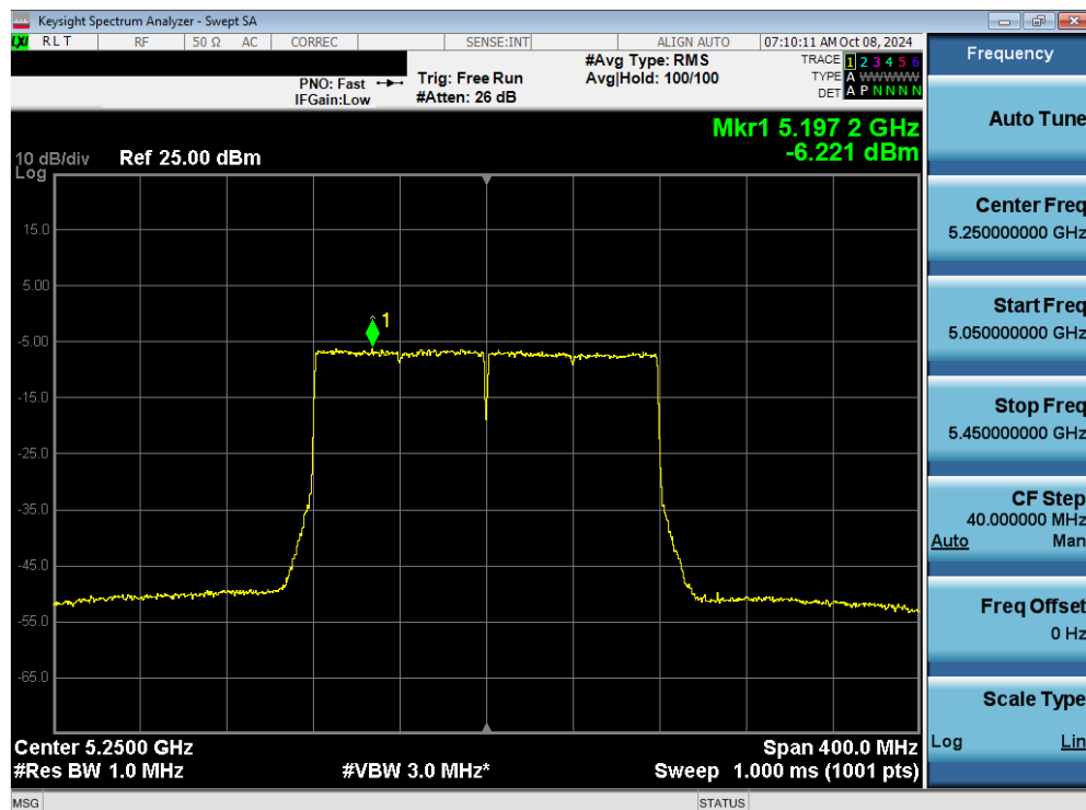
Plot 7-99. Power Spectral Density Plot MIMO ANT2 (160MHz 802.11ac (UNII Band 1/2A) – Ch. 50)
