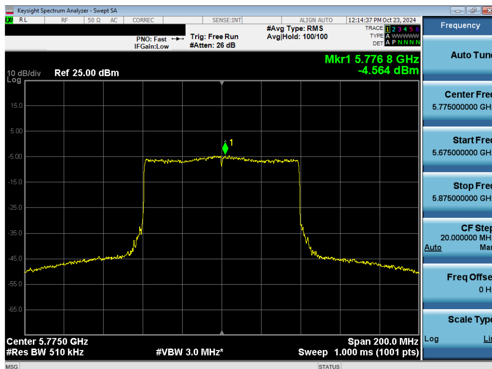
Plot 7-109. Power Spectral Density Plot MIMO ANT2 (80MHz 802.11ax/be (UNII Band 3) – Ch. 155)
