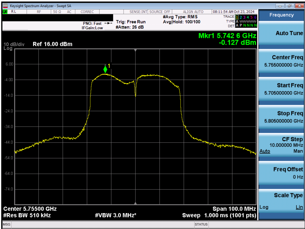
Plot 7-76. Power Spectral Density Plot MIMO ANT1 (40MHz 802.11n (UNII Band 3) – Ch. 151)
