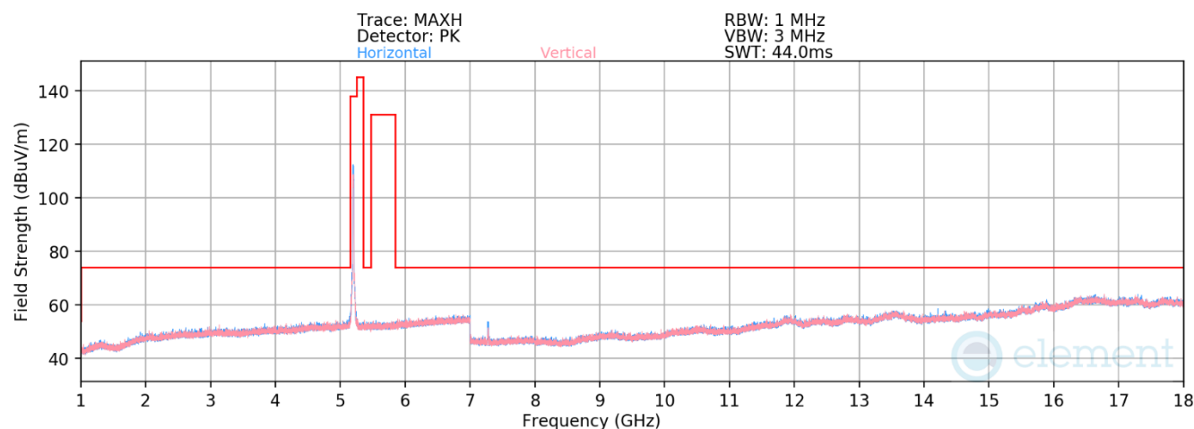
Plot 7-123. Radiated Spurious Plot above 1GHz MIMO (802.11ax – UNII Band 1 Ch. 40)
