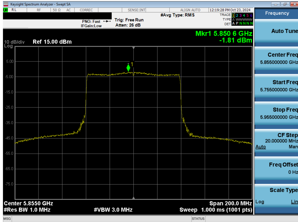
Plot 7-117. Power Spectral Density Plot MIMO ANT2 (80MHz 802.11ax/be (UNII Band 3/4) – Ch. 171)
