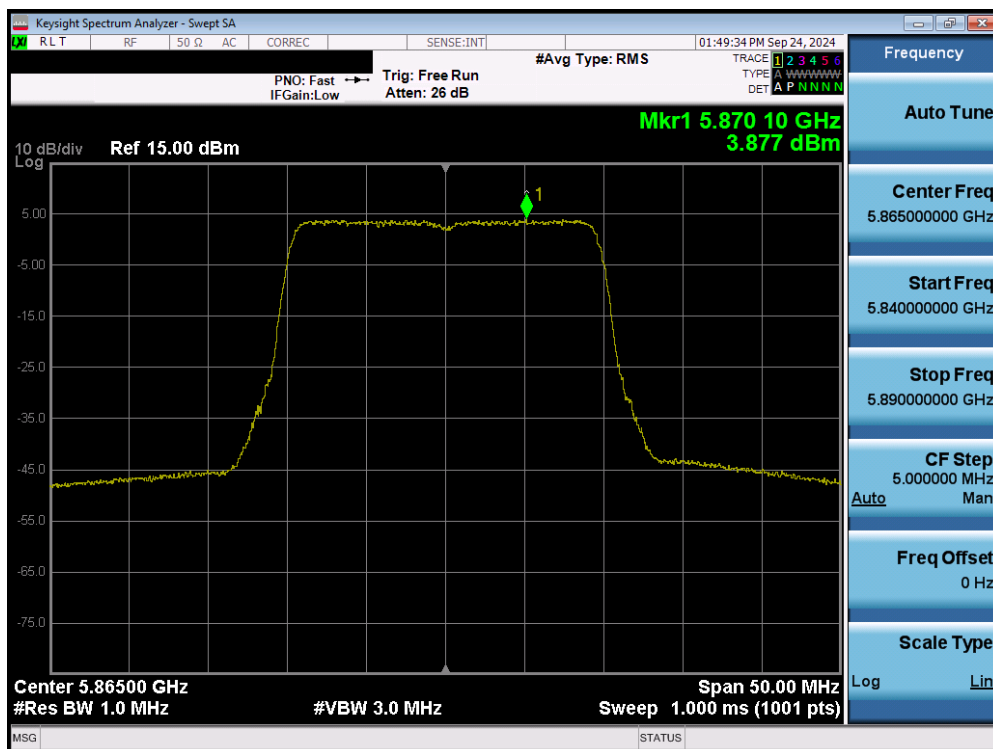
Plot 7-113. Power Spectral Density Plot MIMO ANT2 (20MHz 802.11ax/be (UNII Band 4) – Ch.173)
