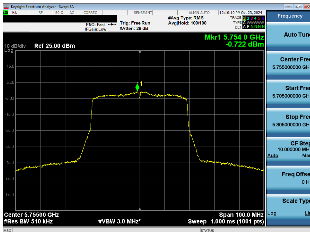
Plot 7-107. Power Spectral Density Plot MIMO ANT2 (40MHz 802.11ax/be (UNII Band 3) – Ch. 151)
