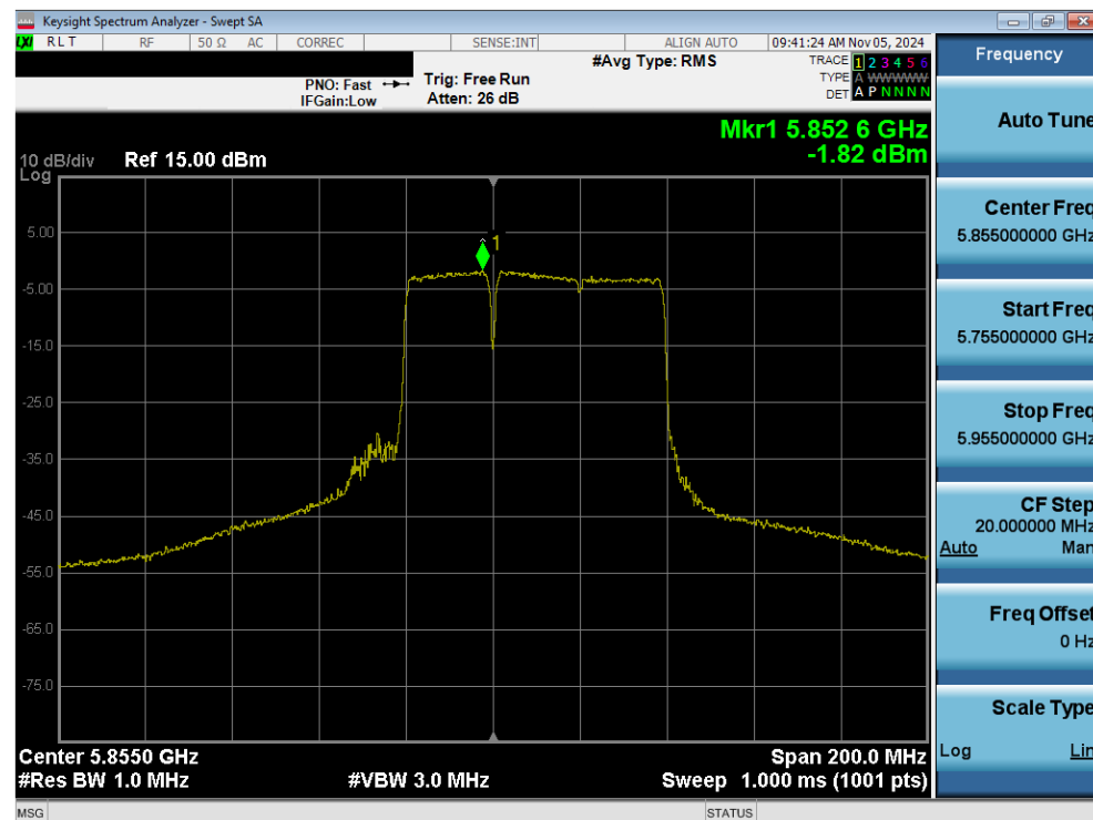
Plot 7-120. Power Spectral Density Plot MIMO ANT2 (80MHz 802.11be (20MHz Puncture) (UNII Band 3/4) – Ch. 171)
