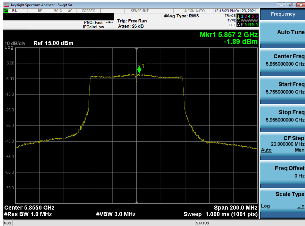
Plot 7-116. Power Spectral Density Plot MIMO ANT2 (80MHz 802.11ac (UNII Band 3/4) – Ch. 171)
