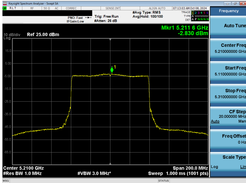
Plot 7-98. Power Spectral Density Plot MIMO ANT2 (80MHz 802.11ax/be (UNII Band 1) – Ch. 42)
