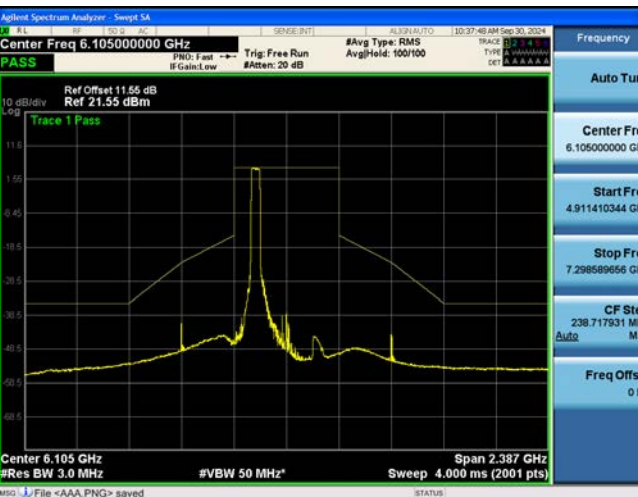
Bandwidth 320M, Ch. 31(6105 MHz) 484 Tones 65 RU
