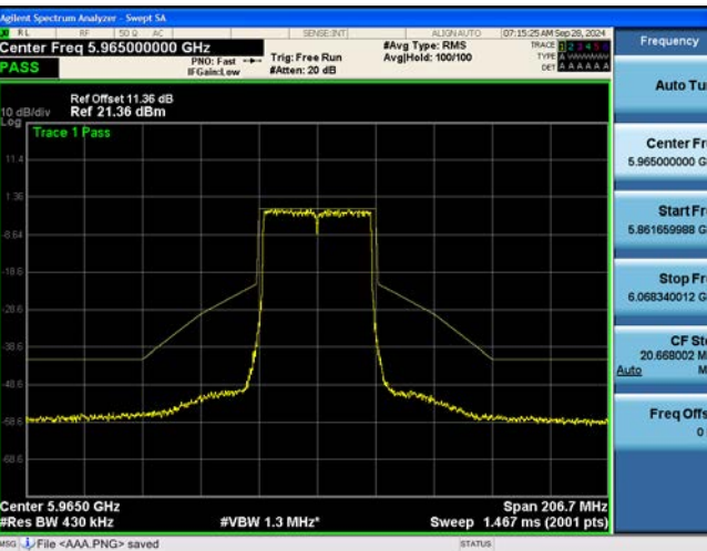
802.11be EHT40M Ch.3(5965 MHz) 484 Tones 65 RU
