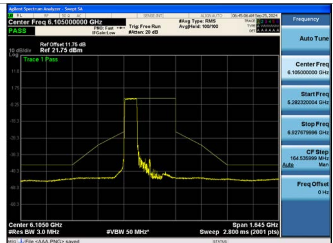
Bandwidth 320M, Ch. 31(6105 MHz) 996 Tones 67 RU
