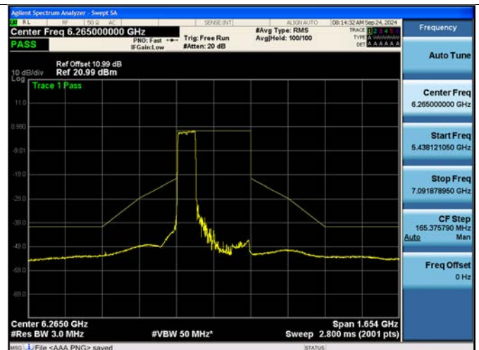
Bandwidth 320M, Ch. 63(6265 MHz) 996 Tones 67 RU
