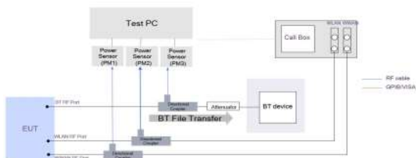
7-1(f) System level compliance
