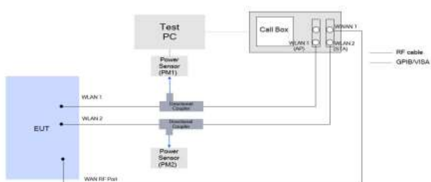
7-1(e) WLAN DBS
