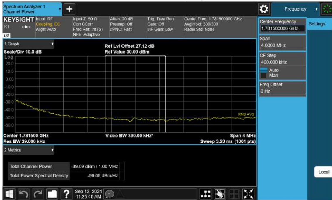
NR66_10 M_Extended Band Edge_High_BPSK_FullIRB
