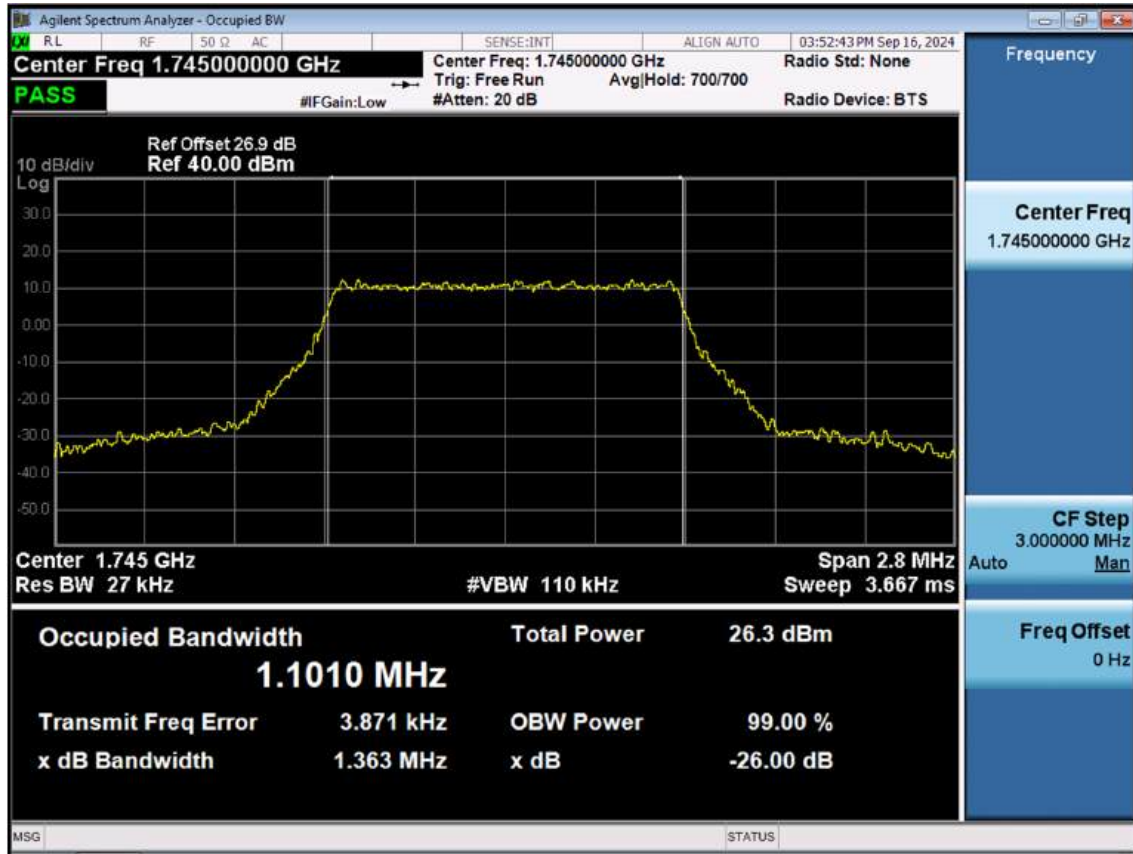
LTE B66_1.4M_OBW_Mid_256QAM_FullRB
