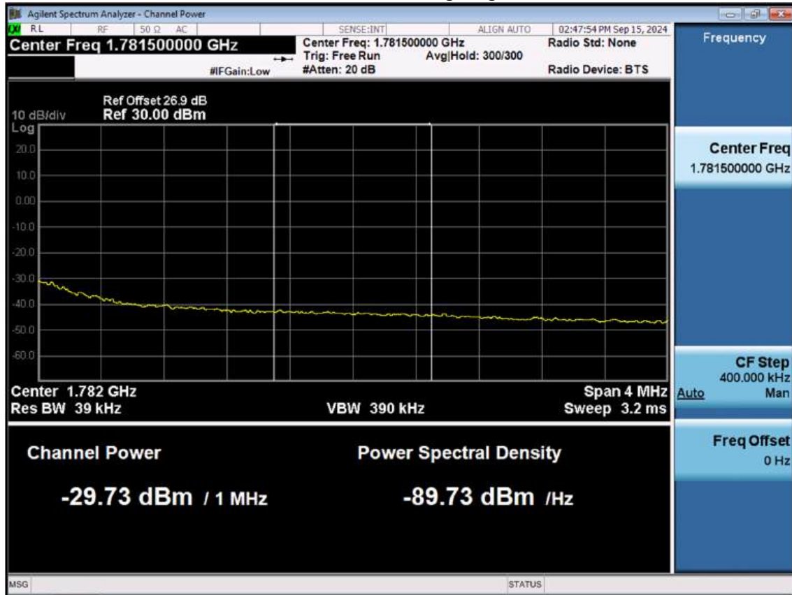
LTE B66_15 M_Extended Band Edge_High_QPSK_FullRB
