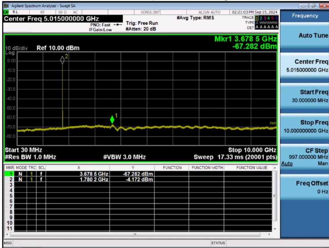
LTE B66_1.4M_Conducted Spurious(30 M-10 G)_High_QPSK_1RB
