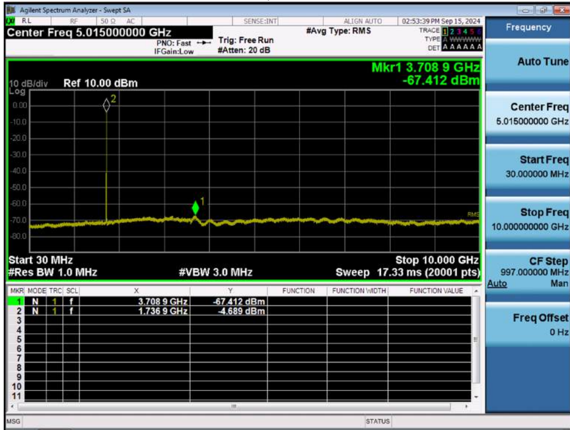
LTE B66_20 M_Conducted Spurious(30 M-10 G)_Mid_QPSK_1RB
