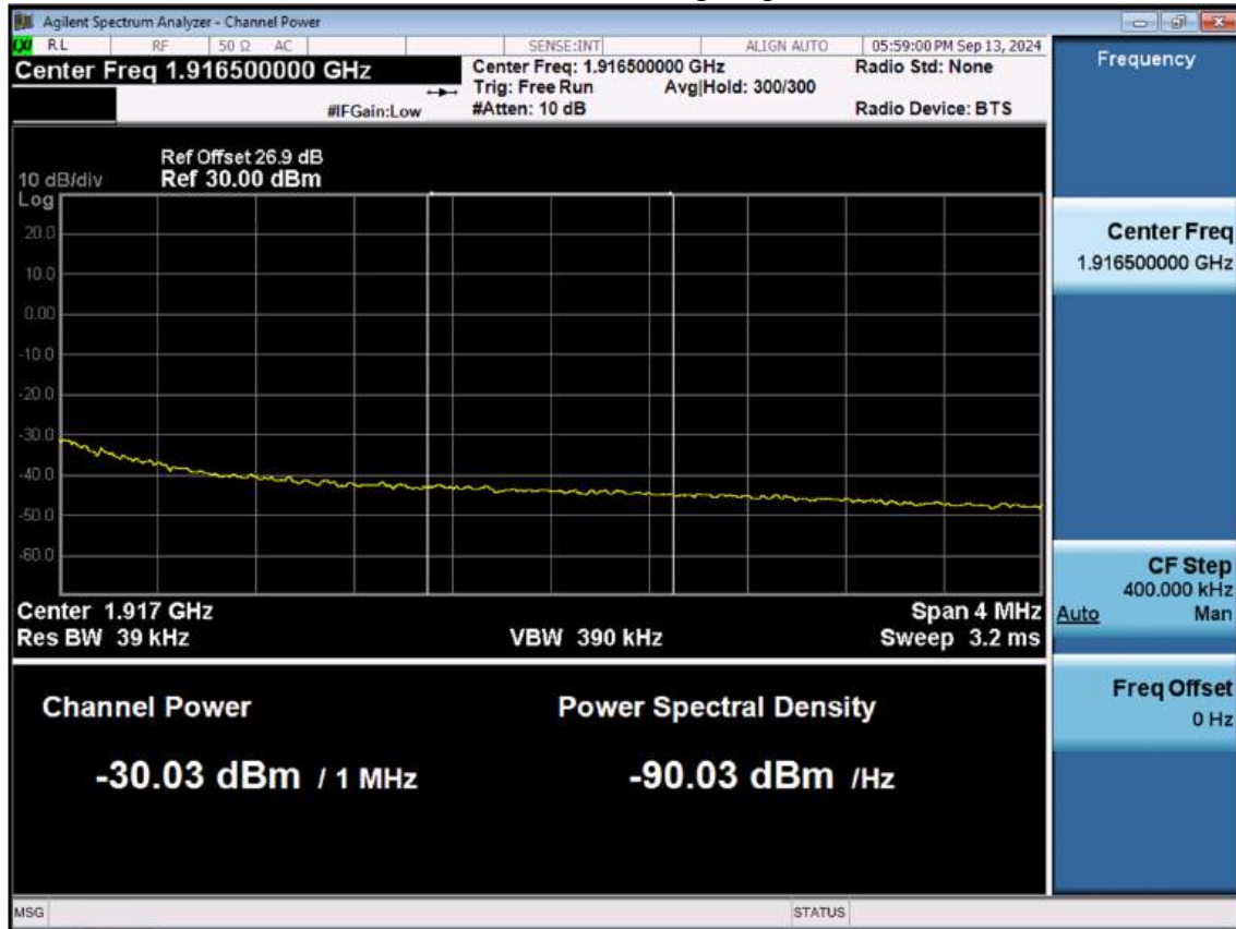
LTE B25_15 M_Extended Band Edge_High_QPSK_FullRB
