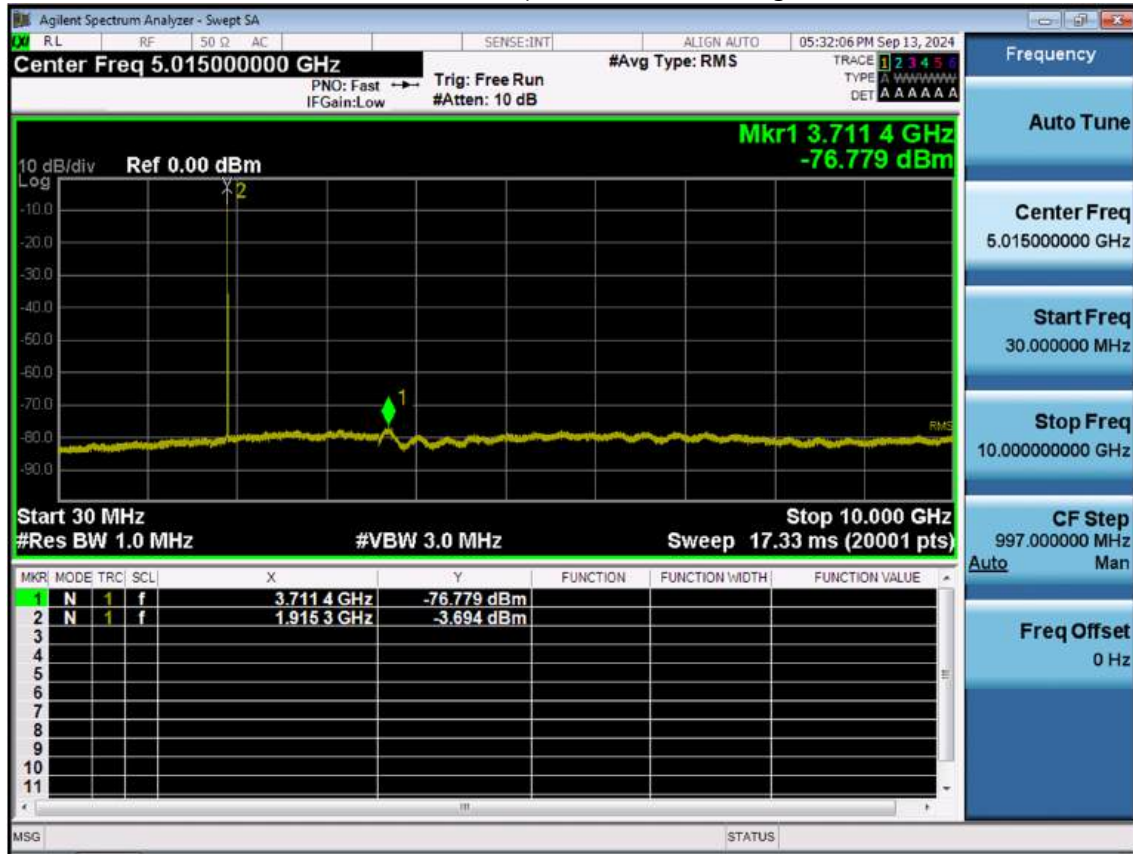
LTE B25_1.4M_Conducted Spurious(30 M-10 G)_High_QPSK_1RB
