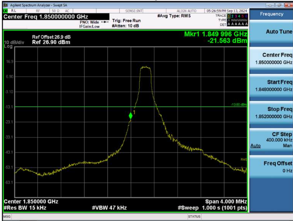
LTE B25_1.4M_Band Edge_Low_QPSK_1RB
