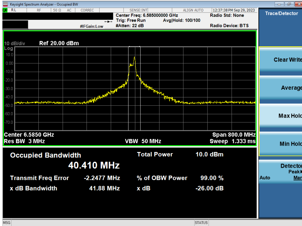
Plot 7-55. Occupied Bandwidth Plot MIMO ANT2 (320MHz BW 802.11ax/be (26 Tones) (UNII Band 6/7) – Ch. 127)
