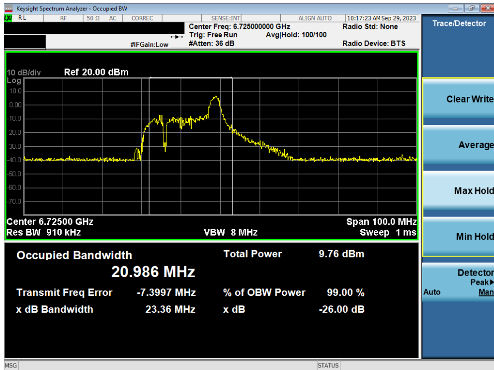
Plot 7-52. Occupied Bandwidth Plot MIMO ANT2 (40MHz BW 802.11ax/be (26 Tones) (UNII Band 7) – Ch. 155)
