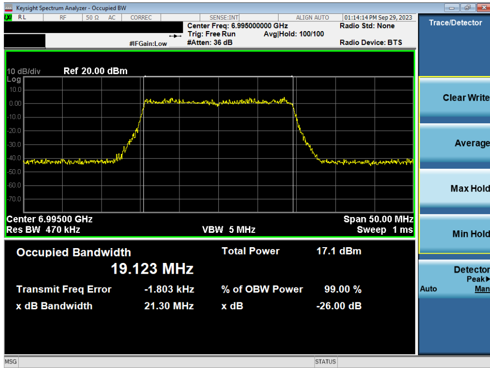
Plot 7-76. Occupied Bandwidth Plot MIMO ANT2 (20MHz BW 802.11ax/be (Full Tone) (UNII Band 8) – Ch. 209)
