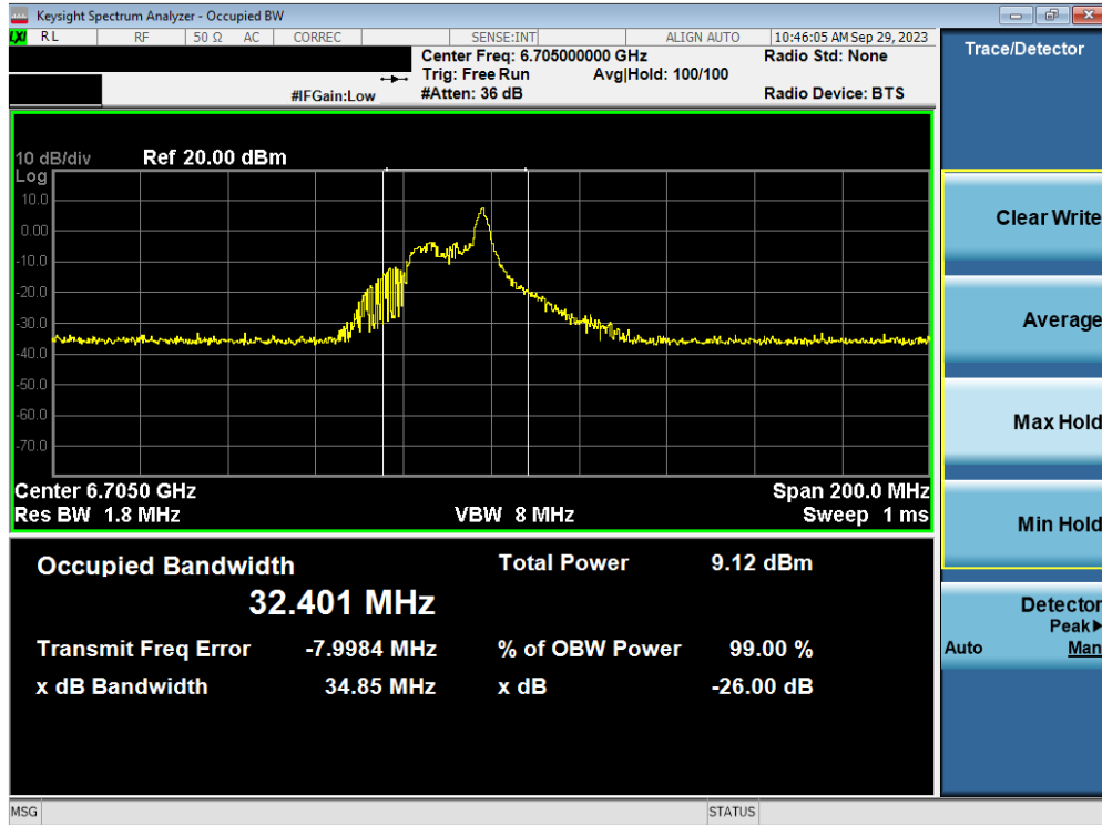
Plot 7-53. Occupied Bandwidth Plot MIMO ANT2 (80MHz BW 802.11ax/be (26 Tones) (UNII Band 7) – Ch. 151)
