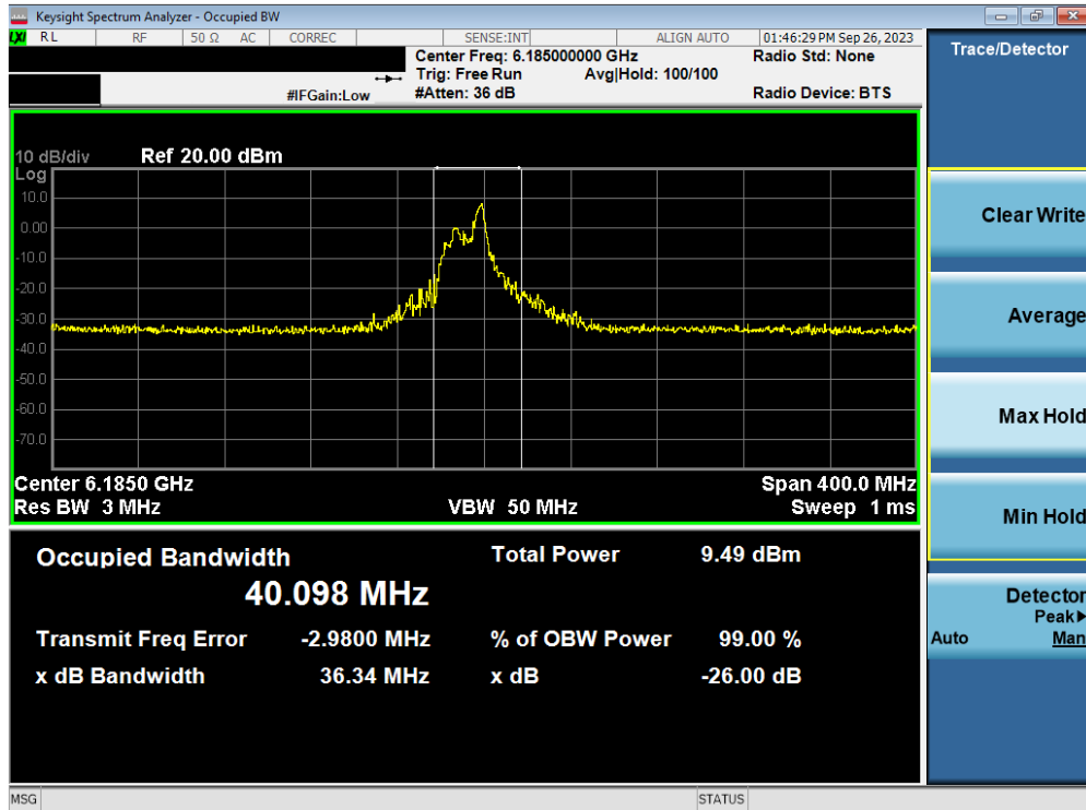
Plot 7-44. Occupied Bandwidth Plot MIMO ANT2 (160MHz BW 802.11ax/be (26 Tones) (UNII Band 5) – Ch. 47)
