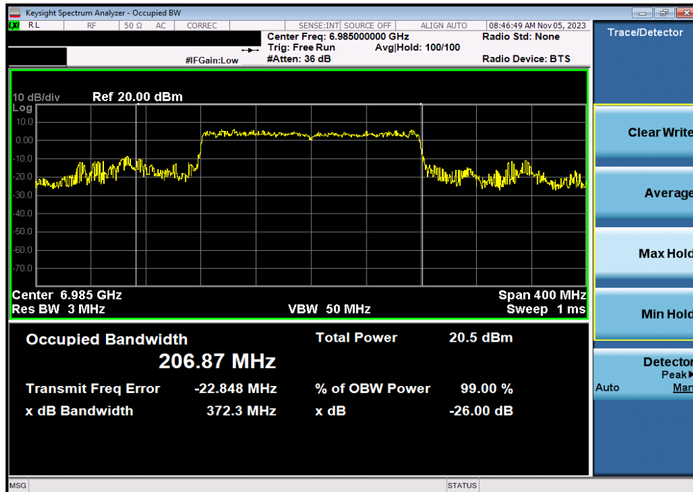
Plot 7-39. Occupied Bandwidth Plot MIMO ANT1 (160MHz BW 802.11ax/be (Full Tone) (UNII Band 8) – Ch. 207)
