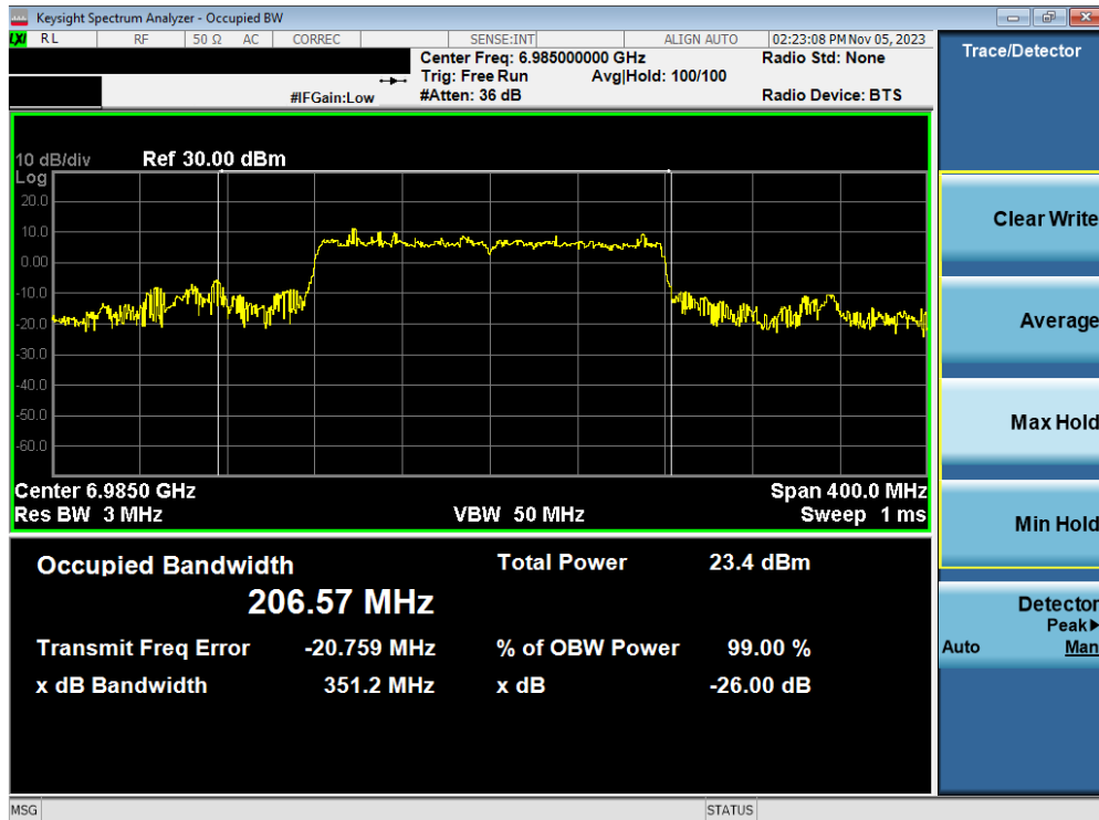
Plot 7-79. Occupied Bandwidth Plot MIMO ANT2 (160MHz BW 802.11ax/be (Full Tone) (UNII Band 8) – Ch. 207)
