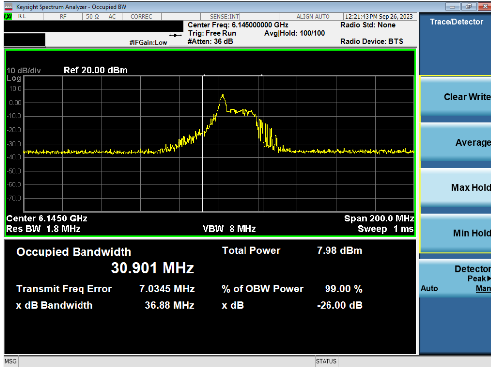
Plot 7-43. Occupied Bandwidth Plot MIMO ANT2 (80MHz BW 802.11ax/be (26 Tones) (UNII Band 5) – Ch. 39)
