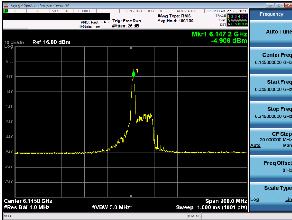
Plot 7-85. Power Spectral Density Plot MIMO ANT1 (80MHz BW 802.11ax/be (26 Tones) (UNII Band 5) – Ch. 39) – LPI
