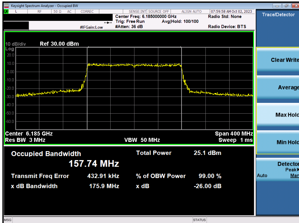
Plot 7-24. Occupied Bandwidth Plot MIMO ANT1 (160MHz BW 802.11ax/be (Full Tone) (UNII Band 5) – Ch. 47)
