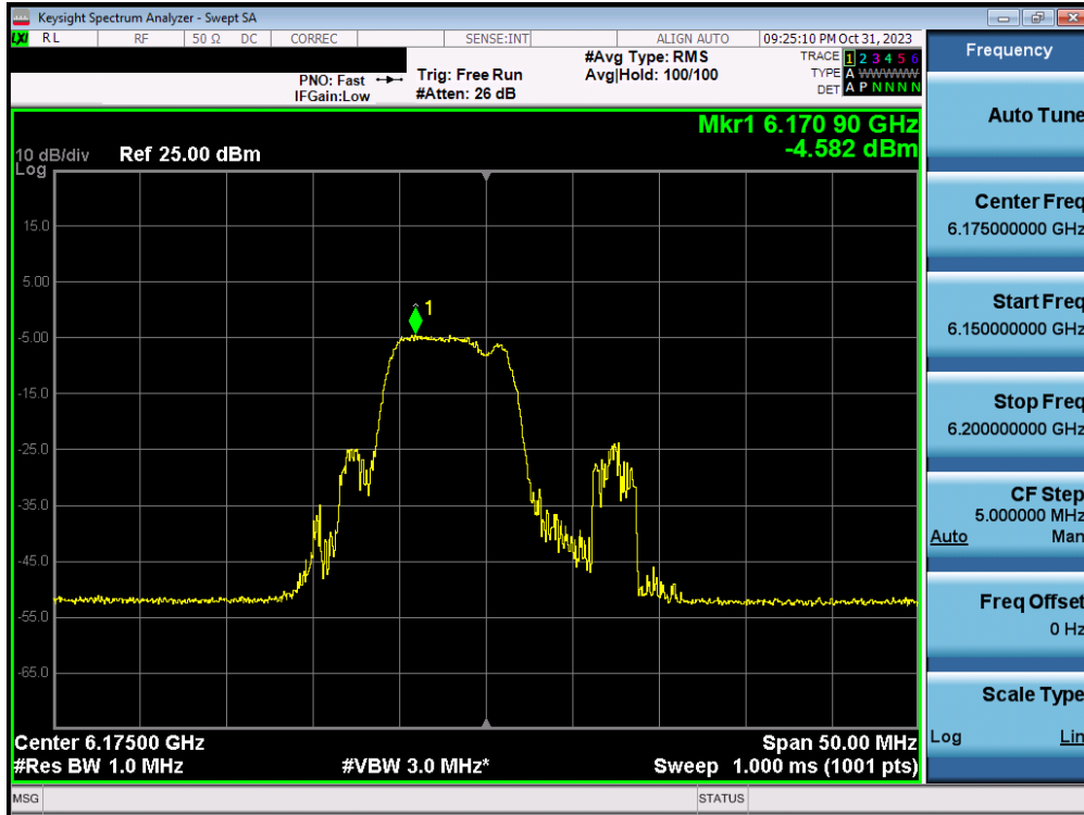
Plot 7-83. Power Spectral Density Plot MIMO ANT1 (20MHz BW 802.11ax/be (MRU) (UNII Band 5) – Ch. 45) – LPI – 52+26T
