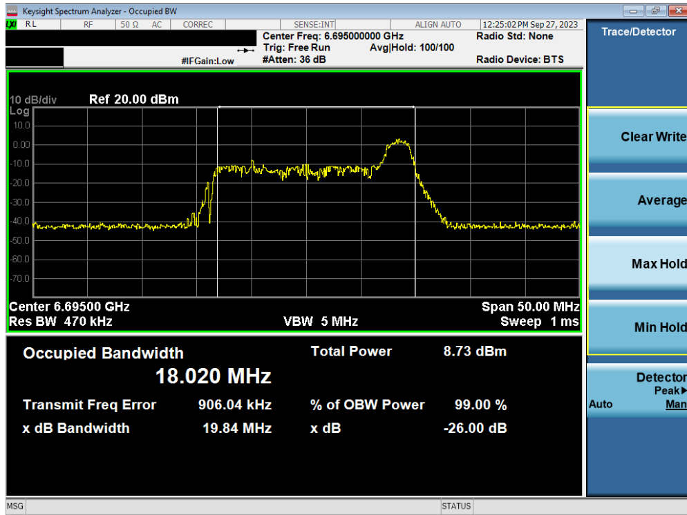
Plot 7-51. Occupied Bandwidth Plot MIMO ANT2 (20MHz BW 802.11ax/be (26 Tones) (UNII Band 7) – Ch. 149)
