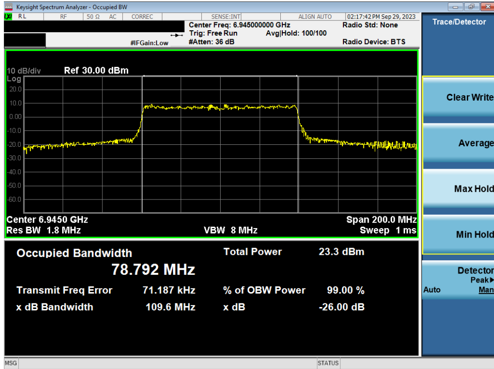
Plot 7-78. Occupied Bandwidth Plot MIMO ANT2 (80MHz BW 802.11ax/be (Full Tone) (UNII Band 8) – Ch. 199)
