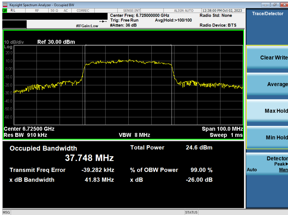
Plot 7-72. Occupied Bandwidth Plot MIMO ANT2 (40MHz BW 802.11ax/be (Full Tone) (UNII Band 7) – Ch. 155)
