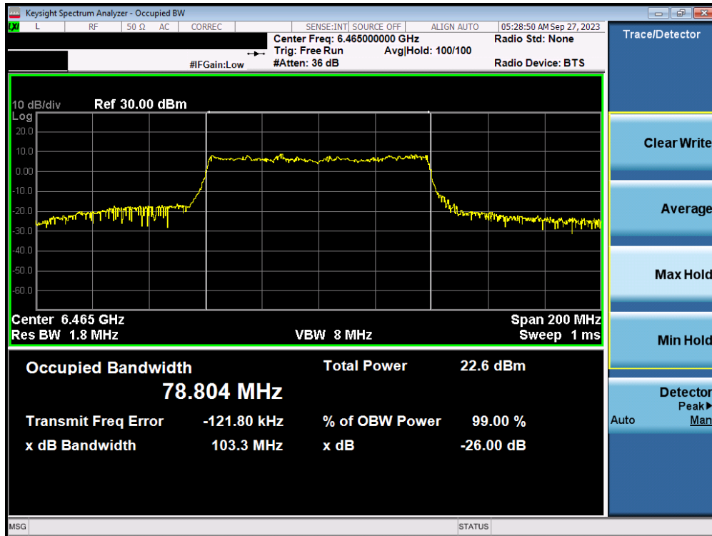
Plot 7-28. Occupied Bandwidth Plot MIMO ANT1 (80MHz BW 802.11ax/be (Full Tone) (UNII Band 6) – Ch. 103)
