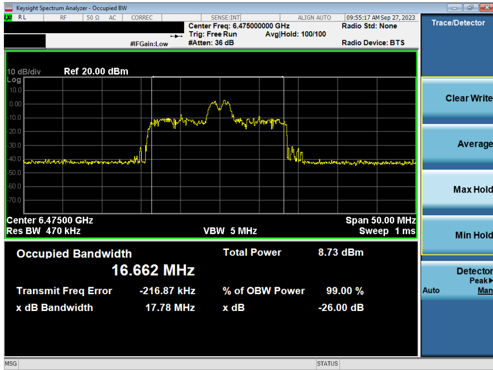
Plot 7-46. Occupied Bandwidth Plot MIMO ANT2 (20MHz BW 802.11ax/be (26 Tones) (UNII Band 6) – Ch. 105)
