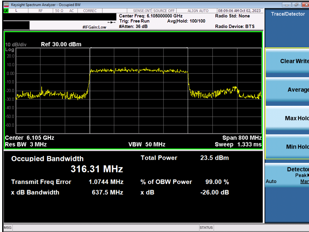
Plot 7-25. Occupied Bandwidth Plot MIMO ANT1 (320MHz BW 802.11ax/be (26 Tones) (UNII Band 5) – Ch. 31)
