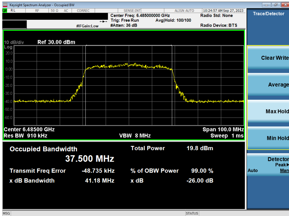
Plot 7-67. Occupied Bandwidth Plot MIMO ANT2 (40MHz BW 802.11ax/be (Full Tone) (UNII Band 6) – Ch. 107)
