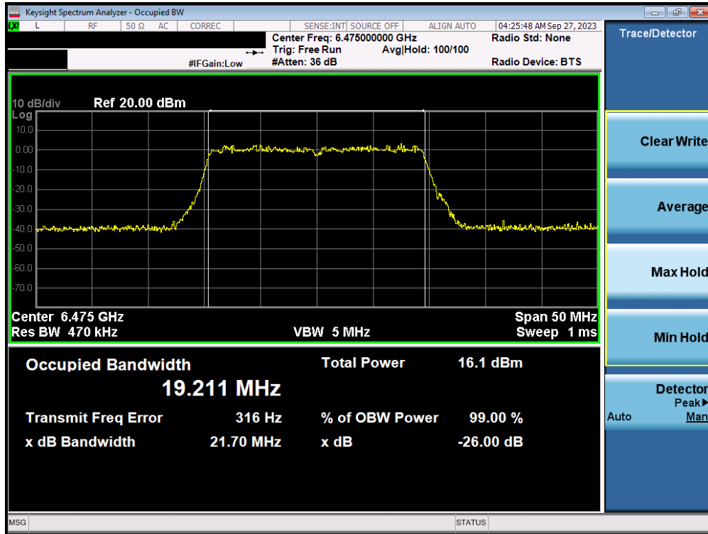
Plot 7-26. Occupied Bandwidth Plot MIMO ANT1 (20MHz BW 802.11ax/be (Full Tone) (UNII Band 6) – Ch. 105)
