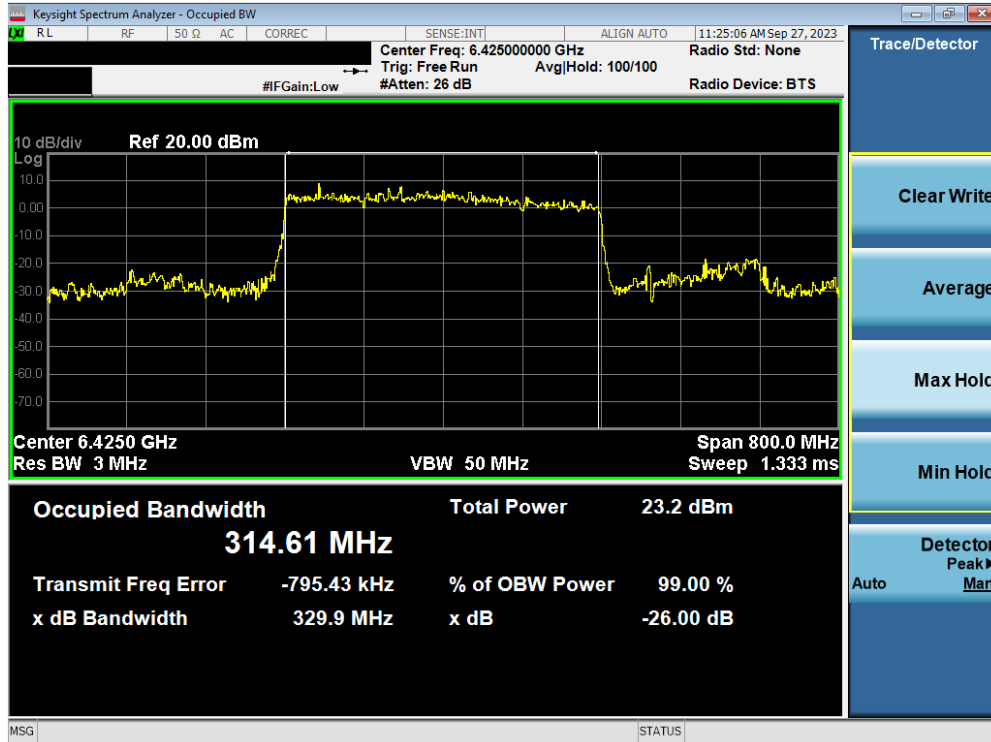
Plot 7-70. Occupied Bandwidth Plot MIMO ANT2 (320MHz BW 802.11ax/be (26 Tones) (UNII Band 5/6/7) – Ch. 95)
