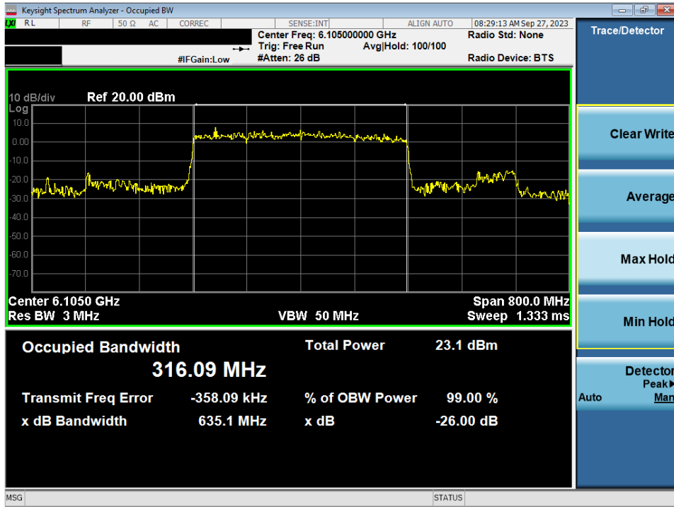
Plot 7-65. Occupied Bandwidth Plot MIMO ANT2 (320MHz BW 802.11ax/be (26 Tones) (UNII Band 5) – Ch. 31)
