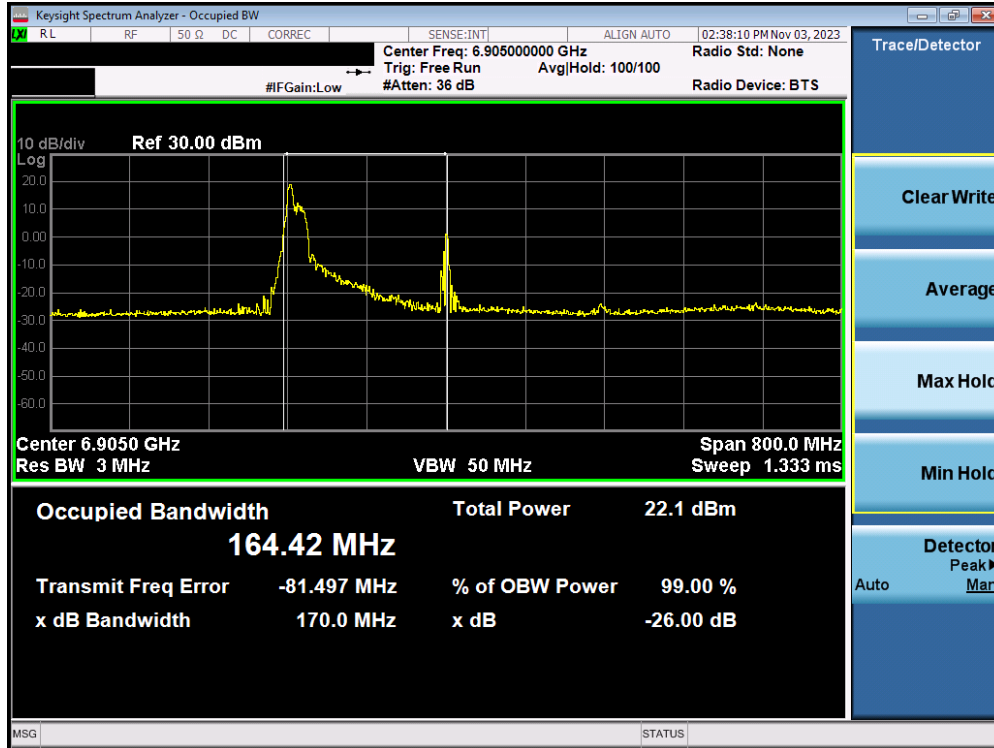
Plot 7-60. Occupied Bandwidth Plot MIMO ANT2 (320MHz BW 802.11ax/be (26 Tones) (UNII Band 7/8) – Ch. 191)
