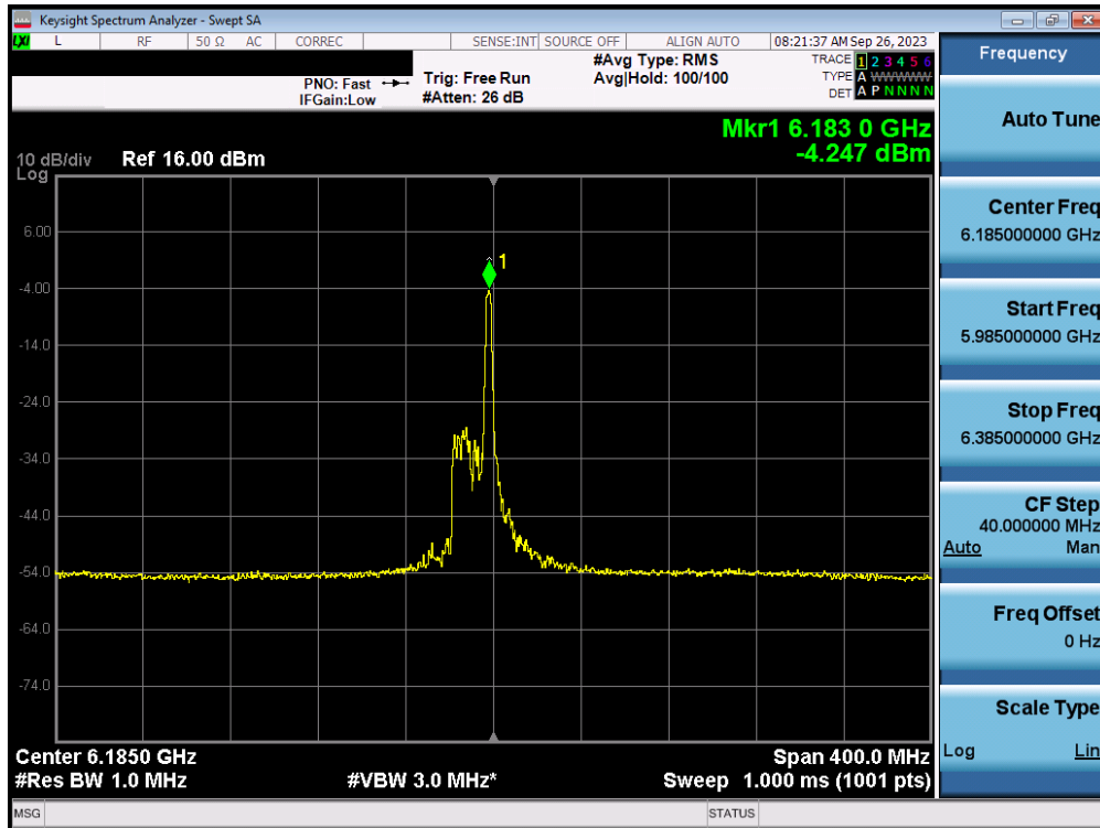
Plot 7-87. Power Spectral Density Plot MIMO ANT1 (160MHz BW 802.11ax/be (26 Tones) (UNII Band 5) – Ch. 47) – LPI
