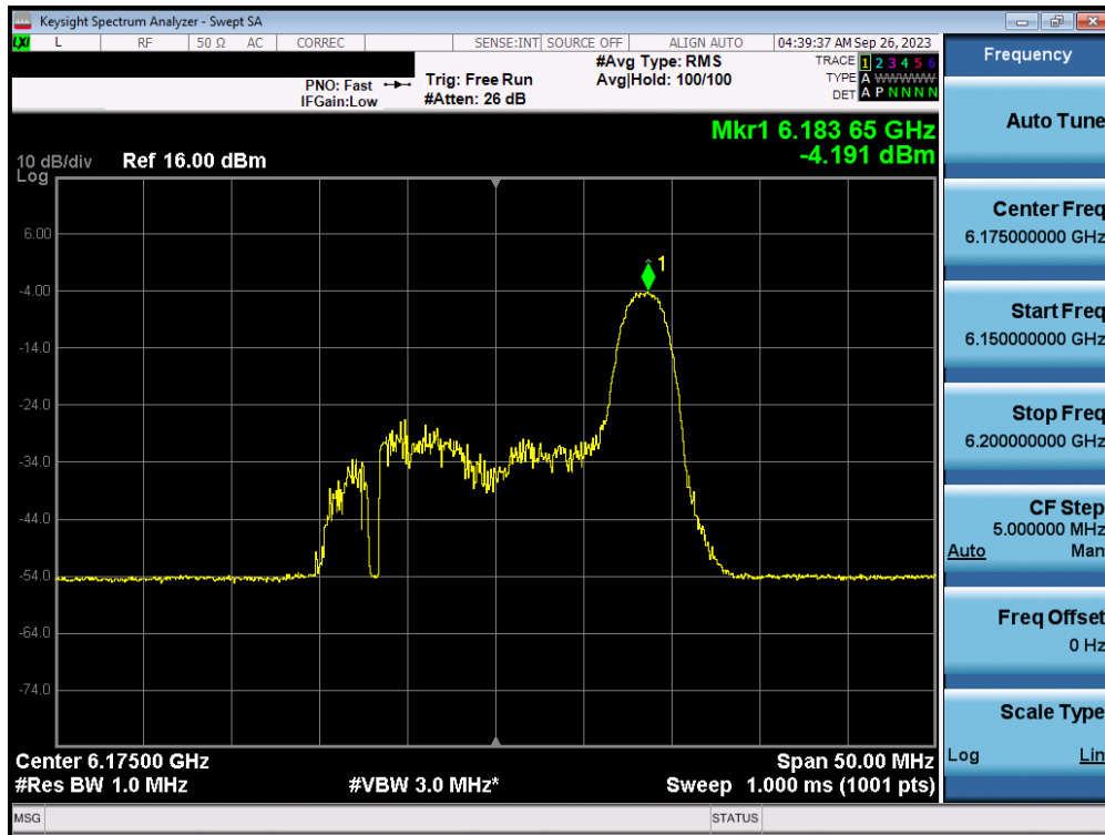
Plot 7-81. Power Spectral Density Plot MIMO ANT1 (20MHz BW 802.11ax/be (26 Tones) (UNII Band 5) – Ch. 45) – LPI
