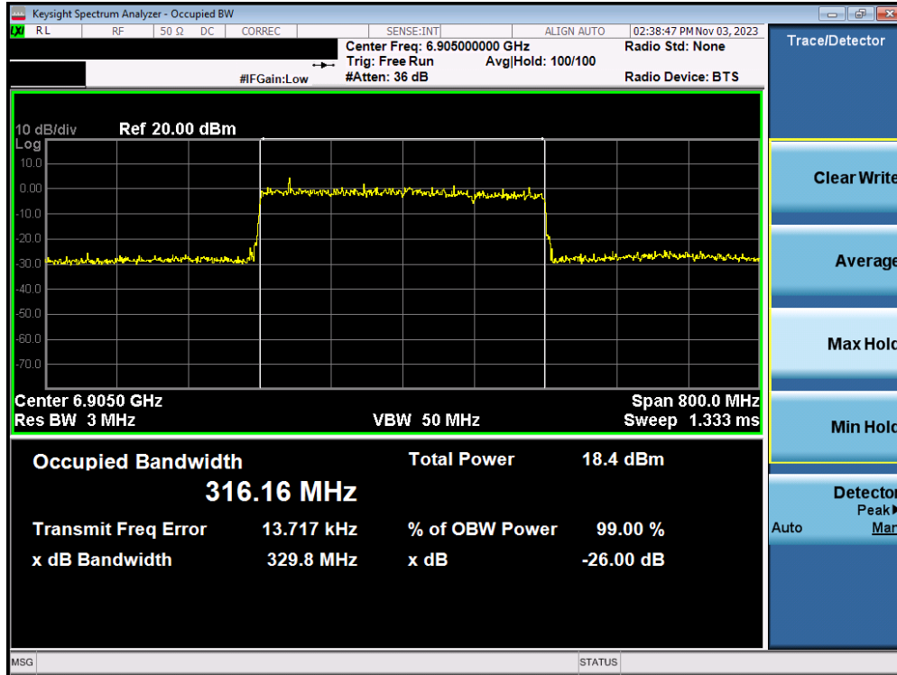
Plot 7-80. Occupied Bandwidth Plot MIMO ANT2 (320MHz BW 802.11ax/be (26 Tones) (UNII Band 8) – Ch. 191)
