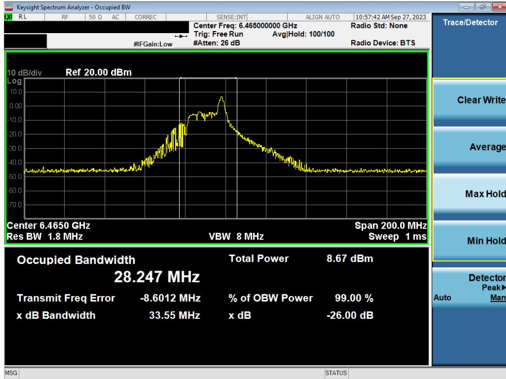
Plot 7-48. Occupied Bandwidth Plot MIMO ANT2 (80MHz BW 802.11ax/be (26 Tones) (UNII Band 6) – Ch. 103)
