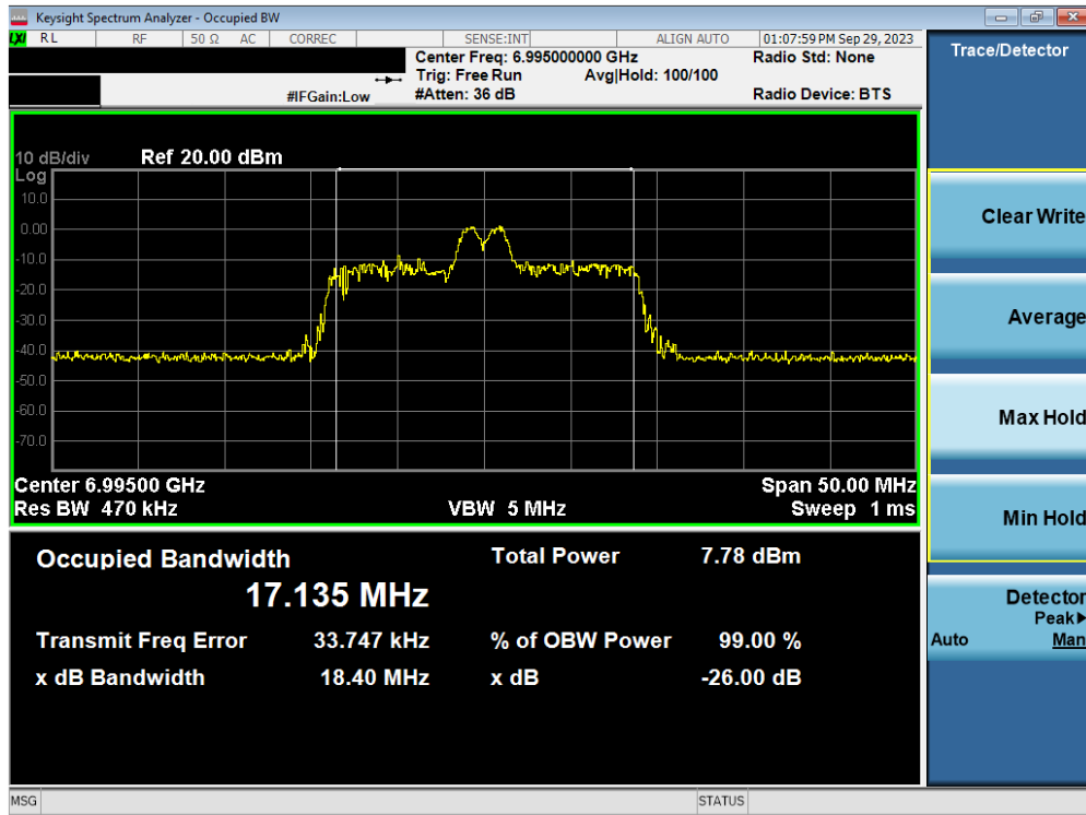
Plot 7-56. Occupied Bandwidth Plot MIMO ANT2 (20MHz BW 802.11ax/be (26 Tones) (UNII Band 8) – Ch. 209)
