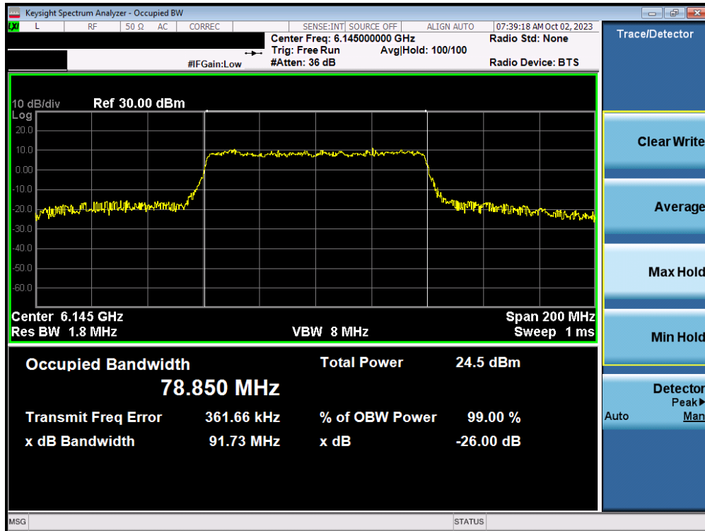
Plot 7-23. Occupied Bandwidth Plot MIMO ANT1 (80MHz BW 802.11ax/be (Full Tone) (UNII Band 5) – Ch. 39)
