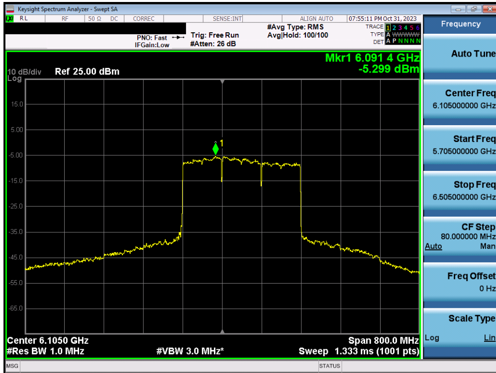
Plot 7-91. Power Spectral Density Plot MIMO ANT1 (320MHz BW 802.11ax/be (MRU) (UNII Band 5) – Ch. 31) – LPI – 3x996T
