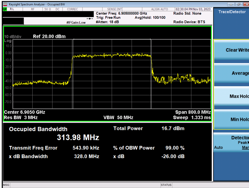
Plot 7-40. Occupied Bandwidth Plot MIMO ANT1 (320MHz BW 802.11ax/be (26 Tones) (UNII Band 8) – Ch. 191)
