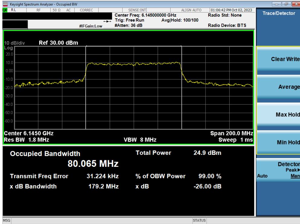
Plot 7-63. Occupied Bandwidth Plot MIMO ANT2 (80MHz BW 802.11ax/be (Full Tone) (UNII Band 5) – Ch. 39)
