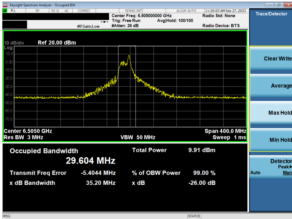
Plot 7-49. Occupied Bandwidth Plot MIMO ANT2 (160MHz BW 802.11ax/be (26 Tones) (UNII Band 6) – Ch. 111)
