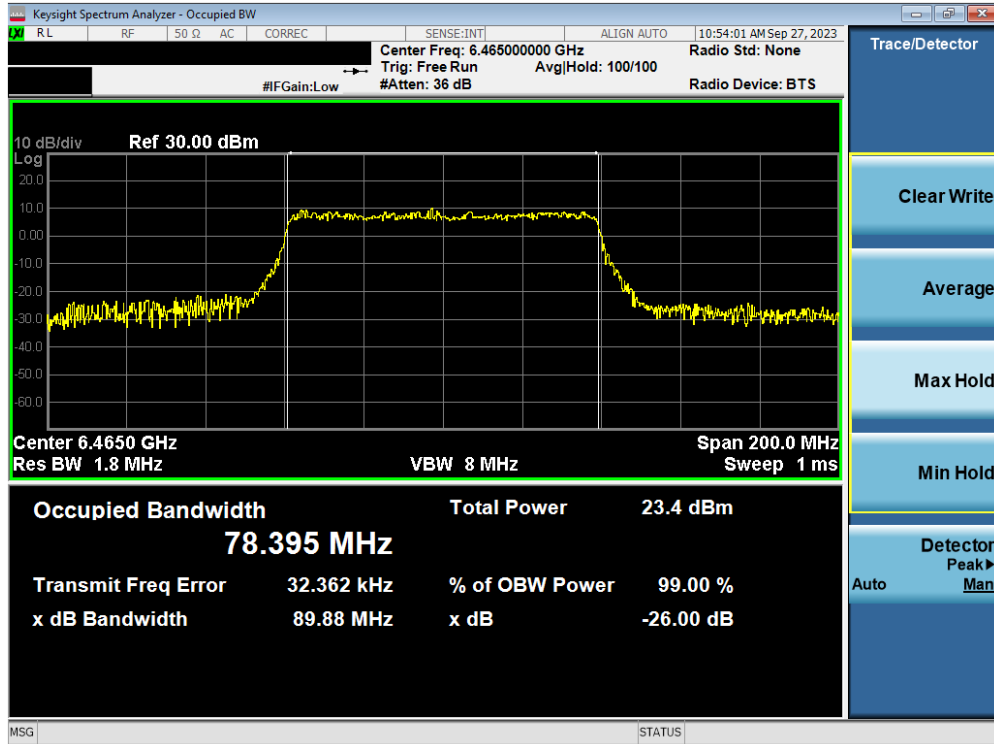
Plot 7-68. Occupied Bandwidth Plot MIMO ANT2 (80MHz BW 802.11ax/be (Full Tone) (UNII Band 6) – Ch. 103)
