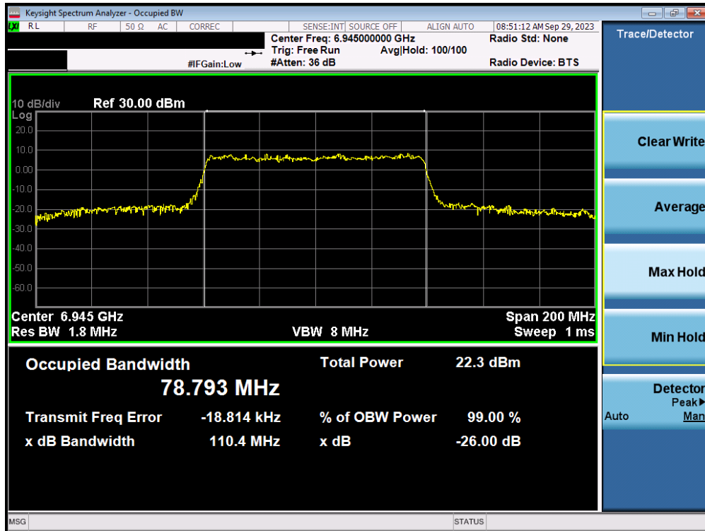
Plot 7-38. Occupied Bandwidth Plot MIMO ANT1 (80MHz BW 802.11ax/be (Full Tone) (UNII Band 8) – Ch. 199)
