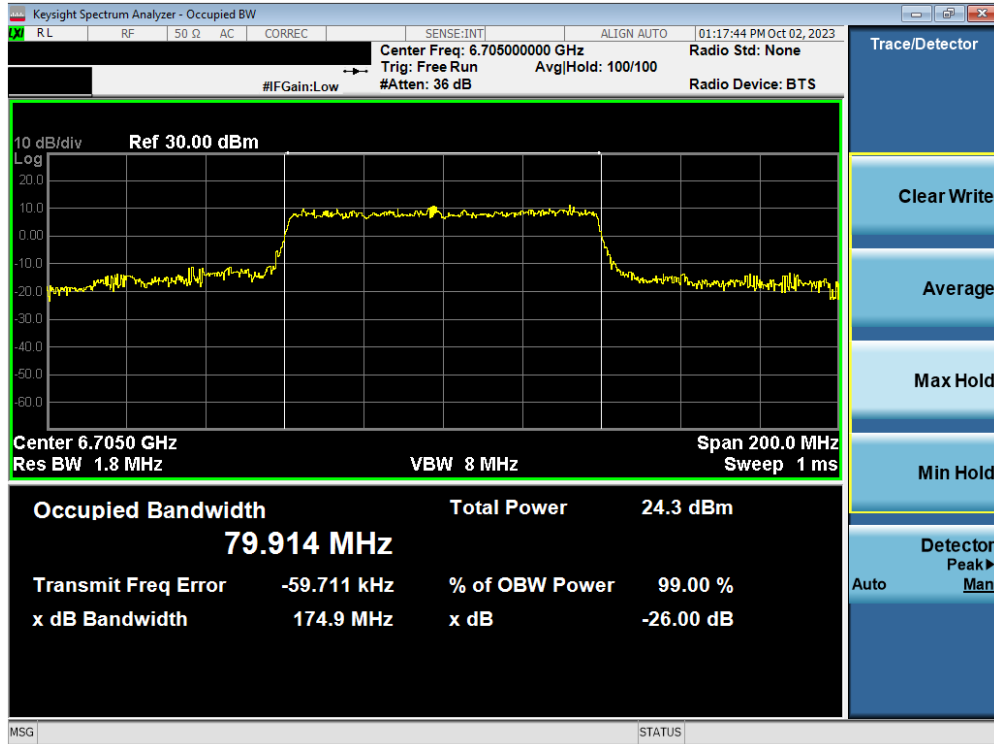
Plot 7-73. Occupied Bandwidth Plot MIMO ANT2 (80MHz BW 802.11ax/be (Full Tone) (UNII Band 7) – Ch. 151)
