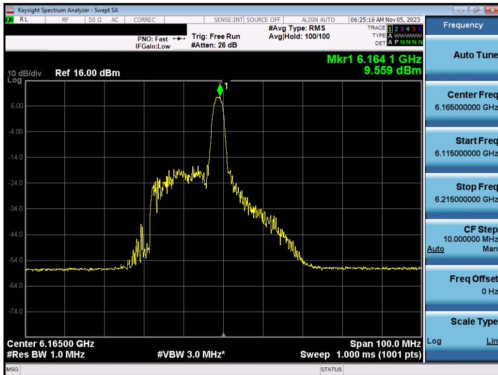
Plot 7-94. Power Spectral Density Plot MIMO ANT1 (40MHz BW 802.11ax/be (26 Tones) (UNII Band 5) – Ch. 43) – SP
