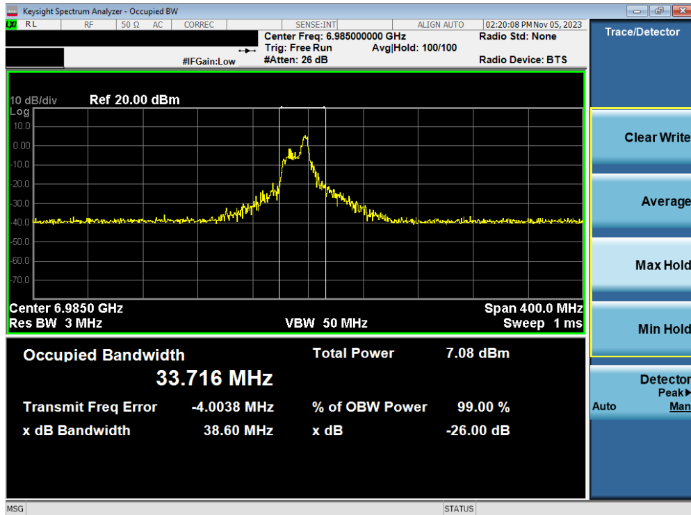
Plot 7-59. Occupied Bandwidth Plot MIMO ANT2 (160MHz BW 802.11ax/be (26 Tones) (UNII Band 8) – Ch. 207)
