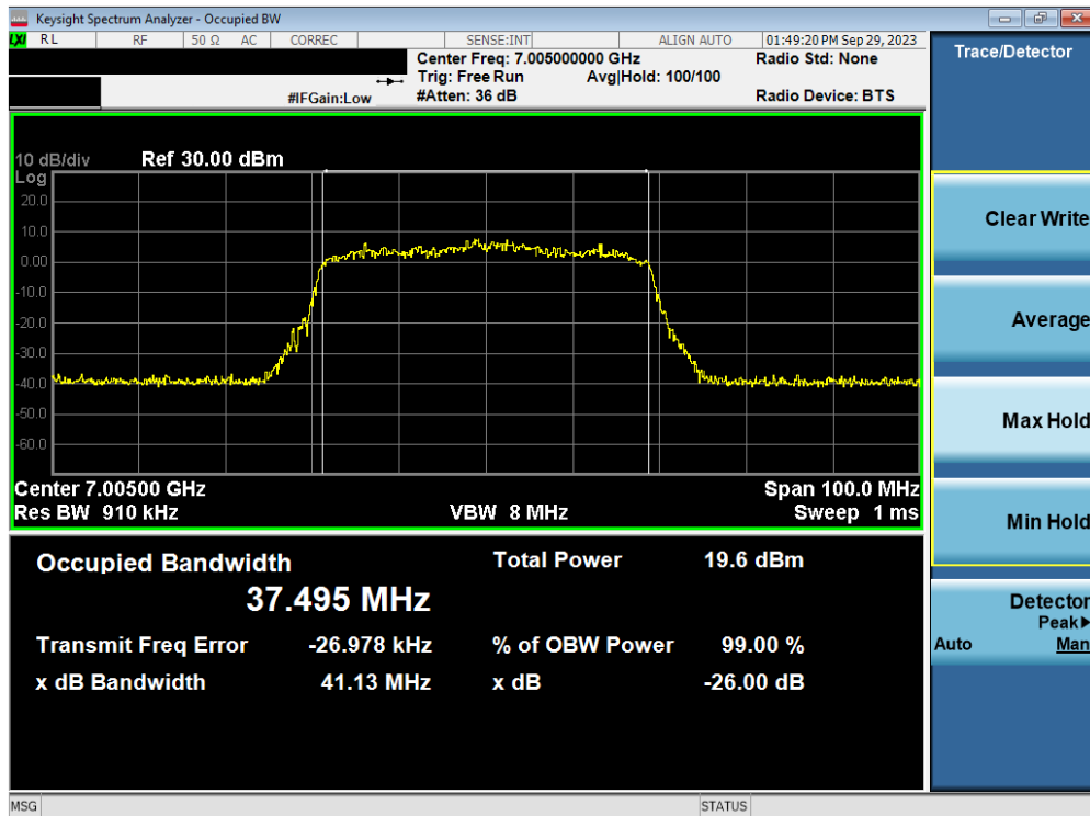
Plot 7-77. Occupied Bandwidth Plot MIMO ANT2 (40MHz BW 802.11ax/be (Full Tone) (UNII Band 8) – Ch. 211)
