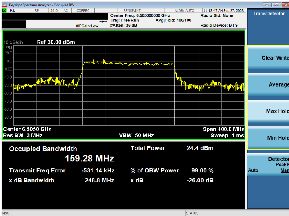
Plot 7-69. Occupied Bandwidth Plot MIMO ANT2 (160MHz BW 802.11ax/be (Full Tone) (UNII Band 6) – Ch. 111)
