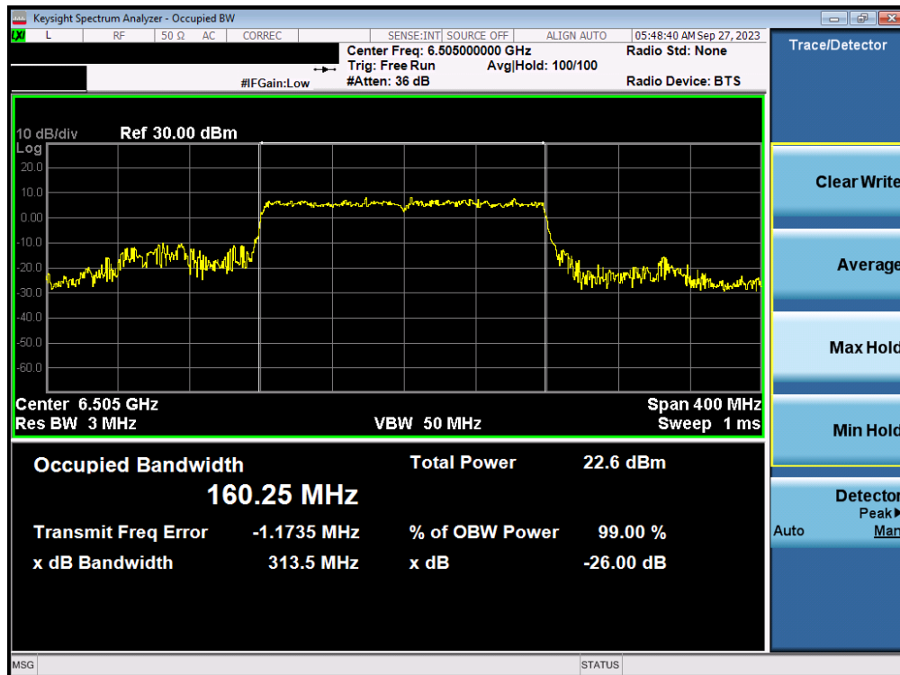
Plot 7-29. Occupied Bandwidth Plot MIMO ANT1 (160MHz BW 802.11ax/be (Full Tone) (UNII Band 6) – Ch. 111)
