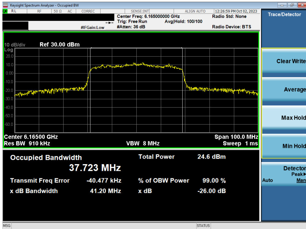
Plot 7-62. Occupied Bandwidth Plot MIMO ANT2 (40MHz BW 802.11ax/be (Full Tone) (UNII Band 5) – Ch. 43)
