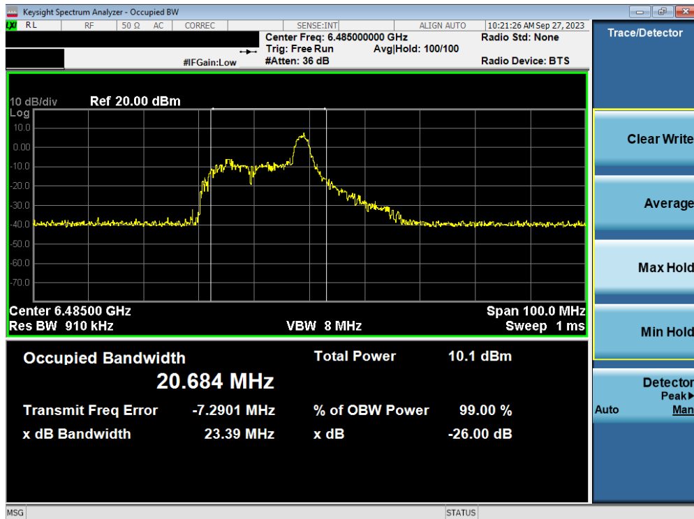
Plot 7-47. Occupied Bandwidth Plot MIMO ANT2 (40MHz BW 802.11ax/be (26 Tones) (UNII Band 6) – Ch. 107)
