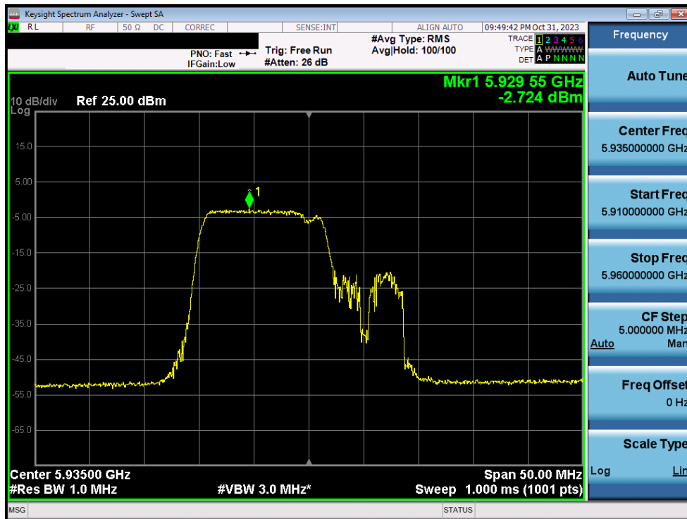
Plot 7-82. Power Spectral Density Plot MIMO ANT1 (20MHz BW 802.11ax/be (MRU) (UNII Band 5) – Ch. 2) – LPI – 106+26T
