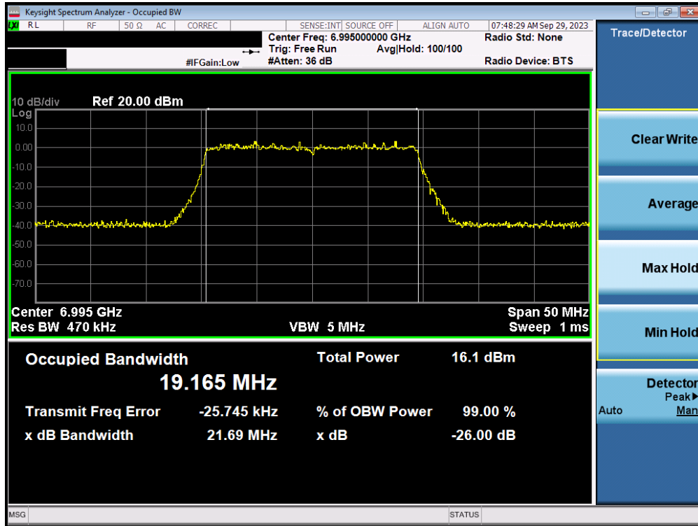
Plot 7-36. Occupied Bandwidth Plot MIMO ANT1 (20MHz BW 802.11ax/be (Full Tone) (UNII Band 8) – Ch. 209)
