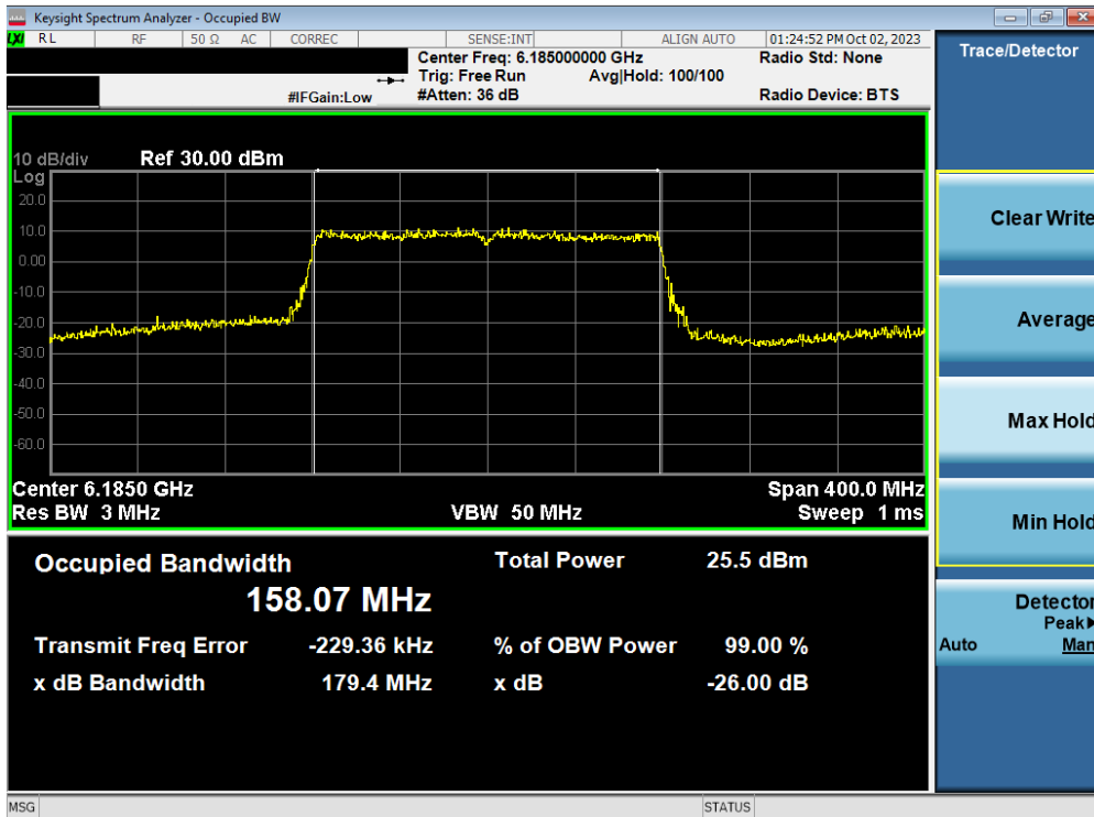
Plot 7-64. Occupied Bandwidth Plot MIMO ANT2 (160MHz BW 802.11ax/be (Full Tone) (UNII Band 5) – Ch. 47)
