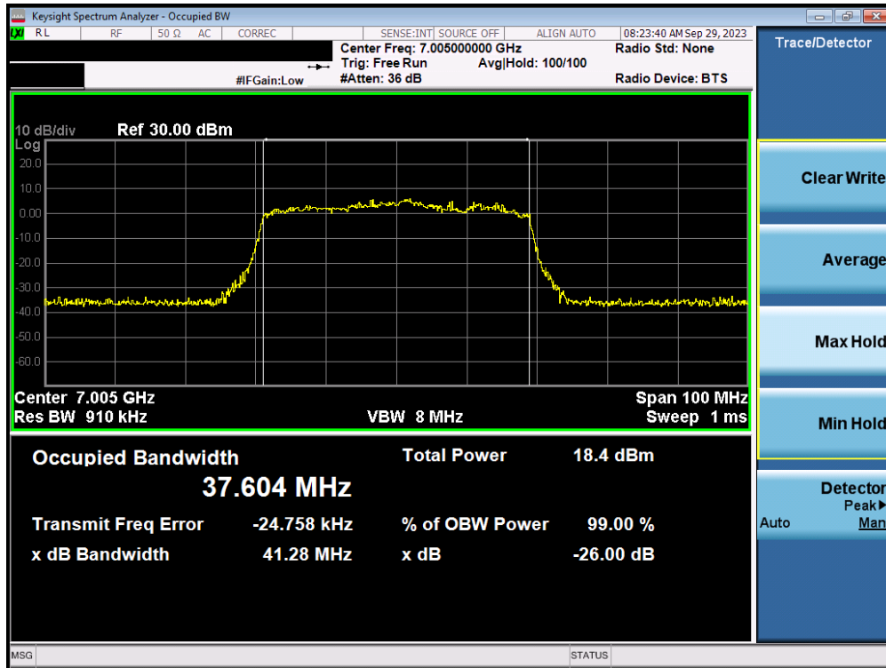
Plot 7-37. Occupied Bandwidth Plot MIMO ANT1 (40MHz BW 802.11ax/be (Full Tone) (UNII Band 8) – Ch. 211)
