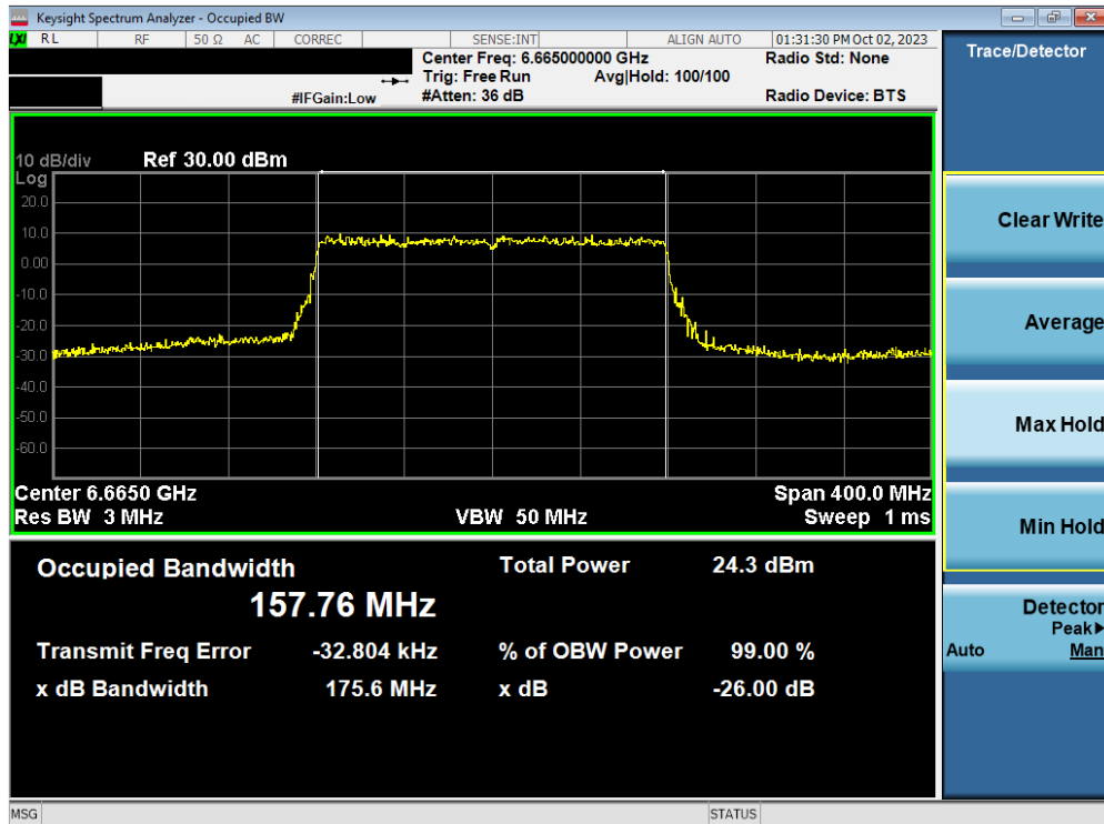
Plot 7-74. Occupied Bandwidth Plot MIMO ANT2 (160MHz BW 802.11ax/be (Full Tone) (UNII Band 7) – Ch. 143)
