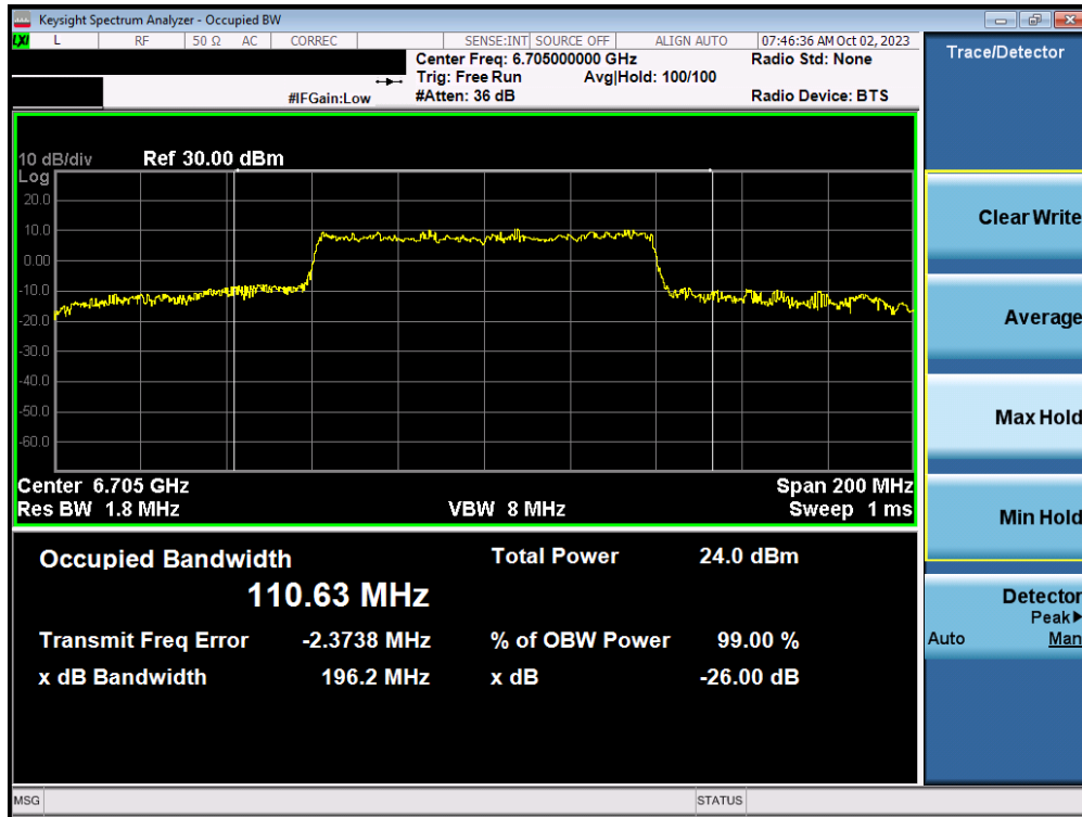
Plot 7-33. Occupied Bandwidth Plot MIMO ANT1 (80MHz BW 802.11ax/be (Full Tone) (UNII Band 7) – Ch. 151)
