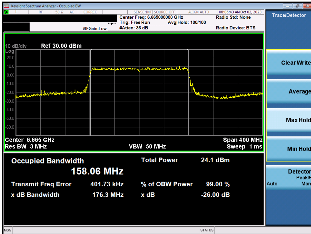
Plot 7-34. Occupied Bandwidth Plot MIMO ANT1 (160MHz BW 802.11ax/be (Full Tone) (UNII Band 7) – Ch. 143)
