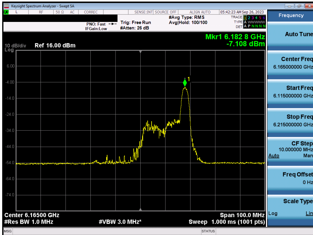
Plot 7-84. Power Spectral Density Plot MIMO ANT1 (40MHz BW 802.11ax/be (26 Tones) (UNII Band 5) – Ch. 43) – LPI
