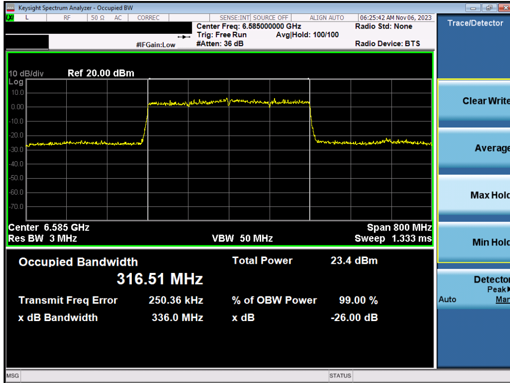
Plot 7-35. Occupied Bandwidth Plot MIMO ANT1 (320MHz BW 802.11ax/be (26 Tones) (UNII Band 6/7) – Ch. 127)
