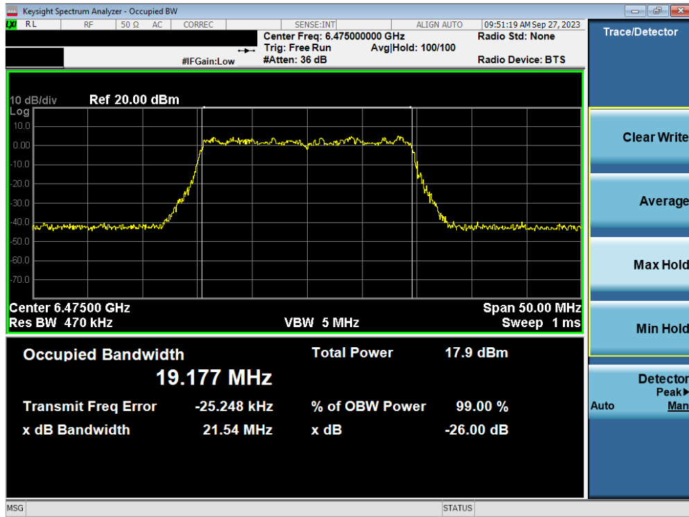
Plot 7-66. Occupied Bandwidth Plot MIMO ANT2 (20MHz BW 802.11ax/be (Full Tone) (UNII Band 6) – Ch. 105)
