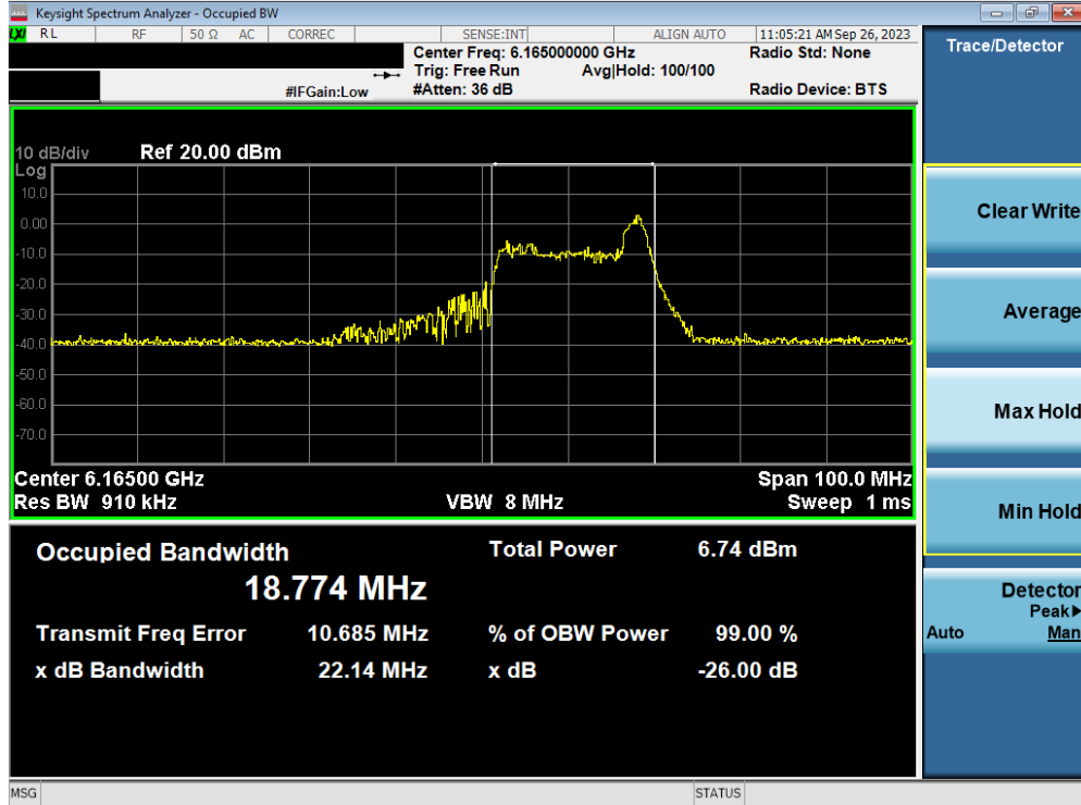
Plot 7-42. Occupied Bandwidth Plot MIMO ANT2 (40MHz BW 802.11ax/be (26 Tones) (UNII Band 5) – Ch. 43)
