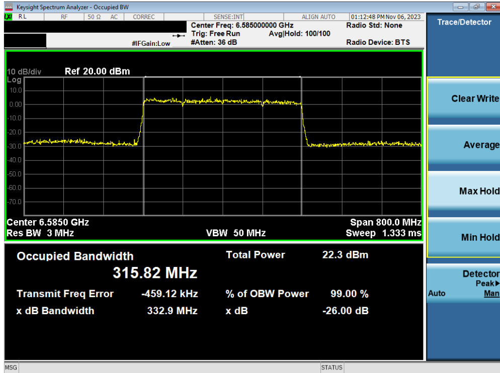
Plot 7-75. Occupied Bandwidth Plot MIMO ANT2 (320MHz BW 802.11ax/be (26 Tones) (UNII Band 6/7) – Ch. 127)
