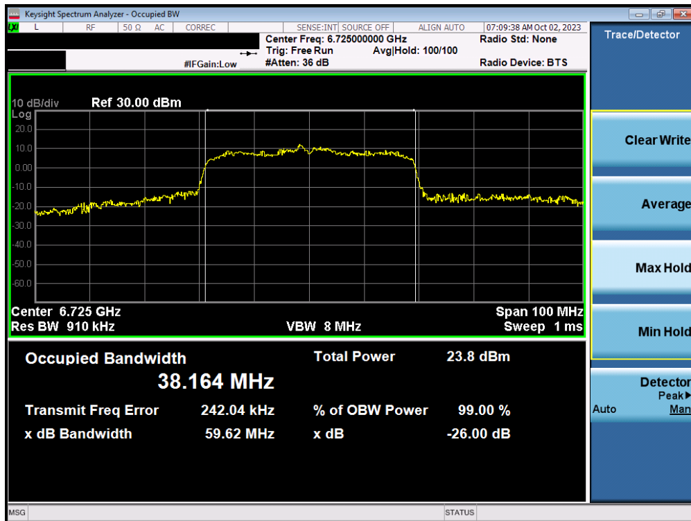
Plot 7-32. Occupied Bandwidth Plot MIMO ANT1 (40MHz BW 802.11ax/be (Full Tone) (UNII Band 7) – Ch. 155)
