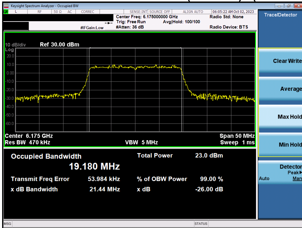
Plot 7-21. Occupied Bandwidth Plot MIMO ANT1 (20MHz BW 802.11ax/be (Full Tone) (UNII Band 5) – Ch. 45)
