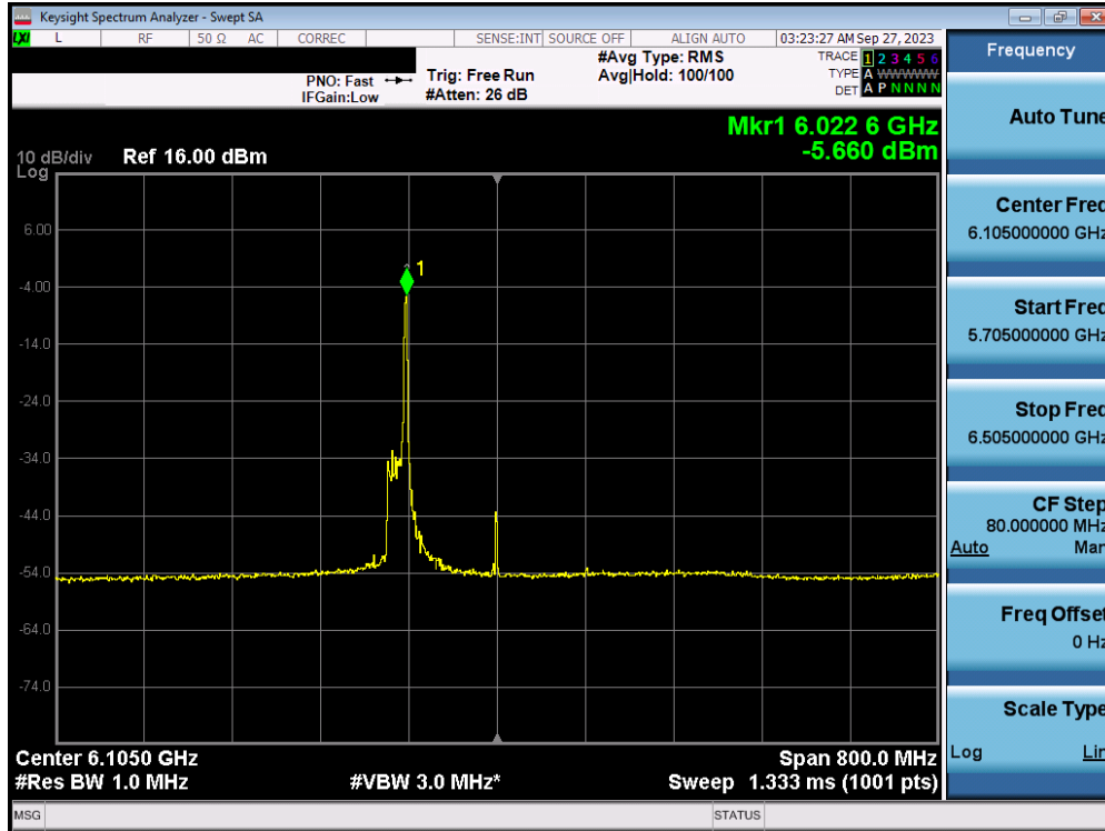
Plot 7-89. Power Spectral Density Plot MIMO ANT1 (320MHz BW 802.11ax/be (26 Tones) (UNII Band 5) – Ch. 31) – LPI
