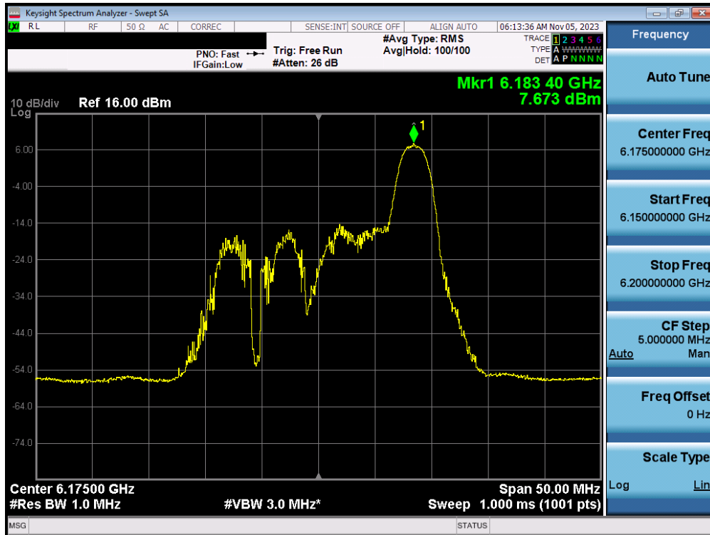
Plot 7-93. Power Spectral Density Plot MIMO ANT1 (20MHz BW 802.11ax/be (26 Tones) (UNII Band 5) – Ch. 45) – SP
