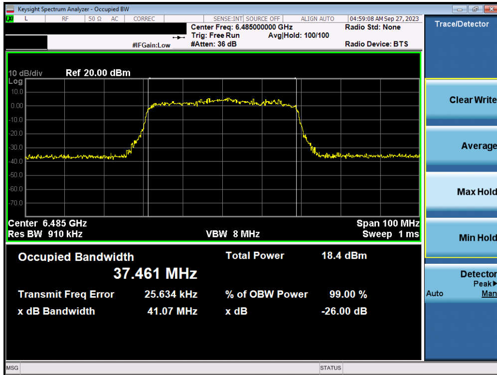
Plot 7-27. Occupied Bandwidth Plot MIMO ANT1 (40MHz BW 802.11ax/be (Full Tone) (UNII Band 6) – Ch. 107)
