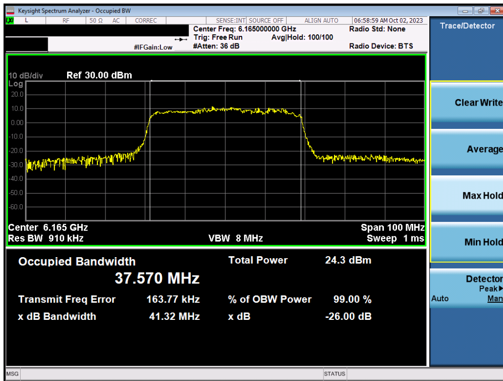
Plot 7-22. Occupied Bandwidth Plot MIMO ANT1 (40MHz BW 802.11ax/be (Full Tone) (UNII Band 5) – Ch. 43)
