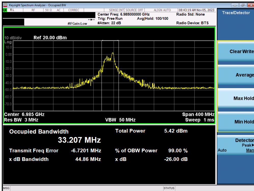
Plot 7-19. Occupied Bandwidth Plot MIMO ANT1 (160MHz BW 802.11ax/be (26 Tones) (UNII Band 8) – Ch. 207)
