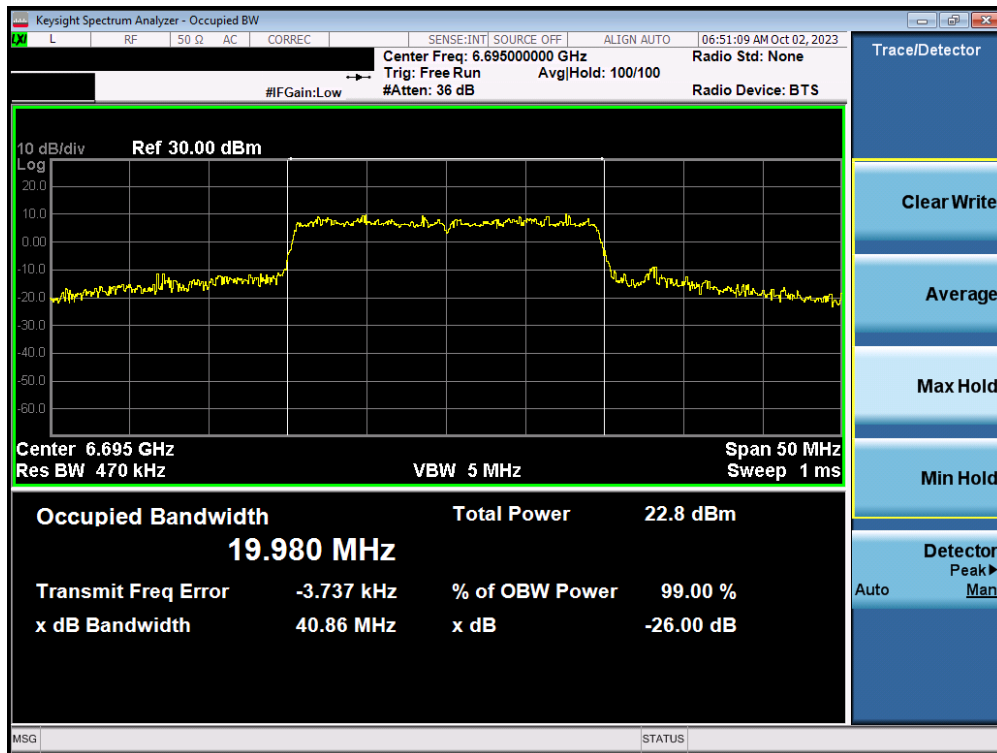
Plot 7-31. Occupied Bandwidth Plot MIMO ANT1 (20MHz BW 802.11ax/be (Full Tone) (UNII Band 7) – Ch. 149)
