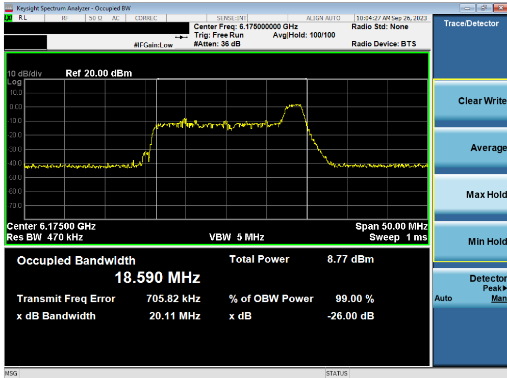
Plot 7-41. Occupied Bandwidth Plot MIMO ANT2 (20MHz BW 802.11ax/be (26 Tones) (UNII Band 5) – Ch. 45)
