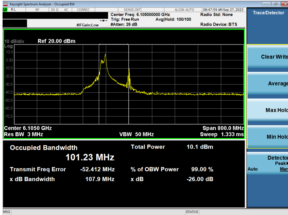
Plot 7-45. Occupied Bandwidth Plot MIMO ANT2 (320MHz BW 802.11ax/be (26 Tones) (UNII Band 5) – Ch. 31)
