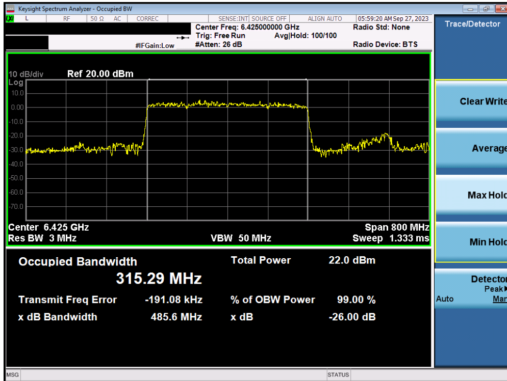
Plot 7-30. Occupied Bandwidth Plot MIMO ANT1 (320MHz BW 802.11ax/be (26 Tones) (UNII Band 5/6/7) – Ch. 95)
