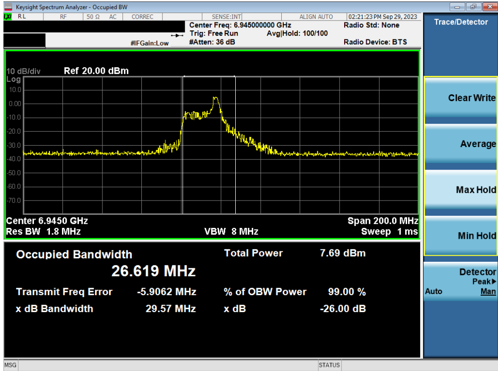
Plot 7-58. Occupied Bandwidth Plot MIMO ANT2 (80MHz BW 802.11ax/be (26 Tones) (UNII Band 8) – Ch. 199)
