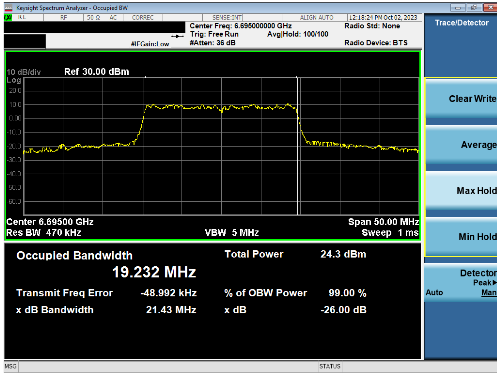
Plot 7-71. Occupied Bandwidth Plot MIMO ANT2 (20MHz BW 802.11ax/be (Full Tone) (UNII Band 7) – Ch. 149)
