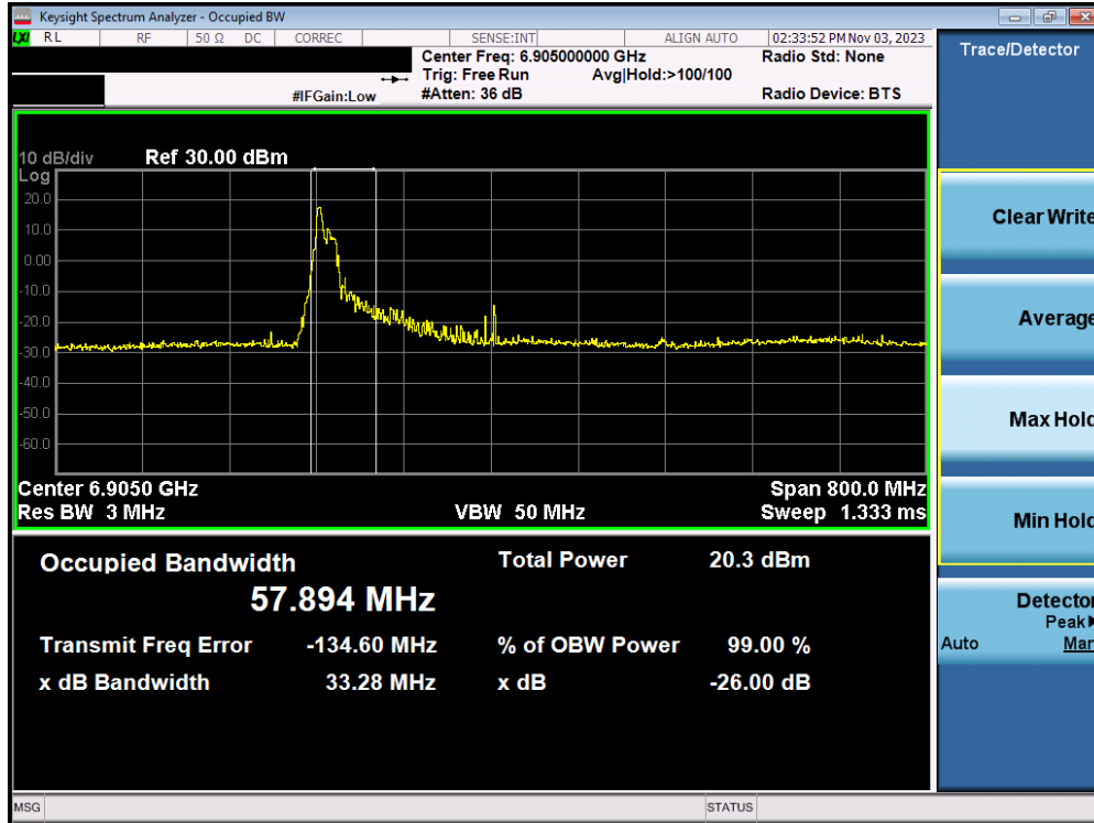
Plot 7-20. Occupied Bandwidth Plot MIMO ANT1 (320MHz BW 802.11ax/be (26 Tones) (UNII Band 7/8) – Ch. 191)
