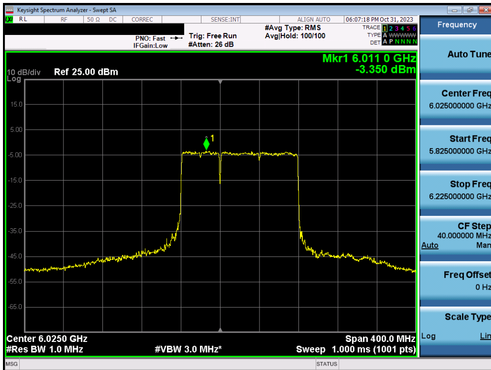
Plot 7-88. Power Spectral Density Plot MIMO ANT1 (160MHz BW 802.11ax/be (MRU) (UNII Band 5) – Ch. 15) – LPI – 996+242T
