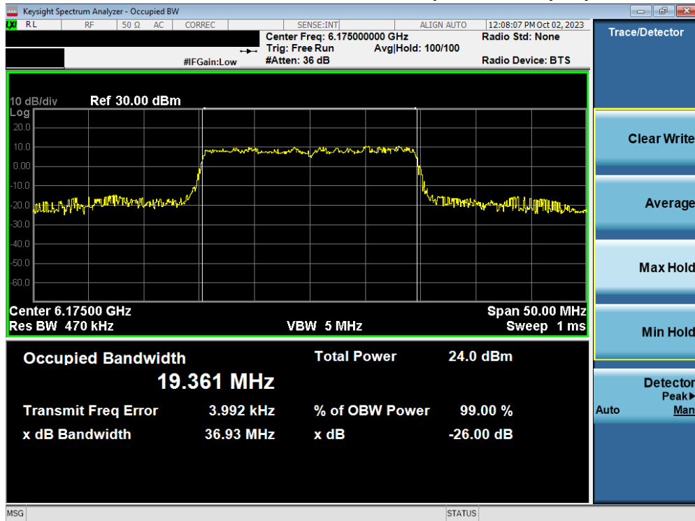
Plot 7-61. Occupied Bandwidth Plot MIMO ANT2 (20MHz BW 802.11ax/be (Full Tone) (UNII Band 5) – Ch. 45)
