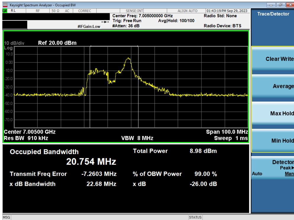
Plot 7-57. Occupied Bandwidth Plot MIMO ANT2 (40MHz BW 802.11ax/be (26 Tones) (UNII Band 8) – Ch. 211)
