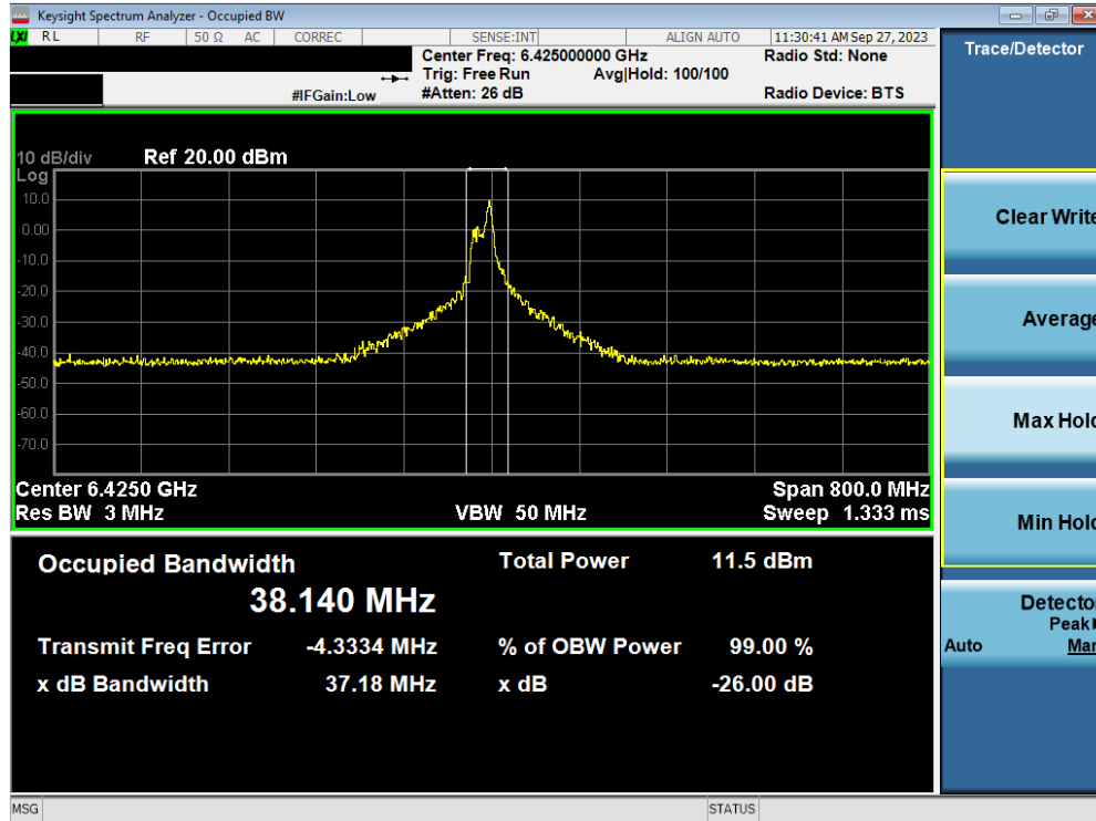
Plot 7-50. Occupied Bandwidth Plot MIMO ANT2 (320MHz BW 802.11ax/be (26 Tones) (UNII Band 5/6/7) – Ch. 95)
