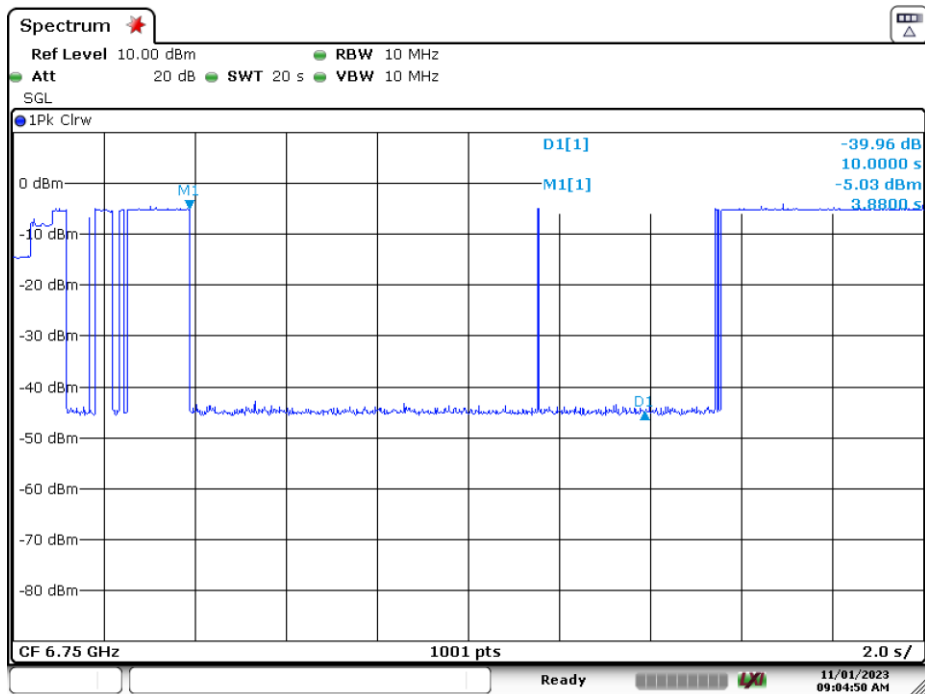
Plot 7-206. Contention Based Protocol Timing Plot (320MHz (UNII Band 8) – Ch. 191 Low)
