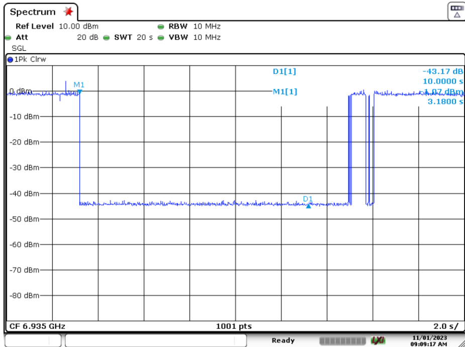
Plot 7-205. Contention Based Protocol Timing Plot (20MHz (UNII Band 8) – Ch. 197)
