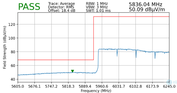
Plot 7-239. Radiated Lower Band Edge Plot MIMO (Average – UNII Band 5)
