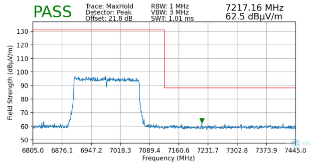
Plot 7-238. Radiated Upper Band Edge Plot MIMO (Peak – UNII Band 8)
