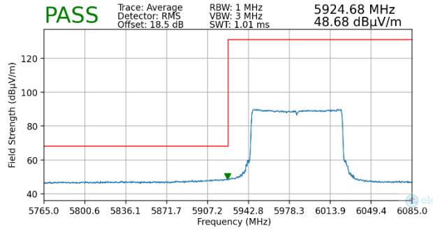
Plot 7-231. Radiated Lower Band Edge Plot MIMO (Average – UNII Band 5)
