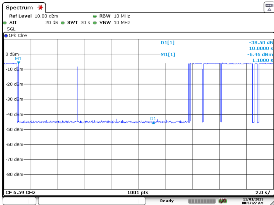
Plot 7-202. Contention Based Protocol Timing Plot (320MHz (UNII Band 7) – Ch. 159 Low)
