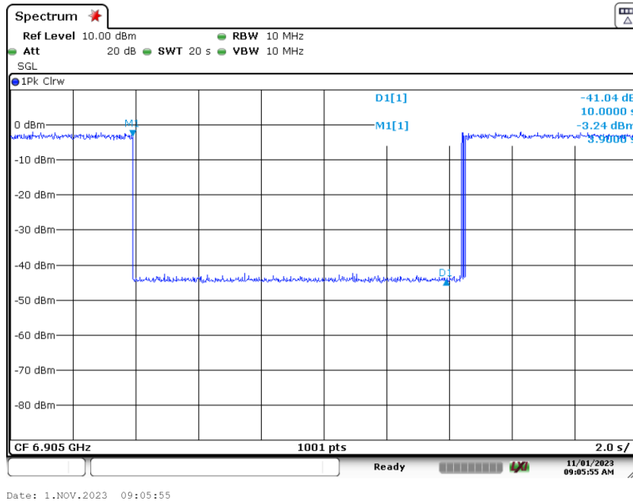
Plot 7-207. Contention Based Protocol Timing Plot (320MHz (UNII Band 8) – Ch. 191 Mid)
