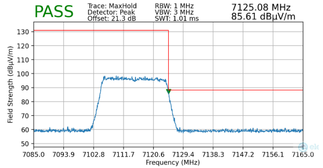
Plot 7-226. Radiated Upper Band Edge Plot MIMO (Peak – UNII Band 8) with WCP
