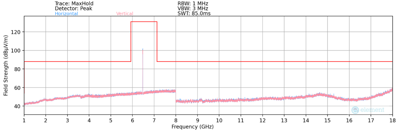
Plot 7-215. Radiated Spurious Plot 1GHz – 18GHz MIMO (802.11ax – UNII Band 6 Ch. 105 – LPI)
