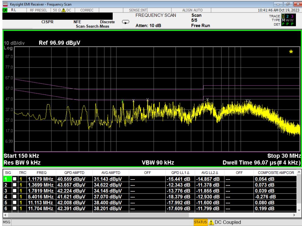
Plot 7-243. Line Conducted Plot with 802.11a UNII Band 5 (L1)
