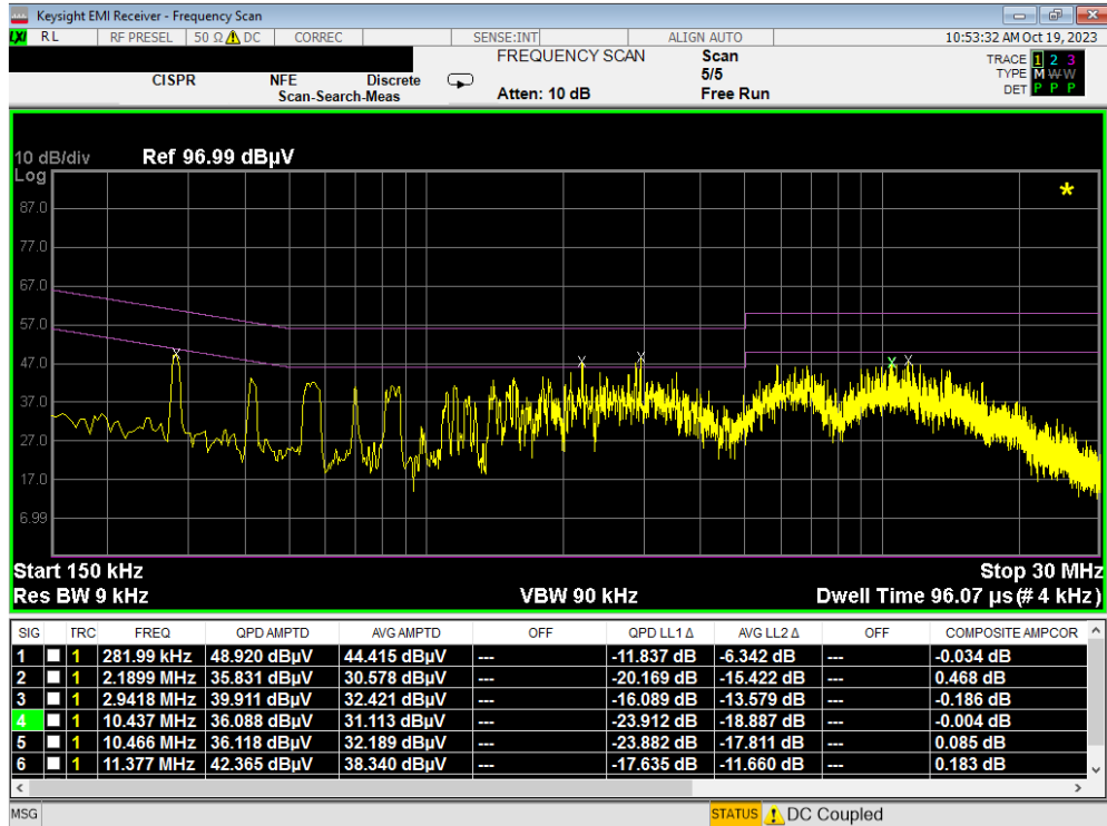
Plot 7-245. Line Conducted Plot with 802.11a UNII Band 6 (L1)
