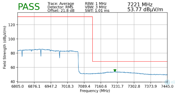
Plot 7-241. Radiated Upper Band Edge Plot MIMO (Average – UNII Band 8)
