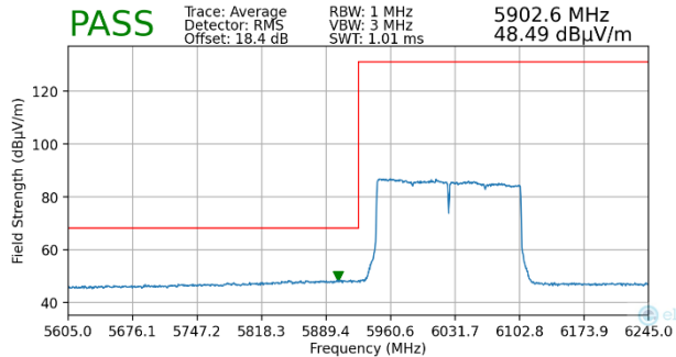
Plot 7-235. Radiated Lower Band Edge Plot MIMO (Average – UNII Band 5)
