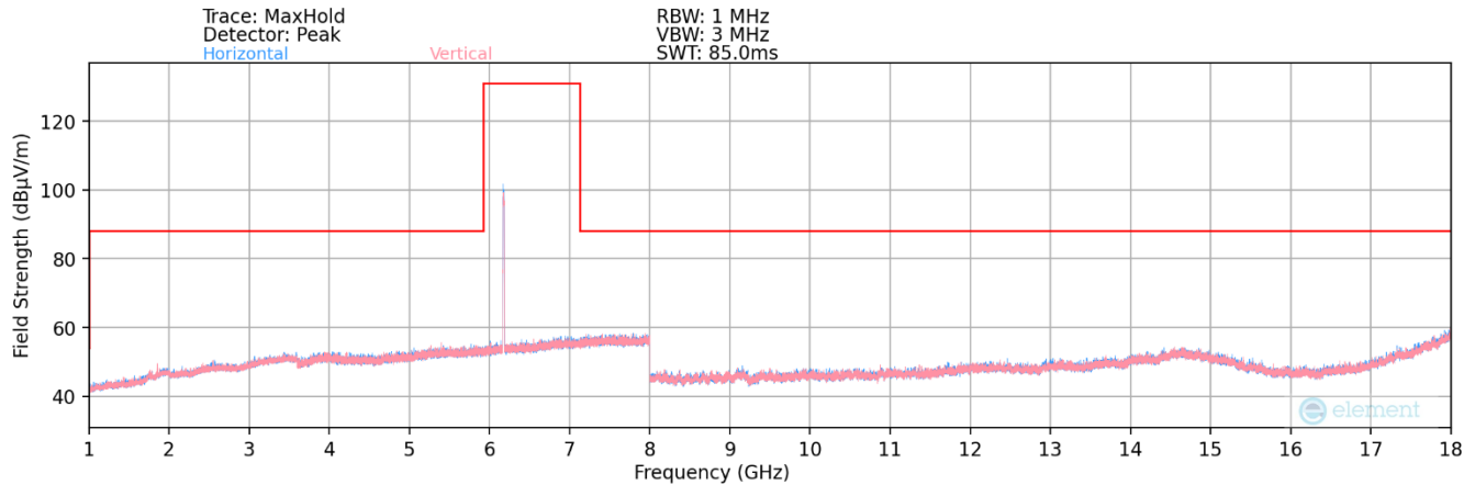
Plot 7-213. Radiated Spurious Plot 1GHz – 18GHz MIMO (802.11ax – UNII Band 5 Ch. 45 – LPI)
