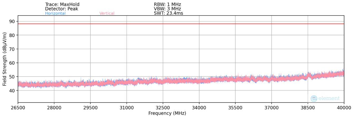
Plot 7-220. Radiated Spurious Plot 26.5GHz - 40GHz (802.11ax)
