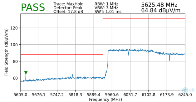
Plot 7-240. Radiated Lower Band Edge Plot MIMO (Peak – UNII Band 5)
