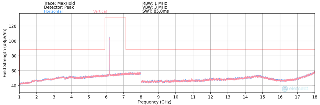
Plot 7-214. Radiated Spurious Plot 1GHz – 18GHz MIMO (802.11ax – UNII Band 5 Ch. 45 – SP)
