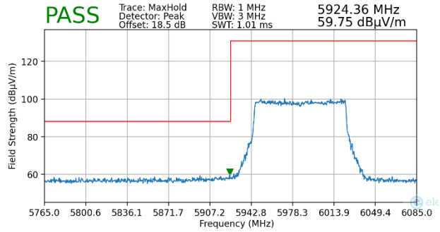
Plot 7-232. Radiated Lower Band Edge Plot MIMO (Peak – UNII Band 5)
