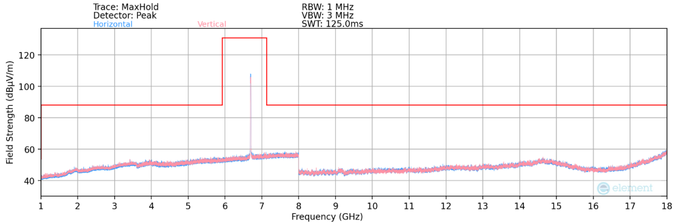
Plot 7-217. Radiated Spurious Plot 1GHz – 18GHz MIMO (802.11ax – UNII Band 7 Ch. 149 – SP)
