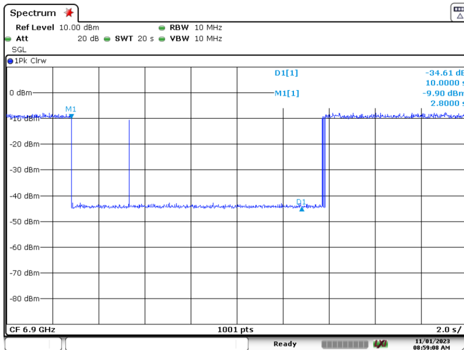
Plot 7-203. Contention Based Protocol Timing Plot (320MHz (UNII Band 7) – Ch. 159 Mid)
