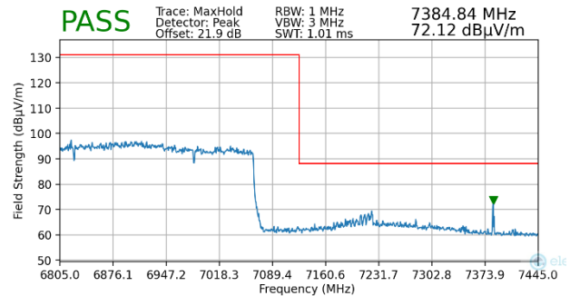
Plot 7-242. Radiated Upper Band Edge Plot MIMO (Peak – UNII Band 8)
