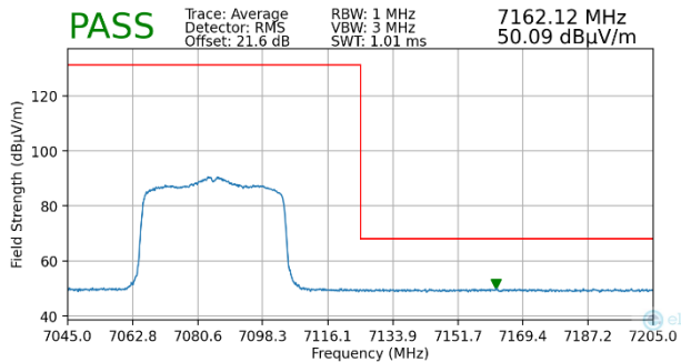
Plot 7-229. Radiated Upper Band Edge Plot MIMO (Average – UNII Band 8)
