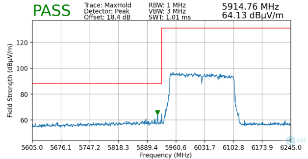
Plot 7-236. Radiated Lower Band Edge Plot MIMO (Peak – UNII Band 5)
