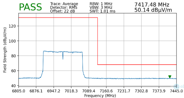
Plot 7-237. Radiated Upper Band Edge Plot MIMO (Average – UNII Band 8)
