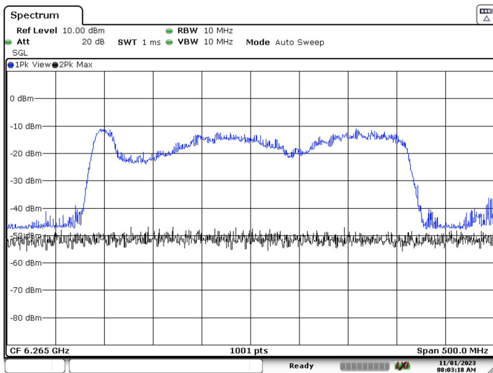
Plot 7-209. CBP 320MHz Channel - Injection Lower Edge – [6110 MHz]
