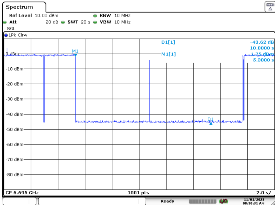
Plot 7-201. Contention Based Protocol Timing Plot (20MHz (UNII Band 7) – Ch. 149)
