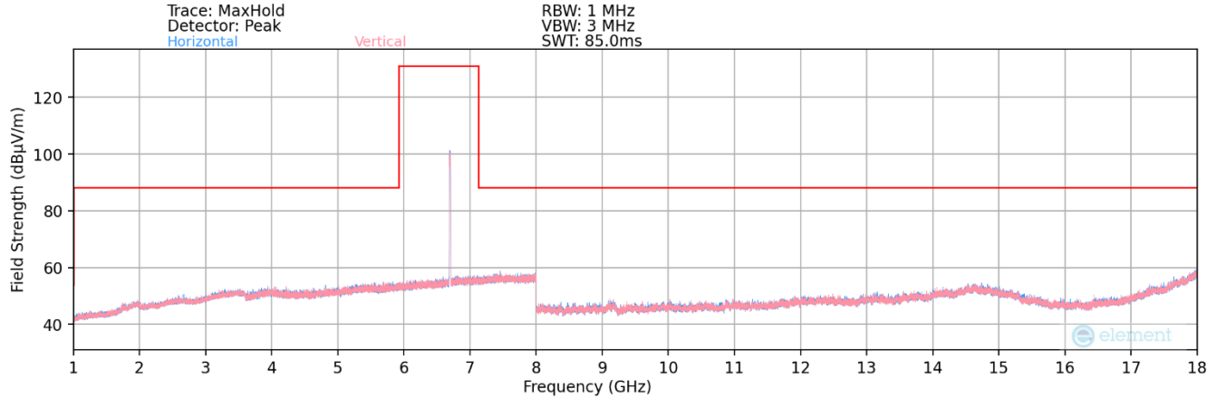
Plot 7-216. Radiated Spurious Plot 1GHz – 18GHz MIMO (802.11ax – UNII Band 7 Ch. 149 – LPI)
