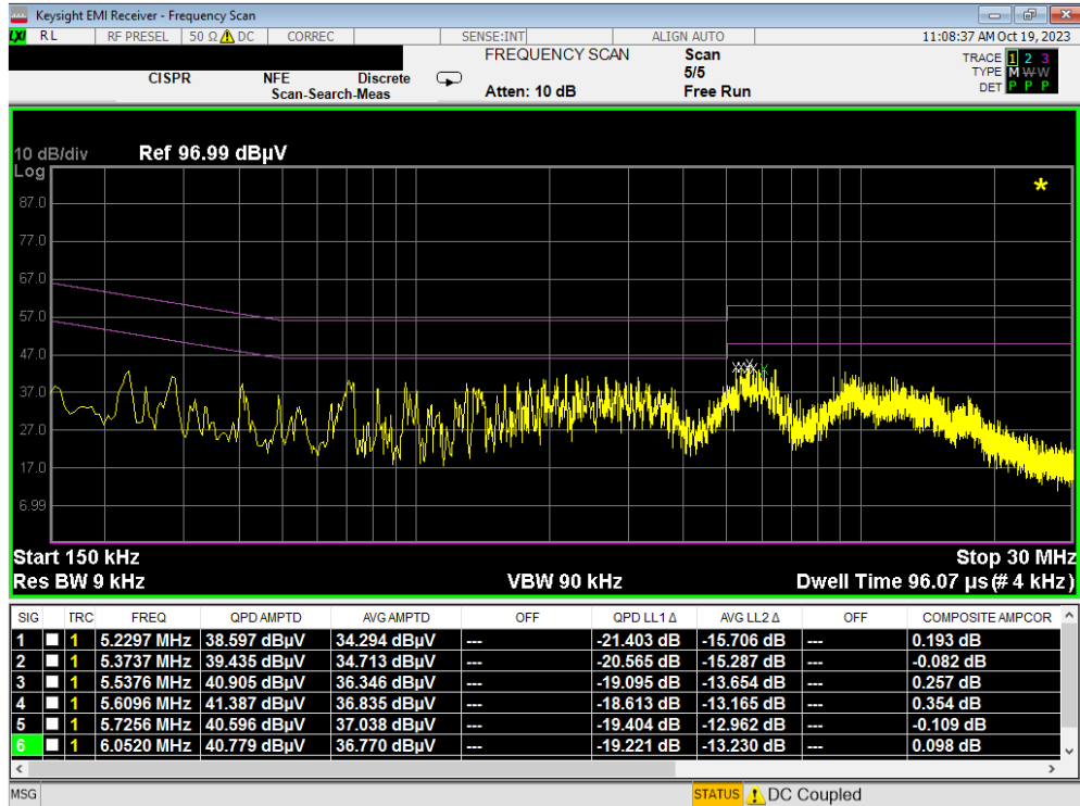
Plot 7-249. Line Conducted Plot with 802.11a UNII Band 8 (L1)
