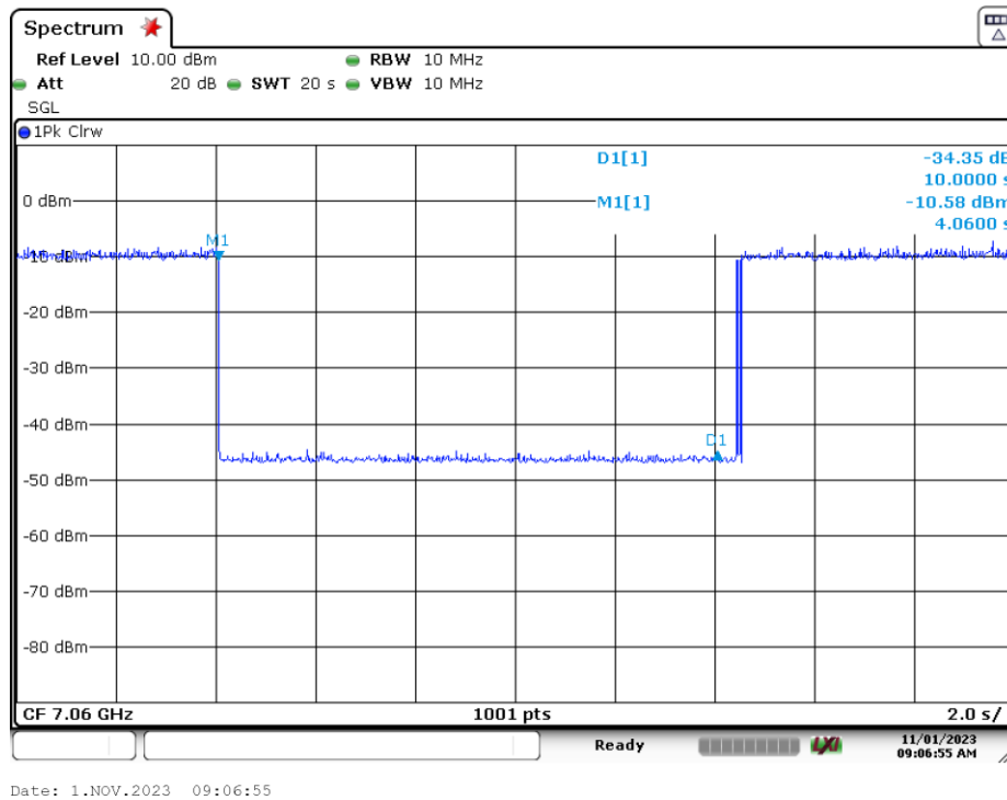
Plot 7-208. Contention Based Protocol Timing Plot (320MHz (UNII Band 8) – Ch. 191 High)
