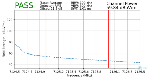
Plot 7-225. Radiated Upper Band Edge Plot MIMO (Average – UNII Band 8) with WCP
