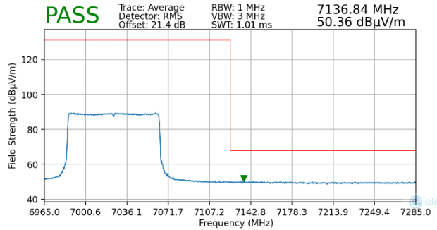
Plot 7-233. Radiated Upper Band Edge Plot MIMO (Average – UNII Band 8)
