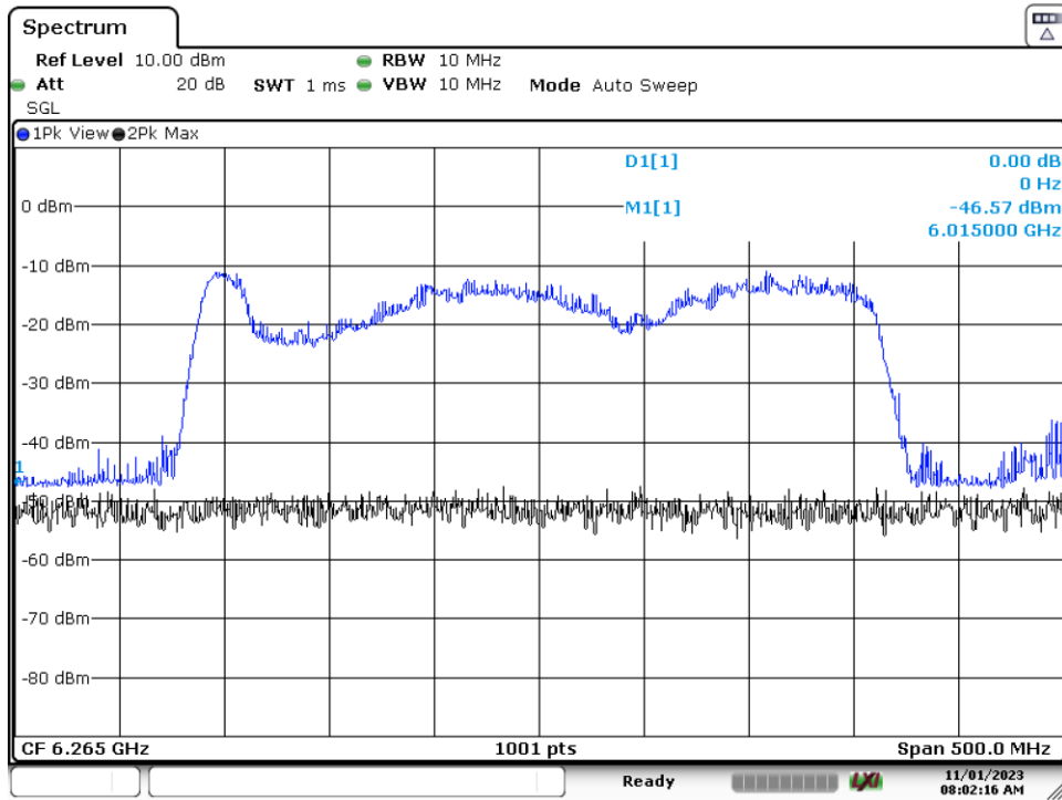
Plot 7-210. CBP 320MHz Channel - Injection Center – [6265 MHz]
