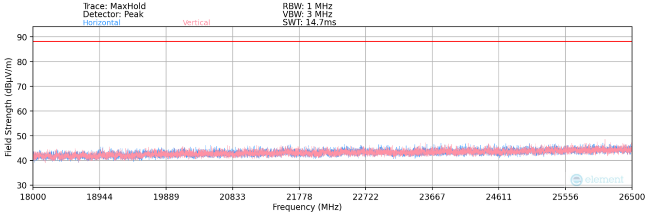
Plot 7-219. Radiated Spurious Plot 18GHz - 26.5GHz (802.11ax)
