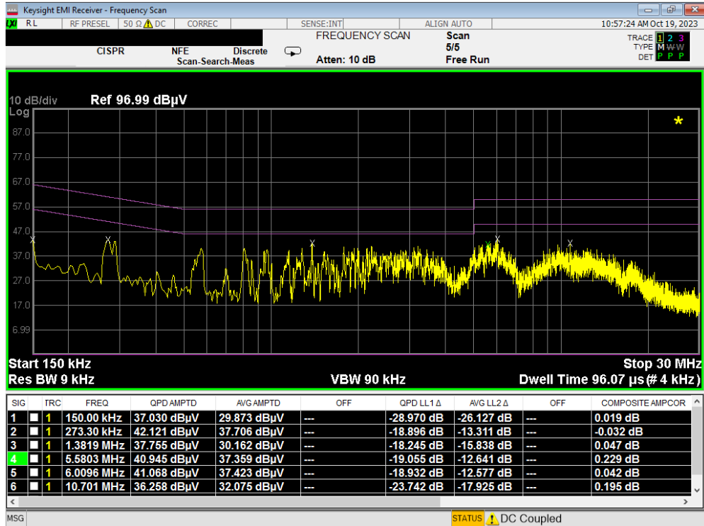
Plot 7-247. Line Conducted Plot with 802.11a UNII Band 7 (L1)
