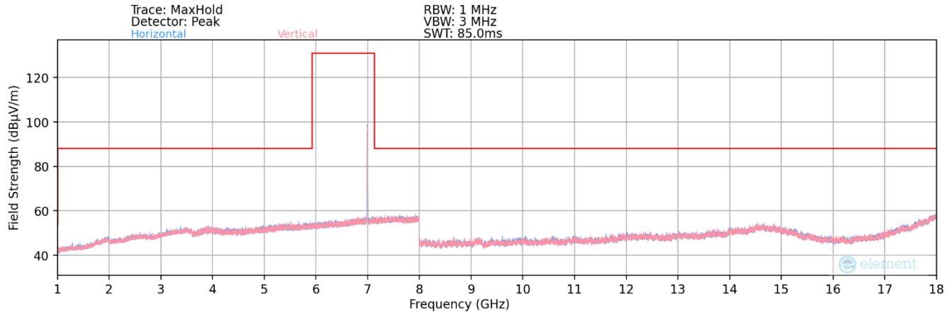
Plot 7-218. Radiated Spurious Plot 1GHz – 18GHz MIMO (802.11ax – U Band 8 Ch. 209 – LPI)
