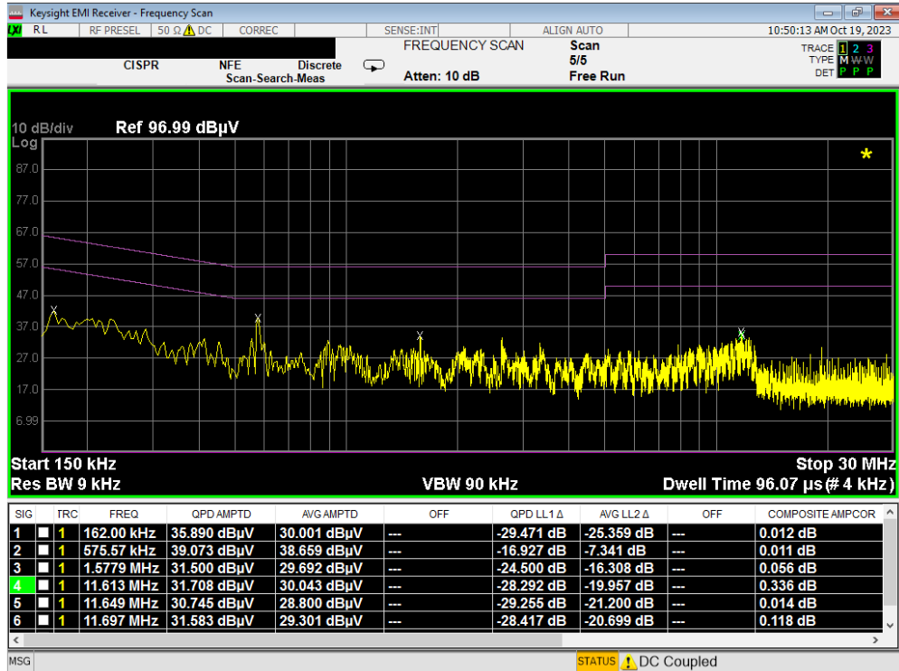
Plot 7-251. Line Conducted Plot with 802.11a UNII Band 5 (L1) with WCP
