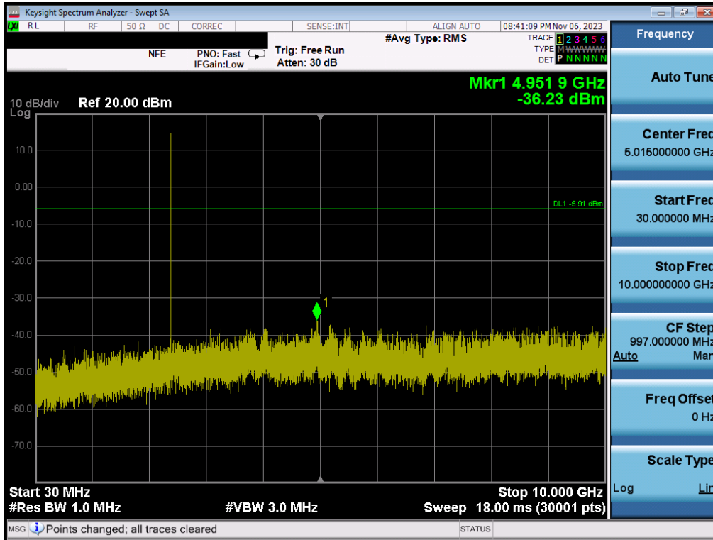
Plot 7-151. Conducted Spurious Plot (Bluetooth (LE), 1Mbps – Ch. 0) – Dual ANT2
