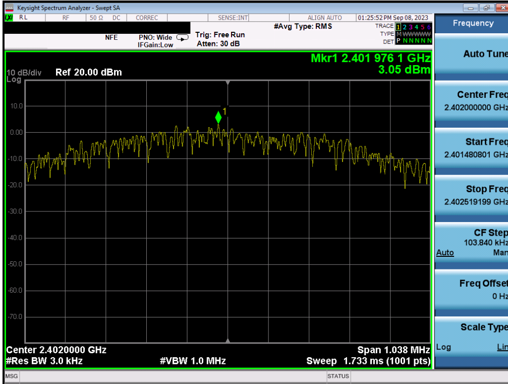
Plot 7-91. Power Spectral Density Plot (Bluetooth (LE), 1Mbps – Ch. 0 ) – ANT2
