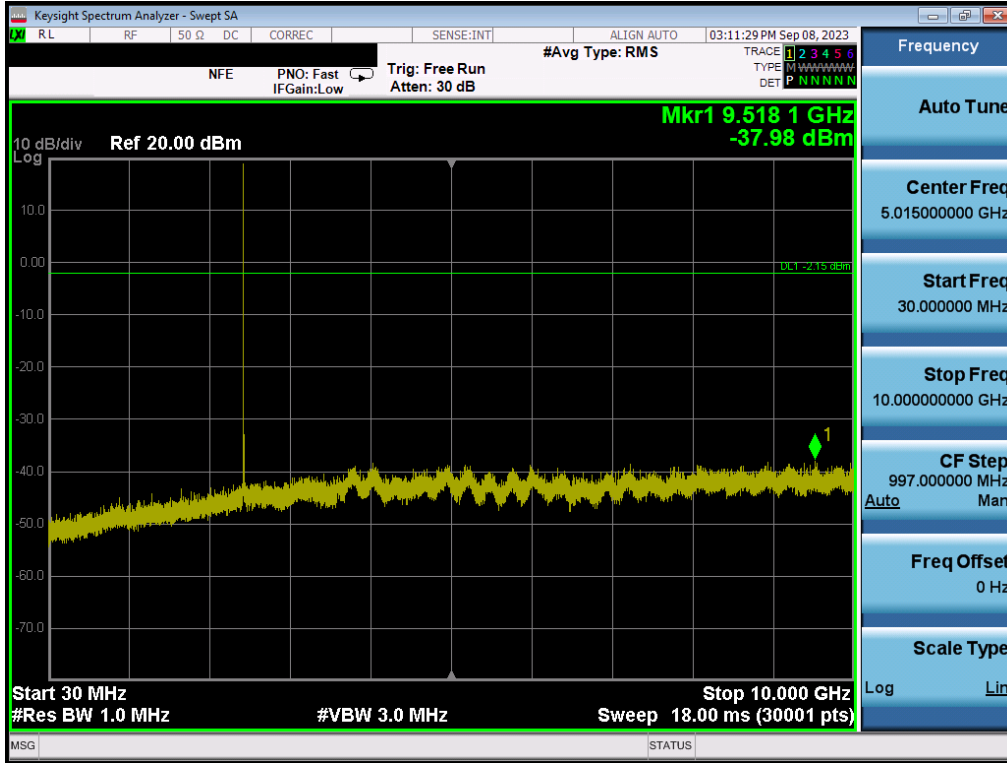
Plot 7-135. Conducted Spurious Plot (Bluetooth (LE), 1Mbps – Ch. 19) – ANT1
