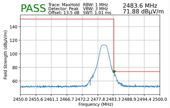
Plot 7-158. Radiated Restricted Upper Band Edge Measurement (Peak) ANT1
