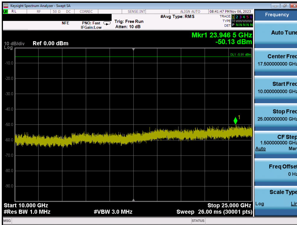
Plot 7-152. Conducted Spurious Plot (Bluetooth (LE), 1Mbps – Ch. 0) – Dual ANT2
