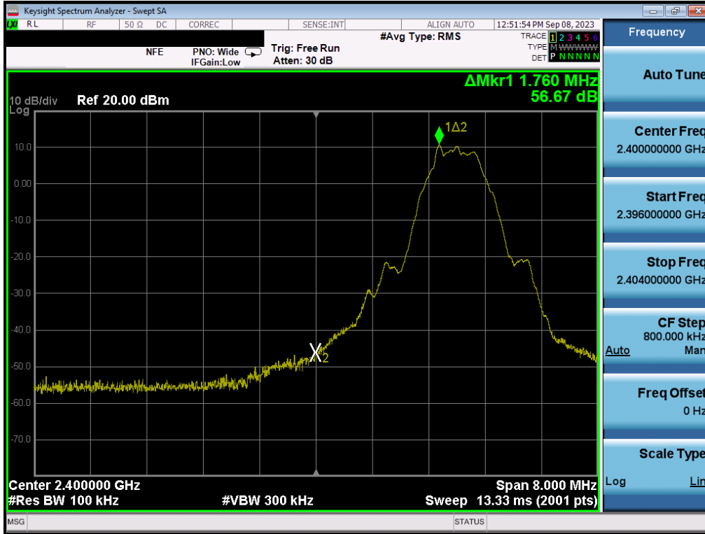
Plot 7-119. Band Edge Plot (Bluetooth (LE), 500kbps – Ch. 0) – ANT2
