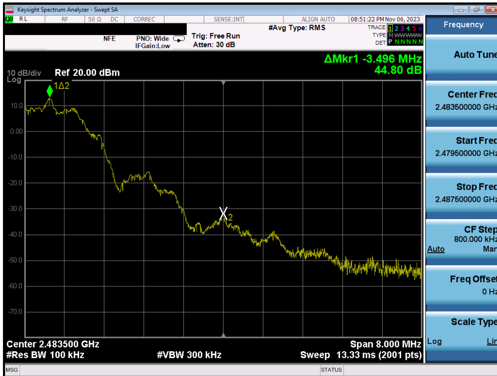
Plot 7-132. Band Edge Plot (Bluetooth (LE), 2Mbps – Ch. 39) – Dual ANT2
