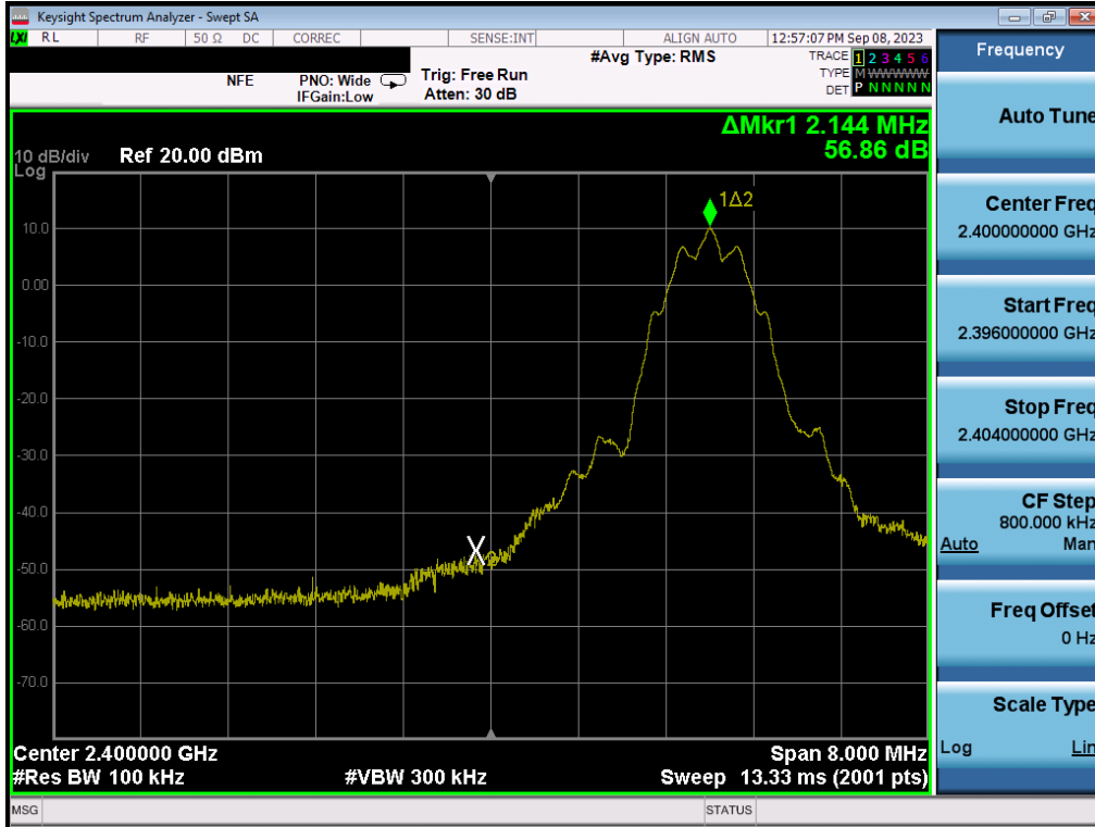
Plot 7-117. Band Edge Plot (Bluetooth (LE), 125kbps – Ch. 0) – ANT2
