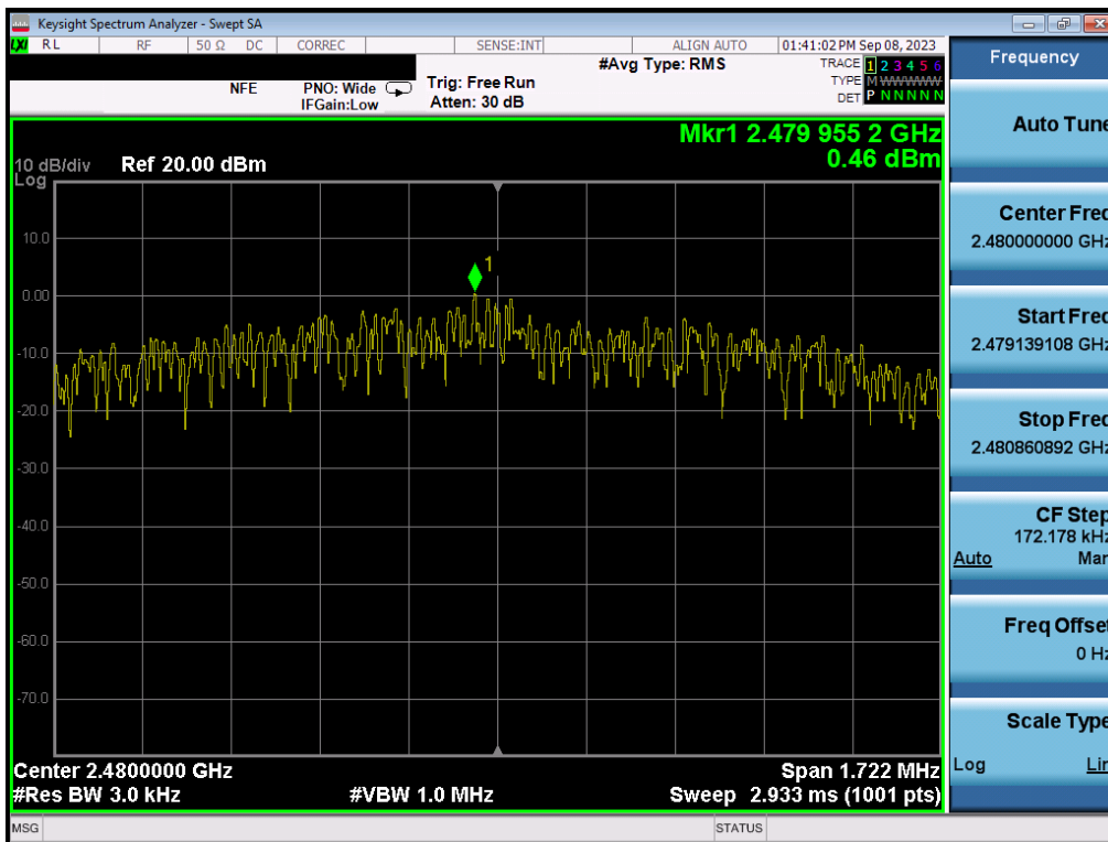
Plot 7-96. Power Spectral Density Plot (Bluetooth (LE), 2Mbps – Ch. 39) – ANT2
