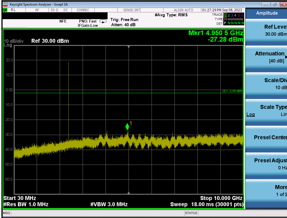
Plot 7-139. Conducted Spurious Plot (Bluetooth (LE), 1Mbps – Ch. 0) – ANT2
