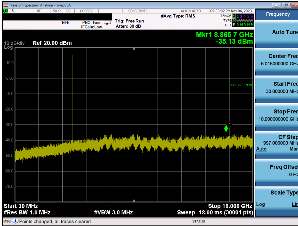
Plot 7-147. Conducted Spurious Plot (Bluetooth (LE), 1Mbps – Ch. 19) – Dual ANT1
