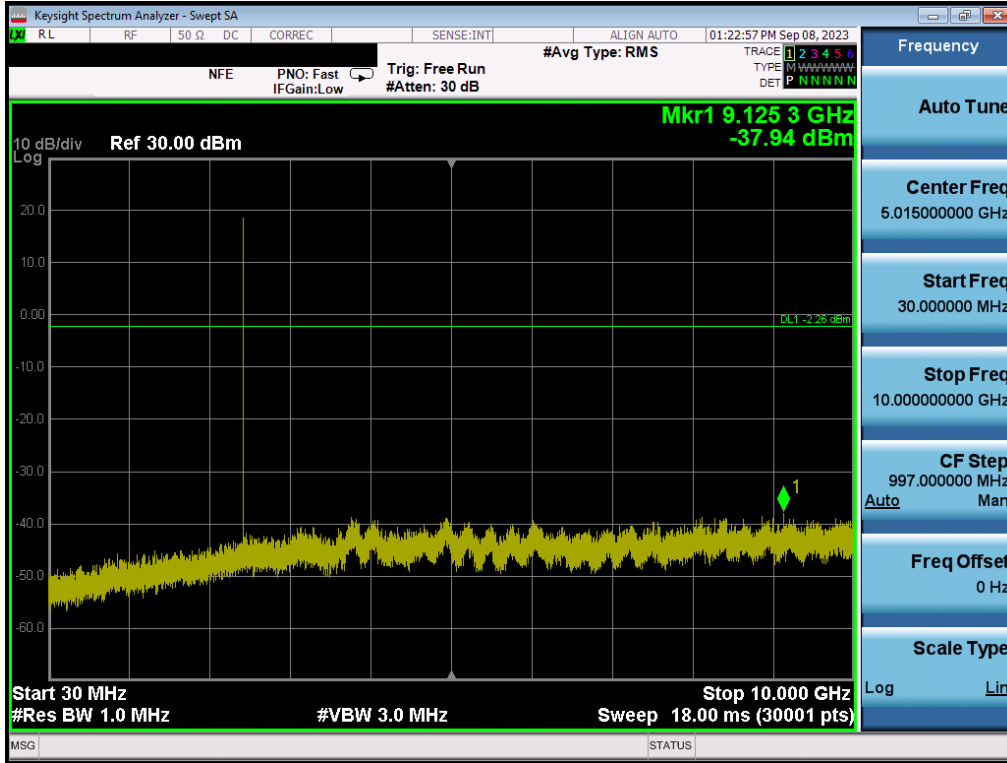
Plot 7-141. Conducted Spurious Plot (Bluetooth (LE), 1Mbps – Ch. 19) – ANT2
