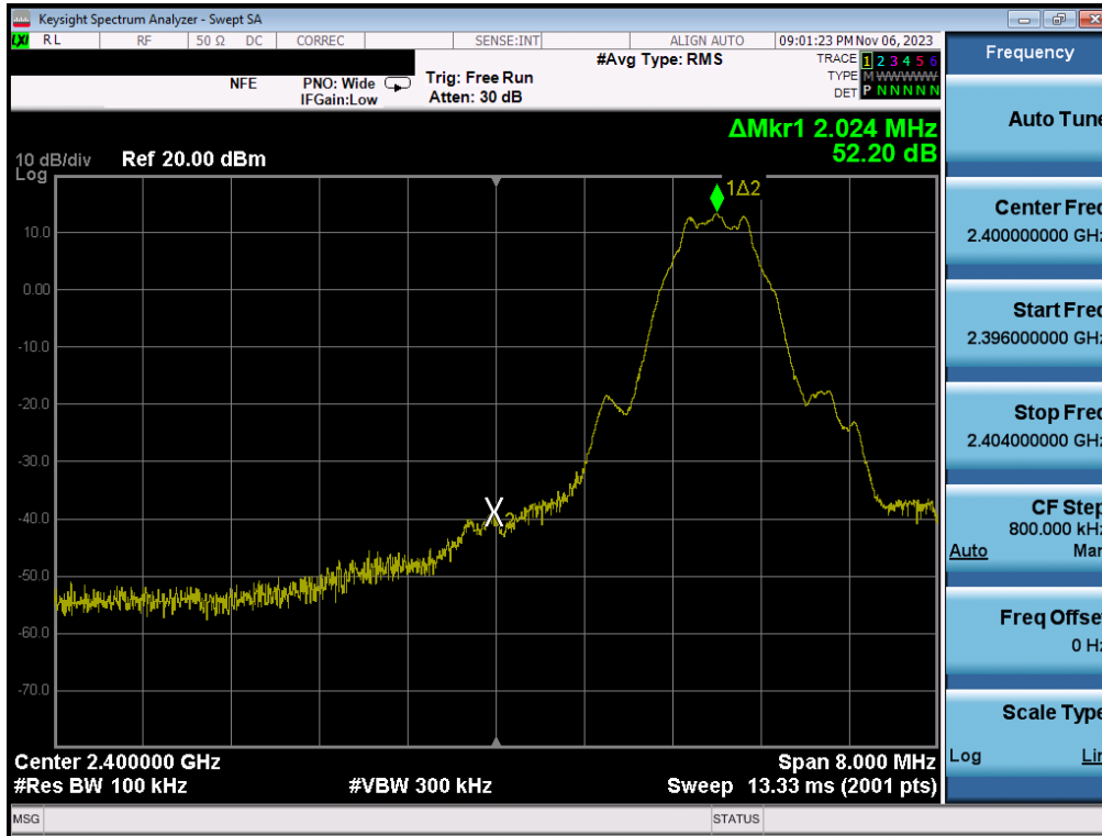
Plot 7-125. Band Edge Plot (Bluetooth (LE), 1Mbps – Ch. 0) – Dual ANT1
