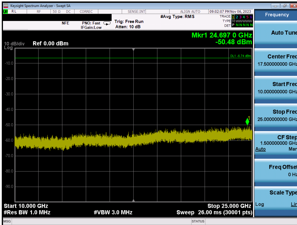
Plot 7-146. Conducted Spurious Plot (Bluetooth (LE), 1Mbps – Ch. 0) – Dual ANT1
