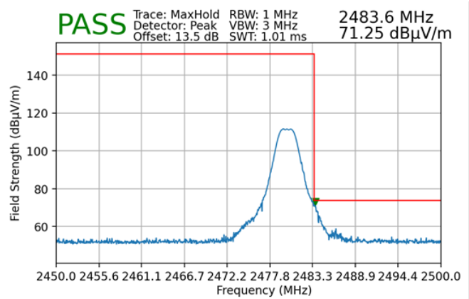
Plot 7-160. Radiated Restricted Upper Band Edge Measurement (Peak) ANT2
