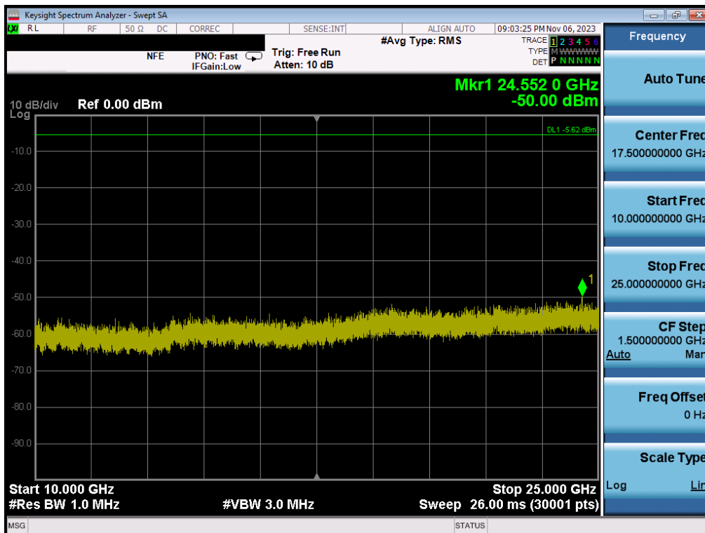
Plot 7-148. Conducted Spurious Plot (Bluetooth (LE), 1Mbps – Ch. 19) – Dual ANT1
