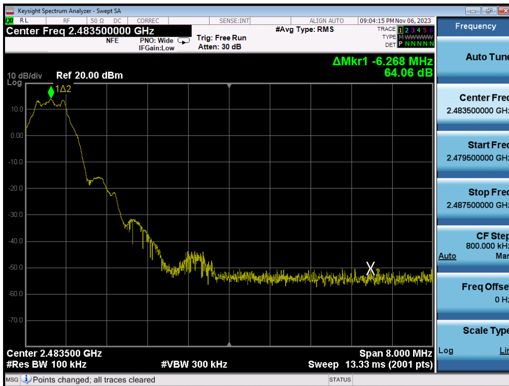
Plot 7-126. Band Edge Plot (Bluetooth (LE), 1Mbps – Ch. 39) – Dual ANT1
