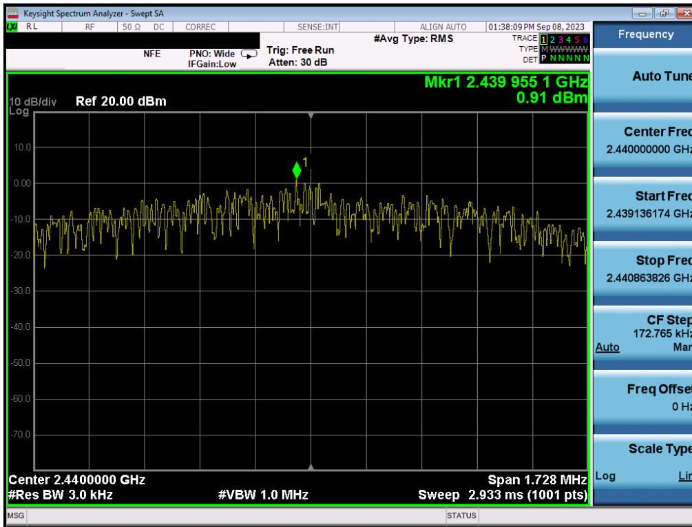
Plot 7-95. Power Spectral Density Plot (Bluetooth (LE), 2Mbps – Ch. 19) – ANT2
