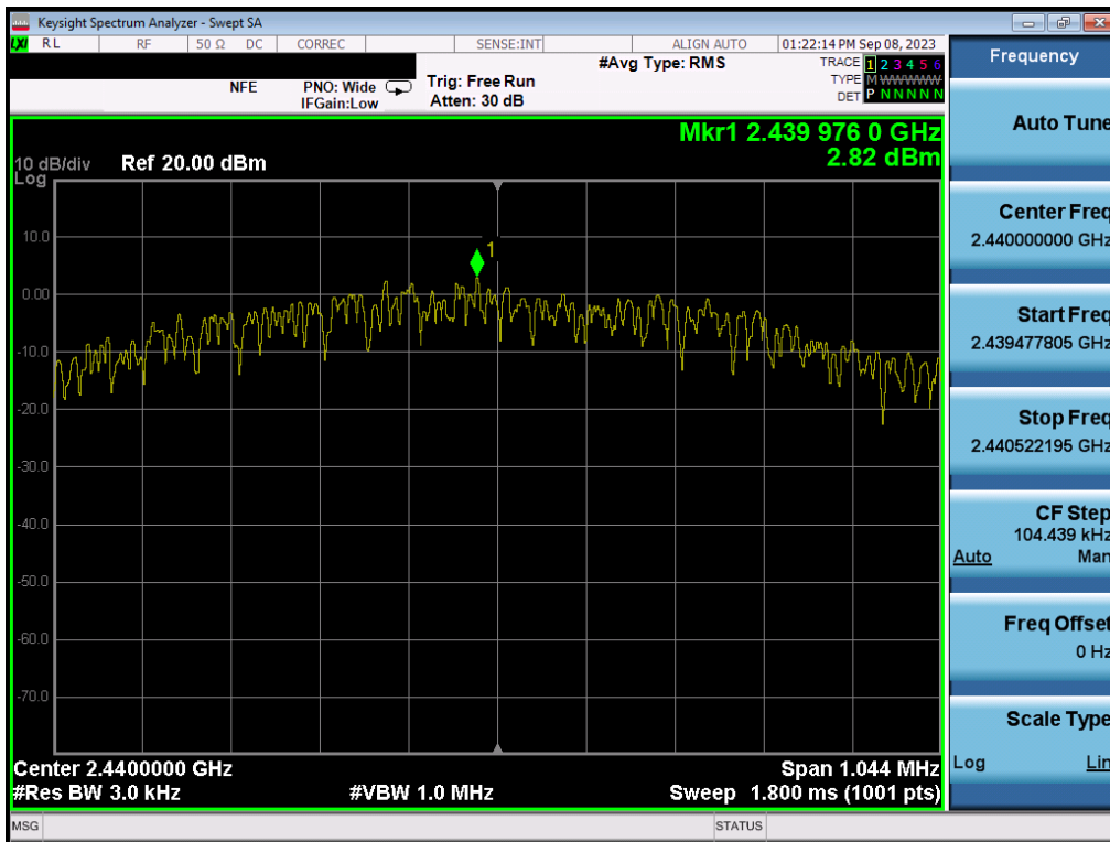
Plot 7-92. Power Spectral Density Plot (Bluetooth (LE), 1Mbps – Ch. 19 ) – ANT2
