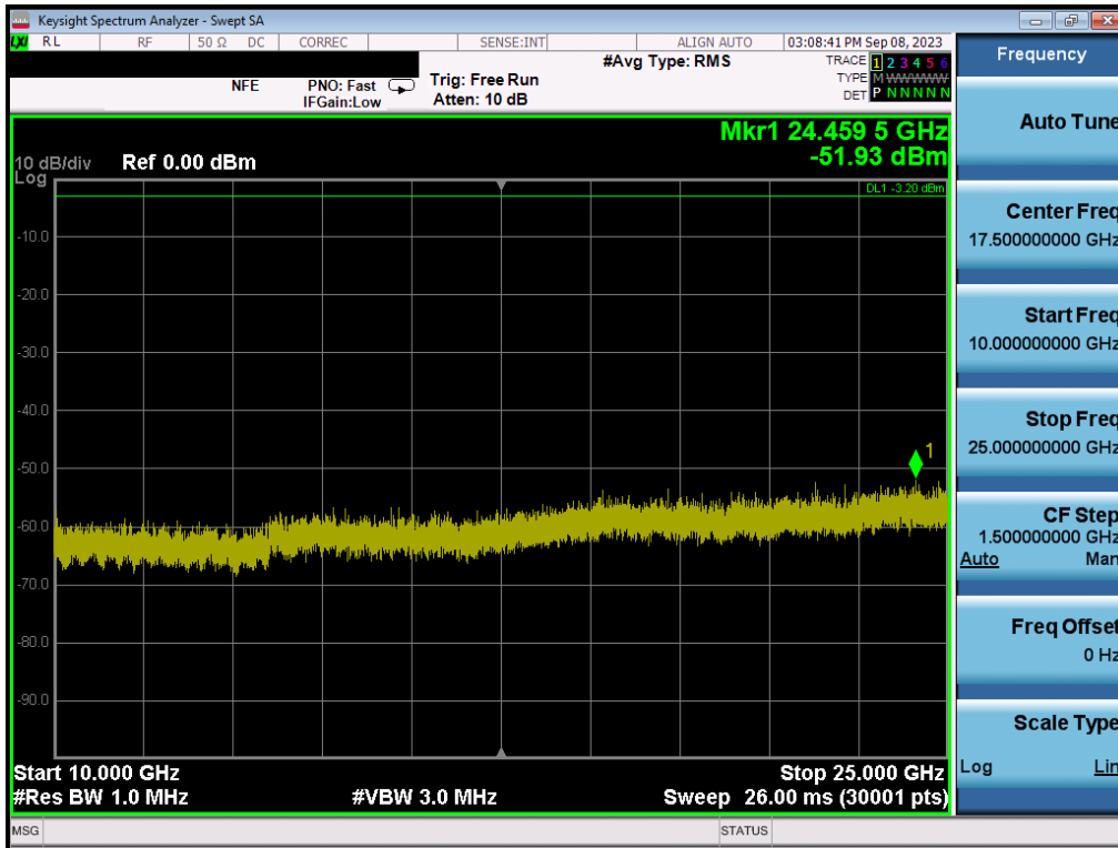
Plot 7-134. Conducted Spurious Plot (Bluetooth (LE), 1Mbps – Ch. 0) – ANT1
