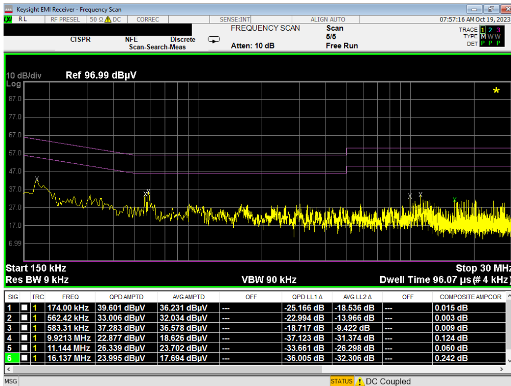
Plot 7-166. Line Conducted Plot with Bluetooth LE (N) WCP
