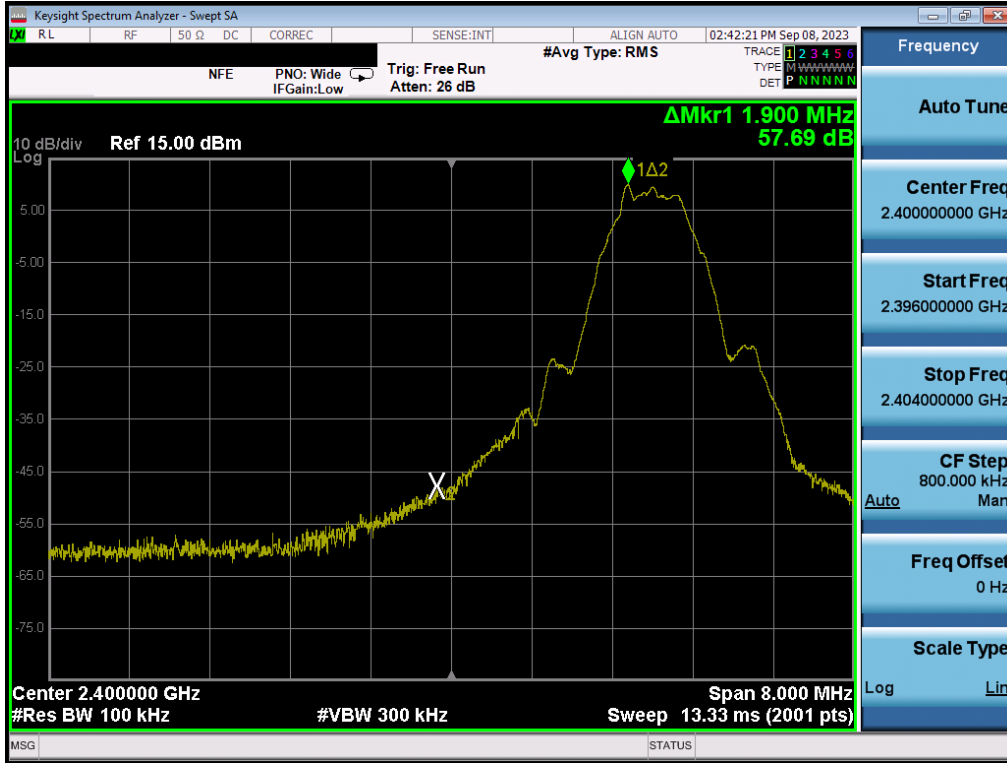
Plot 7-111. Band Edge Plot (Bluetooth (LE), 500kbps – Ch. 0) – ANT1
