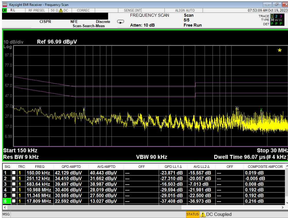
Plot 7-165. Line Conducted Plot with Bluetooth LE (L1) WCP
