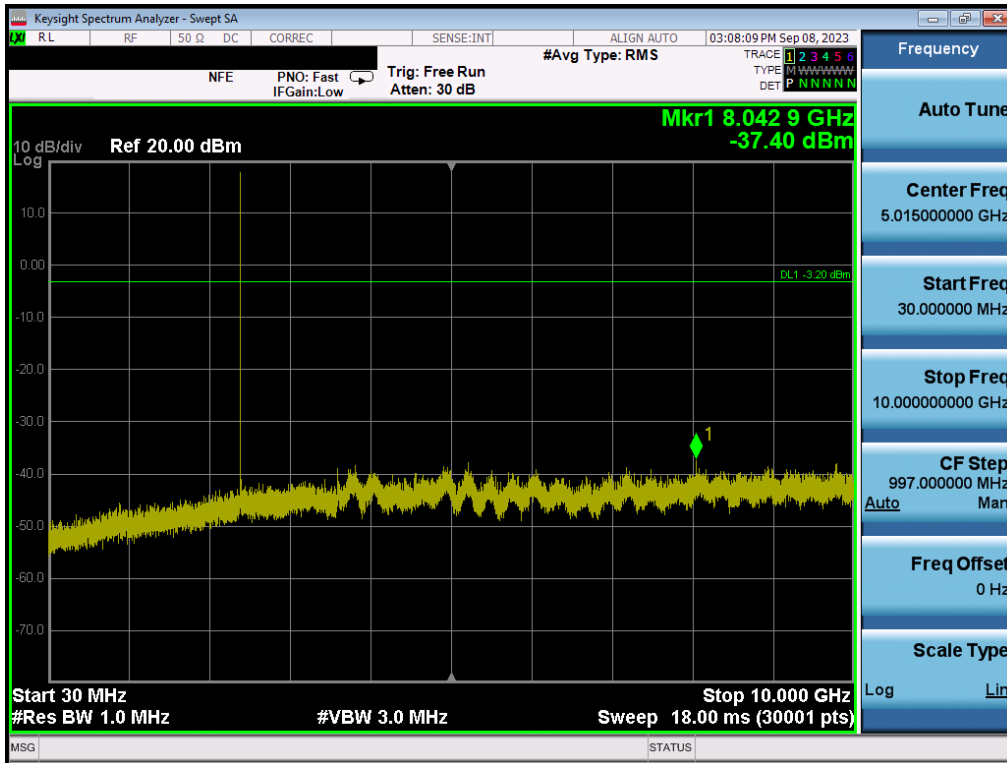
Plot 7-133. Conducted Spurious Plot (Bluetooth (LE), 1Mbps – Ch. 0) – ANT1
