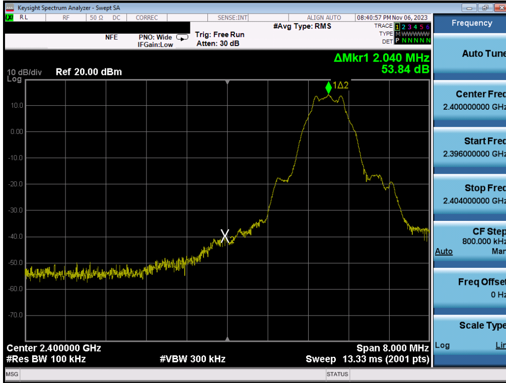
Plot 7-129. Band Edge Plot (Bluetooth (LE), 1Mbps – Ch. 0) – Dual ANT2
