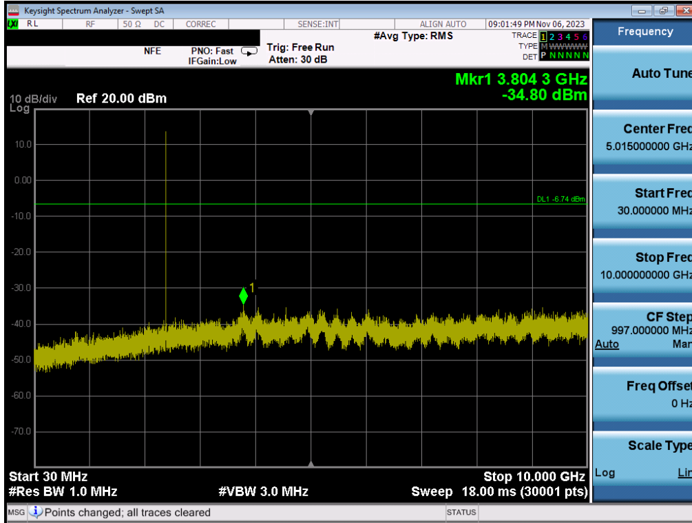
Plot 7-145. Conducted Spurious Plot (Bluetooth (LE), 1Mbps – Ch. 0) – Dual ANT1
