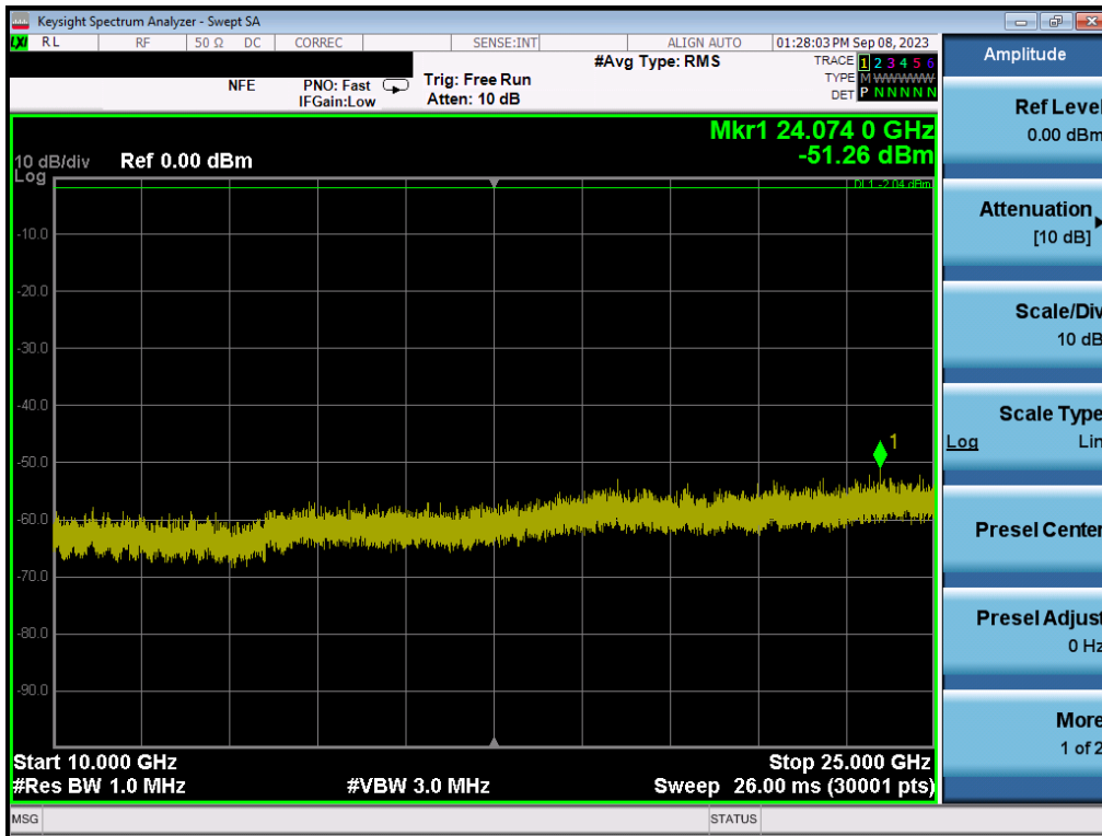
Plot 7-140. Conducted Spurious Plot (Bluetooth (LE), 1Mbps – Ch. 0) – ANT2
