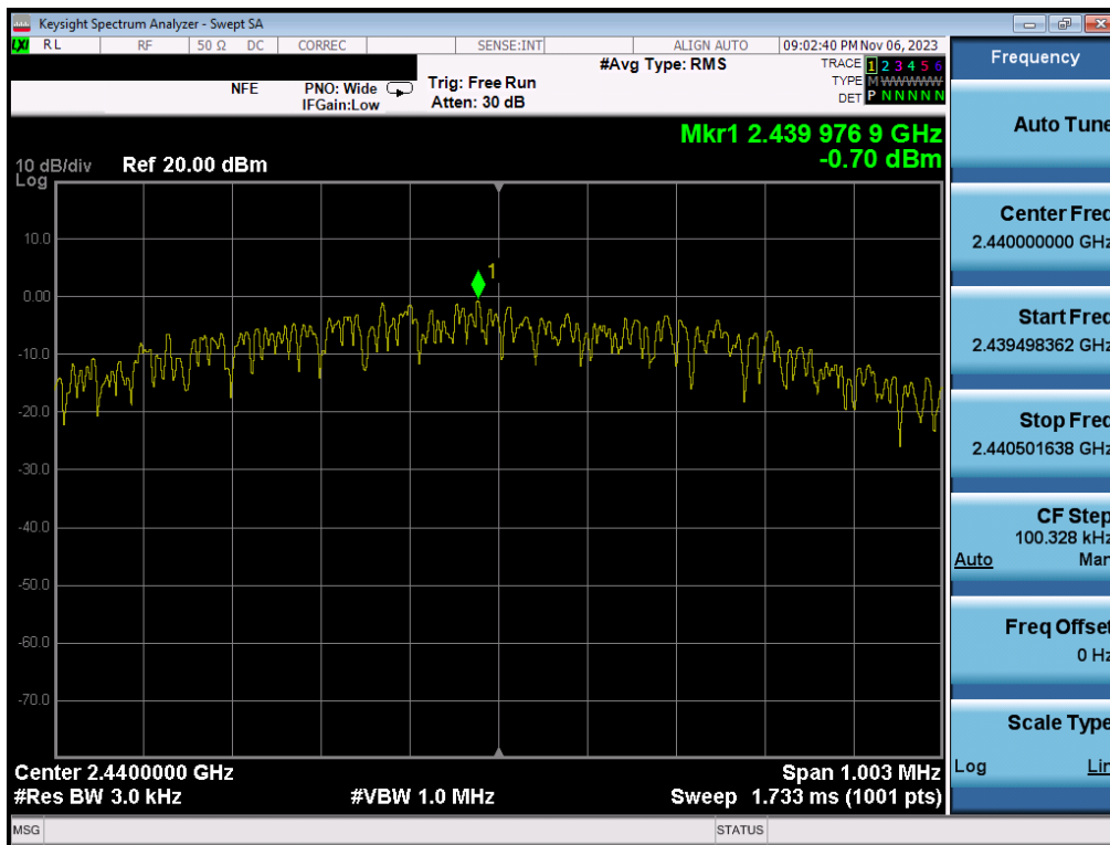
Plot 7-98. Power Spectral Density Plot (Bluetooth (LE), 1Mbps – Ch. 19 ) – Dual ANT1
