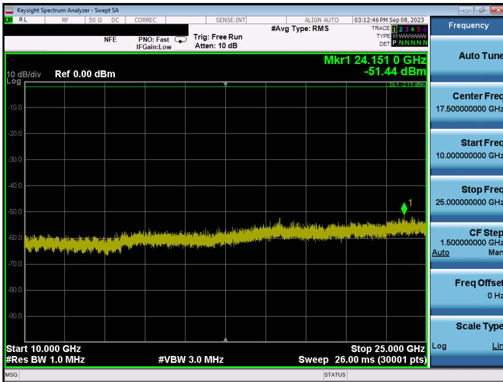
Plot 7-136. Conducted Spurious Plot (Bluetooth (LE), 1Mbps – Ch. 19) – ANT1
