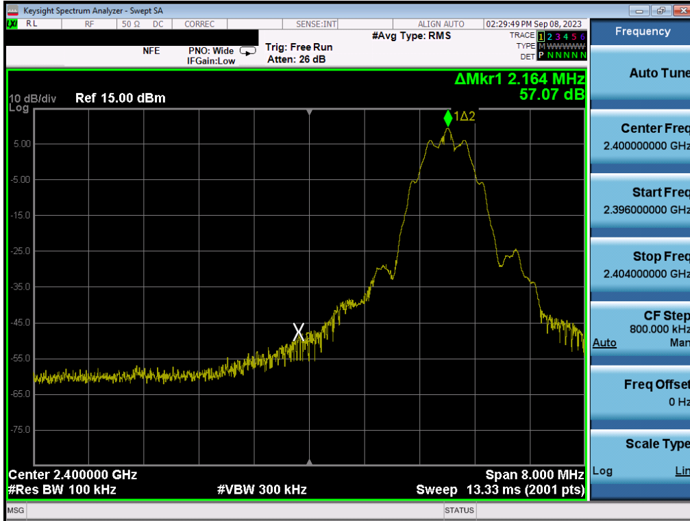
Plot 7-109. Band Edge Plot (Bluetooth (LE), 125kbps – Ch. 0) – ANT1
