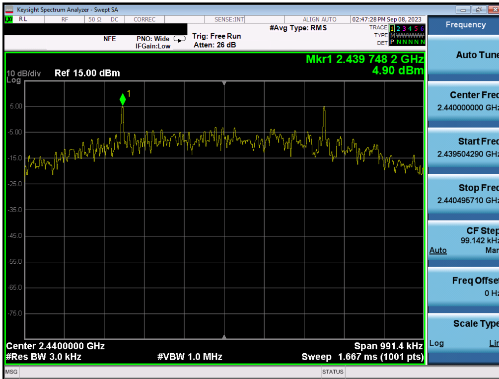
Plot 7-77. Power Spectral Density Plot (Bluetooth (LE), 500kbps – Ch. 19) – ANT1
