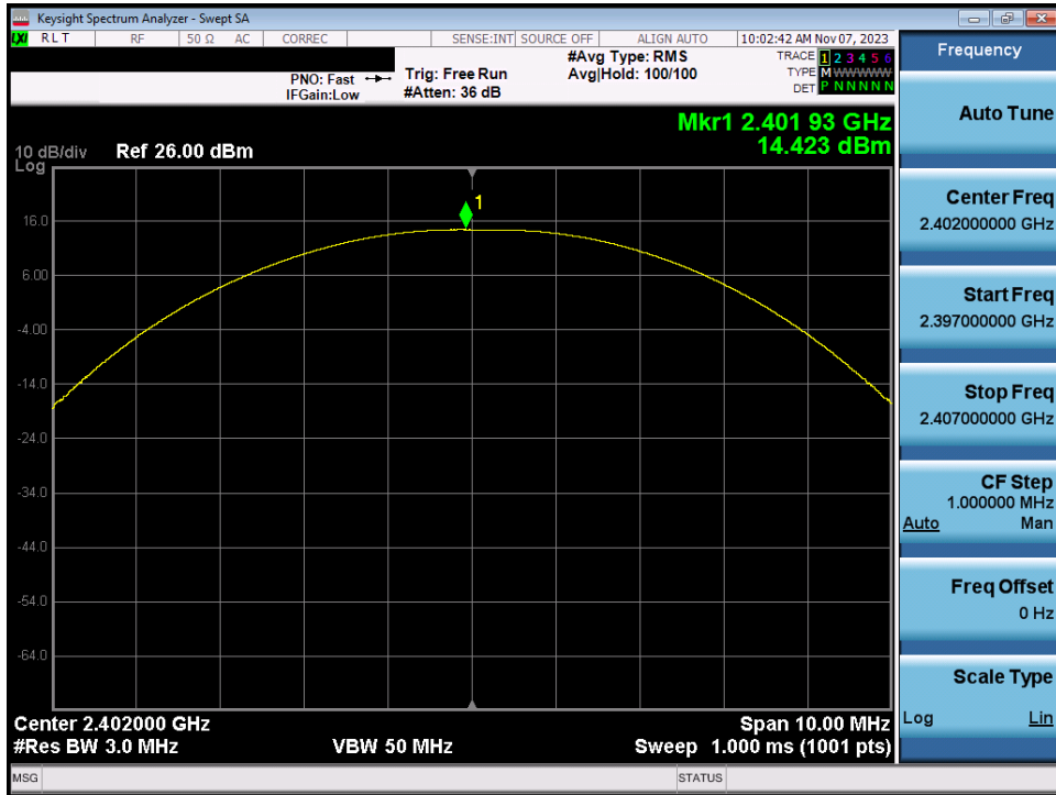
Plot 7-67. Peak Power Plot (Bluetooth (LE), 1Mbps – Ch. 0) – Dual ANT2
