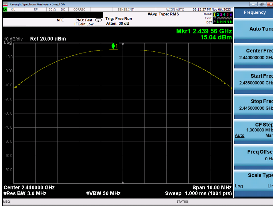
Plot 7-65. Peak Power Plot (Bluetooth (LE), 2Mbps – Ch. 19) – Dual ANT1
