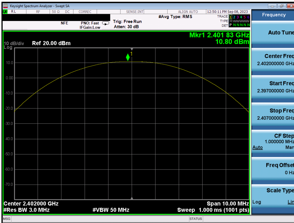
Plot 7-52. Peak Power Plot (Bluetooth (LE), 500kbps – Ch. 0) – ANT2
