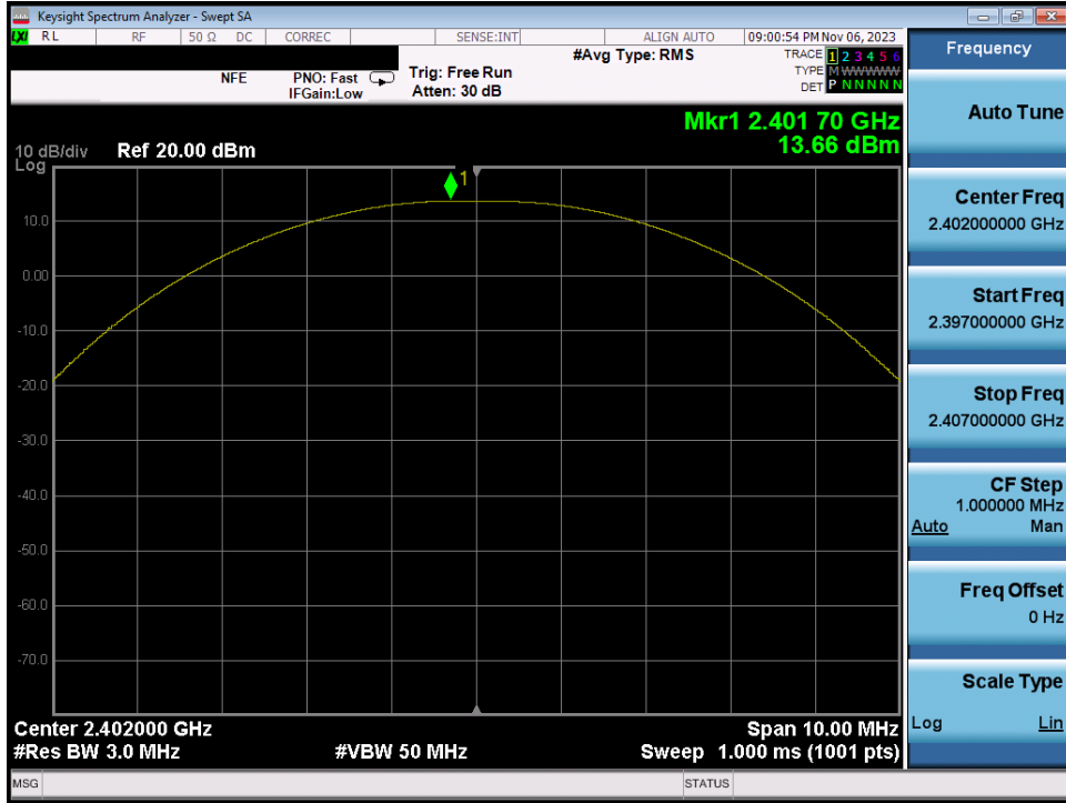
Plot 7-61. Peak Power Plot (Bluetooth (LE), 1Mbps – Ch. 0) – Dual ANT1
