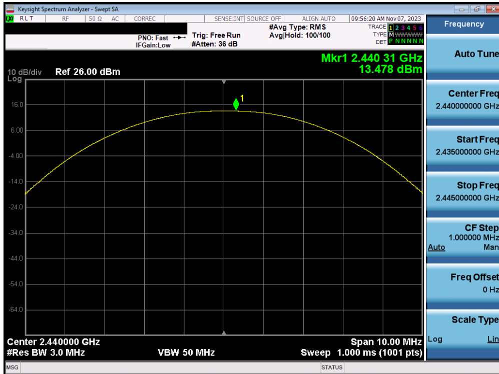
Plot 7-62. Peak Power Plot (Bluetooth (LE), 1Mbps – Ch. 19) – Dual ANT1
