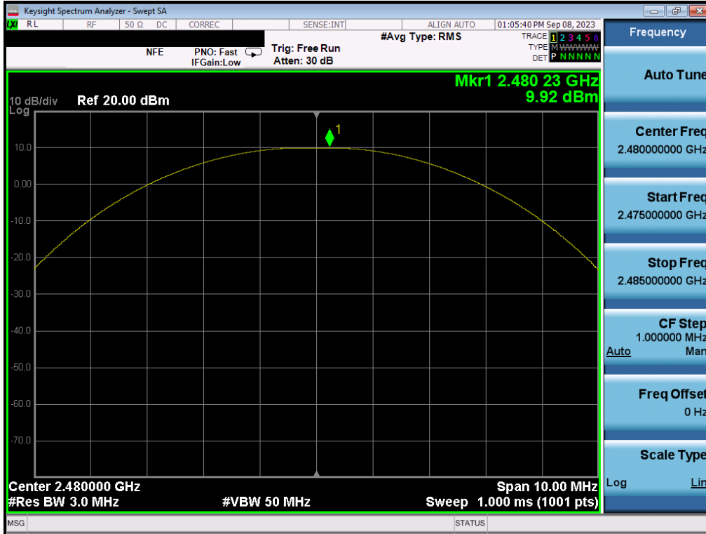
Plot 7-51. Peak Power Plot (Bluetooth (LE), 125kbps – Ch. 39) – ANT2
