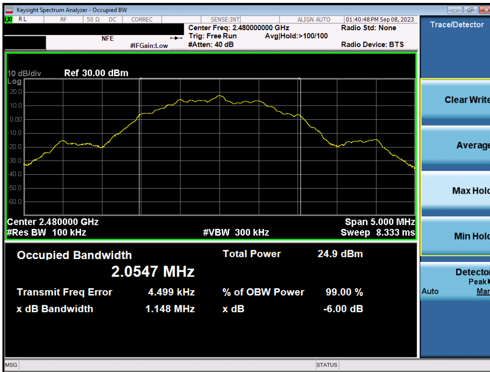
Plot 7-24. 6dB Bandwidth Plot (Bluetooth (LE), 2Mbps – Ch. 39 ANT2)
