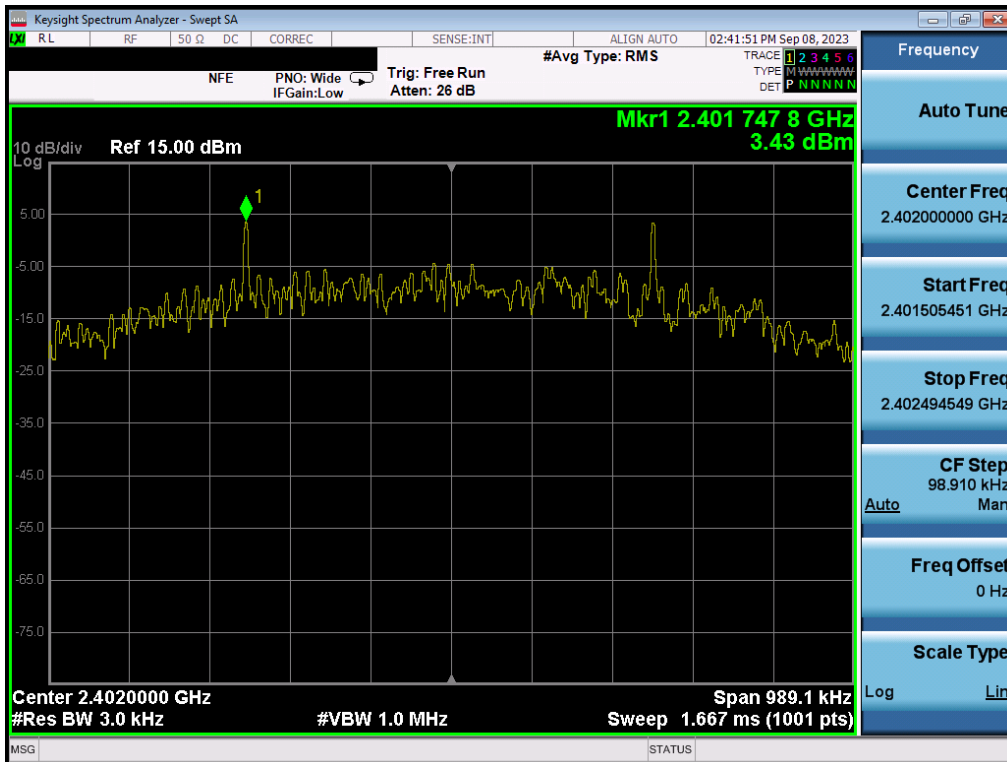
Plot 7-76. Power Spectral Density Plot (Bluetooth (LE), 500kbps – Ch. 0) – ANT1
