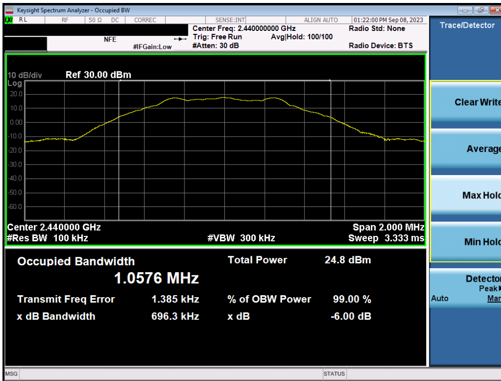
Plot 7-20. 6dB Bandwidth Plot (Bluetooth (LE), 1Mbps – Ch. 19 ANT2)
