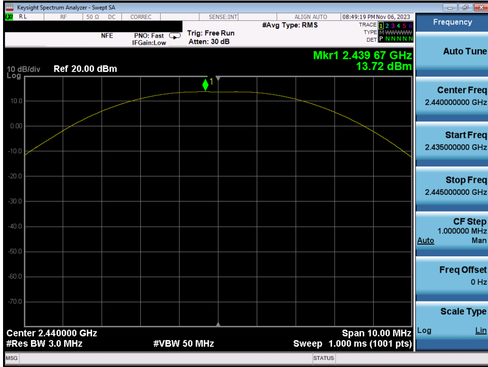
Plot 7-71. Peak Power Plot (Bluetooth (LE), 2Mbps – Ch. 19) – Dual ANT2
