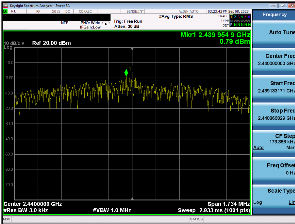
Plot 7-83. Power Spectral Density Plot (Bluetooth (LE), 2Mbps – Ch. 19 ) – ANT1
