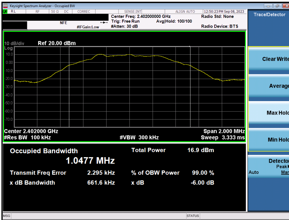
Plot 7-16. 6dB Bandwidth Plot (Bluetooth (LE), 500kbps – Ch. 0 ANT2)
