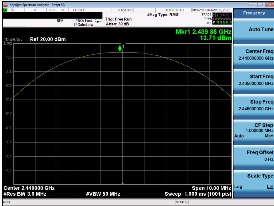
Plot 7-68. Peak Power Plot (Bluetooth (LE), 1Mbps – Ch. 19) – Dual ANT2
