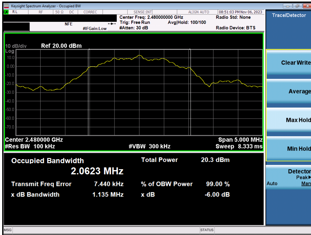
Plot 7-36. 6dB Bandwidth Plot (Bluetooth (LE), 2Mbps – Ch. 39 DUAL ANT2)
