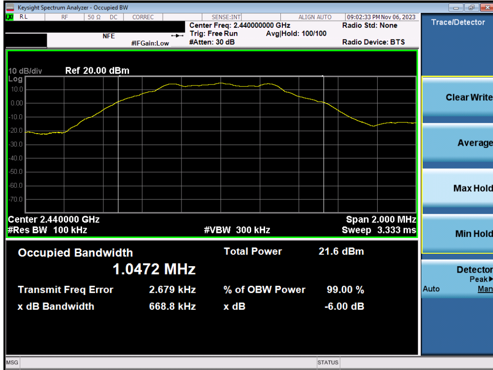
Plot 7-26. 6dB Bandwidth Plot (Bluetooth (LE), 1Mbps – Ch. 19 DUAL ANT1)
