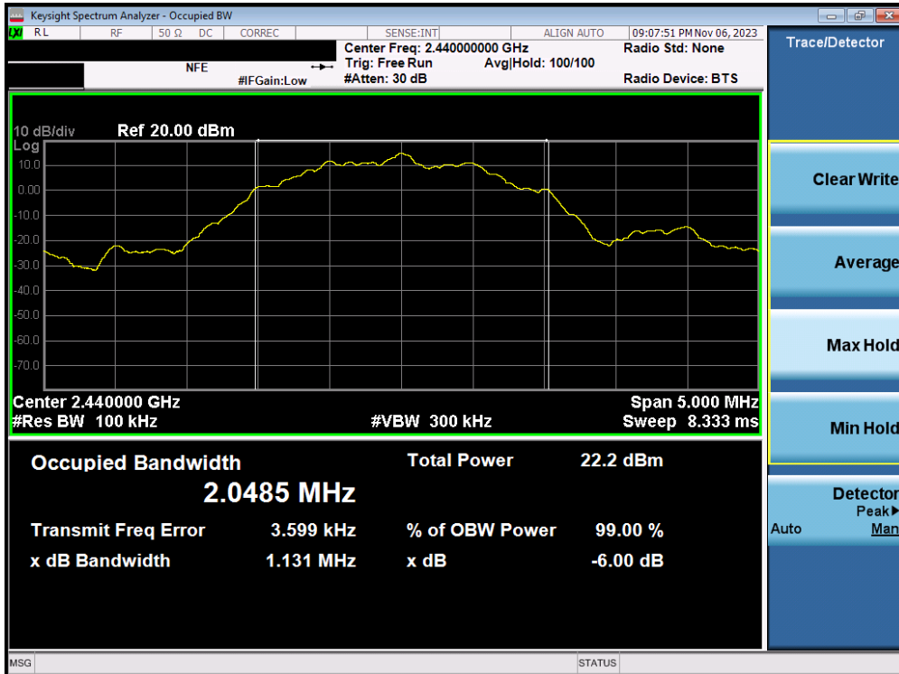
Plot 7-29. 6dB Bandwidth Plot (Bluetooth (LE), 2Mbps – Ch. 19 DUAL ANT1)
