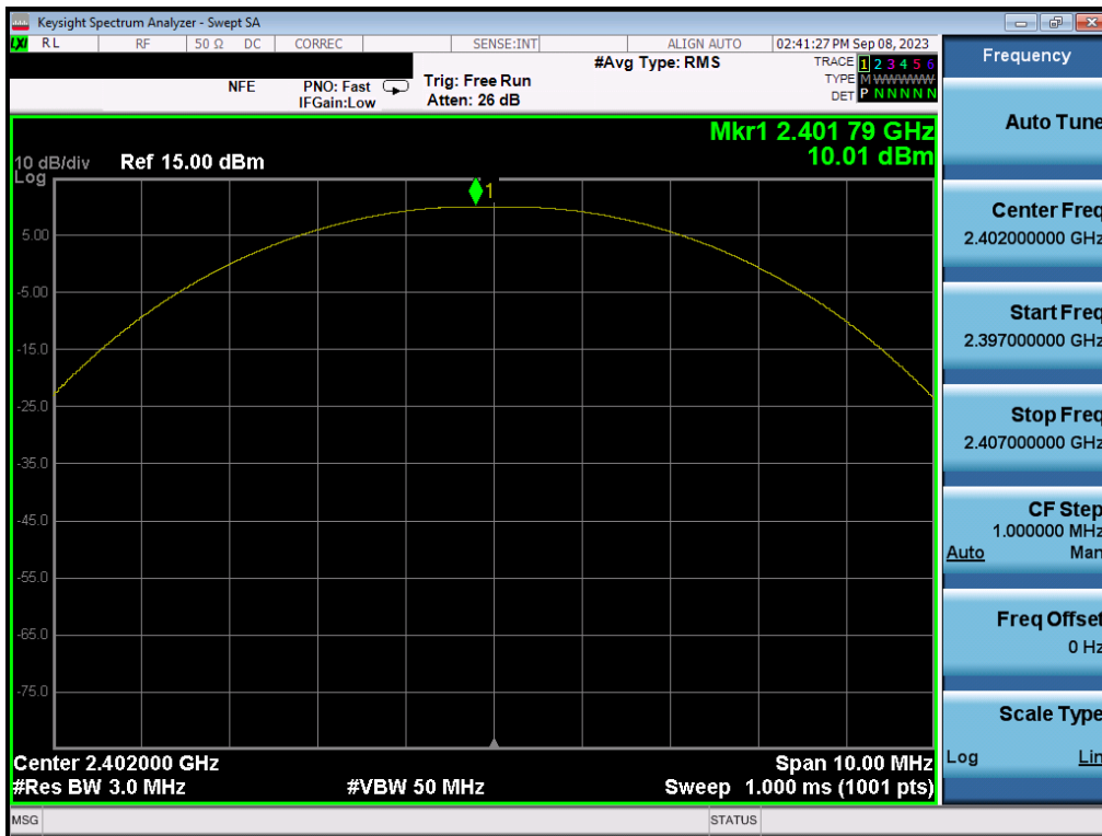
Plot 7-40. Peak Power Plot (Bluetooth (LE), 500kbps – Ch. 0) – ANT1
