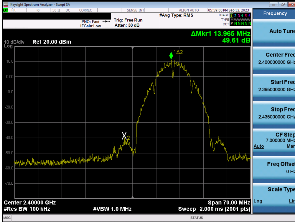
Plot 7-97. Band Edge Plot SISO ANT1 (802.11b – Ch. 1)
