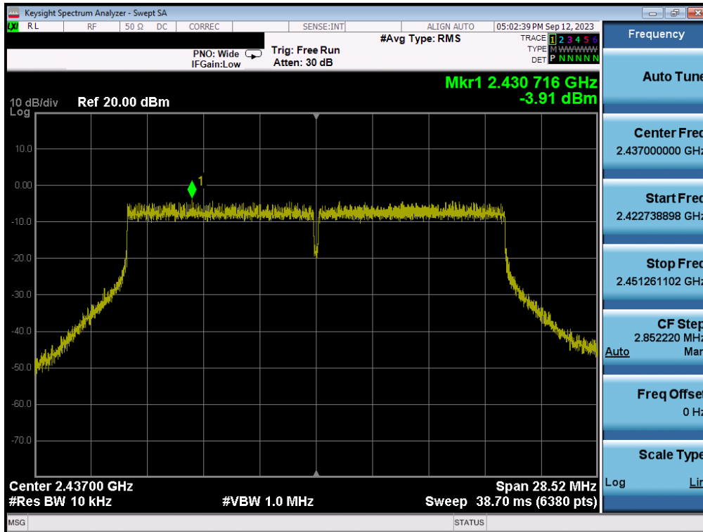
Plot 7-83. Power Spectral Density Plot MIMO ANT1 (802.11be (2.4GHz) – Ch. 6)
