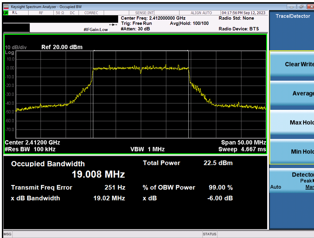
Plot 7-22. 6dB Bandwidth Plot SISO ANT2 (802.11be (2.4GHz) – Ch. 1)
