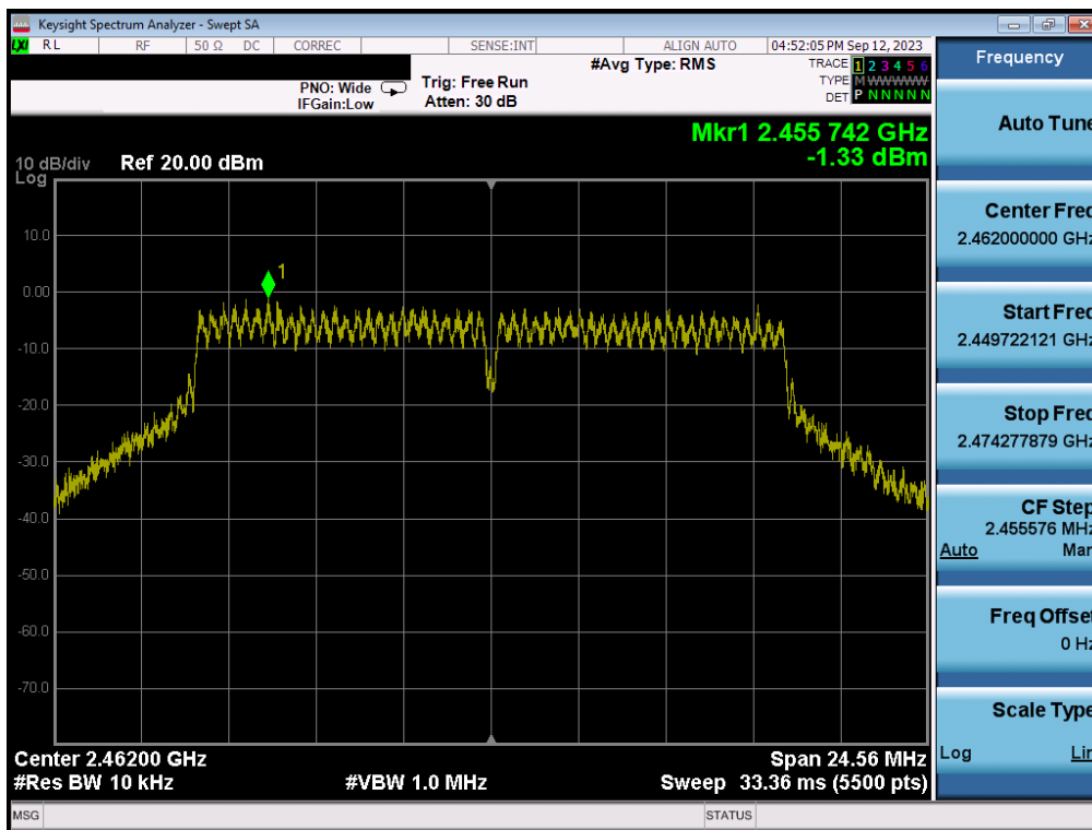
Plot 7-66. Power Spectral Density Plot SISO ANT2 (802.11g – Ch. 11)
