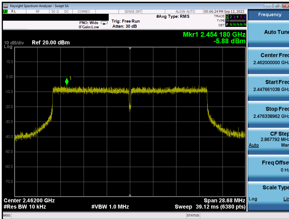
Plot 7-84. Power Spectral Density Plot MIMO ANT1 (802.11be (2.4GHz) – Ch. 11)
