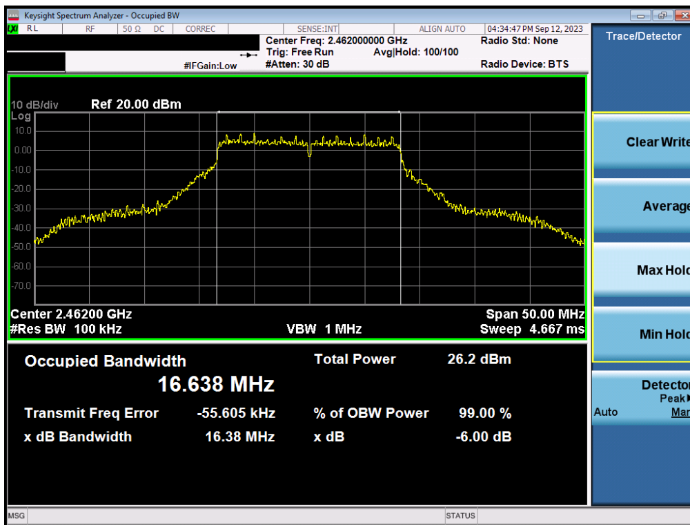
Plot 7-42. 6dB Bandwidth Plot MIMO ANT2 (802.11g – Ch. 11)
