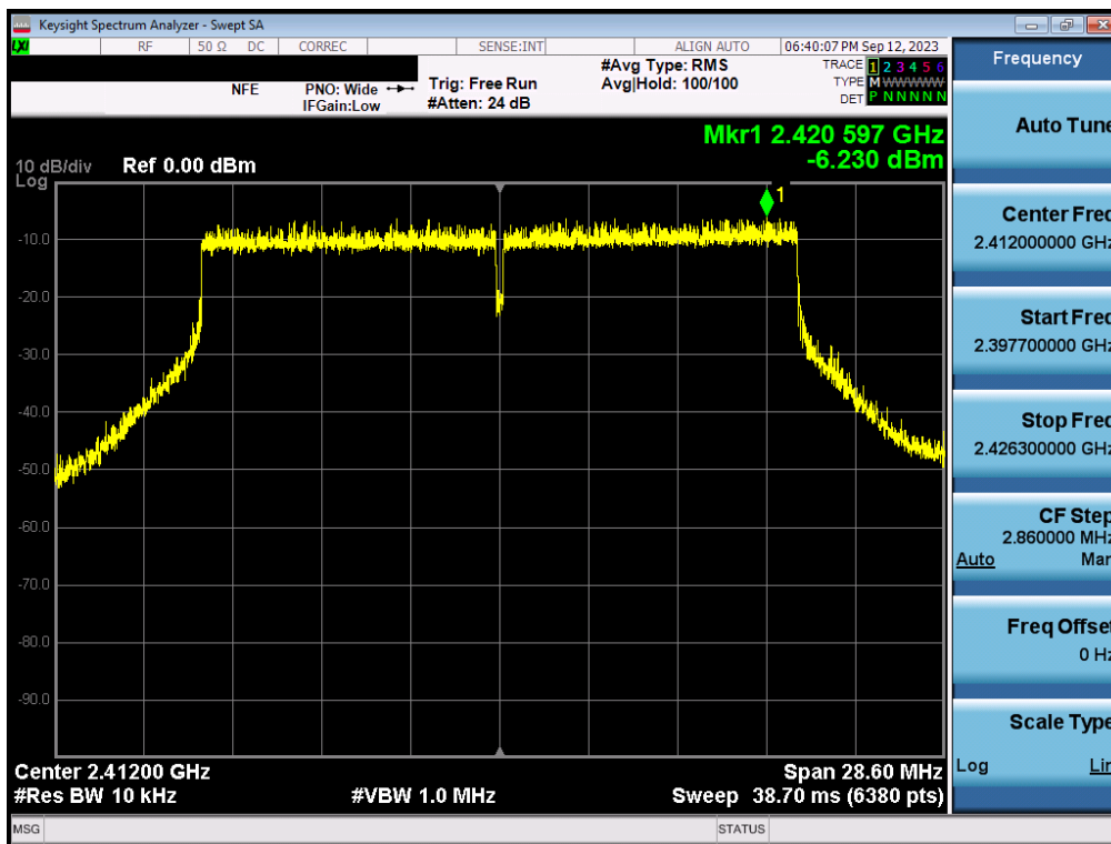
Plot 7-94. Power Spectral Density Plot MIMO ANT2 (802.11be (2.4GHz) – Ch. 1)
