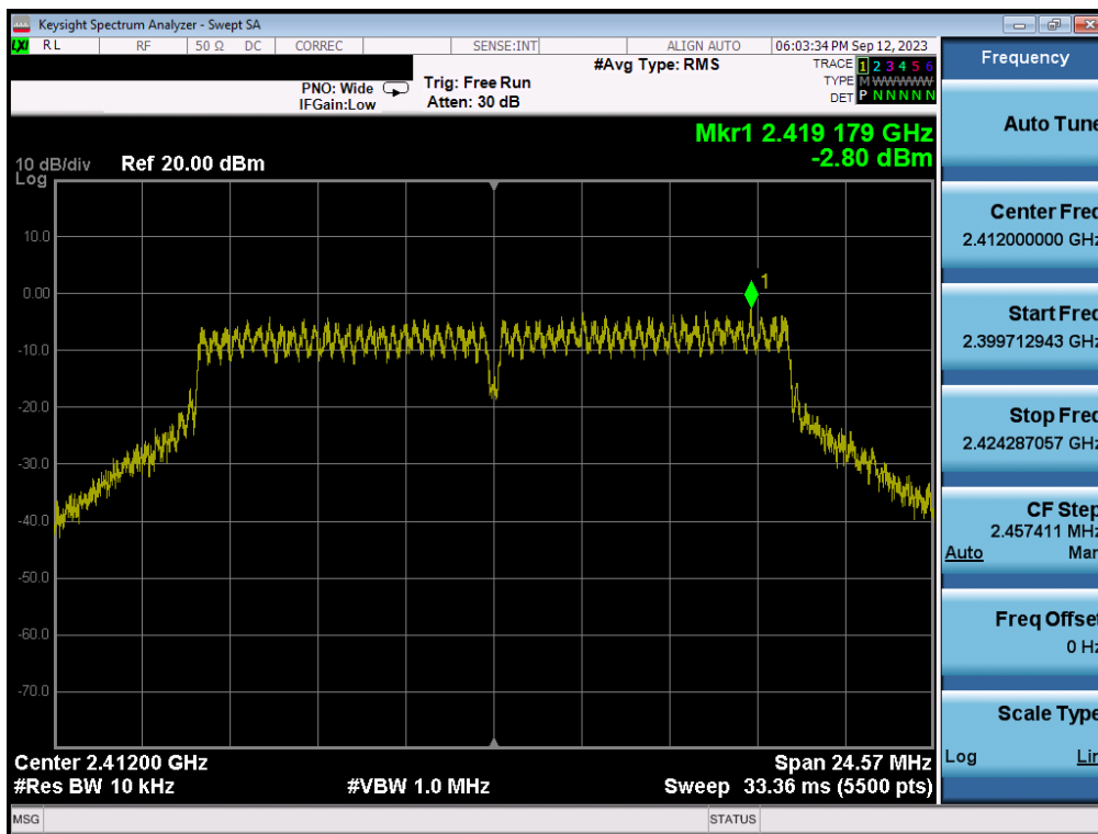
Plot 7-52. Power Spectral Density Plot SISO ANT1 (802.11g – Ch. 1)
