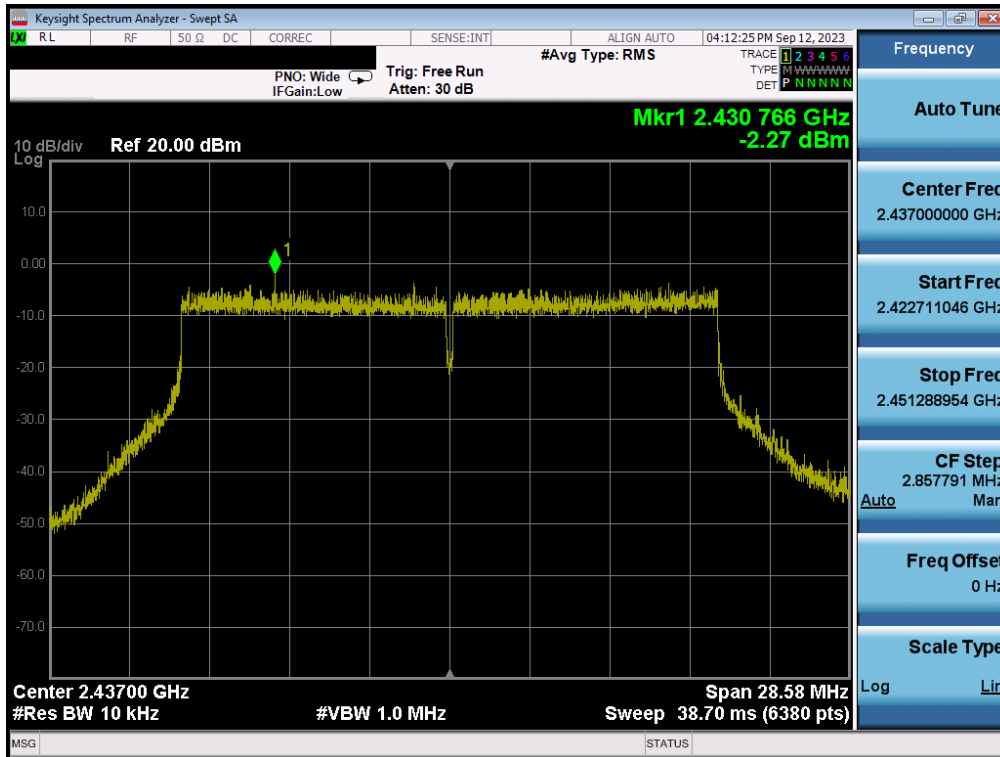
Plot 7-95. Power Spectral Density Plot MIMO ANT2 (802.11be (2.4GHz) – Ch. 6)
