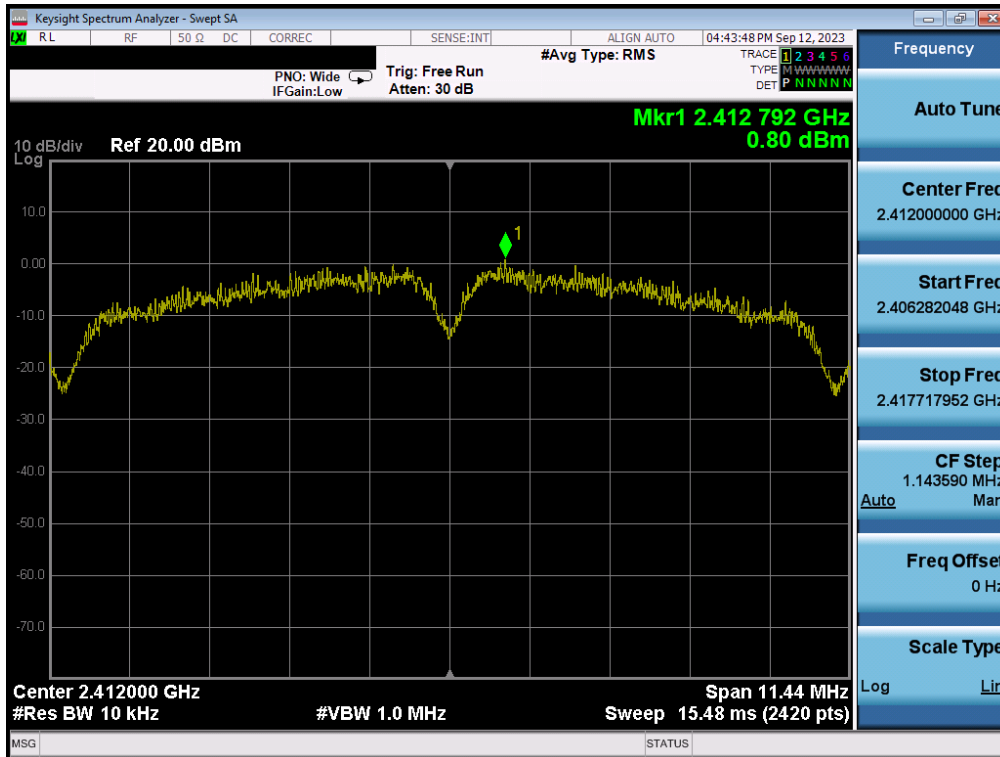
Plot 7-61. Power Spectral Density Plot SISO ANT2 (802.11b – Ch. 1)
