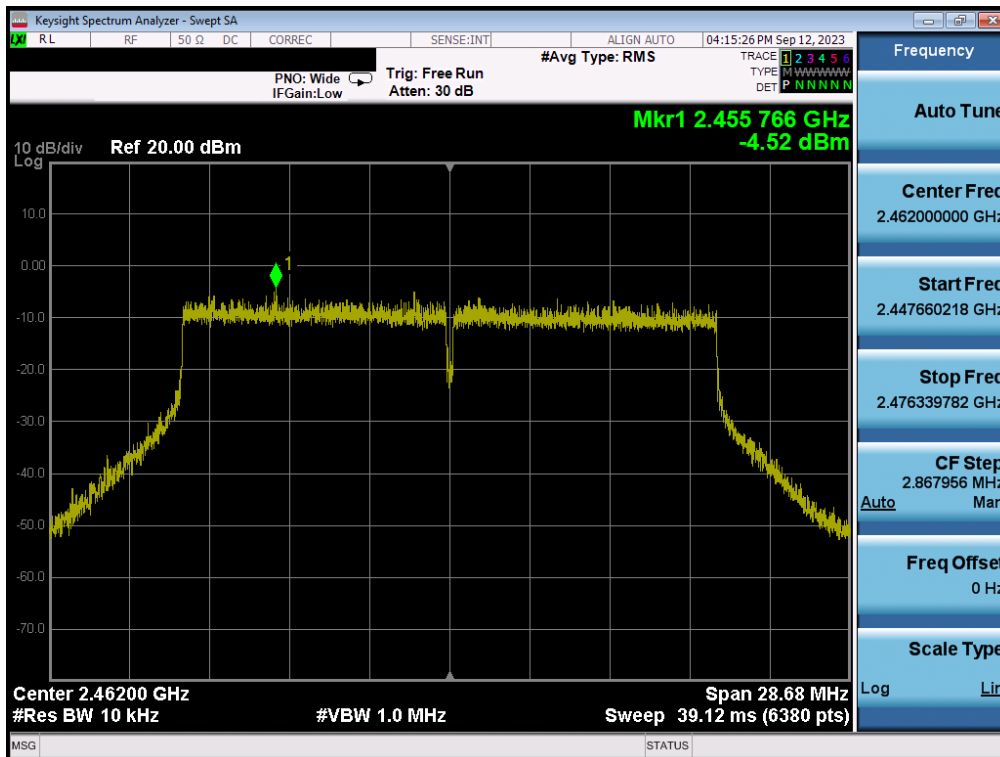
Plot 7-96. Power Spectral Density Plot MIMO ANT2 (802.11be (2.4GHz) – Ch. 11)
