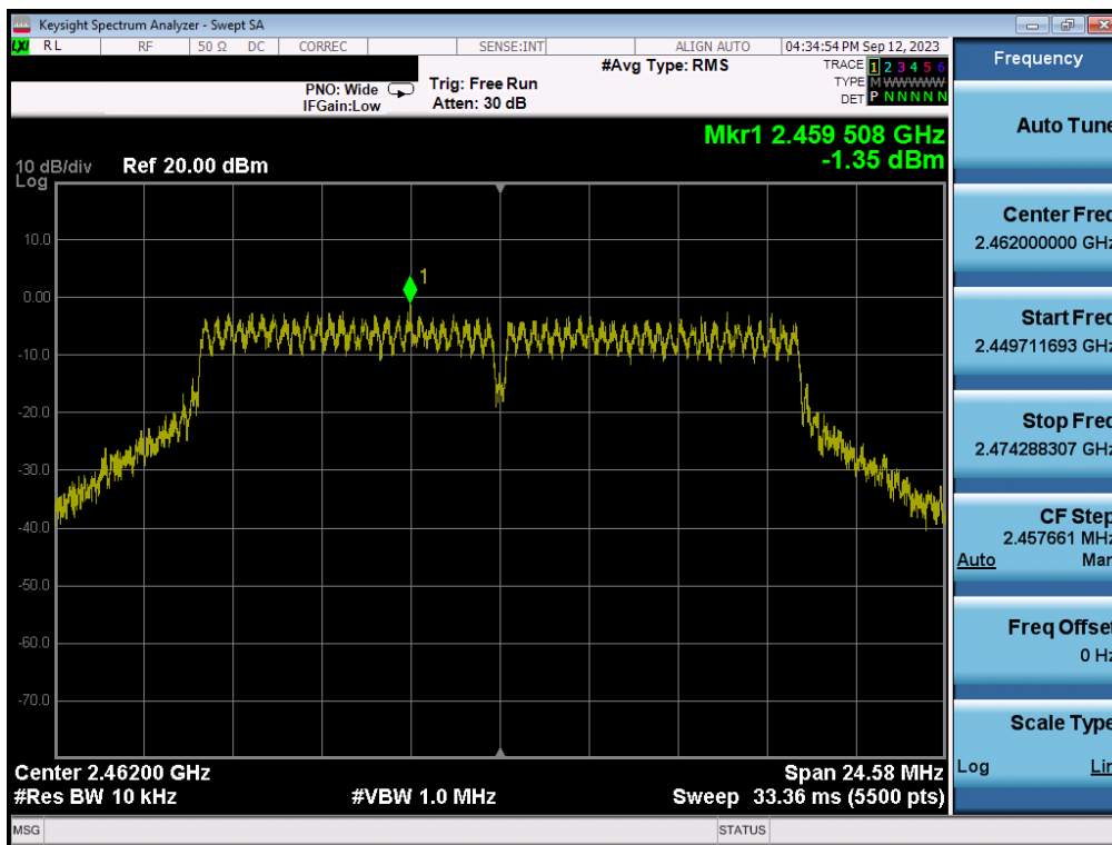
Plot 7-90. Power Spectral Density Plot MIMO ANT2 (802.11g – Ch. 11)
