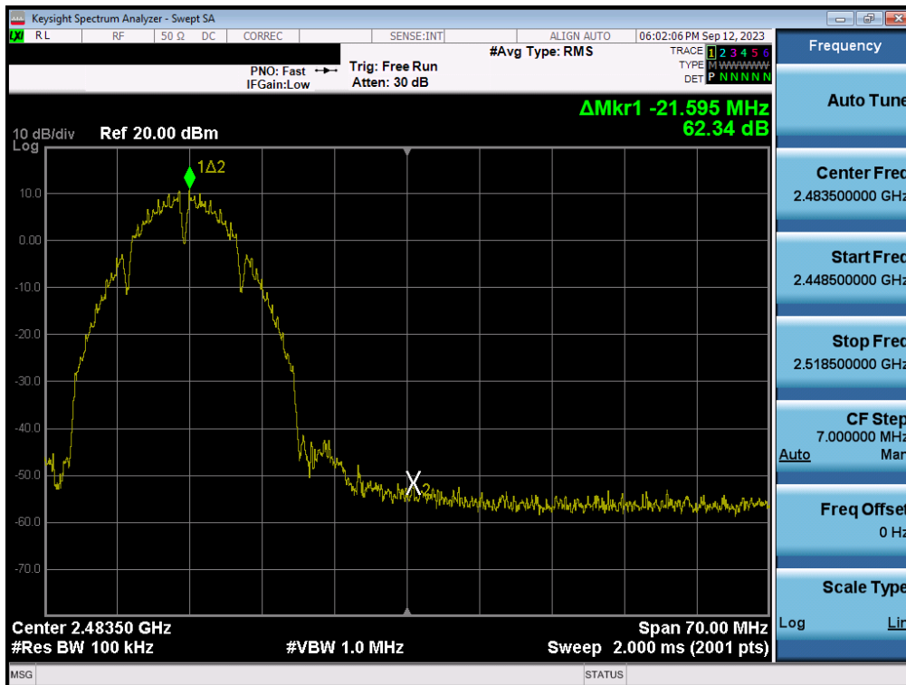
Plot 7-98. Band Edge Plot SISO ANT1 (802.11b – Ch. 11)
