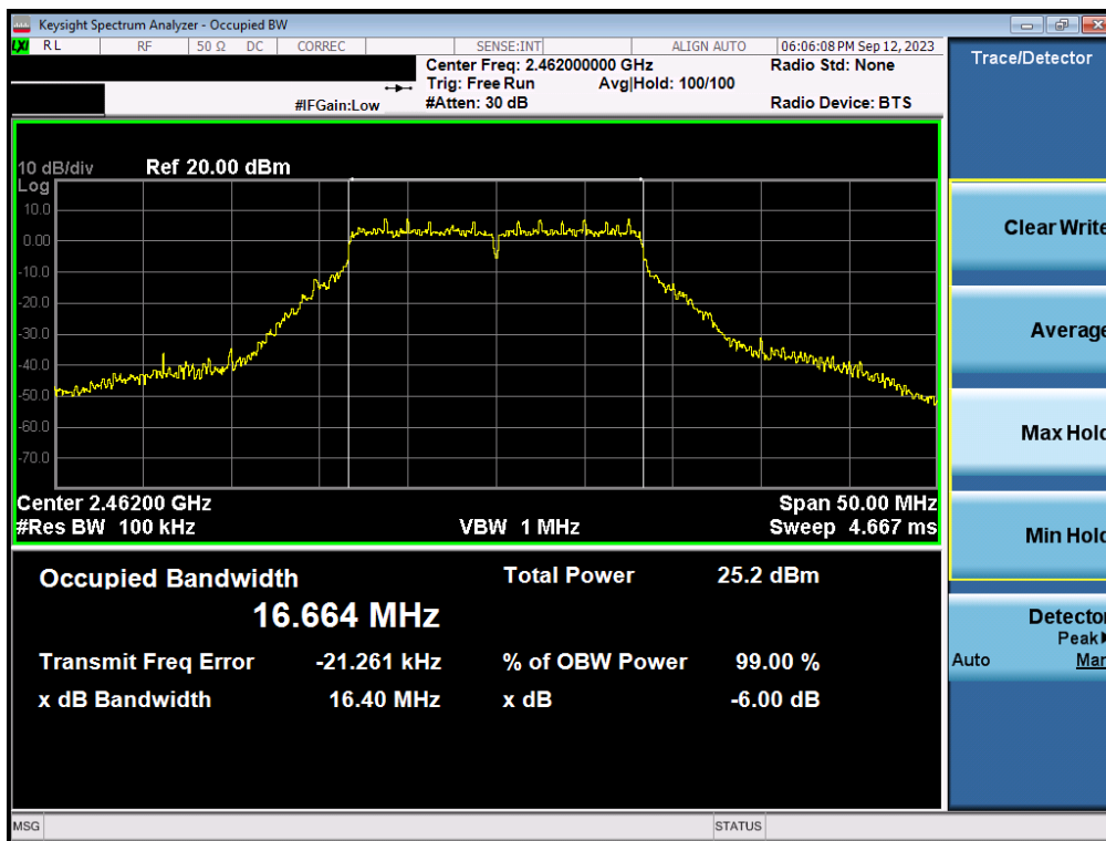
Plot 7-6. 6dB Bandwidth Plot SISO ANT1 (802.11g – Ch. 11)
