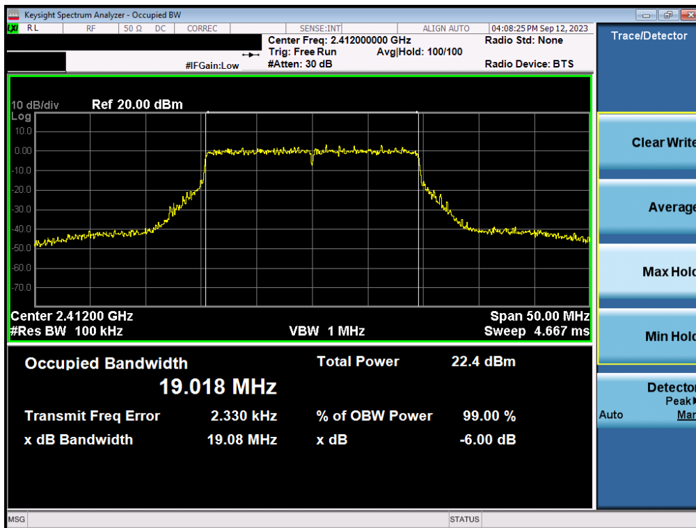
Plot 7-46. 6dB Bandwidth Plot MIMO ANT2 (802.11be (2.4GHz) – Ch. 1)
