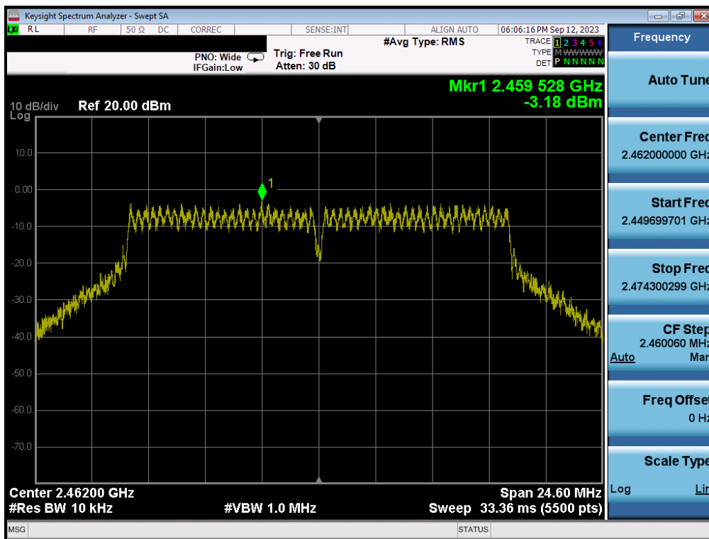
Plot 7-54. Power Spectral Density Plot SISO ANT1 (802.11g – Ch. 11)
