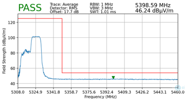
Plot 7-161. Radiated Upper Band Edge Plot MIMO (Average – UNII Band 2A – 106 Tones)
