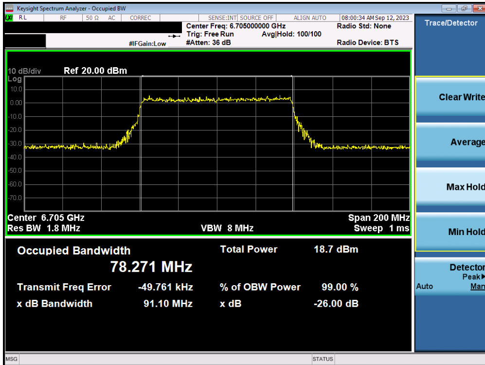
Plot 7-17. 26dB Bandwidth Plot MIMO ANT1 (80MHz 802.11ax/be (UNII Band 7) – Ch. 151)
