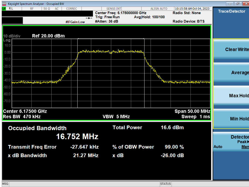
Plot 7-26. 26dB Bandwidth Plot MIMO ANT2 (20MHz 802.11a (UNII Band 5) – Ch. 45)
