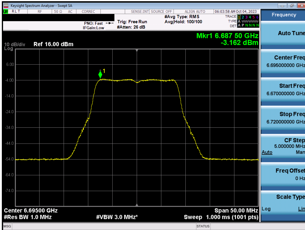
Plot 7-68. Power Spectral Density MIMO ANT1 (20MHz 802.11a (UNII Band 7) – Ch. 149) - LPI
