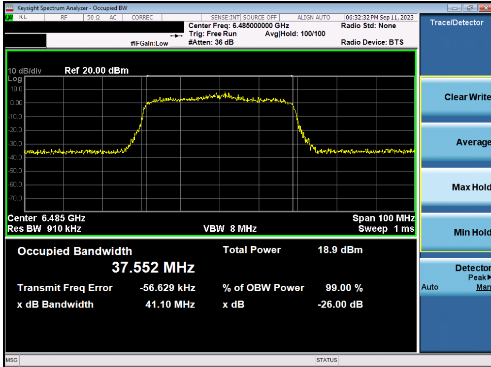
Plot 7-34. 26dB Bandwidth Plot MIMO ANT2 (40MHz 802.11ax/be (UNII Band 6) – Ch. 107)
