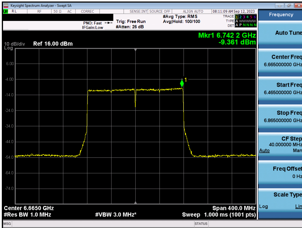
Plot 7-72. Power Spectral Density MIMO ANT1 (160MHz 802.11ax/be (UNII Band 7) – Ch. 143) - LPI
