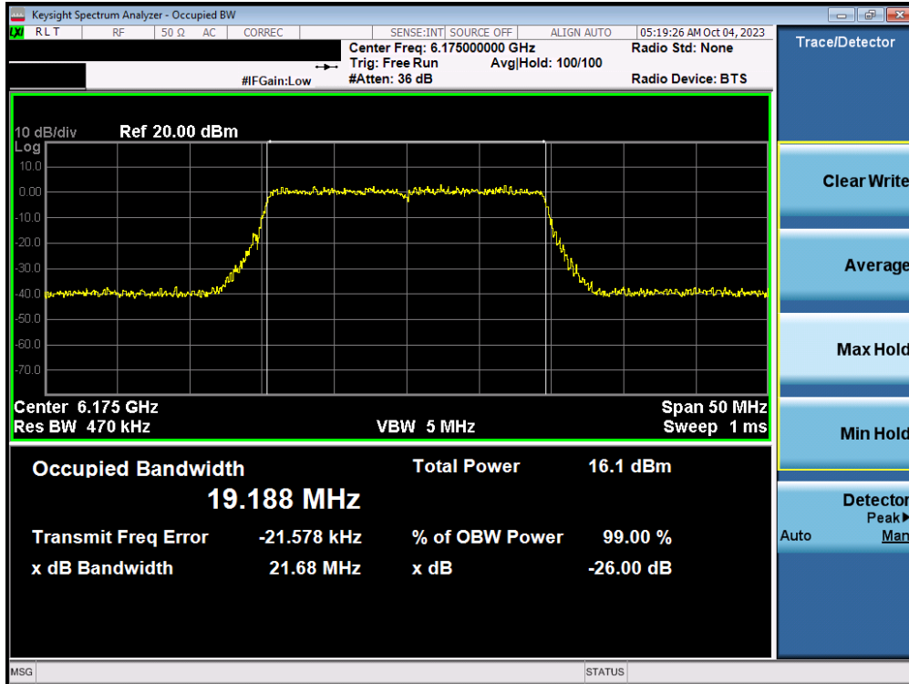
Plot 7-3. 26dB Bandwidth Plot MIMO ANT1 (20MHz 802.11ax/be (UNII Band 5) – Ch. 45)
