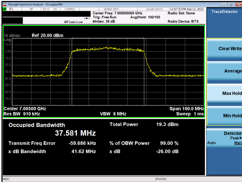
Plot 7-46. 26dB Bandwidth Plot MIMO ANT2 (40MHz 802.11ax/be (UNII Band 8) – Ch. 211)
