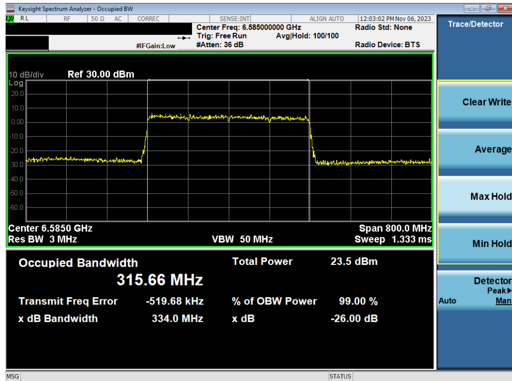
Plot 7-43. 26dB Bandwidth Plot MIMO ANT2 (320MHz 802.11ax/be (UNII Band 6/7) – Ch. 127)
