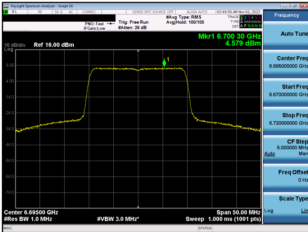
Plot 7-75. Power Spectral Density MIMO ANT1 (20MHz 802.11ax/be (UNII Band 7) – Ch. 149) - SP
