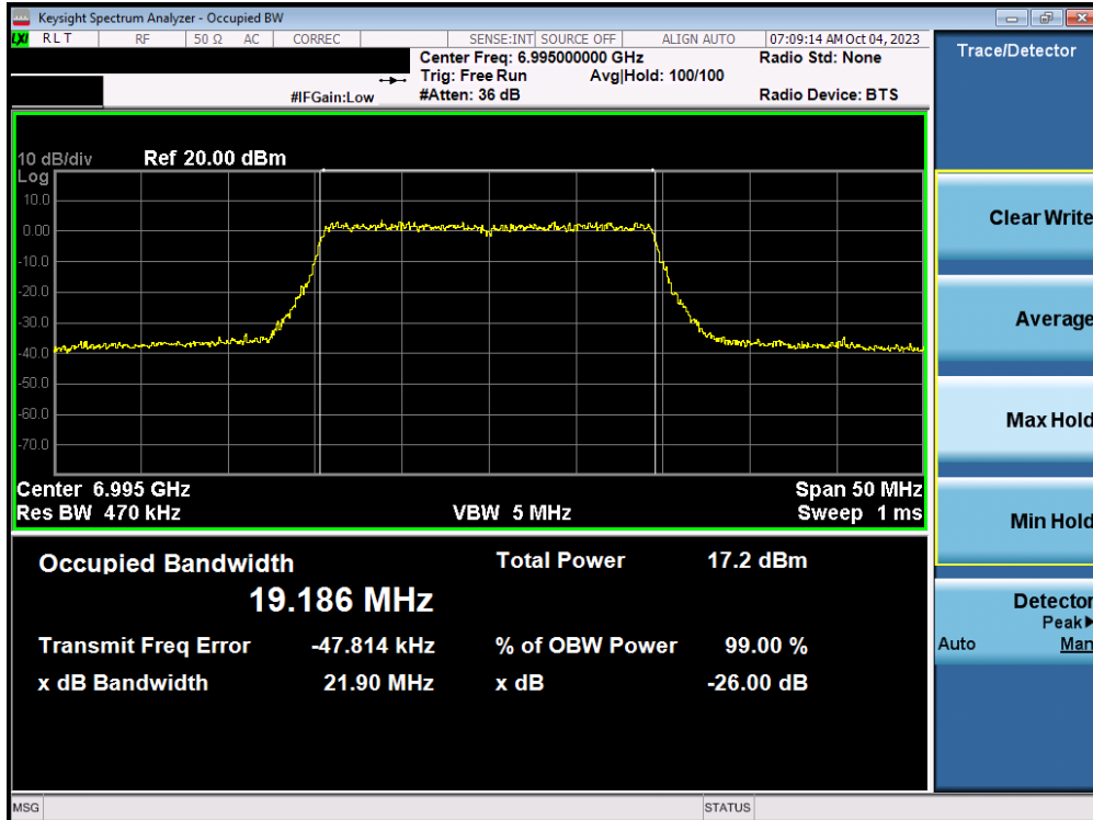
Plot 7-21. 26dB Bandwidth Plot MIMO ANT1 (20MHz 802.11ax/be (UNII Band 8) – Ch. 209)
