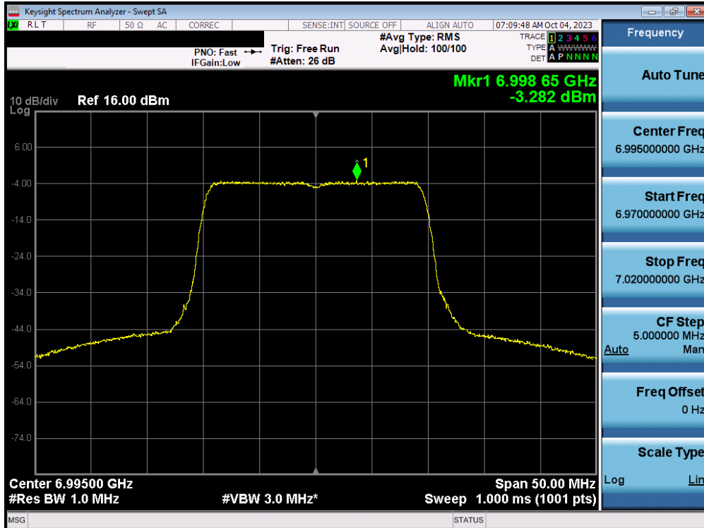
Plot 7-81. Power Spectral Density MIMO ANT1 (20MHz 802.11ax/be (UNII Band 8) – Ch. 209) - LPI
