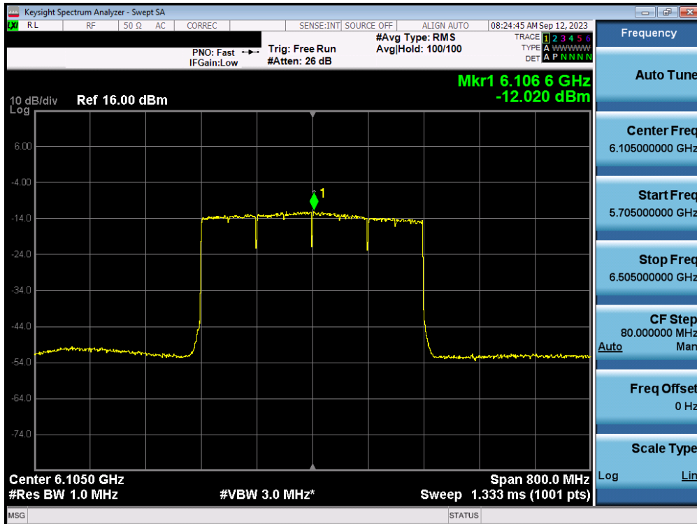
Plot 7-55. Power Spectral Density MIMO ANT1 (320MHz 802.11ax/be (UNII Band 5) – Ch.31) - LPI
