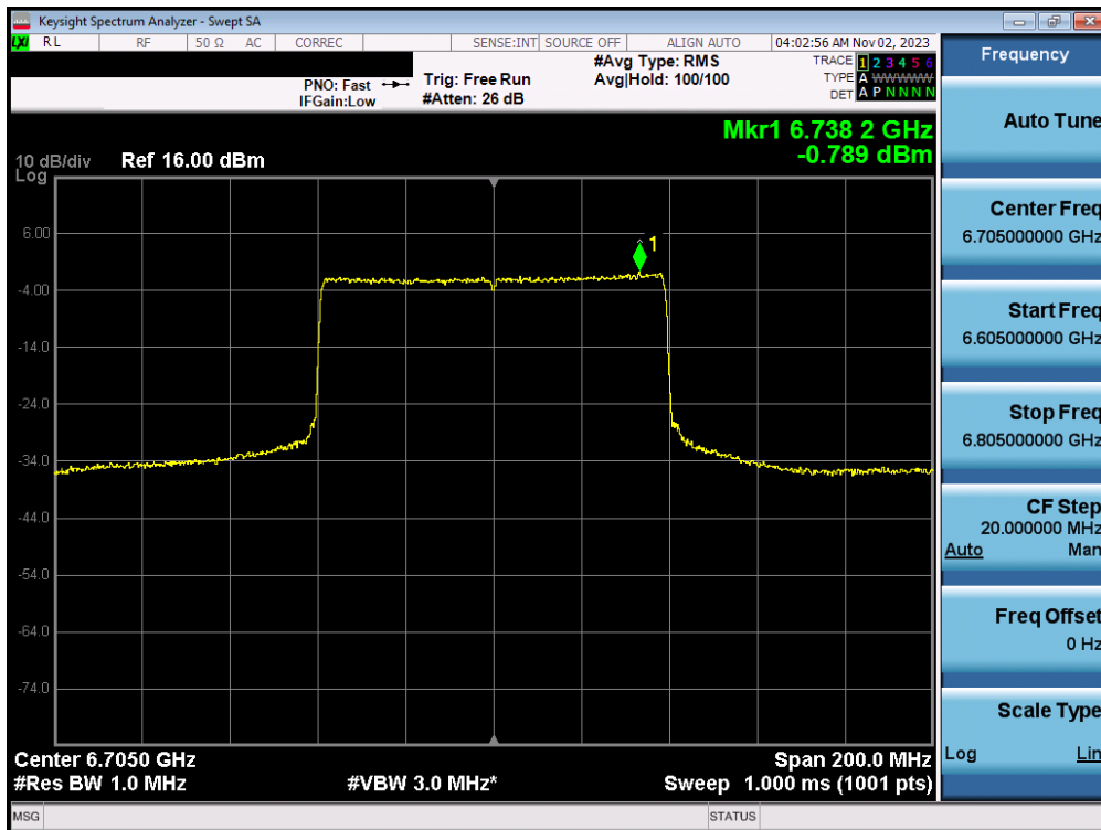
Plot 7-77. Power Spectral Density MIMO ANT1 (80MHz 802.11ax/be (UNII Band 7) – Ch. 151) - SP
