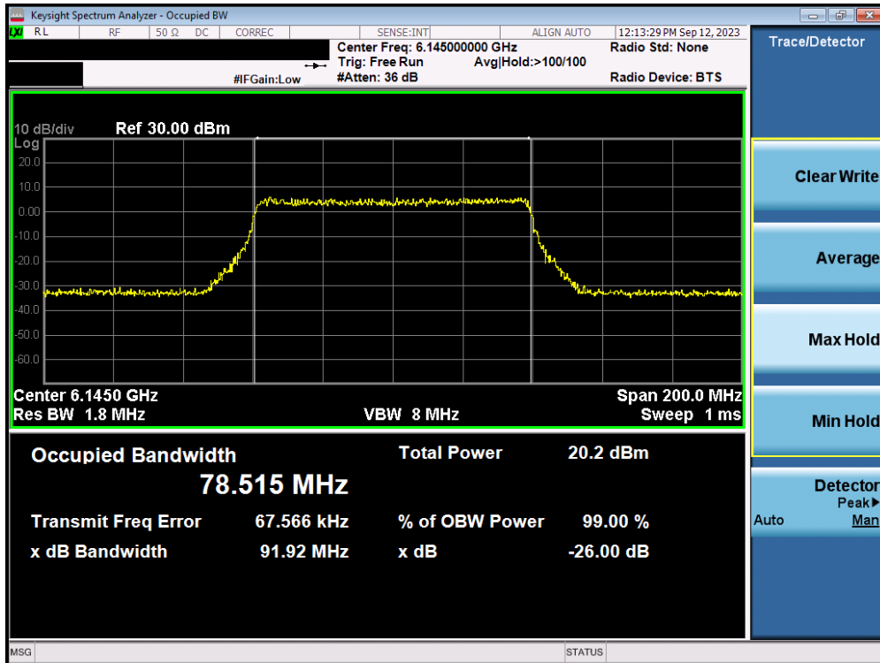
Plot 7-29. 26dB Bandwidth Plot MIMO ANT2 (80MHz 802.11ax/be (UNII Band 5) – Ch. 39)
