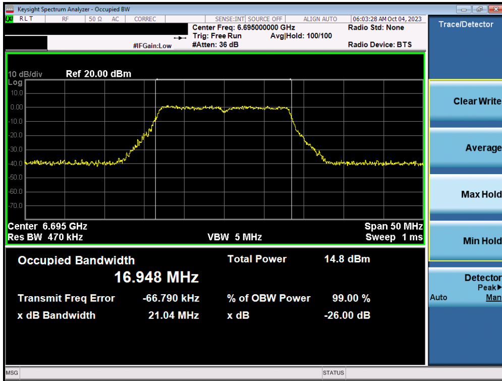
Plot 7-14. 26dB Bandwidth Plot MIMO ANT1 (20MHz 802.11a (UNII Band 7) – Ch. 149)
