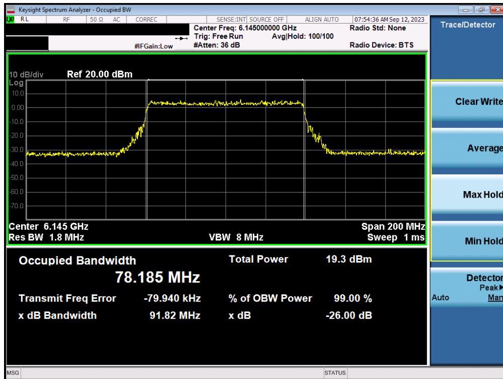
Plot 7-5. 26dB Bandwidth Plot MIMO ANT1 (80MHz 802.11ax/be (UNII Band 5) – Ch. 39)
