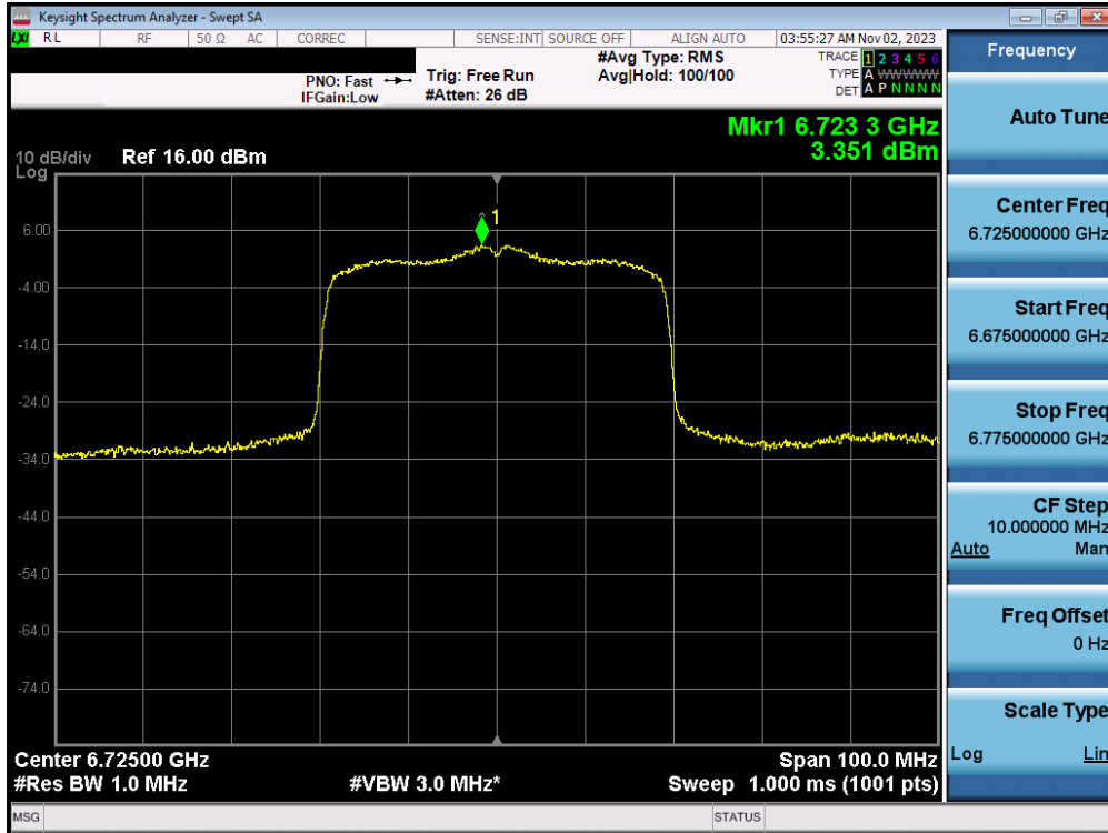
Plot 7-76. Power Spectral Density MIMO ANT1 (40MHz 802.11ax/be (UNII Band 7) – Ch. 155) - SP
