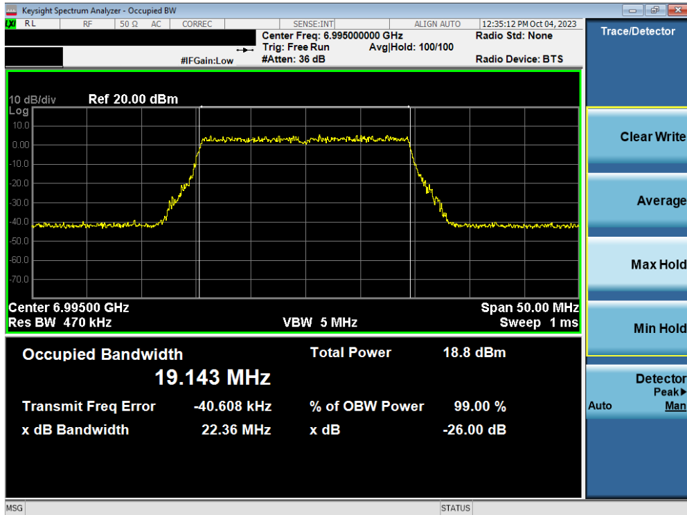
Plot 7-45. 26dB Bandwidth Plot MIMO ANT2 (20MHz 802.11ax/be (UNII Band 8) – Ch. 209)
