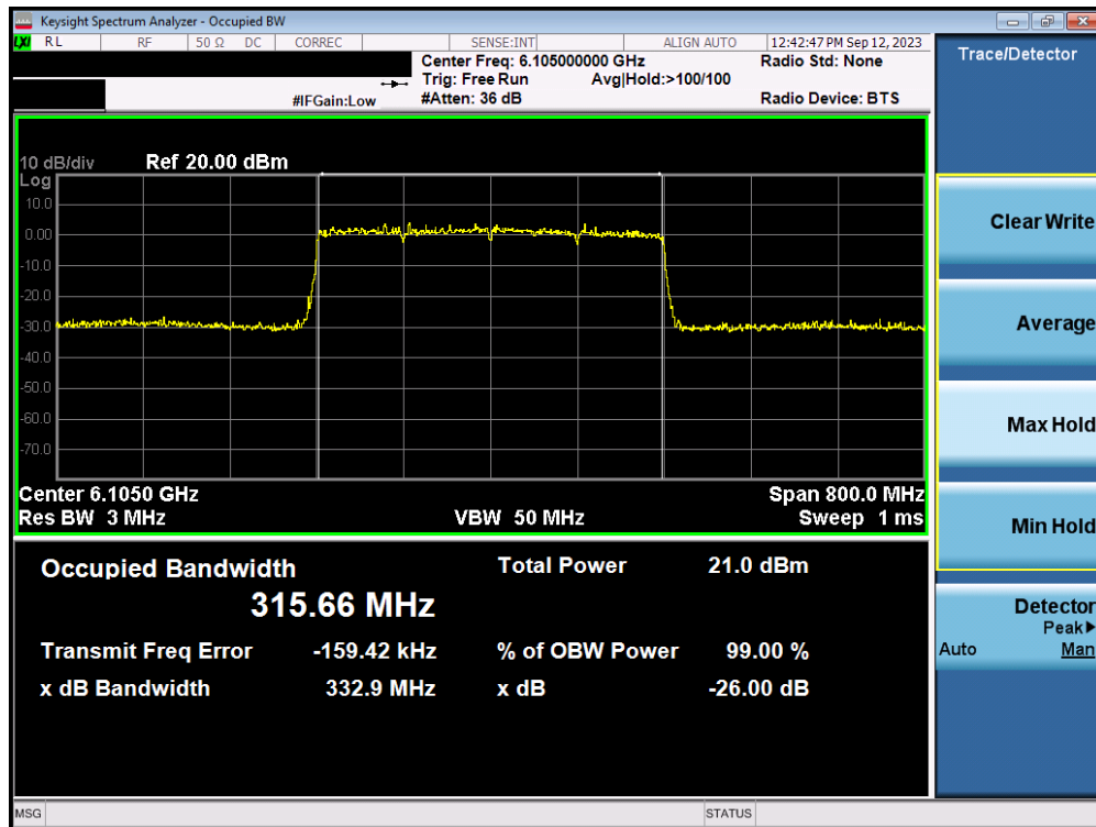
Plot 7-31. 26dB Bandwidth Plot MIMO ANT2 (320MHz 802.11ax/be (UNII Band 5) – Ch.31)
