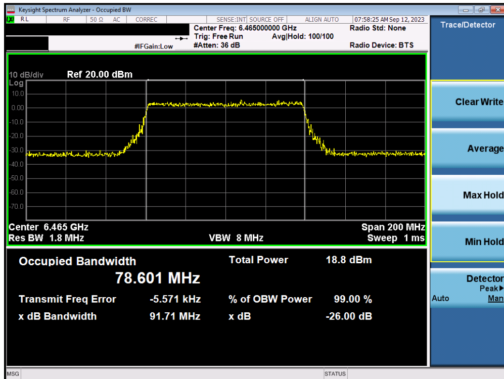
Plot 7-11. 26dB Bandwidth Plot MIMO ANT1 (80MHz 802.11ax/be (UNII Band 6) – Ch. 103)
