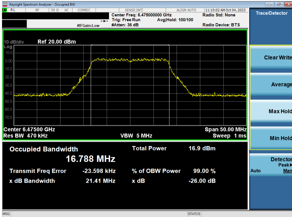
Plot 7-32. 26dB Bandwidth Plot MIMO ANT2 (20MHz 802.11a (UNII Band 6) – Ch. 105)
