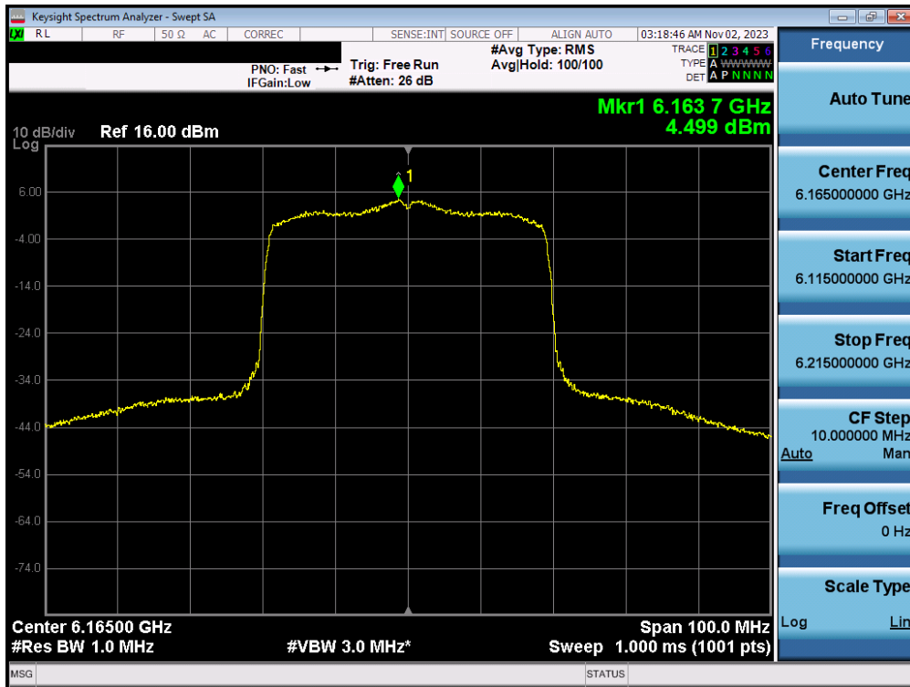
Plot 7-58. Power Spectral Density MIMO ANT1 (40MHz 802.11ax/be (UNII Band 5) – Ch. 43) - SP
