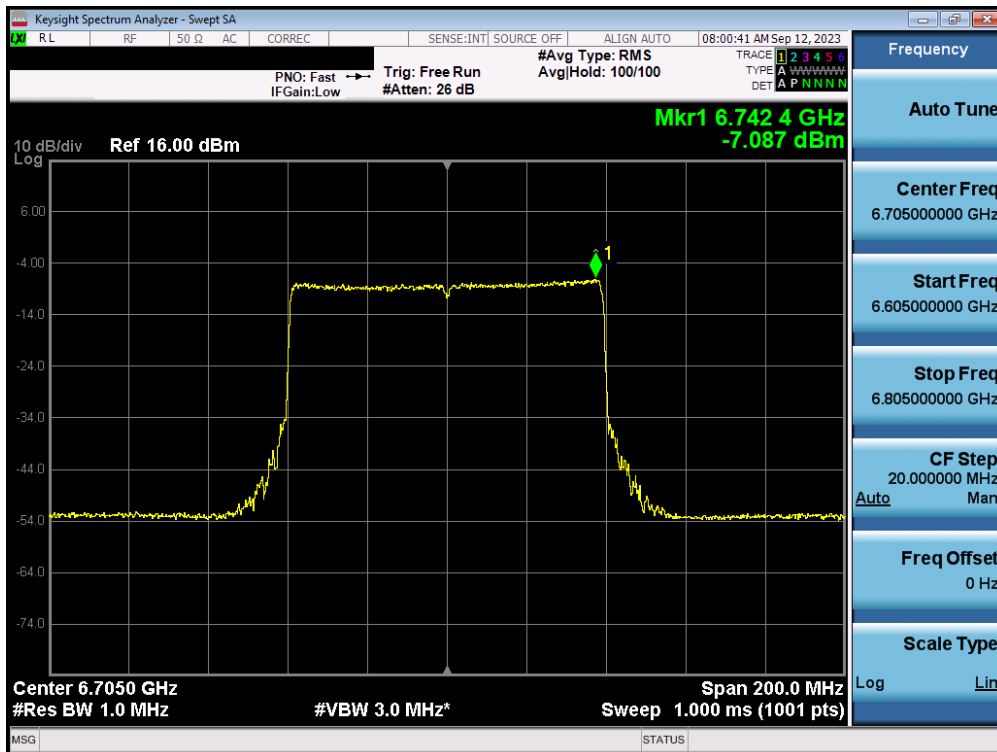
Plot 7-71. Power Spectral Density MIMO ANT1 (80MHz 802.11ax/be (UNII Band 7) – Ch. 151) - LPI
