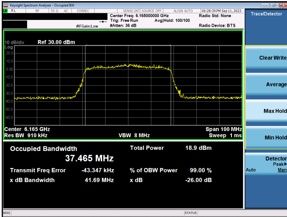
Plot 7-28. 26dB Bandwidth Plot MIMO ANT2 (40MHz 802.11ax/be (UNII Band 5) – Ch. 43)
