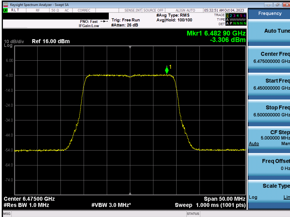
Plot 7-63. Power Spectral Density MIMO ANT1 (20MHz 802.11ax/be (UNII Band 6) – Ch. 105) - LPI
