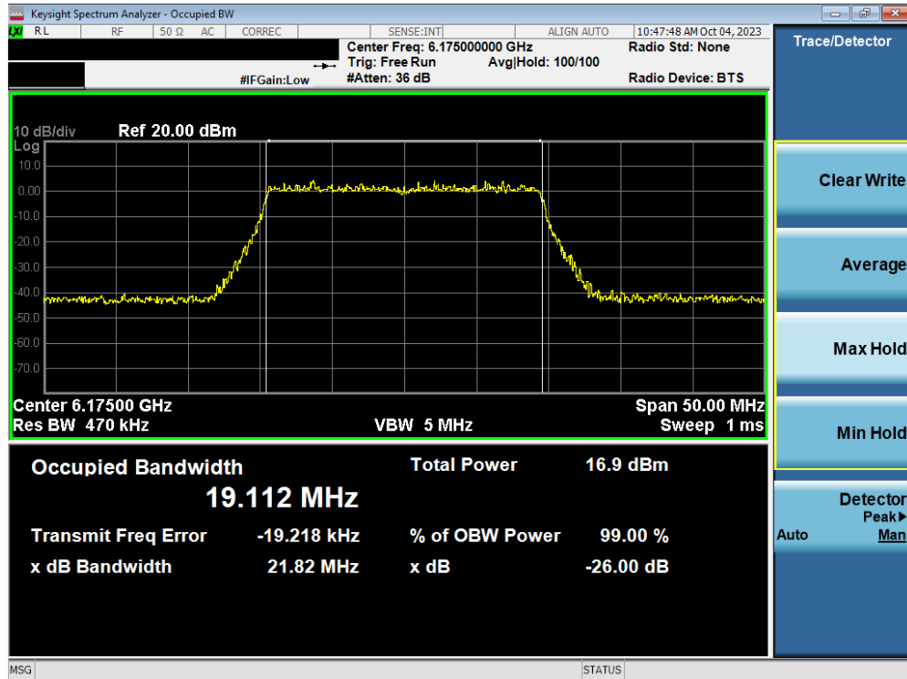
Plot 7-27. 26dB Bandwidth Plot MIMO ANT2 (20MHz 802.11ax/be (UNII Band 5) – Ch. 45)
