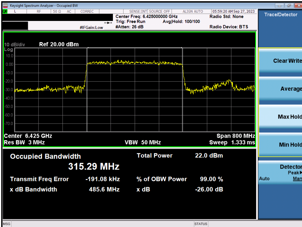
Plot 7-13. 26dB Bandwidth Plot MIMO ANT1 (320MHz 802.11ax/be (UNII Band 5/6/7) – Ch. 95)
