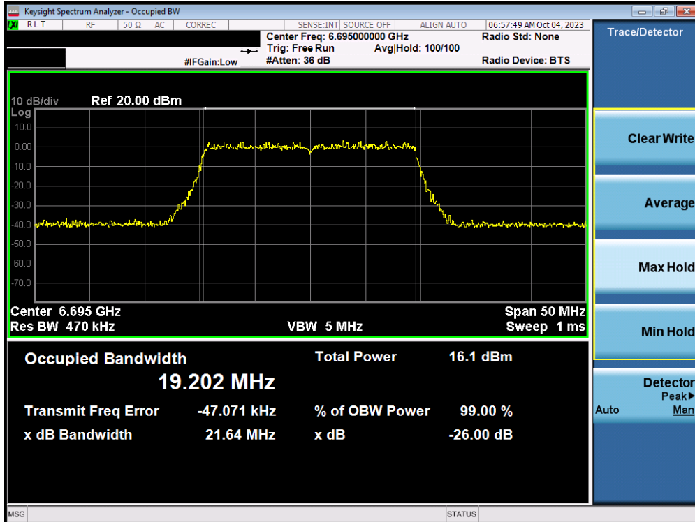
Plot 7-15. 26dB Bandwidth Plot MIMO ANT1 (20MHz 802.11ax/be (UNII Band 7) – Ch. 149)
