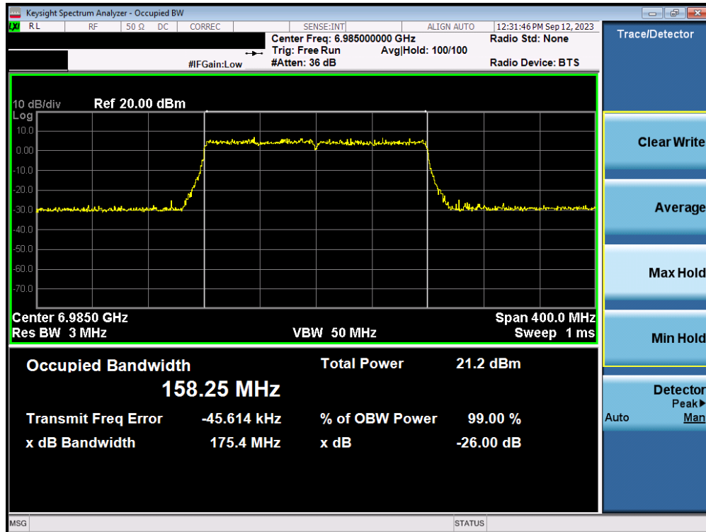
Plot 7-48. 26dB Bandwidth Plot MIMO ANT2 (160MHz 802.11ax/be (UNII Band 8) – Ch. 207)
