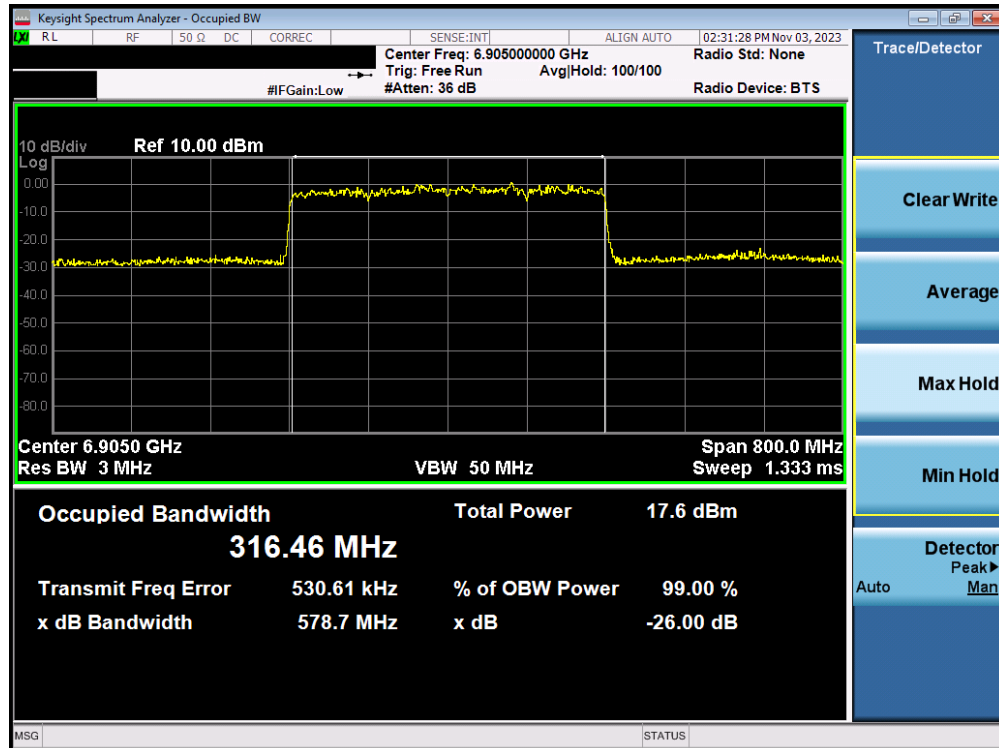
Plot 7-25. 26dB Bandwidth Plot MIMO ANT1 (320MHz 802.11ax/be (UNII Band 7/8) – Ch. 191)
