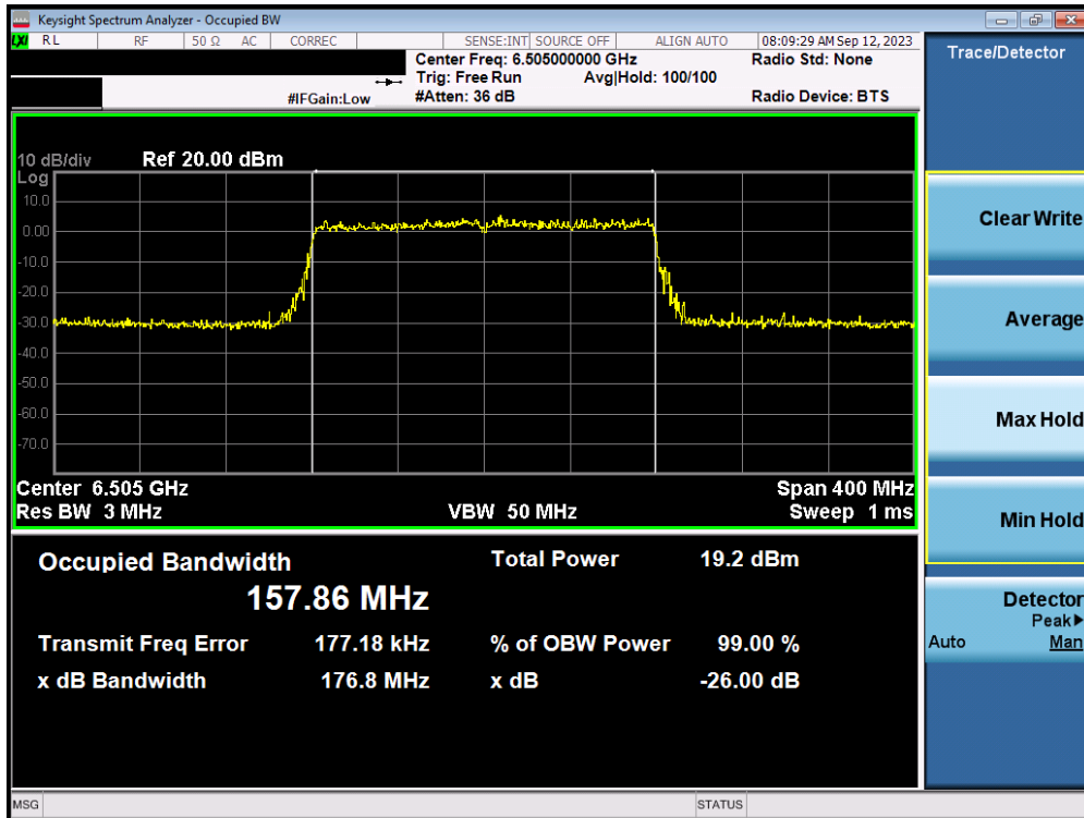
Plot 7-12. 26dB Bandwidth Plot MIMO ANT1 (160MHz 802.11ax/be (UNII Band 6) – Ch. 111)
