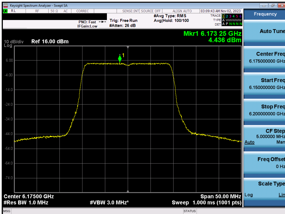
Plot 7-57. Power Spectral Density MIMO ANT1 (20MHz 802.11ax/be (UNII Band 5) – Ch. 45) - SP
