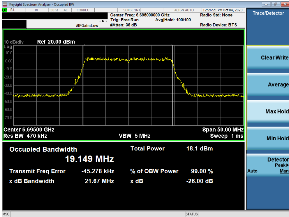
Plot 7-39. 26dB Bandwidth Plot MIMO ANT2 (20MHz 802.11ax/be (UNII Band 7) – Ch. 149)
