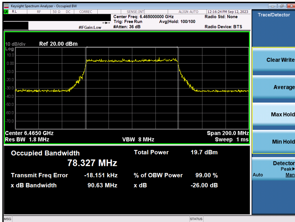
Plot 7-35. 26dB Bandwidth Plot MIMO ANT2 (80MHz 802.11ax/be (UNII Band 6) – Ch. 103)
