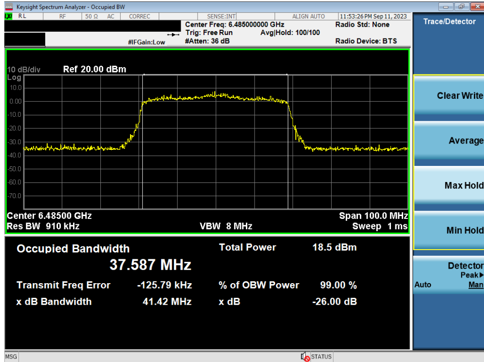
Plot 7-10. 26dB Bandwidth Plot MIMO ANT1 (40MHz 802.11ax/be (UNII Band 6) – Ch. 107)
