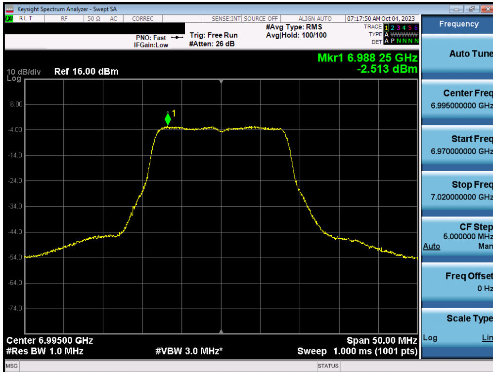
Plot 7-80. Power Spectral Density MIMO ANT1 (20MHz 802.11a (UNII Band 8) – Ch. 209) - LPI
