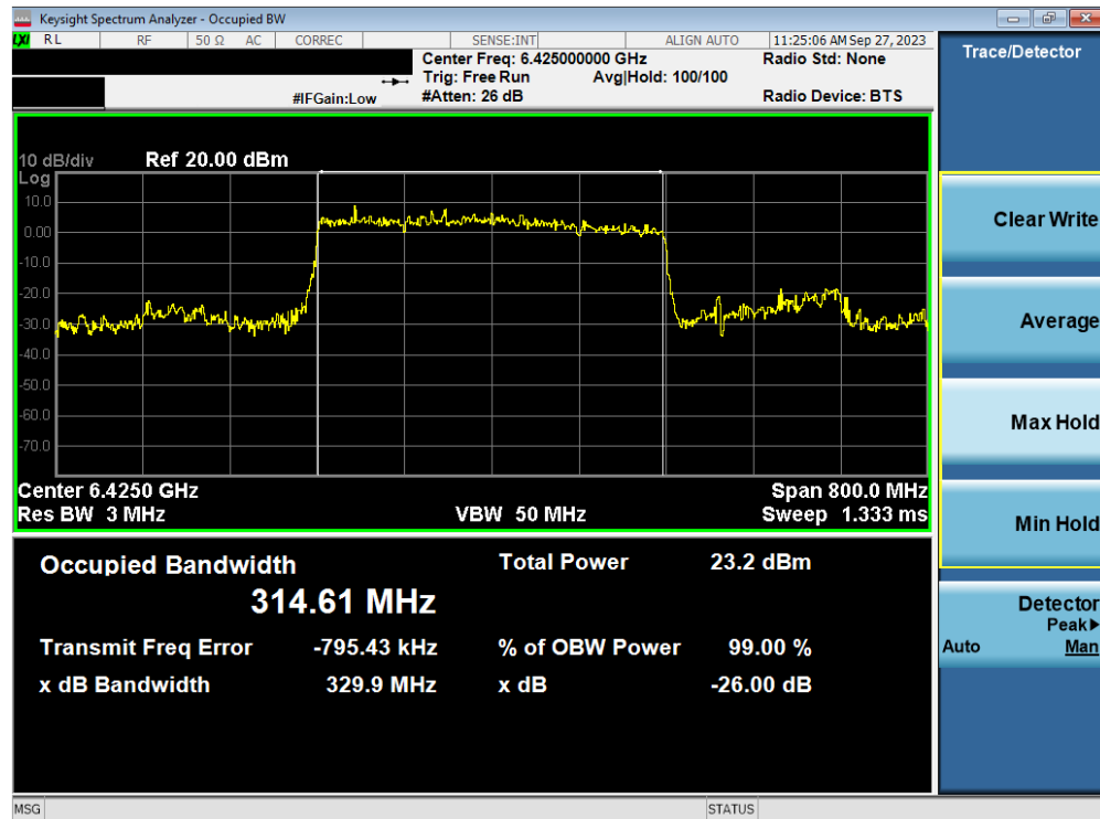
Plot 7-37. 26dB Bandwidth Plot MIMO ANT2 (320MHz 802.11ax/be (UNII Band 5/6/7) – Ch. 95)
