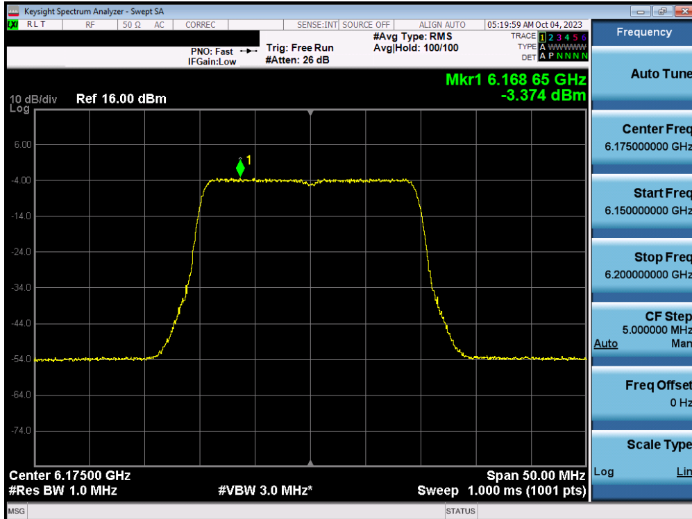
Plot 7-51. Power Spectral Density MIMO ANT1 (20MHz 802.11ax/be (UNII Band 5) – Ch. 45) - LPI
