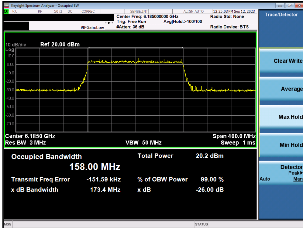
Plot 7-30. 26dB Bandwidth Plot MIMO ANT2 (160MHz 802.11ax/be (UNII Band 5) – Ch. 47)
