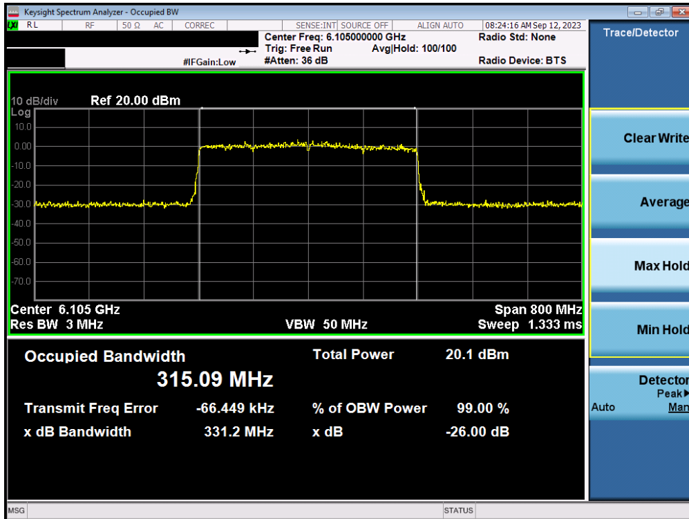
Plot 7-7. 26dB Bandwidth Plot MIMO ANT1 (320MHz 802.11ax/be (UNII Band 5) – Ch.31)
