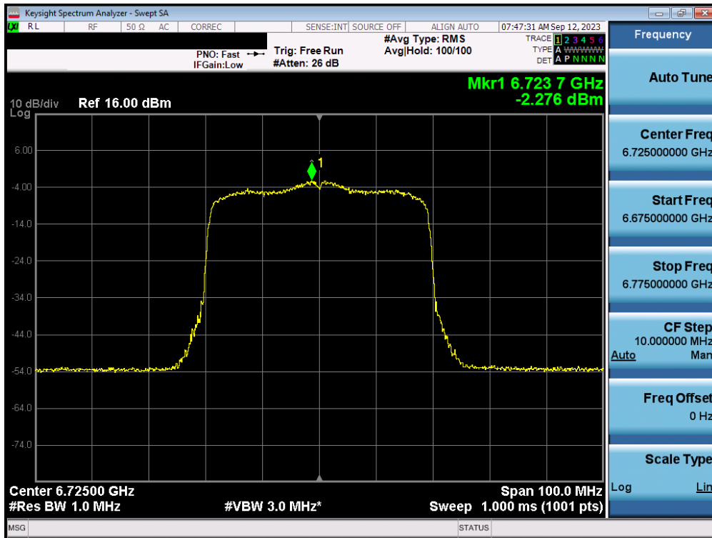
Plot 7-70. Power Spectral Density MIMO ANT1 (40MHz 802.11ax/be (UNII Band 7) – Ch. 155) - LPI
