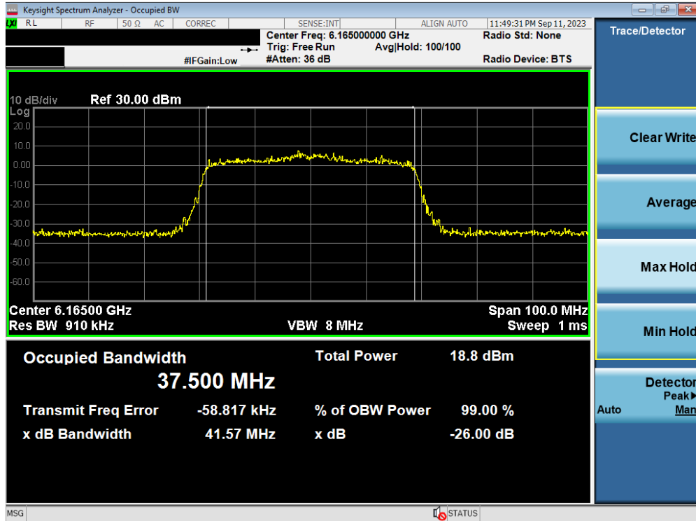
Plot 7-4. 26dB Bandwidth Plot MIMO ANT1 (40MHz 802.11ax/be (UNII Band 5) – Ch. 43)
