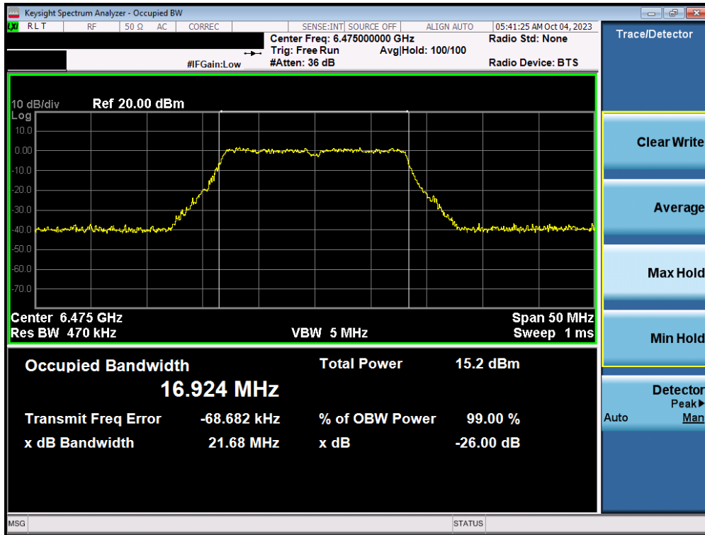
Plot 7-8. 26dB Bandwidth Plot MIMO ANT1 (20MHz 802.11a (UNII Band 6) – Ch. 105)
