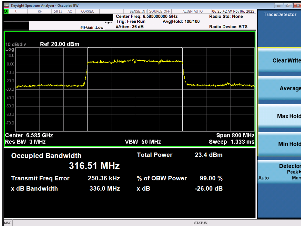
Plot 7-19. 26dB Bandwidth Plot MIMO ANT1 (320MHz 802.11ax/be (UNII Band 6/7) – Ch. 127)
