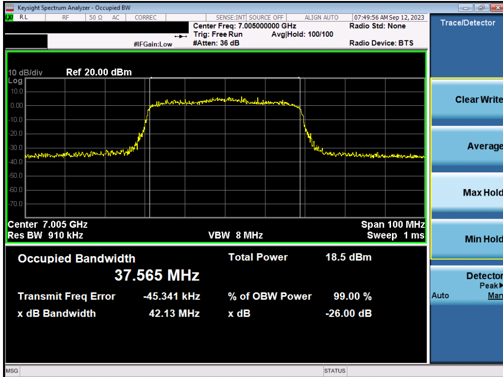
Plot 7-22. 26dB Bandwidth Plot MIMO ANT1 (40MHz 802.11ax/be (UNII Band 8) – Ch. 211)
