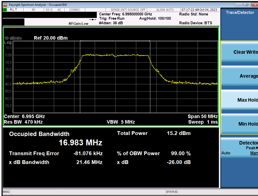
Plot 7-20. 26dB Bandwidth Plot MIMO ANT1 (20MHz 802.11a (UNII Band 8) – Ch. 209)
