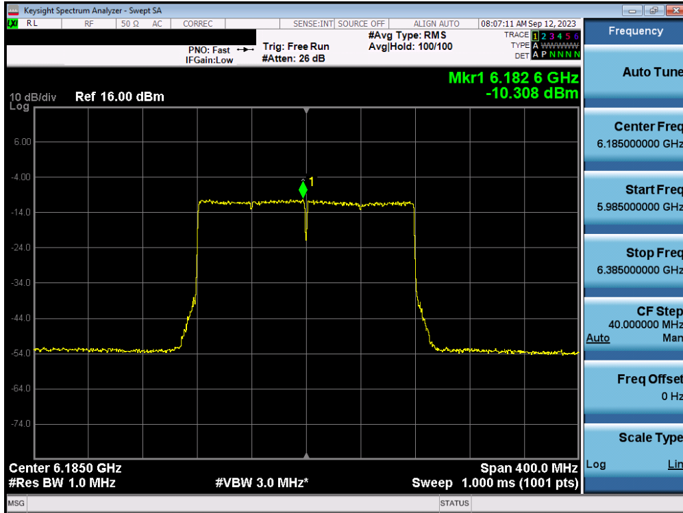
Plot 7-54. Power Spectral Density MIMO ANT1 (160MHz 802.11ax/be (UNII Band 5) – Ch. 47) - LPI
