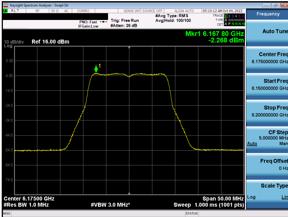
Plot 7-50. Power Spectral Density MIMO ANT1 (20MHz 802.11a (UNII Band 5) – Ch. 45) - LPI
