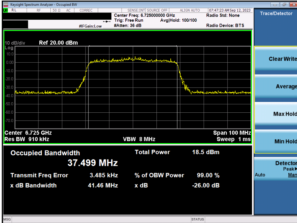
Plot 7-16. 26dB Bandwidth Plot MIMO ANT1 (40MHz 802.11ax/be (UNII Band 7) – Ch. 155)
