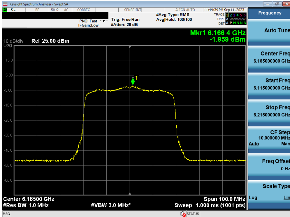
Plot 7-52. Power Spectral Density MIMO ANT1 (40MHz 802.11ax/be (UNII Band 5) – Ch. 43) - LPI
