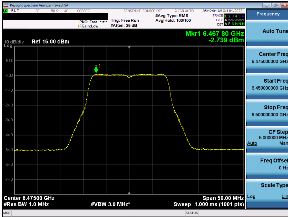
Plot 7-62. Power Spectral Density MIMO ANT1 (20MHz 802.11a (UNII Band 6) – Ch. 105) - LPI
