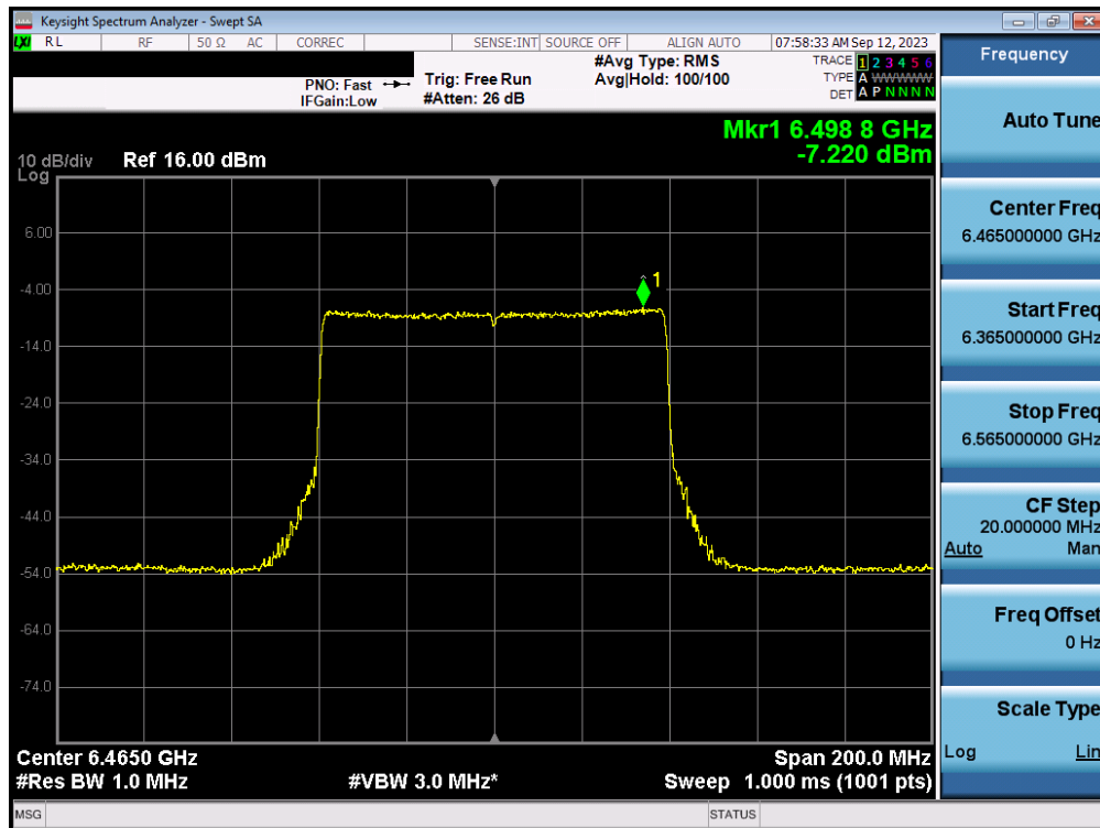
Plot 7-65. Power Spectral Density MIMO ANT1 (80MHz 802.11ax/be (UNII Band 6) – Ch. 103) - LPI
