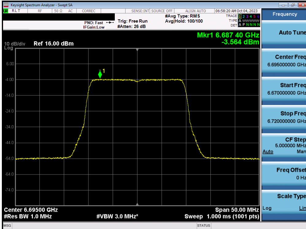
Plot 7-69. Power Spectral Density MIMO ANT1 (20MHz 802.11ax/be (UNII Band 7) – Ch. 149) - LPI
