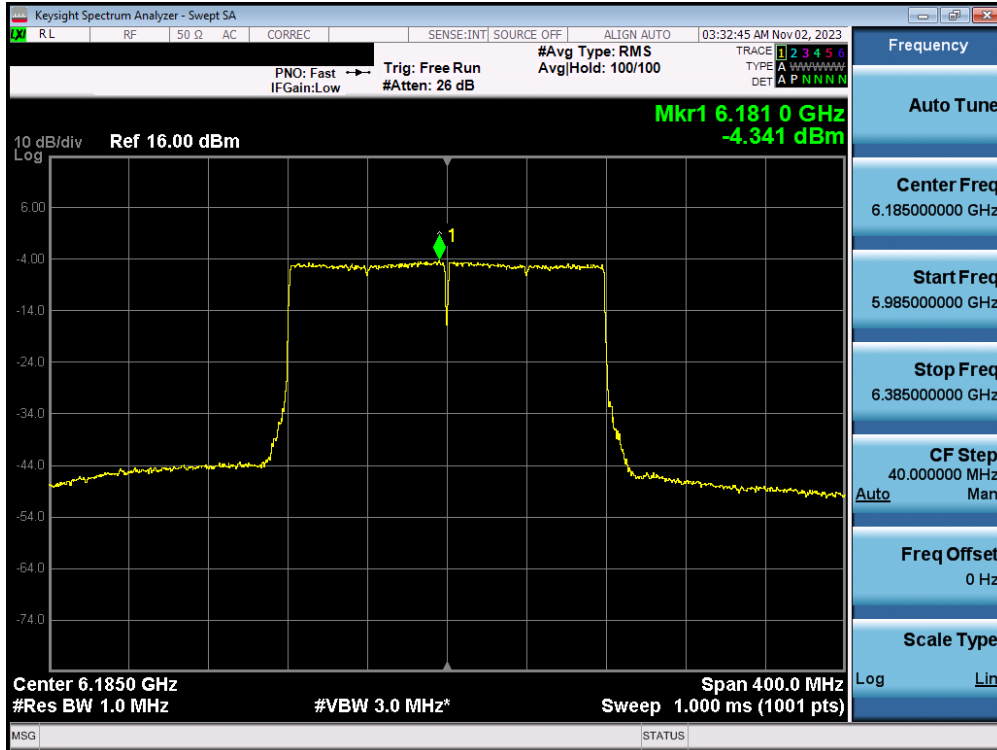
Plot 7-60. Power Spectral Density MIMO ANT1 (160MHz 802.11ax/be (UNII Band 5) – Ch. 47) - SP
