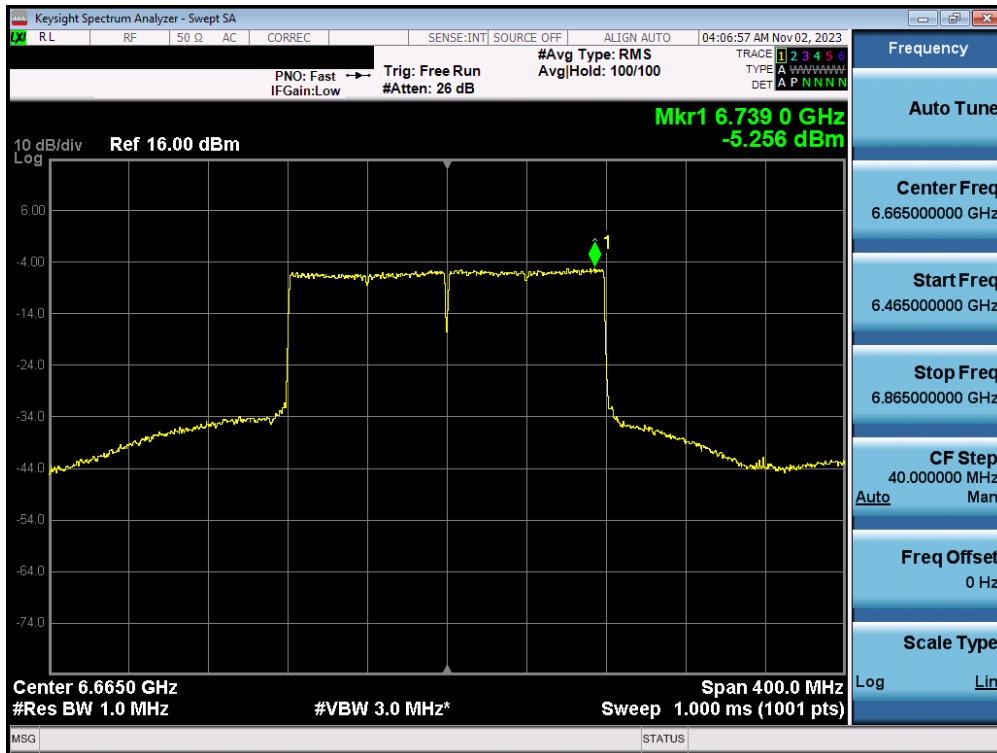
Plot 7-78. Power Spectral Density MIMO ANT1 (160MHz 802.11ax/be (UNII Band 7) – Ch. 143) - SP
