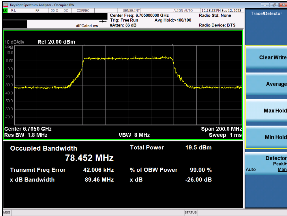
Plot 7-41. 26dB Bandwidth Plot MIMO ANT2 (80MHz 802.11ax/be (UNII Band 7) – Ch. 151)
