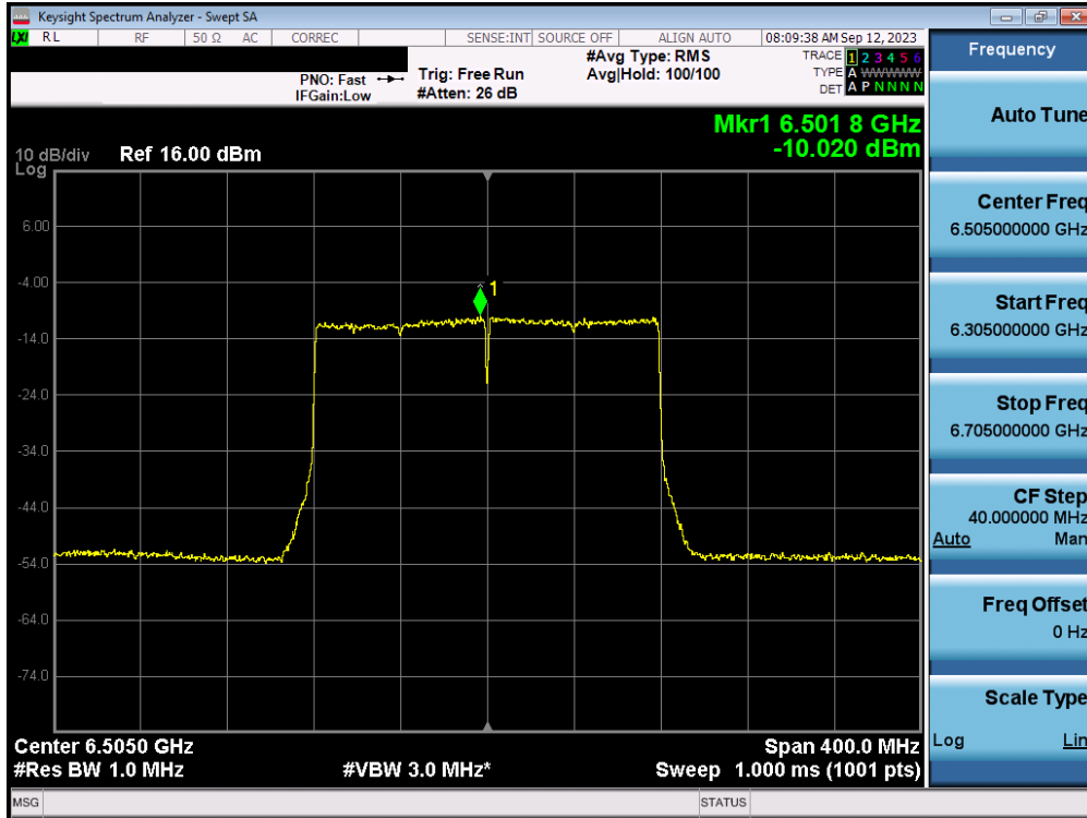
Plot 7-66. Power Spectral Density MIMO ANT1 (160MHz 802.11ax/be (UNII Band 6) – Ch. 111) - LPI
