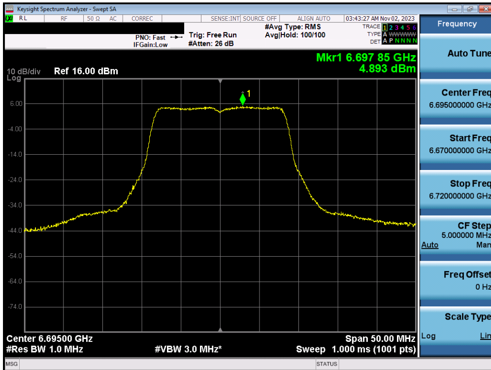
Plot 7-74. Power Spectral Density MIMO ANT1 (20MHz 802.11a (UNII Band 7) – Ch. 149) - SP
