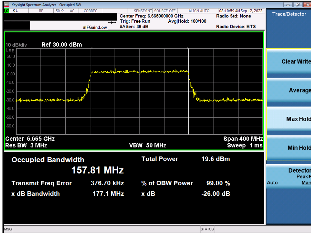
Plot 7-18. 26dB Bandwidth Plot MIMO ANT1 (160MHz 802.11ax/be (UNII Band 7) – Ch. 143)
