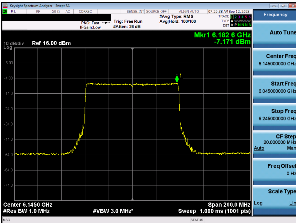
Plot 7-53. Power Spectral Density MIMO ANT1 (80MHz 802.11ax/be (UNII Band 5) – Ch. 39) - LPI
