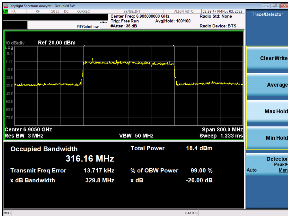
Plot 7-49. 26dB Bandwidth Plot MIMO ANT2 (320MHz 802.11ax/be (UNII Band 7/8) – Ch. 191)
