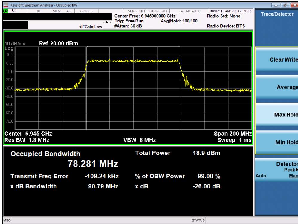
Plot 7-23. 26dB Bandwidth Plot MIMO ANT1 (80MHz 802.11ax/be (UNII Band 8) – Ch. 199)
