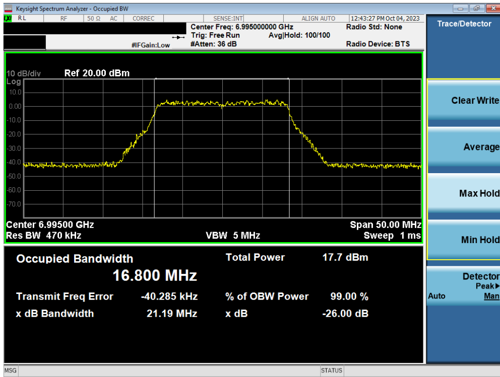
Plot 7-44. 26dB Bandwidth Plot MIMO ANT2 (20MHz 802.11a (UNII Band 8) – Ch. 209)
