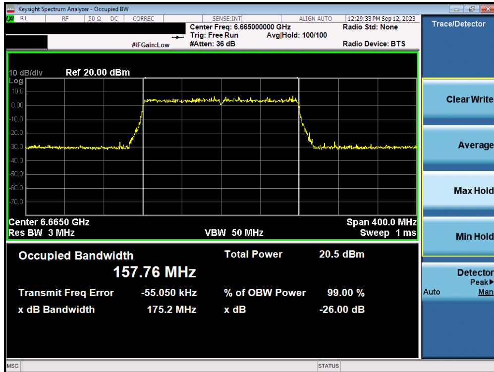
Plot 7-42. 26dB Bandwidth Plot MIMO ANT2 (160MHz 802.11ax/be (UNII Band 7) – Ch. 143)
