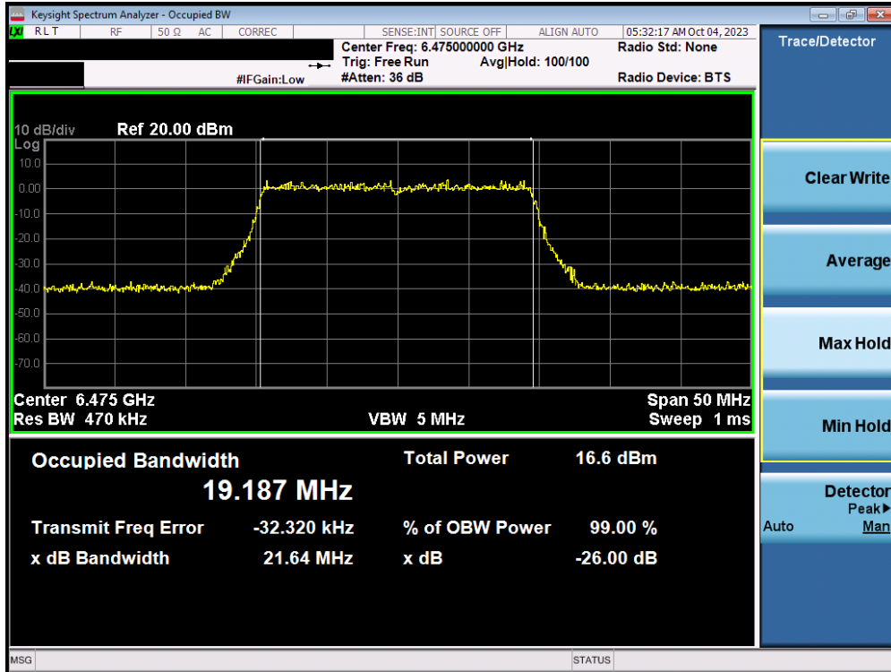
Plot 7-9. 26dB Bandwidth Plot MIMO ANT1 (20MHz 802.11ax/be (UNII Band 6) – Ch. 105)
