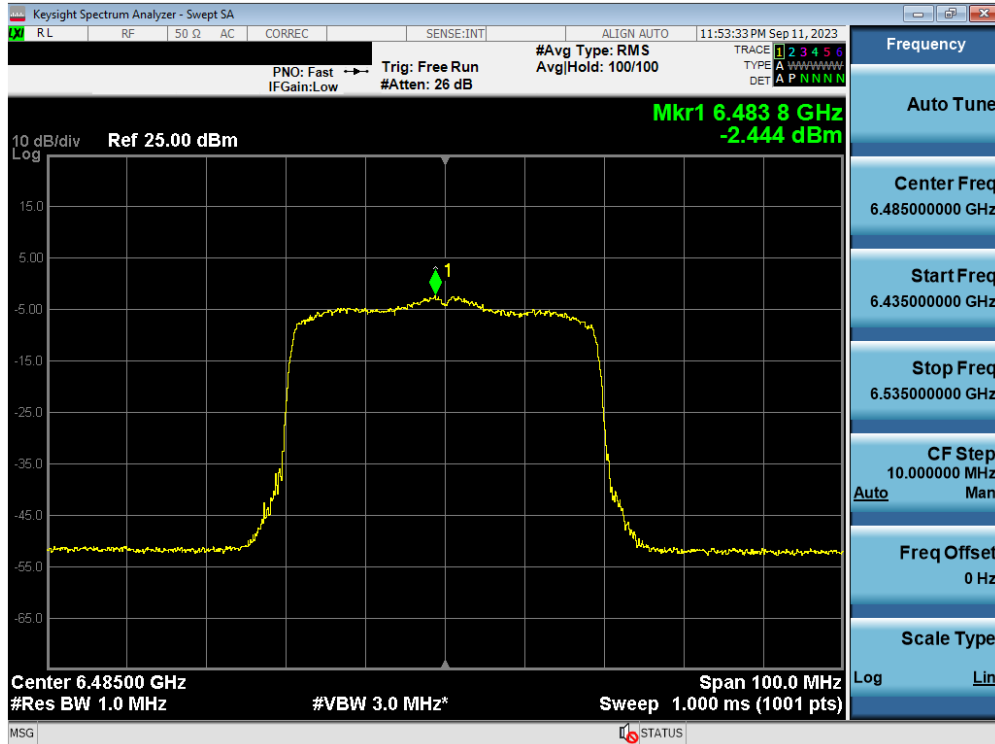
Plot 7-64. Power Spectral Density MIMO ANT1 (40MHz 802.11ax/be (UNII Band 6) – Ch. 107) - LPI
