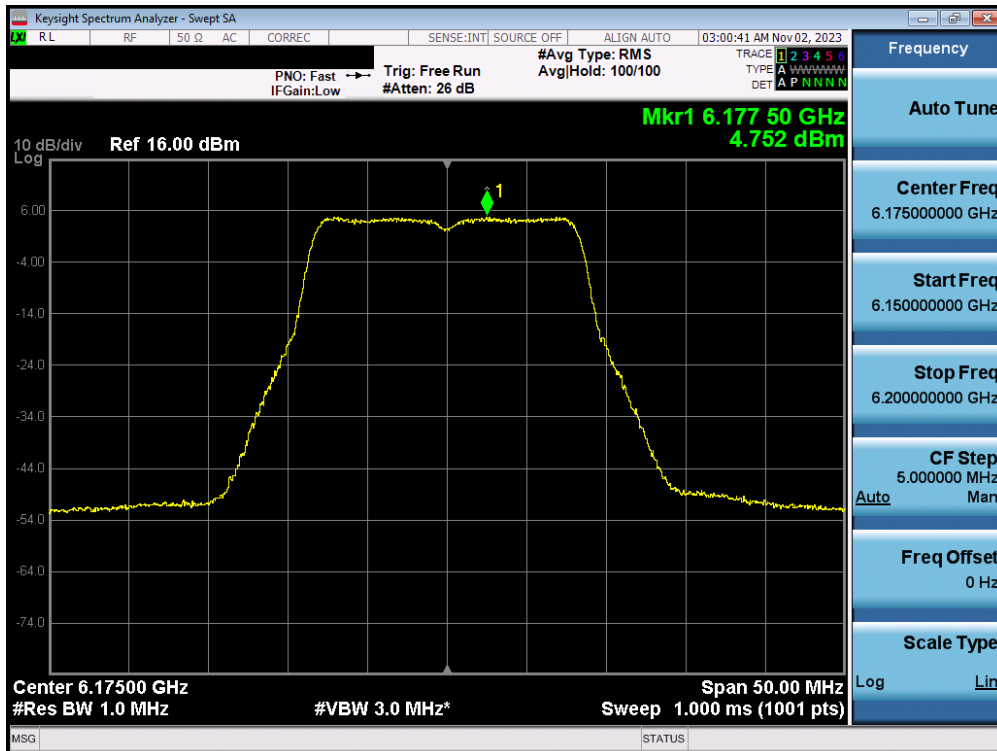
Plot 7-56. Power Spectral Density MIMO ANT1 (20MHz 802.11a (UNII Band 5) – Ch. 45) - SP
