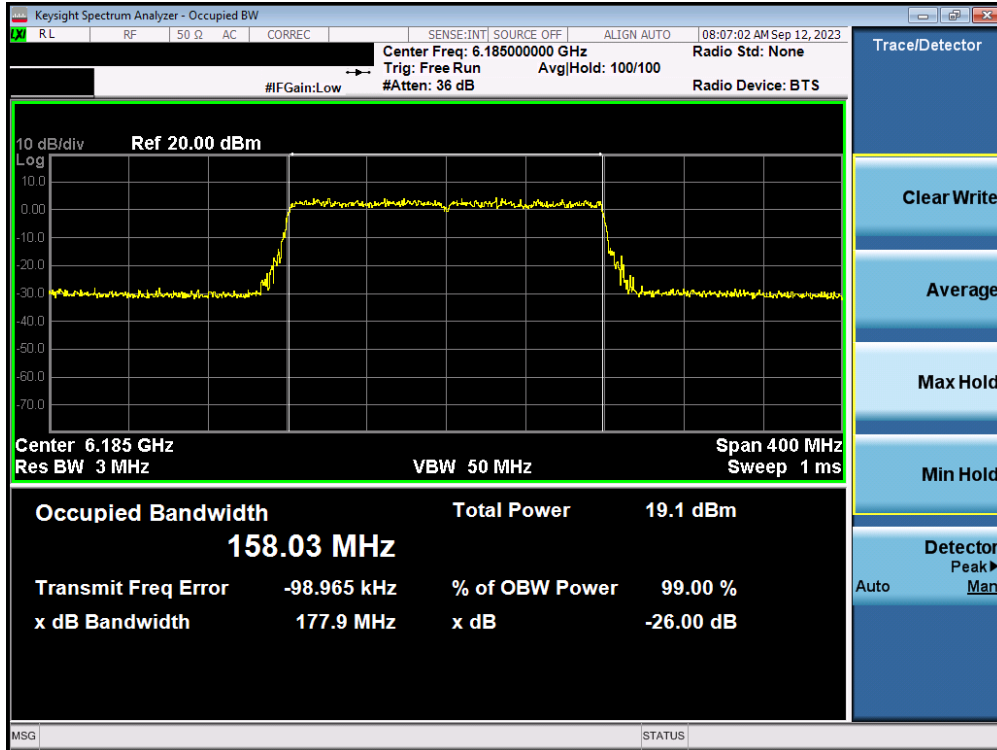
Plot 7-6. 26dB Bandwidth Plot MIMO ANT1 (160MHz 802.11ax/be (UNII Band 5) – Ch. 47)
