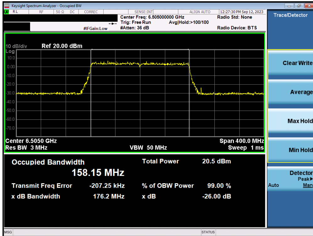
Plot 7-36. 26dB Bandwidth Plot MIMO ANT2 (160MHz 802.11ax/be (UNII Band 6) – Ch. 111)
