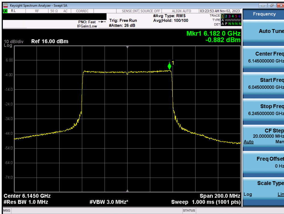
Plot 7-59. Power Spectral Density MIMO ANT1 (80MHz 802.11ax/be (UNII Band 5) – Ch. 39) - SP
