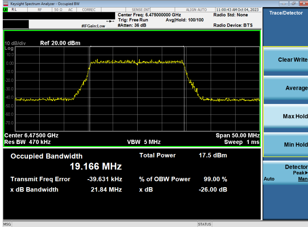
Plot 7-33. 26dB Bandwidth Plot MIMO ANT2 (20MHz 802.11ax/be (UNII Band 6) – Ch. 105)
