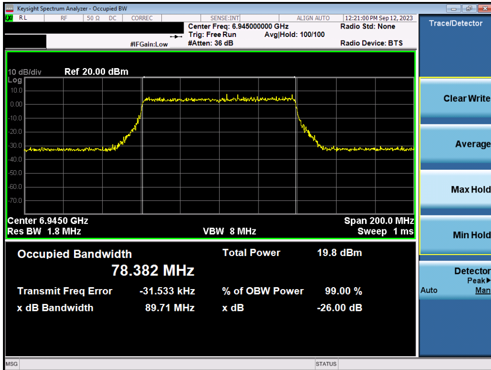
Plot 7-47. 26dB Bandwidth Plot MIMO ANT2 (80MHz 802.11ax/be (UNII Band 8) – Ch. 199)
