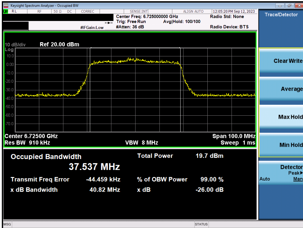
Plot 7-40. 26dB Bandwidth Plot MIMO ANT2 (40MHz 802.11ax/be (UNII Band 7) – Ch. 155)
