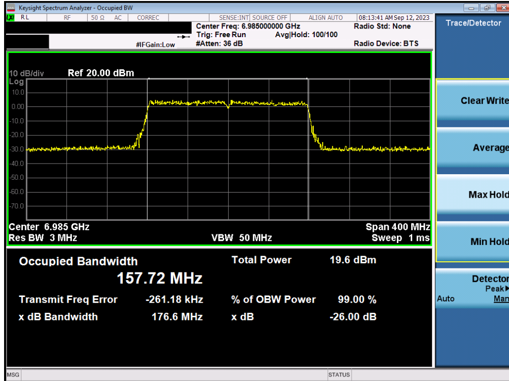
Plot 7-24. 26dB Bandwidth Plot MIMO ANT1 (160MHz 802.11ax/be (UNII Band 8) – Ch. 207)
