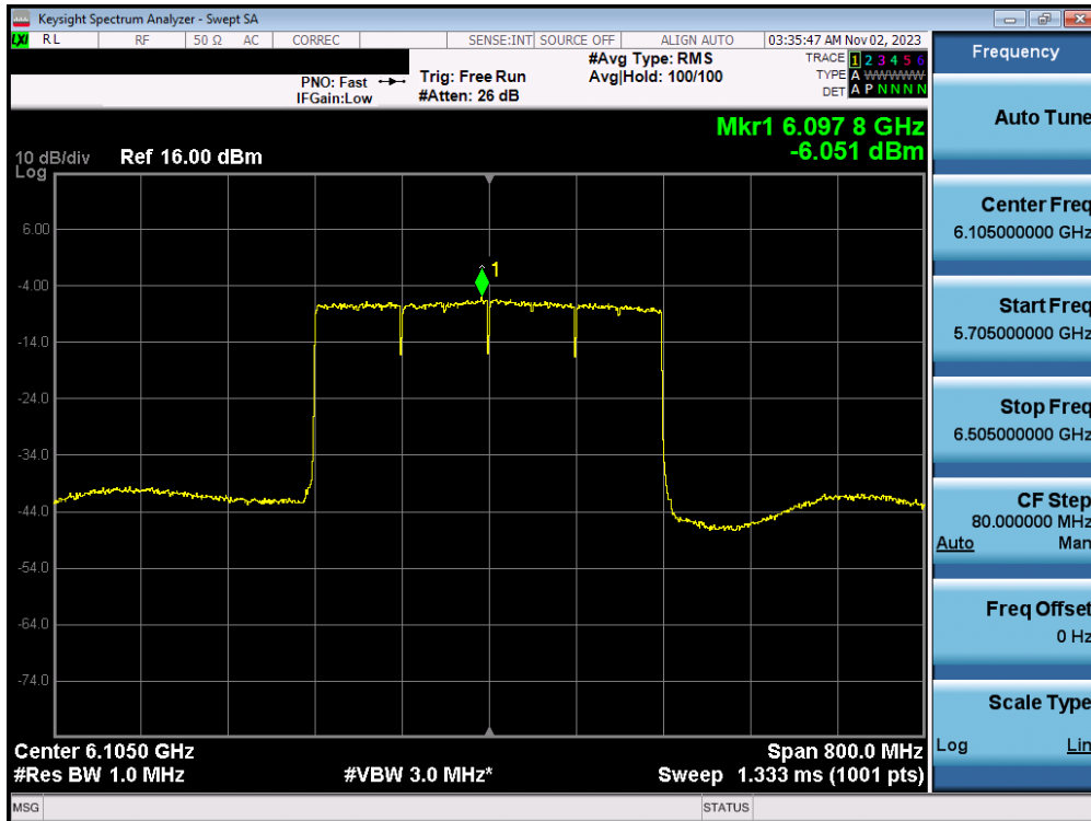
Plot 7-61. Power Spectral Density MIMO ANT1 (320MHz 802.11ax/be (UNII Band 5) – Ch.31) - SP
