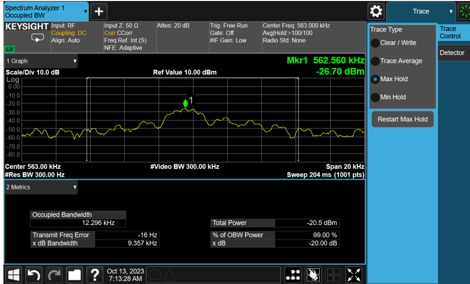
Plot 7-3. Occupied Bandwidth Measurement _ Hover
