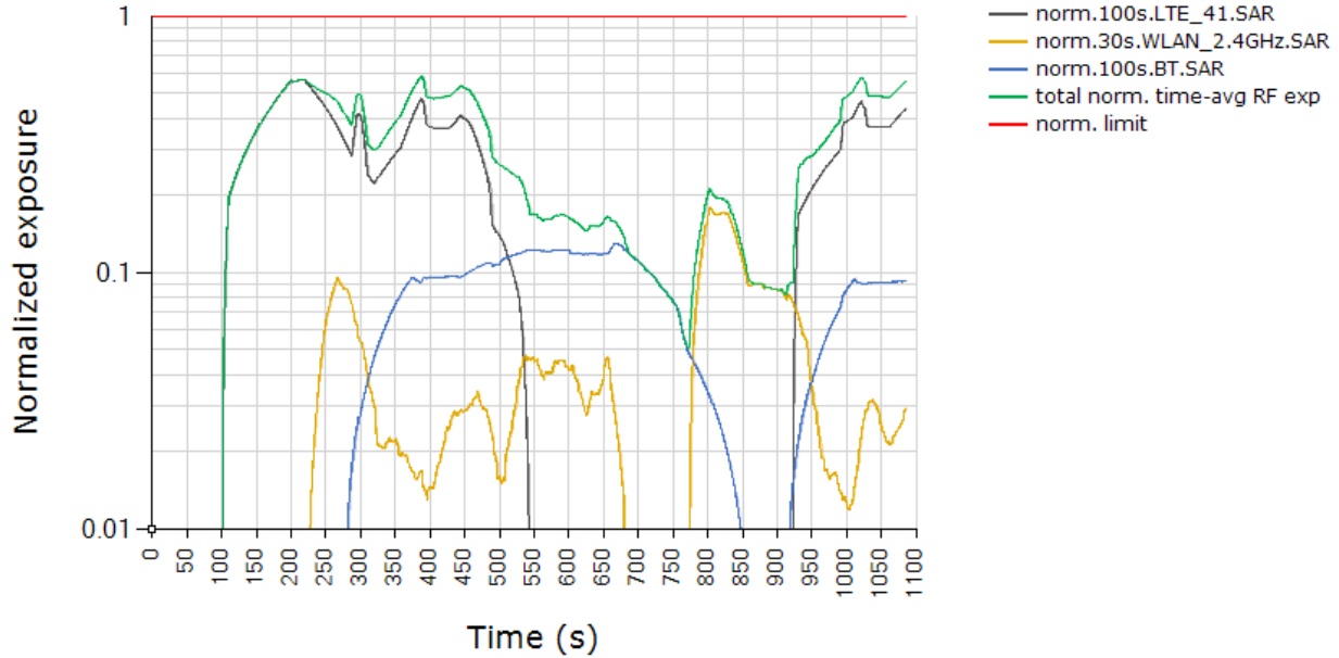
Total Normalized Time-averaged RF Exposure Tech: WLAN, Band 2.4GHz / Tech: LTE, Band 41 / Tech: BT
