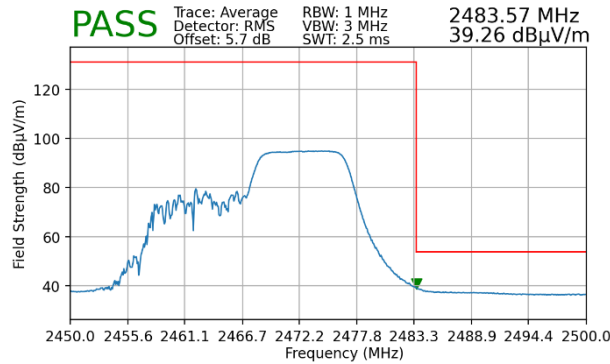
Plot 7-77. Radiated Restricted Upper Band Edge Measurement MIMO (Average – 106 Tones)
