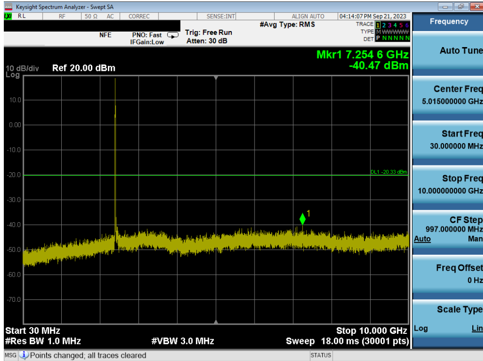
Plot 7-53. Conducted Spurious Plot MIMO ANT1 (802.11ax OFDMA – 26 Tones – Ch. 1)
