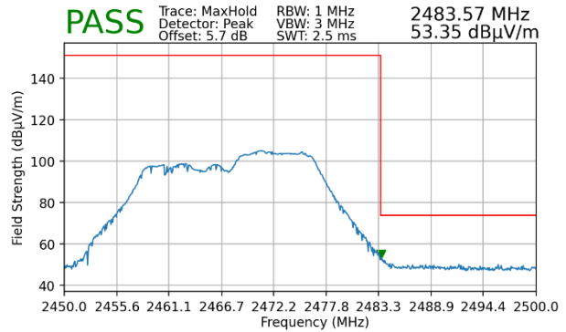
Plot 7-78. Radiated Restricted Upper Band Edge Measurement MIMO (Peak – 106 Tones)
