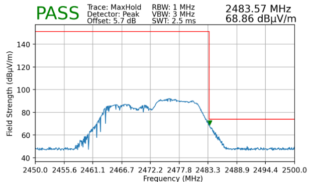
Plot 7-80. Radiated Restricted Upper Band Edge Measurement MIMO (Peak – 106 Tones)
