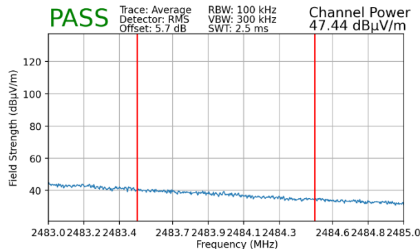
Plot 7-79. Radiated Restricted Upper Band Edge Measurement MIMO (Average – 106 Tones)
