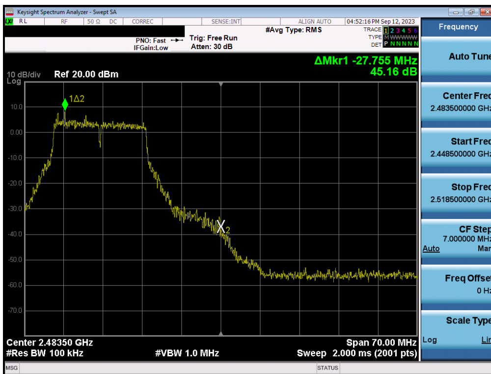
Plot 7-110. Band Edge Plot SISO ANT2 (802.11g - Ch. 11)
