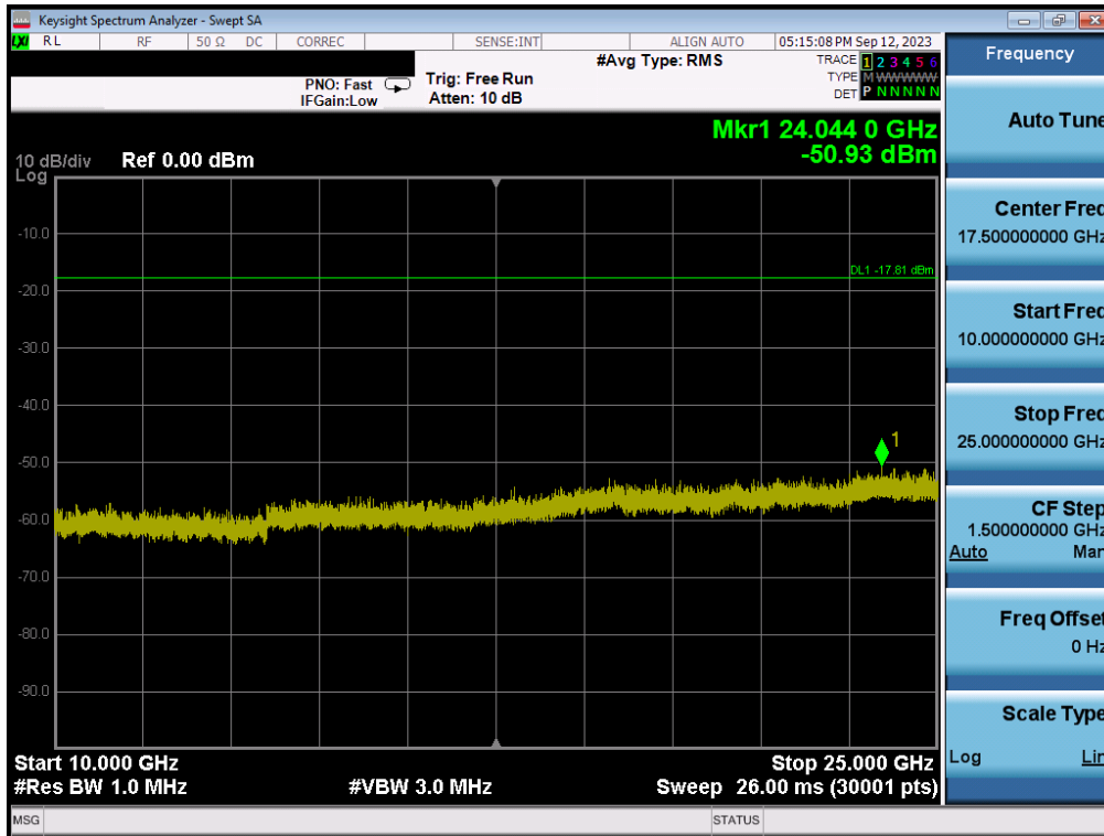
Plot 7-170. Conducted Spurious Plot MIMO ANT1 (802.11b – Ch. 11)
