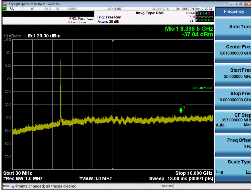
Plot 7-173. Conducted Spurious Plot MIMO ANT2 (802.11b – Ch. 6)
