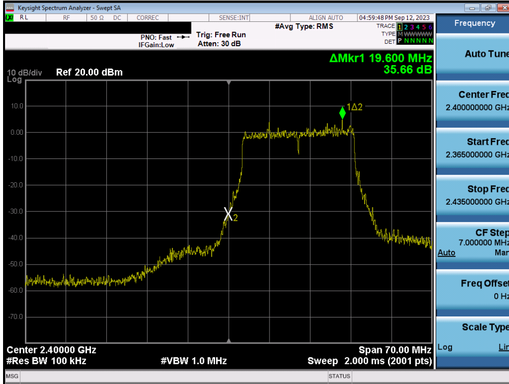
Plot 7-129. Band Edge Plot MIMO ANT1 (802.11be (2.4GHz) – Ch. 1)
