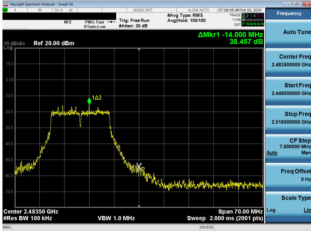
Plot 7-123. Band Edge Plot MIMO ANT1 (802.11g – Ch. 12)
