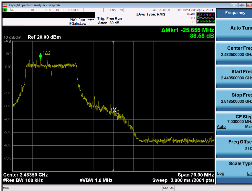
Plot 7-126. Band Edge Plot MIMO ANT1 (802.11n (2.4GHz) – Ch. 11)
