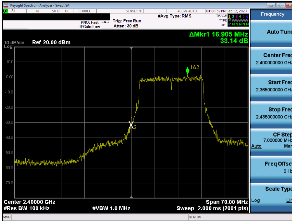
Plot 7-147. Band Edge Plot MIMO ANT2 (802.11be (2.4GHz) – Ch. 1)
