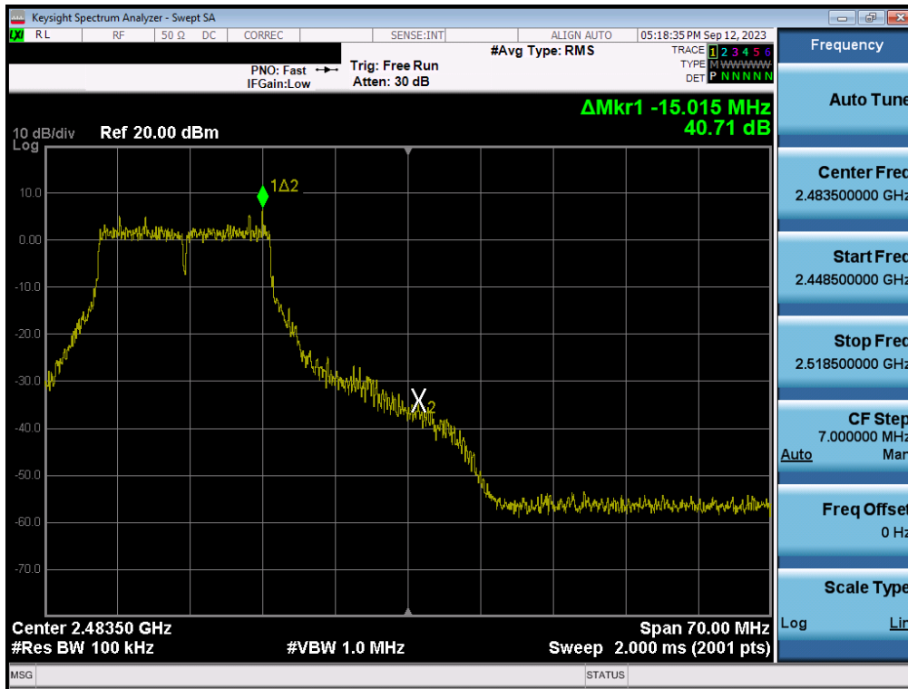
Plot 7-122. Band Edge Plot MIMO ANT1 (802.11g - Ch. 11)
