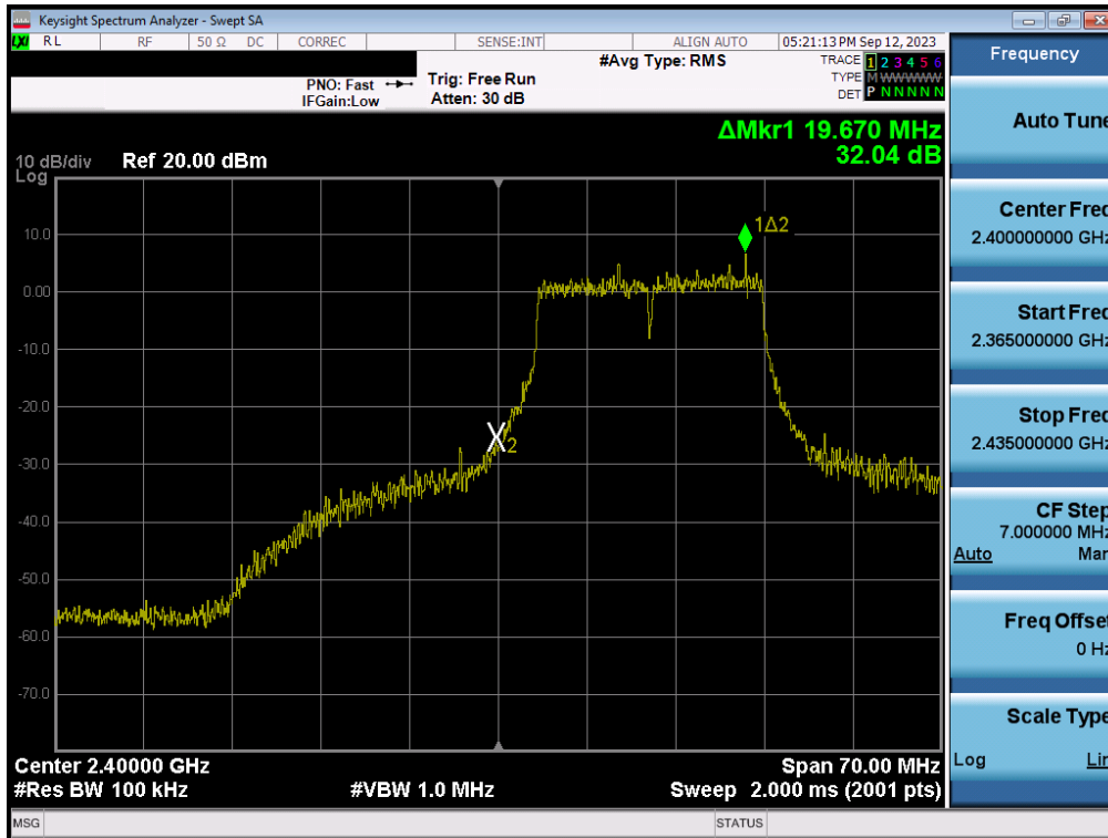
Plot 7-125. Band Edge Plot MIMO ANT1 (802.11n (2.4GHz) – Ch. 1)
