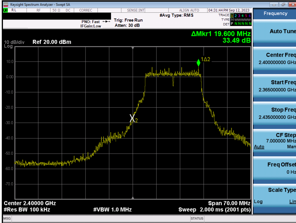
Plot 7-139. Band Edge Plot MIMO ANT2 (802.11g- Ch. 1)
