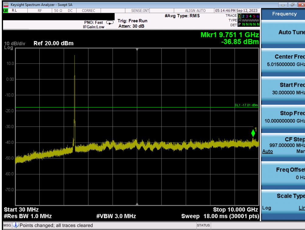
Plot 7-169. Conducted Spurious Plot MIMO ANT1 (802.11b – Ch. 11)
