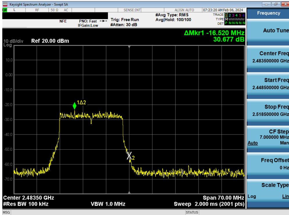
Plot 7-134. Band Edge Plot MIMO ANT1 (802.11be (2.4GHz) – Ch. 13)
