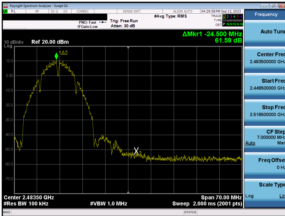
Plot 7-136. Band Edge Plot MIMO ANT2 (802.11b – Ch. 11)
