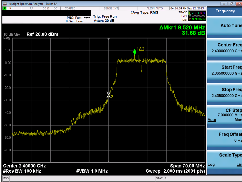
Plot 7-143. Band Edge Plot MIMO ANT2 (802.11n (2.4GHz) – Ch. 1)
