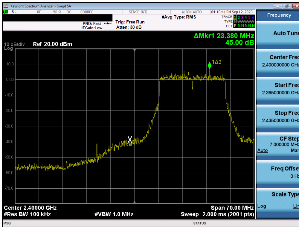
Plot 7-148. Band Edge Plot MIMO ANT2 (802.11be (2.4GHz) – Ch. 2)
