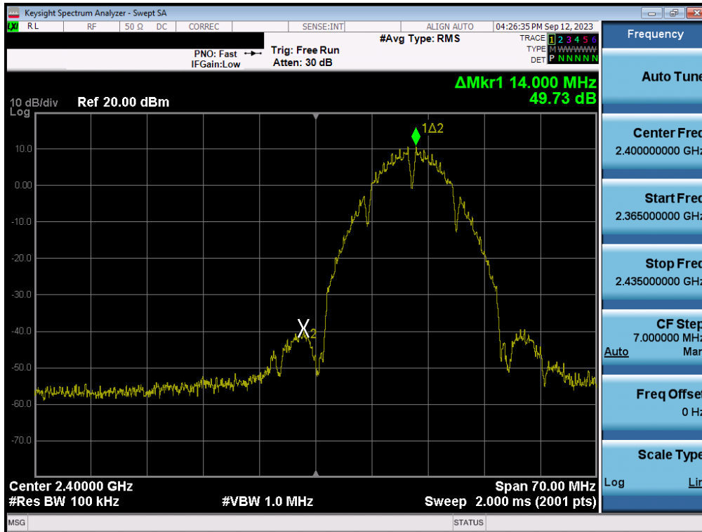
Plot 7-135. Band Edge Plot MIMO ANT2 (802.11b – Ch. 1)
