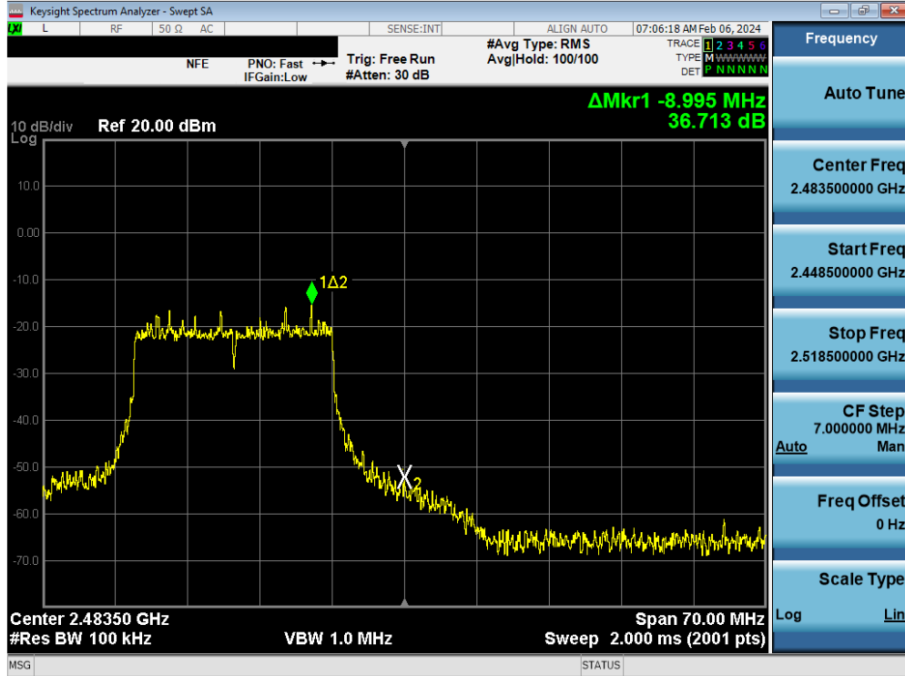
Plot 7-133. Band Edge Plot MIMO ANT1 (802.11be (2.4GHz) – Ch. 12)
