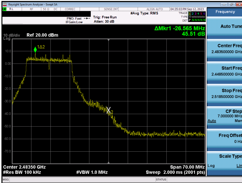
Plot 7-140. Band Edge Plot MIMO ANT2 (802.11g - Ch. 11)
