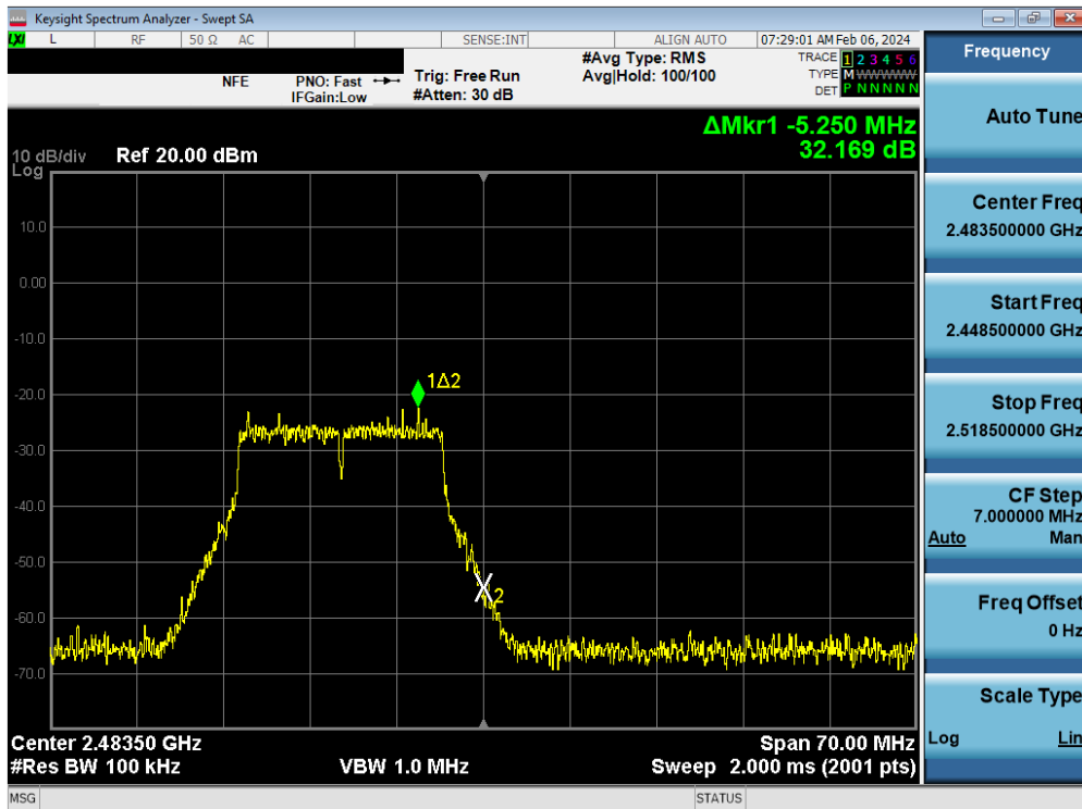
Plot 7-146. Band Edge Plot MIMO ANT2 (802.11n (2.4GHz) – Ch. 13)
