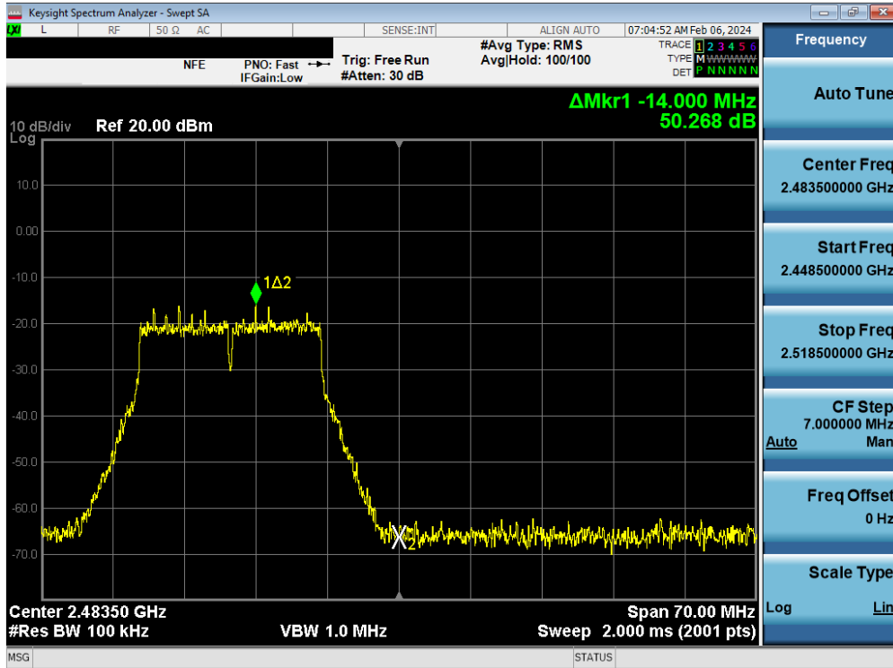
Plot 7-145. Band Edge Plot MIMO ANT2 (802.11n (2.4GHz) – Ch. 12)
