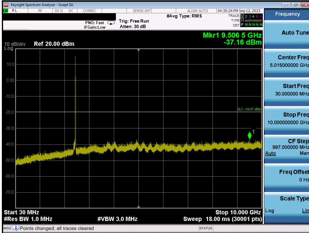
Plot 7-175. Conducted Spurious Plot MIMO ANT2 (802.11b – Ch. 11)
