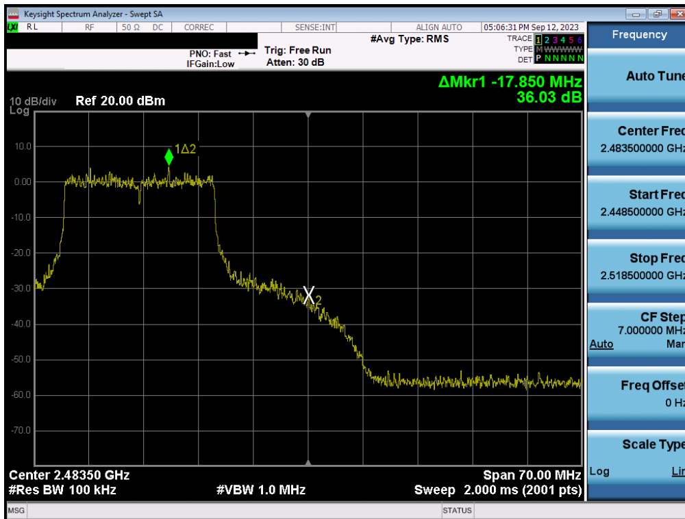
Plot 7-132. Band Edge Plot MIMO ANT1 (802.11be (2.4GHz) – Ch. 11)
