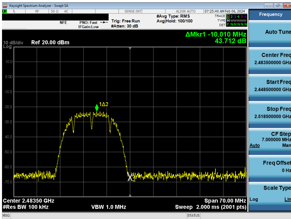
Plot 7-120. Band Edge Plot MIMO ANT1 (802.11b – Ch. 13)
