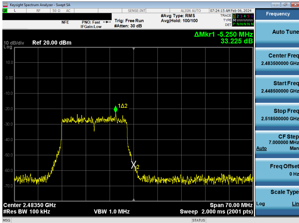
Plot 7-152. Band Edge Plot MIMO ANT2 (802.11be (2.4GHz) – Ch. 11)
