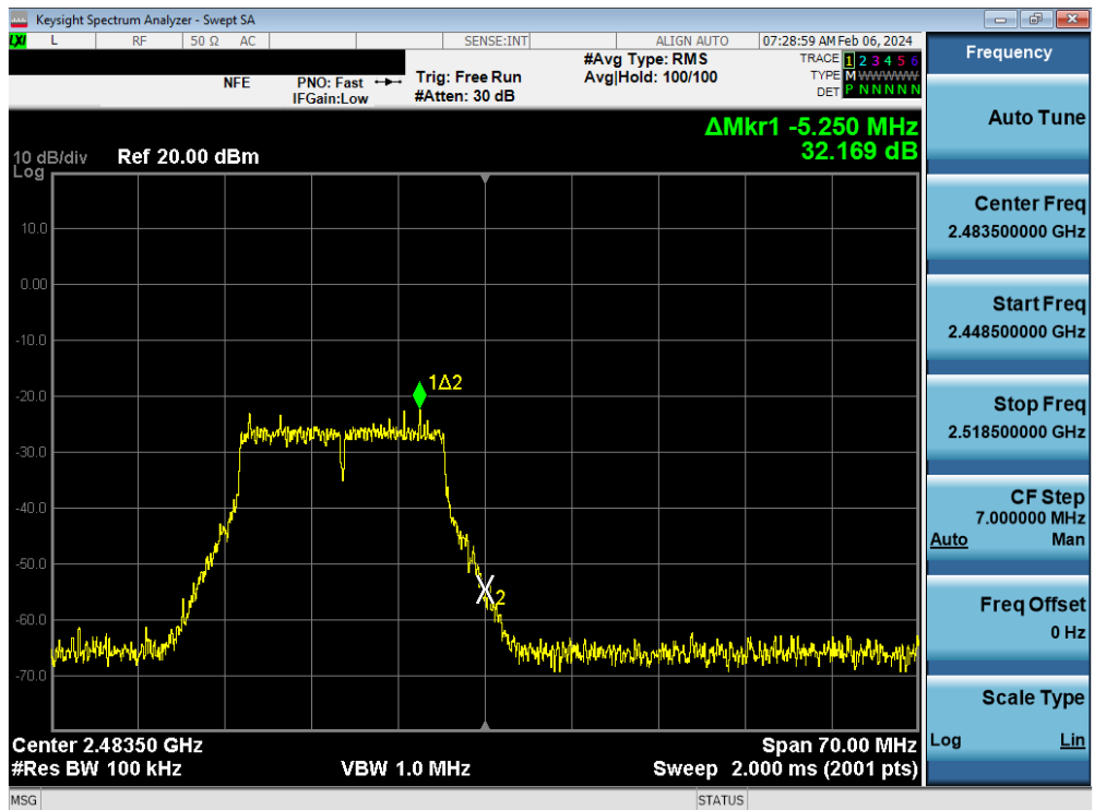
Plot 7-128. Band Edge Plot MIMO ANT1 (802.11n (2.4GHz) – Ch. 13)
