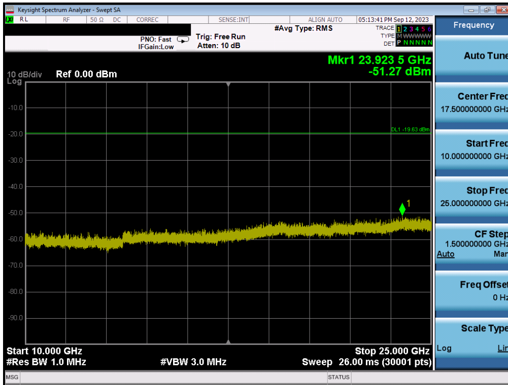
Plot 7-168. Conducted Spurious Plot MIMO ANT1 (802.11b – Ch. 6)
