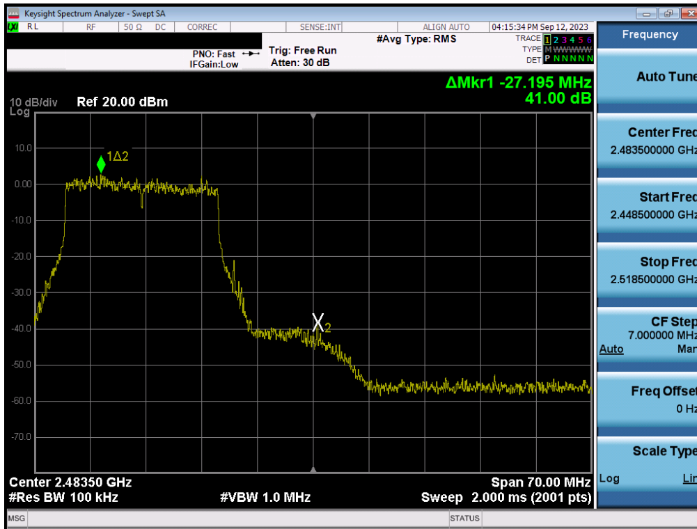
Plot 7-150. Band Edge Plot MIMO ANT2 (802.11be (2.4GHz) – Ch. 11)
