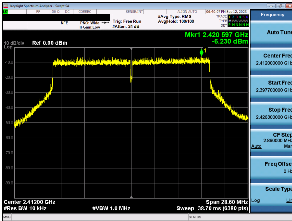
Plot 7-94. Power Spectral Density Plot MIMO ANT2 (802.11be (2.4GHz) – Ch. 1)
