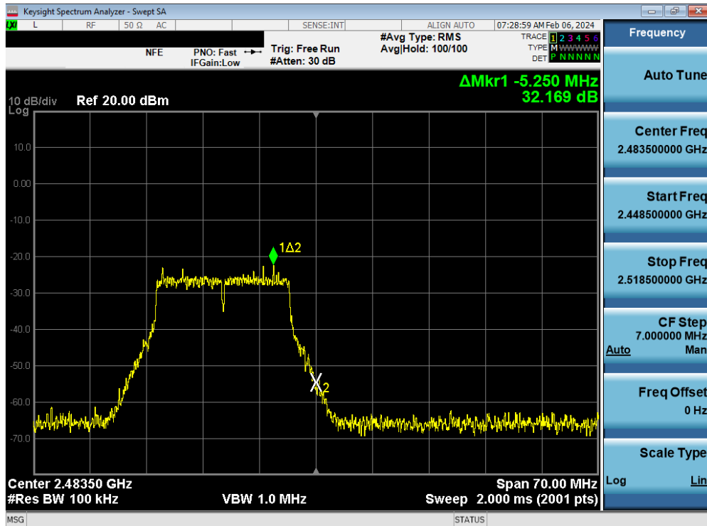
Plot 7-124. Band Edge Plot MIMO ANT1 (802.11g – Ch. 13)
