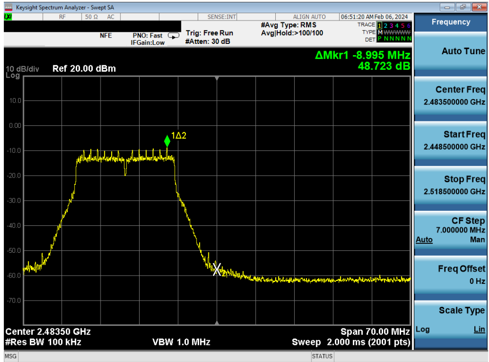
Plot 7-127. Band Edge Plot MIMO ANT1 (802.11n (2.4GHz) – Ch. 12)
