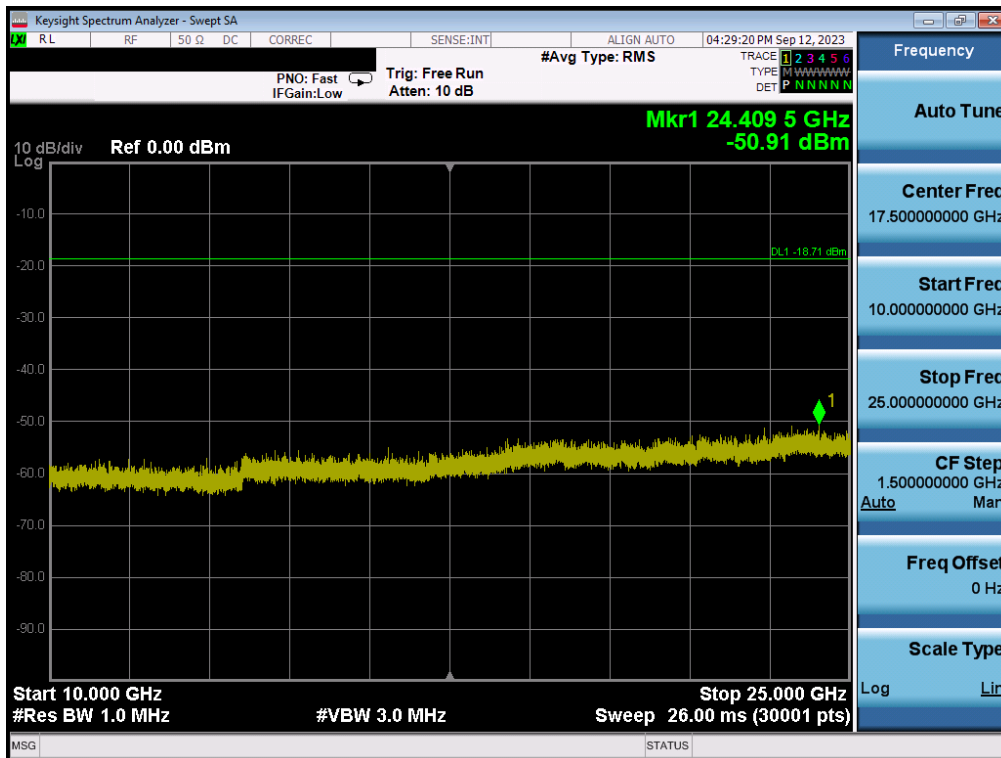
Plot 7-174. Conducted Spurious Plot MIMO ANT2 (802.11b – Ch. 6)
