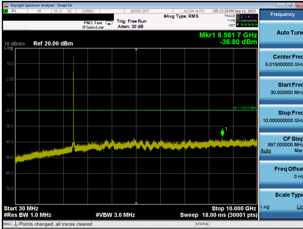
Plot 7-167. Conducted Spurious Plot MIMO ANT1 (802.11b – Ch. 6)
