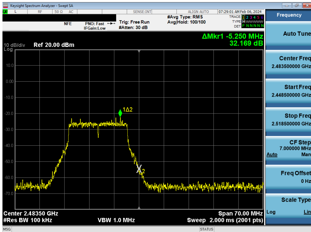
Plot 7-142. Band Edge Plot MIMO ANT2 (802.11g – Ch. 13)
