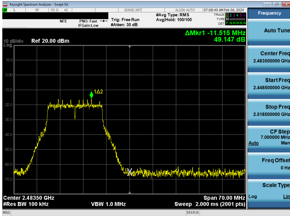
Plot 7-141. Band Edge Plot MIMO ANT2 (802.11g – Ch. 12)
