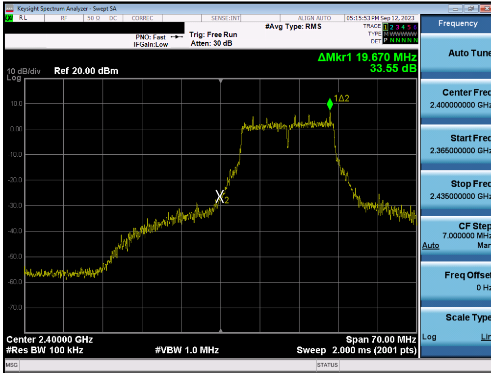
Plot 7-121. Band Edge Plot MIMO ANT1 (802.11g- Ch. 1)
