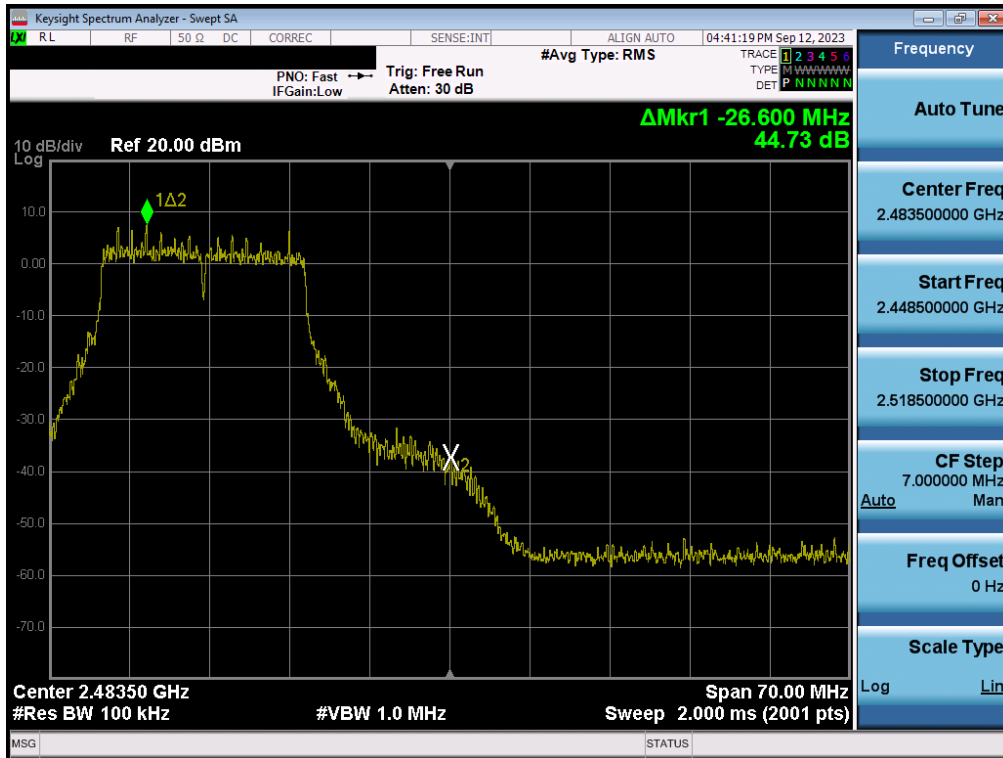
Plot 7-144. Band Edge Plot MIMO ANT2 (802.11n (2.4GHz) – Ch. 11)
