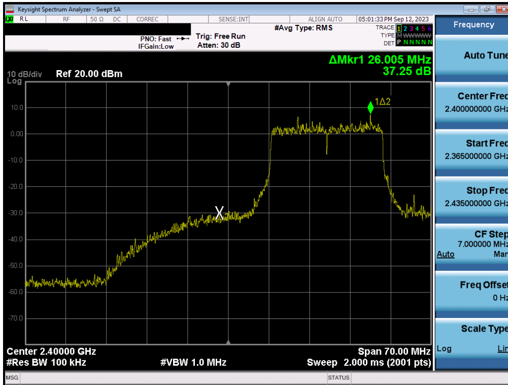
Plot 7-130. Band Edge Plot MIMO ANT1 (802.11be (2.4GHz) – Ch. 2)
