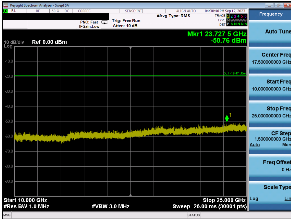
Plot 7-176. Conducted Spurious Plot MIMO ANT2 (802.11b – Ch. 11)
