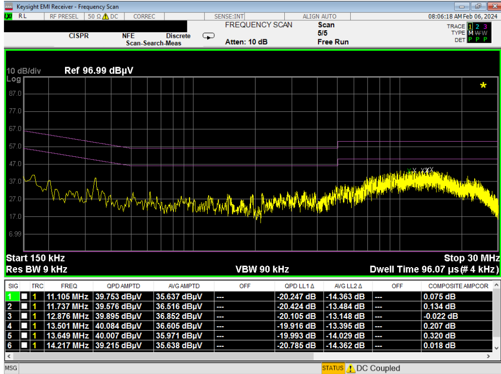
Plot 7-107. Line Conducted Plot with Bluetooth LE (L1) WCP
