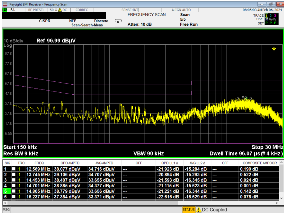
Plot 7-108. Line Conducted Plot with Bluetooth LE (N) WCP
