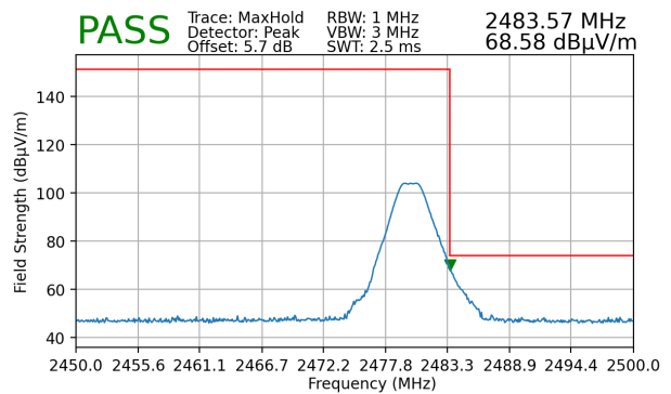
Plot 7-102. Radiated Restricted Upper Band Edge Measurement (Peak) ANT1
