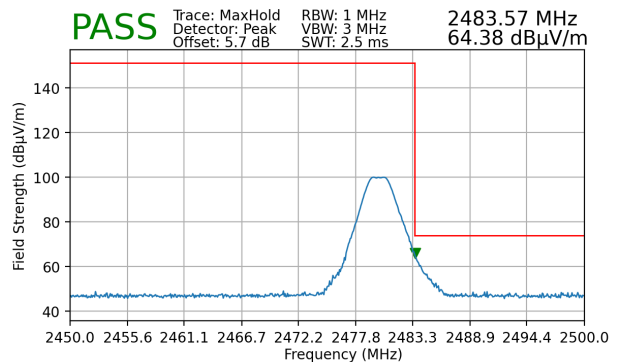
Plot 7-104. Radiated Restricted Upper Band Edge Measurement (Peak) ANT2
