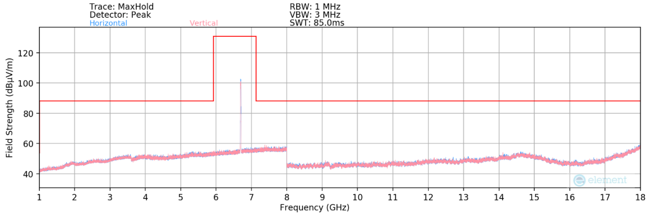
Plot 7-192. Radiated Spurious Plot 1GHz – 18GHz MIMO (802.11ax – UNII Band 7 Ch. 149) – LPI & SP
