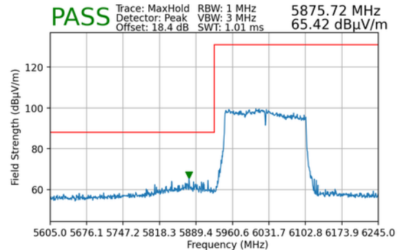
Plot 7-209. Radiated Lower Band Edge Plot MIMO (Peak – UNII Band 5) – LPI & SP
