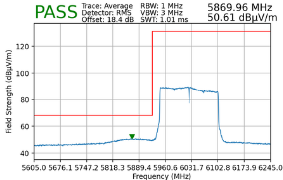
Plot 7-208. Radiated Lower Band Edge Plot MIMO (Average – UNII Band 5) – LPI & SP
