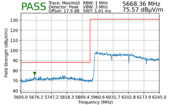
Plot 7-213. Radiated Lower Band Edge Plot MIMO (Peak – UNII Band 5) – LPI & SP
