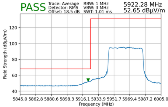
Plot 7-200. Radiated Lower Band Edge Plot MIMO (Average – UNII Band 5) – LPI & SP
