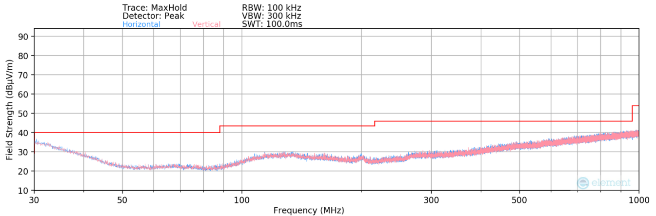
Plot 7-189. Radiated Spurious Plot below 1GHz MIMO (802.11ax) – LPI & SP
