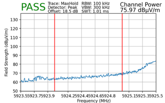
Plot 7-197. Radiated Lower Band Edge Plot MIMO (Peak – UNII Band 5) – LPI & SP
