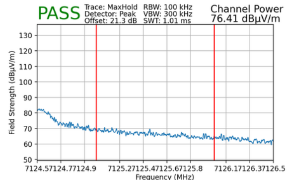
Plot 7-199. Radiated Upper Band Edge Plot MIMO (Peak – UNII Band 8) - LPI
