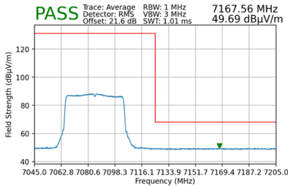
Plot 7-202. Radiated Upper Band Edge Plot MIMO (Average – UNII Band 8) - LPI
