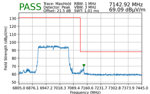
Plot 7-211. Radiated Upper Band Edge Plot MIMO (Peak – UNII Band 8) - LPI
