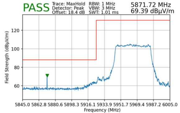
Plot 7-201. Radiated Lower Band Edge Plot MIMO (Peak – UNII Band 5) – LPI & SP
