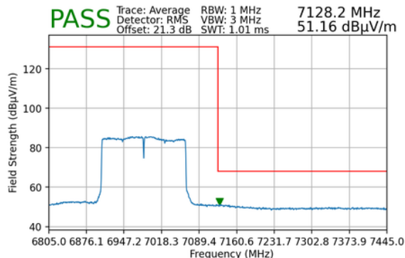
Plot 7-210. Radiated Upper Band Edge Plot MIMO (Average – UNII Band 8) - LPI
