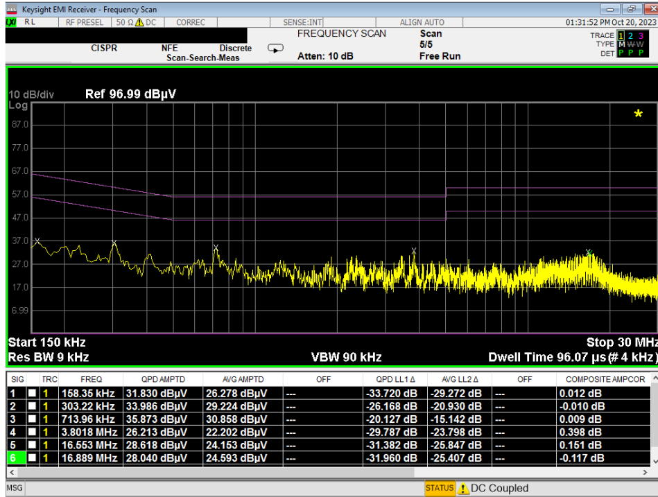
Plot 7-224. Line Conducted Plot with 802.11a UNII Band 5 (L1) with WCP
