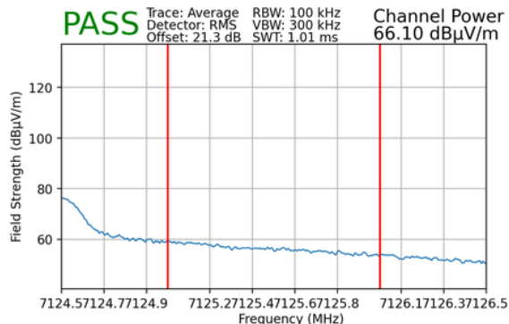
Plot 7-198. Radiated Upper Band Edge Plot MIMO (Average – UNII Band 8) - LPI
