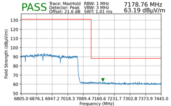
Plot 7-215. Radiated Upper Band Edge Plot MIMO (Peak – UNII Band 8) - LPI
