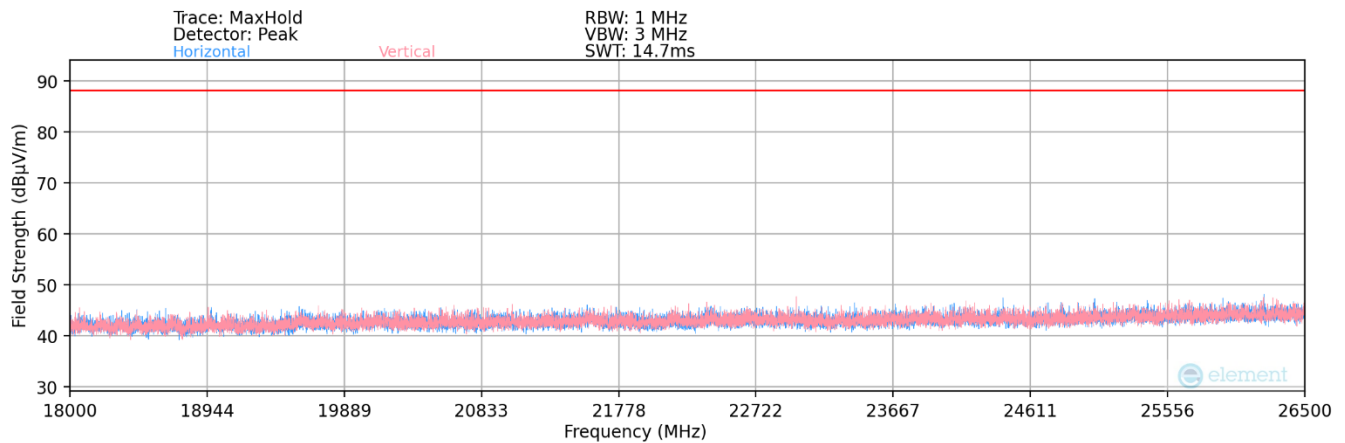
Plot 7-194. Radiated Spurious Plot 18GHz - 26.5GHz (802.11ax) – LPI & SP
