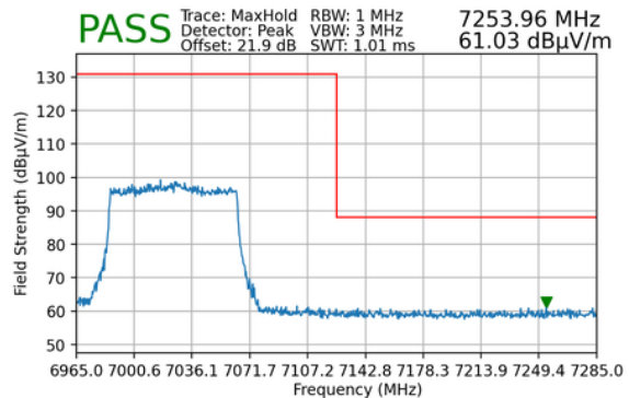
Plot 7-207. Radiated Upper Band Edge Plot MIMO (Peak – UNII Band 8) - LPI
