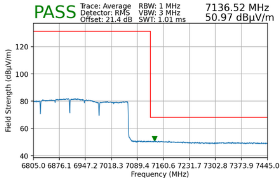
Plot 7-214. Radiated Upper Band Edge Plot MIMO (Average – UNII Band 8) - LPI
