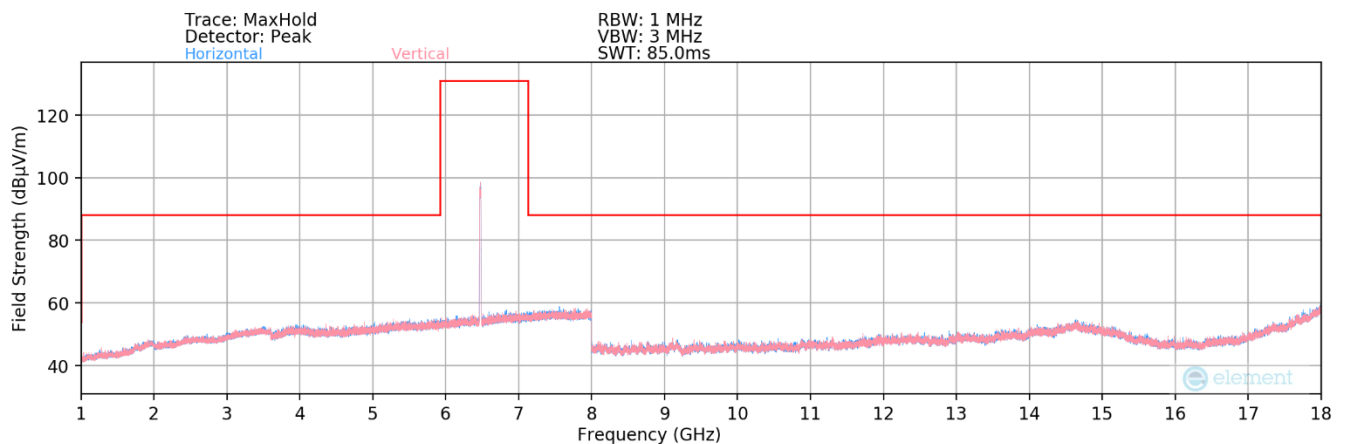
Plot 7-191. Radiated Spurious Plot 1GHz – 18GHz MIMO (802.11ax – UNII Band 6 Ch. 105) - LPI
