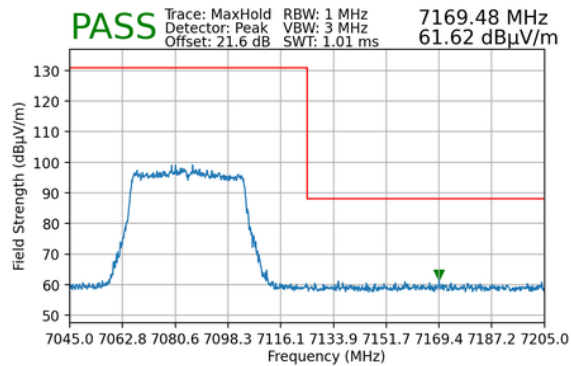
Plot 7-203. Radiated Upper Band Edge Plot MIMO (Peak – UNII Band 8) - LPI
