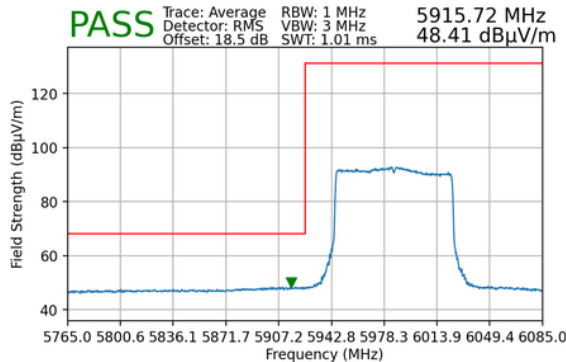
Plot 7-204. Radiated Lower Band Edge Plot MIMO (Average – UNII Band 5) – LPI & SP
