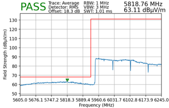
Plot 7-212. Radiated Lower Band Edge Plot MIMO (Average – UNII Band 5) – LPI & SP
