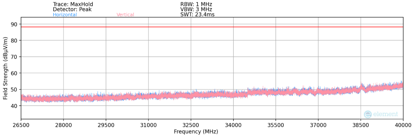
Plot 7-195. Radiated Spurious Plot 26.5GHz - 40GHz (802.11ax) – LPI & SP
