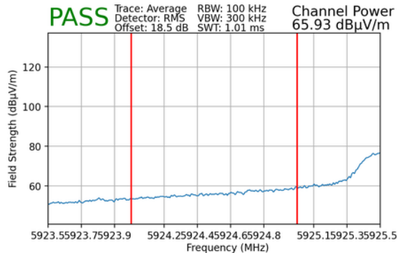
Plot 7-196. Radiated Lower Band Edge Plot MIMO (Average – UNII Band 5) – LPI & SP
