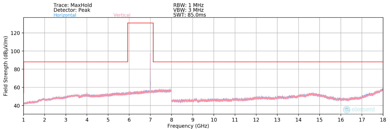
Plot 7-193. Radiated Spurious Plot 1GHz – 18GHz MIMO (802.11ax – UNII Band 8 Ch. 209) - LPI
