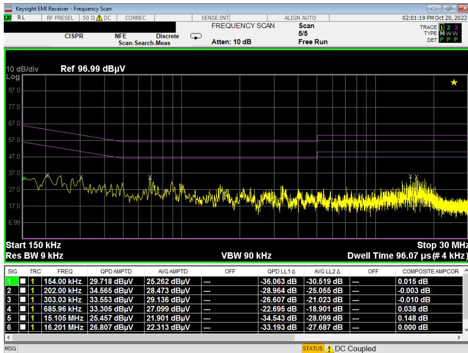
Plot 7-225. Line Conducted Plot with 802.11a UNII Band 5 (N) with WCP
