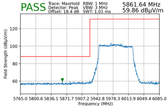
Plot 7-205. Radiated Lower Band Edge Plot MIMO (Peak – UNII Band 5) – LPI & SP
