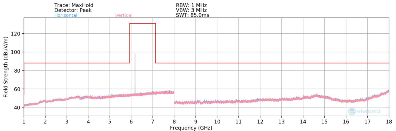
Plot 7-190. Radiated Spurious Plot 1GHz – 18GHz MIMO (802.11ax – UNII Band 5 Ch. 45) – LPI & SP
