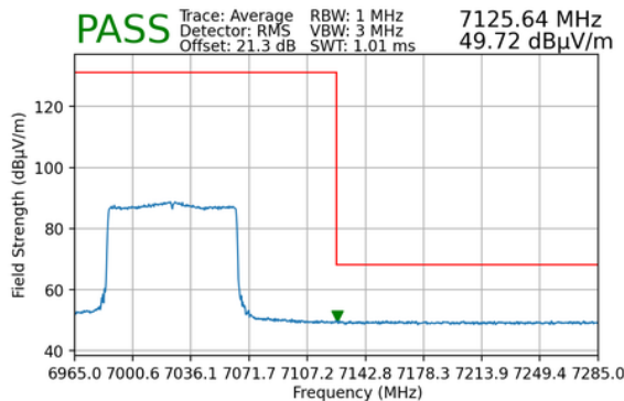
Plot 7-206. Radiated Upper Band Edge Plot MIMO (Average – UNII Band 8) - LPI
