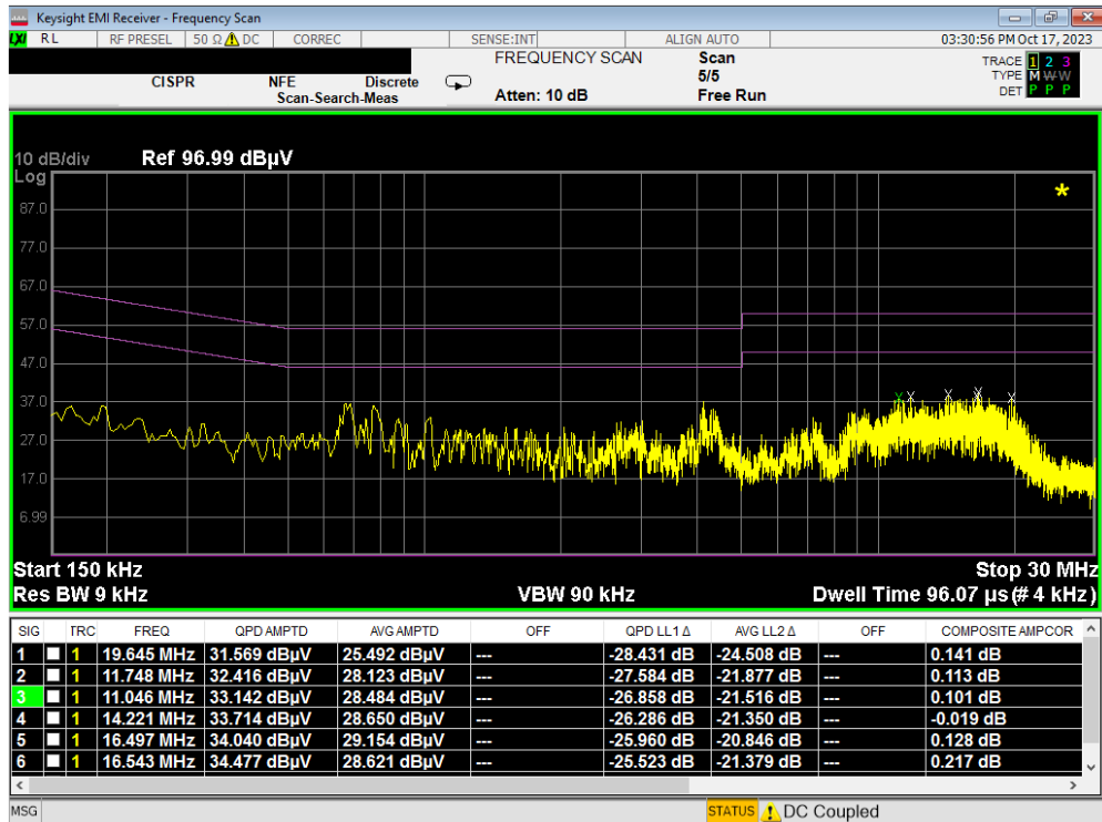
Plot 7-22. Line-Conducted Test Plot (N) – Digitizer (Hover)
