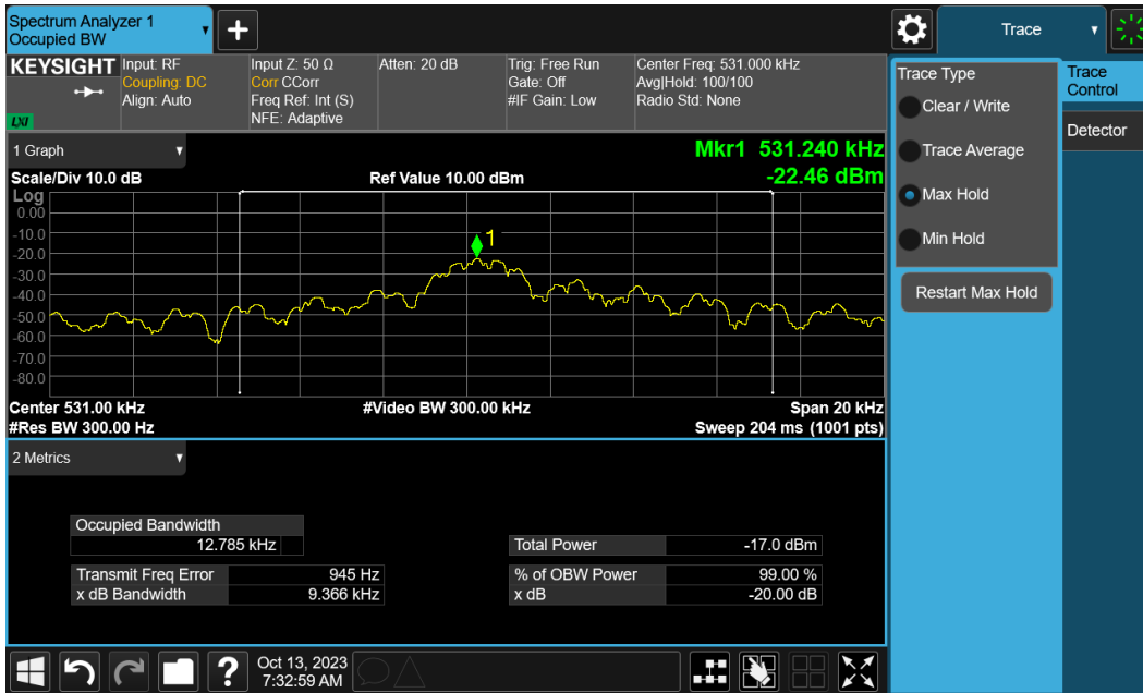
Plot 7-4. Occupied Bandwidth Measurement _ Click
