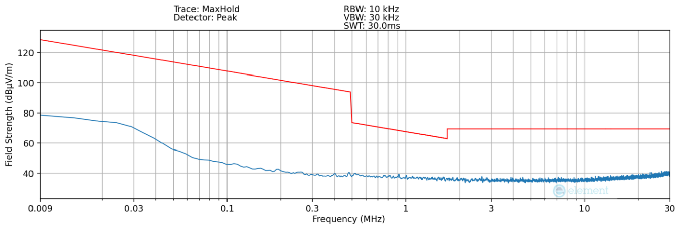
Plot 7-15 Radiated Spurious Plot 9kHz – 30MHz (Pol. Y – Digitizer – Click)
