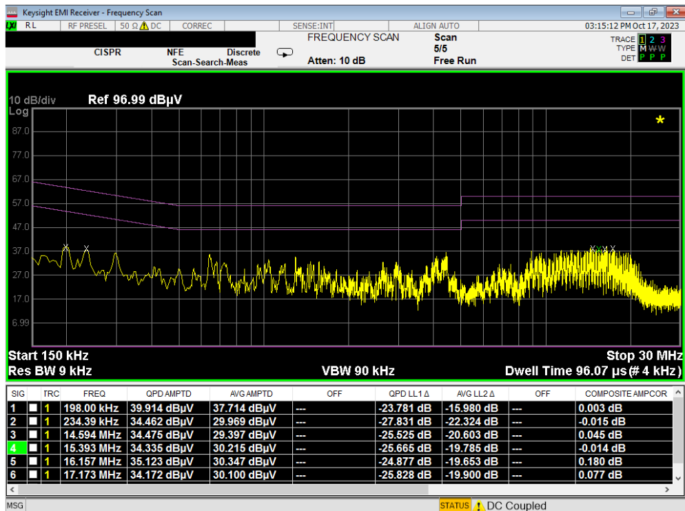
Plot 7-20. Line-Conducted Test Plot (N) - Device to Pen
