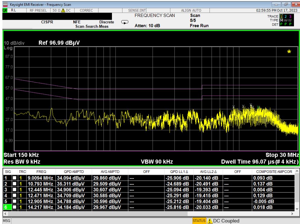
Plot 7-19. Line-Conducted Test Plot (L1) - Device to Pen
