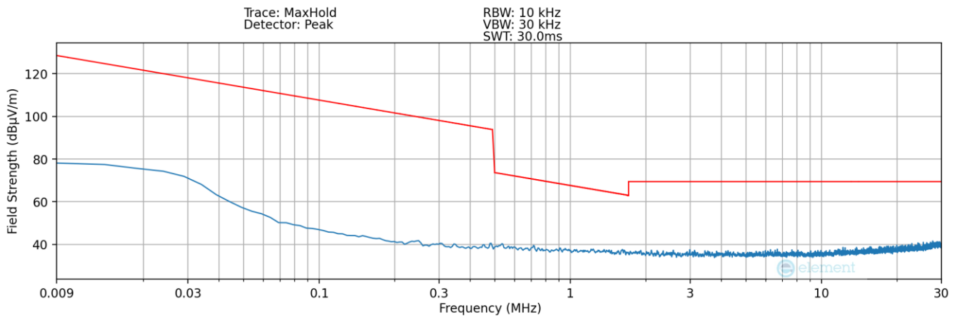
Plot 7-16. Radiated Spurious Plot 9kHz – 30MHz (Pol. Z – Digitizer – Click)
