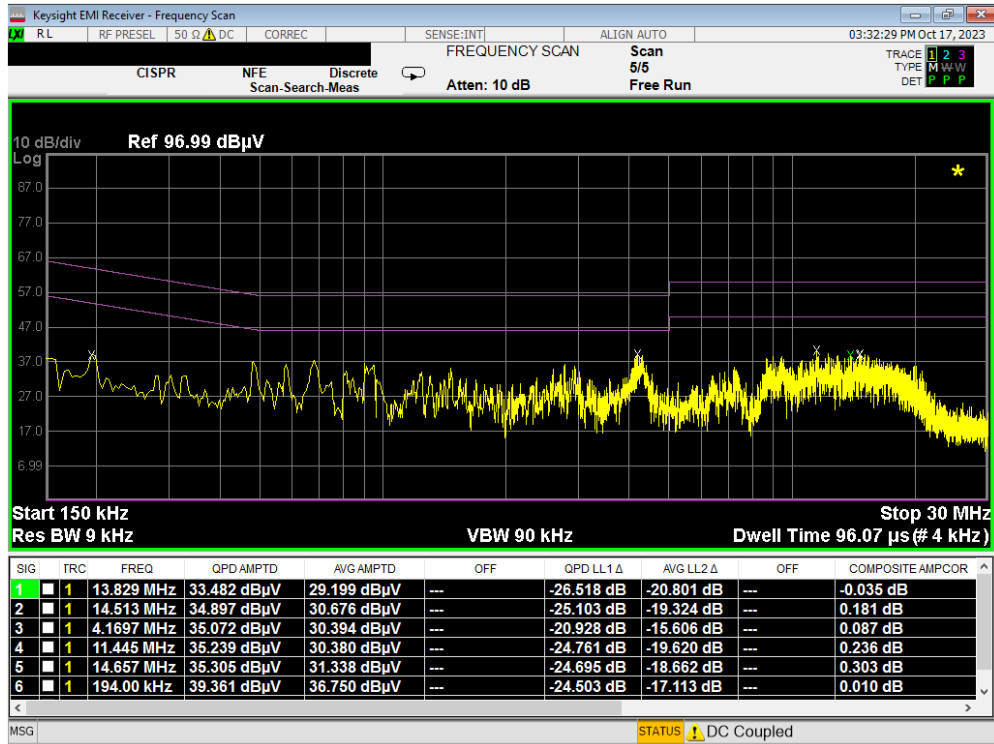
Plot 7-21. Line-Conducted Test Plot (L1) – Digitizer (Hover)
