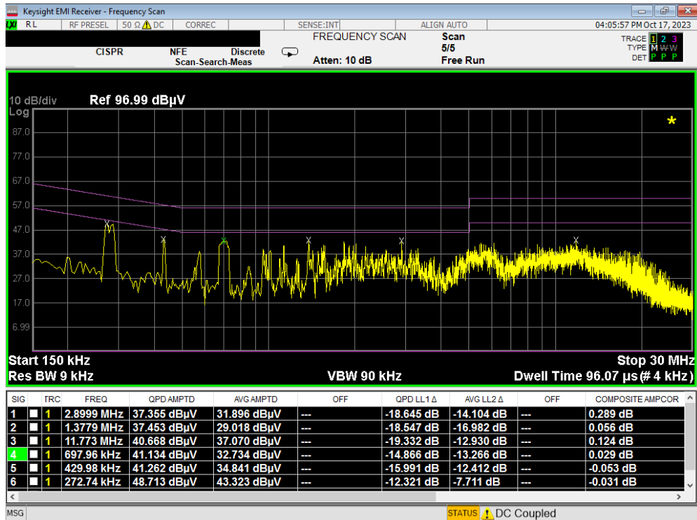
Plot 7-18. Line-Conducted Test Plot (N) - Device to Device
