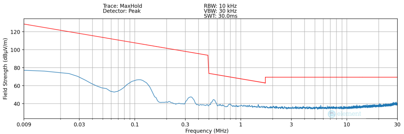
Plot 7-6 Radiated Spurious Plot 9kHz – 30MHz (Pol. Y – Device to Device WPT)
