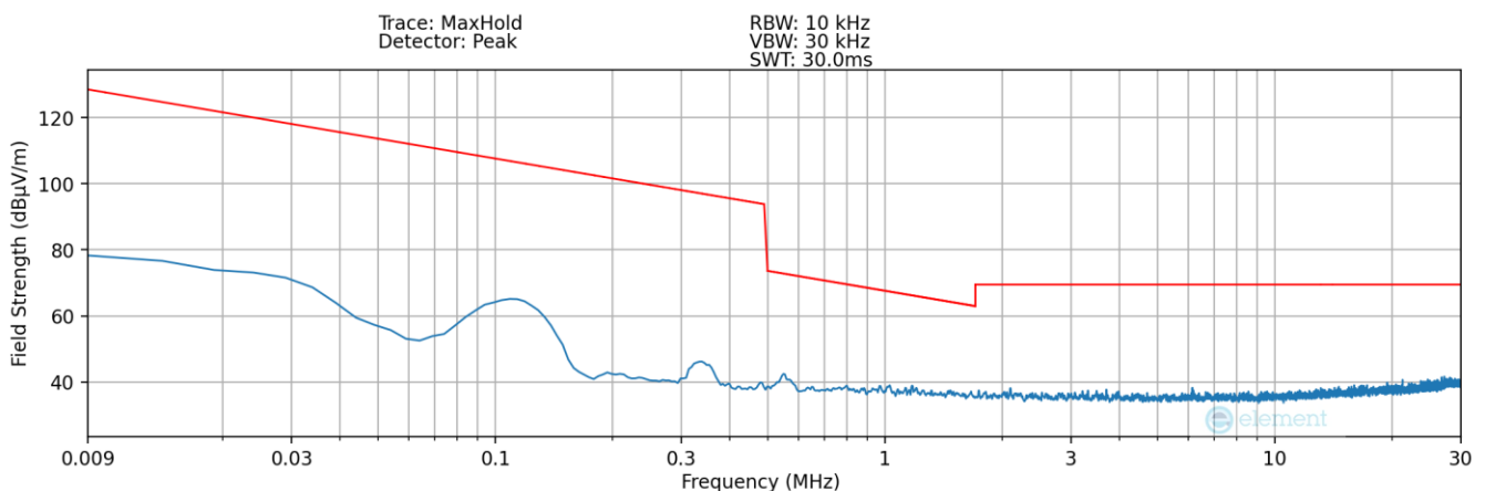
Plot 7-7. Radiated Spurious Plot 9kHz – 30MHz (Pol. Z – Device to Device WPT)
