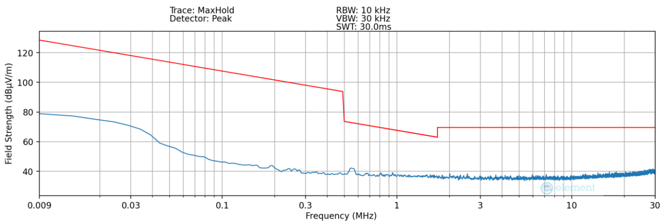
Plot 7-10. Radiated Spurious Plot 9kHz – 30MHz (Pol. Z – Device to Pen WPT)
