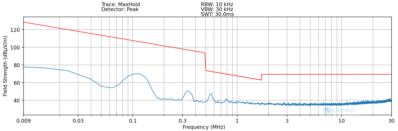
Plot 7-5. Radiated Spurious Plot 9kHz – 30MHz (Pol. X – Device to Device WPT)
