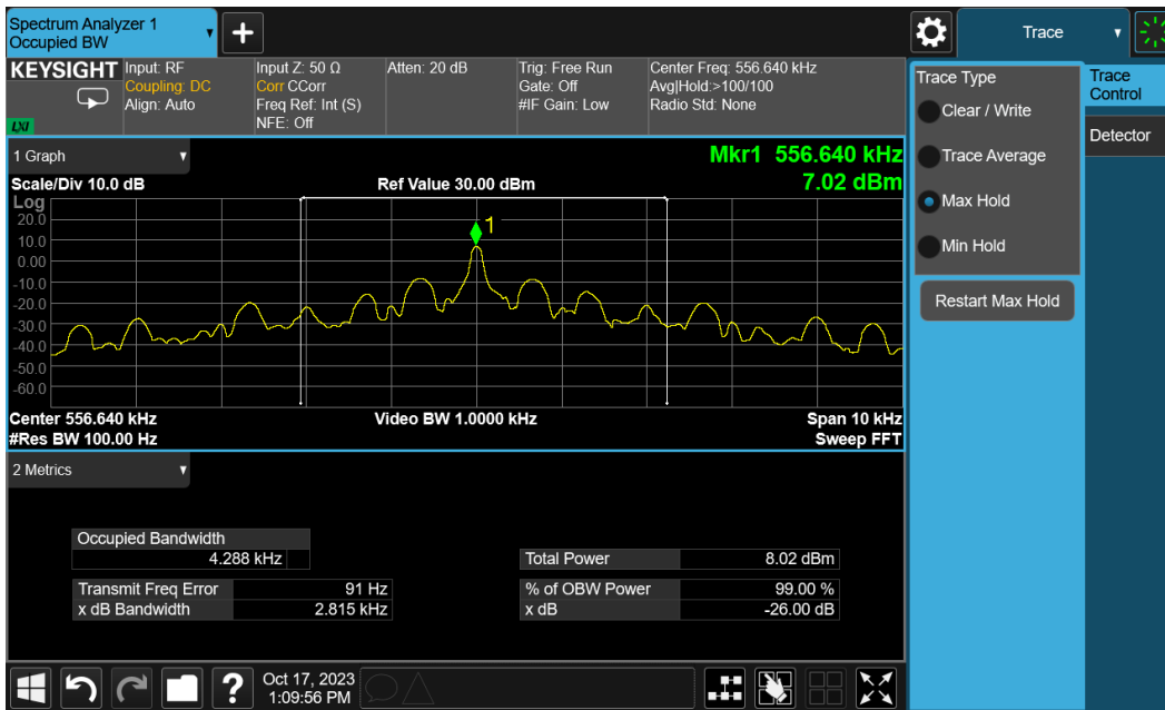
Plot 7-2. Occupied Bandwidth Measurement _ Device to Pen
