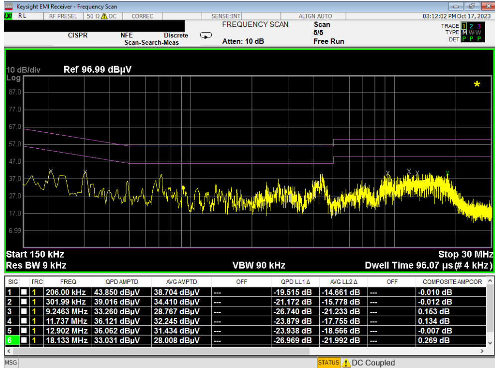
Plot 7-23. Line-Conducted Test Plot (L1) – Digitizer (Click)
