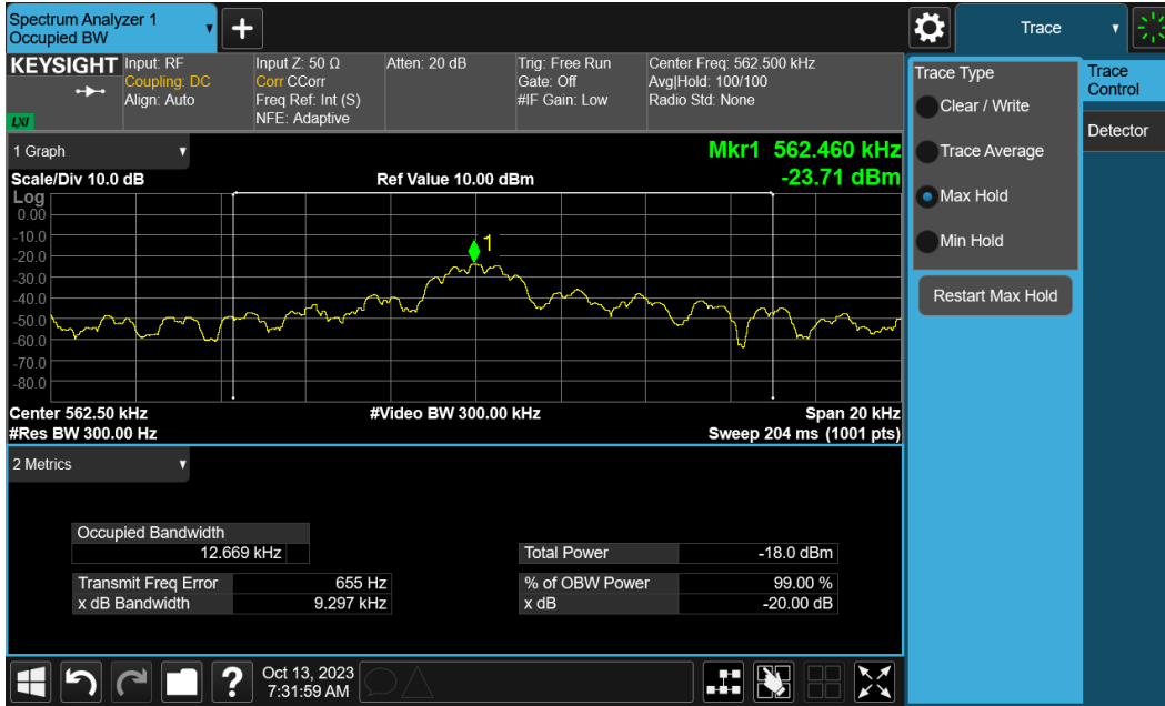
Plot 7-3. Occupied Bandwidth Measurement _ Hover
