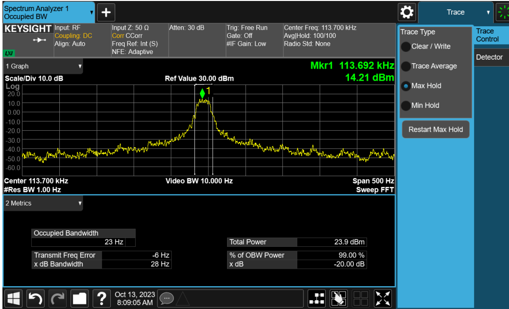
Plot 7-1. Occupied Bandwidth Measurement _ Device to Device
