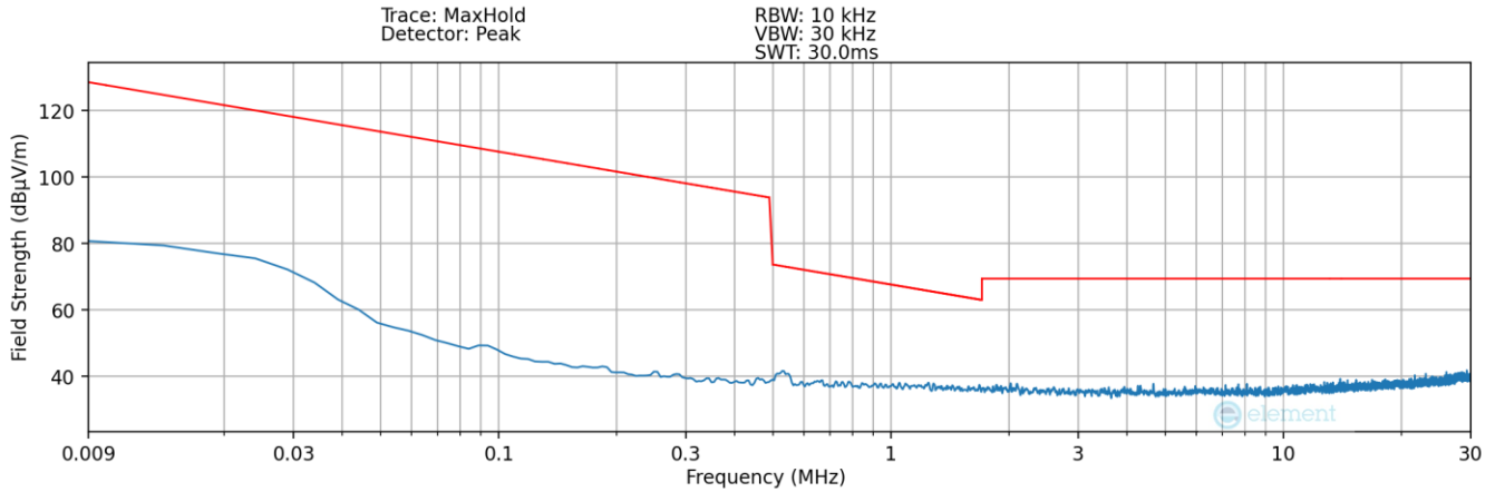
Plot 7-14. Radiated Spurious Plot 9kHz – 30MHz (Pol. X – Digitizer – Click)
