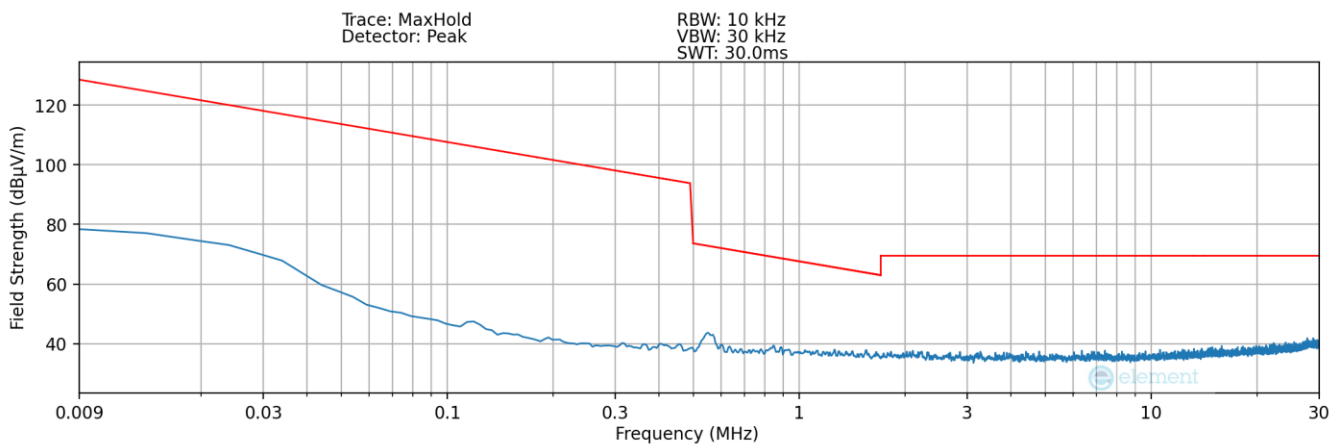
Plot 7-9 Radiated Spurious Plot 9kHz – 30MHz (Pol. Y – Device to Pen WPT)
