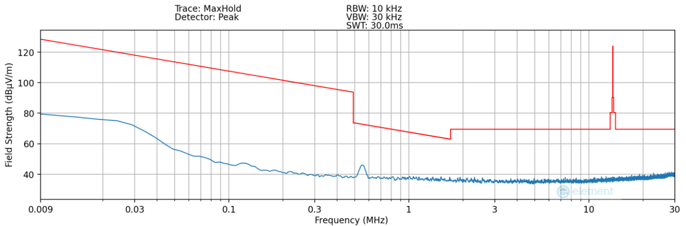
Plot 7-8. Radiated Spurious Plot 9kHz – 30MHz (Pol. X – Device to Pen WPT)
